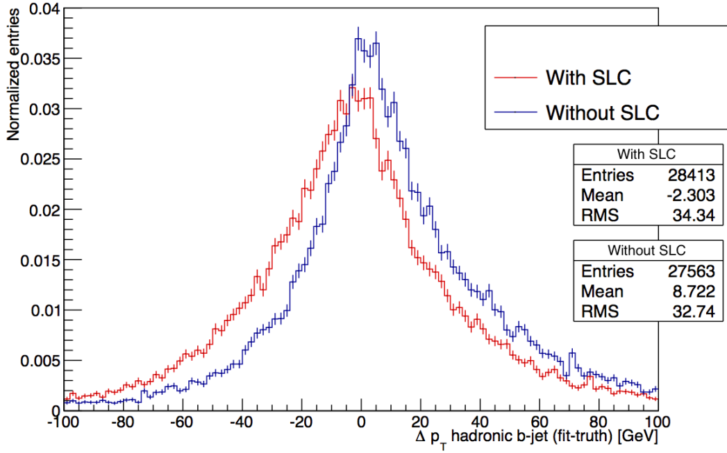
Figure 113.: electron+jets channel, the hadronic side of t\bar{t} decay is shown. Difference between MC truth b -jet p_T (with and without SLC correction) and fitted jet p_T returned by the KLFFitter. The shift of the mean towards zero in the SLC corrections indicates a less strenuous fit performed, and leads to a higher permutation likelihood. The muon+jets distribution is similar.
