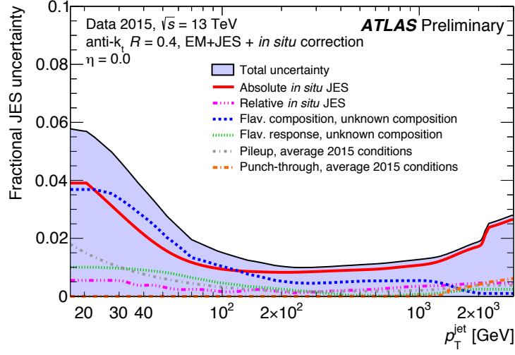
Figure 127.: JES uncertainties, estimated for the 2015 data taking period as a function of jet p_T for jets of \eta = 0 . ([130]).
