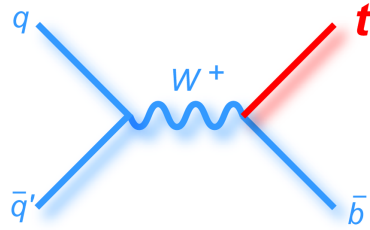
Figure 12.: LO single top production Feynman diagram, s -channel [32].
