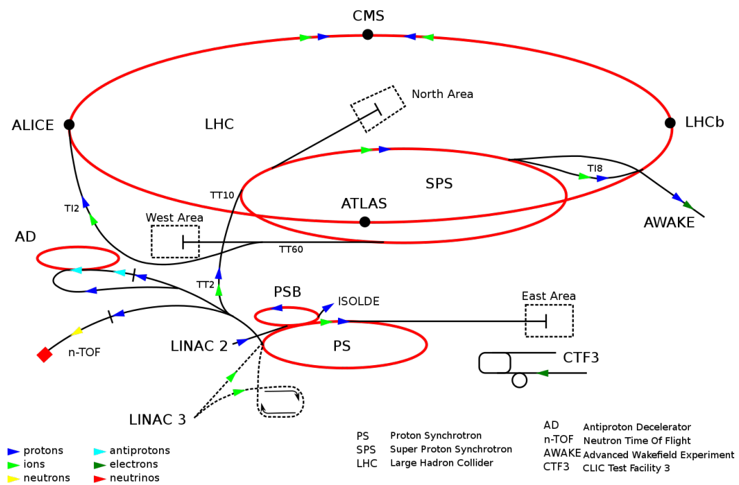
Figure 21.: CERN accelerator facility [48].
