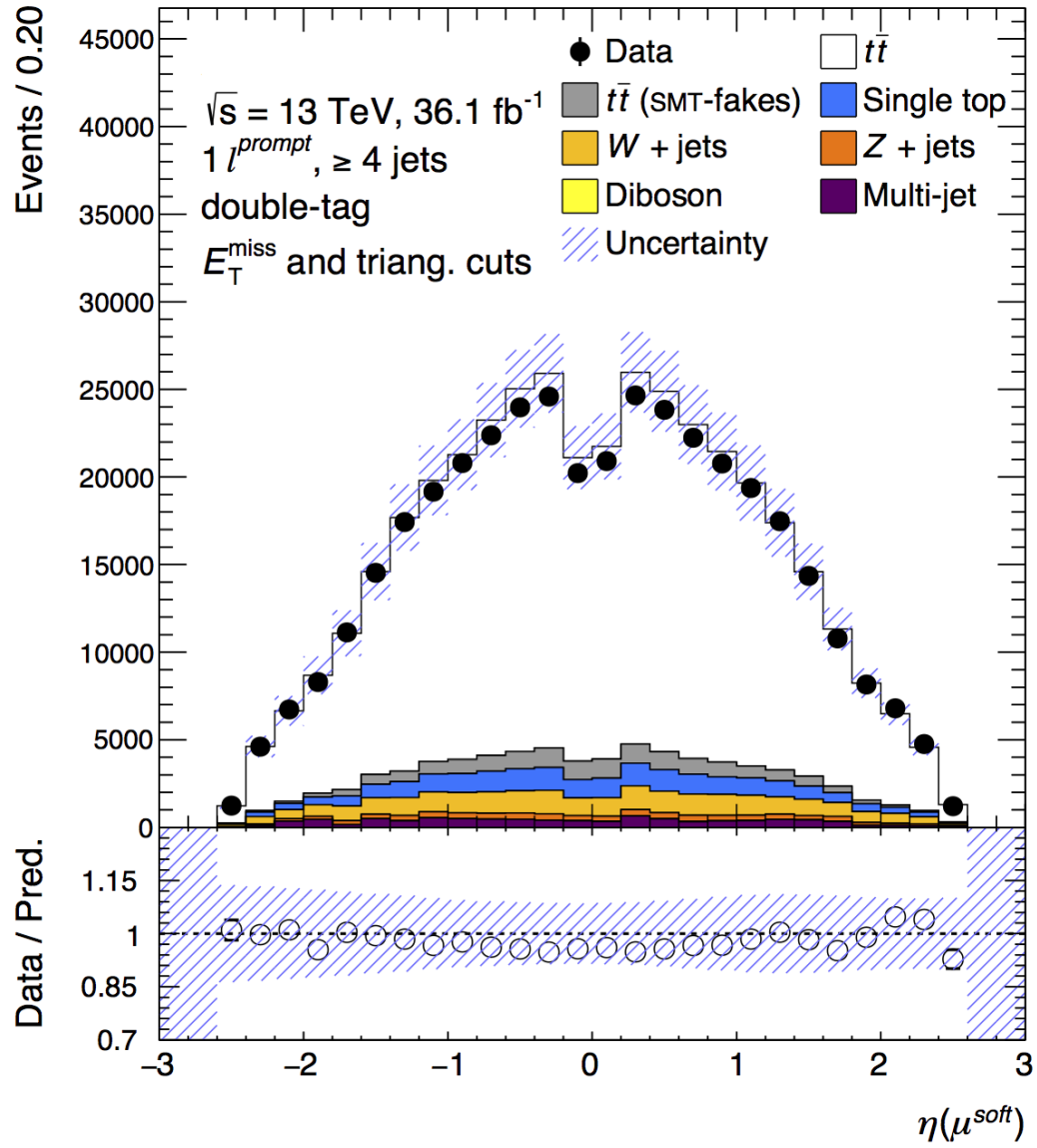
Figure 107.: The soft muon \eta , lepton+jets channel.
