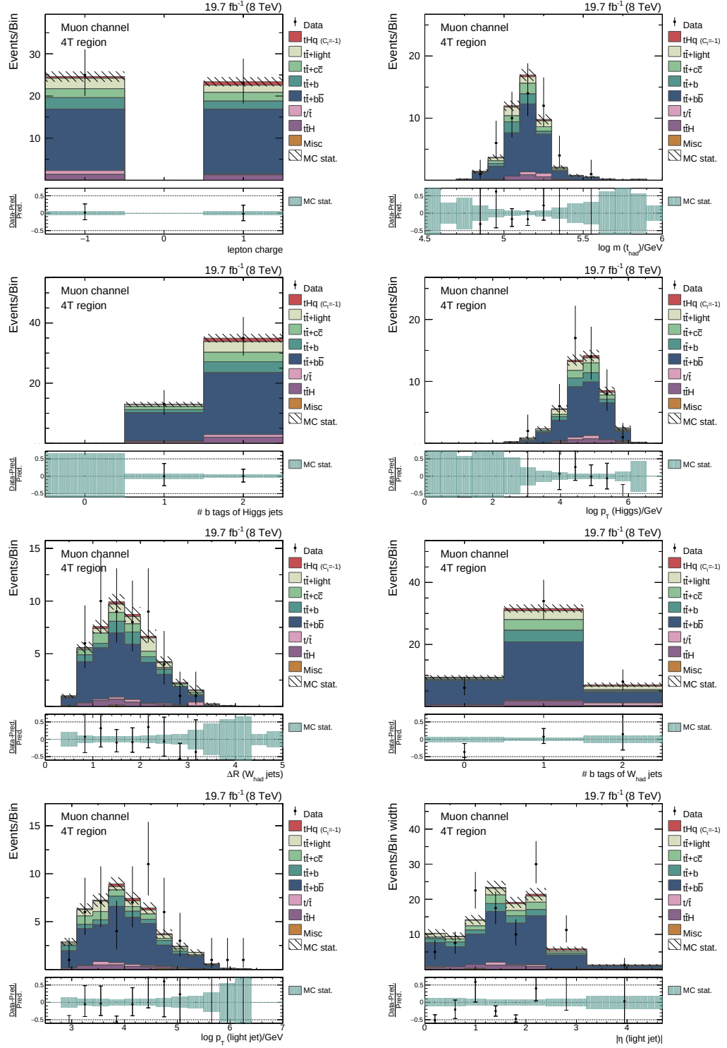
Figure 5.20.: Simulation to data comparisons for the input variables of the classification for the muon channel in the 4T region sorted by their importance in the training. A good agreement of simulation and data is observed. In both diagrams the simulation is scaled to match the event yields observed in data and all simulation corrections are applied.
