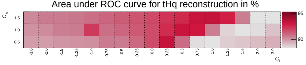
Figure 6.7.: The area under the ROC curve for all 51 tHq reconstruction trainings is shown. With values above 85% good performance is observed for all trainings. A visible ridge on the right side of the plot corresponds to the points with the lowest cross sections. Effectively lower event counts lead to a deterioration of the separation power between correct and wrong assignments.
