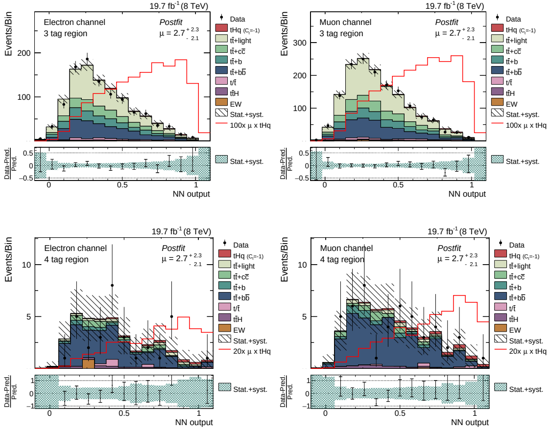
Figure 5.25.: Postfit distributions of the classifier output in both lepton channels and both signal regions. Uncertainty bands include statistical and systematic uncertainties. A good agreement in all four channels is observed, deviations from the prediction are covered by the uncertainties. The signal template is also scaled to its best-fit value of \mu = 2.7 . The corresponding prefit distributions can be found in Appendix A.8.
