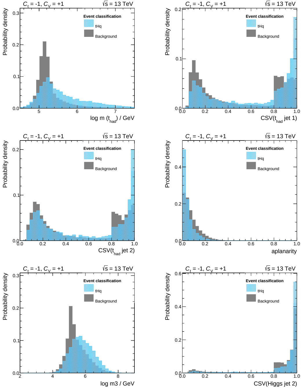
Figure 6.18.: Six of the most important variables used in the final classification sorted by their importance in the training at \sqrt{s} = 13 TeV. All distributions are normalized to unit area. The corresponding variable descriptions can be found in Table 6.6. The remaining variables can be found in Appendix B.6. The third most important variable, the pseudorapidity of the light forward jet, is omitted here, as it is already shown in Figure 6.15.
