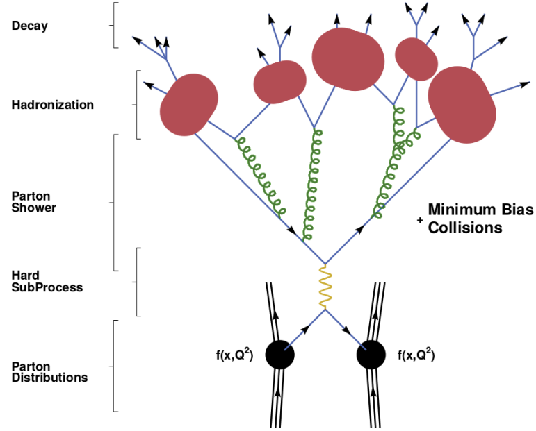
Figure 3.1.: Overview of the event generation process. The diagram shows the different steps of the event generation that can be done sequentially due to the factorization. The parton distribution functions provide the probabilities to colliding partons with a certain fraction of the proton momentum. The hard subprocess describes the actual particle interactions that are the subject of study. During the generation of the hard subprocess the matrix element and therefore the production cross section is calculated. The parton shower is responsible for the generation of gluon radiation. In the hadronization step, all color-charged particles are recombined to form neutral bound states, which subsequently decay in other particles. As last step, the influence of pileup is modeled by overlaying the events with collisions, based on minimum bias collisions. For clarity the underlying event, the influence of the proton remnants, is not depicted in this diagram. Adapted from [64].
