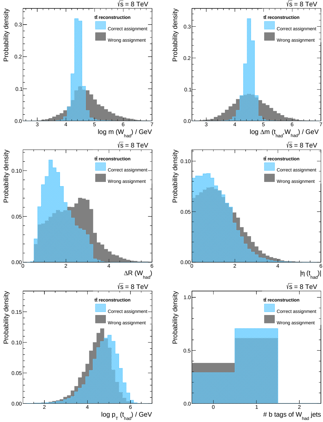
Figure 5.12.: The six most discriminating variables between correct and wrong jet assignments in the t\bar{t} reconstruction are shown sorted by their importance in the training. All distributions are normalized to unit area. The corresponding variable descriptions can be found in Table 5.4. The remaining seven variables can be found in Appendix A.5.
