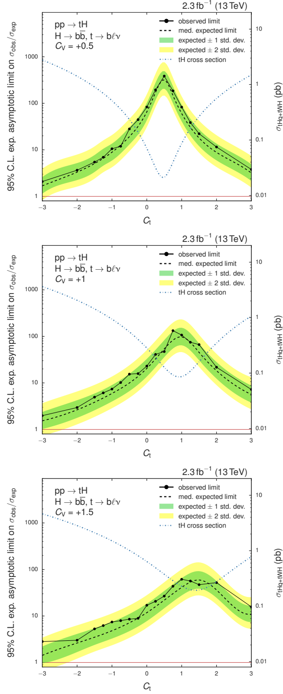
Figure 6.27.: Expected and observed asymptotic CL s limits at 95% C.L. for the combination of 3M and 4M region as a function of C_t . The limits are shown for C_V = +0.5 (top), C_V = +1.0 (center) and C_V = +1.5 (bottom). The sum of the tHq and tHw cross sections as function of C_t is depicted as dotted blue line for each of the three C_V values. Neither an excess nor a strong downward fluctuation is observed. The corresponding limit values for all studied points can be found in the Appendix in Table B.5.
