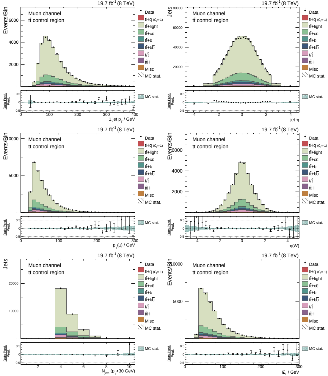
Figure A.1.: A set of control plot in the t\bar{t} control (2T) region in the muon channel is shown. The diagrams show the transverse momentum of the hardest jet of the event, the pseudorapidity of all jets, the transverse momentum of the muon, the pseudorapidity of the reconstructed W boson, the number of jets with a transverse momentum greater than 30 GeV and the missing transverse energy of the event. For all distributions the simulation is scaled to match the observed event yields in data. A good agreement between simulation and data is observed.
