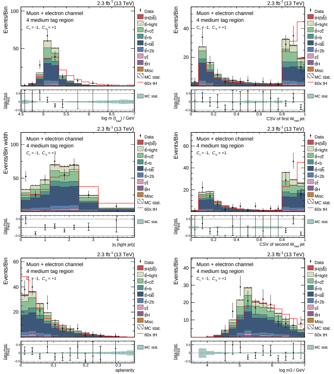
Figure 6.21.: Simulation to data comparisons for the six most important input variables of the classification at \sqrt{s} = 13 TeV. Distributions are sorted by their importance in the training and are shown in the 4M region for the coupling case of C_t = -1 and C_V = +1 . A good agreement of simulation and data is found. In all diagrams the simulation is scaled to match the event yields observed in data and all MC weights are applied. The distributions of the remaining variables of the classification can be found in Appendix B.11 and B.12.
