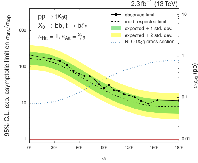
Figure 6.31.: Expected and observed asymptotic CL_s limits at 95% C.L. for the combination of the 3M and 4M region as function of the C\mathcal{P} -mixing angle \alpha . Corresponding numbers for the case of a fully pseudoscalar boson can be found in Table 6.11. The tX_0q cross section as function of \alpha is depicted as dotted blue line. No C\mathcal{P} -mixing angle can be excluded yet, hence only upper limits are set. Neither an excess nor a strong downward fluctuation is observed for any studied angle. The limit values for all mixing angles can be found in the Appendix in Table B.6.
