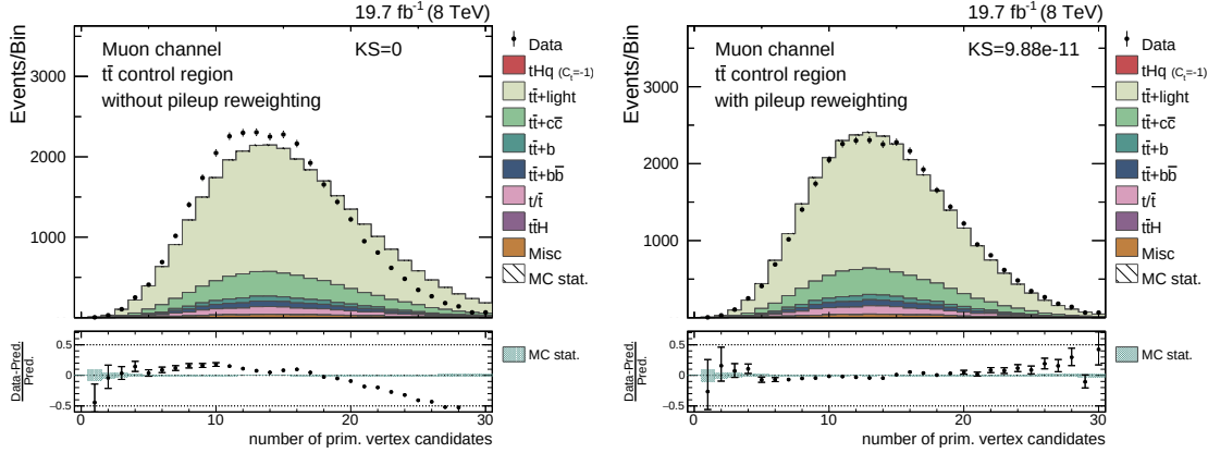
Figure 5.4.: Distribution of the number of primary vertices per event before (left) and after (right) application of the pileup reweighting. The simulation predicts more primary vertices than are observed in data. For both distributions the simulation is scaled to match the observed event numbers. After the reweighting a good agreement of simulation and recorded events is observed.
