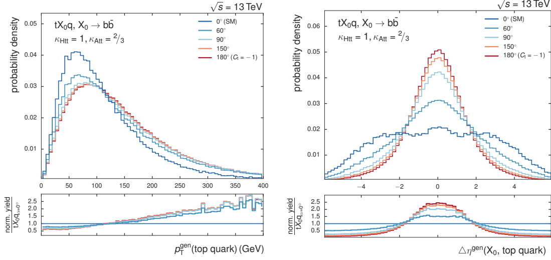
Figure 1.5.: Distributions of the transverse momentum of the top quark and the difference of the pseudo-rapidity of top quark and Higgs boson in the tHq process for different CP -mixing angles.
