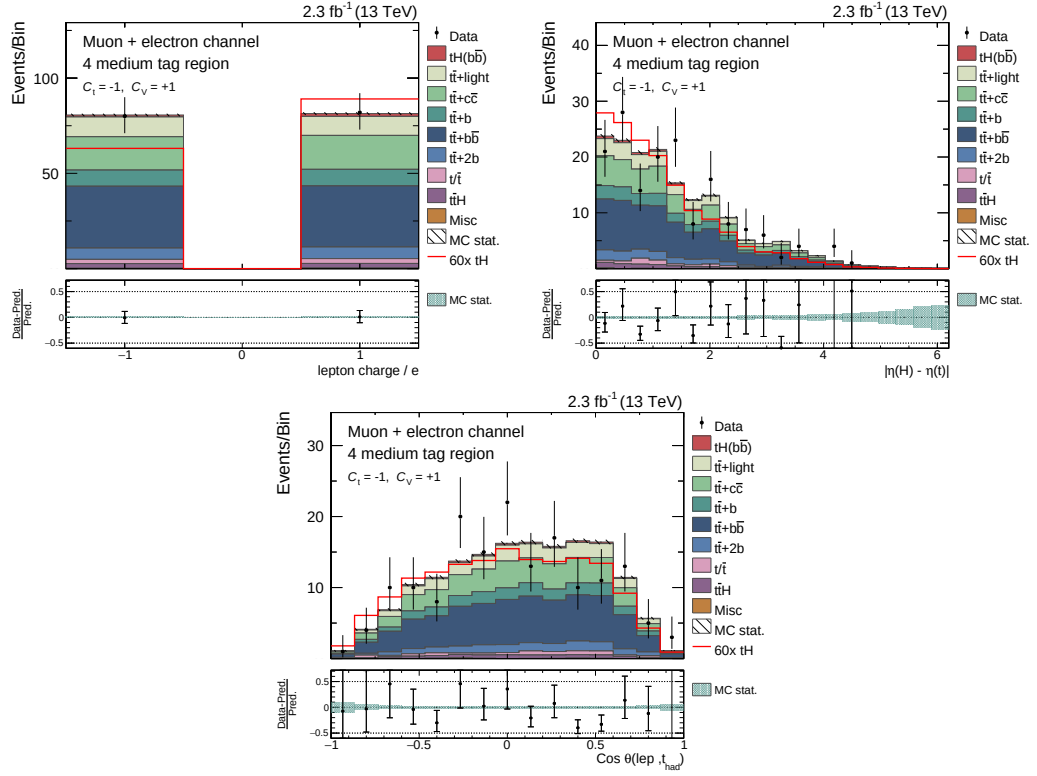
Figure B.12.: Simulation to data comparisons for input variables of the classification ranked 13 th to 15 th at \sqrt{s} = 13 TeV. Distributions are sorted by their importance in the training and are shown in the 4M region for the coupling case of C_t = -1 and C_V = 1 . A good agreement of simulation and data is found. In both diagrams the simulation is scaled to match the event yields observed in data and all MC weights are applied.
