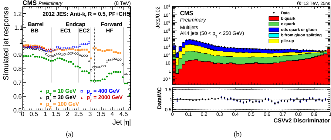
Figure 3.7.: In diagram (a) the simulated detector response in the different detector regions can be seen at \sqrt{s} = 8 TeV. Especially in the forward region, like the HF, and for low- p_T jets the detector shows a lower response, which is mostly corrected in the L2L3 corrections. In diagram (b) the distribution of the CSVv2 discriminator at \sqrt{s} = 13 TeV can be seen. The higher the values of the discriminator the higher the probability for a jet to be stemming from a b quark and the lower the mistagging efficiency. Tested with a multijet sample, the discriminator shows good agreement. The plots are taken from [109] and [114], respectively.
