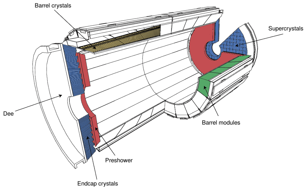
Figure 2.5.: A three-dimensional overview of the CMS ECAL. The central barrel section contains 36 supermodules (green) with each supermodule containing 1700 crystals each (yellow). The barrel endcap region contains four dees with 3662 crystals each (blue). The preshower detectors (red) are located on each side in front of the dees. The original diagram is taken from [48].
