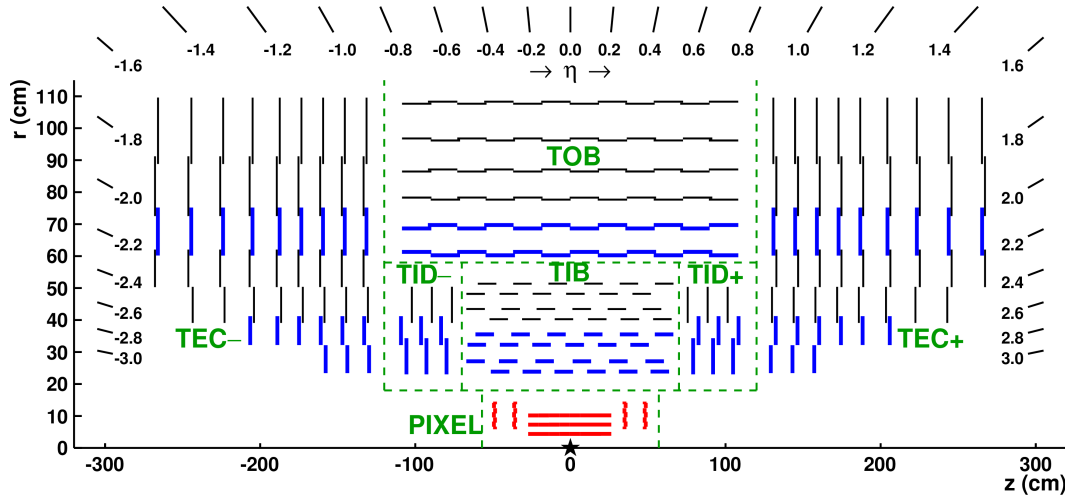
Figure 2.4.: Overview of the CMS tracking system taken from [60]. The pixel tracker (PIXEL) is shown in red surrounding the interaction point (star). The Tracker Inner Barrel (TIB) and Disks (TID) occupy the space r < 55 cm and |z| < 118 cm. The barrel consists of four layers of silicon strip modules in the TIB and the three layers in each disk. These modules achieve a position resolution in r-\phi of 13 - 38 \mu\text{m} . The Tracker Outer Barrel (TOB) covers r > 55 cm and |z| < 118 cm and incorporates six modules. Its position measurement resolution is approximately 18 - 47 \mu\text{m} . The Tracker Endcaps (TEC) cover the region 124 < |z| < 282 cm. Each of the endcaps consists of nine disks with seven concentric rings of silicon strip modules per disk. A similar resolution as in the TOB is reached. The blue lines show the location of the stereo modules.
