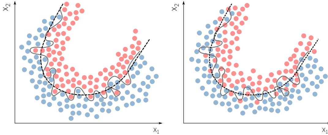
Figure 4.3.: Illustration of the effect of overtraining on an independent testing sample. The distributions show the correlations of variable x_1 and x_2 for two classes of events (red and blue) for a training sample (left) and a testing sample (right). An extremely overtrained method would result in a separation line that perfectly separates the two classes (solid, gray). The application of this separation line to the testing set shows a much worsened performance (right). A robust, non-overtrained MVA would pick a separation line (dashed, black) that performs equally well for training and testing sample.
