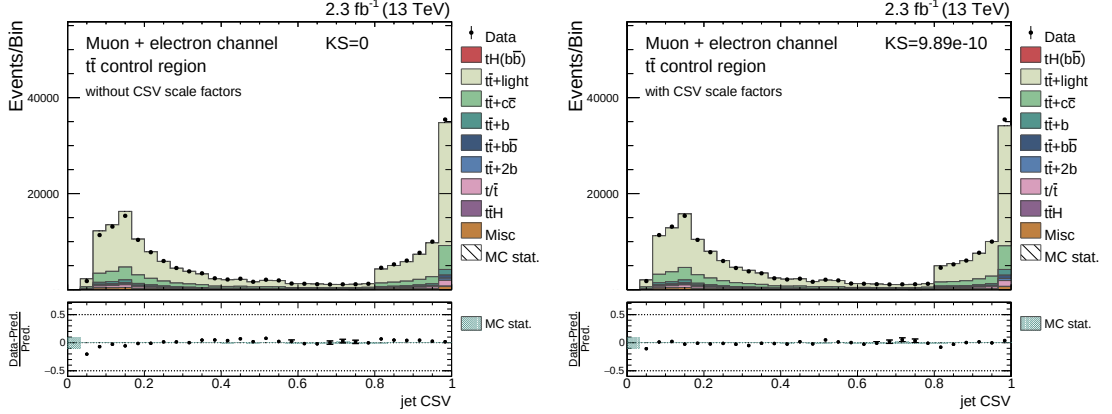
Figure 6.5.: Distribution of the CSV output for all jets per event before (left) and after (right) application of the CSV reweighting. For both distributions the simulation is scaled to match the observed event yields in data. After the reweighting an improved agreement of simulation to recorded events is observed.
