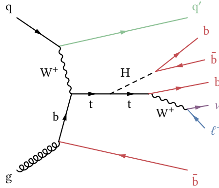
Figure 5.2.: Relevant Feynman diagram of tHq production mechanisms. The diagram shows the case, where the Higgs boson is emitted by the single top quark in the event. The Feynman diagram where the Higgs boson couples to the W boson (see Section 1.3) is omitted, as the final states are identical. The indistinguishable final state for both production mechanism is characterized by four bottom quarks (red), one charged lepton (blue), one neutrino (violet) and one light quark (green).
