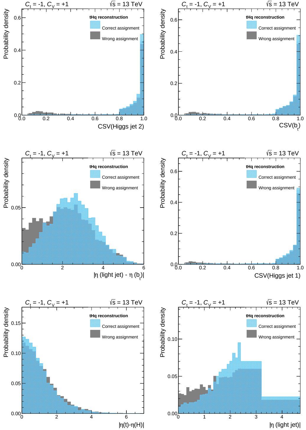
Figure B.1.: Distributions of variables ranked 7 th to 12 th place are shown for correct and wrong jet assignments in the tHq reconstruction. All distributions are normalized to unit area. The corresponding variable descriptions can be found in Table 6.2. The three remaining variables can be found in Appendix B.2.
