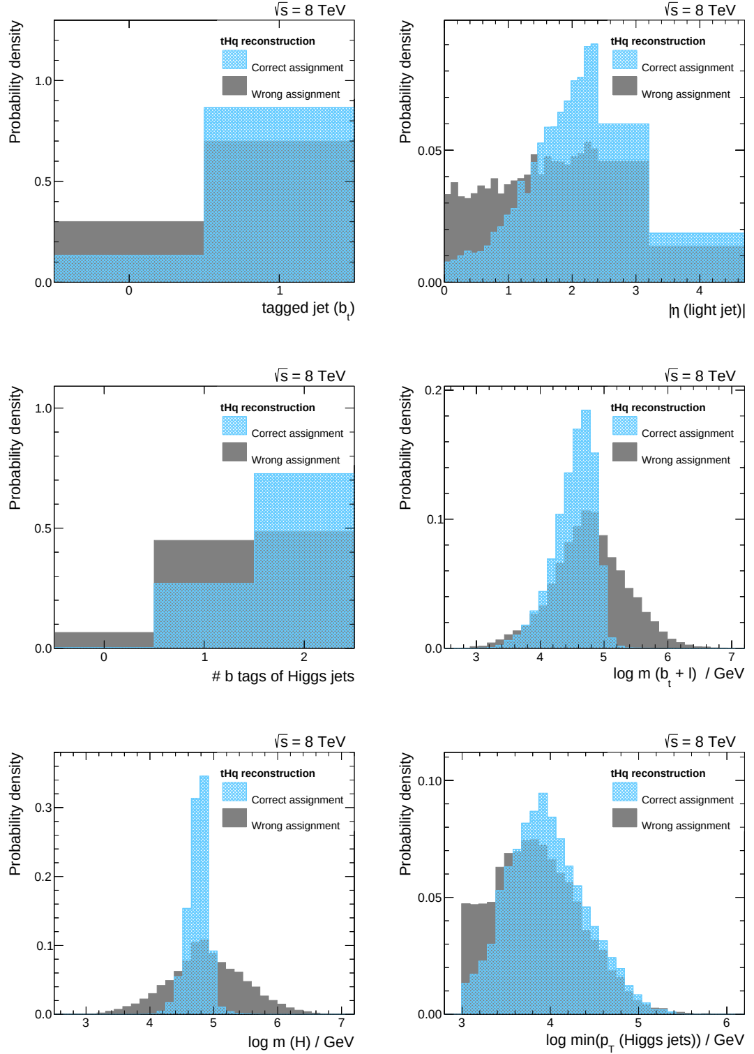
Figure 5.8.: The six most discriminating variables between correct and wrong jet assignments in the tHq reconstruction are shown sorted by their importance in the training. All distributions are normalized to unit area. The corresponding variable descriptions can be found in Table 5.3.
