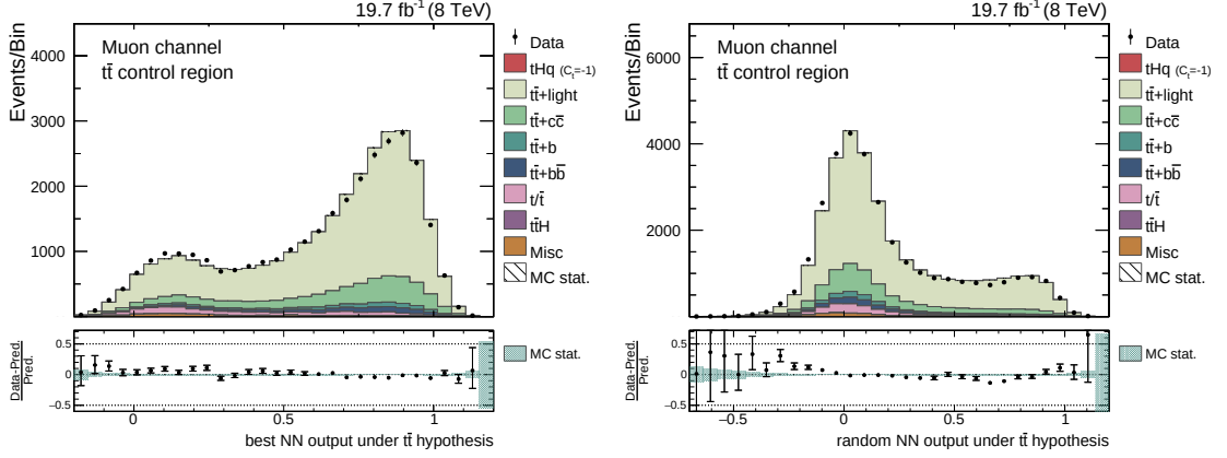
Figure 5.15.: Response of the t\bar{t} reconstruction comparing simulation to data. On the left the highest output value (chosen jet assignment) per event is shown and on the right the NN output value for a random assignment is shown. Both diagrams are shown for the muon channel in the t\bar{t} control region. In both distributions a good agreement between simulation and data is found. In both diagrams the simulation is scaled to match the event yields observed in data and all simulation corrections are applied. The corresponding distributions for the electron channel and 3T and 4T region can be found in Appendix A.6 and A.7.
