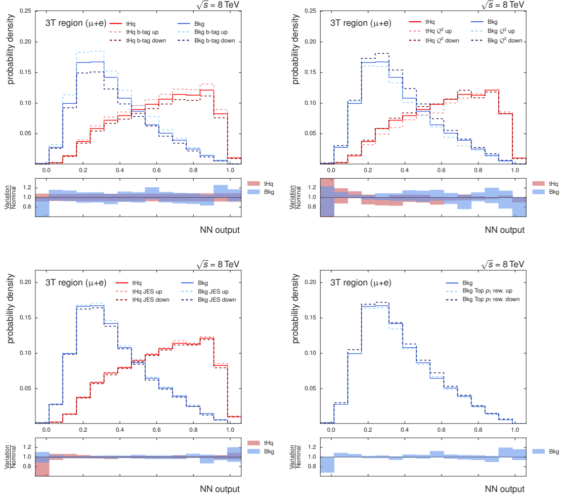
Figure 5.24.: Effect of different systematic shape uncertainties on the final neural network classifier separated into the background shape and signal shape in the 3T region. The diagrams show the effect of the b-tagging efficiency (top left), the Q^2 scale (top right), the combined jet energy scale (bottom left) and top quark p_T reweighting (bottom right) uncertainties. The effect of the 16 independent JES sources is combined by showing the envelope of all systematic variations. The top quark p_T reweighting is only applied for the t\bar{t} background, therefore only the background shape is shown.
