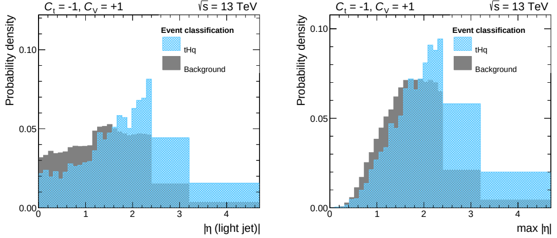
Figure 6.15.: On the left side the distribution of the absolute pseudorapidity of the jet assigned to the light quark by the t\bar{H}q reconstruction is shown. On the right the distributions of the highest absolute pseudorapidity value of all jets in an event is shown. Both distributions are depicted for the signal process and the sum of background processes. The plots are shown for the C_t = -1 and C_V = +1 coupling pair and are normalized to unit area. Both variables show similar separation between signal and background. Although the choice of the most forward jet as light jet is more often correct than the jet chosen by the reconstruction, the variable obtained by the BDT reconstruction has a higher separation power and thus a larger impact in the final classification training.
