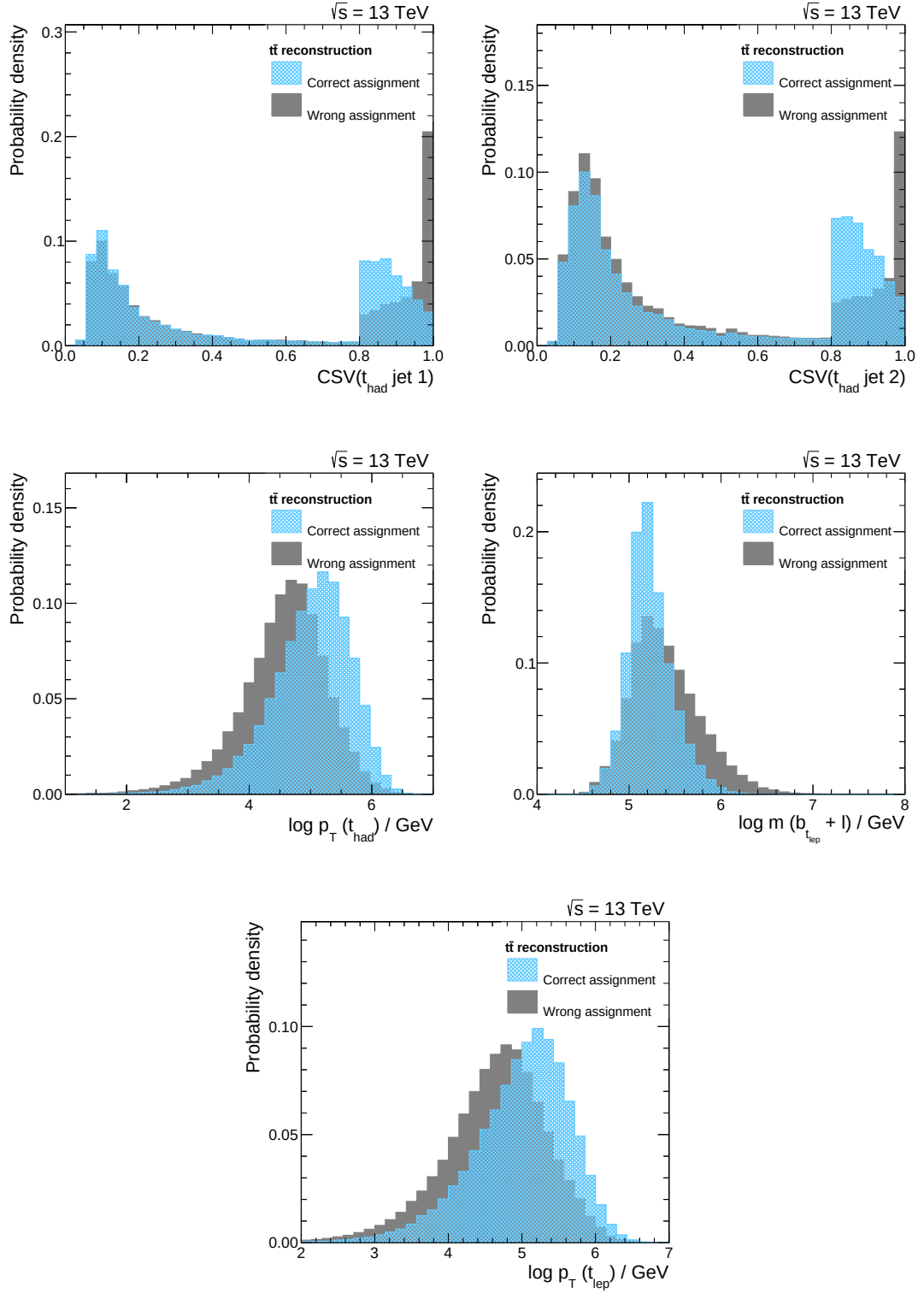
Figure B.3.: The remaining five variables between correct and wrong jet assignments in the t\bar{t} reconstruction are shown sorted by their importance in the training. All distributions are normalized to unit area. The corresponding variable descriptions can be found in Table 6.4.
