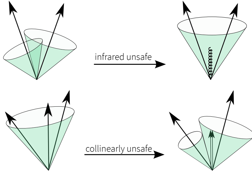
Figure 3.3.: A depiction of infrared (top) and collinear (bottom) safety violations. As shown on the top an additional radiation is able to change the outcome of an infrared unsafe jet clustering algorithm. The diagram on the bottom presents how a collinear splitting can alter the jet clustering, if collinear safety is not provided. Both safety requirements are satisfied by the employed anti- k_t algorithm.
