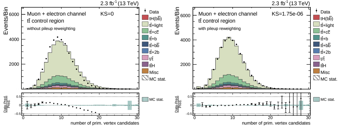
Figure 6.4.: Distribution of the number of primary vertices per event before (left) and after (right) application of the pileup reweighting. The simulation predicted slightly more primary vertices than are observed in data. For both distributions the simulation is scaled to match the observed event numbers in data. After the reweighting a good agreement of simulation to recorded events is observed.
