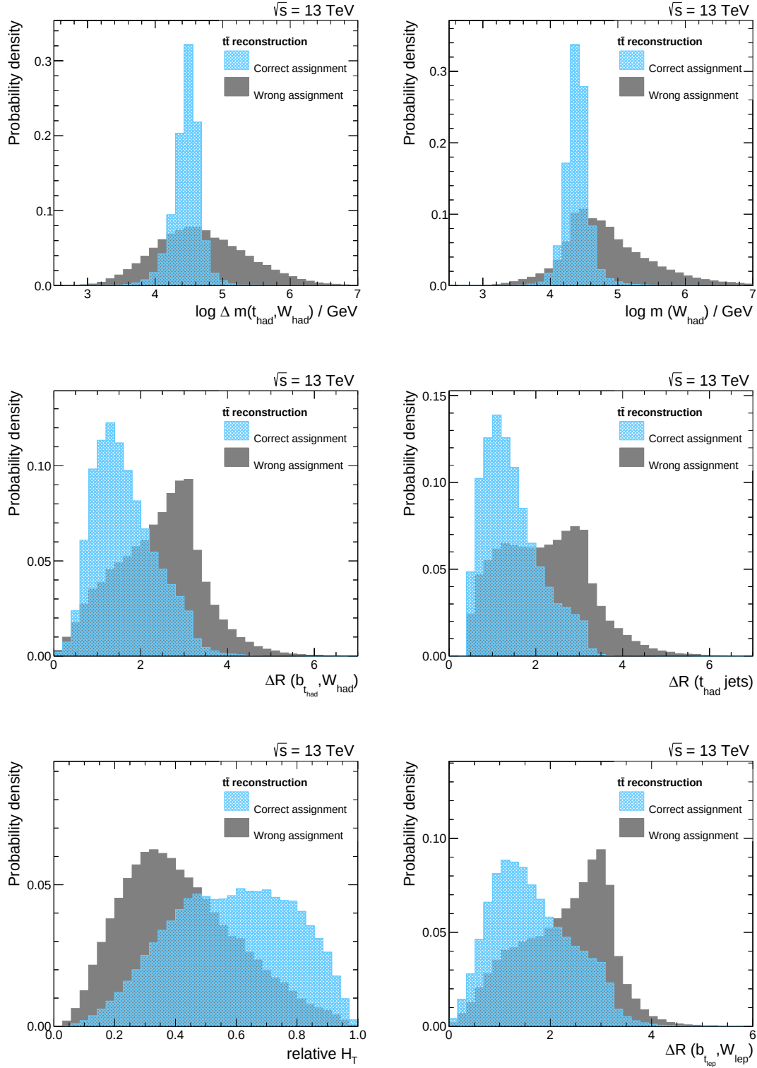
Figure 6.11.: The six most discriminating variables between correct and wrong jet assignments in the t\bar{t} reconstruction at \sqrt{s} = 13 TeV are shown sorted by their importance in the training. All distributions are normalized to unit area. The corresponding variable descriptions can be found in Table 6.4. The remaining variables can be found in Appendix B.3.
