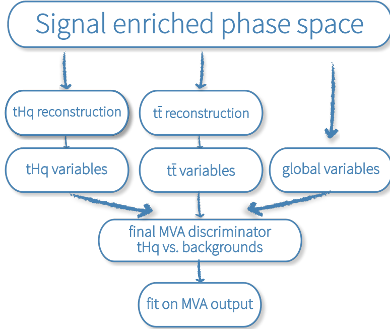
Figure 5.1.: A schematic overview of the analysis workflow. A set of optimized selection cuts ensures a favorable signal to background ratio and puts the analysis in a signal enriched phase space. The final classification uses variables out of three categories: variables based on tHq reconstruction, where jets in the event are assigned to quarks of the tHq final state, variables based on the t\bar{t} reconstruction, where jets are assigned to the quarks in the final state of a semi-leptonic t\bar{t} event and variables that are based on neither. These variables are used in a multivariate method which classifies events to be either more signal- or background-like. The final limit is then derived by performing a likelihood fit in the neural network output distribution and calculating CL_s limits.
