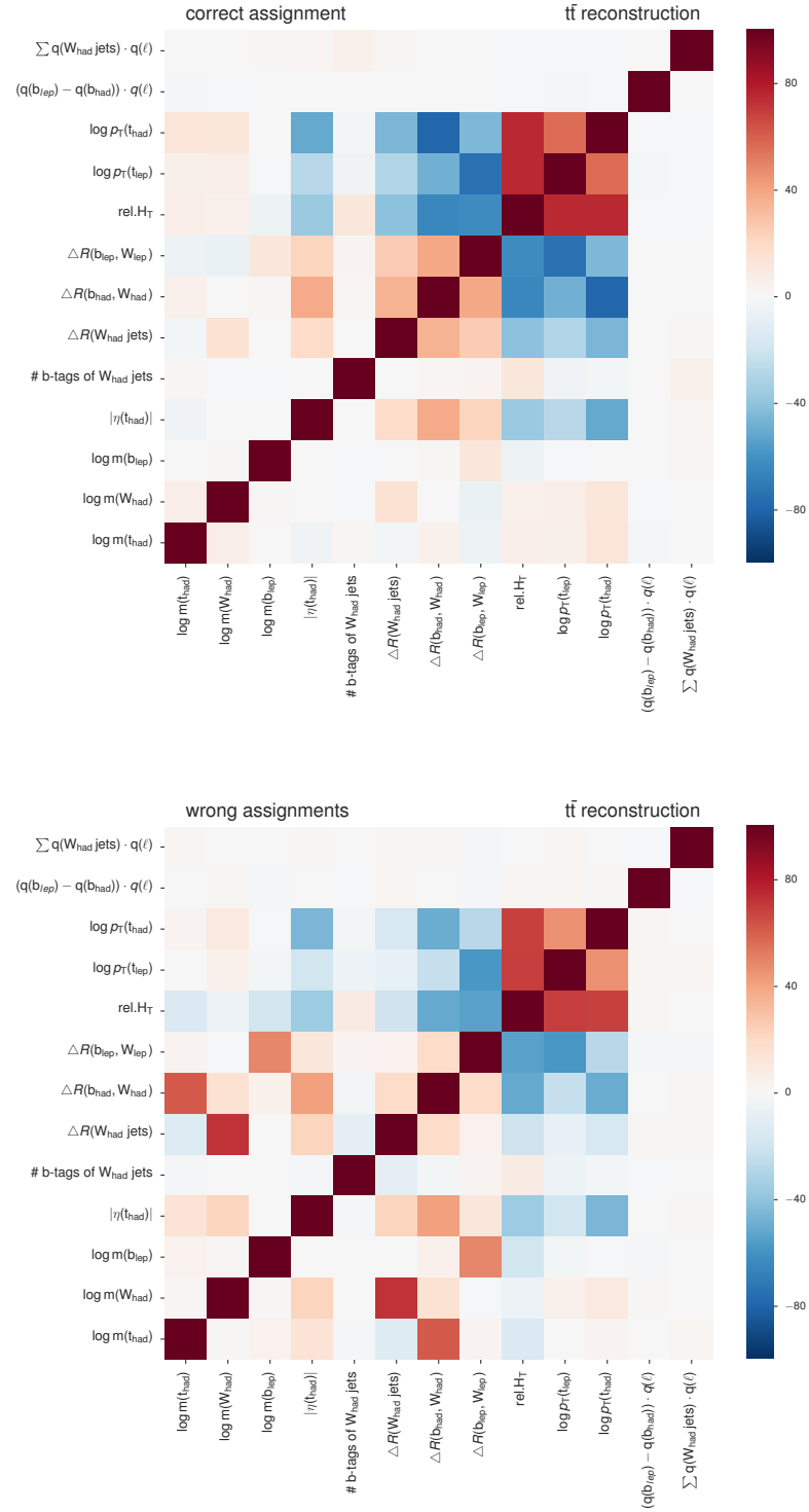
Figure 5.13.: Correlations between the variables used in the t\bar{t} reconstruction for correct and wrong jet assignments. It is visible that stronger (anti-)correlations are apparent between variables for correct assignments than are for wrong assignments. Additionally, correlations are observed in wrong assignments that would be almost uncorrelated for correct assignments, such as the correlation between \Delta R of b quark and W boson and the invariant mass of the reconstructed hadronically decaying top quark.
