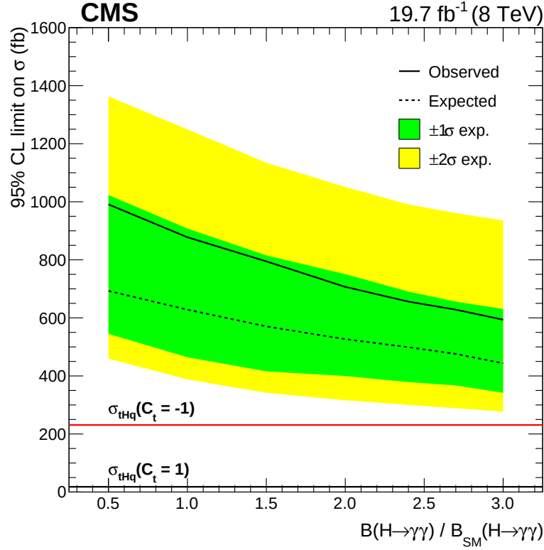
Figure 5.29.: Expected and observed CL_s limits for the tHq production at 95% C.L. provided by the combination as a function of the assumed branching ratio of H \rightarrow \gamma\gamma . The cross section predicted under the assumption of a flipped sign of the top-Yukawa coupling is depicted as a red line, the standard model cross section is depicted as a black line. The combination is not yet able to exclude the case of an anomalous coupling. The diagram is taken from Reference [138].
