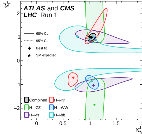
Figure 1.6.: Combined coupling fits of CMS and ATLAS, under the assumption that no BSM particles are resolved in the virtual loops and all coupling parameters for fermions are equal. Whereas four out of five Higgs decay mechanisms favor a negative coupling factor of the Higgs boson to fermions, the measurements are more incompatible for negative values of \kappa_f^f , leading to a best-fit value very close to the SM prediction. This incompatibility stems mainly from the H \rightarrow \gamma\gamma decay which is indirectly sensitive to the relative sign of \kappa_f^f and \kappa_V^f . The diagram is taken from Reference [45].
