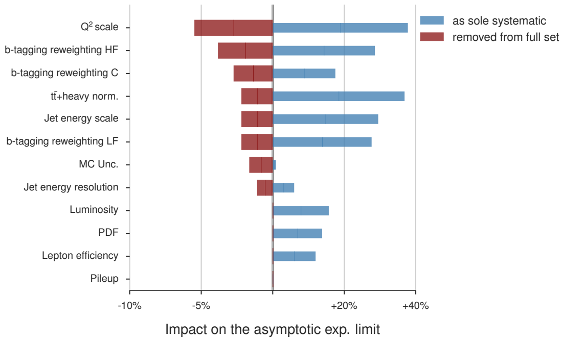
Figure 6.26.: Impact of groups of systematic uncertainties on the expected asymptotic limit. The groups of systematic uncertainties are either removed from the fit by fixing them to their postfit value, or used as single systematic uncertainty by fixing all other uncertainties to their postfit values. The changes displayed in this diagram are calculated relatively to the limit with all systematic uncertainties included (red bars) and to the limit, where all uncertainties are fixed to their best fit value (blue bars).
