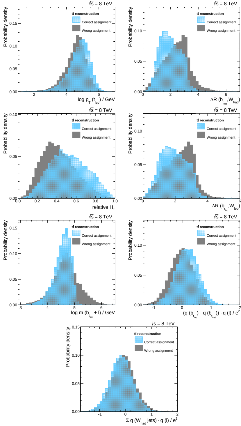
Figure A.5.: The remaining seven variables between correct and wrong jet assignments in the t\bar{t} reconstruction are shown sorted by their importance in the training. All distributions are normalized to unit area. The corresponding variable descriptions can be found in Table 5.4.
