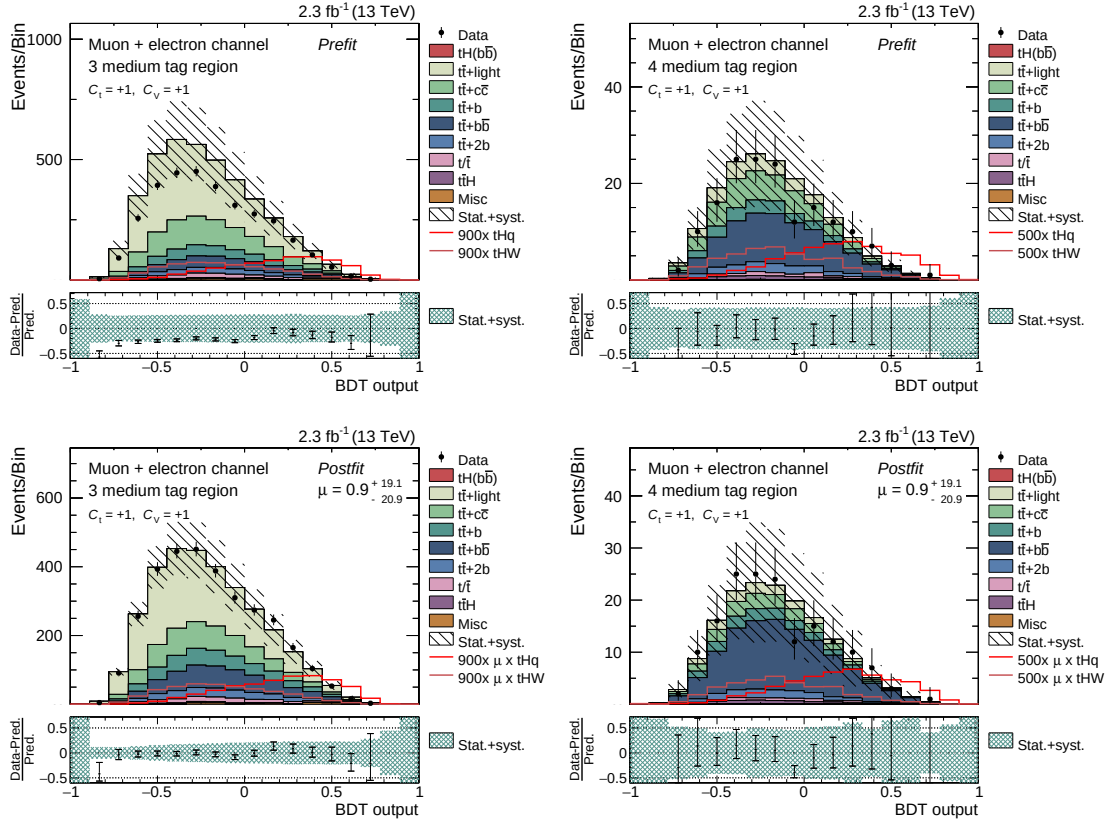
Figure B.13.: Pre- and postfit distributions of the classifier output in the 3M and 4M region for the coupling pair predicted by the SM of C_t = +1 and C_V = +1 . These distributions are fitted simultaneously and a signal strength factor or \mu = 0.9^{+19.1}_{-20.9} has been determined. A good agreement of simulation and data is observed after the fit.
