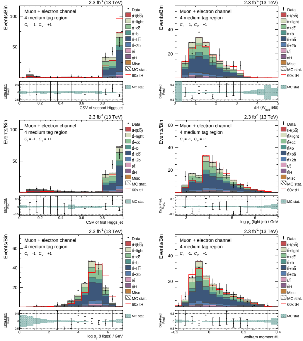
Figure B.11.: Simulation to data comparisons for input variables of the classification ranked 7 th to 12 th at \sqrt{s} = 13 TeV. Distributions are sorted by their importance in the training and are shown in the 4M region for the coupling case of C_t = -1 and C_V = 1 . A good agreement of simulation and data is found. In both diagrams the simulation is scaled to match the event yields observed in data and all MC weights are applied.
