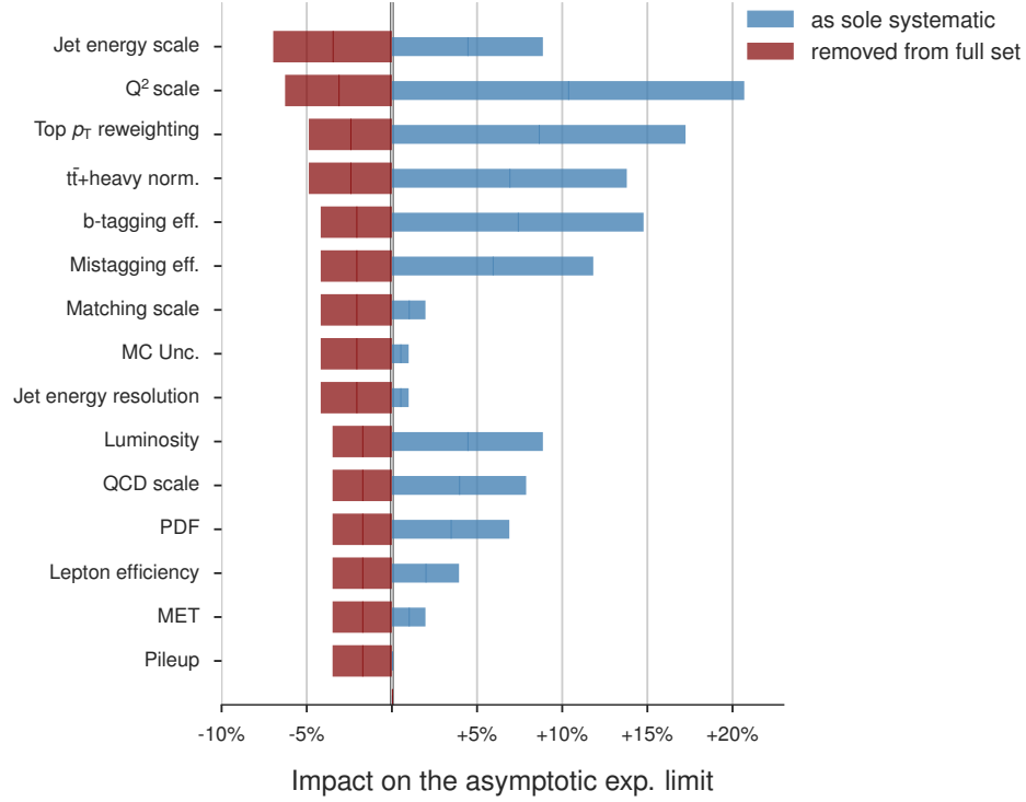
Figure 5.27.: Impact of groups of systematic uncertainties on the expected asymptotic limit. The groups of systematic uncertainties are either removed from the fit by fixing them to their postfit value, or used as single systematic by fixing all other uncertainties to their postfit values. The relative changes displayed in this diagram are calculated to the limit with all systematic uncertainties included (red bars) and to the limit, where all uncertainties are frozen to their best fit value (blue bars).
