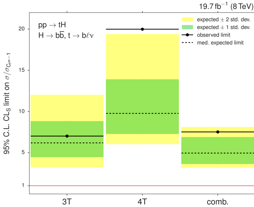
Figure 5.28.: Expected and observed CL s limits at 95% C.L. in the 3T and 4T as well as their combination. Corresponding numbers can be found in Table 5.9.
