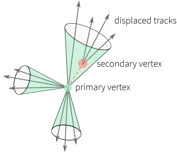
Figure 3.6.: The illustration shows the production of a secondary vertex due to the longer lifetime of a produced B meson. Multiple tracks inside of one jet are interpolated to a displaced vertex, the so called secondary vertex.
