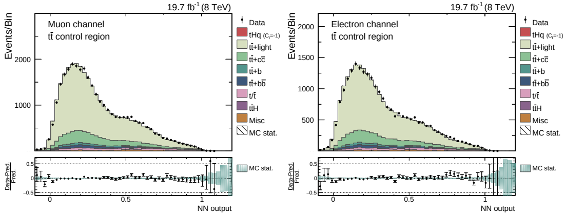
Figure 5.23.: Response of the classification comparing simulation to data in the t\bar{t} control region for the muon channel (left) and the electron channel (right). In both distributions a good agreement between simulation and data is observed. In both diagrams the simulation is scaled to match the event yields observed in data and all simulation corrections are applied. The corresponding distributions for the 3T and 4T region before the fit can be found in Appendix A.8.
