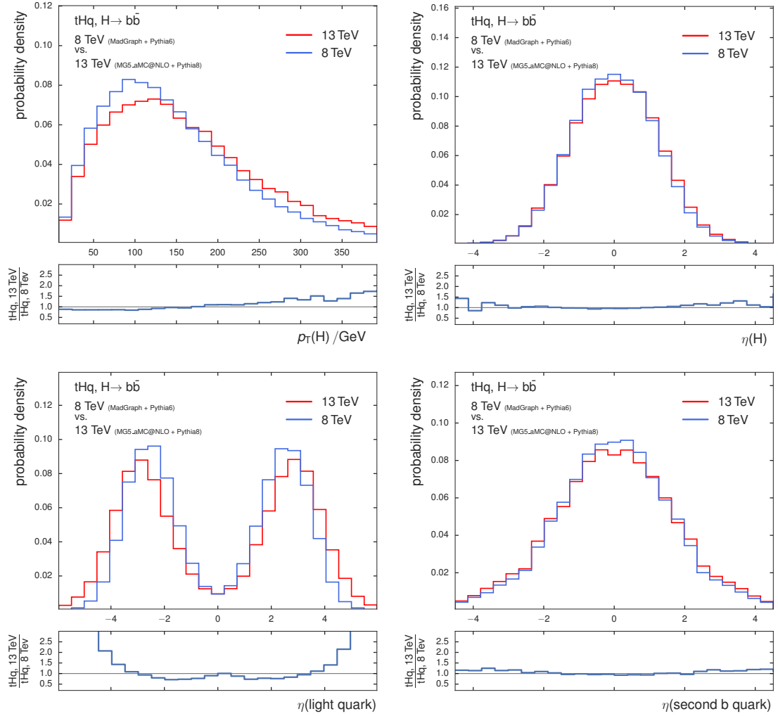
Figure 6.3.: Distributions of kinematic variables of objects of the tHq process for 8 TeV and 13 TeV. The kinematics of the top quark in the process are very similar to those of the Higgs boson, hence only one set is shown. All objects are produced with a higher transverse momentum and are produced in a more forward direction at 13 TeV. This effect is much more pronounced for the light quark in comparison to Higgs boson, top quark and second b quarks.
