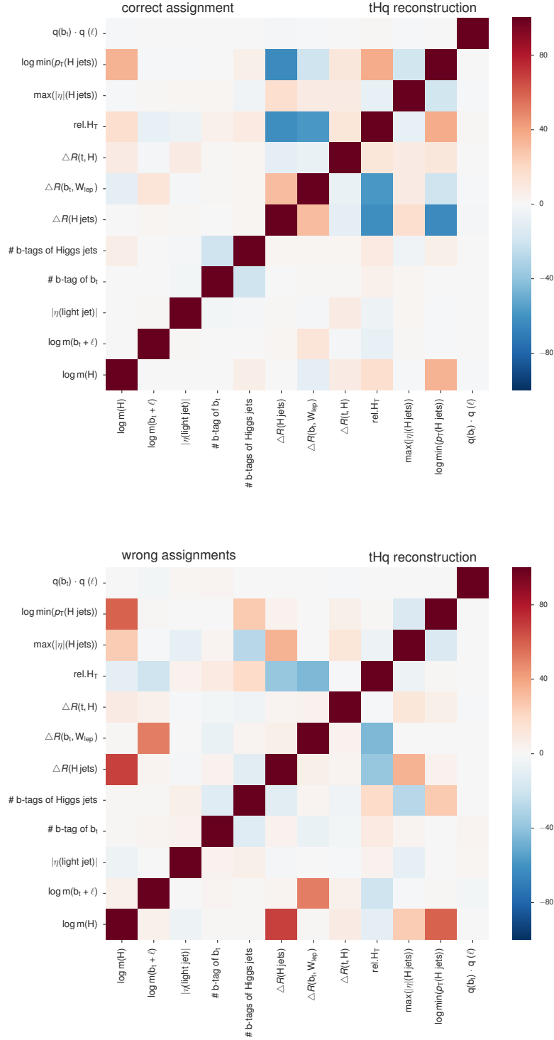
Figure 5.9.: Correlations between variables used in the tHq reconstruction for correct and wrong jet assignments. It is clearly visible that correlations are apparent between variables for correct assignments that are not visible for wrong assignments, such as the correlation between the \Delta R of the two Higgs jets and the transverse momentum of the softer of the two Higgs jets, and vice versa.
