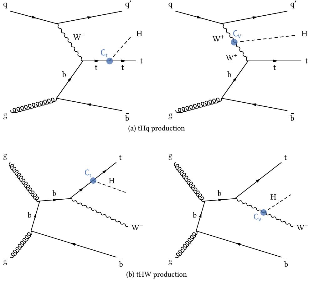
Figure 1.3.: Feynman graphs of the tHq (a) and tHW (b) production mechanism. The graphs are shown in the so-called four-flavor scheme which prohibits the presence of a b quark in the proton and hence requires an initial gluon splitting into b\bar{b} (see Section 3.1.2). The interference between the two diagrams of each channel ultimately leads to the sensitivity of tH production to the sign of C_t .
