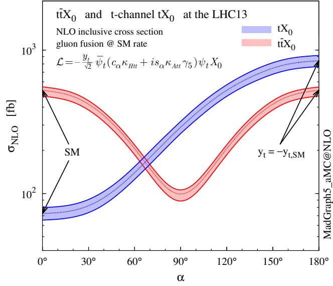
Figure 1.4.: The production cross section for a \mathcal{CP} violating X_0 particle produced in association with a top quark pair (red) and a single top quark (blue) as a function of \mathcal{CP} -mixing angle \alpha . The diagram is taken from Reference [43].
