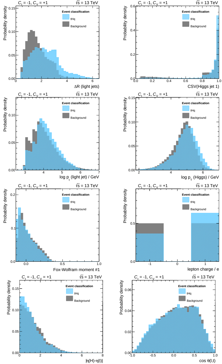
Figure B.6.: Variables ranked 8 th to 15 th used in the final classification of events at \sqrt{s} = 13 TeV. All distributions are normalized to unit area. The corresponding variable descriptions can be found in Table 6.6.
