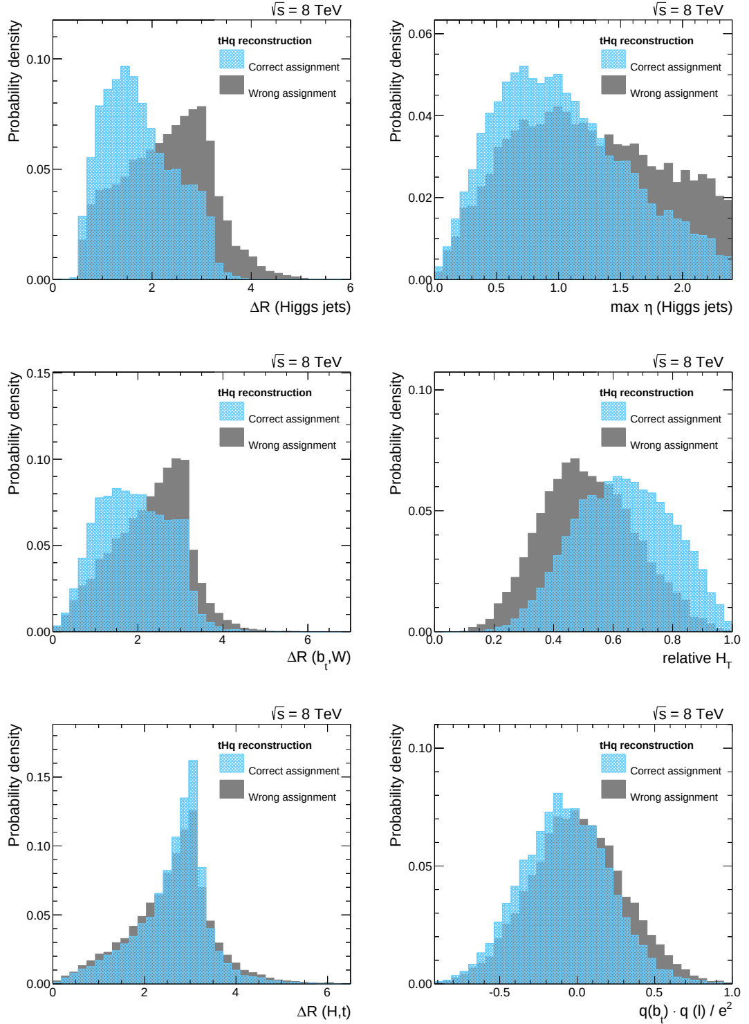
Figure A.2.: The remaining six variables between correct and wrong jet assignments in the tHq reconstruction are shown sorted by their importance in the training. All distributions are normalized to unit area. The corresponding variable descriptions can be found in Table 5.3.
