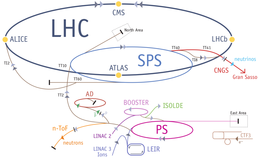
Figure 2.1.: Overview of the LHC accelerator complex, taken from [52]. For the standard proton-proton run mode, protons are accelerated in the LINAC2 accelerator, followed by the PSB (BOOSTER), PS and SPS before they are injected into the LHC. They are brought to collision at the four main experiment sites. When in heavy ion run mode, lead ions of vaporized lead are accelerated in the LINAC3 and the Low Energy Ion Ring (LEIR) before entering the same route as the protons.
