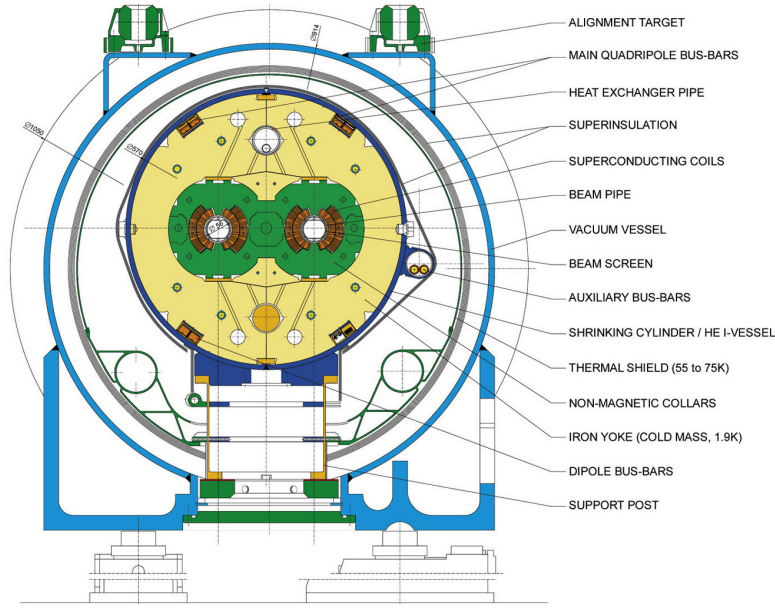
Figure 2.2.: The cross section of one of the 1232 dipole magnets of the LHC. In the center the two separate beam pipes are visible needed for the contra-rotation of the two positively charged proton beams. Taken from [53].
