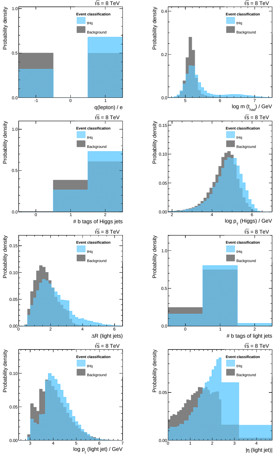
Figure 5.17.: Input Variables used in the final classification of events sorted by their importance in the training. All distributions are normalized to unit area. The corresponding variable descriptions can be found in Table 5.5.
