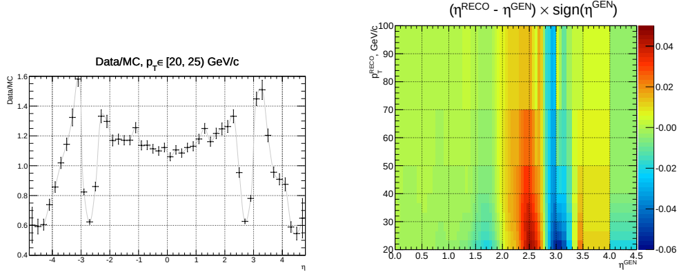
Figure 5.6.: The mismodeling observed in the jet pseudorapidity. On the left the ratio of observed to predicted event yields in bins of \eta for low- p_T jets is shown. An overestimated number of jets at |\eta| \sim 2.7 is followed by an underestimation at |\eta| \sim 3.2 . In the most forward regions the number of predicted jets again exceeds the observed number.
