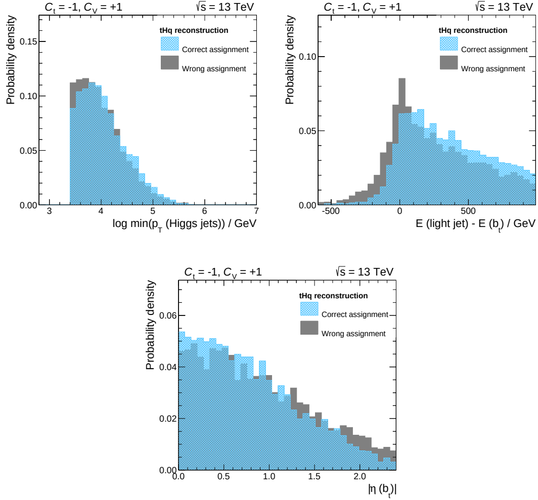
Figure B.2.: Distributions of variables ranked 13 th to 15 th place are shown for correct and wrong jet assignments in the tHq reconstruction. All distributions are normalized to unit area. The corresponding variable descriptions can be found in Table 6.2.
