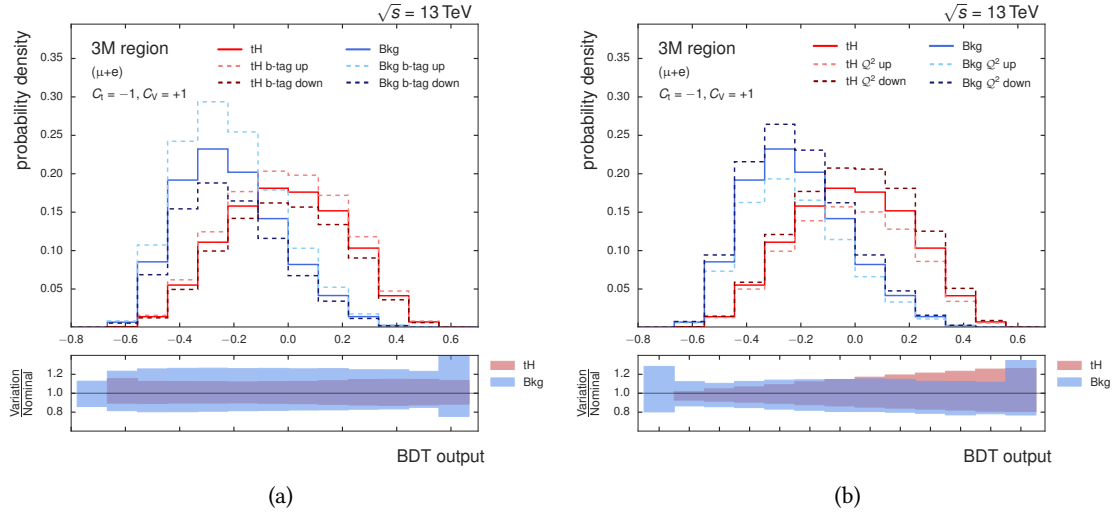
Figure 6.23.: Effect of the CSV reweighting uncertainty (left) and Q^2 scale uncertainties (right) on the final classifier for the background and signal shape in the 3M region are shown. The displayed uncertainties correspond squared sums of the contributing uncertainty sources. The signal and background histograms are normalized to unity, the systematically shifted templates are allowed to change shape as well as the normalization. Whereas the b-tagging uncertainty is mostly flat over the complete BDT output range, thus resulting in a change of normalization, Q^2 uncertainties grow for larger BDT output values.
