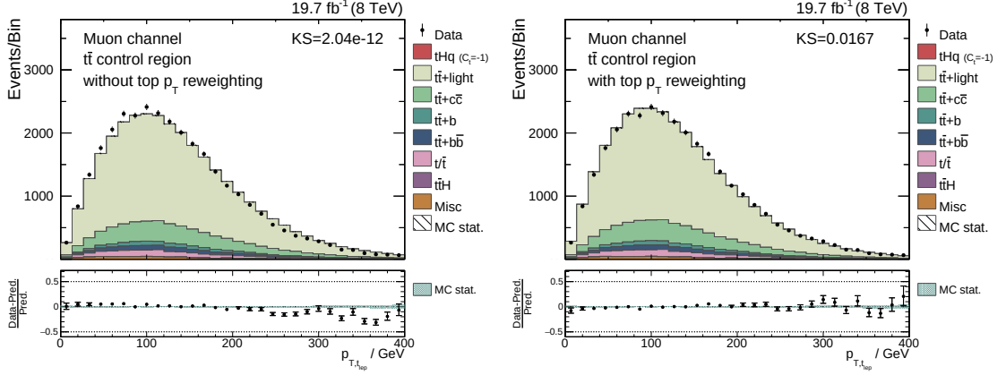
Figure 5.5.: Distribution of the transverse momentum of the reconstructed leptonically decaying top quark of the t\bar{t} process before (left) and after (right) application of the top quark p_T reweighting. The simulation predicts a harder momentum spectrum of the top quarks than what is observed in data. For both distributions the simulation is scaled to match the observed event numbers in data. After the reweighting a good agreement of simulation and recorded events is observed.
