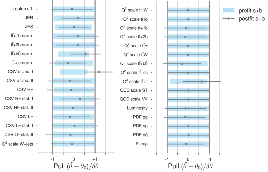
Figure 6.25.: Pre- and postfit pulls of all nuisance parameters of the analysis in an s+b fit (bin-by-bin uncertainties excluded).
