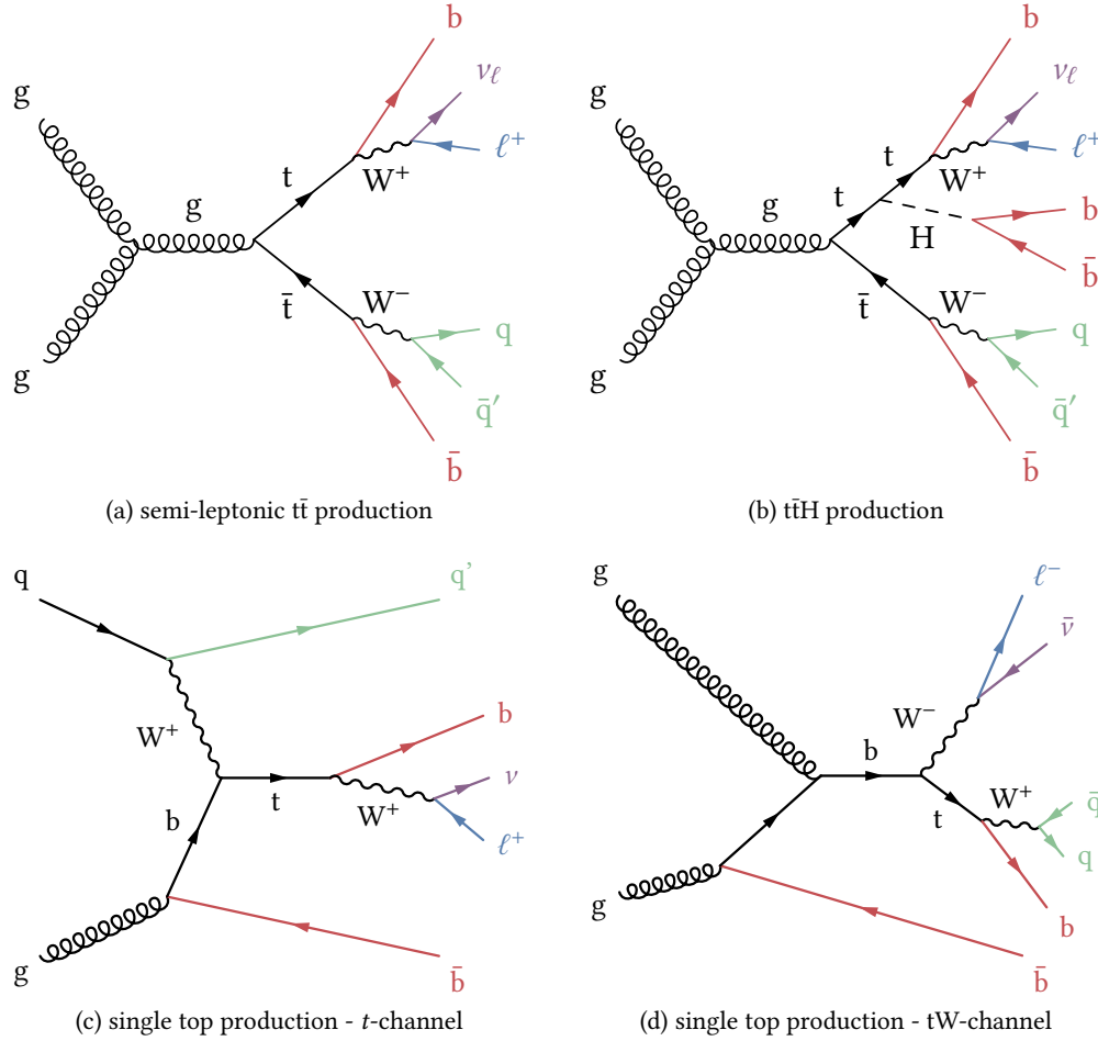
Figure 5.3.: Feynman diagrams of various background processes. In (a) the most prominent semi-leptonic t\bar{t} process can be seen. Its final state consists of two b quarks (red), one charged lepton (blue), one neutrino (violet) and two light jets (green).
