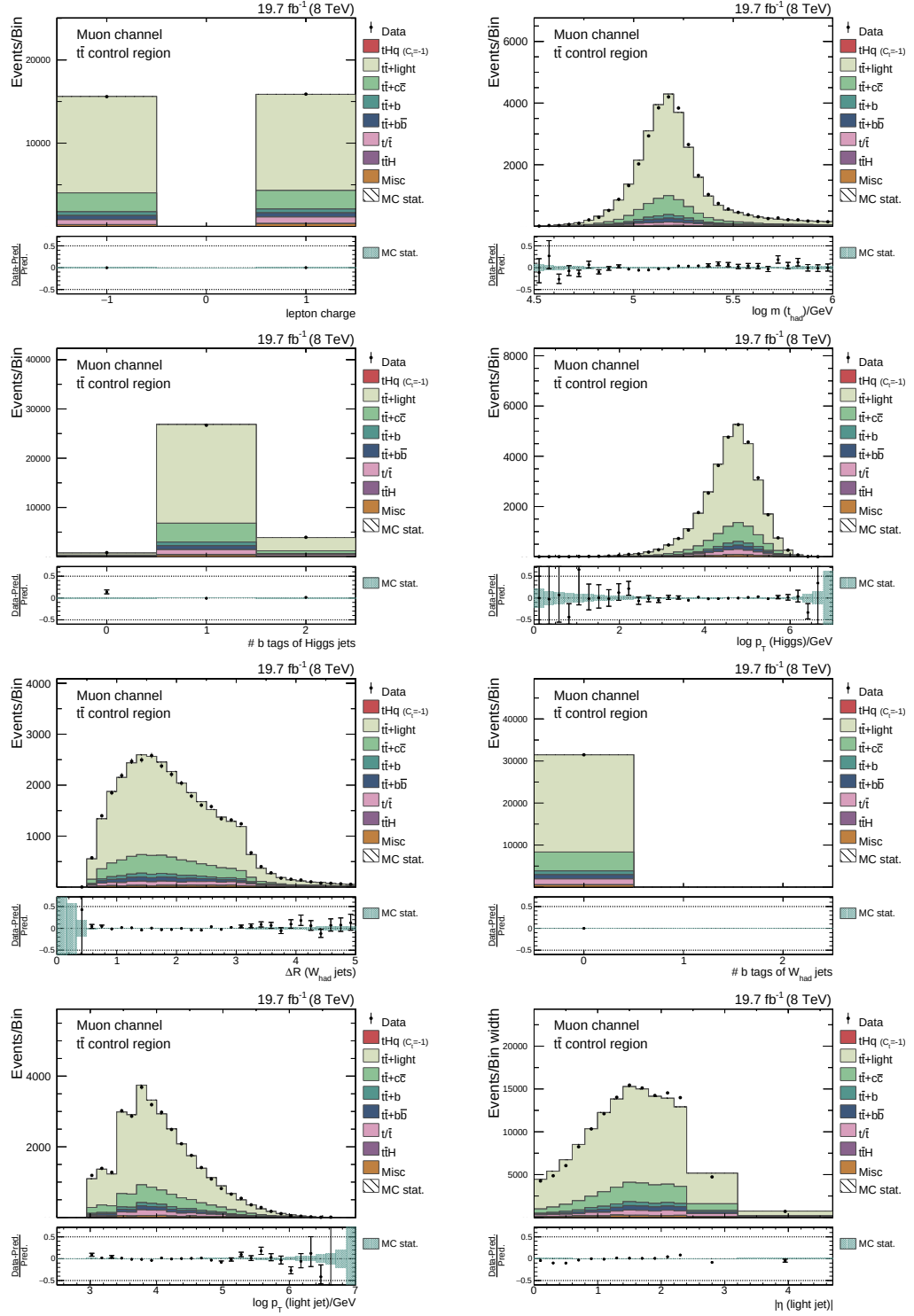
Figure 5.18.: Simulation to data comparisons for the input variables of the classification for the muon channel in the t\bar{t} control region sorted by their importance in the training. A good agreement between simulation and data is observed. In both diagrams the simulation is scaled to match the event yields observed in data and all simulation corrections are applied.
