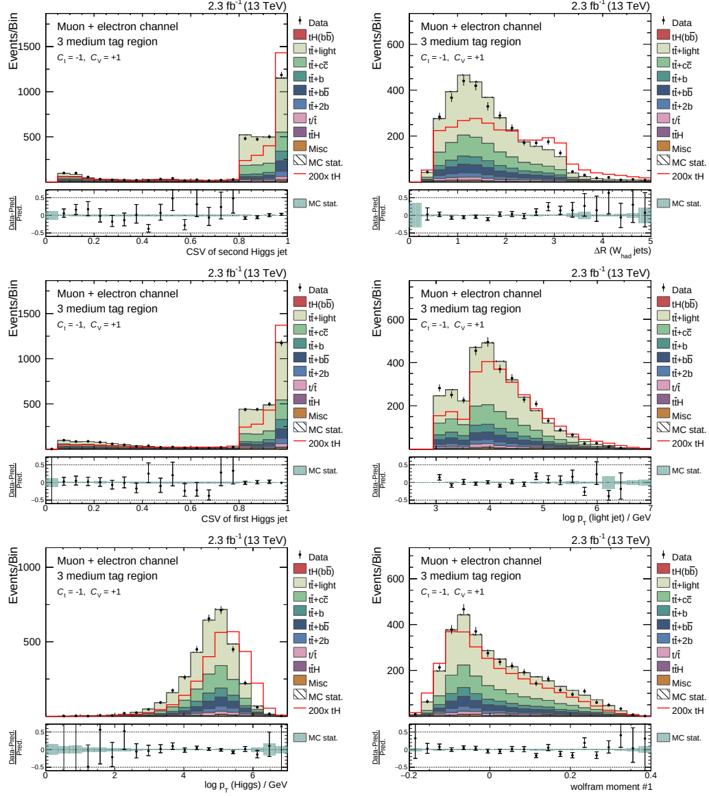
Figure B.9.: Simulation to data comparisons for input variables of the classification ranked 7 th to 12 th at \sqrt{s} = 13 TeV. Distributions are sorted by their importance in the training and are shown in the 3M region for the coupling case of C_t = -1 and C_V = 1 . A good agreement of simulation and data is found. In both diagrams the simulation is scaled to match the event yields observed in data and all MC weights are applied.
