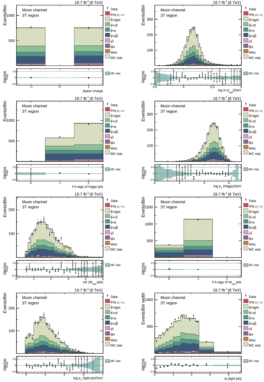
Figure 5.19.: Simulation to data comparisons for the input variables of the classification for the muon channel in the 3T region sorted by their importance in the training. A good agreement between simulation and data is observed. In both diagrams the simulation is scaled to match the event yields observed in data and all simulation corrections are applied.
