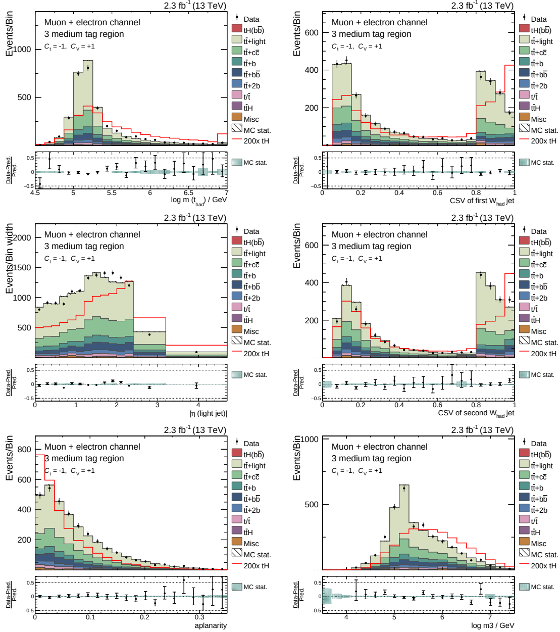
Figure 6.20.: Simulation to data comparisons for the six most important input variables of the classification at \sqrt{s} = 13 TeV. Distributions are sorted by their importance in the training and are shown in the 3M region for the coupling case of C_t = -1 and C_V = +1 . Besides a small normalization offset a good agreement of simulation and data is found. In all diagrams the simulation is scaled to match the event yields observed in data and all MC weights are applied. The distributions of the remaining variables of the classification can be found in Appendix B.9 and B.10.
