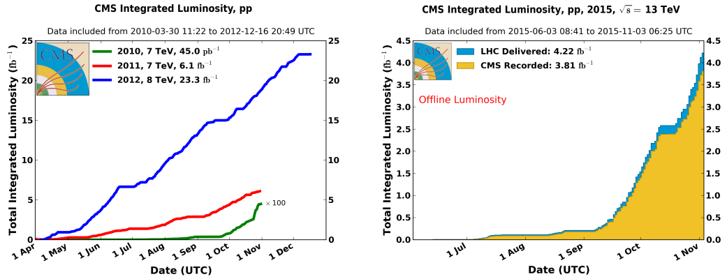
Figure 2.3.: An overview of the collected data in Run I and Run II, respectively. On the left side the total integrated luminosity for the complete Run I can be found. It can be seen by the enhanced green line that in 2010 only 45 \text{ pb}^{-1} at \sqrt{s} = 7 \text{ TeV} were recorded, as it was made sure that every detail in the LHC was working properly. In 2011 the integrated luminosity grew constantly until 6.4 \text{ fb}^{-1} were gathered. After the upgrade to a slightly higher center of mass energy of \sqrt{s} = 8 \text{ TeV} CMS collected its major part of data in 2012.
