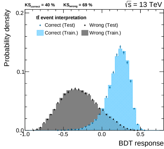
Figure 6.12.: Output values of the t\bar{t} reconstruction BDTs for correct and wrong jet assignments. A clear separation is visible. The reconstruction training procedure is examined with an independent set of events that were not part of the training sample. Events used in the training are presented as histograms, whereas the independent testing sample is represented by markers. A good agreement between the testing and training sample is observed, verified by high KS-values of the two distributions. No sign of overtraining can be found.
