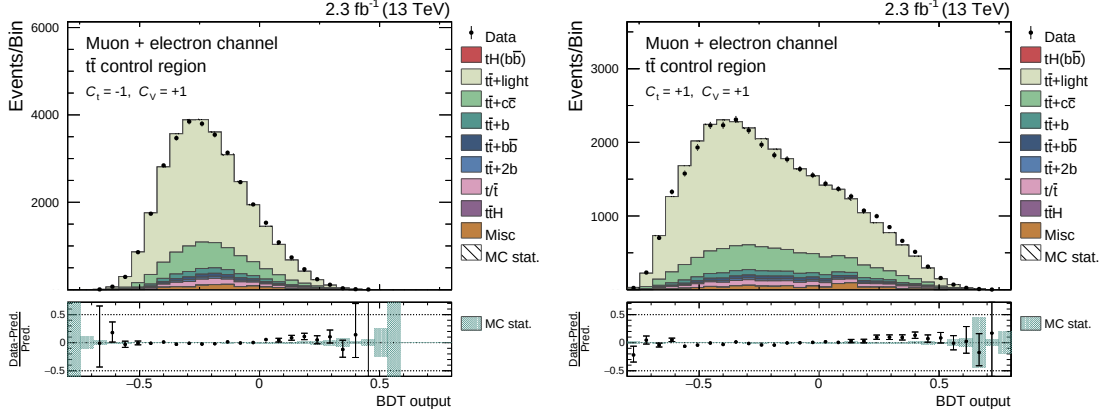
Figure 6.22.: Simulation to data comparisons for the output of the classification in the t\bar{t} control region at \sqrt{s} = 13 TeV. The training output is shown for the C_t = -1 and C_V = +1 coupling point (left) and the coupling point predicted by the SM (right). In both distributions a good agreement between simulation and data is observed. The simulation is scaled to match the event yields observed in data and all MC weights are applied.
