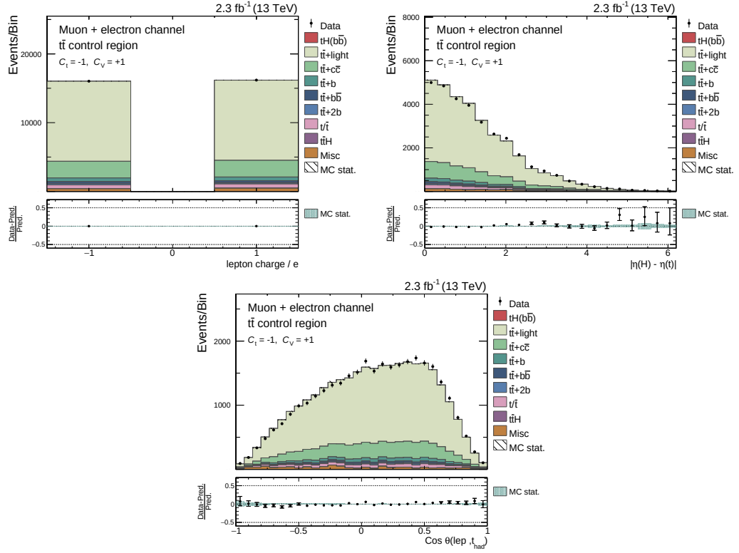
Figure B.8.: Simulation to data comparisons for input variables of the classification ranked 13 th to 15 th at \sqrt{s} = 13 TeV. Distributions are sorted by their importance in the training and are shown in the t\bar{t} control region for the coupling case of C_t = -1 and C_V = 1 . A good agreement of simulation and data is found. In both diagrams the simulation is scaled to match the event yields observed in data and all MC weights are applied.
