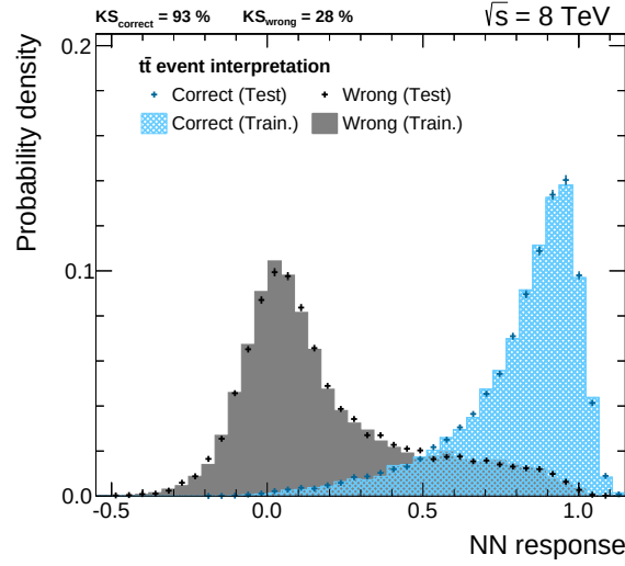
Figure 5.14.: Output values for the t\bar{t} reconstruction neural network for correct and wrong jet assignments. A clear separation between correct and wrong assignments is visible. The output of the neural net for the events used in the training are shown as histograms. The training is examined with an independent set of events that were not part of the training sample. The response for this testing sample is shown as colored markers and a good agreement between the testing and training sample is seen, verified by high KS-values of the two distributions. Thus, no sign of overtraining can be found.
