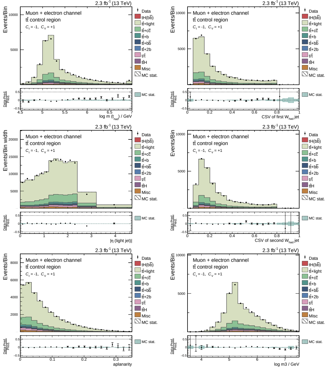
Figure 6.19.: Simulation to data comparisons for the six most important input variables of the classification at \sqrt{s} = 13 TeV. Distributions are sorted by their importance in the training and are shown in the t\bar{t} control region for the coupling case of C_t = -1 and C_V = +1 . Besides a small normalization offset a good agreement of simulation and data is found. In all diagrams the simulation is scaled to match the event yields observed in data and all MC weights are applied. The distributions of the remaining variables of the classification can be found in Appendix B.7 and B.8.
