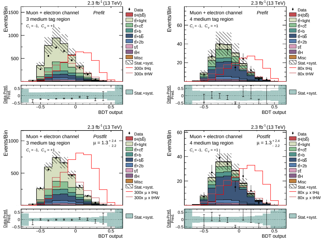
Figure 6.24.: Pre- and postfit distributions of the classifier output in the 3M and 4M region for the coupling pair of C_t = -1 and C_V = +1 . These distributions are fitted simultaneously and a signal strength factor of \mu = 1.3^{+2.4}_{-2.2} has been determined. A good agreement of simulation and data is observed after the fit. Pre- and postfit distributions for coupling parameters predicted by the SM can be found in Appendix B.13.
