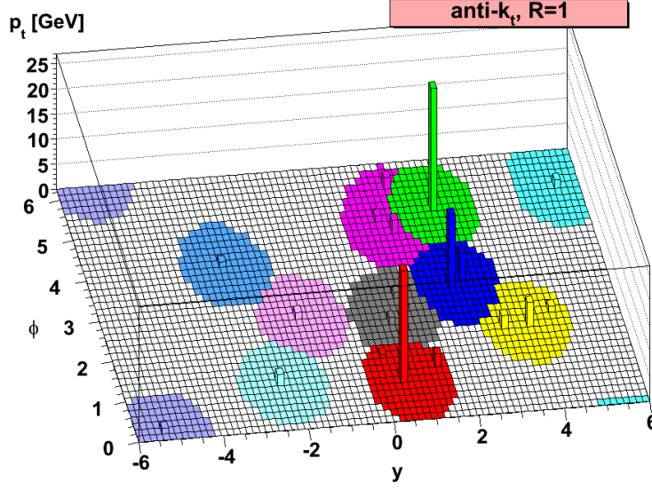
Figure 3.4.: A depiction of a jet clustering employing the anti- k_t algorithm. The diagram shows a flat projection of the HCAL with energy deposits shown as towers. The anti- k_t algorithm produces cone-like shaped jets and successfully resolves overlapping jets. Taken from [102].
