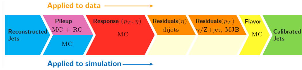
Figure 3.5.: Overview of the different jet energy correction levels. The Level-1 corrections negate the influence of pileup jets in the energy measurements and are determined in MC simulations. Additional data correction factors are derived with a random cone method (RC). Level-2 and Level-3 corrections improve the varying detector response. Further, Level-2 and Level-3 residual corrections fix remaining deviations between data and simulation. The Level-5 corrections would account for flavor-dependent variations in the detector response, but are not applied in the analyses of this thesis. The diagram is taken from [108].
