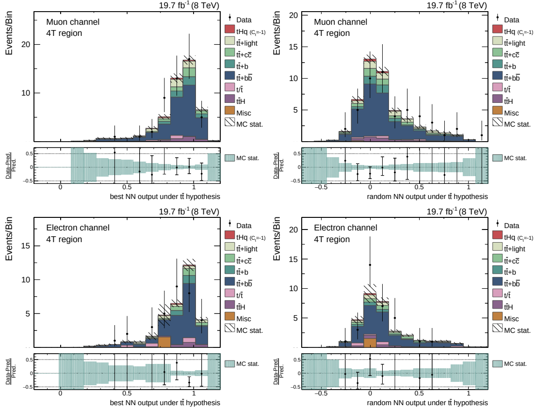
Figure A.7.: Response of the t\bar{t} reconstruction comparing simulation to data. In the left column the highest output value (chosen jet assignment) per event is shown and on the right the NN output value for a random assignment is shown. The diagrams show the situation in the 4T region for the muon channel (top row) and the electron channel (bottom row). In all distributions a good agreement between simulation and data is found. The simulation is scaled to match the event yields observed in data and all MC weights are applied.
