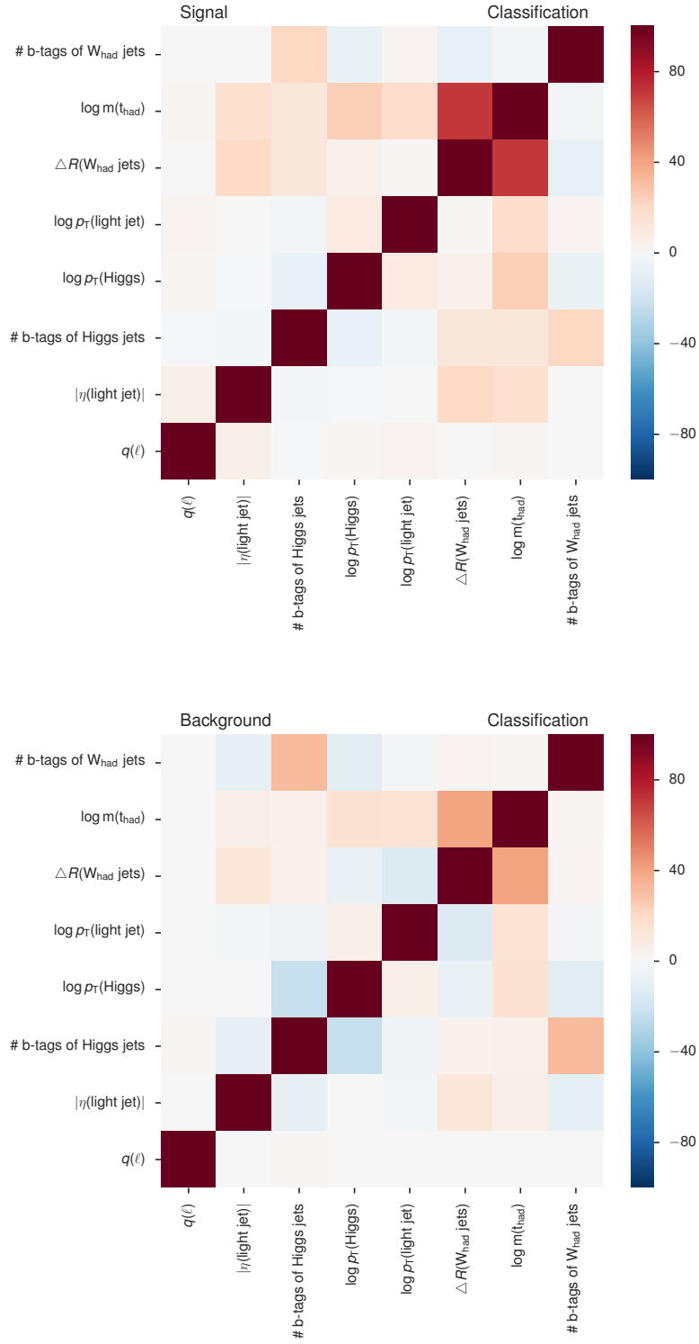
Figure 5.21.: Linear correlations between the variables used in the classification for signal and background events in the 3T region for the electron and muon channel combined.
