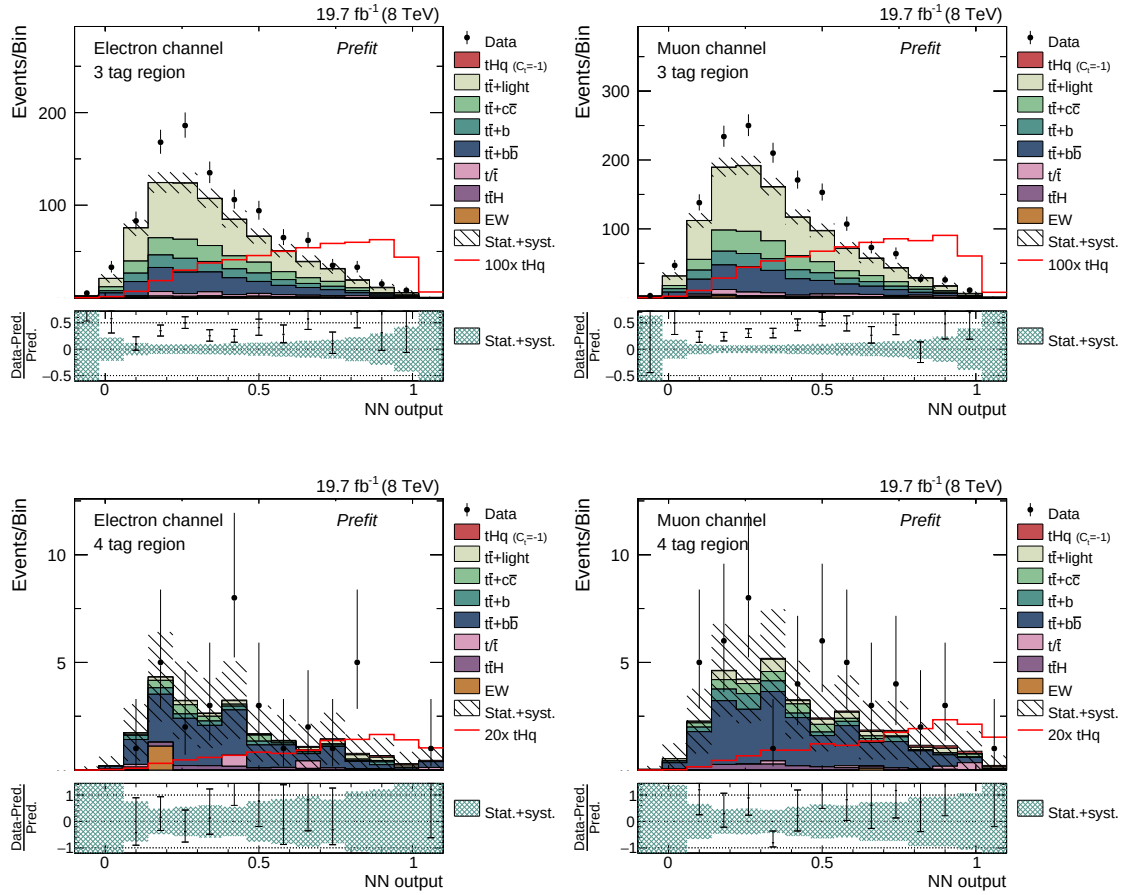
Figure A.8.: Prefit distributions of the classifier output in both lepton channels and both signal regions. Uncertainty bands include statistical and systematic uncertainties. Besides a clear offset a fair agreement in all four channels is observed, deviations from the prediction are covered by the uncertainties. The simulation samples are scaled to their expected event yields.
