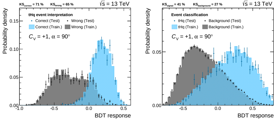
Figure 6.28.: The responses of the tX_0q reconstruction (left) and the classification (right) trainings for the training set (histograms) and the independent testing set (markers) under the assumption of a fully pseudoscalar CP boson. Training and testing sample agree well and no sign of overtraining is observed.
