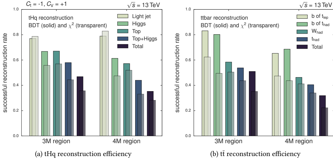
Figure 6.14.: Efficiencies of two reconstruction methods for the tHq hypothesis (left) and the tt̄ hypothesis (right), one employing BDTs and the other using a simpler \chi^2 approach, are shown in the 3M and 4M region. The bars represent the percentage that a certain object or the complete event is reconstructed correctly. The solid bars represent the reconstruction using BDTs for the assignment and the transparent bars represent the \chi^2 reconstruction. The BDT reconstruction is clearly superior to the \chi^2 method, as jets are assigned to their correct partons more frequently.
