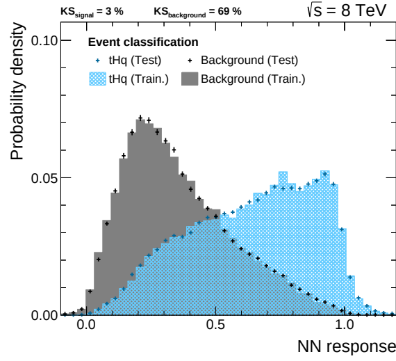
Figure 5.22.: Output values for the classification neural network for signal and background events in the 3T region for the electron and muon channel combined. A clear separation is visible. Events of the two training samples are depicted in the colored histograms. The training is examined with an independent set of events that were not part of the training sample. The response for this testing sample is shown as colored markers and a good agreement between the testing and training sample is seen, verified by high KS-values of the two distributions. No sign of overtraining can be found.
