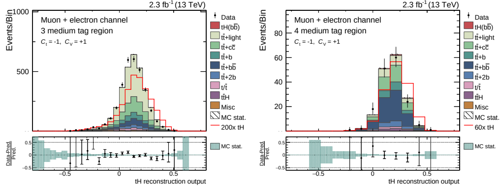
Figure B.4.: Response of the tHq reconstruction comparing simulation to data. The distribution of the highest output value (chosen jet assignment) per event is shown for the C_t = -1 and C_V = +1 point in the 3M region (left) and in the 4M region (right). In both distributions a good agreement between simulation and data is found. The simulation is scaled to match the event yields observed in data and all MC weights are applied.
