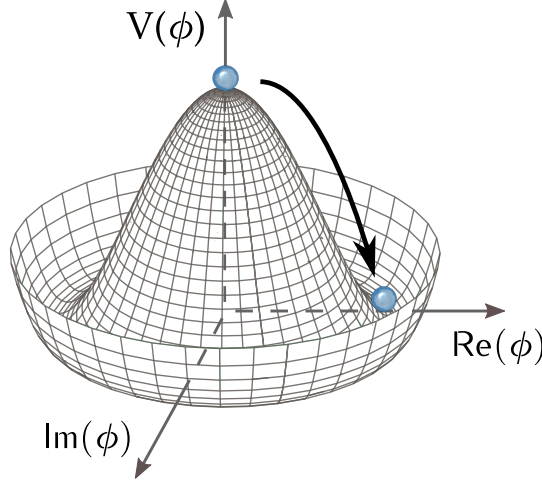
Figure 1.1.: Simplified visualization of the potential of a complex scalar field \phi with two degrees of freedom and parameters as described in Section 1.2.1. The potential has a local maximum for \phi = 0 , but an infinite number of minima located at |\phi| = v . By choosing one distinct minimum, e. g. \text{Re}(\phi) = v , \text{Im}(\phi) = 0 , the symmetry of the initial potential is broken.
