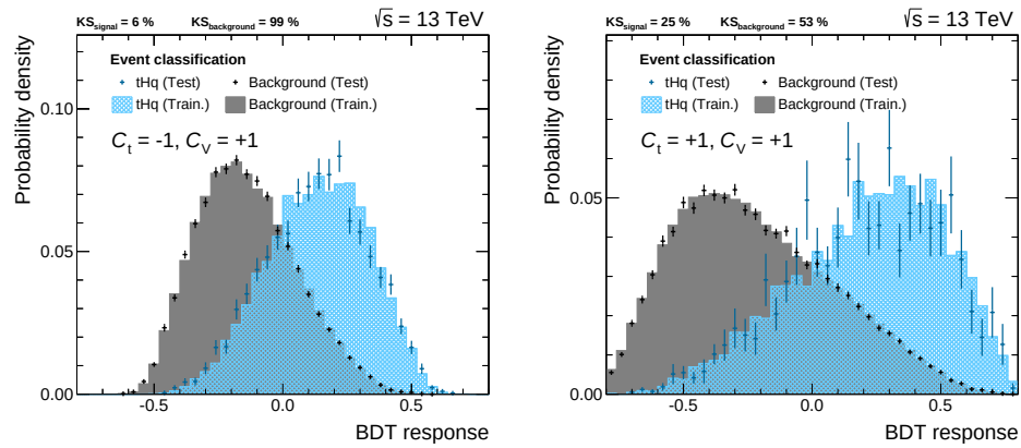
Figure 6.17.: Output values of the classification BDTs for the coupling case of C_t = -1 and C_v = +1 (left) and the SM prediction (right). A clear separation between signal and background is visible for both distributions. The classification is examined with an independent set of events. The events used in the training are presented as histograms, whereas the independent testing sample is represented by markers. A good agreement between the testing and training sample is seen, verified by high KS-values of the two distributions. No sign of overtraining is found.
