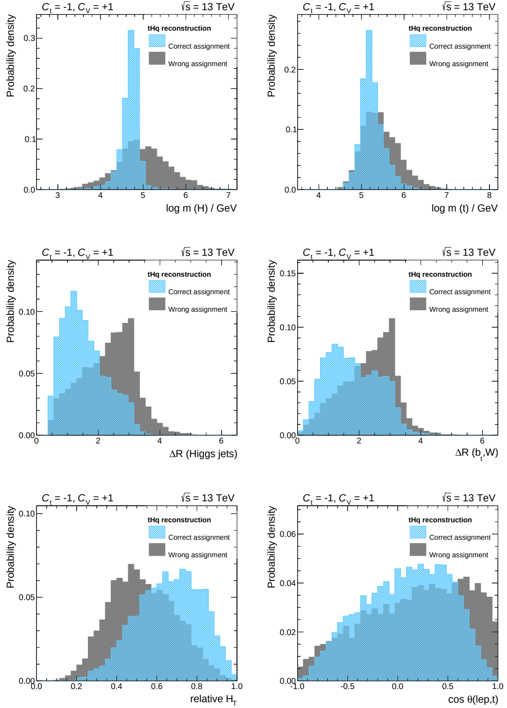
Figure 6.9.: The six most discriminating variables between correct and wrong jet assignments in the tHq reconstruction at \sqrt{s} = 13 TeV are shown sorted by their importance in the training. All distributions are normalized to unit area. The corresponding variable descriptions can be found in Table 6.2. The remaining variables can be found in Appendix B.1 and B.2.
