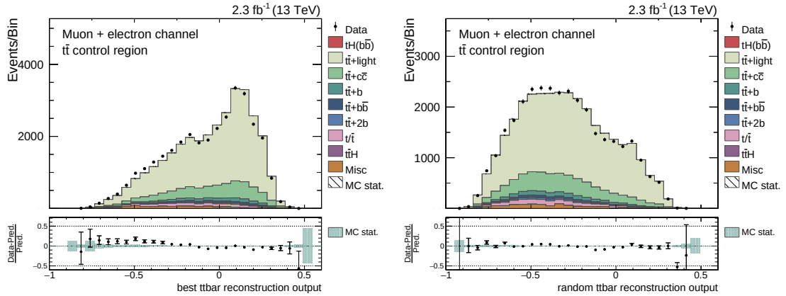
Figure 6.13.: Response of the t\bar{t} reconstruction comparing simulation to data. On the left the highest output value (chosen jet assignment) per event is shown and on the right the BDT output value for a random assignment can be seen. Both diagrams are shown in the t\bar{t} control region. In both distributions a reasonable agreement between simulation and data is found. In both diagrams the simulation is scaled to match the event yields observed in data and all MC weights are applied. The corresponding distributions in the 3M and 4M regions can be found in Appendix B.5.
