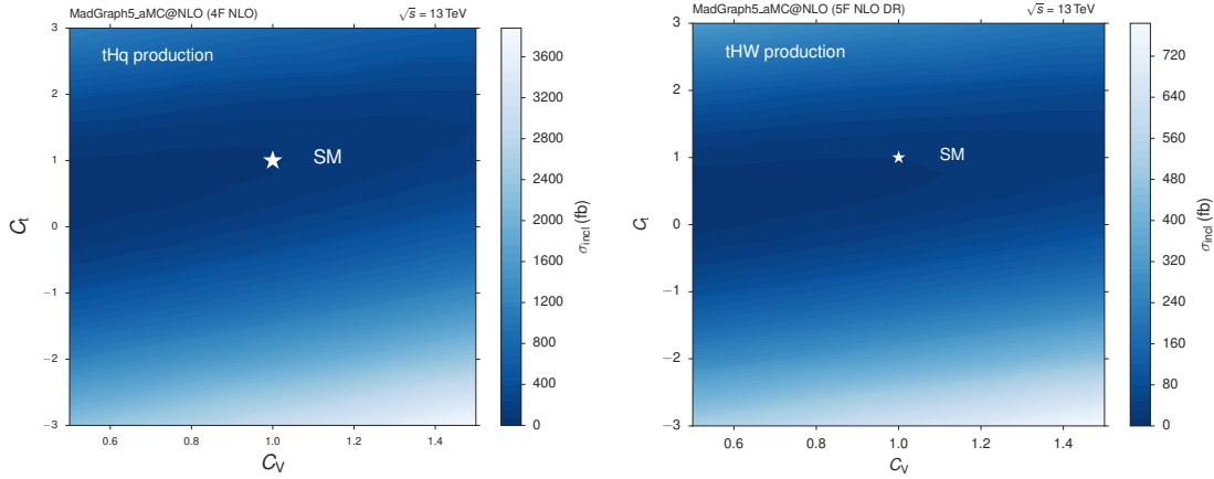
Figure 6.2.: Visualization of the cross sections of the tHq process (left) and the tHW process (right) for different points in the C_V - C_t parameter plane.
