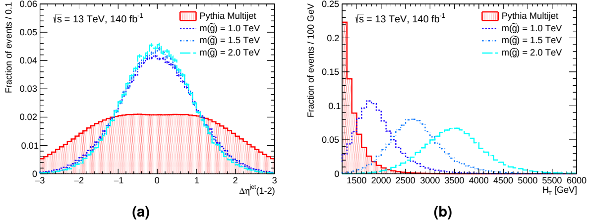
Figure 8.2: Distributions normalized to unit area of (a) \Delta\eta between the two leading jets, and (b) the total H_T in the event. In red the PYTHIA8 simulation of background events is shown. The blue lines represent three different gluino mass points. The trigger requirement and event preselection cut are applied.
