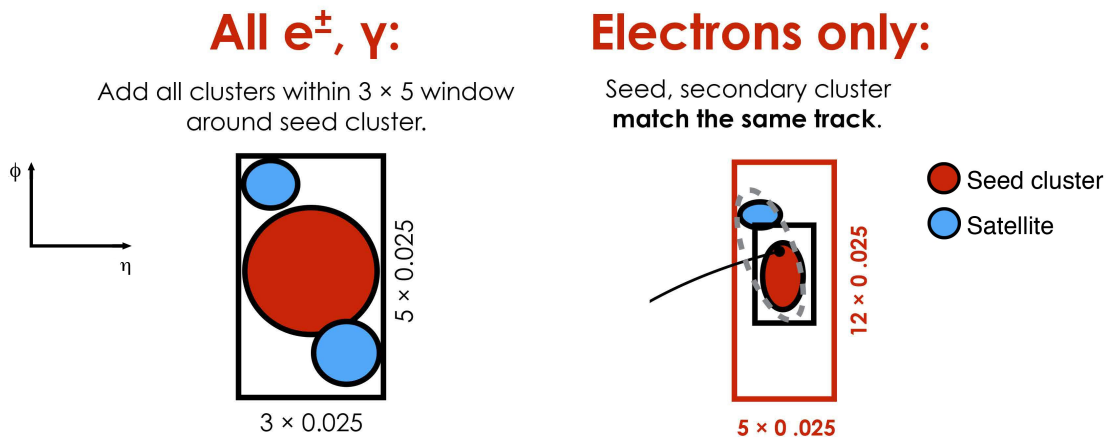
Figure 3.9: Summary of the supercluster formation for electrons and photons reconstruction [135].
