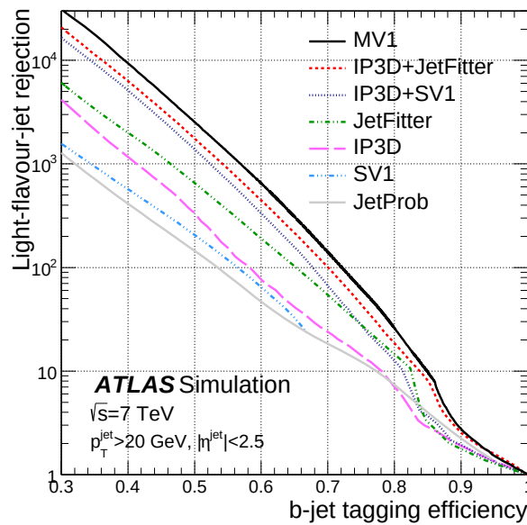
Figure 4.6: The ROC curves for b -jet efficiency versus light-jets rejection (the inverse of the mis-tag rate for light-jets) for the Run 1 taggers [167].
