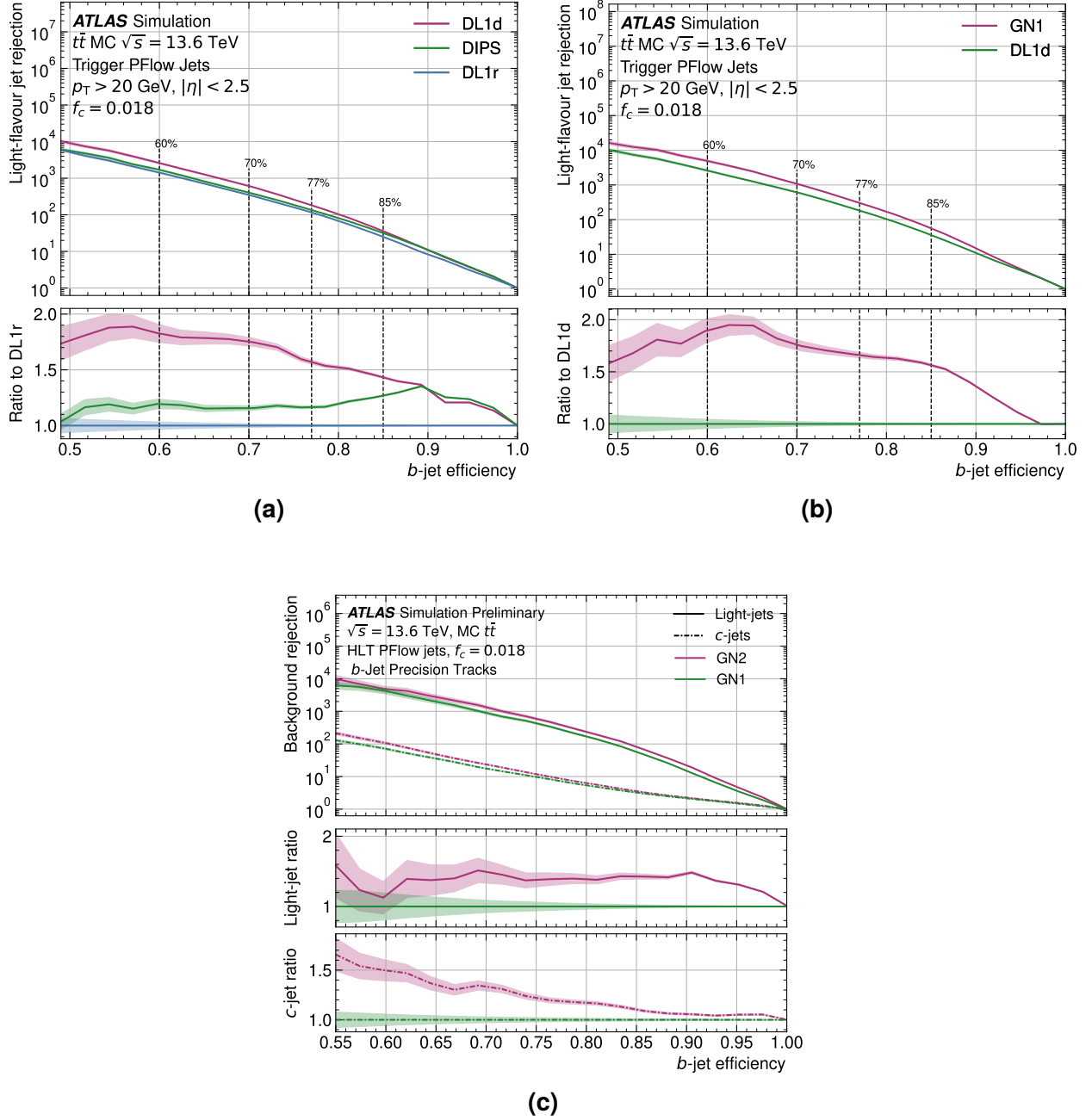
Figure 5.3: The ROC curves for several b-tagging discriminants calculated in simulated t\bar{t} events for PFlow jets [3, 189]. The (a) trigger DIPS and DL1d are compared to the DL1r algorithm, (b) the GN1 tagger introduced since 2023 is compared to DL1d, and (c) the improvement obtained with GN2 is showed in comparison with GN1.
