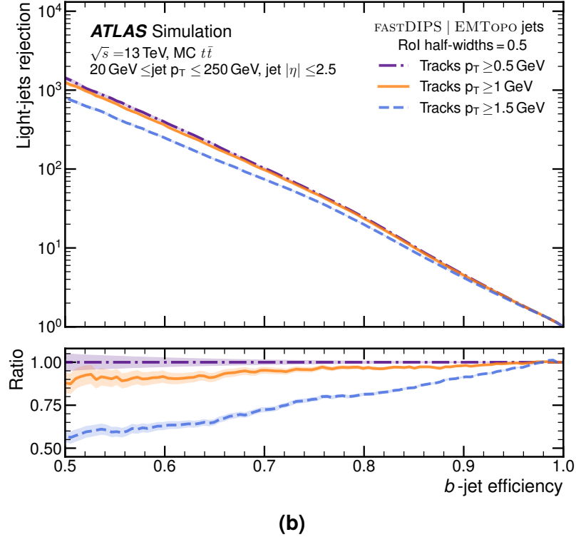
Figure 6.4: Optimisation of the Rol parameters used to run FTF tracking for the fast b -tagging preselection with EMTOPo jets. The ROC curves of different FASTDIPS versions, trained with different track sets determined by the Rol size, are reported with for a scan in (a) Rol half-widths and (b) track seeding p_T requirement. Statistical uncertainties for each ROC curve, represented with shaded regions, are computed assuming binomial efficiency errors.
