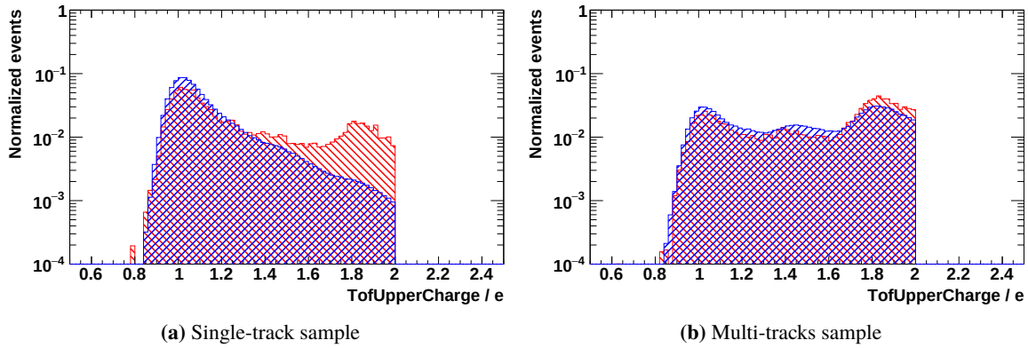
Figure A.2: Example of TofUpperCharge distribution in the energy bin 17.98 – 18.99 GeV in the electron Monte-Carlo simulation. The red histogram shows the charge-confused sample ( R > 0 ) and the blue histogram the correct reconstructed sample ( R < 0 ), after applying all preselection, selection and e^\pm identification cuts.
