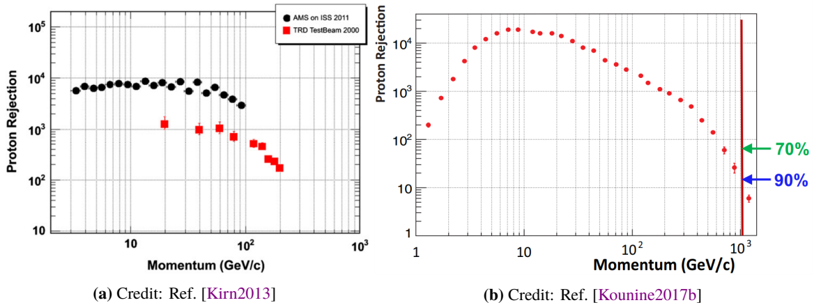
Figure 3.12: Proton rejection of the TRD as function of the e^\pm momentum at 90 % e^\pm efficiency. The left plot shows the proton rejection determined during testbeam in 2000, in comparison with the proton rejection determined from ISS data in 2011. The right plot shows the most recent measurement of the proton rejection, which greatly improved with more ISS statistics and sophisticated reconstruction algorithms.
