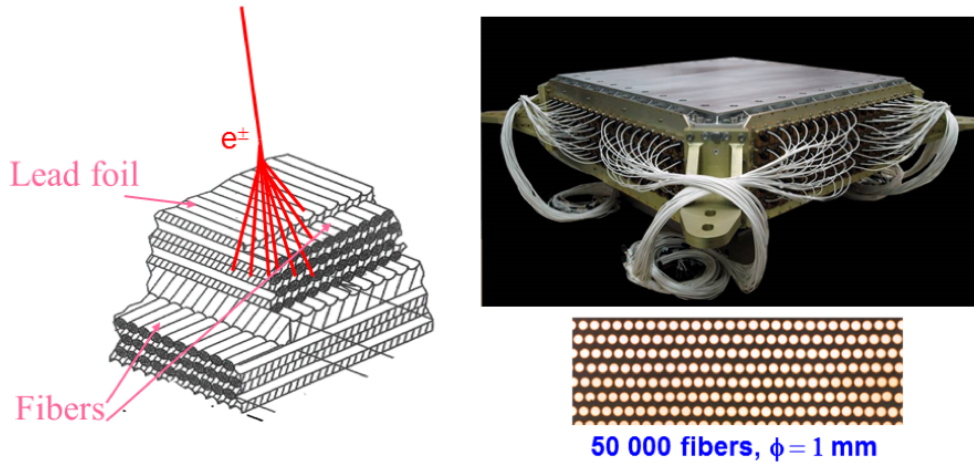
Figure 3.13: Schematic of the electromagnetic shower development in the ECAL. Credit: Ref. [AmsWebsite]
