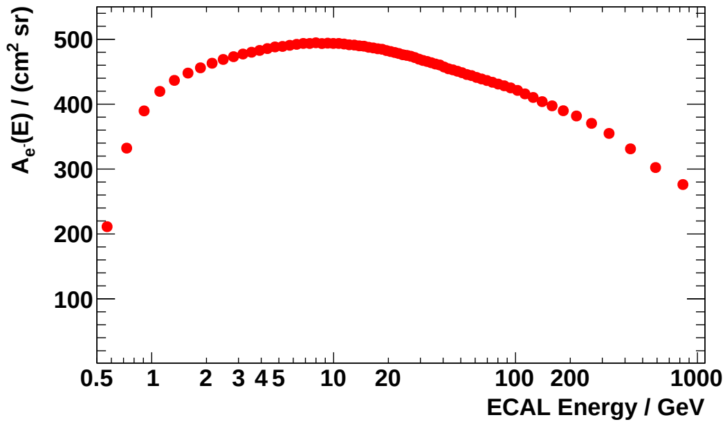
Figure 4.59: Final result of the acceptance A_e(E) as function of energy, including all Data/Monte-Carlo corrections (1 + \delta(E)) . The red symbols show that the acceptance is a smooth function with a well-behaving energy dependence.
