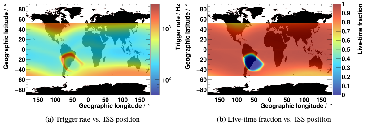
Figure 4.51: The left plot shows the trigger rate of the experiment vs. ISS position and the right plot shows the live-time fraction of the experiment vs. ISS position. The live-time fraction is exceptionally low at the South Atlantic Anomaly (SAA) [Kurnosova1962] due to an intense flux of low-energy particles, filling the detector.
