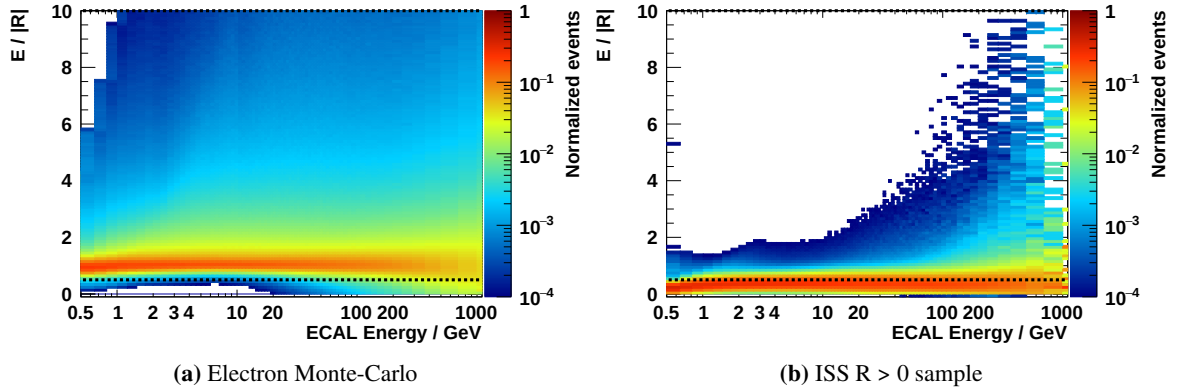
Figure 4.18: Plot of the E/|R| distribution as function of energy for the electron Monte-Carlo simulation (left) and the ISS R > 0 sample (right). The applied lower and upper cut values are shown as black dashed lines.
