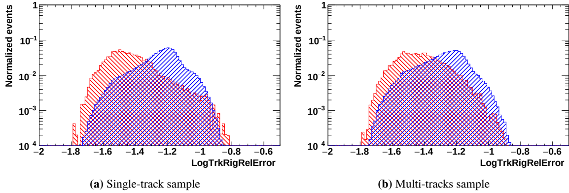
Figure A.5: Example of LogTrkRigRelError distribution in the energy bin 17.98 – 18.99 GeV in the electron Monte-Carlo simulation.
