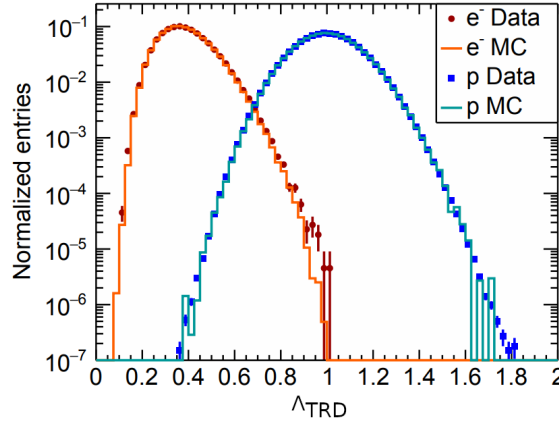
Figure 3.11: Example showing the TRD estimator, which combines the dE/dx measurements from all 20 TRD layers into a single estimator, in the energy range 10 – 100 GeV. Credit: Ref. [Raiha2017]
