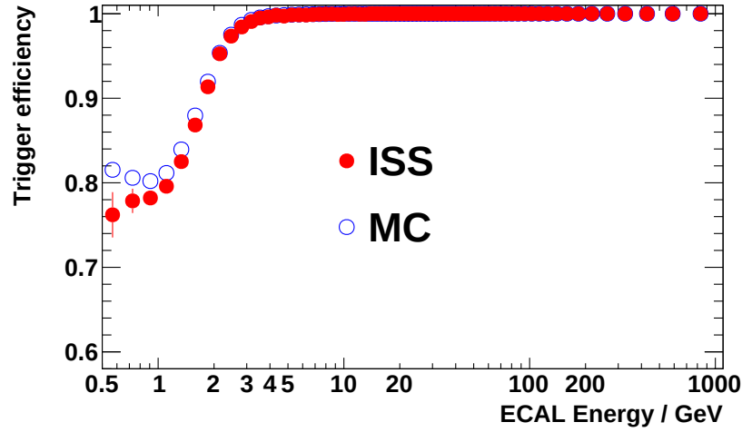
Figure 4.50: Comparison of the trigger efficiency \epsilon_{\text{trigger}}(E) as function of energy between ISS data and Monte-Carlo simulation. The red symbols represent the trigger efficiency determined from ISS data according to Eq. (4.19). The blue symbols show the trigger efficiency determined by the Monte-Carlo simulation, by counting the number of unbiased and physics triggers.
