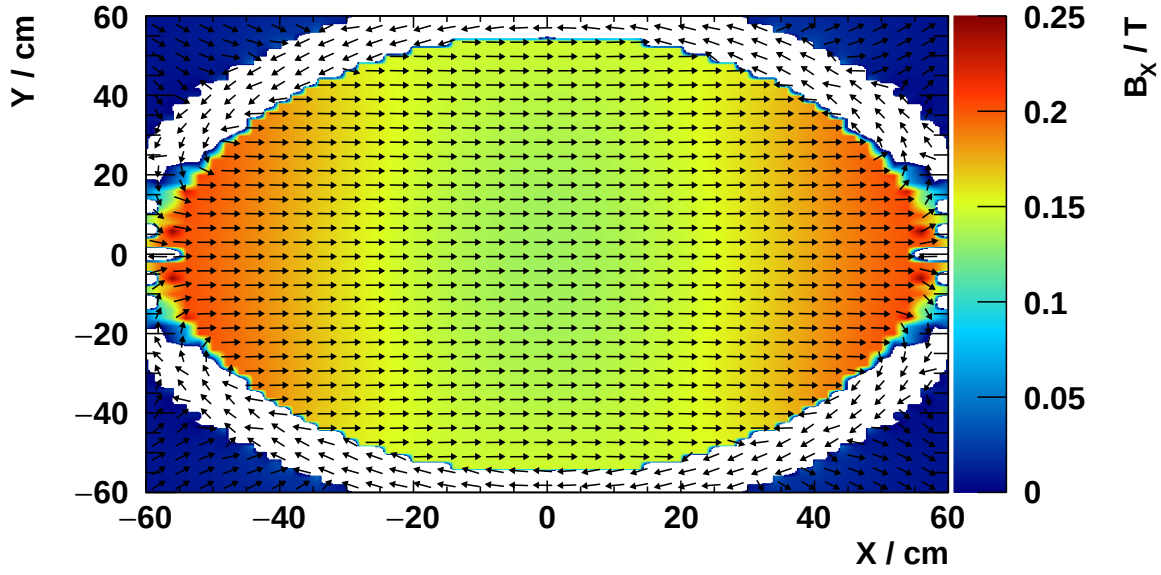
Figure 3.3: Visualization of the magnetic field in X-Y direction of the AMS-02 permanent magnet at Z = 0 cm (center of AMS). Credit: B. Beischer.
