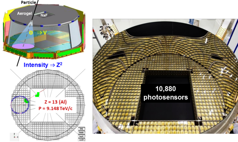
Figure 3.17: Picture of the RICH and its working principle. Credit: Ref. [AmsWebsite]
