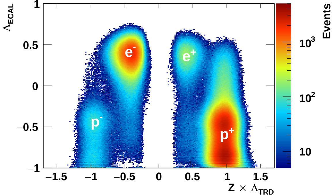
Figure 4.21: Overview of the ISS data sample after applying all selection cuts in the energy range 20 – 50 GeV. The ECAL estimator \Lambda_{\text{ECAL}} is drawn on the y-axis and the TRD estimator \Lambda_{\text{TRD}} multiplied by the charge sign Z of the primary tracker track on the x-axis. Clearly these two estimators allow to separate the different species: electrons, positrons, protons and charge-confused protons or antiprotons.
