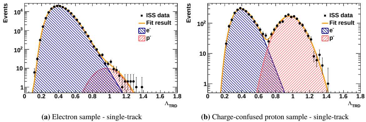
Figure 4.23: Simultaneous fit of the electron template Eq. (4.6) and the charge-confused proton template Eq. (4.7) in the energy bin 17.98 – 18.99 GeV for the single-track sample. The dark blue area corresponds to the electron template, the light red area to the charge-confused proton template and the orange line to the sum of all templates.
