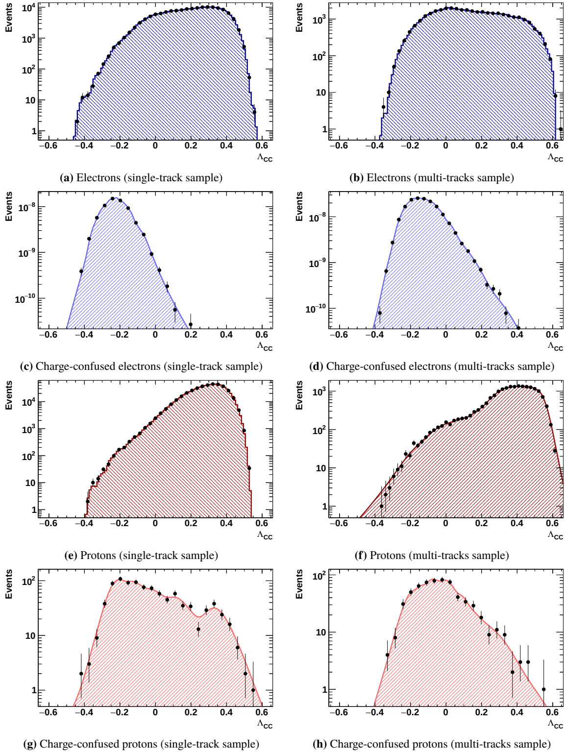
Figure 4.31: Overview of the CCMVA templates in the energy bin 17.98 – 18.99 GeV: electrons (dark blue area), charge-confused electrons (light blue area), protons (dark red area) and charge-confused protons (light red area). The black points show the CCMVA estimator output, either obtained from electron Monte-Carlo simulation or ISS data - depending on the data sample.
