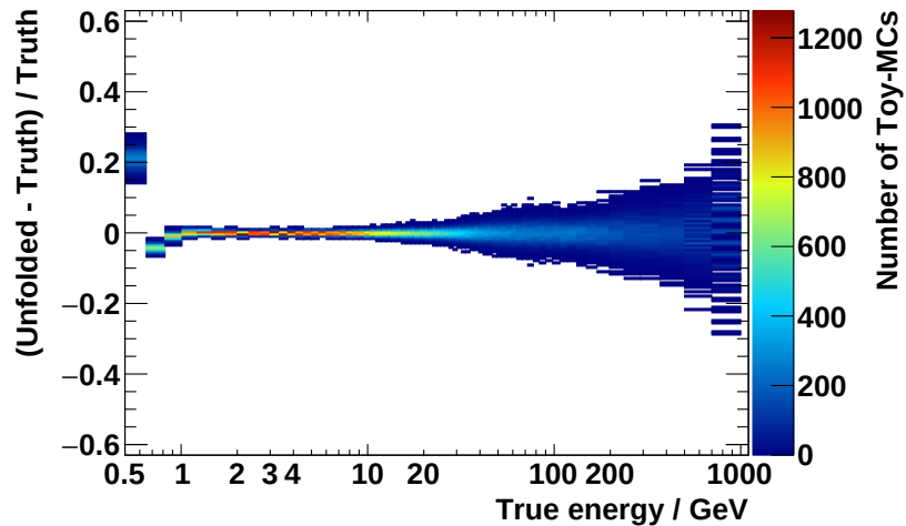
Figure 4.81: Distribution of the deviation of the unfolded e^+ flux \tilde{\Phi}_{\text{unfolded}} from the true flux \Phi_{\text{true}} divided by the true flux for P Toy-MCs as function of the true energy.
