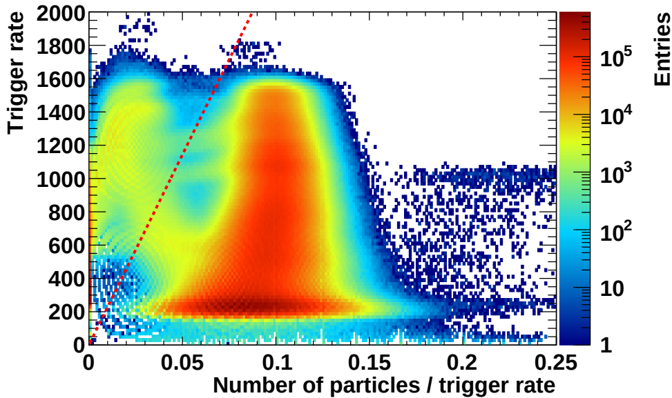
Figure A.1: Plot of the trigger rate as function of the ratio reconstructed particles over trigger rate. The red dashed line illustrates the applied cut. All seconds distributed on the left of the line are rejected for further analysis, due to non-nominal reconstruction quality of that time period.
