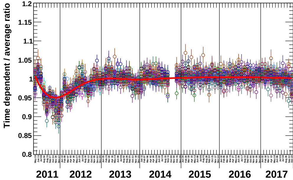
Figure 4.102: Time-dependence of the \sigma_{\text{prot, novo}} parameter for selected energy bins (1.72 – 52.33 GeV), as example, in the time-dependent analysis for the single-track sample.
