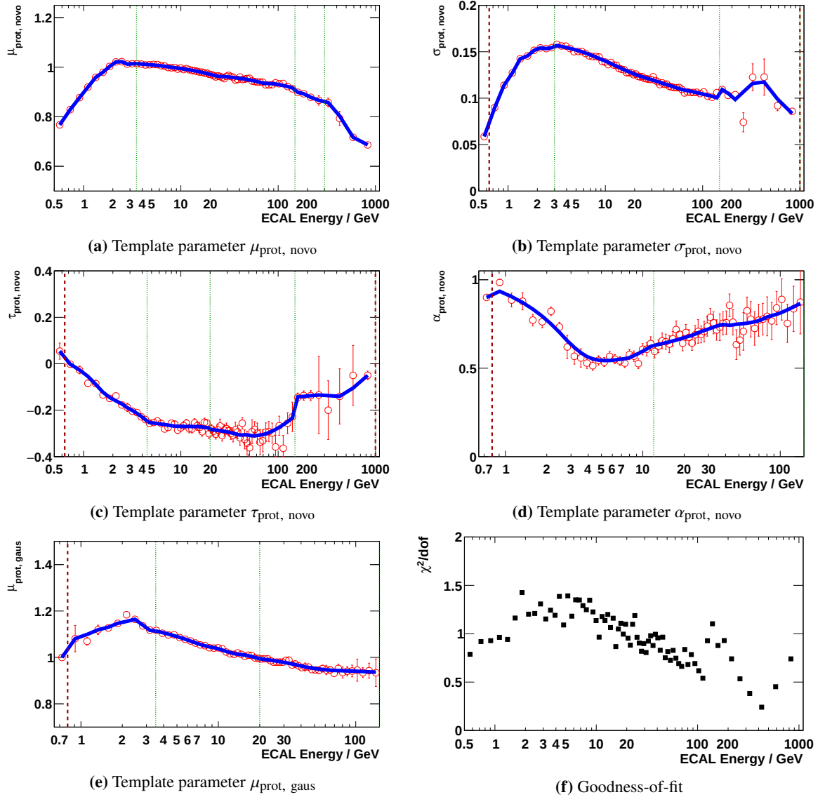
Figure A.19: Analytical TRD template parameters describing the evolution of the proton template as function of energy for the multi-tracks sample.
