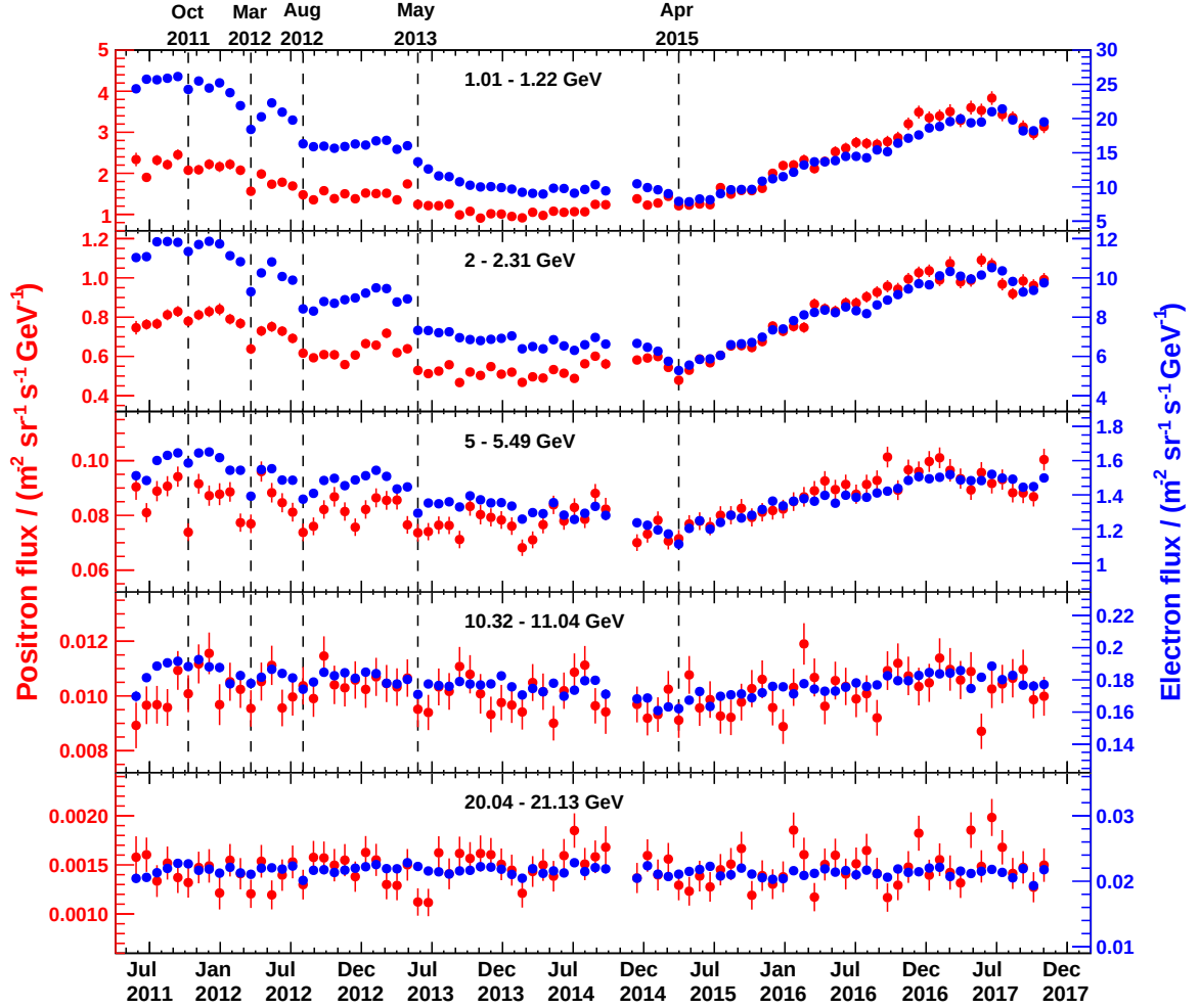
Figure 5.21: Fluxes of primary cosmic-ray positrons (red, left axis) and electrons (blue, right axis) as functions of time, for five of the 49 energy bins. The error bars are the statistical uncertainties. Prominent and distinct time structures visible in both the positron spectrum and the electron spectrum and at different energies are marked by dashed vertical lines.
