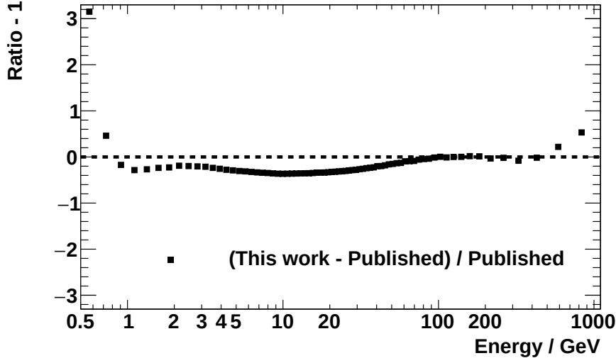
Figure B.3: Ratio of the total uncertainty of the electron flux derived in this work over the uncertainty of the recently published AMS-02 electron flux [Aguilar2019a].
