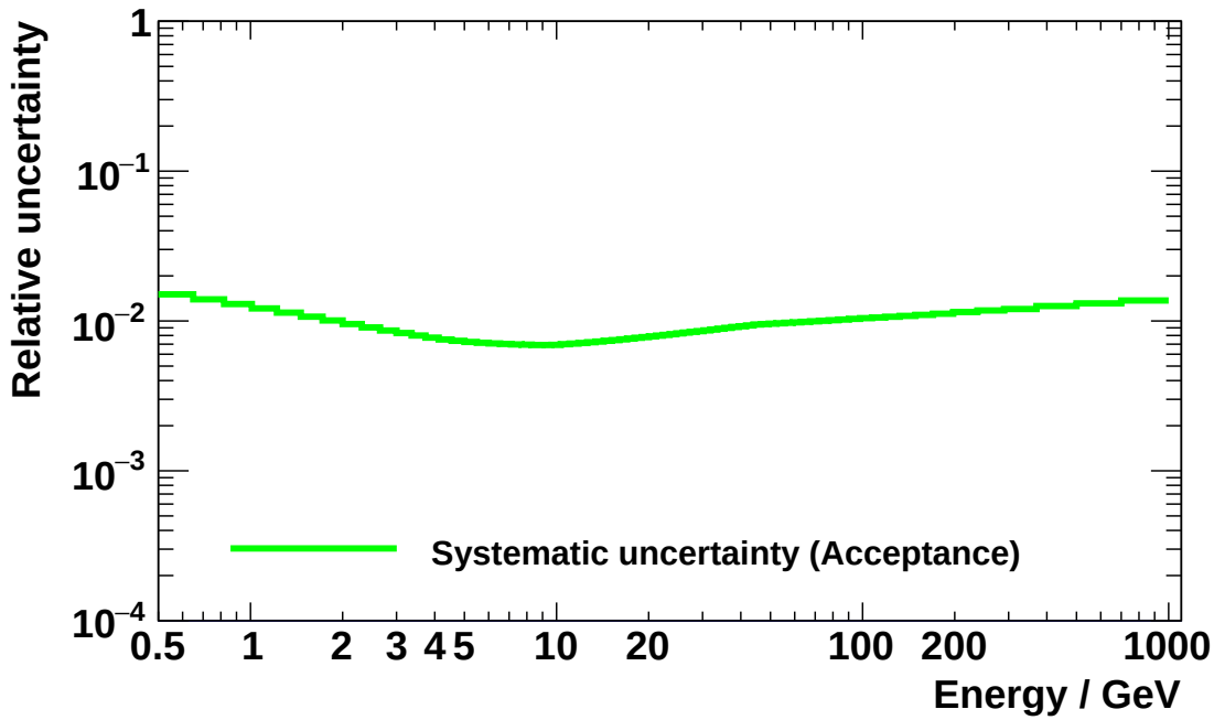
Figure 4.72: Visualization of the relative systematic uncertainty associated with the electron flux and the positron flux due to the knowledge of the acceptance.
