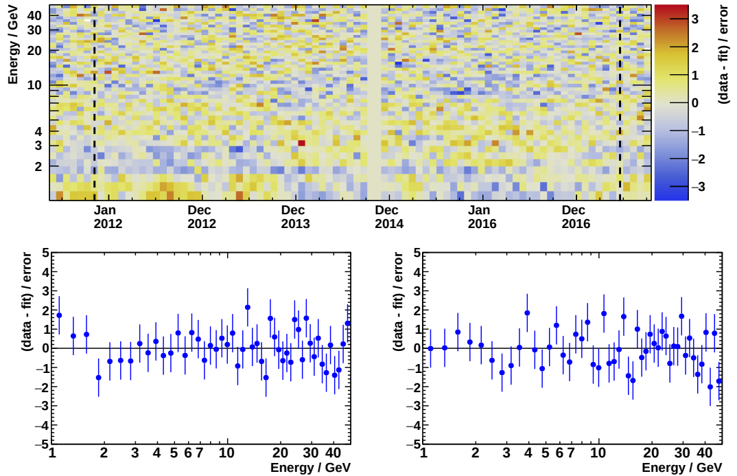
Figure 5.19: For the electron flux, the difference between data and model [Cavazonza2017] fits normalized to the experimental uncertainties: for each Bartels Rotation as a function of energy (upper plot). The distribution for the electrons reveals a model-dependent structure stable in time in the energy range between 2 – 3 GeV, emphasized for Bartels Rotation 2432 (lower left) and Bartels Rotation 2508 (lower right). The times for these two Bartels Rotations are indicated by the vertical dashed lines in the upper graph.
