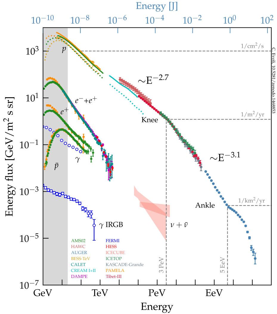
Figure 2.1: The cosmic-ray energy spectrum. Credit: Ref. [Evoli2018]
