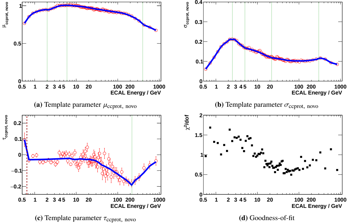
Figure 4.26: Analytical TRD template parameters describing the evolution of the charge-confused proton template as function of energy for the single-track sample. In each energy bin the analytical function - Eq. (4.7) - is fit to the template data sample, yielding the red points. A smoothing procedure yields the blue curves, which are used as template parameters for the analysis. The vertical dashed green lines mark areas where different isolated smoothing procedures are applied. The goodness-of-fit is indicated by the black points in the lower right plot.
