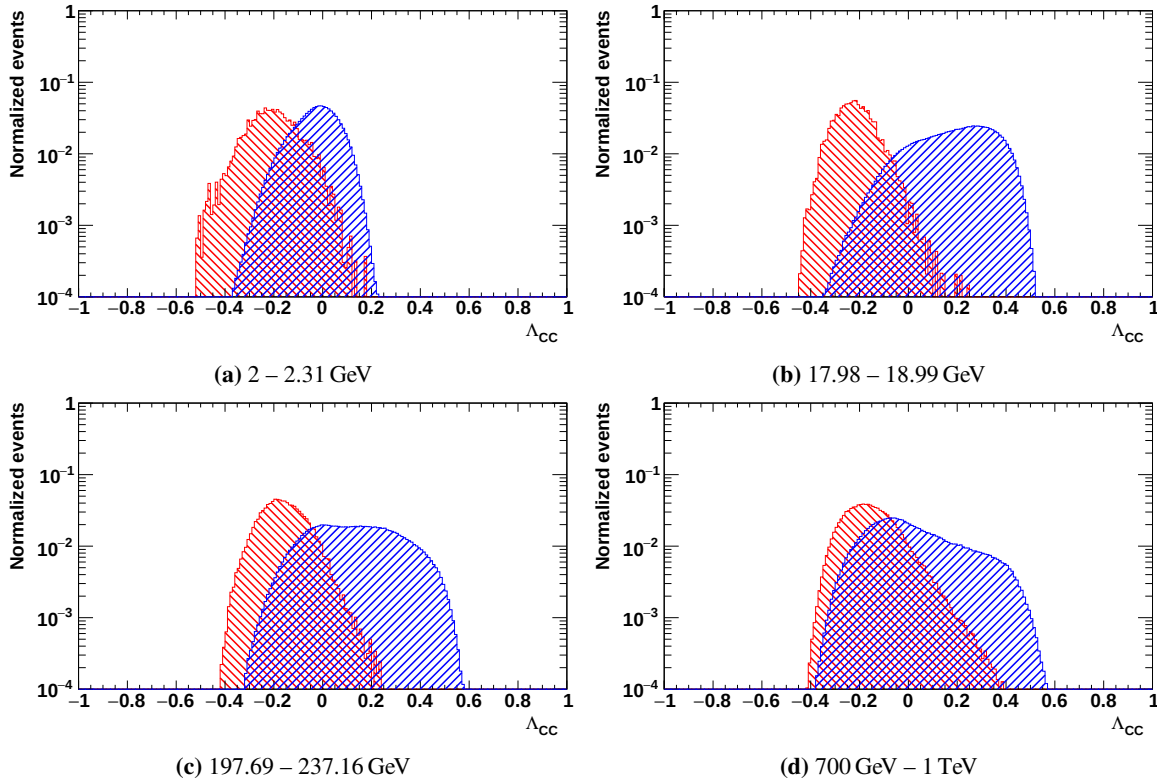
Figure 4.8: Overview of the CCMVA estimator in the single-track sample in four different energy intervals, from low energies to the highest energy in this analysis. The red histogram shows the charge-confused sample ( R > 0 ) and the blue histogram the correct reconstructed sample ( R < 0 ), after applying all preselection, selection and e^\pm identification cuts.
