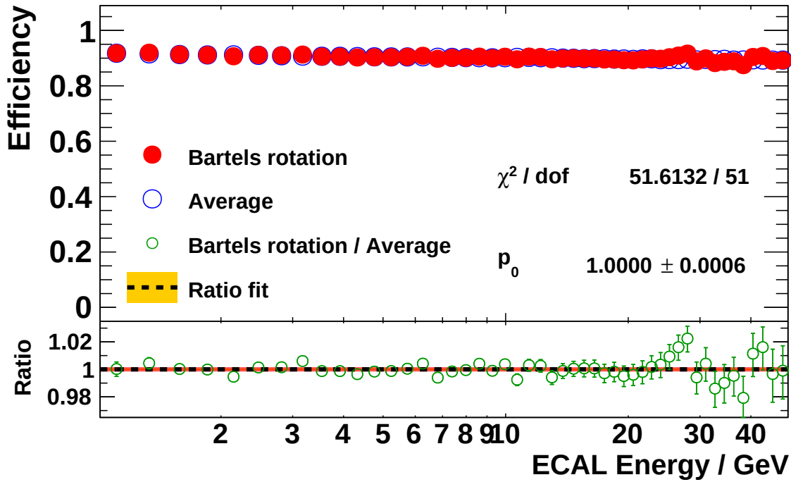
Figure 4.93: Determination of the ratio: time-averaged cut efficiency (1 + \delta^c(E)) over time-dependent cut efficiency (1 + \delta_i^c(E)) in Bartels rotation i = 26 (Apr 16 th , 2013 - May 13 th , 2013) for the selection cut: “ Tracker hit pattern ” (Section 4.3.3 - Item 5). The blue symbols in the upper plot show the cut efficiency determined from ISS data for the time-averaged analysis on a dedicated sample: the tag sample. The red symbols in the upper plot show the cut efficiency determined from ISS data in Bartels rotation i = 26 using the same tag cuts. The lower plot shows the ratio time-averaged efficiency over efficiency in Bartels rotation i = 26 as green symbols. A constant is fit to the ratio, shown as dashed black line including the orange uncertainty band.
