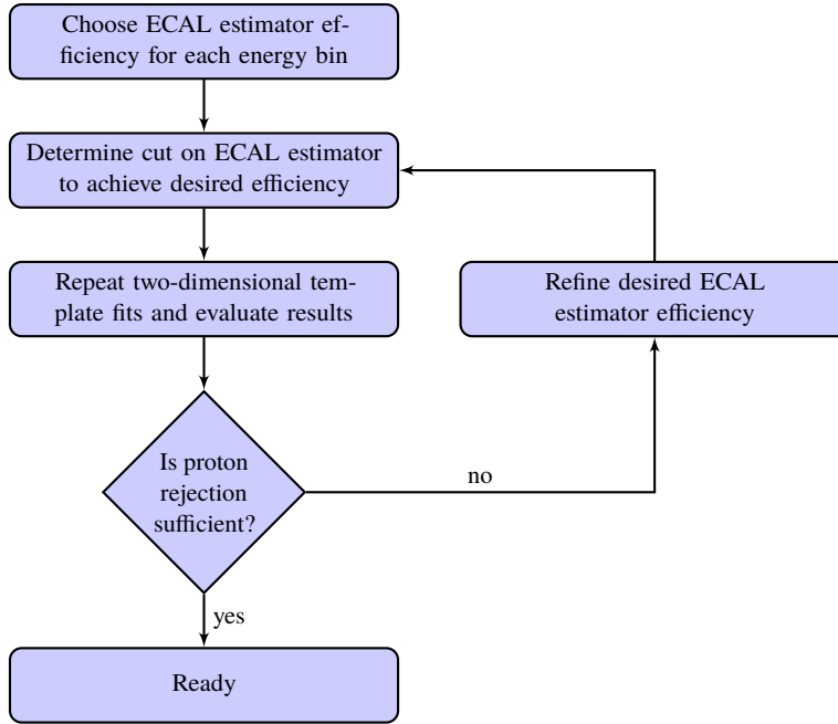
Figure 4.44: Illustration of the iterative procedure used to determine the ECAL estimator cut value / efficiency.
