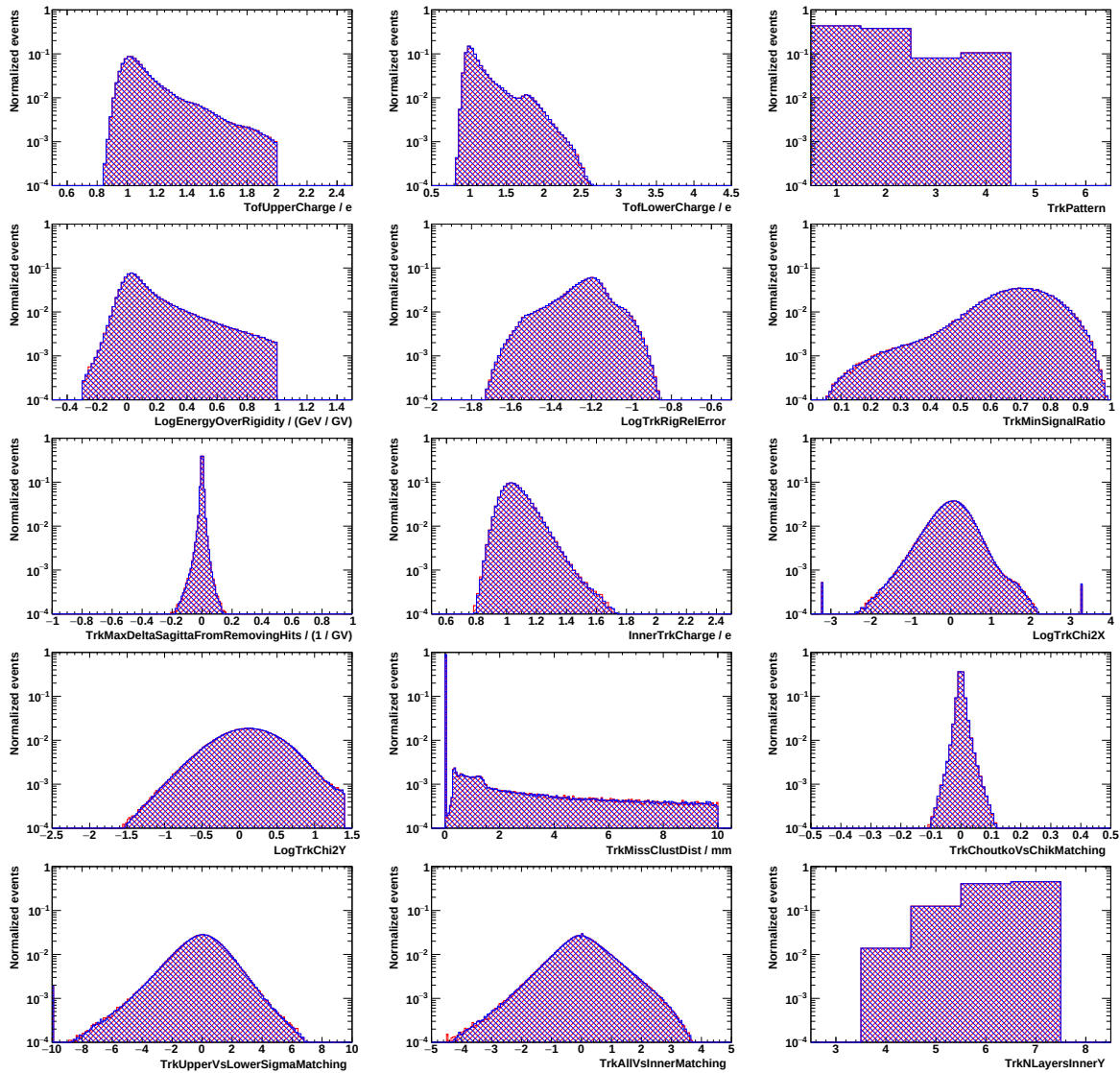
Figure A.13: Comparison of all 15 CCMVA input variables for the single-track sample between the positron Monte-Carlo simulation (red) and the electron Monte-Carlo simulation (blue) in the energy bin 17.98 – 18.99 GeV.
