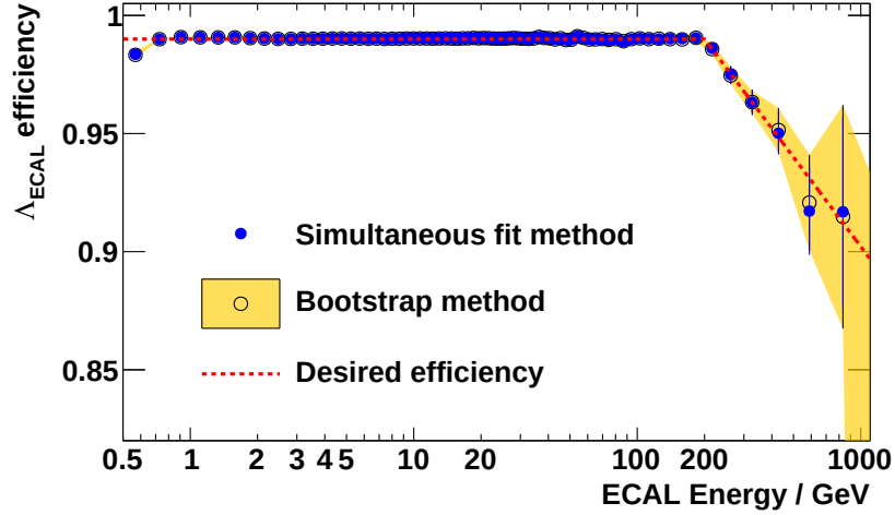
Figure 4.47: Final result showing the ECAL estimator efficiency \epsilon_{\text{ecal}}(E) as function of energy derived using two different methods. The dashed red line represents the desired ECAL estimator efficiency and the blue symbols the actual efficiency in each energy bin, determined by a simultaneous fit on the passed/failed data sample. The black open symbols belong to the efficiency determined by the bootstrap method and the orange band represents the associated uncertainty.
