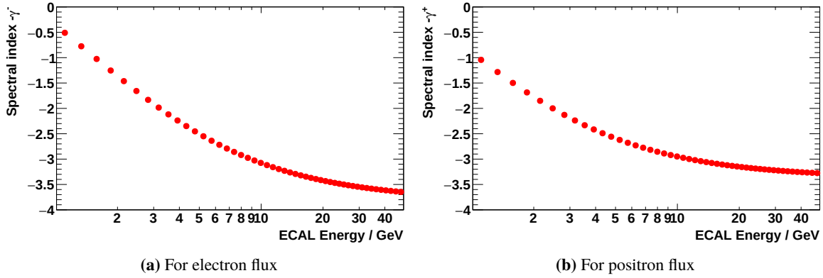
Figure 4.111: Spectral index of the electron flux (left plot) and the positron flux (right plot), determined via the computation of the spectral derivative, Eq. (4.38), using the flux model - Eq. (4.37) - for the time-dependent e^\pm flux in Bartels rotation i = 26 (Apr 16 th , 2013 - May 13 th , 2013), after unfolding. Note that the y-axis shows -\gamma_i^\pm : by convention \gamma_i^\pm is positive.
