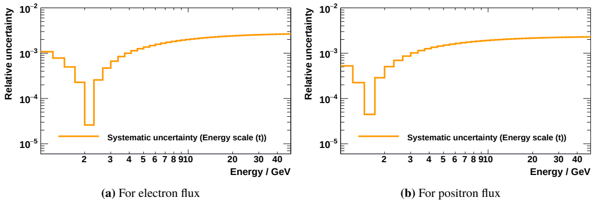
Figure 4.112: Visualization of the relative systematic uncertainty associated with the electron flux (left plot) and the positron flux (right plot) due to the time-stability of the energy scale, in an example Bartels rotation i = 26 (Apr 16 th , 2013 - May 13 th , 2013).
