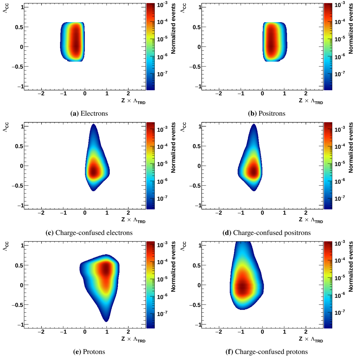
Figure A.20: Two-dimensional TRD / CCMVA templates in the energy bin 17.98 – 18.99 GeV for the multi-tracks sample.
