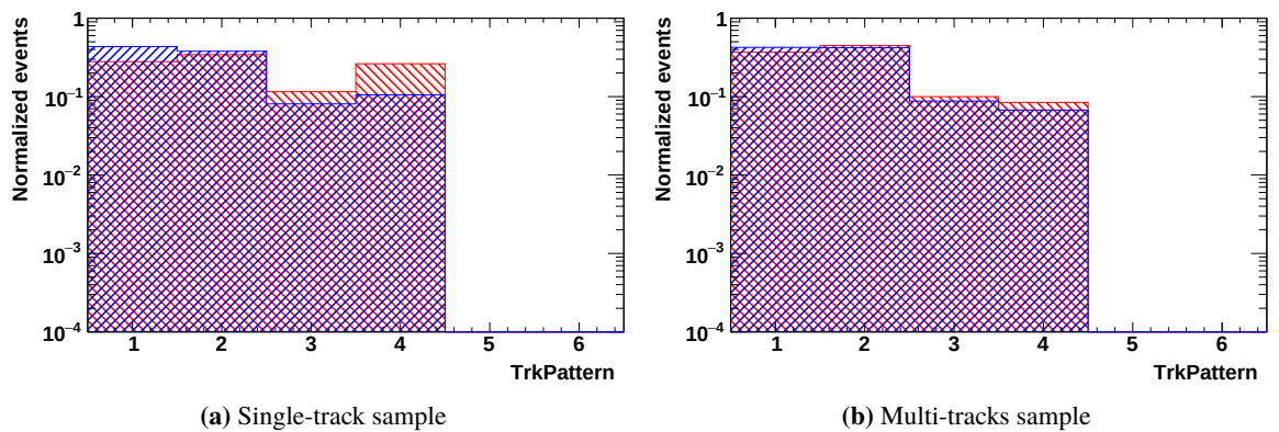
Figure A.6: Example of TrkPattern distribution in the energy bin 17.98 – 18.99 GeV in the electron Monte-Carlo simulation.
