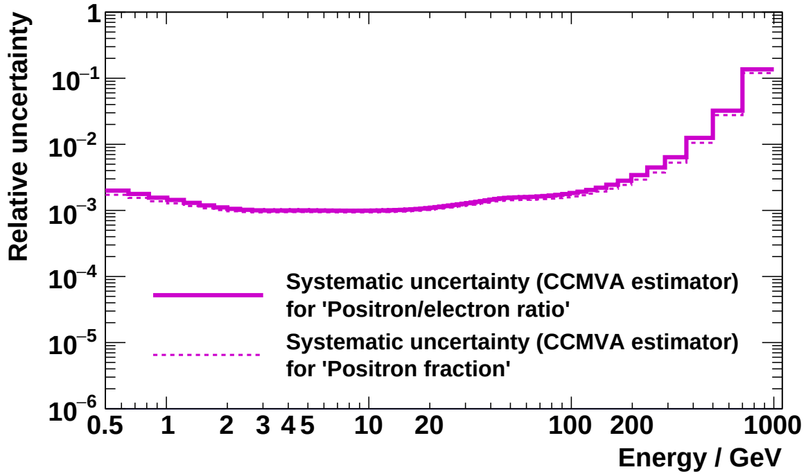
Figure 4.89: Visualization of the relative systematic uncertainty associated with the positron/electron ratio and the positron fraction due to the knowledge of the charge-confusion.
