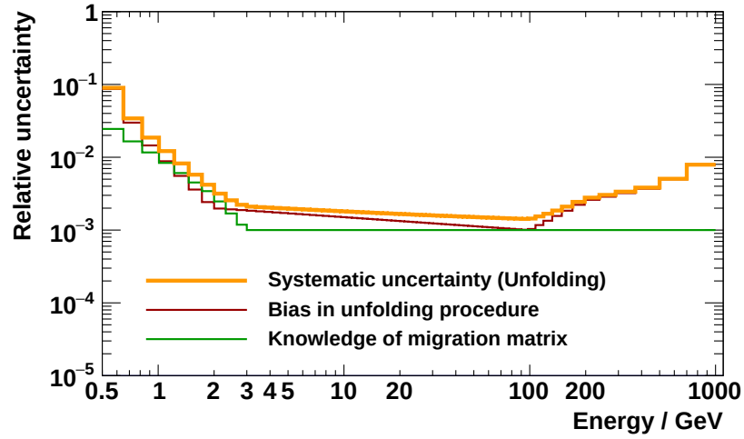
Figure 4.87: Visualization of the relative systematic uncertainty associated with the positron/electron ratio and the positron fraction due to unfolding.
