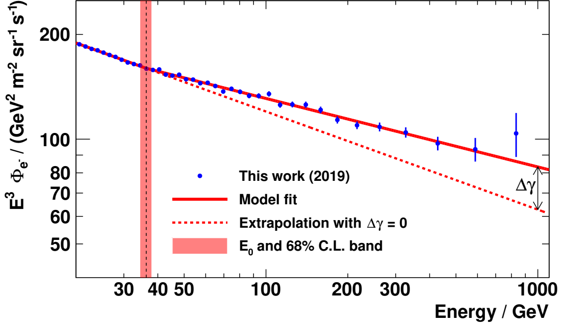
Figure 5.5: Fit of the double power law approximation Eq. (5.1) to the electron flux in the range 21.13 – 1,000 GeV. The electron flux is shown as blue data points, scaled by E^3 . The red line corresponds to the fit result of Eq. (5.1). The vertical dashed line indicates the transition energy E_0 and the red band corresponds to the uncertainty. The red dashed line corresponds to an extrapolation of the model, with \Delta\gamma = 0 .
