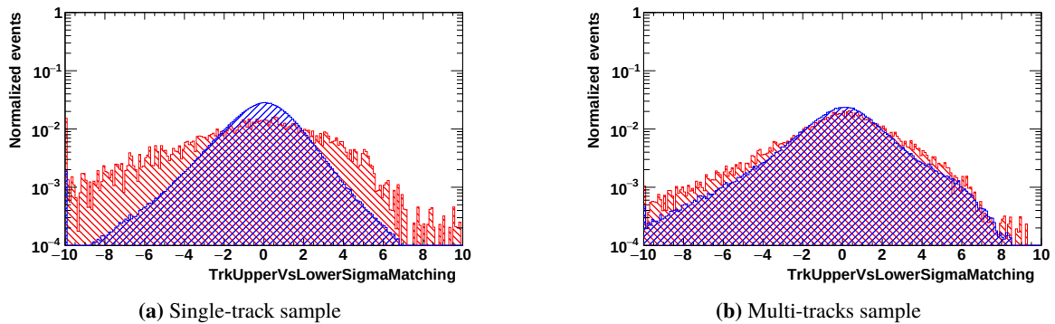
Figure A.8: Example of TrkUpperVsLowerSigmaMatching distribution in the energy bin 17.98 – 18.99 GeV in the electron Monte-Carlo simulation.
