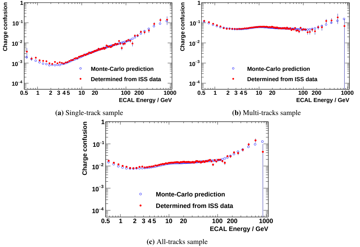
Figure 4.41: Comparison of the amount of charge-confusion determined from ISS data with the prediction from the Monte-Carlo simulation for the single-track sample, the multi-tracks sample and the all-tracks sample.
