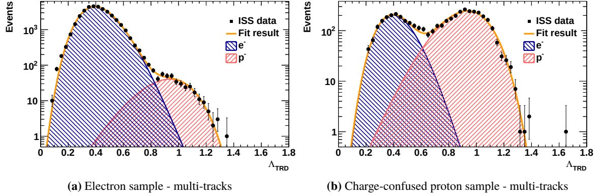
Figure 4.24: Simultaneous fit of the electron template Eq. (4.6) and the charge-confused proton template Eq. (4.7) in the energy bin 17.98 – 18.99 GeV for the multi-tracks sample. The dark blue area corresponds to the electron template, the light red area to the charge-confused proton template and the orange line to the sum of all templates.
