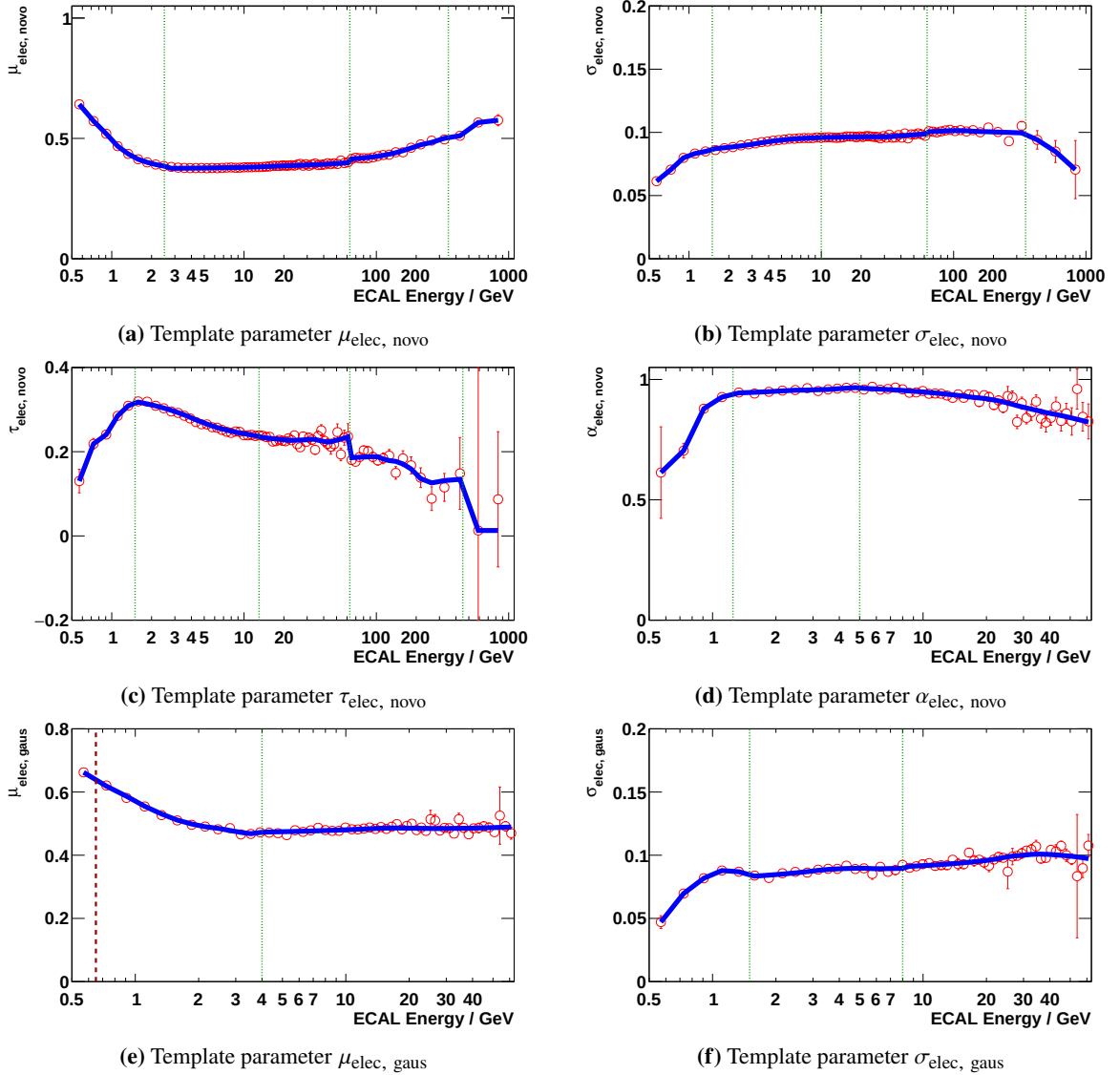
Figure 4.27: Analytical TRD template parameters describing the evolution of the electron template as function of energy for the single-track sample. In each energy bin the analytical function - Eq. (4.6) - is fit to the template data sample, yielding the red points. A smoothing procedure yields the blue curves, which are used as template parameters for the analysis. The vertical dashed green lines mark areas where different isolated smoothing procedures are applied. The vertical dashed red lines mark energies where the smoothing procedure starts – points before this border are preserved.
