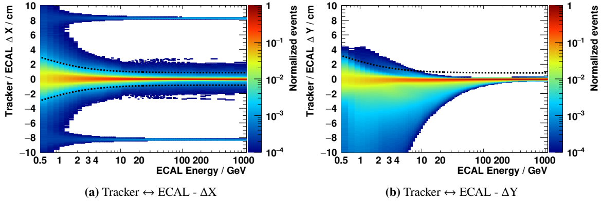
Figure 4.20: Plot of the \Delta X (left) and \Delta Y (right) between the tracker track extrapolation and the ECAL shower centre of gravity as function of energy for the electron Monte-Carlo simulation. The applied lower and upper cut values are shown as black dashed lines.
