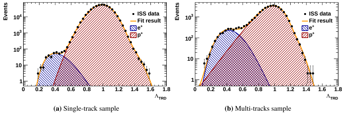
Figure 4.25: Fit of the proton template Eq. (4.8) in the energy bin 17.98 – 18.99 GeV for the single-track sample and the multi-tracks sample. The dark blue area corresponds to the electron template, the light red area to the charge-confused proton template and the orange line to the sum of all templates.
