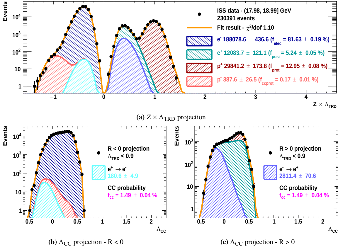
Figure 4.40: Results of the two-dimensional TRD / CCMVA template fit in the energy bin 17.98 – 18.99 GeV for the all-tracks sample drawn as stacked histograms.
