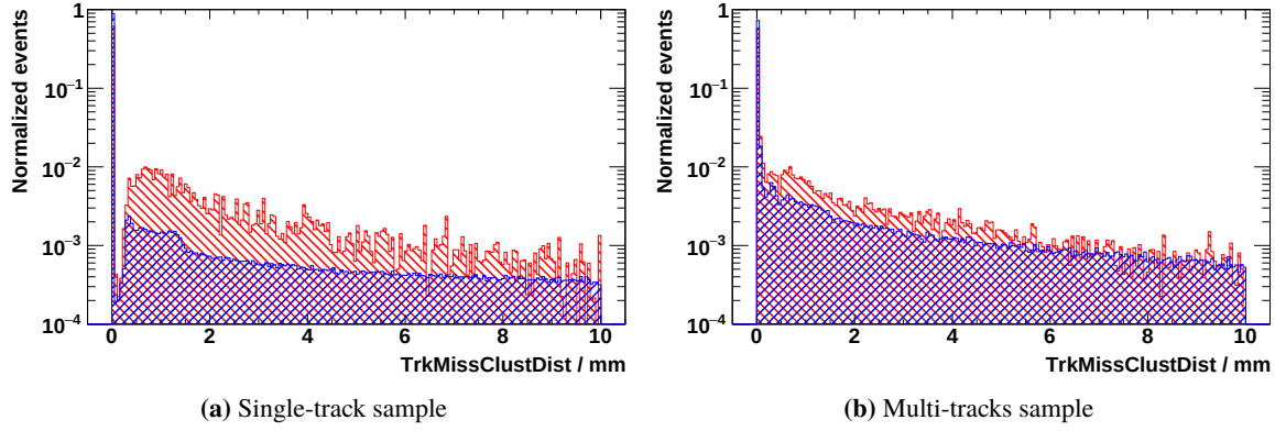
Figure A.4: Example of TrkMissClustDist distribution in the energy bin 17.98 – 18.99 GeV in the electron Monte-Carlo simulation.
