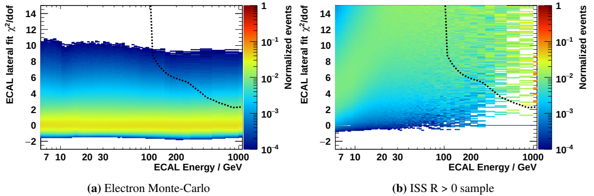
Figure 4.19: Plot of the ECAL lateral goodness-of-fit distribution as function of energy for the electron Monte-Carlo simulation (left) and the ISS R > 0 sample (right). The applied upper cut value is shown as black dashed line.
