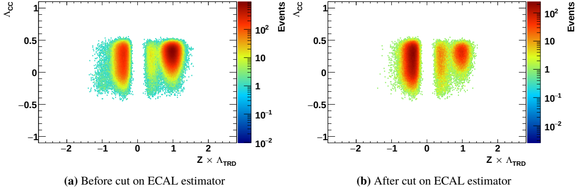
Figure 4.35: ISS data distribution in the energy bin 17.98 – 18.99 GeV for the single-track sample, as example, before and after applying a cut on the ECAL estimator to reduce the proton background.
