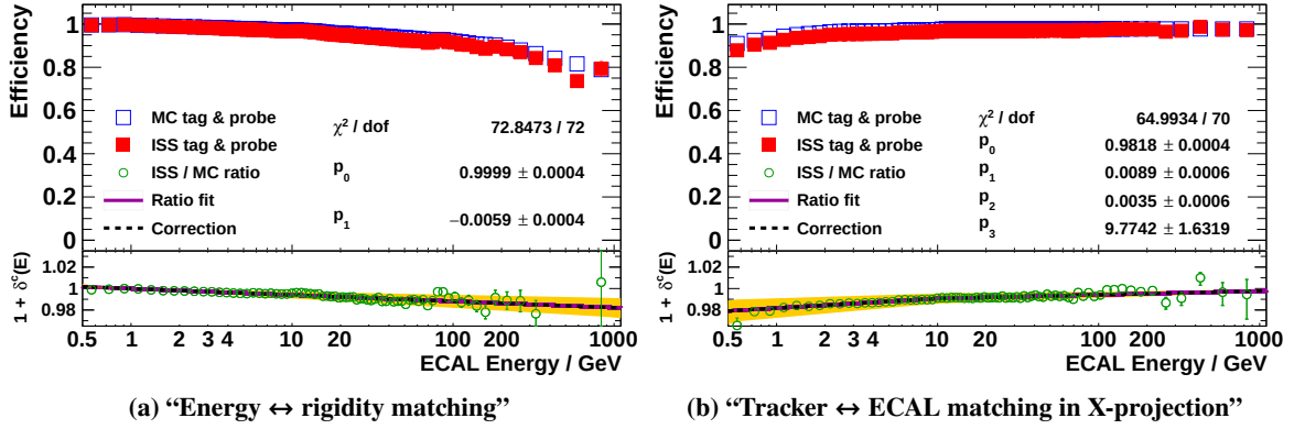
Figure 4.58: Determination of the Data/Monte-Carlo correction factors ( 1 + \delta^c(E) ) for the e^\pm identification cuts: “Energy \leftrightarrow rigidity matching” (left) and “Tracker \leftrightarrow ECAL matching in X-projection” (right) (Section 4.3.4 - Items 1 and 3). The open blue symbols in the upper plots show the cut efficiency determined on the electron Monte-Carlo simulation on a dedicated sample: the tag sample. The filled red symbols in the upper plots show the cut efficiency determined from ISS data using the same tag cuts. The lower plots show the ratio ISS efficiency over MC efficiency as open green symbols. Equation (4.23) is fit to the left ratio, Eq. (4.24) is fit to the right ratio, represented as magenta lines. The dashed black lines show that half of the deviation from unity is taken as correction to the Monte-Carlo acceptance A_e^{\text{MC}}(E) . The associated systematic uncertainty is visualized by the orange bands.
