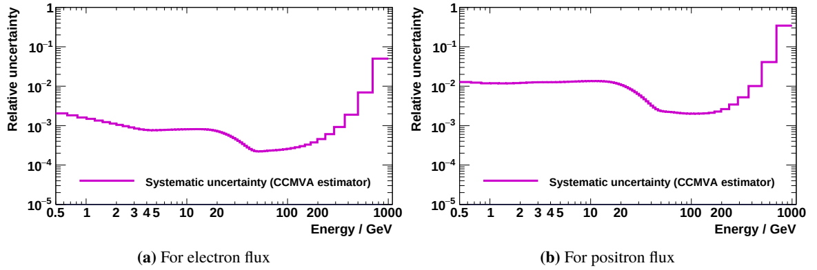
Figure 4.68: Visualization of the relative systematic uncertainty associated with the electron flux (left plot) and associated with the positron flux (right plot) due to the knowledge of the charge-confusion.
