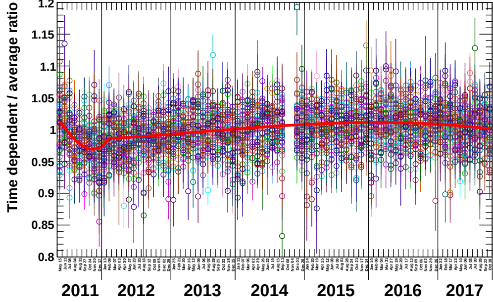
Figure A.24: Time-dependence of the \mu_{\text{ccprot, novo}} parameter for selected energy bins (1.22 – 52.33 GeV), as example, in the time-dependent analysis for the multi-tracks sample.
