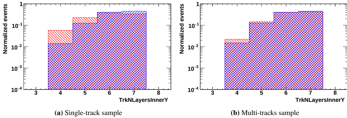
Figure A.10: Example of TrkNLayersInnerY distribution in the energy bin 17.98 – 18.99 GeV in the electron Monte-Carlo simulation.
