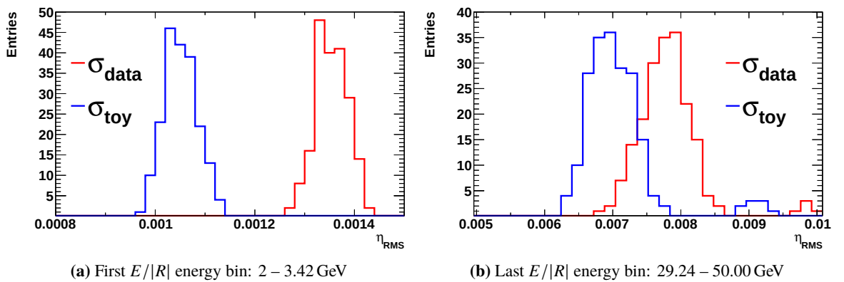
Figure 4.109: \eta_{\text{RMS}} distribution for the ISS data sample and the Toy-MC sample . The mean of the distributions is denoted as \sigma_{\text{data}} and \sigma_{\text{toy}} , respectively.
