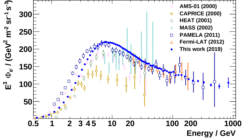
Figure 5.2: Comparison of the electron flux derived in this work with other experiments: AMS-01 [Alcaraz2000], CAPRICE [Boezio2000], HEAT [DuVernois2001], MASS [Grimani2002], PAMELA [Adriani2011] and Fermi-LAT [Ackermann2012].
