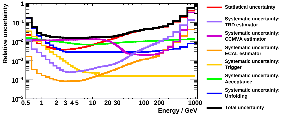
Figure 4.86: Composition of the relative systematic uncertainty associated with the positron flux.
