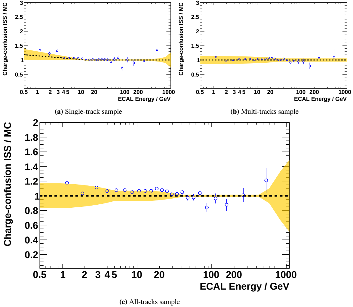
Figure 4.67: Comparison of the ratio of charge-confusion determined from ISS data divided by the prediction from the Monte-Carlo simulation (blue symbols) for the single-track sample, the multi-tracks sample and the all-tracks sample. The orange band represents the chosen systematic uncertainty to cover the differences between the ISS data and the Monte-Carlo simulation.
