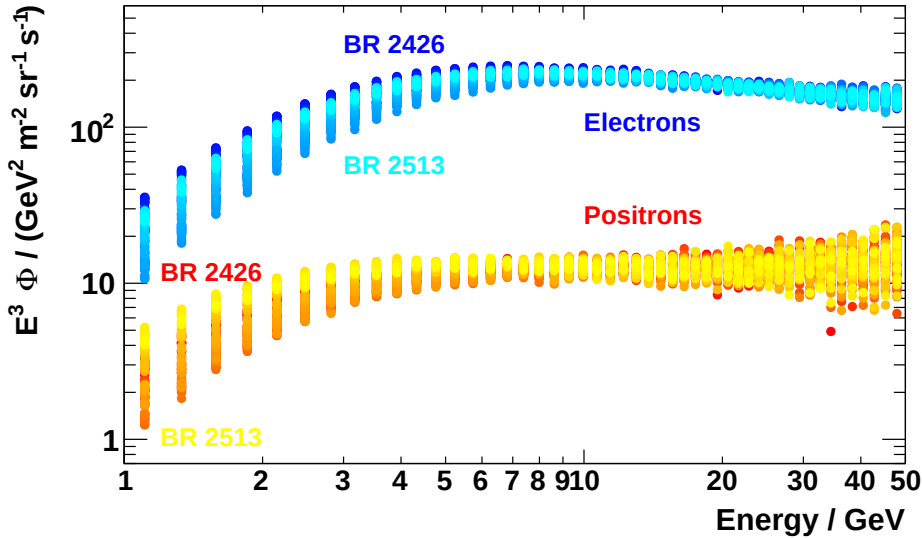
Figure 5.17: The electron / positron fluxes for each Bartels rotation analyzed in this work. The error bars on the individual flux points were omitted for clarity.
