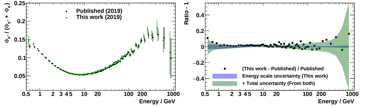
Figure B.9: Comparison of the positron fraction derived in this work with the recent AMS-02 positron fraction publication [Aguilar2019b]. To ease the comparison the published data points are shifted horizontally by 5 %. Within the quoted systematic uncertainties the results are compatible.
