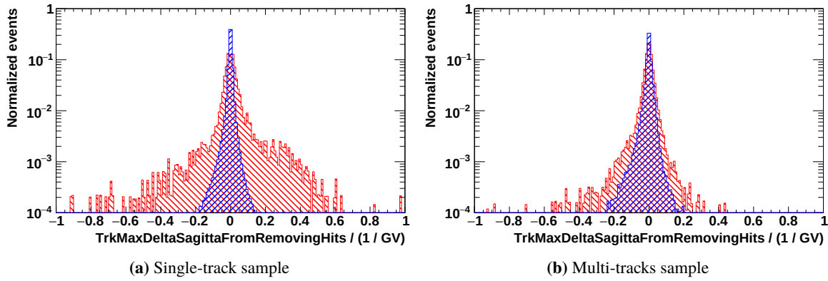
Figure 4.3: Example of \text{TrkMaxDeltaSagittaFromRemovingHits} distribution in the energy bin 17.98 – 18.99 GeV in the electron Monte-Carlo simulation. The red histogram shows the charge-confused sample ( R > 0 ) and the blue histogram the correct reconstructed sample ( R < 0 ), after applying all preselection, selection and e^\pm identification cuts.
