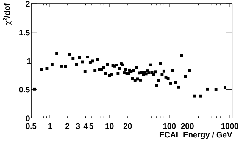
Figure 4.28: Goodness of fit of the model Eq. (4.6) with respect to the template data in the single-track sample. The black points show the \chi^2/\text{dof} as function of energy. The result is consistent with 1 for all energies for the single-track sample.
