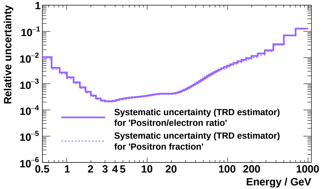
Figure 4.90: Visualization of the relative systematic uncertainty associated with the positron/electron ratio and the positron fraction due to the knowledge of the TRD estimator.
