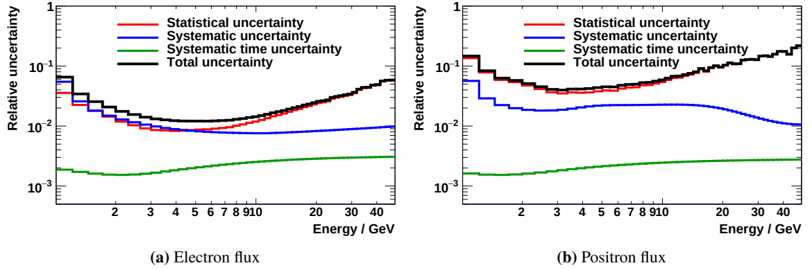
Figure 5.18: Breakdown of the uncertainty of the electron flux (left) and the positron flux (right) into a statistical and systematic part, in an example Bartels rotation i = 26 (Apr 16 th , 2013 - May 13 th , 2013).
