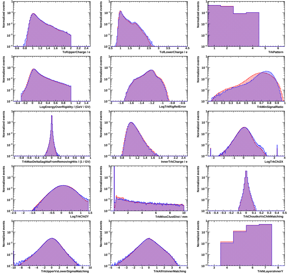
Figure A.16: Comparison of all 15 CCMVA input variables for the single-track sample between the ISS data (blue) and the electron Monte-Carlo (red) in the energy bin 17.98 – 18.99 GeV. There are no visible differences in all variables except TrkMinSignalRatio, except for small fluctuations in the tails, proving the consistency of the input quantities between ISS data and simulation. The whole comparison was performed on a negative rigidity sample, as it is impossible to select pure samples of electrons with wrong reconstructed rigidity on ISS data.
