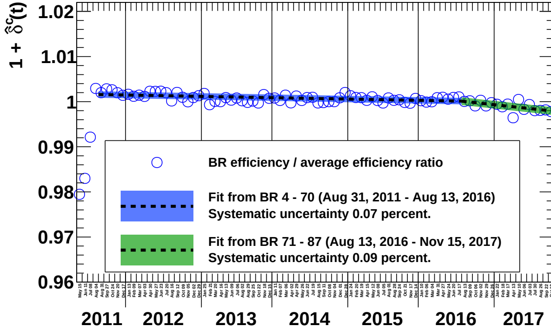
Figure 4.95: Determination of the time-dependent correction factor ( 1 + \hat{\delta}^c(t) ) for the selection cut: “ Tracker hit pattern ” (Section 4.3.3 - Item 5). The open blue symbols show the ratio: time-dependent cut efficiency over time-averaged cut efficiency for all Bartels rotations (an example of the ratio determined in a single Bartels rotation is shown in Fig. 4.93). The black dashed lines show regions parameterized using straight lines. When the efficiency remains stable over an extended period of time, following a simple trend (e.g. slowly decreasing or constant) a parameterization of the time period is used instead of the individual data points to describe the time dependency. The colored bands indicate the systematic uncertainty on the time-dependent correction factor ( 1 + \hat{\delta}^c(t) ). For individual data points, the uncertainty on the data point - from the previous ratio fit procedure - is taken.
