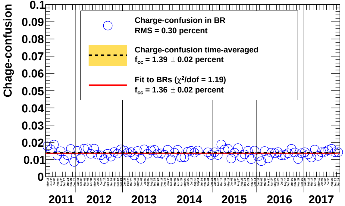
Figure A.21: Time-dependent charge-confusion for the energy bin 9.62 – 10.32 GeV. The x-axis spans 88 Bartels rotations and each bin label denotes the date when the Bartels rotation started (in UTC). The blue symbols show the charge-confusion for the all-tracks sample in the specific energy bin as function of time. The black dashed line shows the time-averaged charge-confusion for comparison. The red line shows a fit of a constant to the red symbols, yielding an acceptable \chi^2/\text{dof} = 1.19 value.
