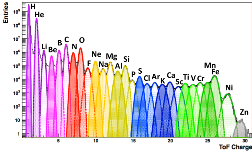
Figure 3.8: The charge distribution measured by the TOF, from Z = 1 (protons) up to Z = 30 (Zinc). Credit: Ref. [ AmsWebsite ]
