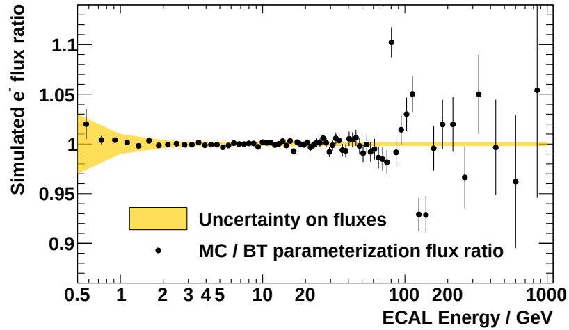
Figure 4.75: Ratio of the toy e^- flux forward folded with the Monte-Carlo parameterization over the toy e^- flux forward-folded with the testbeam parameterization - shown as black symbols. The orange band represents the systematic uncertainty on the fluxes due to the knowledge of the migration matrix.
