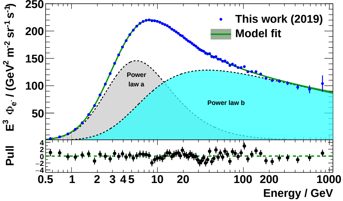
Figure 5.6: The electron flux, scaled with E^3 , is shown as blue points. The result of the fit of Eq. (5.2) is shown as green line, enclosed by a green band, indicating the uncertainty of the fit result. The two power law components a and b are indicated by the gray and turquoise areas, respectively. The lower plot shows the pull distribution of the fit (data minus model divided by data uncertainty) – the model describes the data accurately over the whole energy range.
