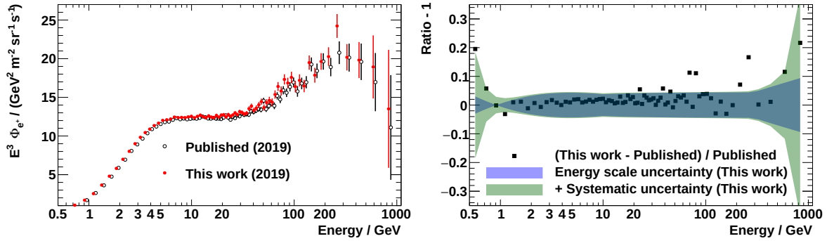
Figure B.4: Comparison of the positron flux derived in this work with the recent AMS-02 positron flux publication [Aguilar2019b]. To ease the comparison the published data points are shifted horizontally by 5 %. Within the quoted systematic uncertainties the results are compatible.
