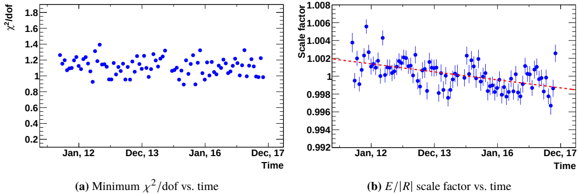
Figure 4.107: Results of the \chi^2 scan procedure in the first E/|R| energy bin ( 2 - 3.42 GeV) as function of time. The left plot shows the minimum \chi^2/\text{dof} as function of time and the right plot the obtained scale factor S_i for each Bartels rotation i .
