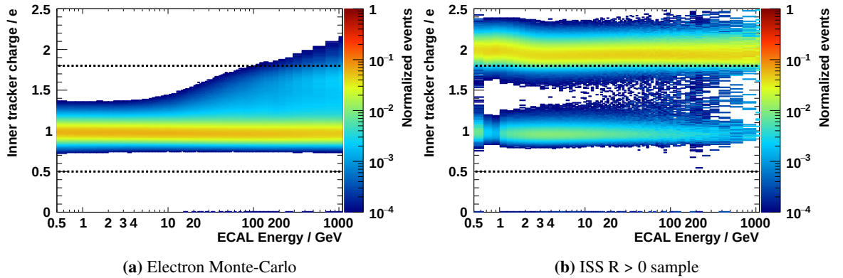
Figure 4.16: Plot of the charge measurement in the inner tracker as function of energy for the electron Monte-Carlo simulation (left) and the ISS R > 0 sample (right). The applied lower and upper cut values are shown as black dashed lines.
