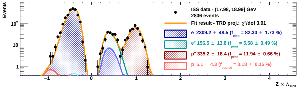
Figure 4.104: Results of the two-dimensional TRD / CCMVA template fit in Bartels rotation i = 6 for the energy bin 17.98 – 18.99 GeV (all-tracks sample) using the time-averaged TRD templates.
