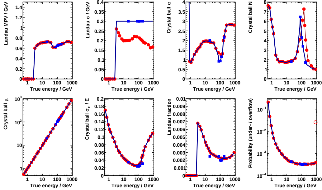
Figure 4.74: Results of the fit of the analytical model - Eq. (4.26) - to all bins in y-direction (true energy) of the migration matrix obtained from the Monte-Carlo simulation (red symbols), compared to the analytical model fit to the migration matrices obtained from the mono-energetic testbeam data sets (blue symbols). The testbeam data sets that were analyzed are e^+ at 20 and 80 GeV, e^- at 100, 120 and 180 GeV, yielding five different migration matrices. The analytical model is fit to all five migration matrices and the parameters are extracted, shown as blue symbols. The testbeam results can be compared to the prediction from the Monte-Carlo simulation: Three parameters show a significant deviation: the Landau \sigma , the Crystal Ball \alpha and N parameters. The dark blue line marks the extrapolation of the parameters obtained from the discrete test beam data points towards the whole energy range.
