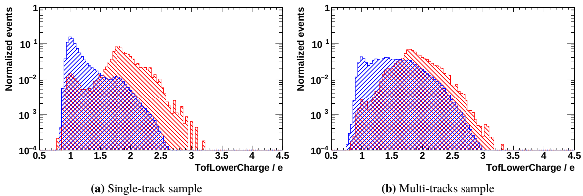
Figure 4.1: Example of TofLowerCharge distribution in the energy bin 17.98 – 18.99 GeV in the electron Monte-Carlo simulation. The red histogram shows the charge-confused sample ( R > 0 ) and the blue histogram the correct reconstructed sample ( R < 0 ), after applying all preselection, selection and e^\pm identification cuts.
