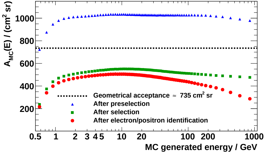
Figure 4.54: Determination of the acceptance A_{e^\pm}^{\text{MC}}(E) from the electron Monte-Carlo simulation as function of the generated energy of the simulated particles. The black dashed line shows the geometrical acceptance A_{\text{geom}} . The other symbols show the acceptance after applying the preselection, selection and e^\pm identification cuts. The acceptance after applying only the preselection cuts is higher than the geometrical acceptance, since in the preselection tracker requirements are not imposed yet, unlike in the definition of the geometrical acceptance. After applying the selection cuts, the acceptance curve is smaller than the geometrical acceptance.
