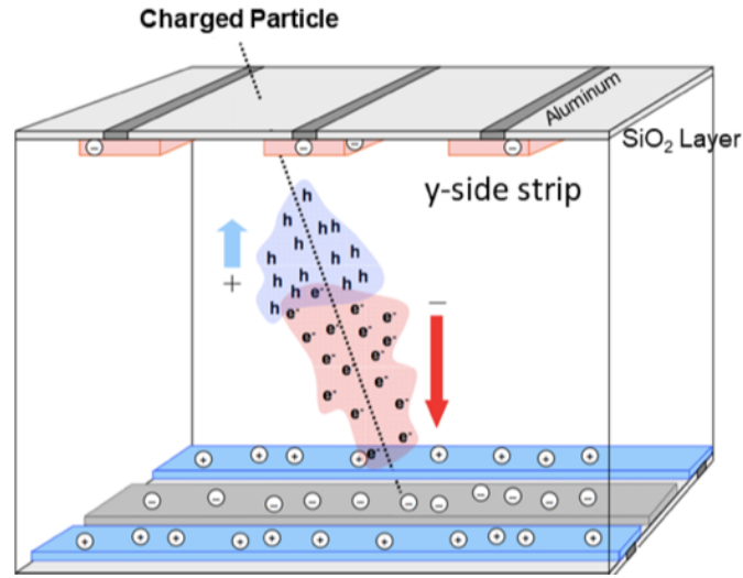
Figure 3.4: Schematic of the measurement principle of the “S side” silicon sensor. Credit: Ref. [AmsWebsite]
