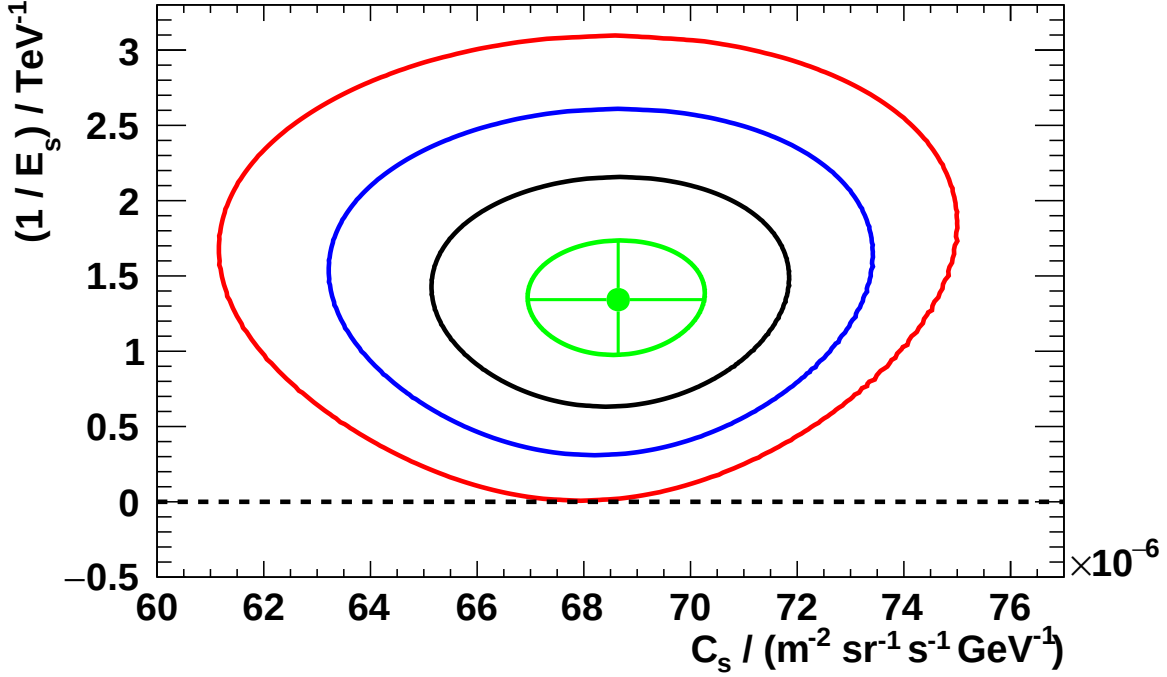
Figure 5.14: The contour plot between the C_s and 1/E_s parameters shows that the cut-off significance is established with 4\sigma . The regions corresponding to 1\sigma up to 4\sigma are drawn in green (68.26 % C.L.), black (95.54 % C.L.), blue (99.74 % C.L.) and red (99.99 % C.L.), respectively.
