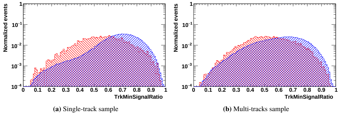
Figure A.3: Example of \text{TrkMinSignalRatio} distribution in the energy bin 17.98 – 18.99 GeV in the electron Monte-Carlo simulation.
