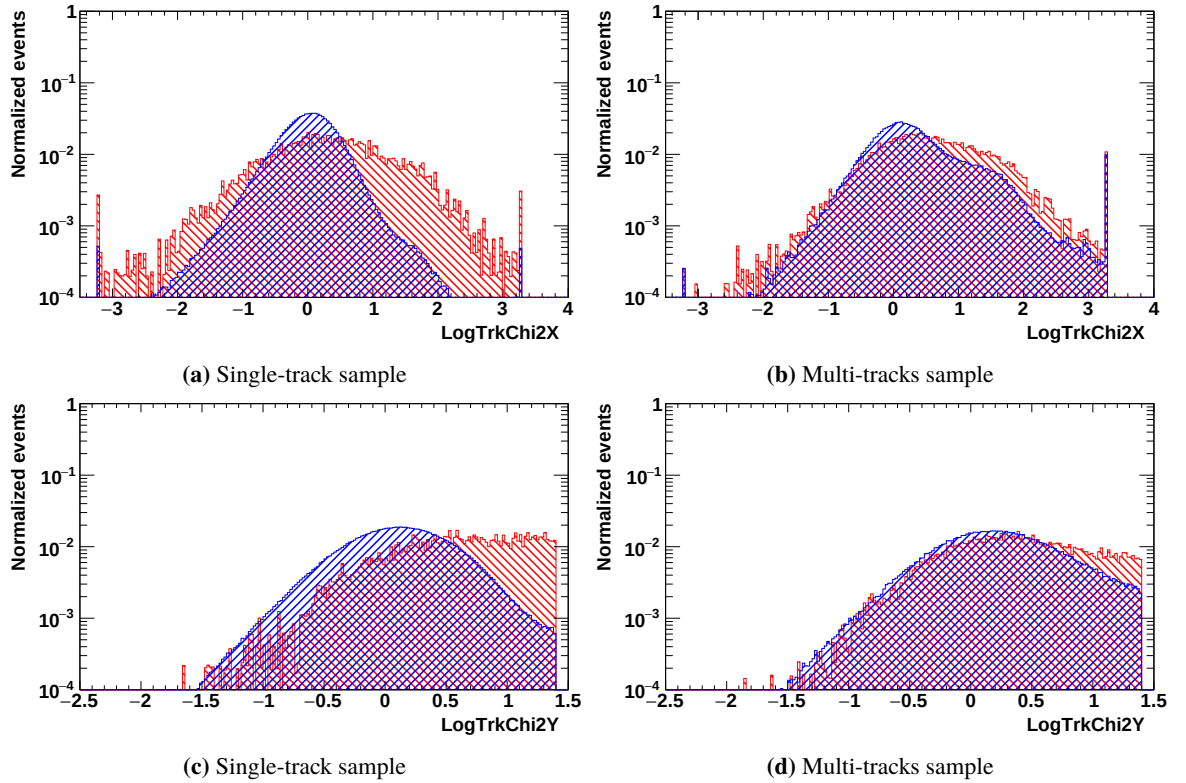
Figure 4.5: Example of LogTrkChi2X / LogTrkChi2Y distribution in the energy bin 17.98 – 18.99 GeV in the electron Monte-Carlo simulation. The red histogram shows the charge-confused sample ( R > 0 ) and the blue histogram the correct reconstructed sample ( R < 0 ), after applying all preselection, selection and e^\pm identification cuts.
