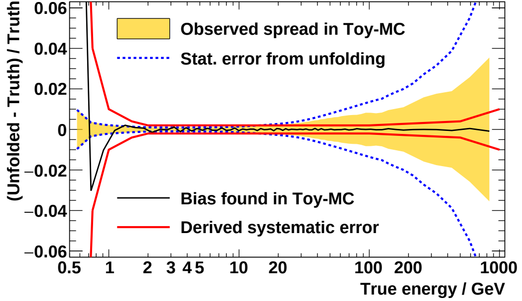
Figure 4.80: Visualization of the bias of the unfolding procedure for the e^- flux, extracted from the gaussian fits of Fig. 4.79, as function of the true energy. The black line shows the bias of the unfolded flux with respect to the true flux. The red line shows the associated systematic error, which by construction encloses the black line. The blue line shows the statistical uncertainty of the unfolded flux and the orange band the observed spread from the toy Monte-Carlo simulation - corresponding to the width of the gaussians in Fig. 4.79.
