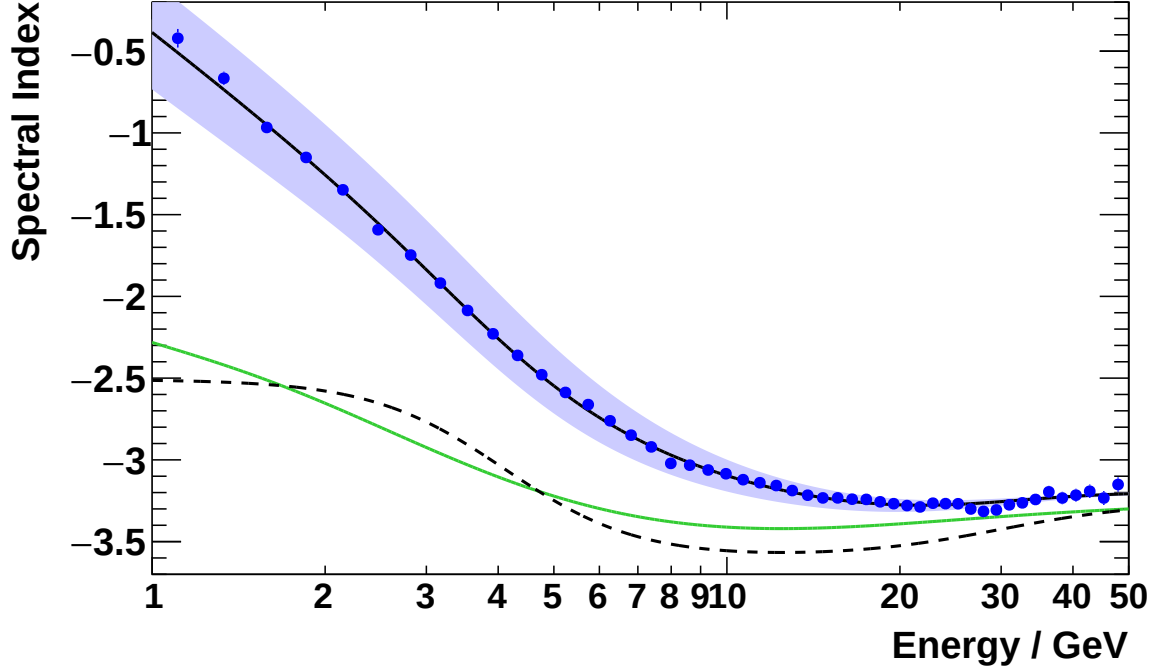
Figure B.15: Energy dependence of the electron spectral index \gamma^-(E) = d(\log \Phi_{e^-}(E))/d(\log E) obtained in a model independent way (see Section 5.1.1) from the time averaged data and the spectral index obtained from the model described in Ref. [Cavazonza2017] fitted to the time-averaged electron flux data (solid black curve). The shaded band indicates the time-variation. The spectral index from this model without solar modulation (dashed black curve) clearly shows a break in the spectral index between 2 – 10 GeV. A recent model describing the local interstellar electron spectrum [Potgieter2015] is also shown (green curve).
