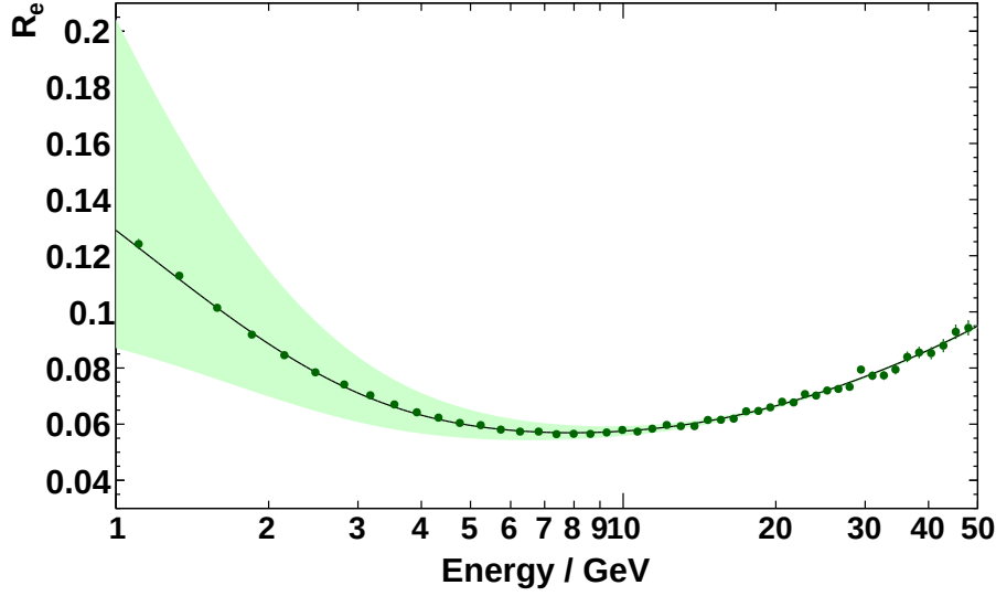
Figure 5.22: Visualization of the time-averaged positron/electron ratio R_e . The time-variation range is indicated by the shaded regions, see text. The fit of the model in Refs. [Corti2016; Cavasonza2017] to the time-averaged data points is shown by the black curves.
