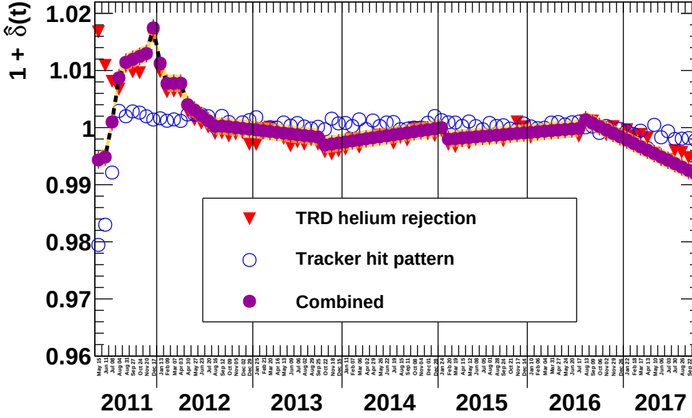
Figure 4.97: Determination of the time-dependent correction factor ( 1 + \hat{\delta}(t) ). The red triangle symbols show the correction factor for the “ TRD helium rejection ” cut and the blue circle symbols show the correction factor for the “ Tracker hit pattern ” cut. The combined correction factor is shown as magenta symbols. The uncertainty is shown as orange band on top of the magenta symbols.
