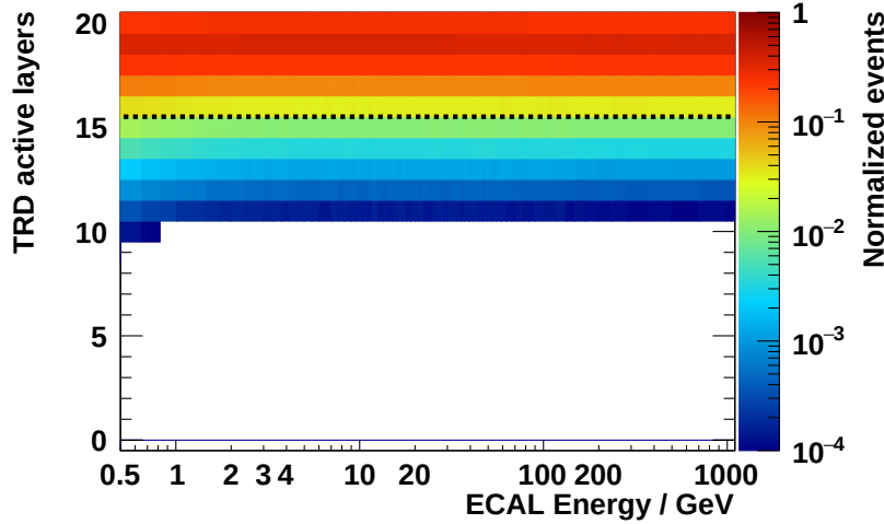
Figure 4.14: Plot of the active layers in the TRD as function of energy for the electron Monte-Carlo simulation. The applied lower cut value is shown as black dashed line.
