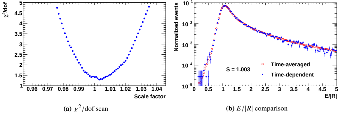
Figure 4.106: Control plots of the \chi^2 scan procedure in the first E/|R| energy bin ( 2 - 3.42 GeV) to determine the best matching scale factor S , in an example Bartels rotation, that leads to agreement between the time-dependent and the time-averaged E/|R| distribution.
