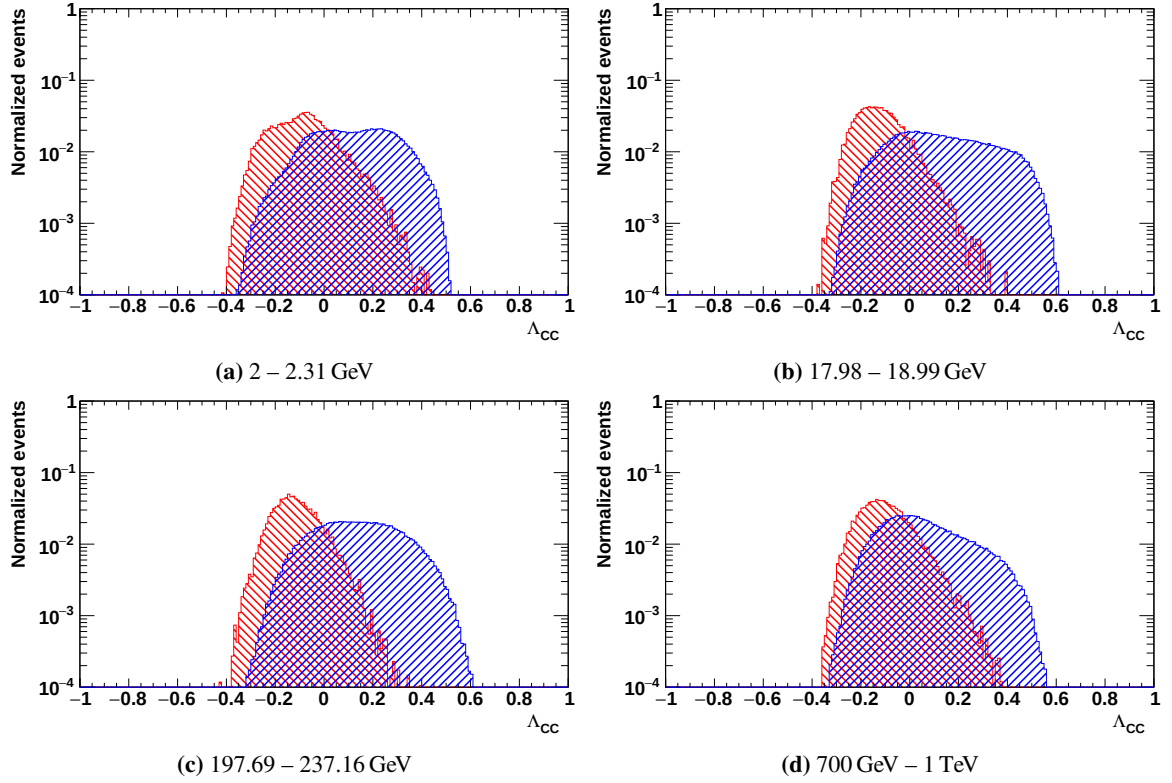
Figure 4.9: Overview of the CCMVA estimator in the multi-tracks sample in four different energy intervals, from low energies to the highest energy in this analysis.
