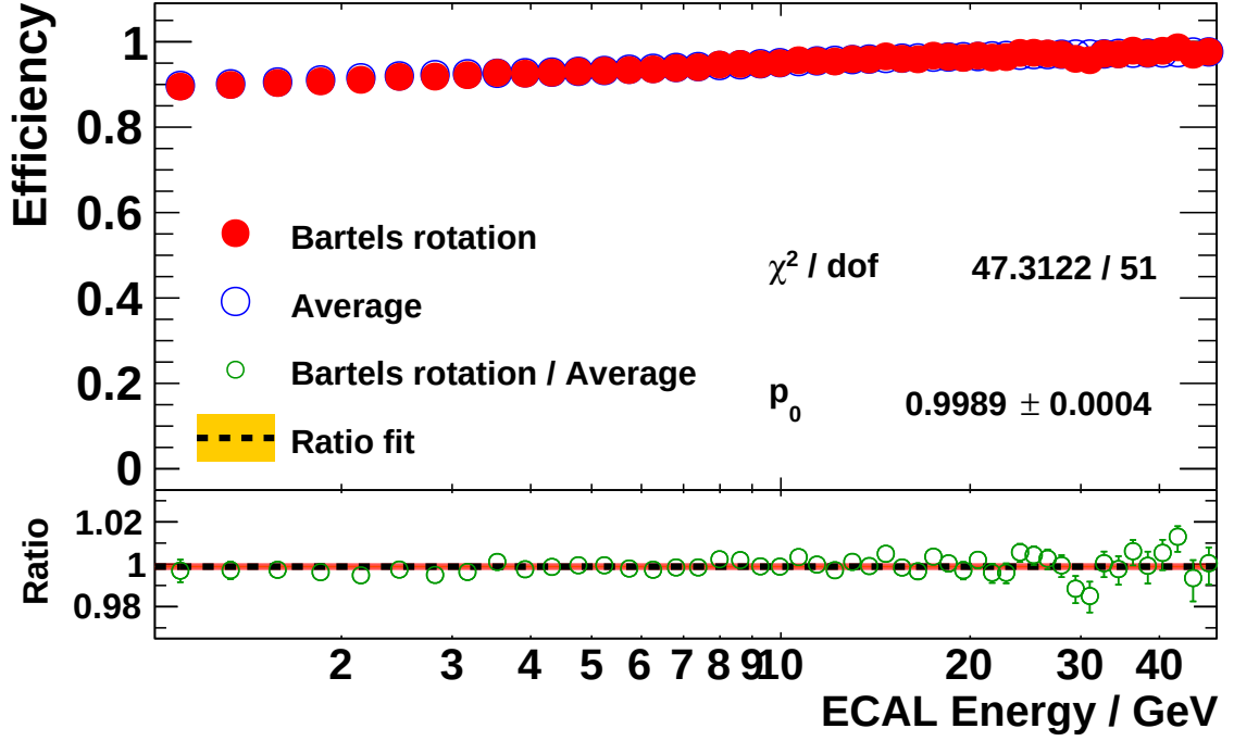
Figure 4.94: Determination of the ratio: time-averaged cut efficiency ( 1 + \delta^c(E) ) over time-dependent cut efficiency ( 1 + \delta_i^c(E) ) in Bartels rotation i = 26 (Apr 16 th , 2013 - May 13 th , 2013) for the selection cut: “TRD helium rejection” (Section 4.3.3 - Item 4). The blue symbols in the upper plot show the cut efficiency determined from ISS data for the time-averaged analysis on a dedicated sample: the tag sample. The red symbols in the upper plot show the cut efficiency determined from ISS data in Bartels rotation i = 26 using the same tag cuts. The lower plot shows the ratio time-averaged efficiency over efficiency in Bartels rotation i = 26 as green symbols. A constant is fit to the ratio, shown as dashed black line including the orange uncertainty band.
