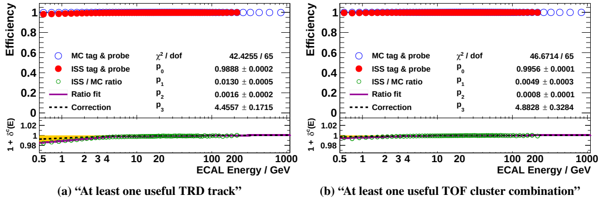
Figure 4.55: Determination of the Data/Monte-Carlo correction factors ( 1 + \delta^c(E) ) for the preselection cuts: “At least one useful TRD track” (left) and “At least one useful TOF cluster combination” (right) (Section 4.3.2 - Items 2 and 3). The open blue symbols in the upper plots show the cut efficiency determined on the electron Monte-Carlo simulation on a dedicated sample: the tag sample. The filled red symbols in the upper plots show the cut efficiency determined from ISS data using the same tag cuts. The lower plots show the ratio ISS efficiency over MC efficiency as open green symbols. Equation (4.24) is fit to the ratios, represented as magenta lines. The dashed black lines show that half of the deviation from unity is taken as correction to the Monte-Carlo acceptance A_e^{\text{MC}}(E) . The associated systematic uncertainty is visualized by the orange bands.
