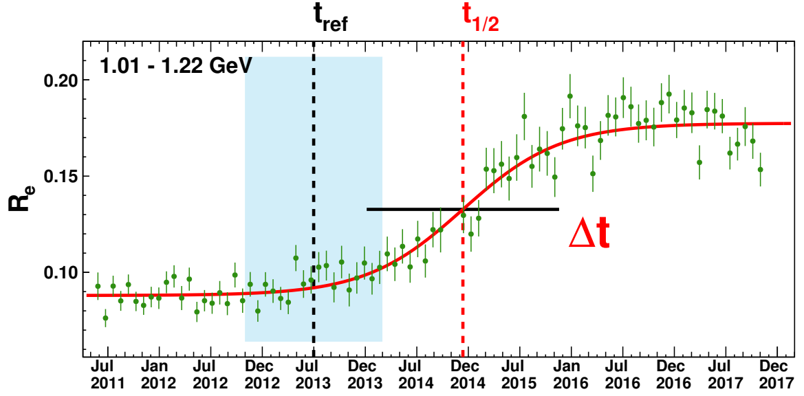
Figure 5.26: Illustration of the parameters in Eqs. (5.5) and (5.6) describing the time and energy dependence of R_e , using two energy bins from Fig. 5.23 as examples. The best-fit parameterizations according to Eq. (5.5) are shown by red curves. The period without well-defined polarity is marked by the shaded area [Sun2015]. The choice for the effective time of the reversal of the solar magnetic field t_{\text{rev}} is marked by black dashed vertical lines. The fit results for the midpoint of the transition t_{1/2} are marked by red dashed vertical lines. The value of t_{1/2} is found to be energy dependent. The width of the red horizontal bars indicate the duration of the transition \Delta t , which is found to be independent of energy at 682 \pm 27 days. It takes time \Delta t for the transition to proceed from 10% to 90% of the change in magnitude.
