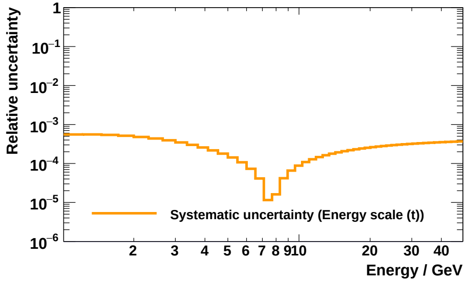
Figure 4.114: Visualization of the relative systematic uncertainty associated with the positron/electron ratio due to the time-stability of the energy scale, in an example Bartels rotation i = 26 (Apr 16 th , 2013 - May 13 th , 2013).
