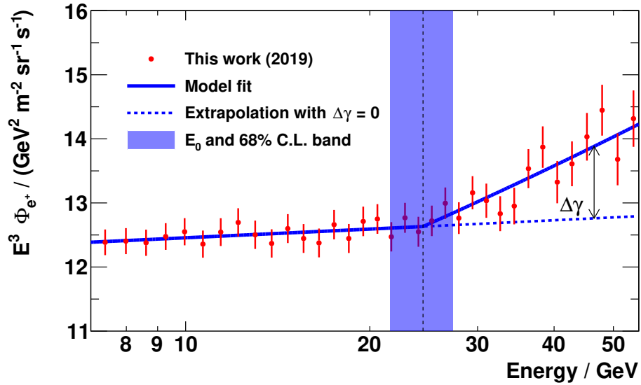
Figure 5.11: Fit of the double power law approximation Eq. (5.3) to the positron flux in the range 7.10 – 55.58 GeV. The positron flux is shown as red data points, scaled by E^3 . The blue line corresponds to the fit result of Eq. (5.3). The vertical dashed line indicates the transition energy E_0 , where the positron flux starts rising, and the blue band corresponds to the uncertainty. The blue dashed line corresponds to an extrapolation of the model, with \Delta\gamma = 0 .
