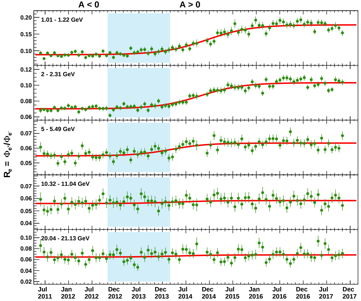
Figure 5.23: The ratio R_e of the positron flux to the electron flux as a function of time. The error bars are statistical. The best-fit parametrization according to Eq. (5.5) is shown by red curves. The polarity of the heliospheric magnetic field is denoted by A < 0 and A > 0 . The period without well-defined polarity is marked by the shaded area [Sun2015].
