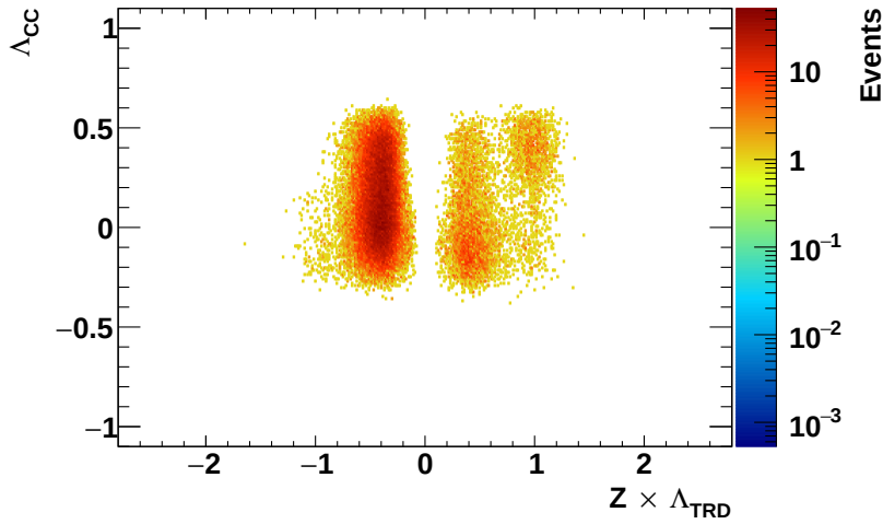
Figure 4.38: ISS data distribution in the energy bin 17.98 – 18.99 GeV for the multi-tracks sample, after applying a cut on the ECAL estimator to reduce the proton background.
