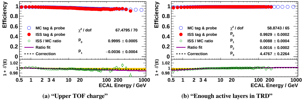
Figure 4.56: Determination of the Data/Monte-Carlo correction factors (1 + \delta^c(E)) for the selection cuts: “Upper TOF charge” (left) and “Enough active layers in TRD” (right) (Section 4.3.3 - Items 2 and 3). The open blue symbols in the upper plots show the cut efficiency determined on the electron Monte-Carlo simulation on a dedicated sample: the tag sample. The filled red symbols in the upper plots show the cut efficiency determined from ISS data using the same tag cuts. The lower plots show the ratio ISS efficiency over MC efficiency as open green symbols. Equation (4.23) is fit to the left ratio, Eq. (4.24) is fit to the right ratio, represented as magenta lines. The dashed black lines show that half of the deviation from unity is taken as correction to the Monte-Carlo acceptance A_e^{\text{MC}}(E) . The associated systematic uncertainty is visualized by the orange bands.
