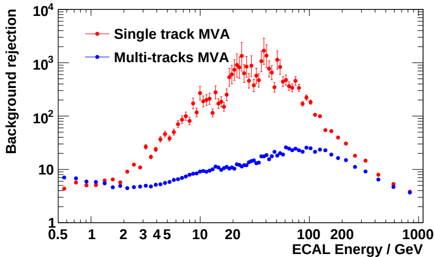
Figure 4.11: Rejection of the CCMVA estimator as function of energy. The background rejection exceeds 10^2 in the energy range 10 – 100 GeV, when choosing a fixed signal efficiency of 70 %.
