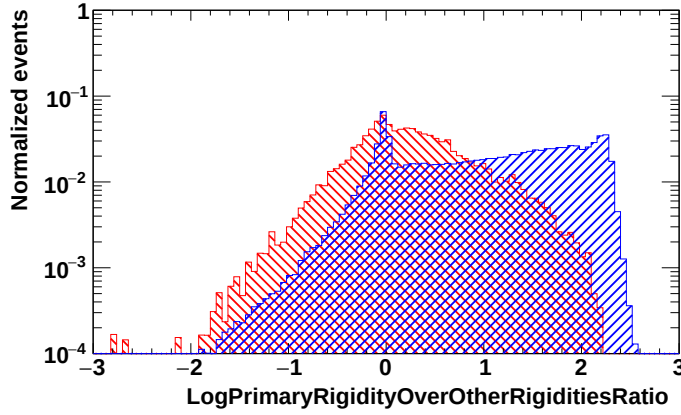
Figure 4.6: Example of LogPrimaryRigidityOverOtherRigiditiesRatio distribution in the energy bin 17.98 – 18.99 GeV in the electron Monte-Carlo simulation. The red histogram shows the charge-confused sample ( R > 0 ) and the blue histogram the correct reconstructed sample ( R < 0 ), after applying all preselection, selection and e^\pm identification cuts.
