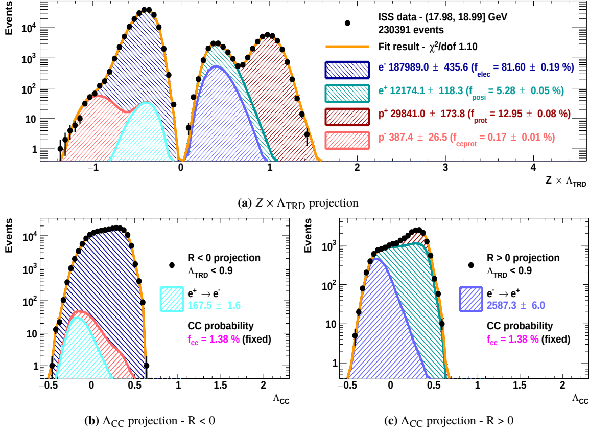
Figure 4.42: Results of the two-dimensional TRD / CCMVA template fit in the energy bin 17.98 – 18.99 GeV for the all-tracks sample drawn as stacked histograms with the amount of charge-confusion fixed by the prediction from the Monte-Carlo simulation.
