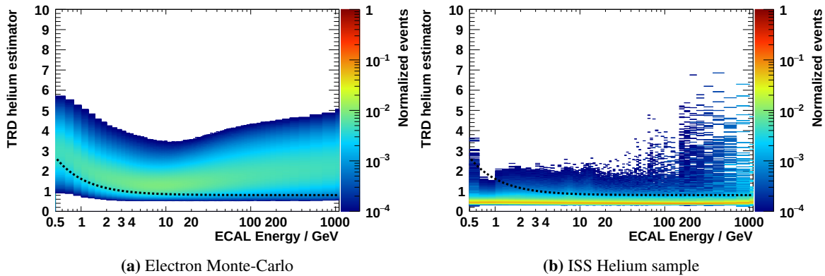
Figure 4.15: Plot of the TRD likelihood estimator \mathcal{L}_{e^-/\text{He}} as function of energy for the electron Monte-Carlo simulation (left) and the ISS Helium sample (right). The applied lower cut value is shown as black dashed line.
