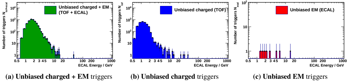
Figure 4.49: Distribution of the unbiased triggers as function of energy. The most abundant unbiased triggers are the Unbiased charged + Unbiased EM triggers, followed by the Unbiased charged triggers. The least abundant triggers are the Unbiased EM triggers.
