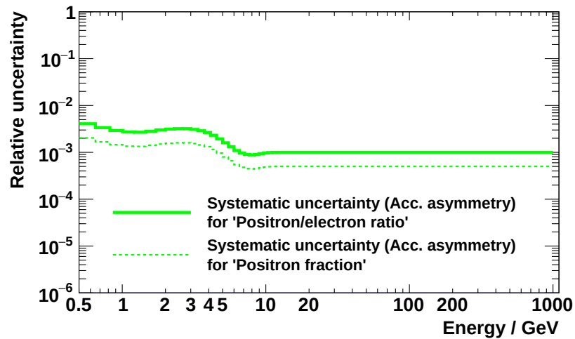
Figure 4.88: Visualization of the relative systematic uncertainty associated with the positron/electron ratio and the positron fraction due to the acceptance asymmetry between e^- / e^+ .
