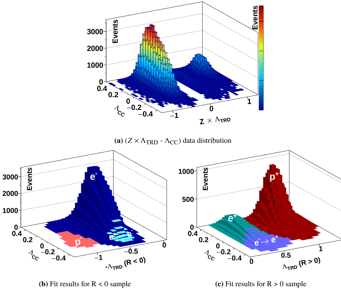
Figure 4.36: ISS data distribution in the energy bin 17.98 – 18.99 GeV for the single-track sample as three-dimensional plot (top) along with the results of the fit procedure, split in two parts: one plot showing the fit results in the negative rigidity sample (lower left) and another plot showing the fit results in the positive rigidity sample (lower right).
