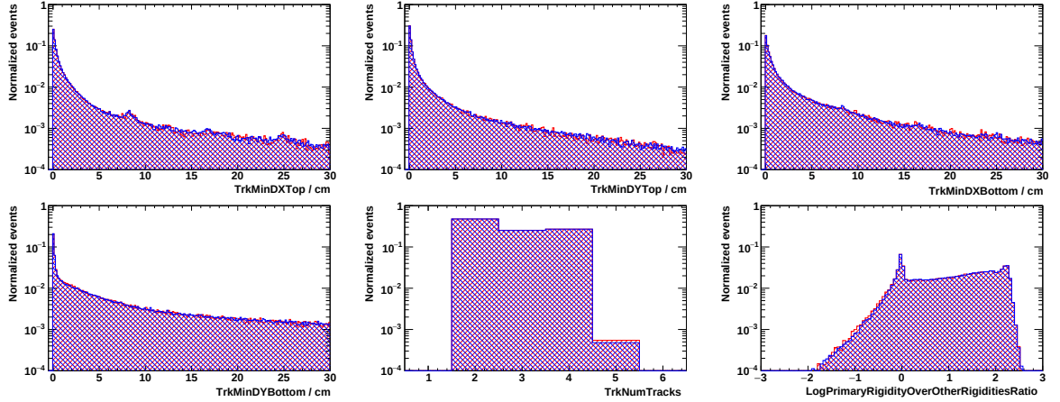
Figure A.14: Comparison of the six multi-tracks sample specific CCMVA input variables between the positron Monte-Carlo simulation (red) and the electron Monte-Carlo simulation (blue) in the energy bin 17.98 – 18.99 GeV. There are no visible differences, except for small fluctuations in the tails, proving the consistency of the input quantities between electron and positrons.
