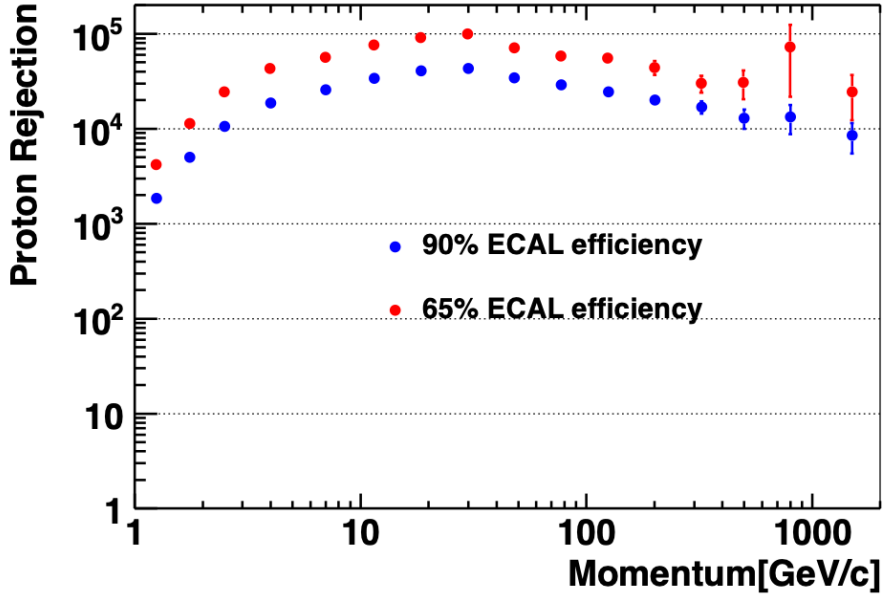
Figure 3.14: Proton rejection of the ECAL as function of the e^\pm momentum. Credit: Ref. [AmsWebsite]
