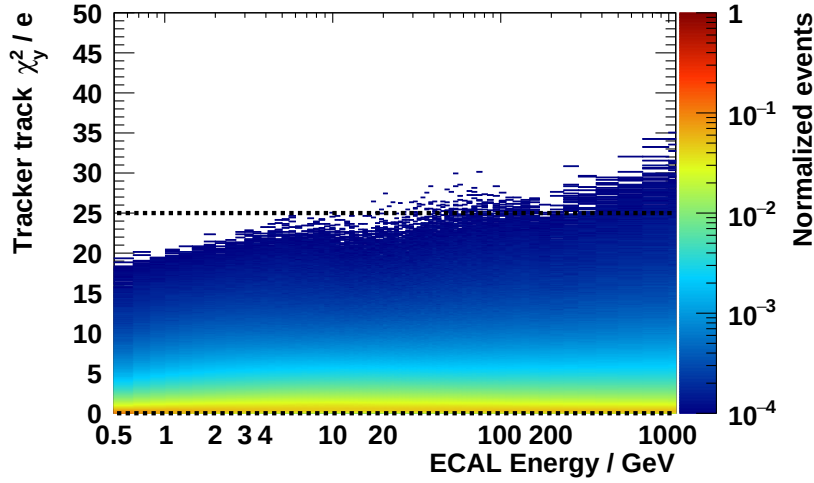
Figure 4.17: Plot of the tracker track goodness-of-fit \chi_y^2 as function of energy for the electron Monte-Carlo simulation. The applied lower and upper cut values are shown as black dashed lines.
