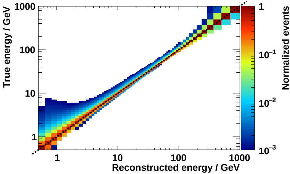
Figure 4.62: Migration matrix \mathbf{M} obtained from the electron Monte-Carlo simulation, using the same binning as the flux analysis.
