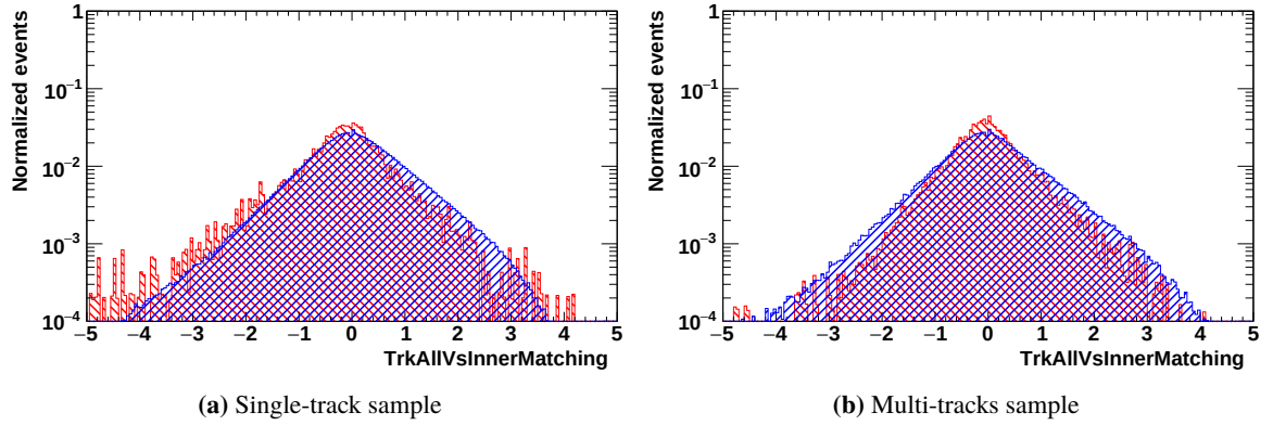
Figure A.9: Example of TrkAllVsInnerMatching distribution in the energy bin 17.98 – 18.99 GeV in the electron Monte-Carlo simulation.
