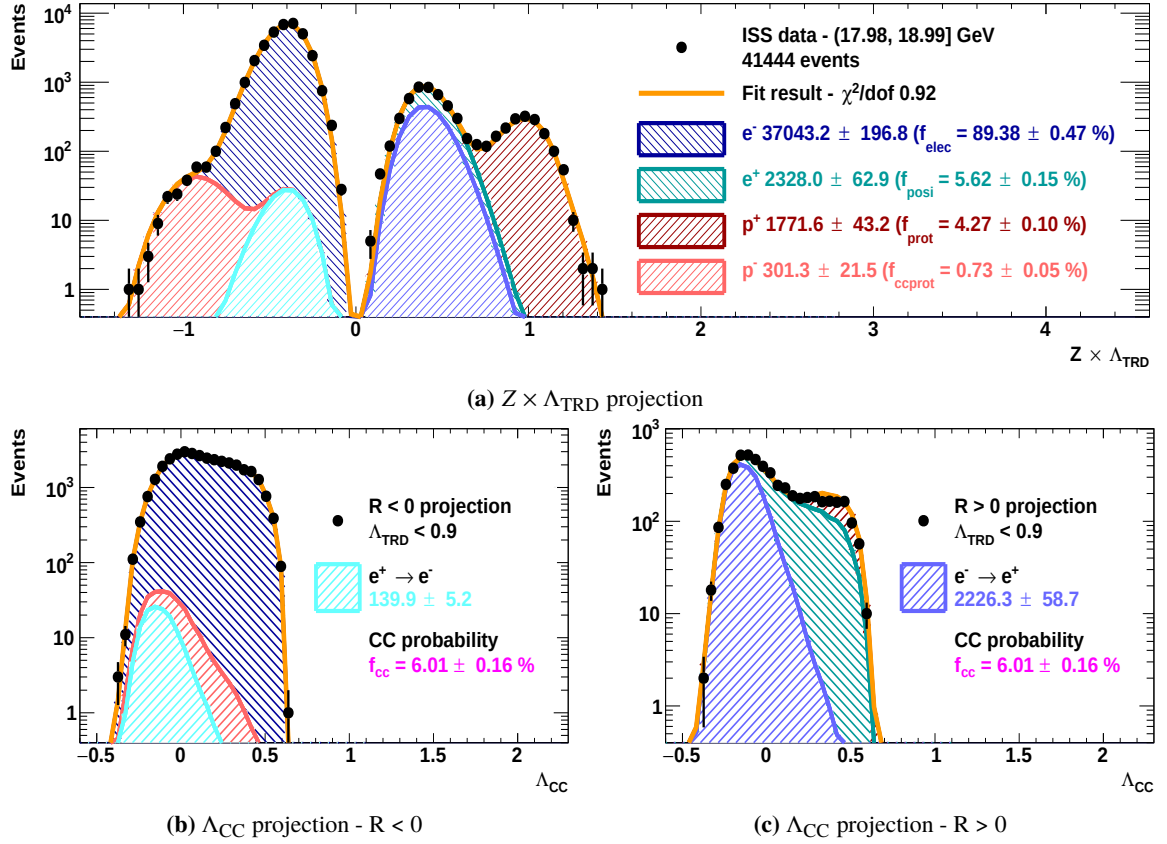
Figure 4.39: Results of the two-dimensional TRD / CCMVA template fit in the energy bin 17.98 – 18.99 GeV for the multi-tracks sample drawn as stacked histograms. The upper panel shows the projection of the two-dimensional fit to the x-axis. The lower left panel shows the projection to the y-axis, containing only events with R < 0 . In this plot electrons , charge-confused positrons and charge-confused protons are visible. The lower right panel shows the projection to the y-axis, containing only events with R > 0 . In this plot positrons , charge-confused electrons and protons are visible.
