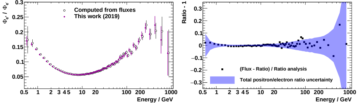
Figure B.11: Comparison of the positron/electron ratio derived using the single-track analysis with the ratio computed from the fluxes, that were derived from the all-track analysis. To ease the comparison the all-track analysis data points are shifted horizontally by 5 %. Within the quoted systematic uncertainties the results are compatible.
