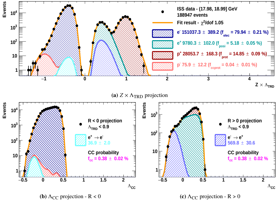
Figure 4.37: Results of the two-dimensional TRD / CCMVA template fit in the energy bin 17.98 – 18.99 GeV for the single-track sample drawn as stacked histograms. The upper panel shows the projection of the two-dimensional fit to the x-axis. The lower left panel shows the projection to the y-axis, containing only events with R < 0 . In this plot electrons , charge-confused positrons and charge-confused protons are visible. The lower right panel shows the projection to the y-axis, containing only events with R > 0 . In this plot positrons , charge-confused electrons and protons are visible.
