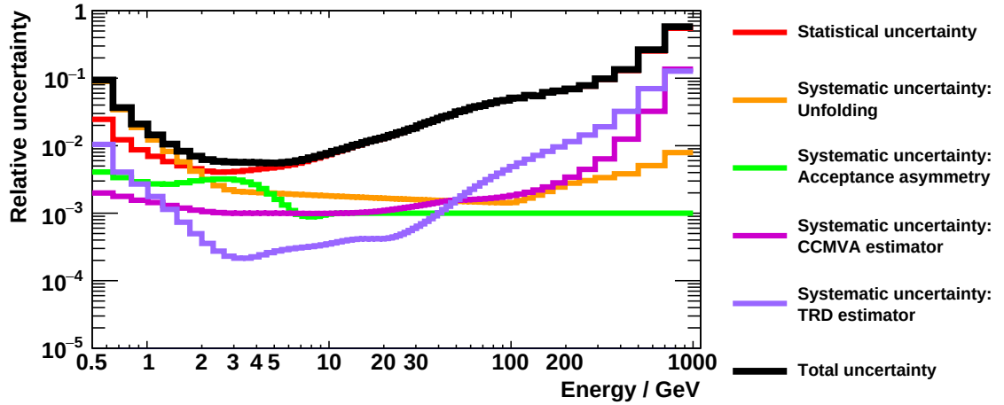
Figure 4.91: Composition of the relative systematic uncertainty associated with the positron/electron ratio.
