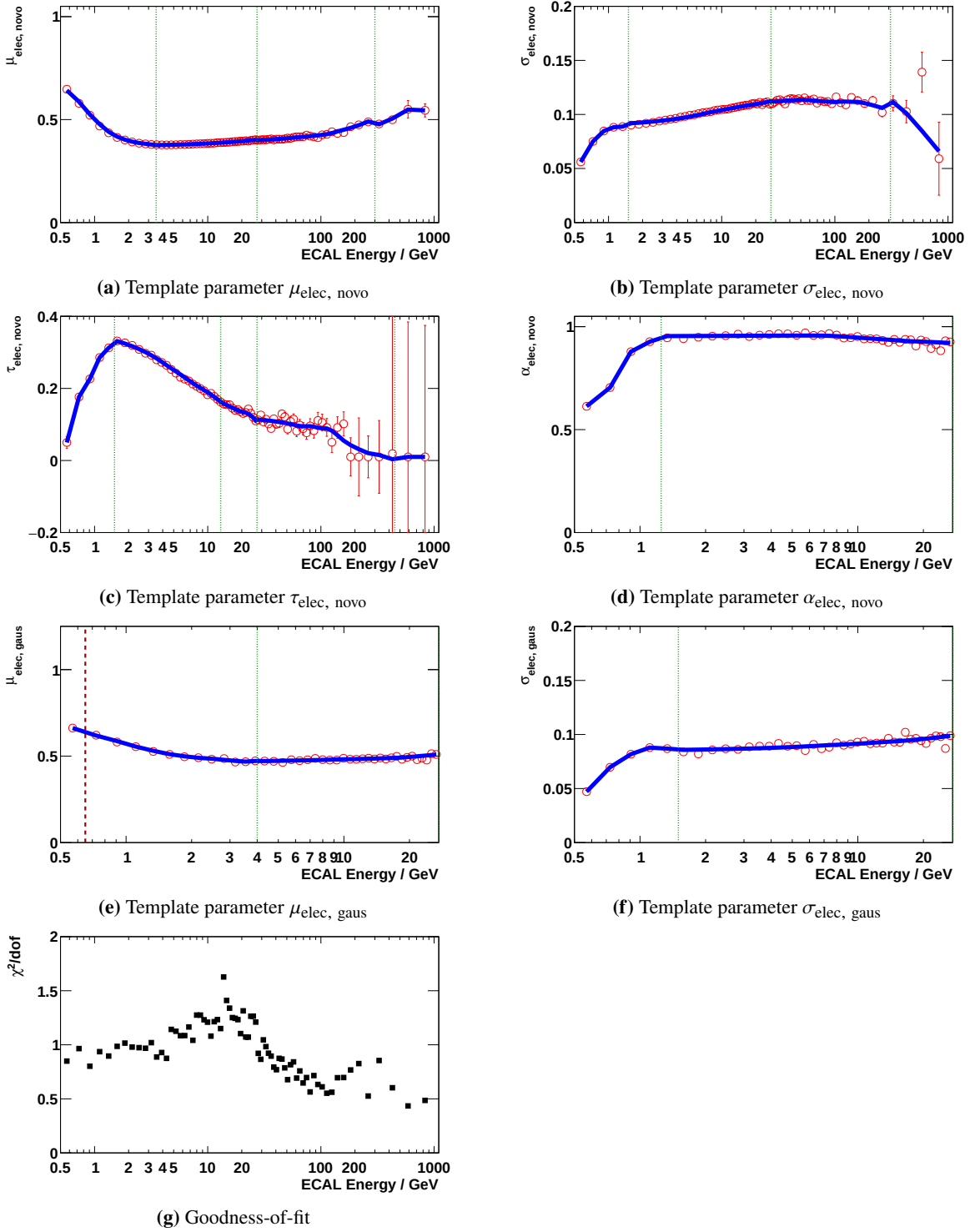
Figure A.18: Analytical TRD template parameters describing the evolution of the electron template as function of energy for the multi-tracks sample. The meaning of the red points, the blue curve and the dashed lines is given in the caption of Fig. A.17.
