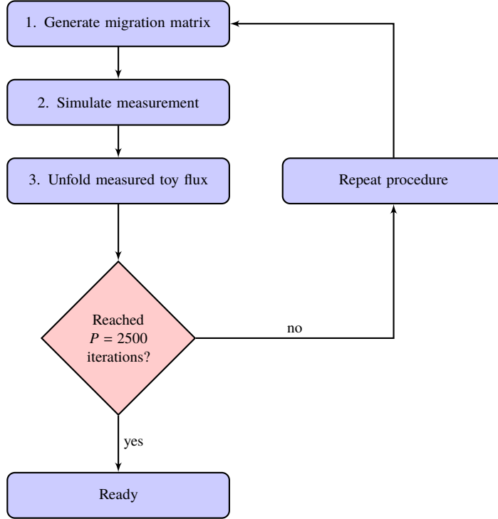
Figure 4.77: Illustration of the procedure to assess the stability of the unfolding procedure.
