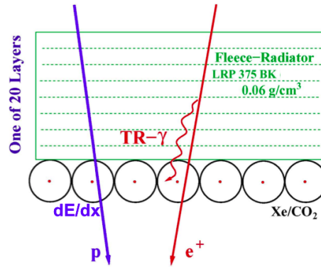
Figure 3.10: Working principle of the TRD. Credit: Ref. [AmsWebsite]
