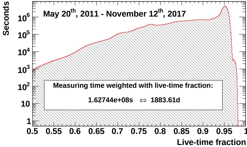
Figure 4.52: The plot shows the distribution of the live-time fraction of the experiment for all seconds that form the measuring time period. The distribution peaks at 95 % with a long tail towards smaller live-time fractions. Live-time fractions below 50 % are excluded for analysis by the detector quality cuts.
