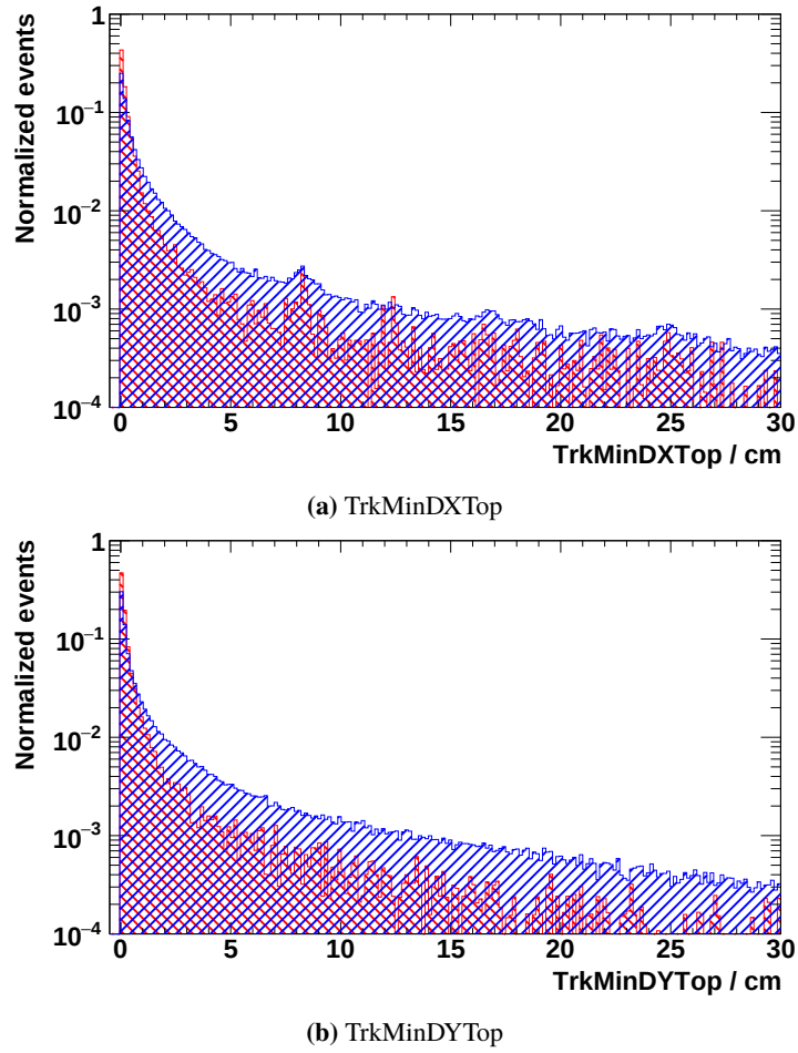
Figure A.12: Example of TrkMinDXTop / TrkMinDYTop distributions in the energy bin 17.98 – 18.99 GeV in the electron Monte-Carlo simulation.
