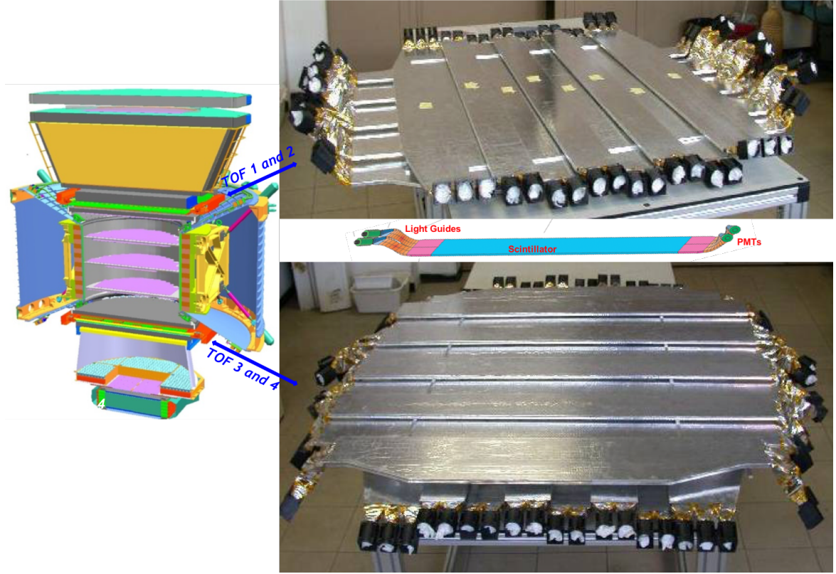
Figure 3.7: Picture of the Time-Of-Flight system. The upper and low TOF, each consists of two planes. Credit: Ref. [ AmsWebsite ]
