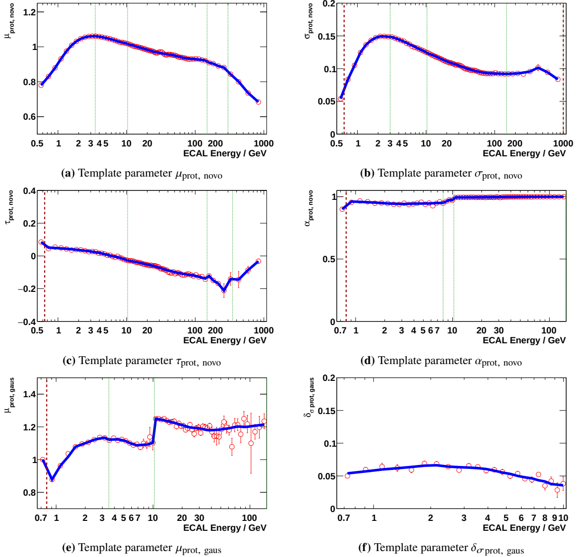
Figure 4.29: Analytical TRD template parameters describing the evolution of the proton template as function of energy for the single-track sample. In each energy bin the analytical function - Eq. (4.8) - is fit to the template data sample, yielding the red points. A smoothing procedure yields the blue curves, which are used as template parameters for the analysis. The vertical dashed green lines mark areas where different isolated smoothing procedures are applied. The vertical dashed red lines mark energies where the smoothing procedure starts/ends – points before/after this border are preserved.
