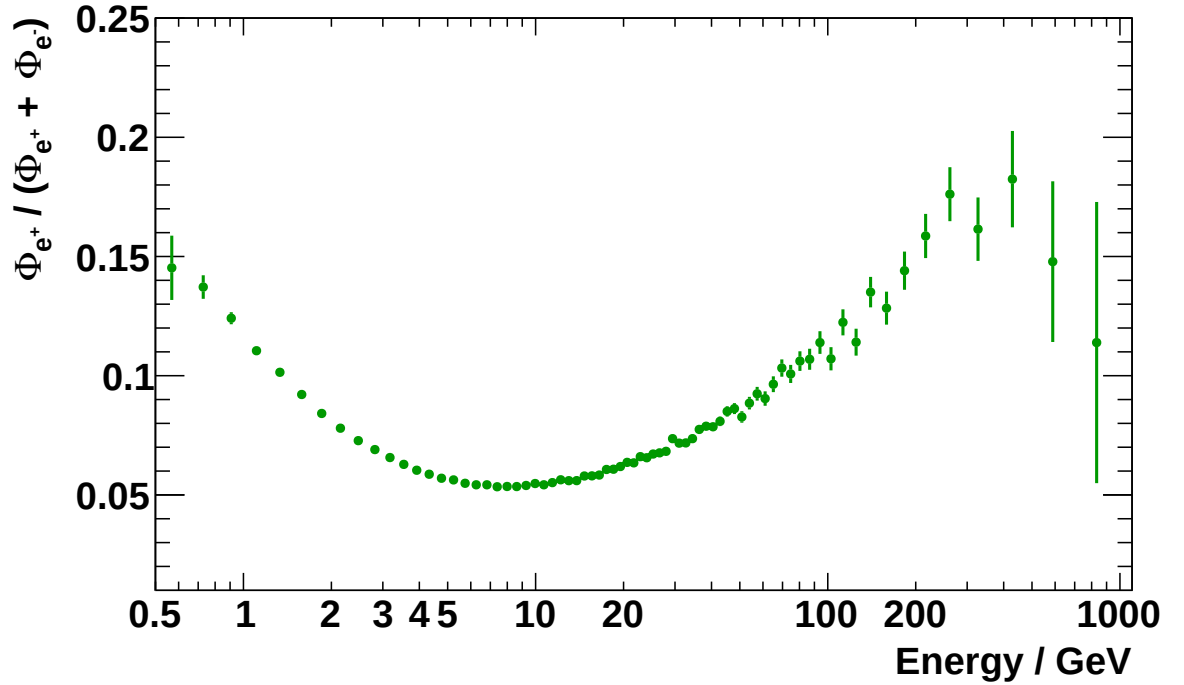
Figure B.6: The positron fraction measured by AMS-02.
