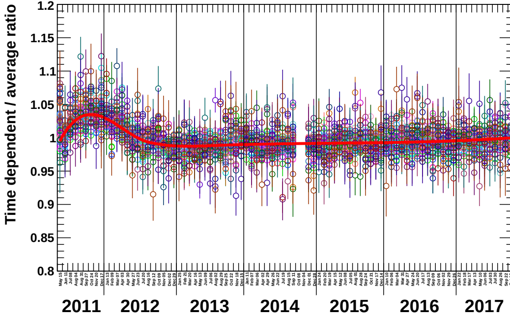
Figure A.22: Time-dependence of the \mu_{\text{elec, novo}} parameter for all energy bins - 0.65 – 52.33 GeV - in the time-dependent analysis for the multi-tracks sample. Each energy bin is represented by a different color. The filled red line denote the result of a spline fit, simultaneously to all data points, describing the average time-dependence of the \mu_{\text{elec, novo}} parameter.
