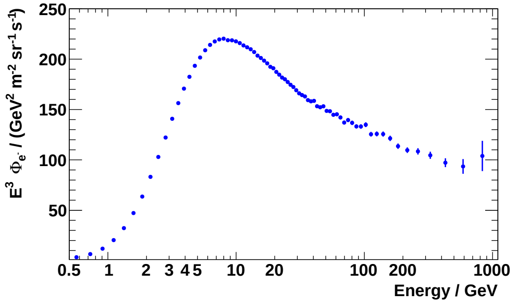
Figure 5.1: The electron flux measured by AMS-02 using the analysis procedure described in this work. The y-axis shows the unfolded flux, multiplied by energy E^3 for illustration purposes.
