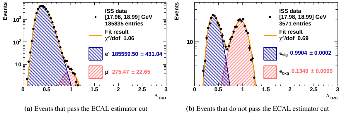
Figure 4.46: Results of the simultaneous fit to extract the ECAL estimator efficiency in the energy bin 17.98 – 18.99 GeV for the all-tracks sample. The dark blue area corresponds to the electron template, the light red area to the charge-confused proton template and the orange line to the sum of all templates.
