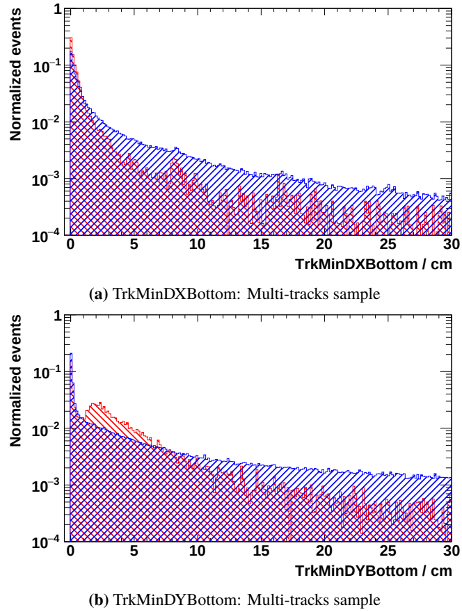
Figure 4.7: Example of TrkMinDXBottom / TrkMinDYBottom distributions in the energy bin 17.98 – 18.99 GeV in the electron Monte-Carlo simulation. The red histogram shows the charge-confused sample ( R > 0 ) and the blue histogram the correct reconstructed sample ( R < 0 ), after applying all preselection, selection and e^\pm identification cuts.
