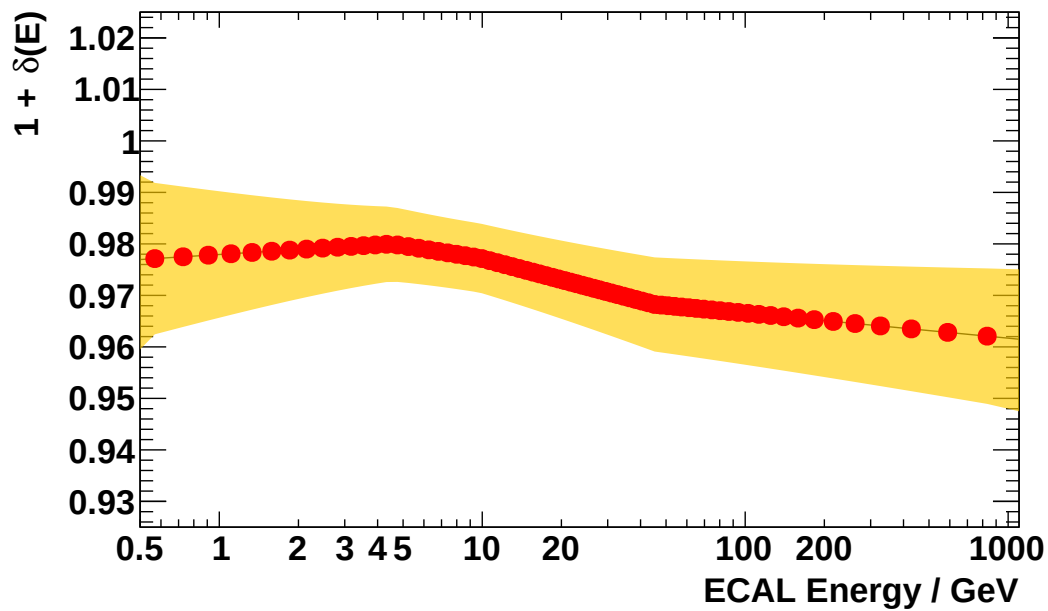
Figure 4.60: The magnitude of the combined Data/Monte-Carlo correction factor (1 + \delta(E)) is shown as red symbols. The correction applied to the Monte-Carlo acceptance varies from 2 % at low energies up to 4 % at high energies and is known for all energies better than 1.5 %, indicated by the orange band.
