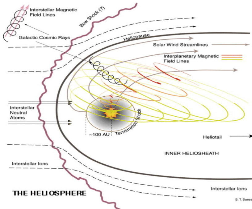
Figure 2.2: Sketch of the heliosphere. Credit: S. T. Suess.
