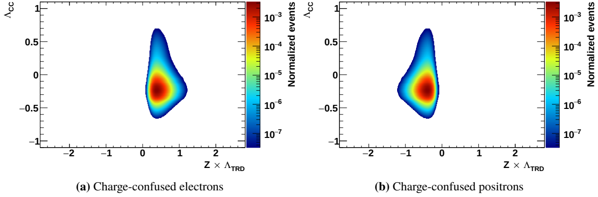
Figure 4.33: Two-dimensional TRD / CCMVA templates in the energy bin 17.98 – 18.99 GeV for the charge-confused electrons and charge-confused positrons in the single-track sample. The color encodes the amount of normalized entries in the histogram, a red color corresponds to a large number of events, a blue color to a small number of events.
