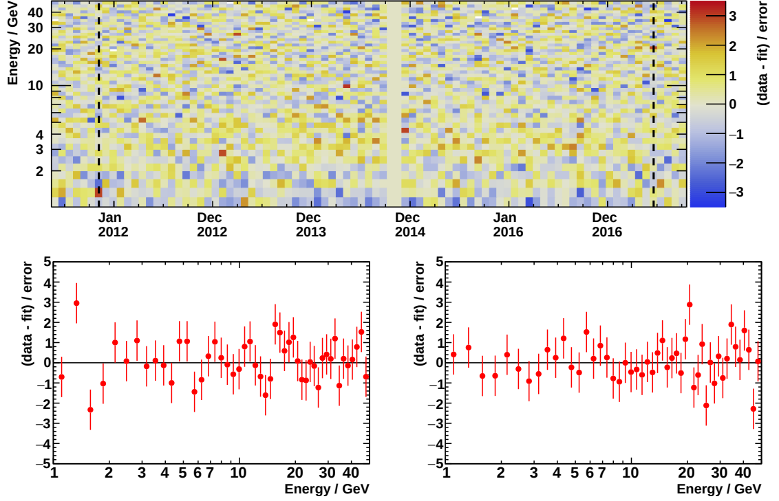
Figure B.16: For the positron flux, the difference between data and model [Cavasonza2017] fits normalized to the experimental uncertainties: for each Bartels Rotation as a function of energy (upper plot). The distribution for the positrons reveals no visible structures, emphasized for Bartels Rotation 2432 (lower left) and Bartels Rotation 2508 (lower right). The times for these two Bartels Rotations are indicated by the vertical dashed lines.
