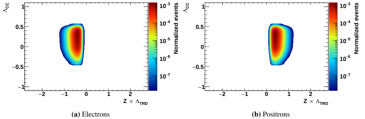
Figure 4.32: Two-dimensional TRD / CCMVA templates in the energy bin 17.98 – 18.99 GeV for the electrons and positrons in the single-track sample. The color encodes the amount of normalized entries in the histogram, a red color corresponds to a large number of events, a blue color to a small number of events.
