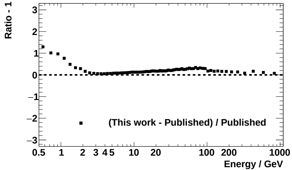
Figure B.10: Ratio of the total uncertainty of the positron fraction derived in this work over the uncertainty of the recently published AMS-02 positron fraction [Aguilar2019b].
