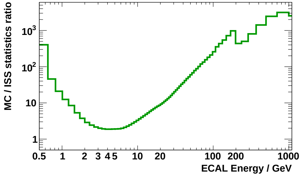
Figure 4.71: Comparison of the available Monte-Carlo statistics to the ISS statistics after applying all data quality, preselection, selection and identification cuts. The green line shows the ratio of negative rigidity Monte-Carlo event counts divided by ISS event counts.
