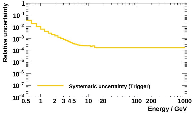
Figure 4.70: Visualization of the relative systematic uncertainty associated with the electron flux and the positron flux due to the knowledge of the trigger efficiency.
