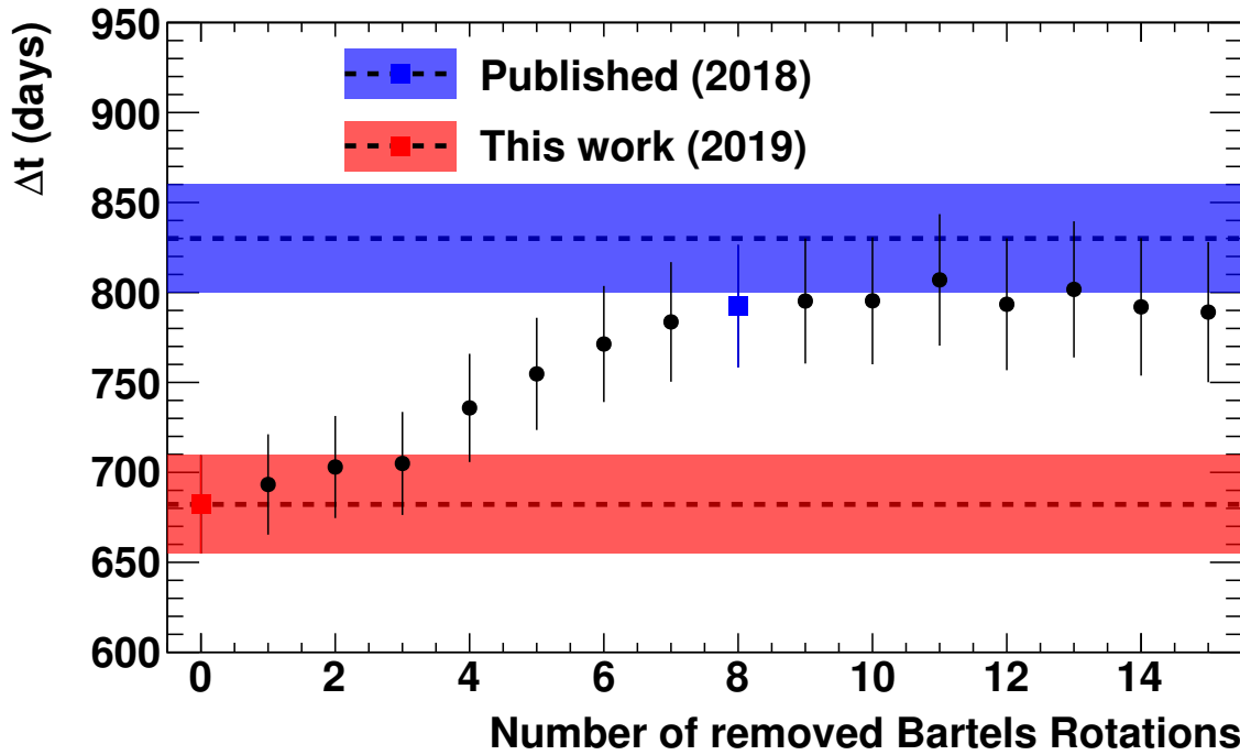
Figure 5.25: Dependence of the \Delta t parameter on the amount of Bartels Rotations that are included in the fit of Eq. (5.5) to the ratio R_e . The number of excluded Bartels Rotations at the end of the data taking period is correlated with \Delta t .
