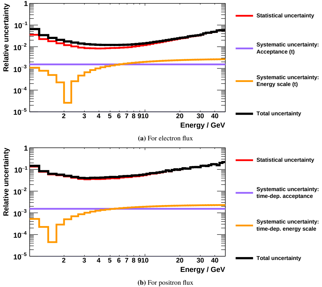
Figure 4.113: Composition of the relative systematic uncertainty associated with the electron flux (upper plot) and the positron flux (lower plot) in Bartels rotation i = 26 (Apr 16 th , 2013 - May 13 th , 2013), as example.
