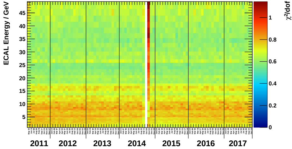
Figure 4.103: Goodness of fit results for the two-dimensional template fit, performed using the time-dependent TRD templates on the all-tracks sample. The color encodes the \chi^2/\text{dof} value for each Bartels rotation i and each energy bin j of the time-dependent analysis. All \chi^2/\text{dof} values are acceptable.
