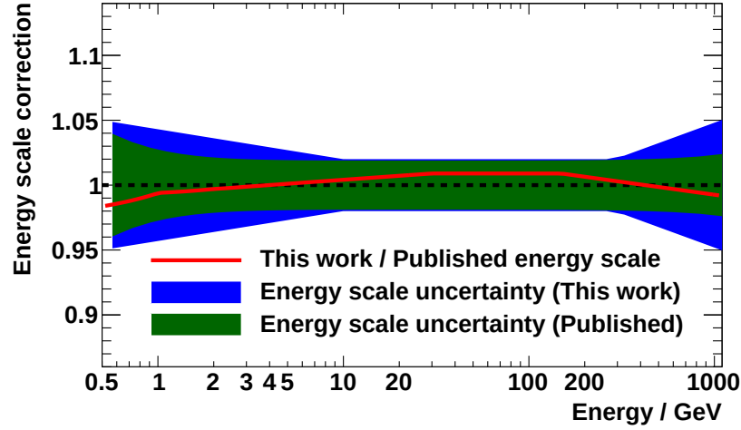
Figure B.1: Correction applied to the Aachen energy scale used in this work to match the MIT energy scale used in recent AMS-02 electron and positron flux publications [Aguilar2019a; Aguilar2019b]. The red line shows the necessary energy scale correction and the colored bands the energy scale uncertainties used for this work (blue band) and for recent publications (green band).
