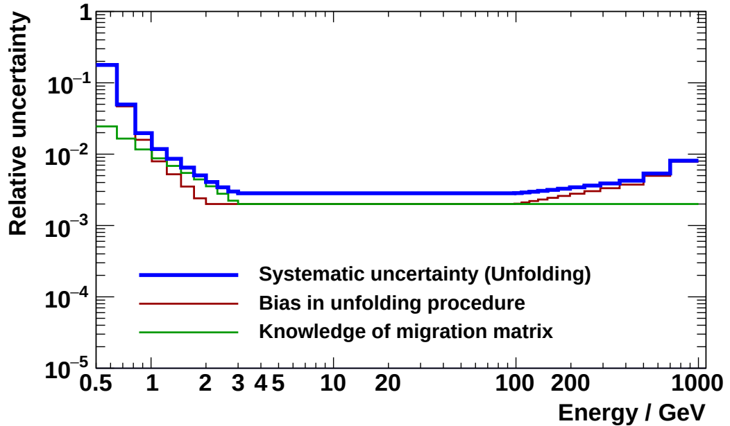
Figure 4.84: Visualization of the relative systematic uncertainty associated with the electron flux and the positron flux due to the unfolding procedure.
