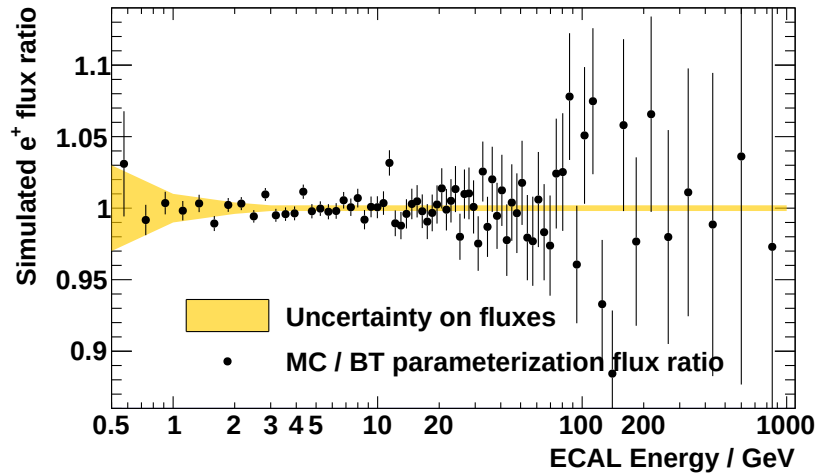
Figure 4.76: Ratio of the toy e^+ flux forward folded with the Monte-Carlo parameterization over the toy e^+ flux forward-folded with the testbeam parameterization - shown as black symbols. The orange band represents the systematic uncertainty on the fluxes due to the knowledge of the migration matrix.
