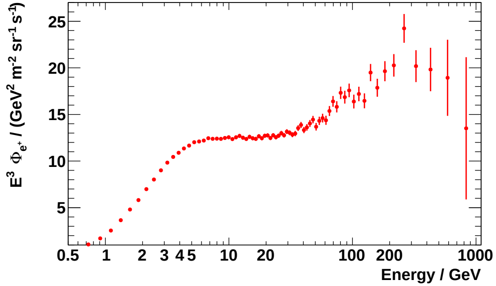
Figure 5.7: The positron flux measured by AMS-02 using the analysis procedure described in this work. The y-axis shows the unfolded flux, multiplied by energy E^3 for illustration purposes.
