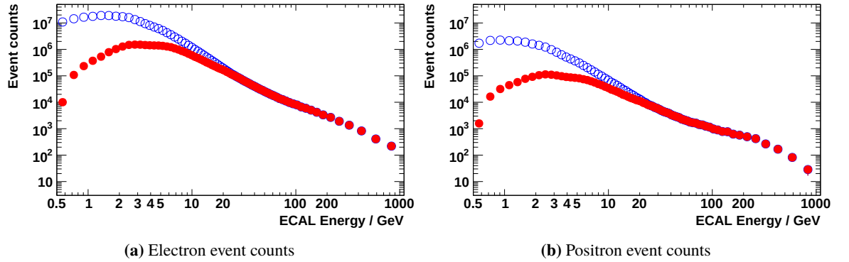
Figure 4.63: Comparison of the event counts \mathbf{n} determined from the two-dimensional template fit (red symbols) with the artificial event counts \mathbf{n}_{\text{no cut-off}} that AMS-02 would measure if there was no geomagnetic cut-off effect (blue symbols). The left plot shows the electron event counts, the right plot the positron event counts.
