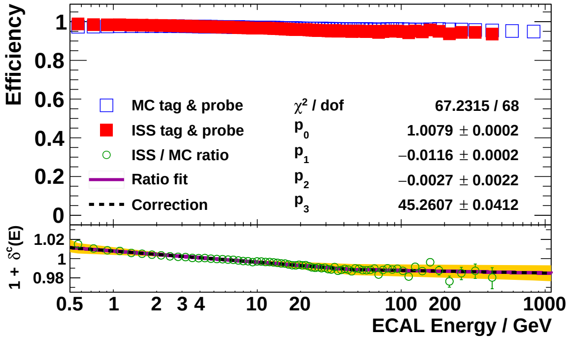
Figure 4.57: Determination of the Data/Monte-Carlo correction factor ( 1 + \delta^c(E) ) for the selection cut: “Tracker track goodness-of-fit in Y-projection” (Section 4.3.3 - Item 7). The open blue symbols in the upper plots show the cut efficiency determined on the electron Monte-Carlo simulation on a dedicated sample: the tag sample. The filled red symbols in the upper plots show the cut efficiency determined from ISS data using the same tag cuts. The lower plots show the ratio ISS efficiency over MC efficiency as open green symbols. Equation (4.24) is fit to the ratio, represented as magenta line. The dashed black line shows that half of the deviation from unity is taken as correction to the Monte-Carlo acceptance A_e^{\text{MC}}(E) . The associated systematic uncertainty is visualized by the orange band.
