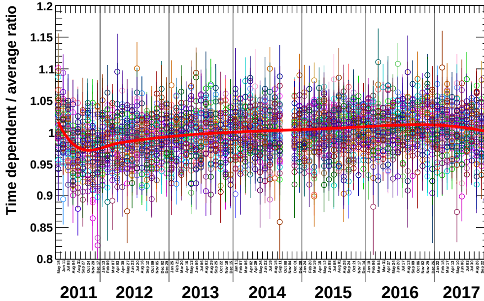
Figure 4.100: Time-dependence of the \mu_{\text{ccprot, novo}} parameter for selected energy bins (1.22 – 52.33 GeV), as example, in the time-dependent analysis for the single-track sample.
