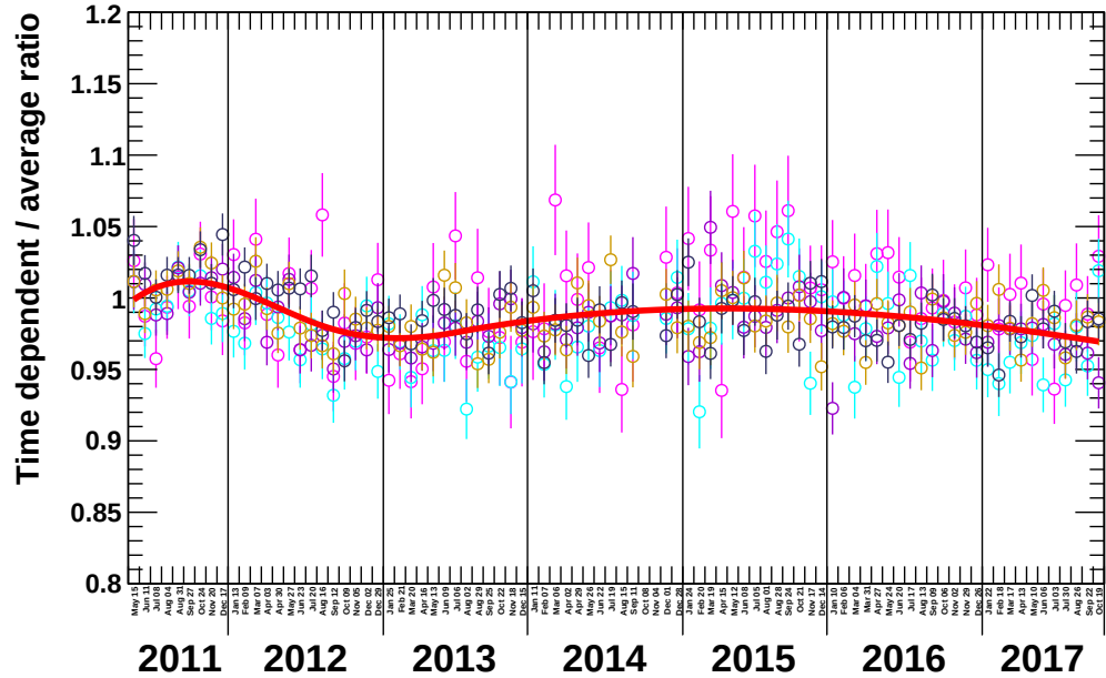
Figure A.25: Time-dependence of the \sigma_{\text{elec, novo}} parameter for selected energy bins (1.46 – 3.00 GeV), as example, in the time-dependent analysis for the multi-tracks sample.
