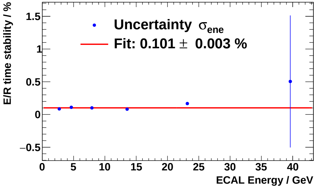
Figure 4.110: Relative energy scale uncertainty \sigma_{\text{ene}}/E as function of energy. It is identical for all Bartels rotations i , since the energy scale is independent of time.
