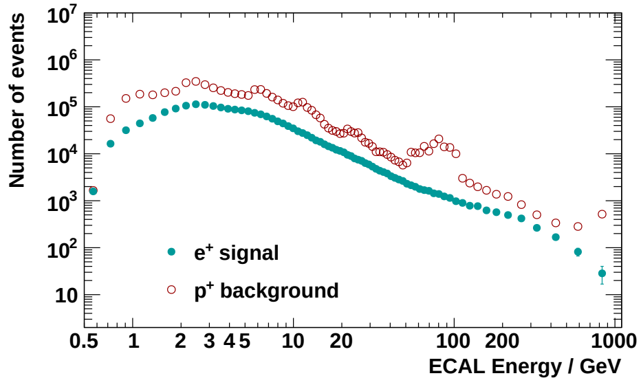
Figure 4.43: Number of signal and background events for the all-tracks sample, extracted from the two-dimensional fit procedure.
