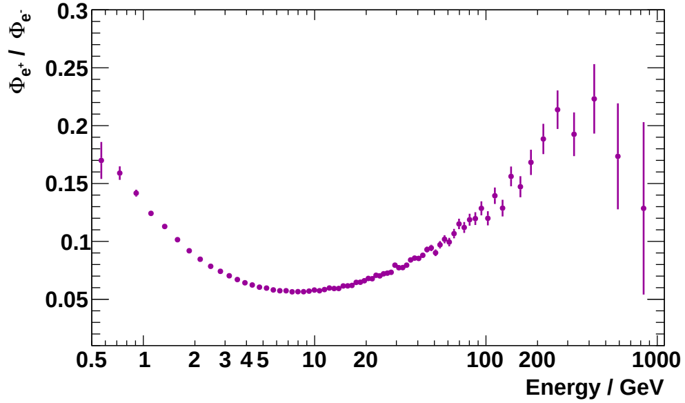
Figure 5.15: The positron/electron ratio measured by AMS-02.
