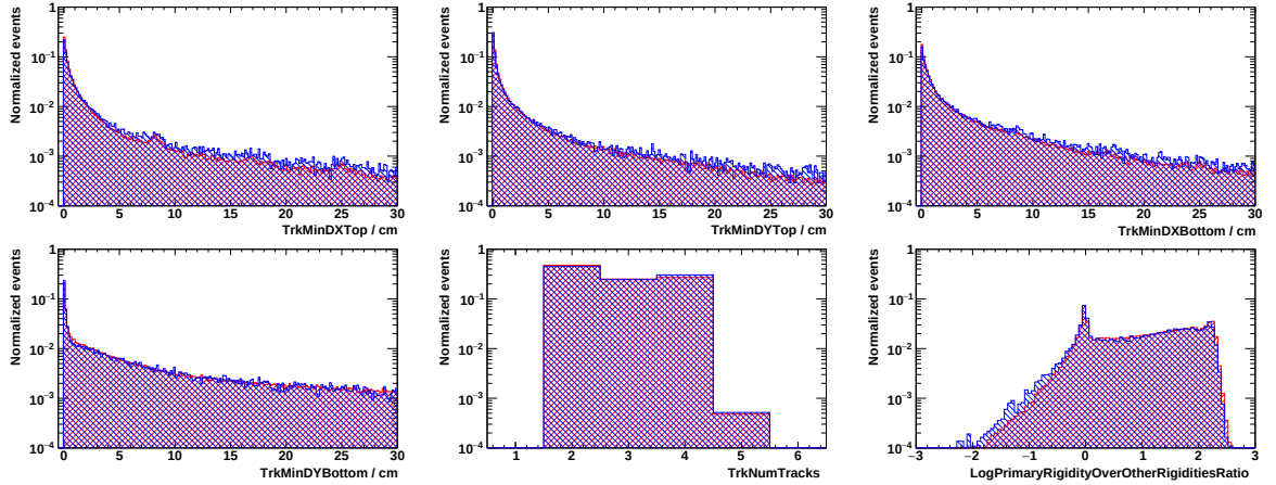
Figure A.15: Comparison of the six multi-tracks sample specific CCMVA input variables between the ISS data (blue) and the electron Monte-Carlo (red) in the energy bin 17.98 – 18.99 GeV. There are no visible differences, except for small fluctuations in the tails, proving the consistency of the input quantities between ISS data and simulation.
