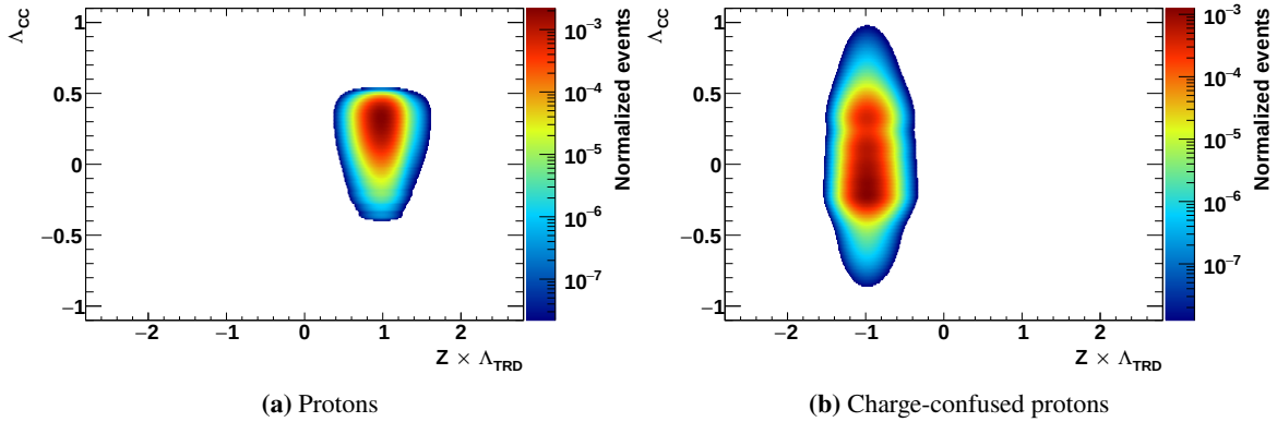
Figure 4.34: Two-dimensional TRD / CCMVA templates in the energy bin 17.98 – 18.99 GeV for the protons and charge-confused protons in the single-track sample. The color encodes the amount of normalized entries in the histogram, a red color corresponds to a large number of events, a blue color to a small number of events.
