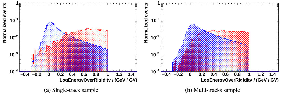
Figure 4.2: Example of LogEnergyOverRigidity distribution in the energy bin 17.98 – 18.99 GeV in the electron Monte-Carlo simulation. Note that LogEnergyOverRigidity is bounded between -0.3 < \log (E_{\text{ECAL}}/|R_{\text{primary}}|) < 1 , due to the E |R| cut in the e^\pm identification cuts.
