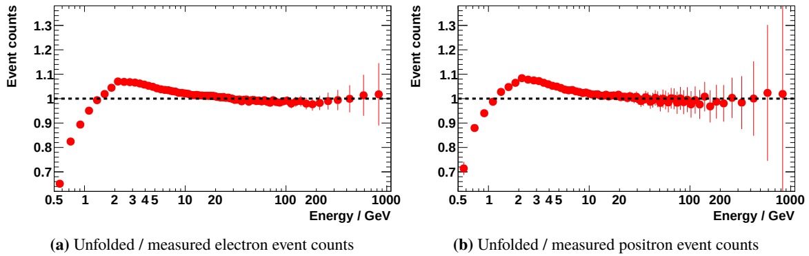
Figure 4.65: Plot of the ratio of unfolded event counts over measured event counts to quantify the magnitude of unfolding. Above 100 GeV the effect of the unfolding becomes negligible. At low energies the effect is large with corrections up to 60 % in the first energy bin: 0.5 – 0.65 GeV. With increasing energy the magnitude of the unfolding decreases, but it is still a sizeable effect over the whole energy range.
