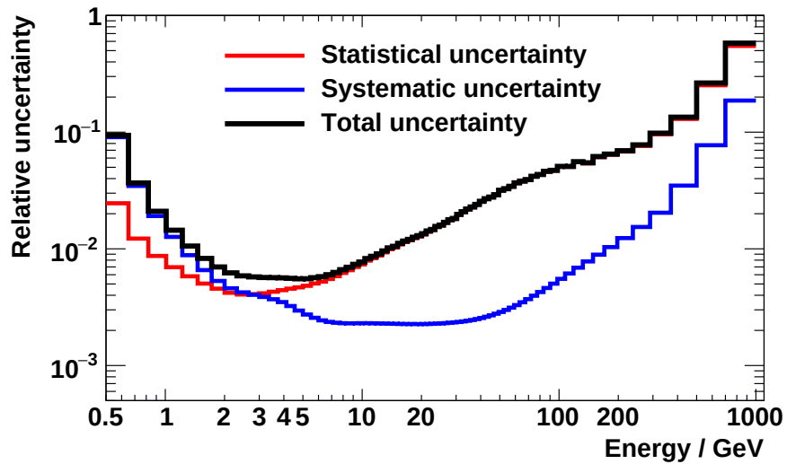
Figure 5.16: Breakdown of the uncertainty of the positron/electron ratio into a statistical and systematical part.
