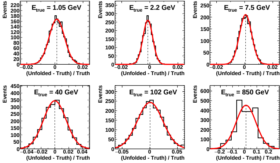
Figure 4.82: Example projections in several energy bins from Fig. 4.81 to the y-axis for the e^+ fluxes.
