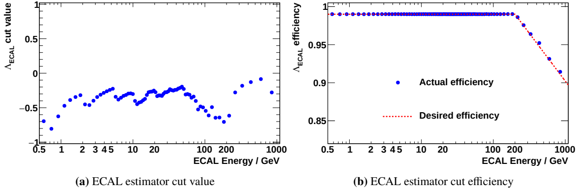
Figure 4.45: Chosen ECAL estimator efficiency for the analysis of the all-tracks sample. The left plot shows the ECAL estimator cut value that is used in the analysis. The visible structures originate in different training intervals used to train the ECAL estimator. The right plot shows the ECAL estimator efficiency \epsilon_{\text{ecal}}(E) as function of energy. The dashed red line in the right plot represents the desired ECAL estimator efficiency and the blue symbols the actual efficiency in each energy bin, determined by a one-dimensional TRD template fit on the negative rigidity sample on ISS data.
