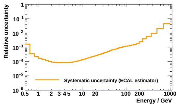
Figure 4.69: Visualization of the relative systematic uncertainty associated with the electron flux and the positron flux due to the knowledge of the ECAL estimator efficiency.
