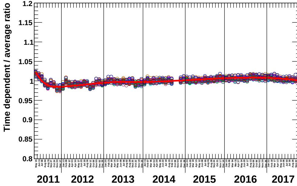
Figure 4.99: Time-dependence of the \mu_{\text{prot, novo}} parameter for all energy bins - 0.65 – 52.33 GeV - in the time-dependent analysis.
