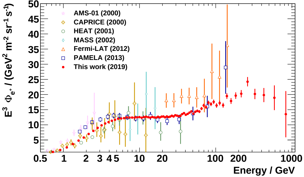
Figure 5.9: Comparison of the positron flux derived in this work with other experiments: AMS-01 [Alcaraz2000], CAPRICE [Boezio2000], HEAT [DuVernois2001], MASS [Grimani2002], Fermi-LAT [Ackermann2012] and PAMELA [Adriani2013].
