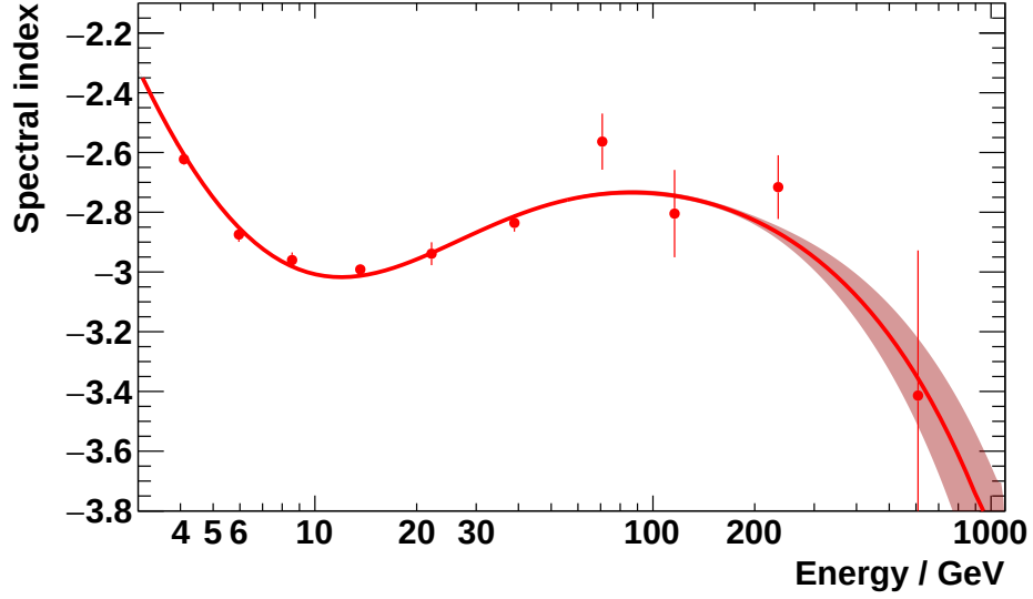
Figure 5.10: The spectral index of the positron flux in non-overlapping energy intervals shown as red points. The red band corresponds to the uncertainty determined from a fit of Eq. (5.4) to the data.
