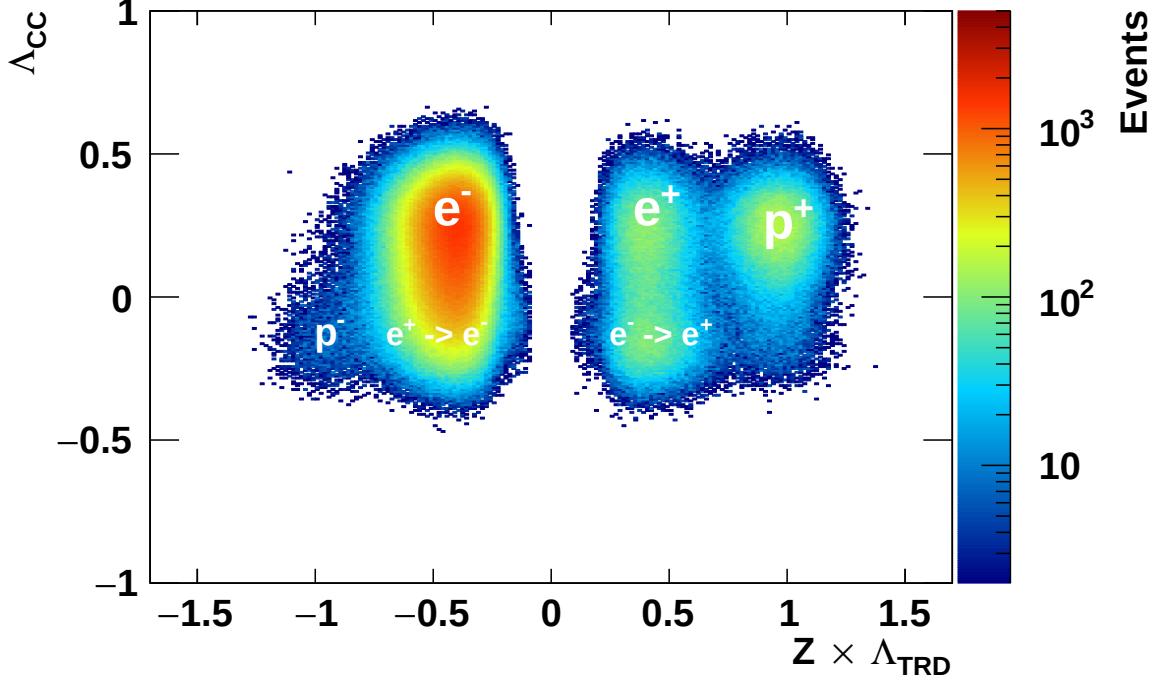
Figure 4.22: Overview of the ISS data sample after applying all selection cuts and an additional cut on the ECAL estimator \Lambda_{\text{ECAL}} to reduce the proton background in the energy range 20 – 50 GeV. The CCMVA estimator \Lambda_{\text{CC}} is drawn on the y-axis and the TRD estimator \Lambda_{\text{TRD}} multiplied by the charge sign Z of the primary tracker track on the x-axis. Clearly these two estimators allow to separate the different species: electrons, positrons, protons and their charge-confused counterparts.
