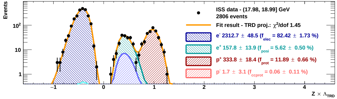
Figure 4.105: Results of the two-dimensional TRD / CCMVA template fit in Bartels rotation i = 6 for the energy bin 17.98 – 18.99 GeV (all-tracks sample) using the time-dependent TRD templates.
