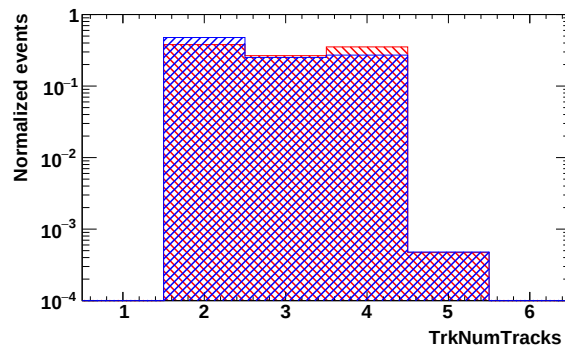
Figure A.11: Example of TrkNumTracks distribution in the energy bin 17.98 – 18.99 GeV in the electron Monte-Carlo simulation.
