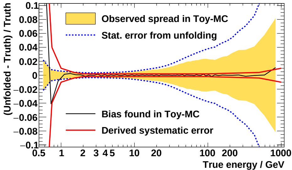
Figure 4.83: Visualization of the bias of the unfolding procedure for the e^+ flux, extracted from the gaussian fits of Fig. 4.82, as function of the true energy.
