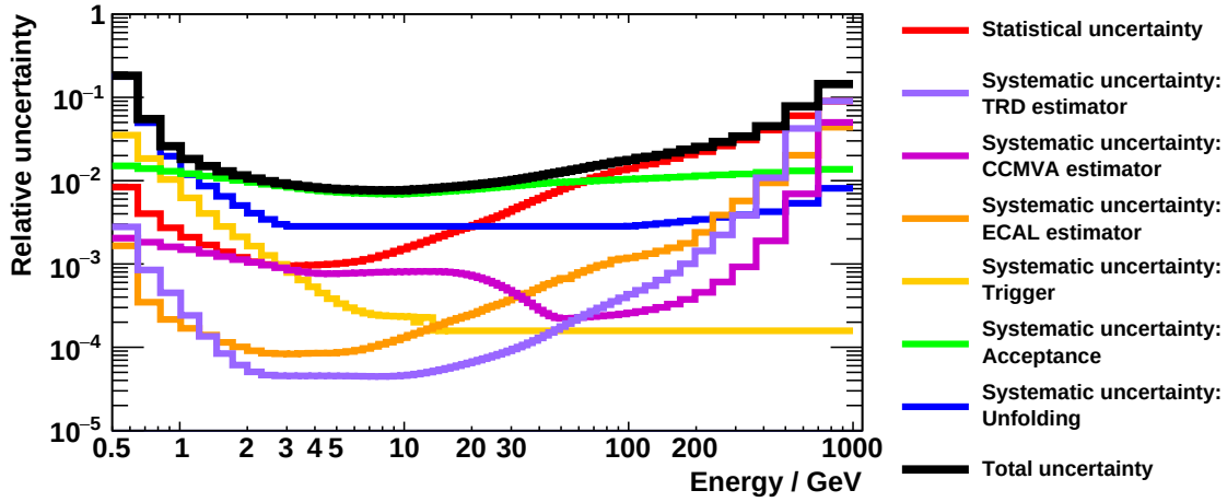
Figure 4.85: Composition of the relative systematic uncertainty associated with the electron flux.
