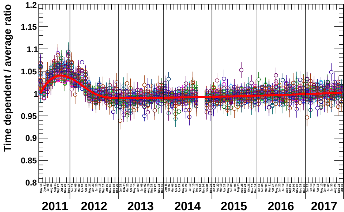
Figure 4.98: Time-dependence of the \mu_{\text{elec, novo}} parameter for all energy bins - 0.65 – 52.33 GeV - in the time-dependent analysis for the single-track sample. Each energy bin is represented by a different color. The filled red line denote the result of a spline fit, simultaneously to all data points, describing the average time-dependence of the \mu_{\text{elec, novo}} parameter.
