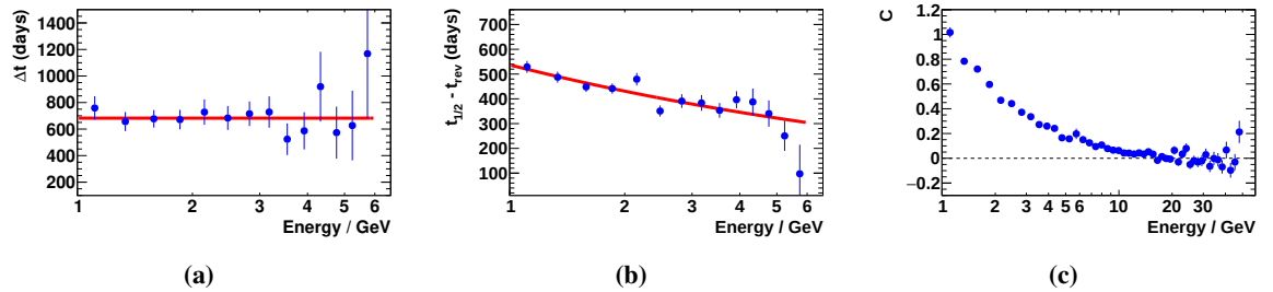
Figure 5.24: Results of the fits of the parameterization in Eq. (5.5) to the ratio R_e as a function of energy (blue circles): (a) \Delta t and the best-fit constant value of 682 days (red line), (b) t_{1/2} - t_{\text{rev}} with the parameterization according to Eq. (5.6) (red curve), (c) amplitude C with a dashed line at zero to guide the eye.
