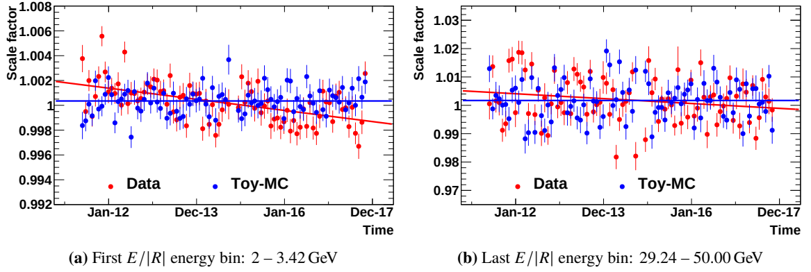
Figure 4.108: Scale factors S_i of both the ISS data sample and the Toy-MC sample as function of time. The ISS data sample time dependence is parameterized using a straight line, and the time dependence in the Toy-MC sample using a constant.
