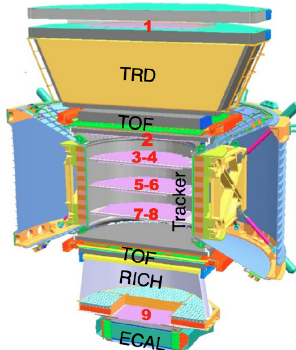
Figure 3.1: Schematic view of the AMS-02 detector. Credit: Ref. [ AmsWebsite ]
