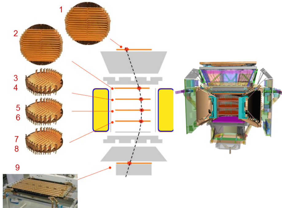
Figure 3.5: Schematic of the tracker showing the locations of the nine tracker planes. Credit: Ref. [AmsWebsite]
