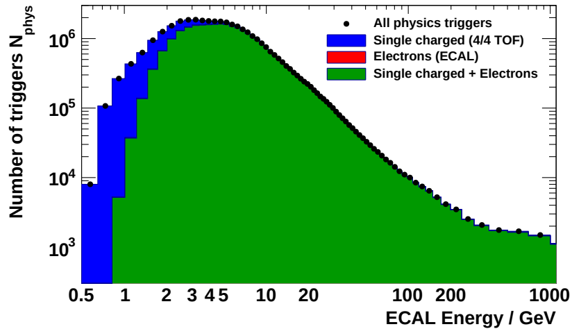
Figure 4.48: Decomposition of the physics triggers as stacked histograms. Two main trigger branches form the physics trigger for the e^\pm analysis: the Single charged trigger and the Electrons trigger.
