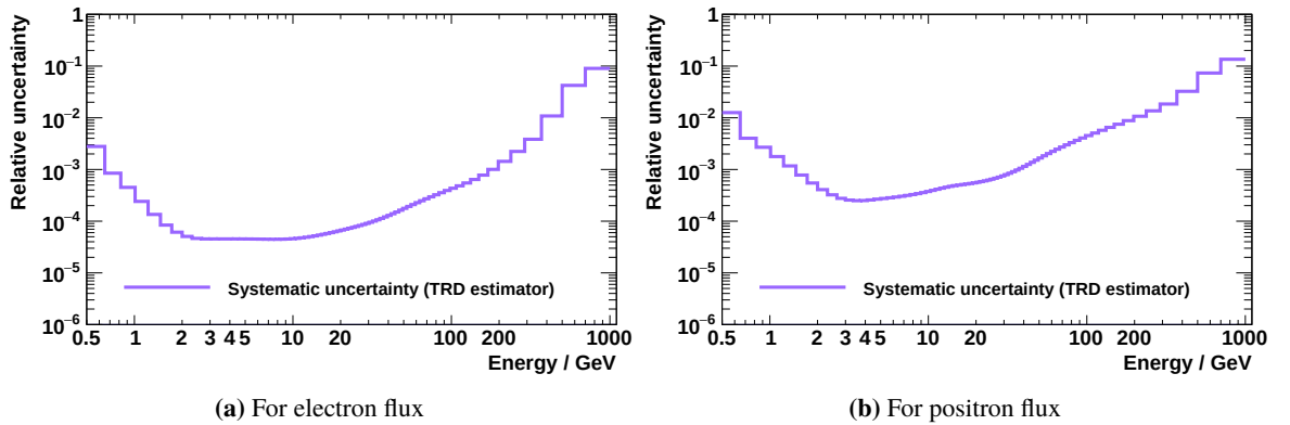
Figure 4.66: Visualization of the relative systematic uncertainty associated with the electron flux (left plot) and associated with the positron flux (right plot) due to the knowledge of the TRD estimator.
