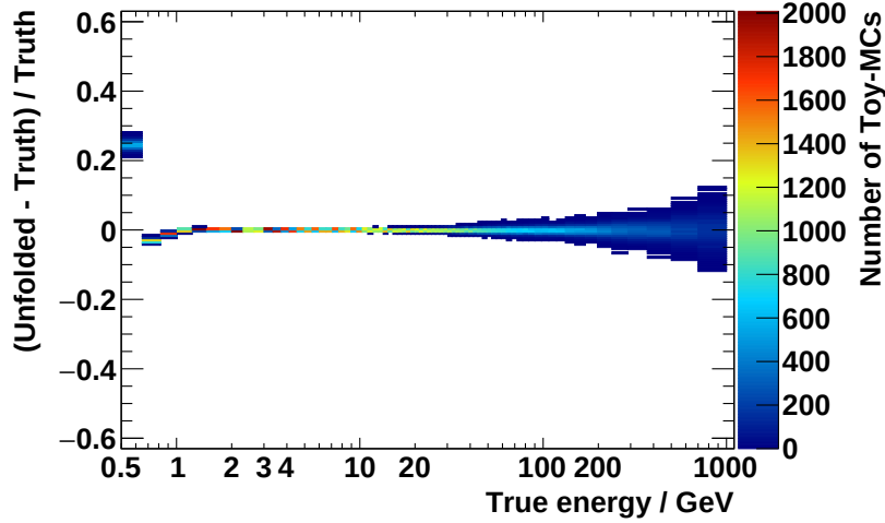
Figure 4.78: Distribution of the deviation of the unfolded e^- flux \tilde{\Phi}_{\text{unfolded}} from the true flux \Phi_{\text{true}} divided by the true flux for P Toy-MCs as function of the true energy.
