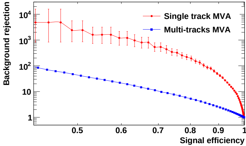
Figure 4.10: ROC curve of the CCMVA estimator in the energy bin 17.98 – 18.99 GeV. The red curve represents the ROC curve for the single-track sample and the blue curve represents the multi-tracks sample.
