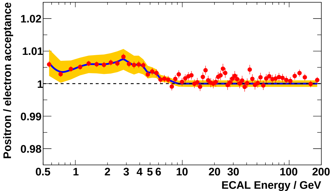
Figure 4.61: Visualization of the positron over electron acceptance ratio A_{e^+}(E)/A_{e^-}(E) , shown as red symbols. The difference is around 1 % at 3 GeV where the difference between the electron and the positron acceptance is largest. The blue curve multiplied to the electron acceptance yields the positron acceptance.
