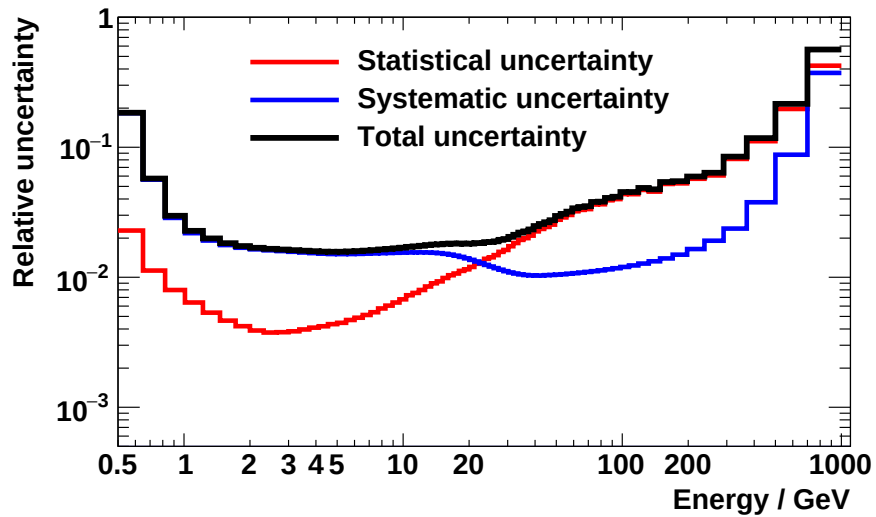
Figure 5.8: Breakdown of the uncertainty of the positron flux into a statistical and systematical part.
