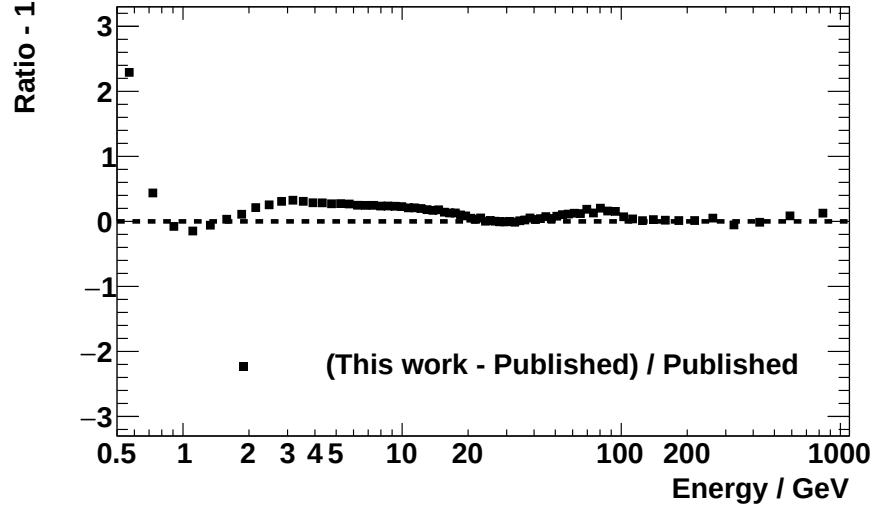
Figure B.5: Ratio of the total uncertainty of the positron flux derived in this work over the uncertainty of the recently published AMS-02 positron flux [Aguilar2019b].
