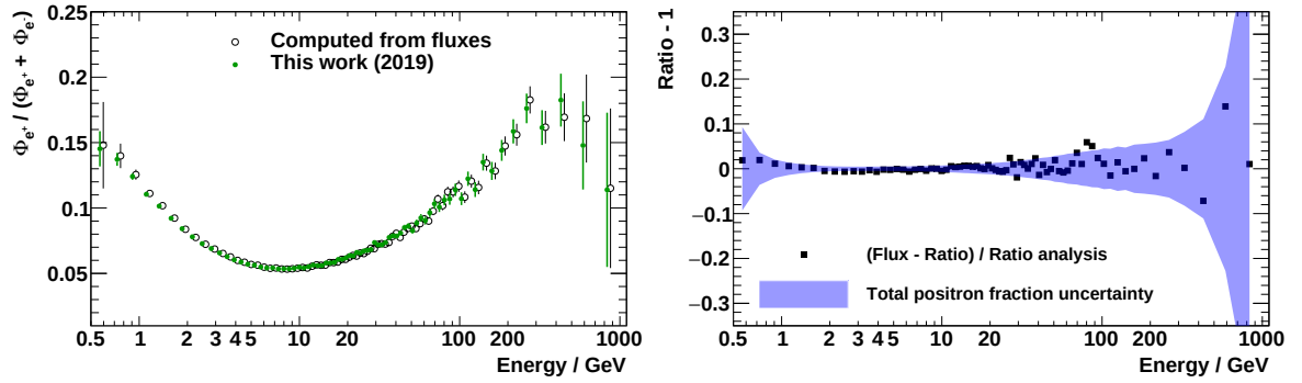
Figure B.13: Comparison of the positron fraction derived using the single-track analysis with the ratio computed from the fluxes, that were derived from the all-track analysis. To ease the comparison the all-track analysis data points are shifted horizontally by 5 %. Within the quoted systematic uncertainties the results are compatible.
