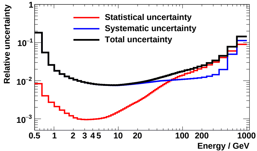
Figure 5.3: Breakdown of the uncertainty of the electron flux into a statistical and systematical part.
