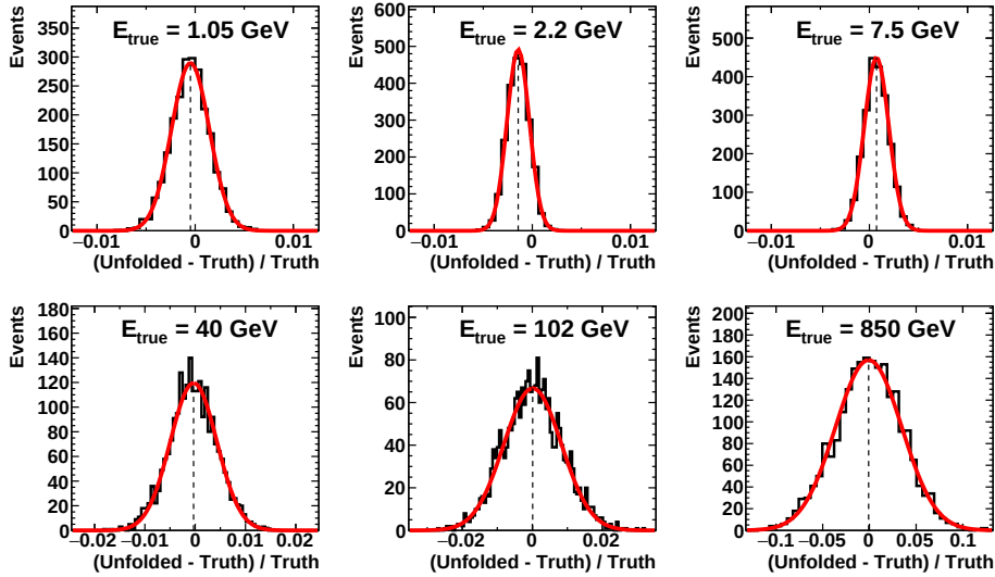
Figure 4.79: Example projections in several energy bins from Fig. 4.78 to the y-axis for the e^- fluxes. The black histogram shows the projection and the red line a gaussian fit to the histogram. The black dashed line indicates the mean of the gaussian, which is a measure of the bias.
