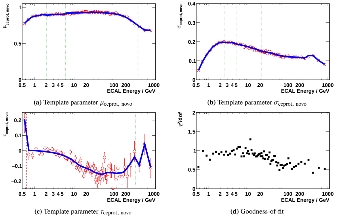
Figure A.17: Analytical TRD template parameters describing the evolution of the charge-confused proton template as function of energy for the multi-tracks sample. In each energy bin the analytical function - Eq. (4.7) - is fit to the template data sample, yielding the red points. A smoothing procedure yields the blue curves, which are used as template parameters for the analysis. The vertical dashed green lines mark areas where different isolated smoothing procedures are applied. The goodness-of-fit is indicated by the black points in the lower right plot.
