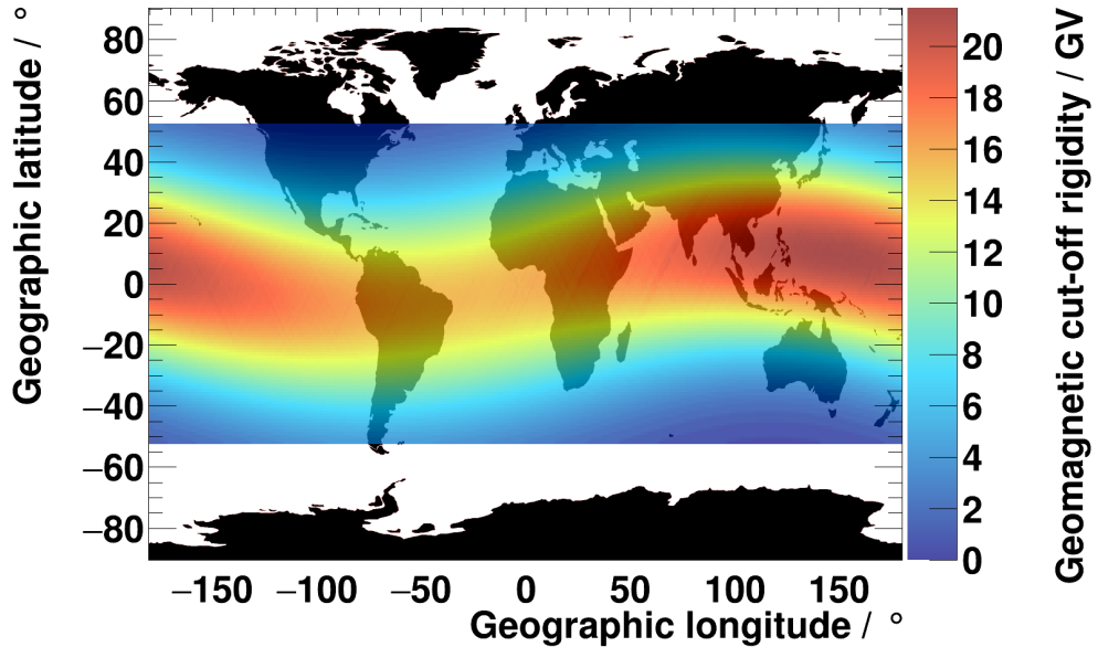
Figure 2.5: The plots shows the geomagnetic cut-off rigidity as function of the geomagnetic longitude/latitude.
