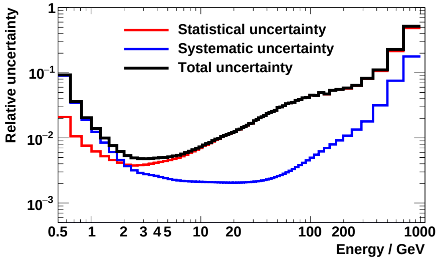
Figure B.8: Breakdown of the uncertainty of the positron fraction into a statistical and systematical part.
