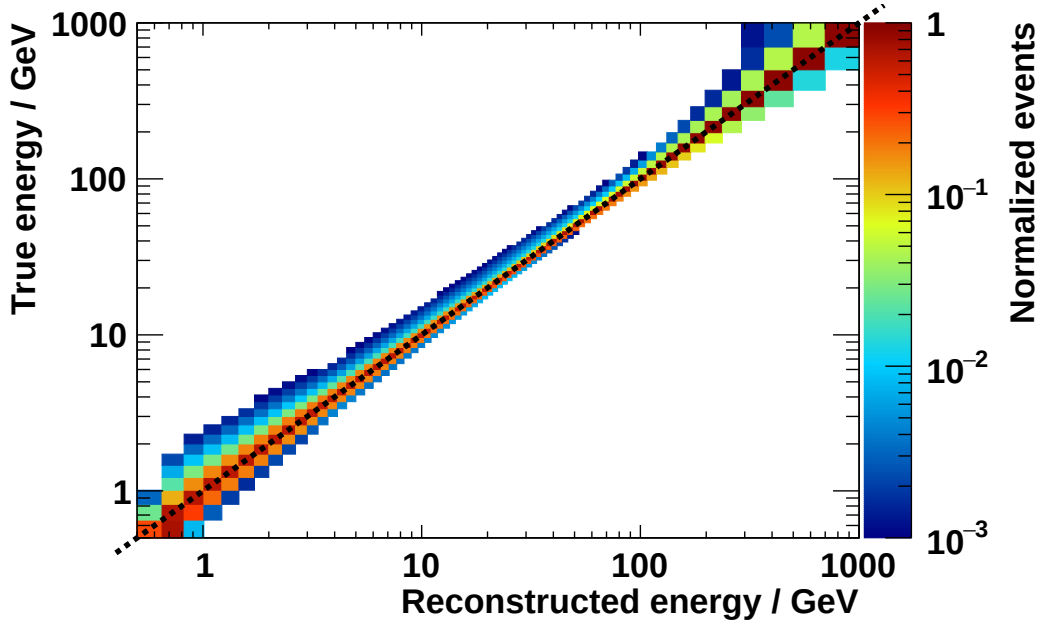
Figure 4.64: Plot of the migration matrix, additionally weighted using the geomagnetic cut-off weight w_{\text{cut-off}}(E) determined from ISS data.
