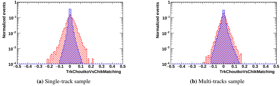
Figure A.7: Example of TrkChoutkoVsChikMatching distribution in the energy bin 17.98 – 18.99 GeV in the electron Monte-Carlo simulation.
