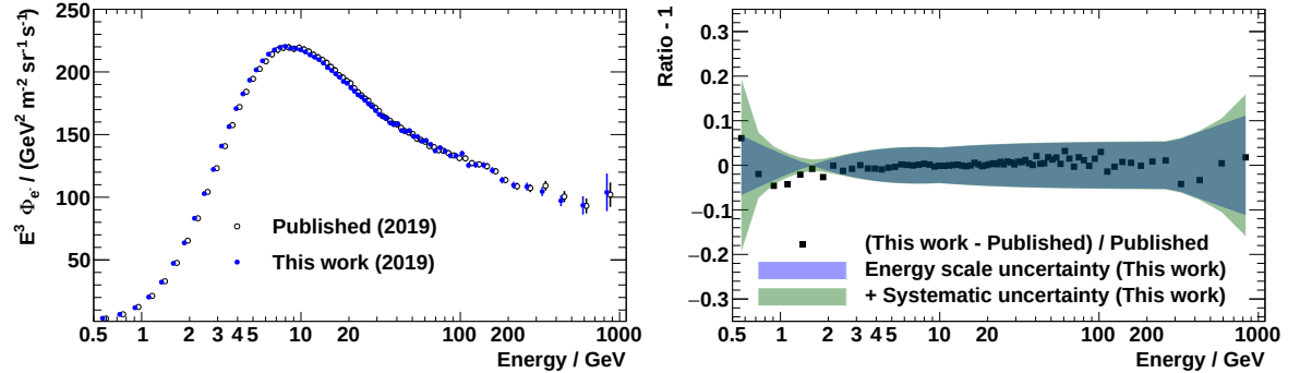
Figure B.2: Comparison of the electron flux derived in this work with the recent AMS-02 electron flux publication [Aguilar2019a]. To ease the comparison the published data points are shifted horizontally by 5 %. Within the quoted systematic uncertainties the results are compatible.
