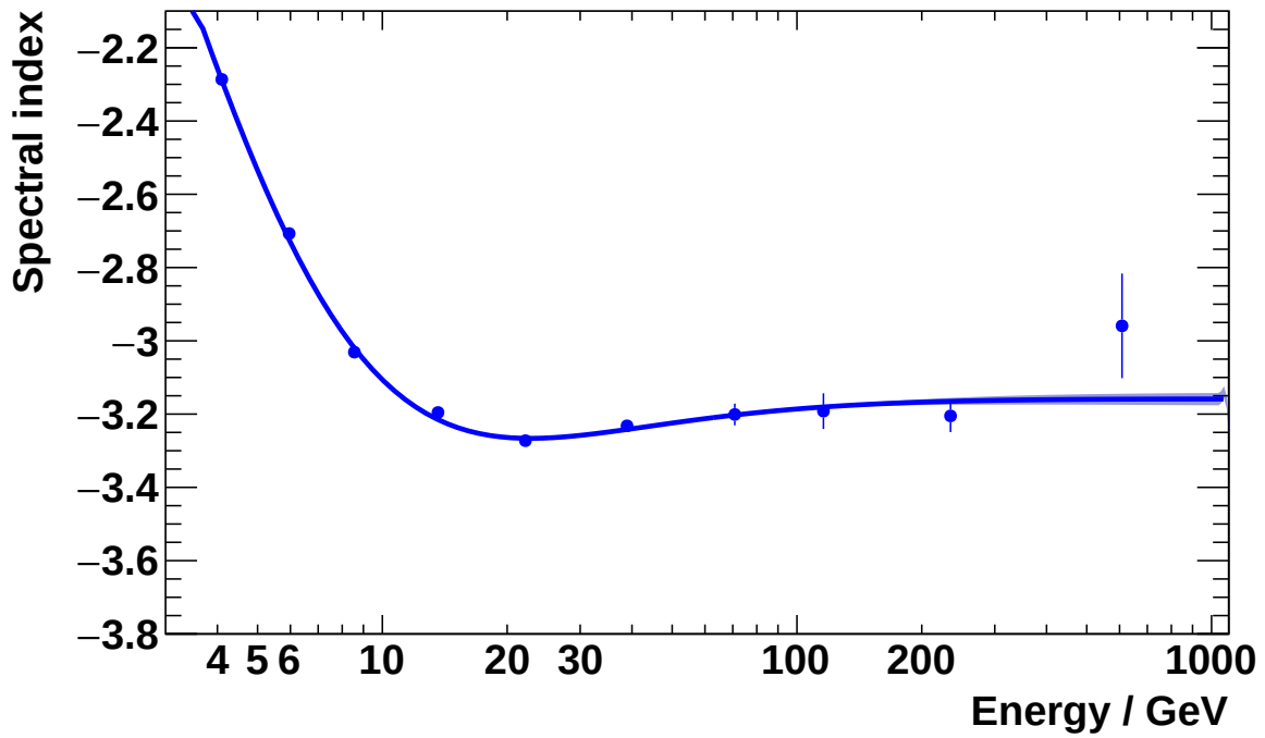
Figure 5.4: The spectral index of the electron flux as function of the energy in non-overlapping energy intervals shown as blue points. The blue band corresponds to the uncertainty determined from a fit of Eq. (5.2) to the data.
