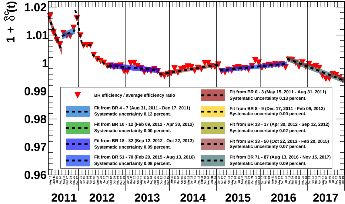
Figure 4.96: Determination of the time-dependent correction factor ( 1 + \hat{\delta}^c(t) ) for the selection cut: “TRD helium rejection” (Section 4.3.3 - Item 4). The red triangle symbols show the ratio: time-dependent cut efficiency over time-averaged cut efficiency for all Bartels rotations (an example of the ratio determined in a single Bartels rotation is shown in Fig. 4.94). The black dashed lines show regions parameterized using straight lines. When the efficiency remains stable over an extended period of time, following a simple trend (e.g. slowly decreasing or constant) a parameterization of the time period is used instead of the individual data points to describe the time dependency. The colored bands indicate the systematic uncertainty on the time-dependent correction factor ( 1 + \hat{\delta}^c(t) ). For individual data points, the uncertainty on the data point - from the previous ratio fit procedure - is taken.
