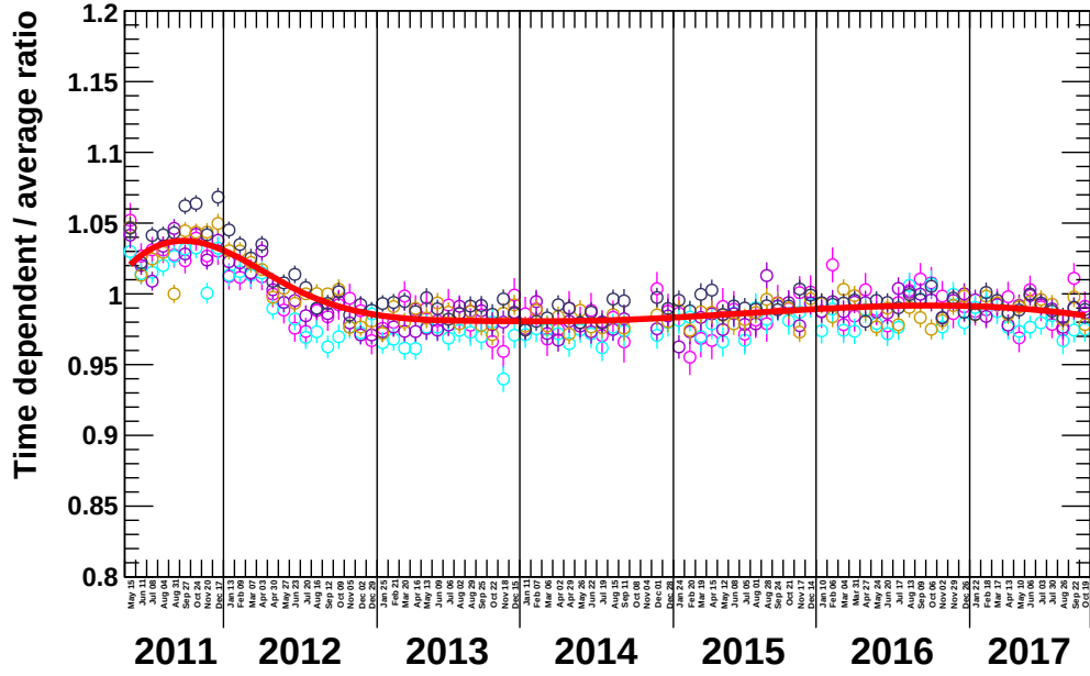
Figure 4.101: Time-dependence of the \sigma_{\text{elec, novo}} parameter for selected energy bins (1.46 – 3.00 GeV), as example, in the time-dependent analysis for the single-track sample.
