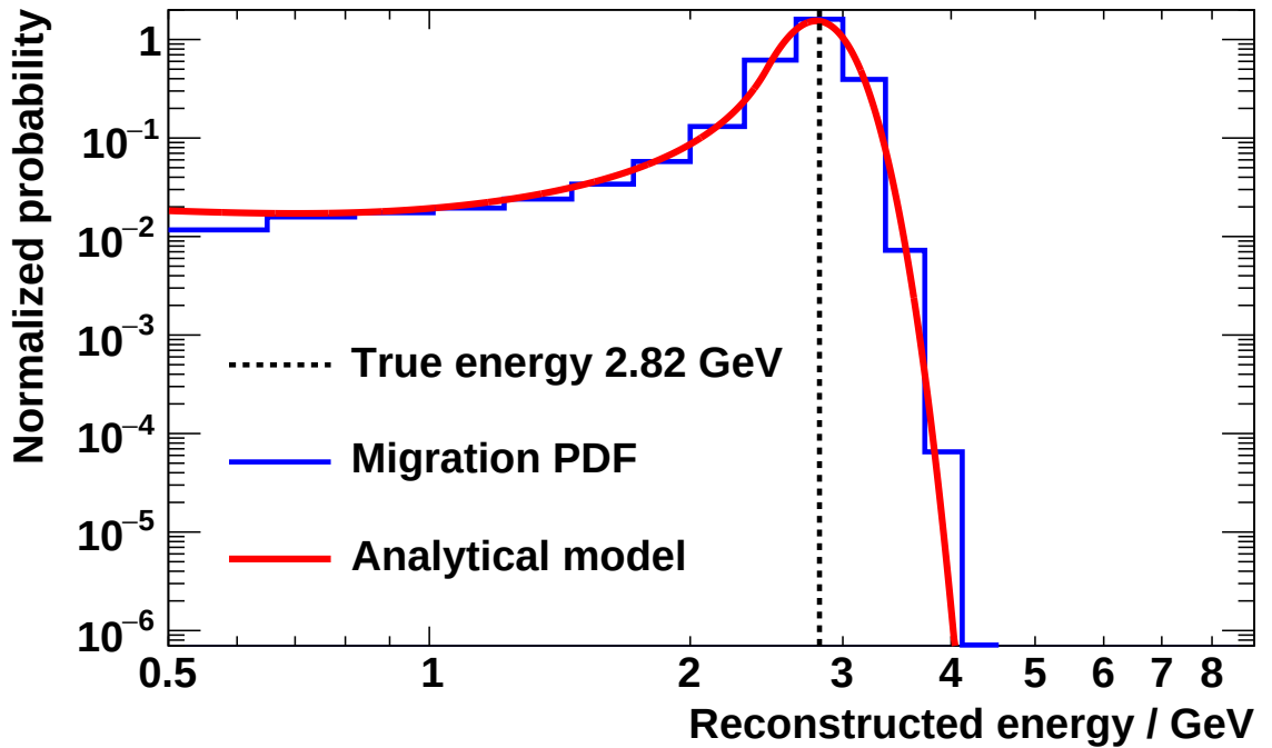
Figure 4.73: Projection of the migration matrix, Fig. 4.62, to the x-axis (reconstructed energy) for a given true energy. The projection is shown as blue histogram and the red line shows the analytical model - Eq. (4.26) - fit to the blue histogram. The black dashed line shows the true energy ( y = 2.82 GeV) for comparison.
