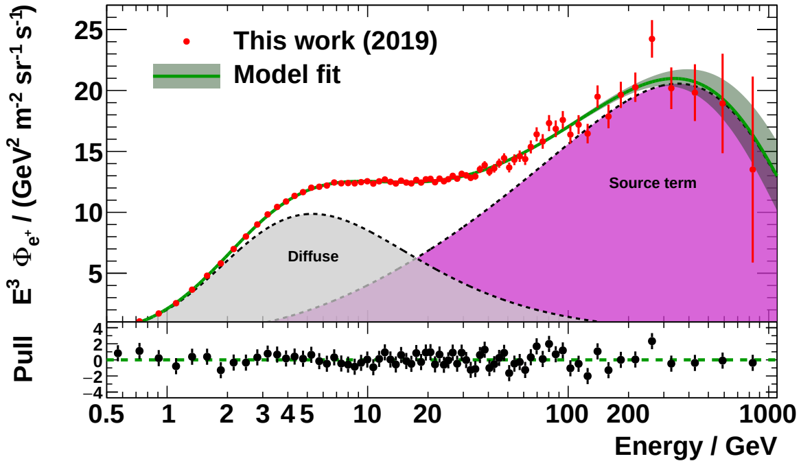
Figure 5.13: The positron flux, scaled with E^3 , is shown as red points. The result of the fit of Eq. (5.4) is shown as green line, enclosed by a green band, indicating the uncertainty of the fit result. The diffuse and source components are indicated by the gray and magenta areas, respectively. The lower plot shows the pull distribution of the fit (data minus model divided by data uncertainty) – the model describes the data accurately over the whole energy range.
