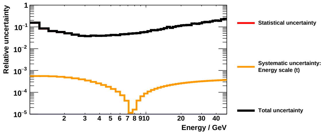
Figure 4.115: Composition of the relative systematic uncertainty associated with the positron/electron ratio.
