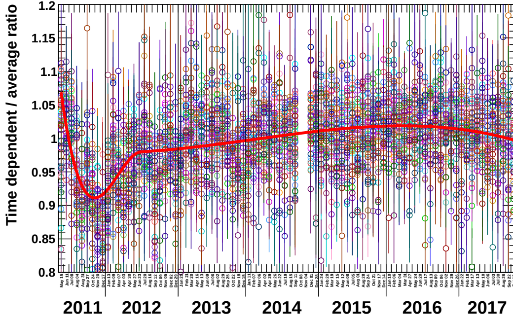
Figure A.26: Time-dependence of the \sigma_{\text{prot, novo}} parameter for selected energy bins (1.72 – 52.33 GeV), as example, in the time-dependent analysis for the multi-tracks sample.
