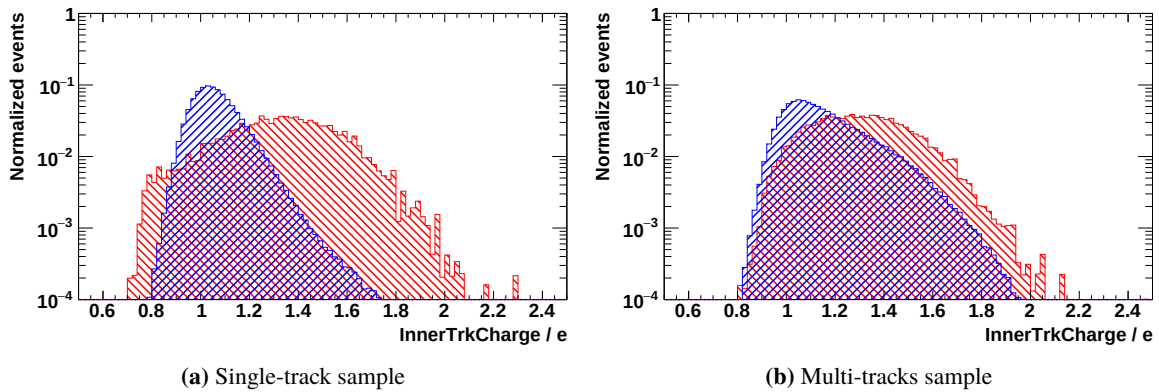
Figure 4.4: Example of \text{InnerTrkCharge} distribution in the energy bin 17.98 – 18.99 GeV in the electron Monte-Carlo simulation. The red histogram shows the charge-confused sample ( R > 0 ) and the blue histogram the correct reconstructed sample ( R < 0 ), after applying all preselection, selection and e^\pm identification cuts.
