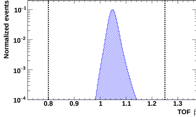
Figure 4.12: Plot of the TOF velocity \beta in the energy range 0.5 - 1,000 GeV for the electron Monte-Carlo simulation. The applied lower and upper cut values are shown as black dashed lines. The chosen cut values are loose: all signal events are kept and only a few slow protons/ions at low energies are rejected.
