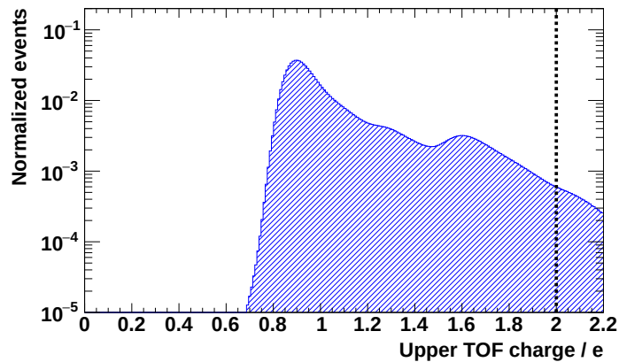
Figure 4.13: Plot of the charge measurement in the upper TOF in the energy range 0.5 - 1,000 GeV for the electron Monte-Carlo simulation. The applied upper cut value is shown as black dashed line.
