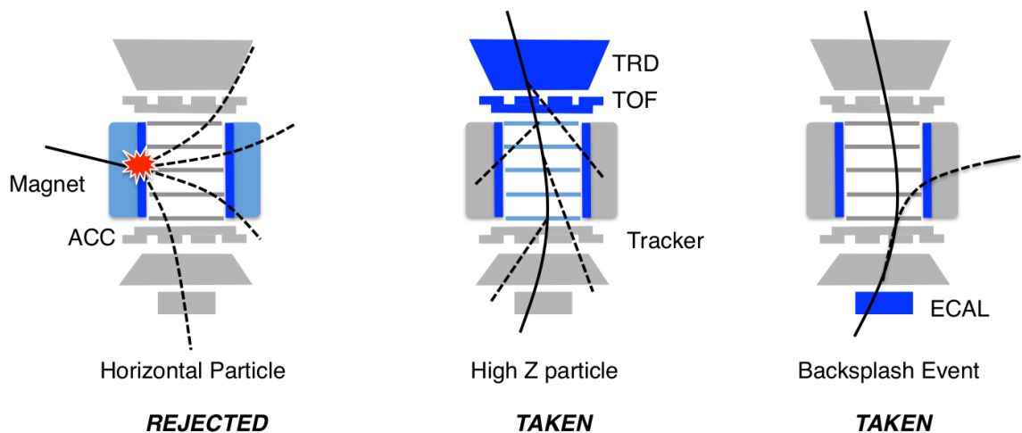
Figure 3.16: Illustration of the operation mode of the ACC. Credit: Ref. [AmsWebsite]
