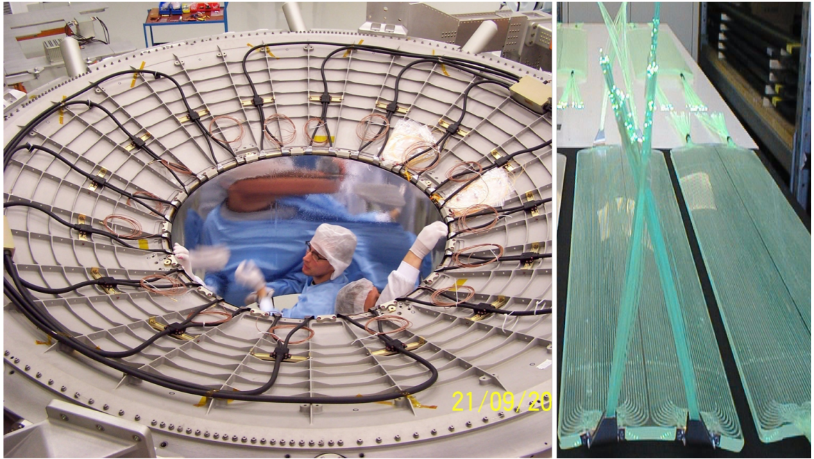
Figure 3.15: Picture of the ACC during construction. Credit: Ref. [AmsWebsite]
