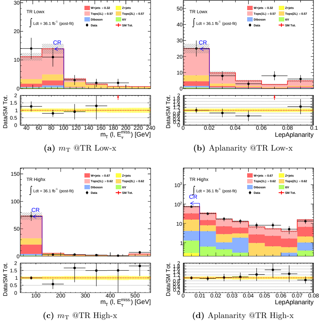
Figure C.4.6: Distributions in m_T , aplanarity and topness in TR Low-x and TR High-x after the MC normalization in CRs. The yellow band in the bottom panel represents only statistical error. The overflow is included in the highest bin.
