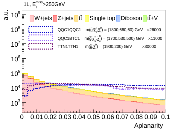
(f) Aplanarity
