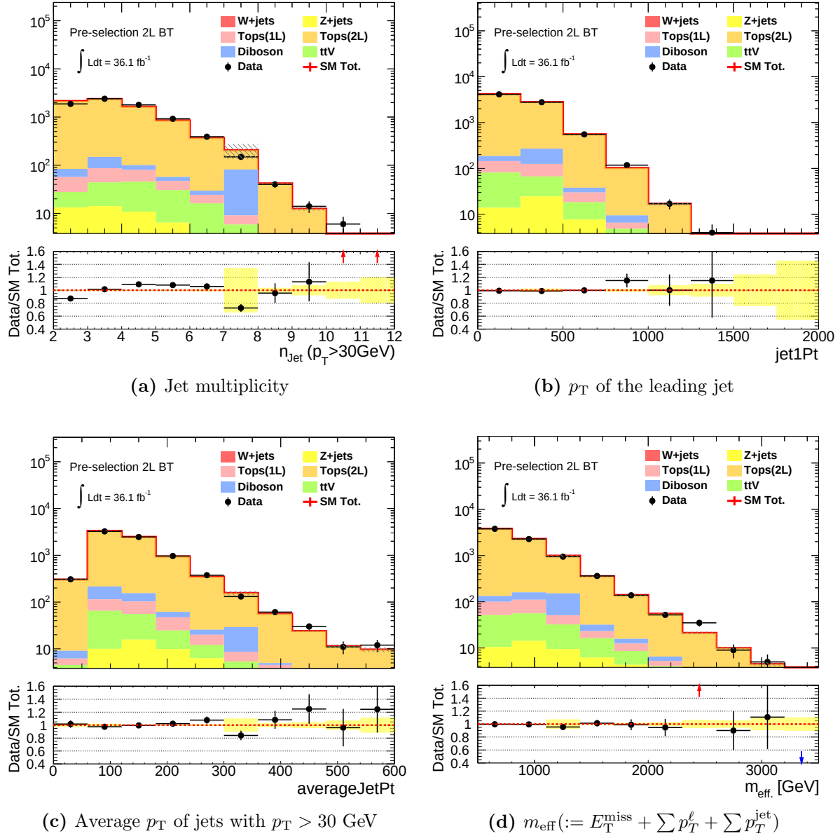
Figure C.1.5: Kinematical distribution of data (black dots) and MC (colored stack) in the 2LBT pre-selection region, reweighting w = 1.05 \times [1 - 0.061 \times p_T(t\bar{t})] being applied for t\bar{t} MC.
