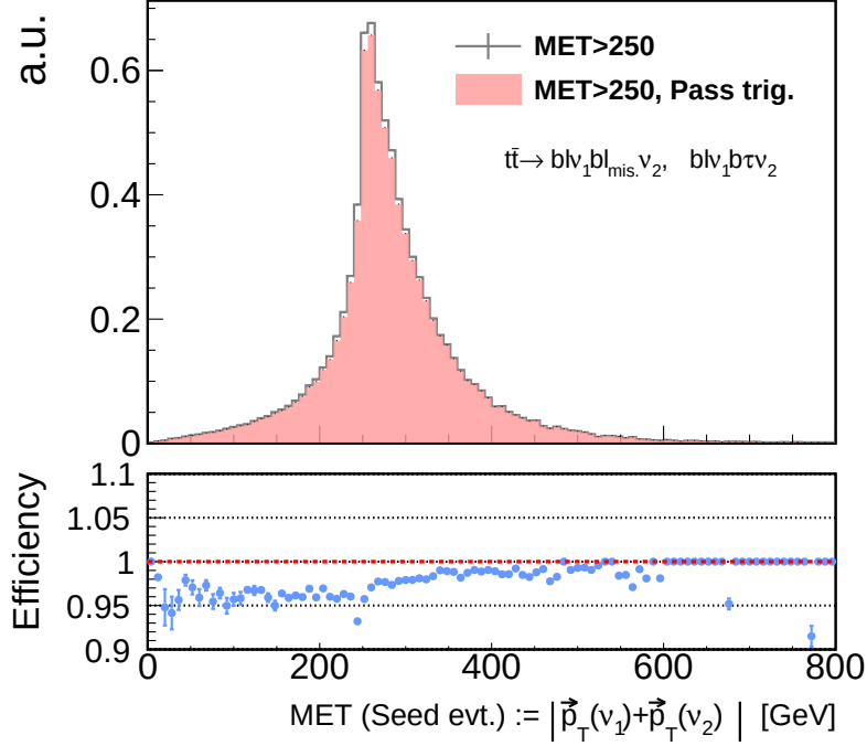
Figure 7.18: Seed MET distribution (gray) for the \ell\ell_{\text{mis.}} and \ell\tau_h events from t\bar{t} resulting in E_T^{\text{miss}} > 250 GeV. The seed MET is defined by the vectorial sum of neutrinos from top decays: |\mathbf{p}_T(\nu_1) + \mathbf{p}_T(\nu_2)| , which is roughly equivalent to the MET in corresponding seed events ( t\bar{t} \rightarrow b\ell\nu_1\bar{b}\ell\nu_2 ). Over 95% of the seed events are shown to be accepted by the combined trigger strategy defined in Table 7.9 (pink).
