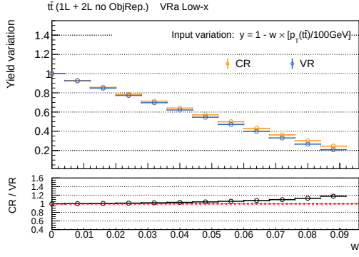
(b) VRa/CR Low-x for t\bar{t}
