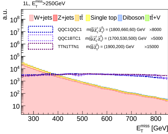
(c) E_T^{\text{miss}}
