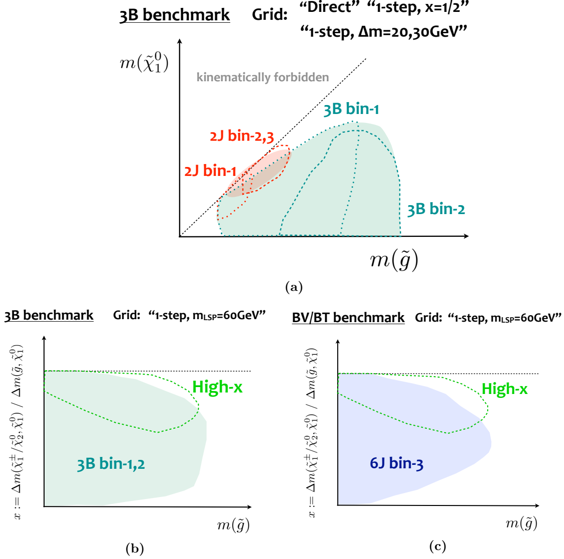
Figure 6.8: Sensitivity coverage by individual signal region towers (shades) or m_{\text{eff}} -bins (dashed contours) (a) to the 3B benchmark models in the Direct, x=1/2 , DM20 and DM30 grids, (b) in the LSP60 grid, and (c) to the BT/BV benchmark models in the LSP60 grid.
