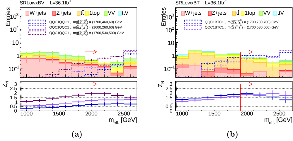
Figure 6.14: m_{\text{eff}} distribution in the (a) b-vetoed (BV) and (b) b-tagged (BT) slices of the optimized Low- x signal region. The red arrow indicates the cut position of m_{\text{eff}} . Bottom row display the sensitivity Z_N := S/\sqrt{B + \alpha^2 B^2} for each reference signals.
