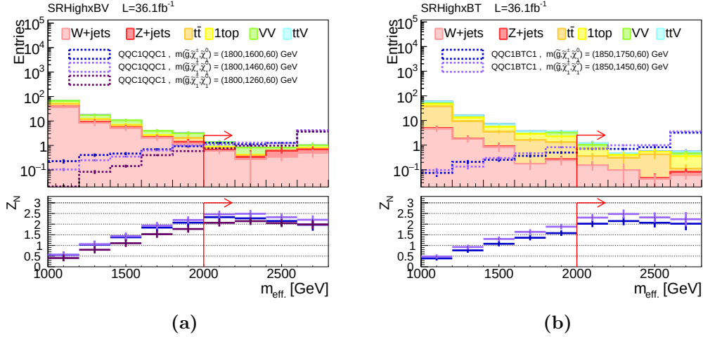
Figure 6.15: m_{\text{eff}} distribution in the (a) b-vetoed (BV) and (b) b-tagged (BT) slices of the optimized High- x signal region. The red arrow indicates the cut position of m_{\text{eff}} . Bottom row display the sensitivity Z_N := S/\sqrt{B + \alpha^2 B^2} for each reference signals.
