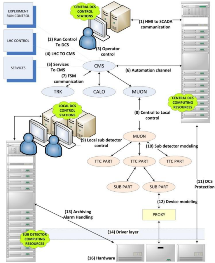
Figure 4.1: A schematic view of main CMS DCS with its sub-DCS. (Bauer et al., 2012).
