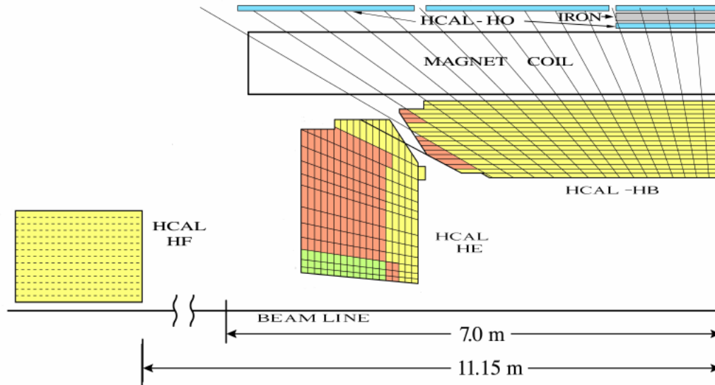
Figure 3.8: A schematic view of the HCAL. (TDR, 2006).
