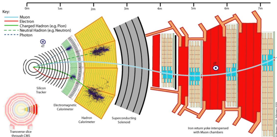
Figure 3.4: Sublayers of CMS detector with different signatures of the particles. (Murnane, 2014).
