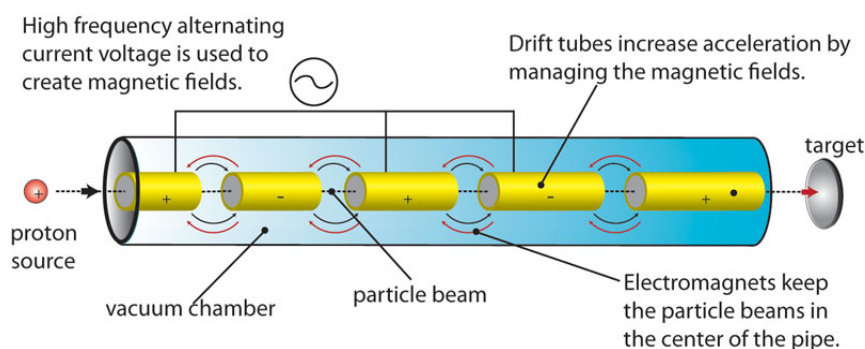
Figure 2.3: Design of a linear accelerator. ( The Atomic Age, A Linda Hall Library Exhibition , Unknown).
