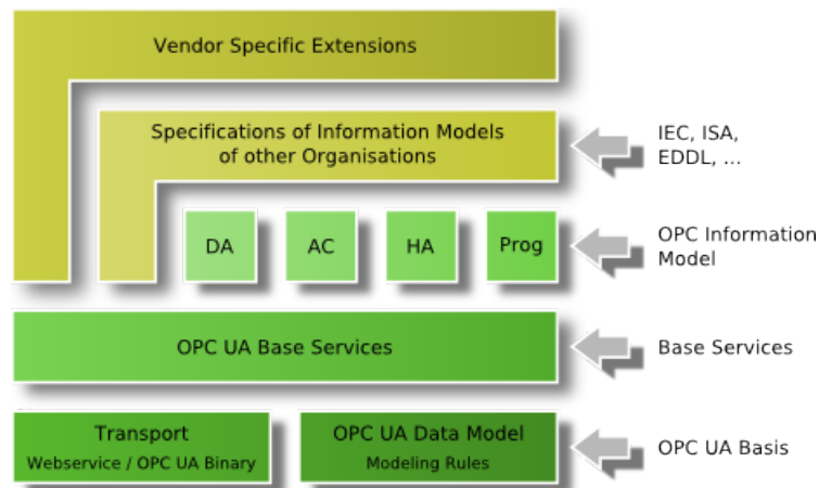
Figure 7.2: The OPC UA structure that composed variety layers. (Automation, n.d.-c).
