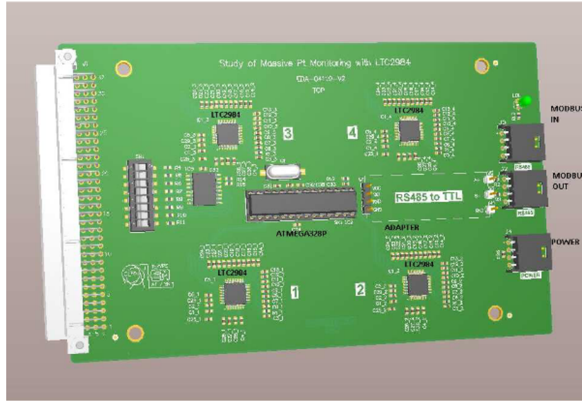
Figure 6.13: The Stage 2 of the MTRS board.
