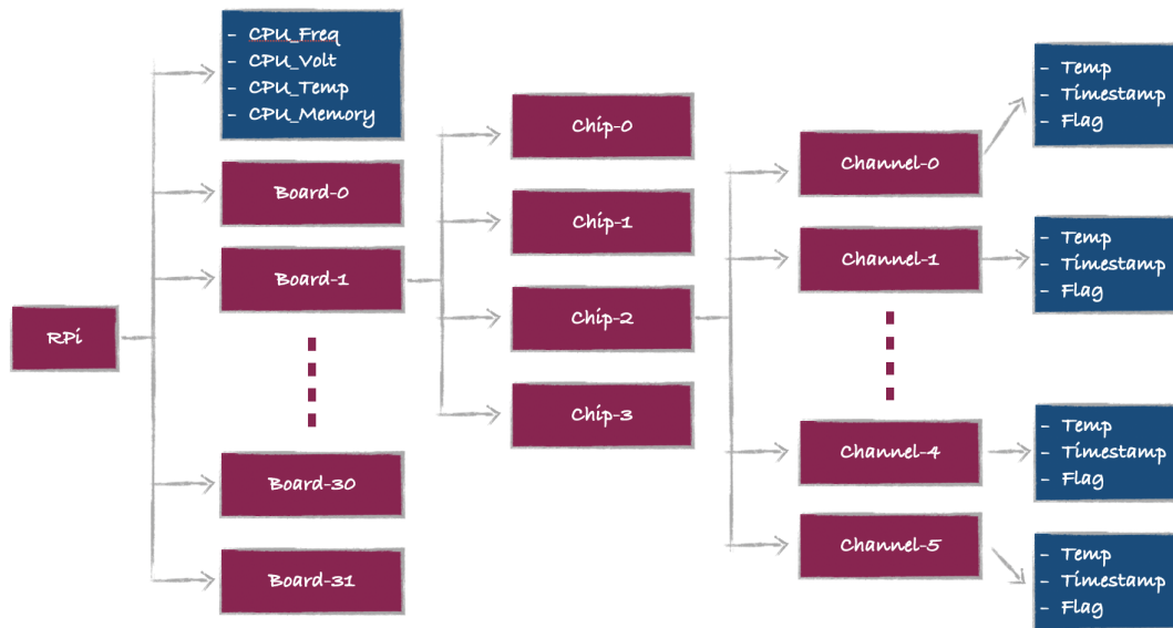
Figure 6.8: An overview of MTRS structure.
