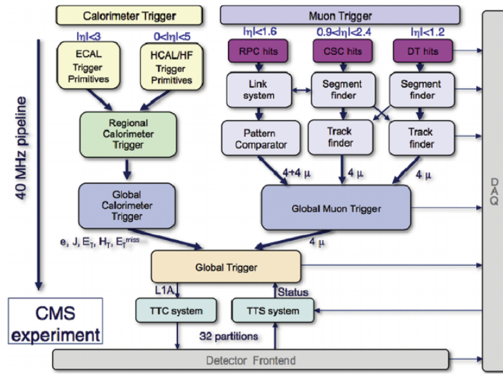
Figure 3.11: Data flow in L1 triggering system of the CMS detector. (Jeitler, 2013).
