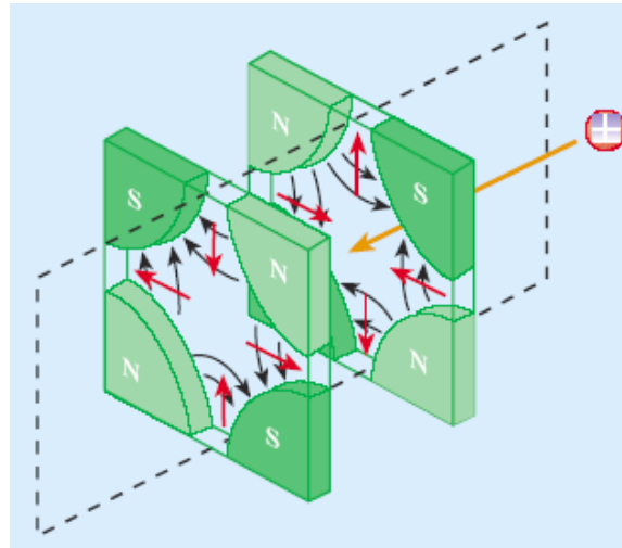
Figure 2.9: F and Q type quadrupole magnets. (Cid-Vidal X. and Cid R., 2010).
