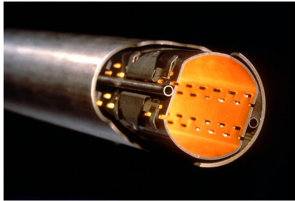
Figure 2.7: The cross section of LHC ultra-high vacuum pipe. (Kahle, Steerenberg, & Pandolfi, 2017).
