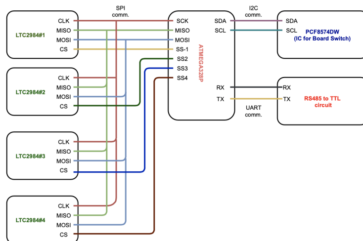
Figure 6.6: Three different communication protocols were used with Atmega328P.
