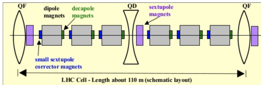
Figure 2.10: The structure of each arc cell at the LHC. Dipole magnets aims to keep the beams inside the ring and quadrupole magnets focus them in both directions. (Wenninger, n.d.).
