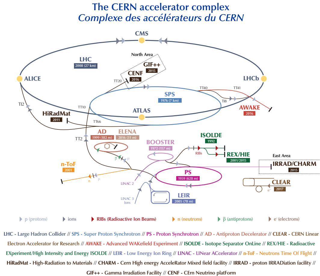
Figure 2.4: Accelerator complex at CERN. (Mobs, 2018).
