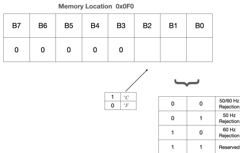
Figure 5.11: The global configuration register of the LTC2984 chip is used for defining the notch frequency and temperature format.
