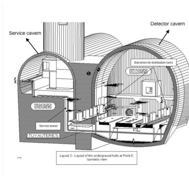
Figure 3.2: CMS cavern consists of UXC (experimental cavern) and USC (underground cavern). (Focardi, 2008).
