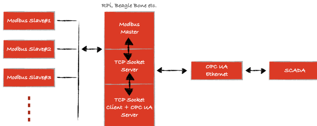
Figure 6.11: The rich implementation of the MTRS with intermediary partner.
