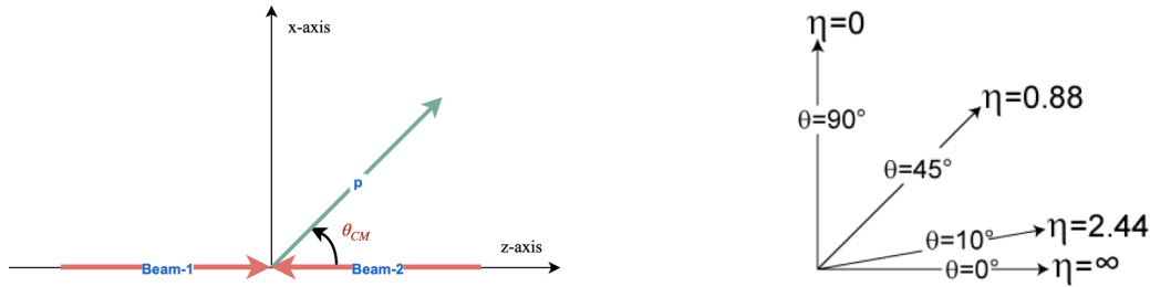
Figure 3.3: (a) Illustration of the longitudinal scattering angle \theta_{CM} is presented (left) and (b) a variety of pseudorapidity corresponding to different values of \theta_{CM} is given (right).
