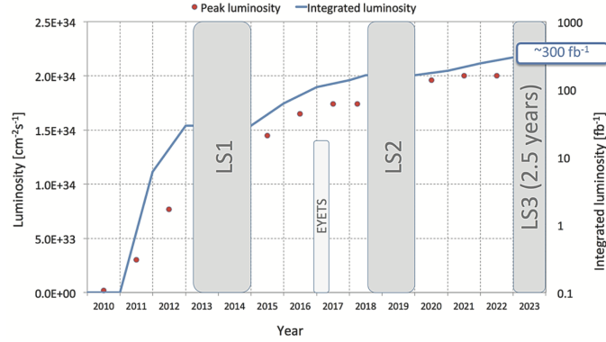
Figure 2.5: Instantaneous the LHC luminosity over 10 years with the evolution of possible peak luminosity at LHC.
