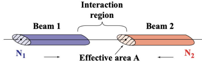
Figure 2.1: Instantaneous luminosity is calculated by taking the geometry of the bunches of protons and the parameters of the beam into consideration.
