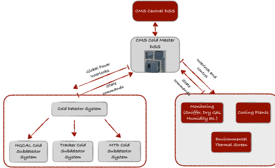
Figure 4.3: CMS Cold Detector Safety System.
