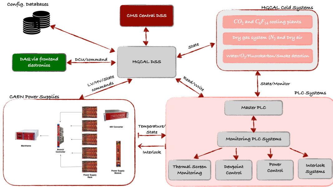
Figure 4.2: Overview of HGCAL Detector Safety System.
