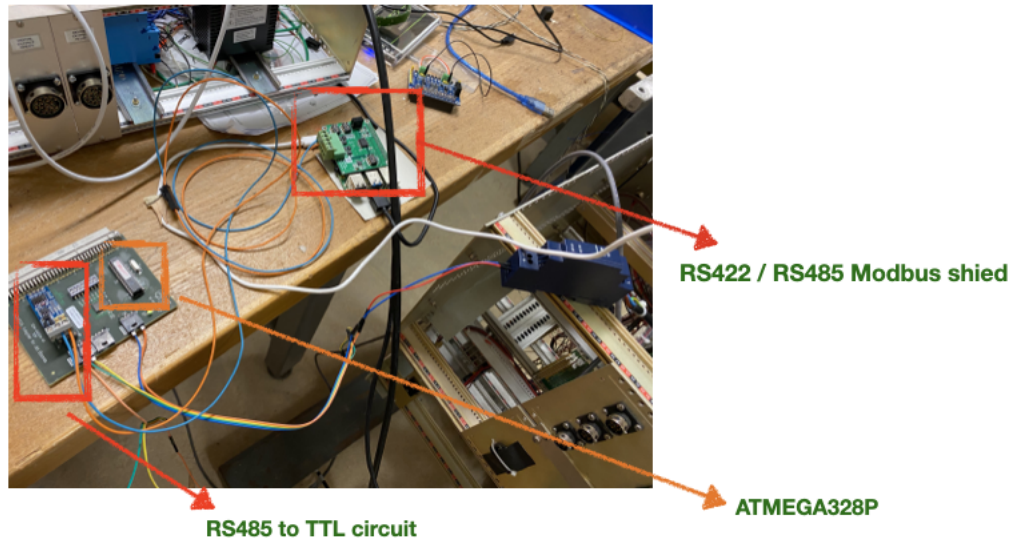
Figure 6.5: Adaptor Board including RS485 and ATMEGA328P is connected to RS422/RS485 Modbus shield onto Raspberry Pi 4B+.
