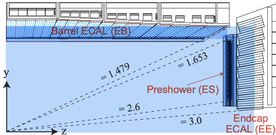
Figure 3.7: The ECAL sublayer of CMS detector. (TDR, 2006).
