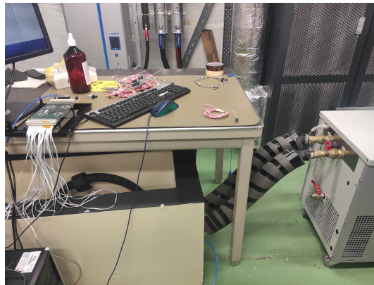
Figure 6.3: It is the first version of MTRS board which were connected Arduino to the first VME input and tied chiller via sensors to its second VME input.
