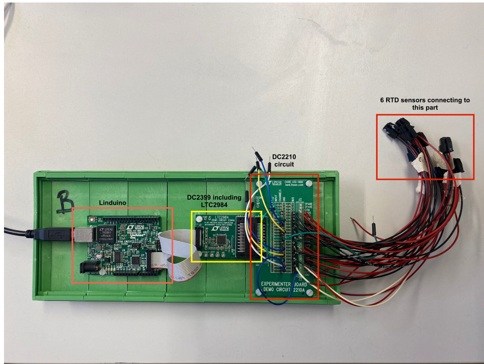
Figure 5.4: The DC2420 evaluation kit comprises of Linduino, DC2399 circuit including LTC2984 chip and DC2210 circuit for connection of six RTD sensors.
