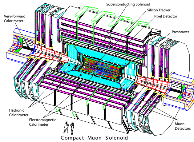
Figure 3.1: Labelled schema of the CMS detector. (Drollinger, 2006).
