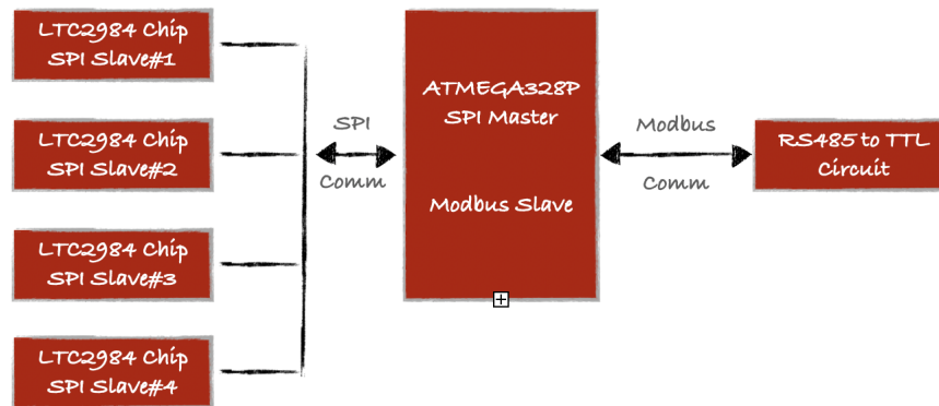
Figure 6.9: Board connectivity with minimal implementation (adaptor board).
