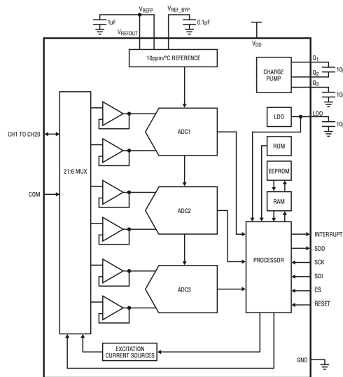
Figure 5.3: Blok diagram of the LTC2984 chip. (Device, n.d.-b, p. 11)
