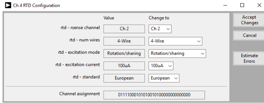
Figure 5.6: Configuration of a RTD sensor tied to Channel-4 is performed using QuikEval software.
