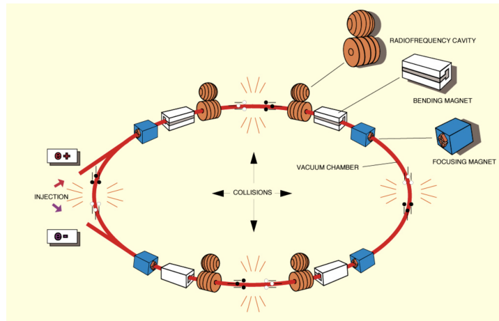
Figure 2.2: A circular accelerator with RF cavities, bending and focusing magnets. (Burnet, 2016).
