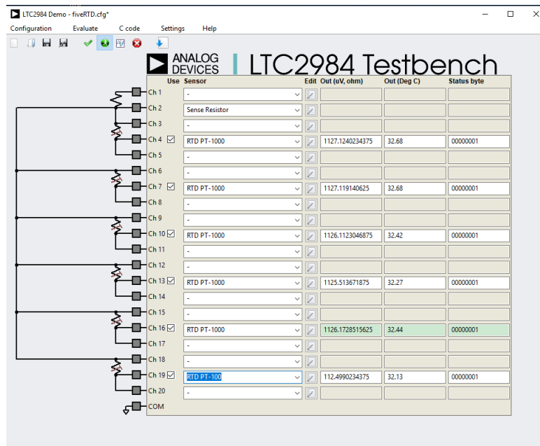
Figure 5.5: Configuration of five RTD PT-1000 and a RTD PT-100 sensors tied to LTC2984 board.
