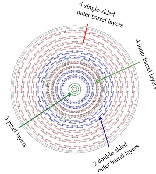
Figure 3.6: The barrel part of CMS Tracker in xy plane. (Luciano, 2017).
