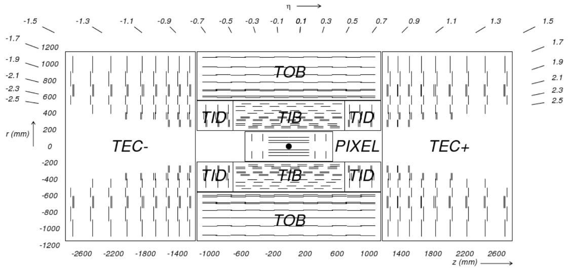
Figure 3.5: Schematic view of CMS Tracker in r-z plane. (TDR, 2006).
