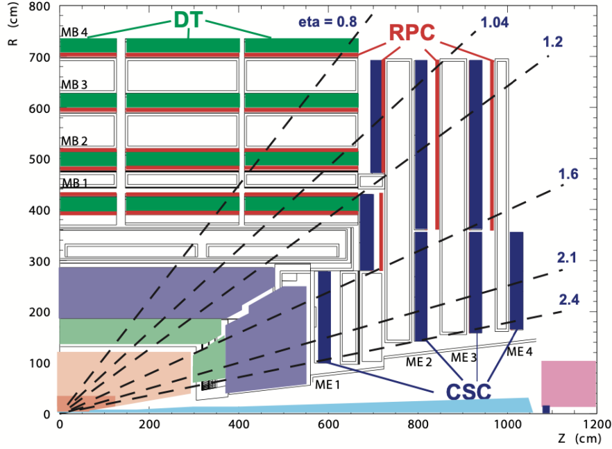
Figure 3.9: The muon chamber with its three gaseous detectors. (TDR, 2006).
