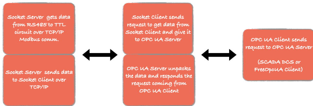
Figure 7.1: The sensor data flow from the boards to the DCS by developing socket server/client and OPC UA server/client.
