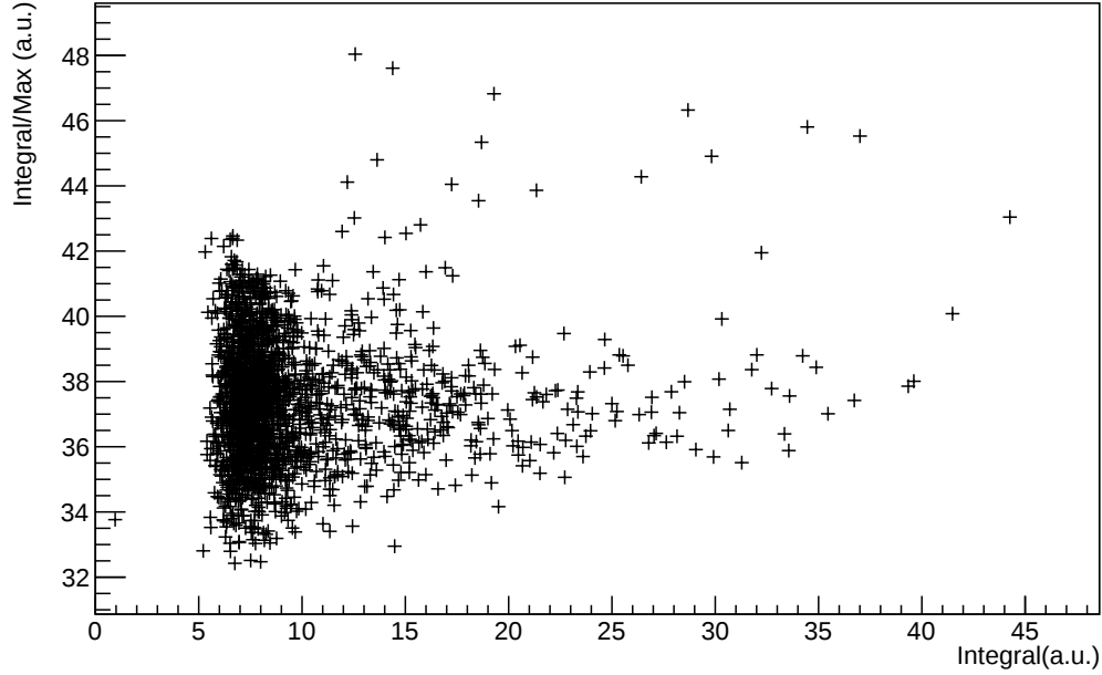
Figure 2.6: Example integral/maximum distribution before applying the final cut.
