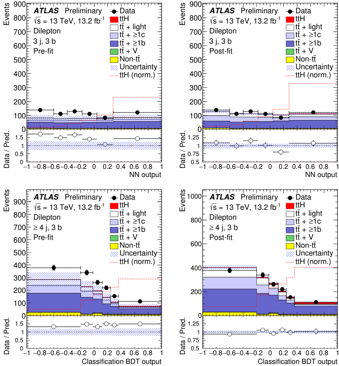
Figure 5.11: Comparison of the data and prediction before (left) and after (right) performing the combined single-lepton and dilepton fit. Shown is the neural network output in the (3j, 3b) analysis region (top), and the boosted decision tree output in the ( \geq 4j , 3b) analysis region (bottom), which both entered the fit. The t\bar{t}H distribution (solid) is normalised to the SM predicted cross section before the fit and to the best-fit cross section after the fit. The dashed line shows the t\bar{t}H distribution normalised to the total yield (from [7]).
