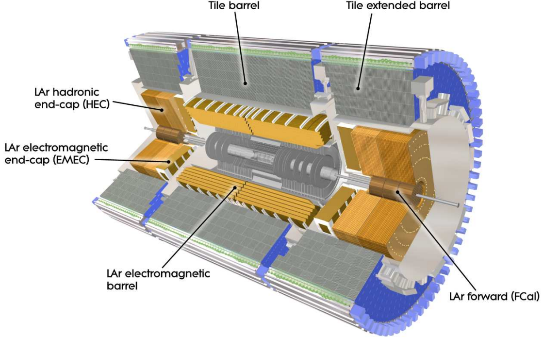
Figure 2.6: A diagram showing the layout of the calorimeters in ATLAS (from [33]).
