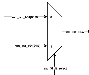
(b) Channel RAM wishbone read multiplexer.
