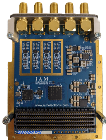
Figure 1.6: IAM500 mezzanine back view.
