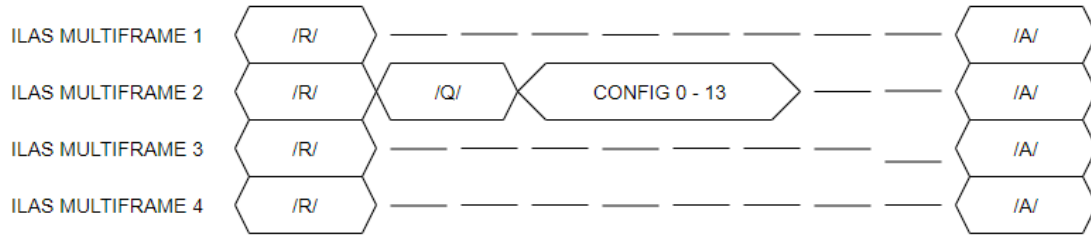
Figure 2.13: ILAS phase.
