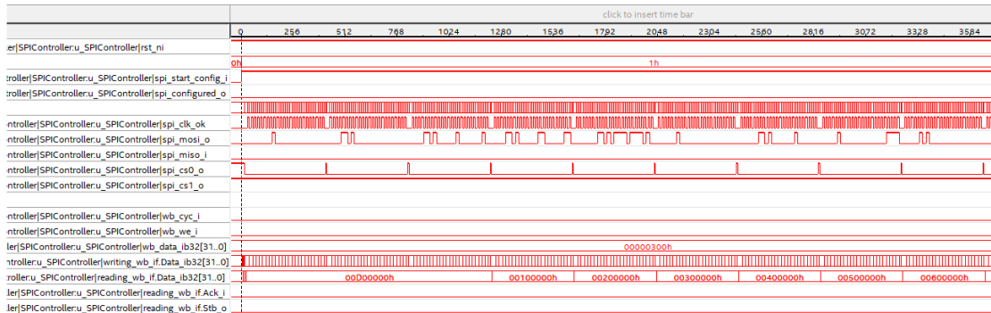
Figure 3.34: Signal Tap output for SPI Controller.
