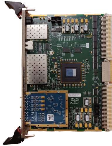
(b) VFC with a IAM500 mezzanine installed.
