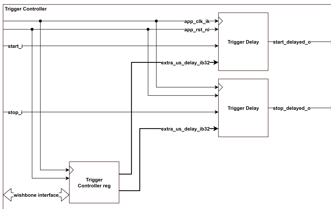
Figure 3.31: Trigger controller module in detail.
