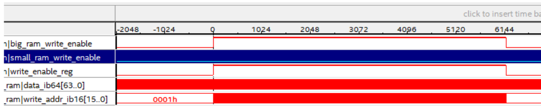
Figure 3.50: RAM Controller Signal Tap output for writing.
