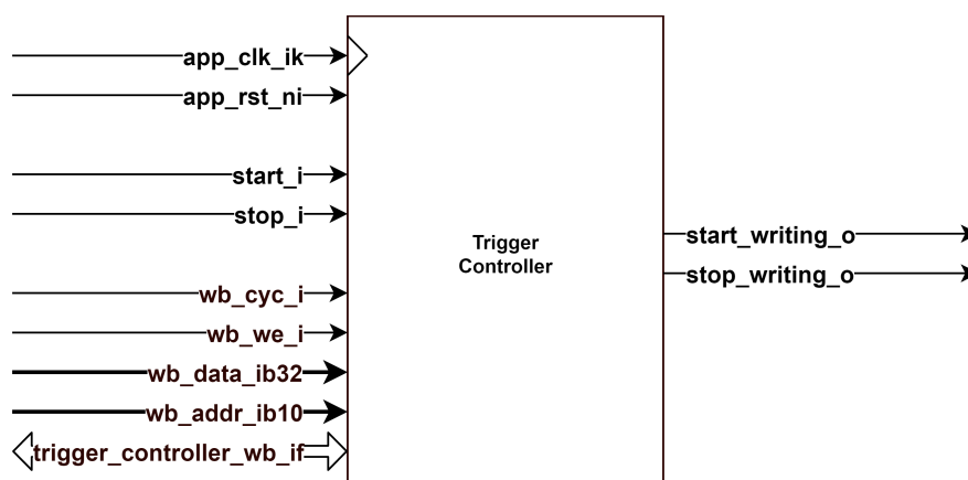
Figure 3.30: Trigger controller module.
