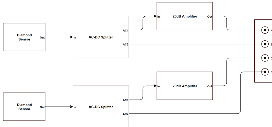
Figure 2.2: Analog front-end.
