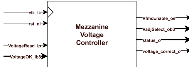
Figure 3.7: MezzanineVoltageController module.
