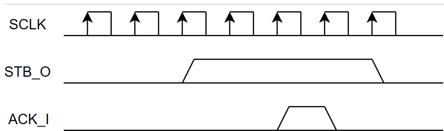
Figure 2.20: Wishbone Handshake.
