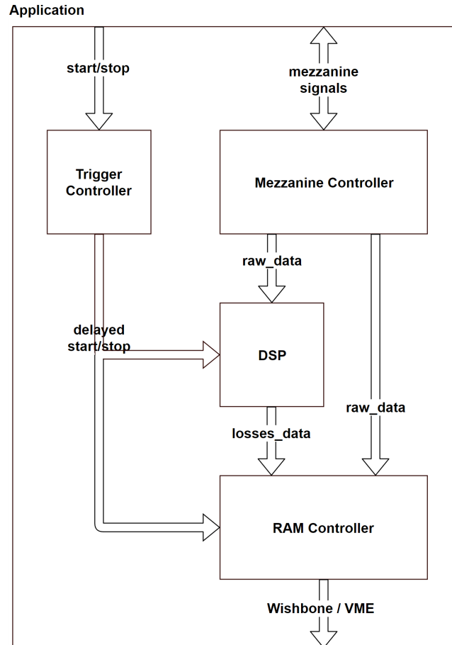
Figure 3.2: Firmware architecture.
