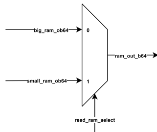
(a) Channel RAM read select multiplexer.
