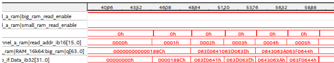
Figure 3.51: RAM Controller Signal Tap output for reading.
