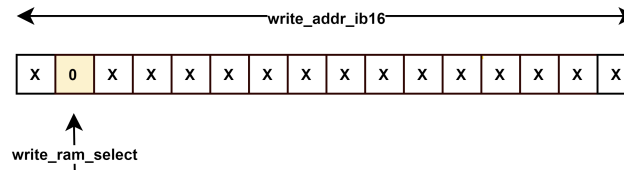
Figure 3.25: Channel RAM write address.
