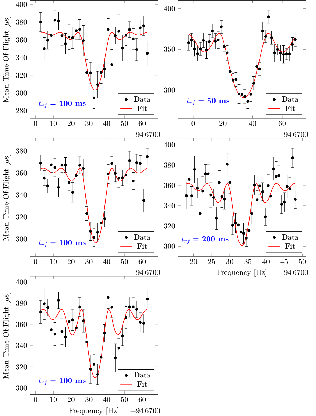
Figure B.2.: TOF resonances of ^{96}\text{Kr}^+ from the precision Penning trap. Excitation time T_{rf} = 100 \text{ ms} (left), T_{rf} = 50 \text{ ms} (top right) and T_{rf} = 200 \text{ ms} (bottom right).
