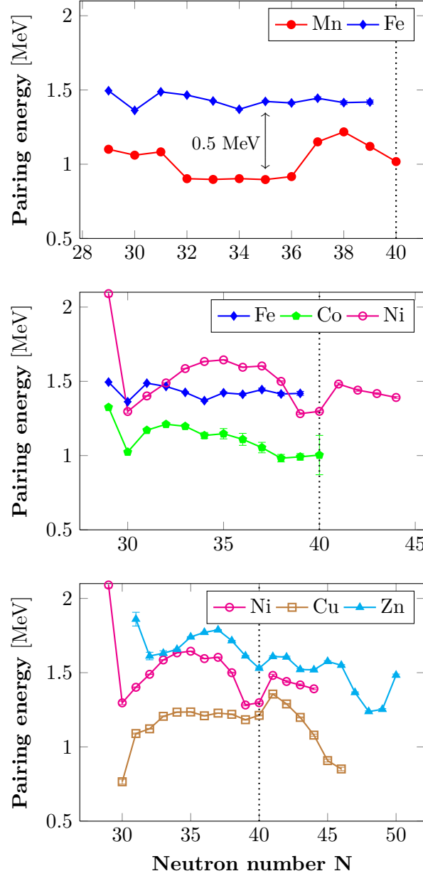
Figure 6.15.: The experimental pairing energies plotted with N for 25 < Z < 30 (Mn, Fe, Co, Ni, Cu and Zn).
