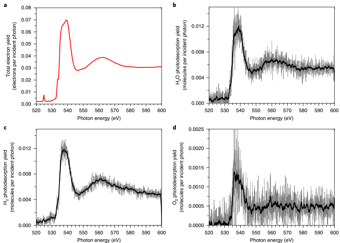
Fig. 2 | Photodesorption yields of the neutral species observed, as a function of photon energy. a–d, Total electron yield ( a ) in electrons per incident photon, and H 2 O ( b ), H 2 ( c ) and O 2 ( d ) photodesorption yields in molecules per incident photon, as a function of photon energy, for a 100 ML compact amorphous solid water ice at 15 K. The grey traces are the raw data, and the black traces have been smoothed. The total electron yield is assumed to represent the absorption of the ice (see Methods).
