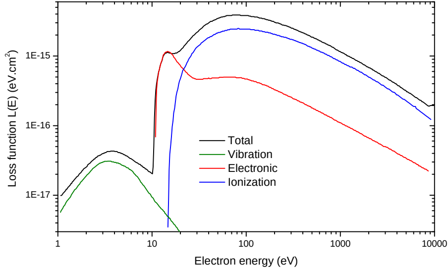
Figure V.15: Loss function of electrons in \text{H}_2 , as a function of electron energy. The total loss function is displayed in black, and the contribution of vibration excitation, electronic excitation and ionization are displayed respectively in green, red and blue. The curves are directly taken from ref. [333].
