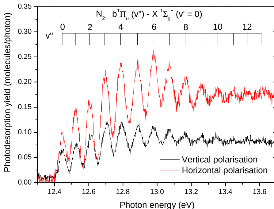
Figure IV.31: Photodesorption yield of \text{N}_2 in vertical (black line) and horizontal (red line) polarization settings. The vibronic peaks of the electronic transition are attributed on the figure.
