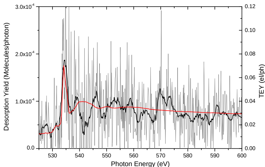
Figure VI.13: Photodesorption spectrum of neutral \text{C}_2\text{O} from solid CO near the O 1s edge. In grey is the raw data, the black line is a smooth. The TEY (red line, normalized so as to roughly match the photodesorption spectrum) is also shown for comparison. This ice had already been irradiated with a high photon dose and the scan was done with a high photon flux: \sim 1.4 \times 10^{13} \text{ ph.s}^{-1} .
