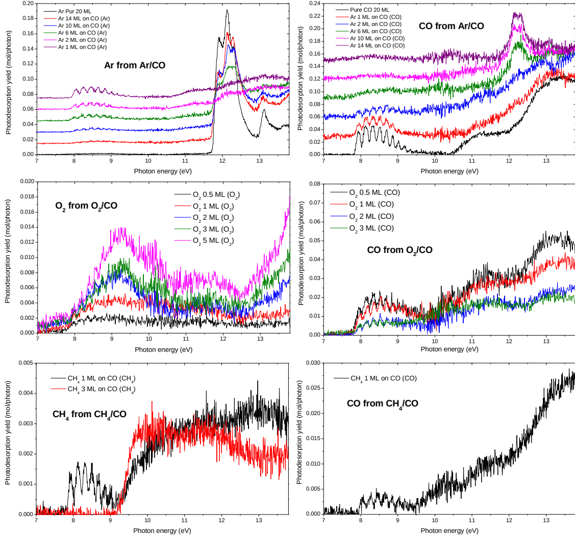
Figure IV.36: Photodesorption spectra of multiple layers of Ar, \text{O}_2 and \text{CH}_4 on CO. Top: photodesorption of Ar (left) and CO (right) from Ar on CO for several thicknesses. Middle: photodesorption of \text{O}_2 (left) and CO (right) from \text{O}_2 on CO for several thicknesses. Bottom: photodesorption of \text{CH}_4 (left) and CO (right) from \text{CH}_4 on CO for several thicknesses.
