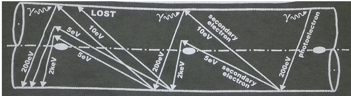
Figure I.8: Principle of the electron cloud effect in accelerators. An initial photon ("γ") from synchrotron radiation ejects a photoelectron (of e.g. 200 eV here), which by hitting the chamber walls eject several secondary electrons with low energies (typically 5-10 eV). These slow electrons can be accelerated by the electric field of a proton bunch to high energies (e.g. 2 keV here) and hit the walls, generating again secondary electrons. Drawing taken from the back of the t-shirts distributed at the e'cloud 18 conference.
