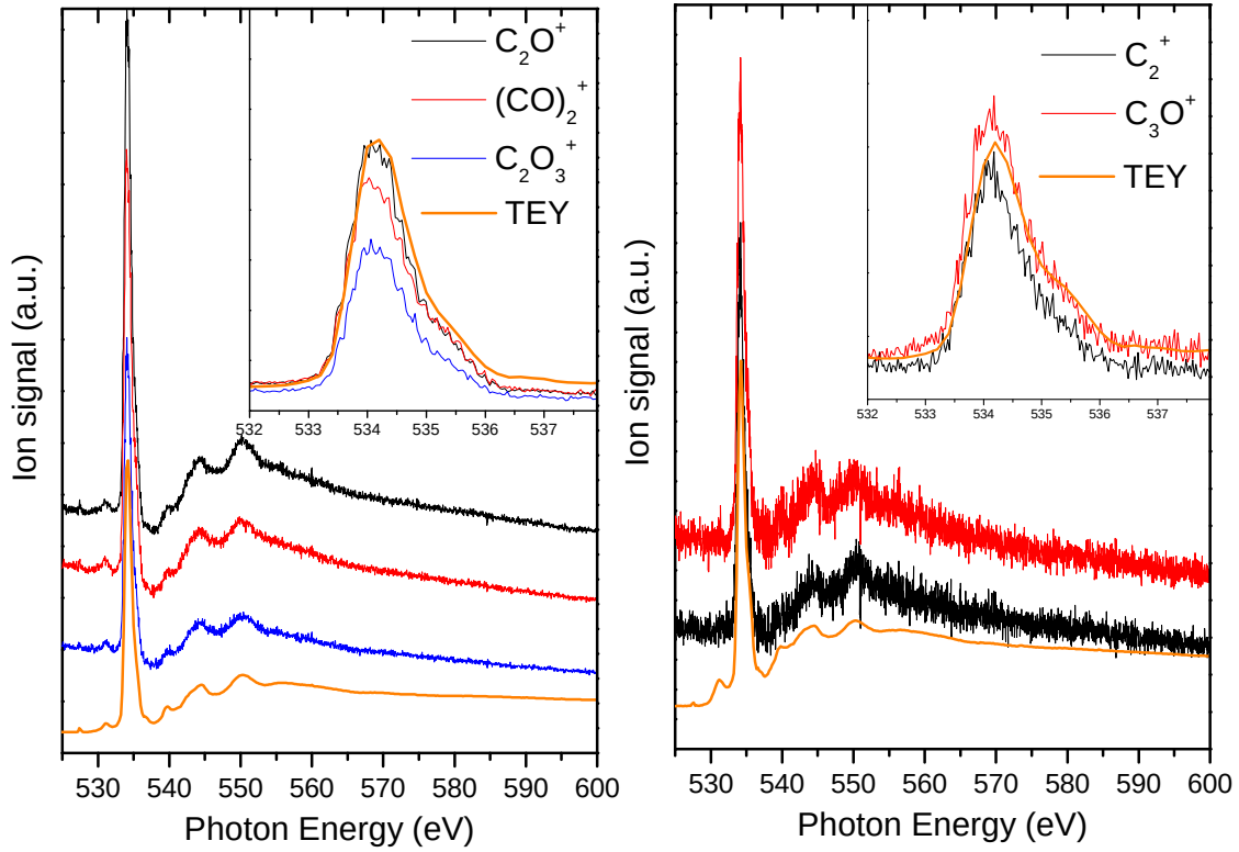
Figure VI.19: Photodesorption spectra of \text{C}_2\text{O}^+ , (\text{CO})_2^+ and \text{C}_3\text{O}_2^+ (left panel), and \text{C}_2^+ and \text{C}_3\text{O}^+ (right panel). For each panel the corresponding ice had already received about two scans worth of photons prior. The respective TEYs are also shown for comparison in orange. The spectra have been offset for clarity.
