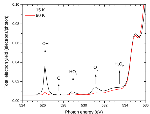
FIG. 2. Total electron yield (TEY) as a function of photon energy in the pre-edge region at 15 K (black trace) and 90 K (red trace) from a compact ASW ice grown at 90 K. Attribution of the peaks following Laffon et al. 34 are indicated.
