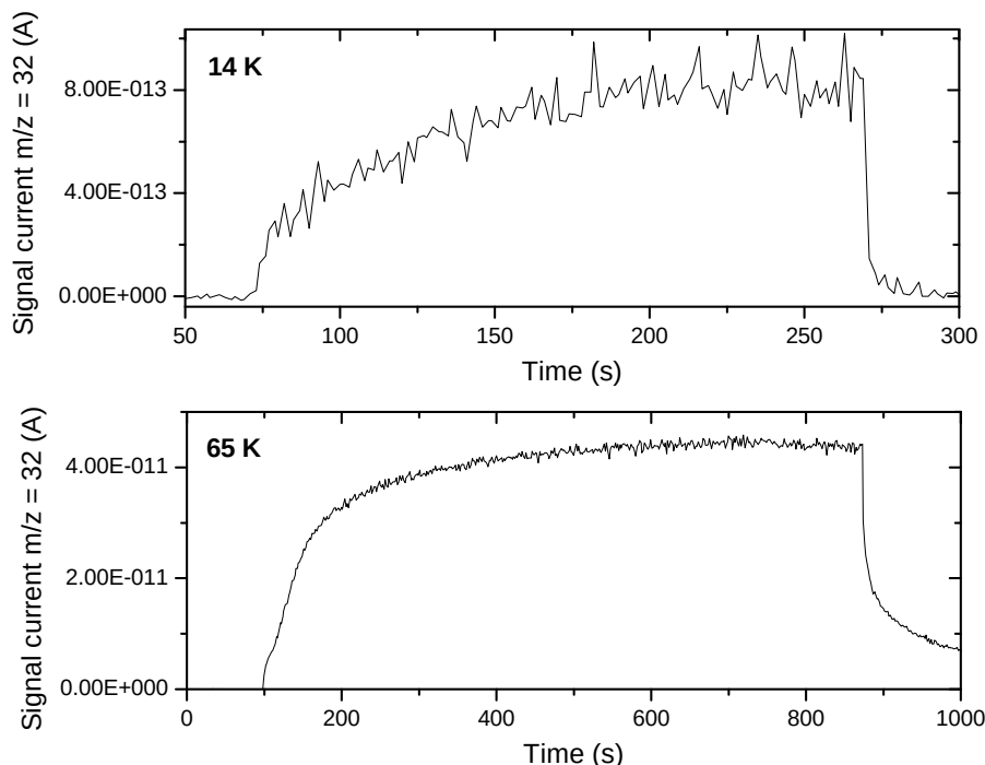
Figure V.11: \text{O}_2 desorption signal as a function of time, for a 200 ML crystalline (grown at 75 K) ice irradiated at either 14 K (upper panel) or 65 K (lower panel).
