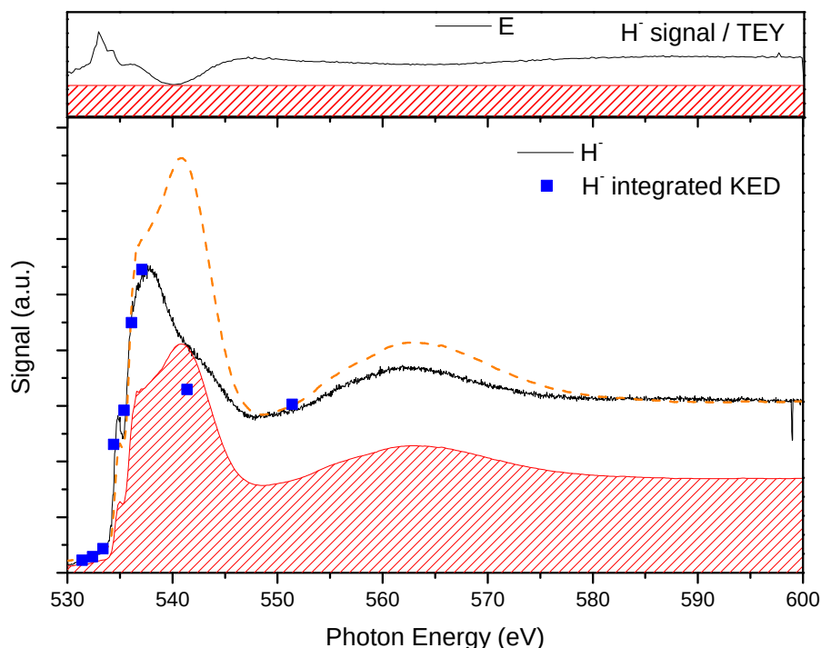
Figure VI.5: Photodesorption spectrum of \text{H}^- at 90 K, at the maximum of kinetic energy (black trace). In blue dots the integrated KEDs of \text{H}^- at 90 K are indicated. The TEY is indicated twice with two different normalizations, by the dashed orange trace and the hashed red area. The inset above represents the \text{H}^- signal divided by the TEY. The red hashed area constrained by the minimum of this curve corresponds to the maximum contribution of XESD to \text{H}^- desorption.
