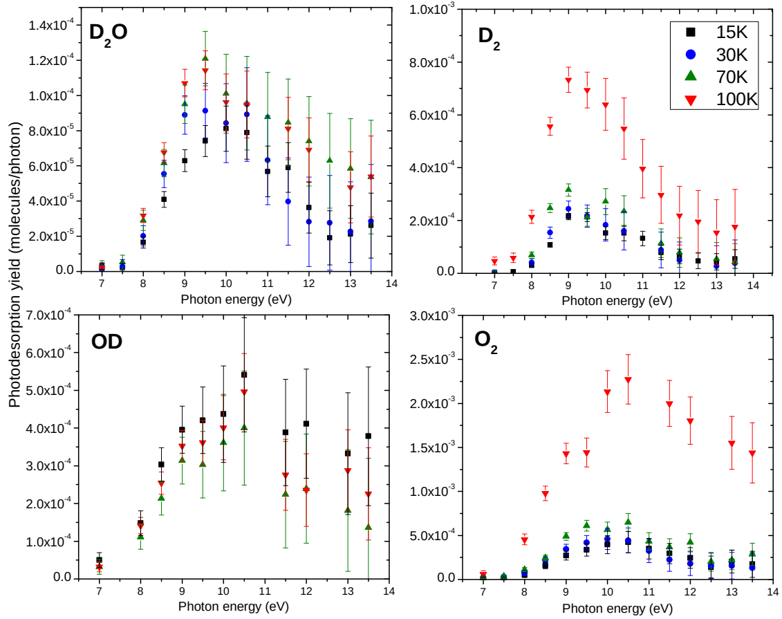
Figure IV.24: Photodesorption spectra of \text{D}_2\text{O} , \text{O}_2 , \text{D}_2 and \text{OD} from 20 ML compact amorphous \text{D}_2\text{O} ice, at different temperatures.
