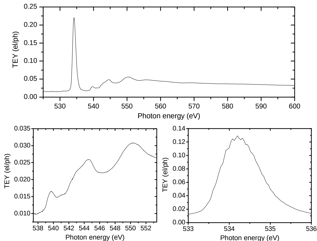
Figure VI.9: Photoabsorption spectrum of solid CO, measured with the TEY. The top panel shows the whole spectrum from 525 to 600 eV, taken with a positive value on the extractor of the Hidden QMS which increases the absolute value of the TEY (in electron per photon) relative to the field-free value. Bottom panels are scans made with more scan steps on specific regions of the spectrum, recorded with negative values of the extractor (which is why the absolute TEY value do not match with the top panel). The bottom right panel is a zoom onto the 533-536 eV region ( \pi^* resonance) and the bottom left panel is a zoom onto the 537-553 eV region. Attributions are made in the text. The spectral resolution of the light is \sim 80 meV.
