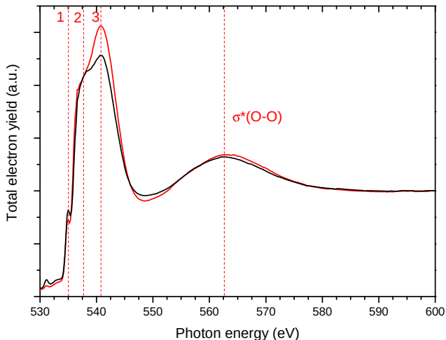
FIG. 1. Total electron yield (TEY) as a function of photon energy at 15 K (black trace) and 90 K (red trace) from c-ASW grown at 90 K. The curves have been normalized at 600 eV. The water features are indicated by vertical dashed red lines (see the text for attributions).
