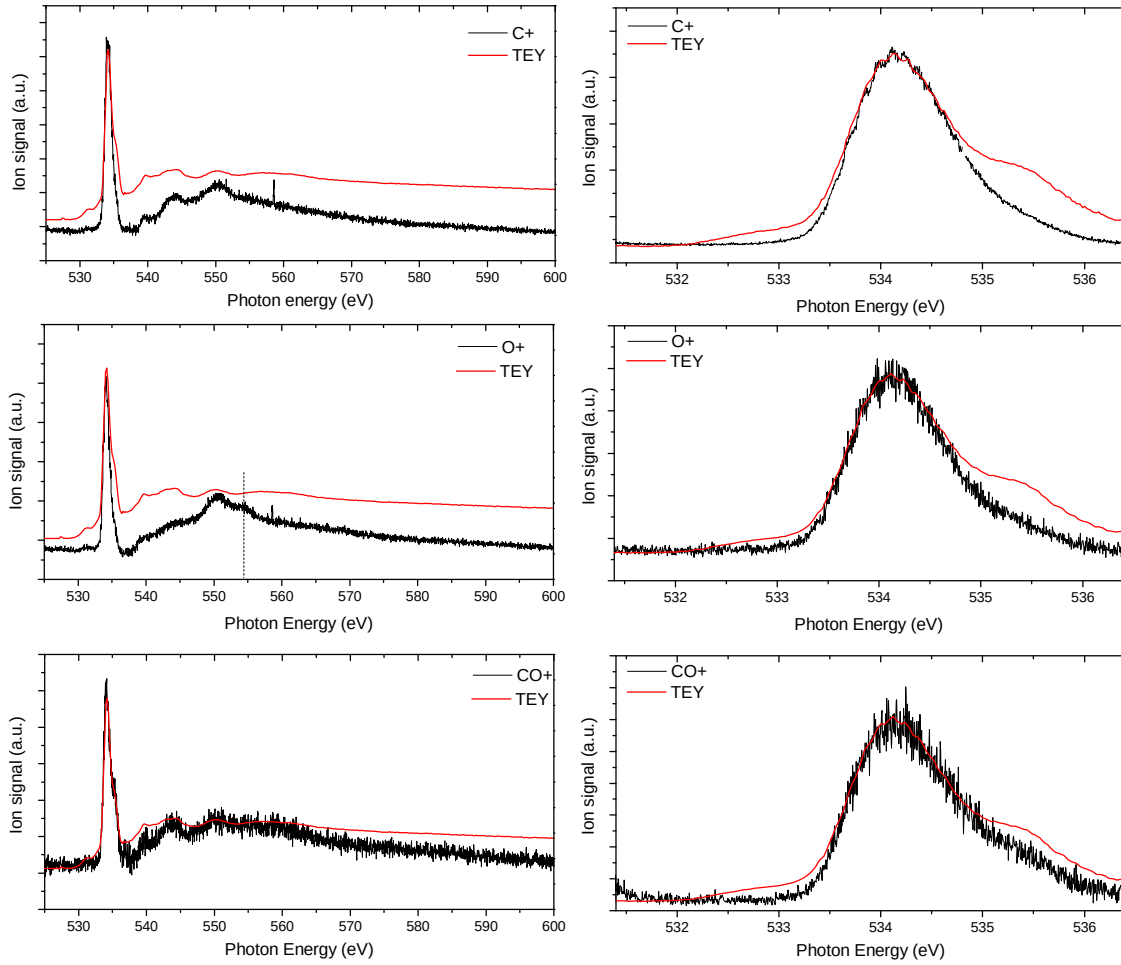
Figure VI.16: Photodesorption spectra of \text{C}^+ (top panels), \text{O}^+ (middle panels) and \text{CO}^+ (bottom panels), in full range (left panels) or near the \pi^* resonance (right panels). These spectra were taken on a CO ice that had already received a high photon dose.
