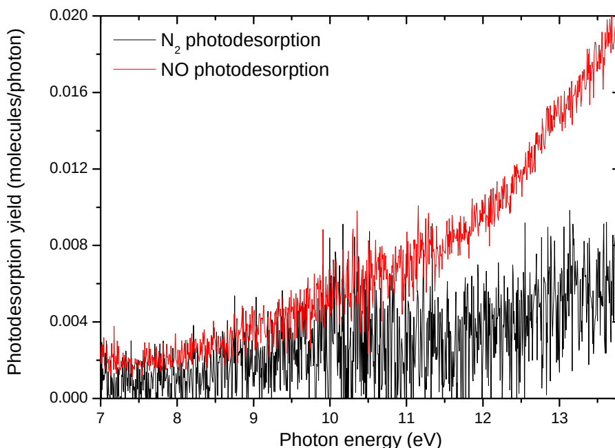
Figure IV.8: Photodesorption spectrum of \text{N}_2 from NO ice on the Au substrate (corresponding to the 4th scan of fig. IV.7). Also shown is the NO photodesorption yield of the corresponding scan.
