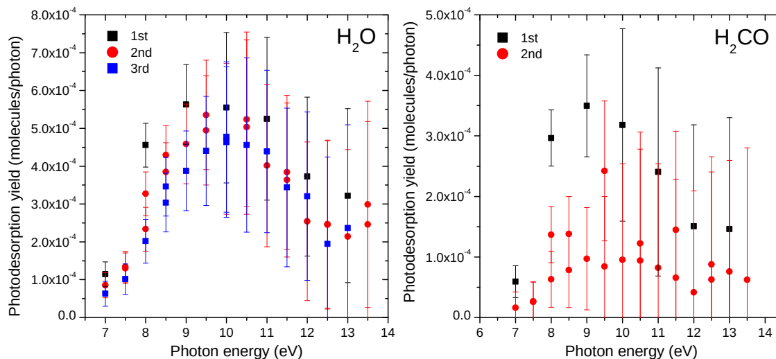
Figure IV.30: Photodesorption yields of \text{H}_2\text{O} (left panel) and \text{H}_2\text{CO} (right panel) from \text{HCOOH} ice (initially fresh ice). Black points were taken first, red points second and blue points third. See the text for more details.
