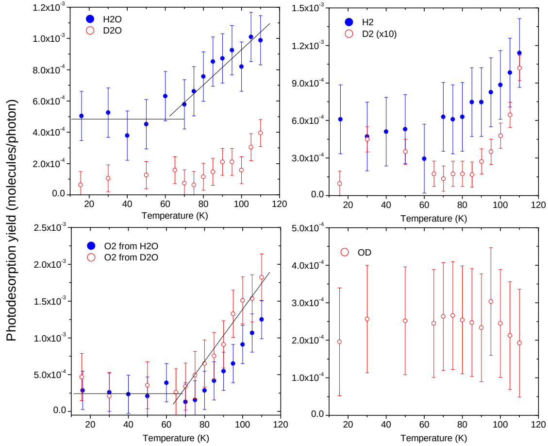
Figure IV.25: Photodesorption yields from 20 ML \text{H}_2\text{O} and \text{D}_2\text{O} compact amorphous ices, as a function of irradiation temperature, at a fixed photon energy of 10.2 eV.
