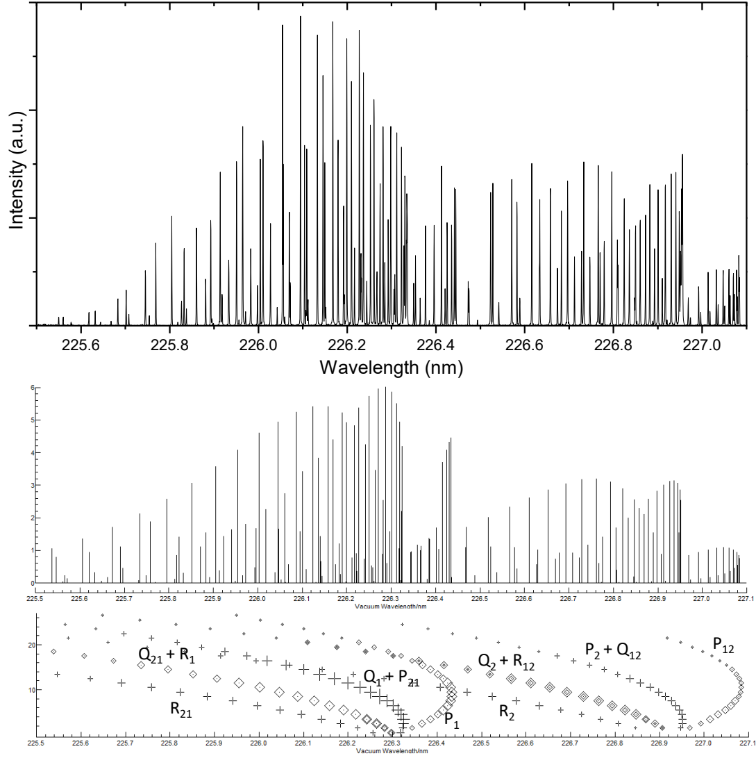
Figure IV.11: Gas-phase REMPI spectrum of the A^2\Sigma^+(v''=0) \leftarrow X^2\Pi(v'=0) transition of NO at 300 K. The top panel is the experimental spectrum. The middle panel is a spectrum simulated with PGOPHER (Ground state parameters: band origin 948\text{ cm}^{-1} , rotational constant B = 1.701\text{ cm}^{-1} , spin-orbit splitting A = 124.87\text{ cm}^{-1} ; excited state parameters: band origin 45074\text{ cm}^{-1} , rotational constant B = 1.9925\text{ cm}^{-1} ). The last panel is the attribution of the different branches. REMPI laser power: \sim 40\text{--}70\text{ }\mu\text{J/pulse} . Accumulation per wavelength step of 50 laser pulses at 10 Hz, 0.5 pm per step.
