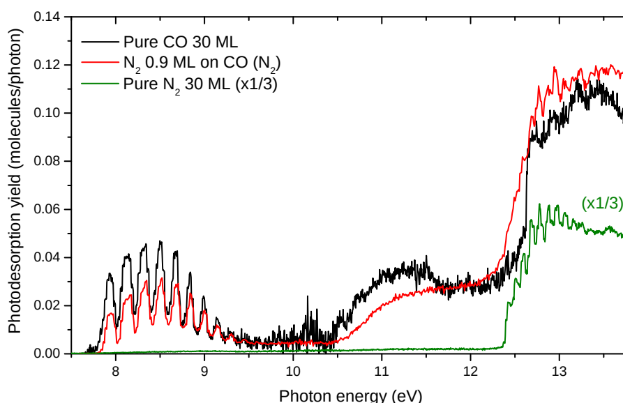
Figure IV.33: Photodesorption spectrum of \text{N}_2 from 0.9 ML of \text{N}_2 on CO ice. Also shown for comparisons are the photodesorption spectra of pure CO and pure \text{N}_2 .
