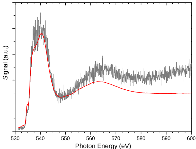
FIG. 5. Photodesorption spectrum of (\text{H}_2\text{O})_3\text{H}^+ at 90 K from c-ASW. Indicated in red is the TEY for comparison, normalized so as to best make the different features match.
