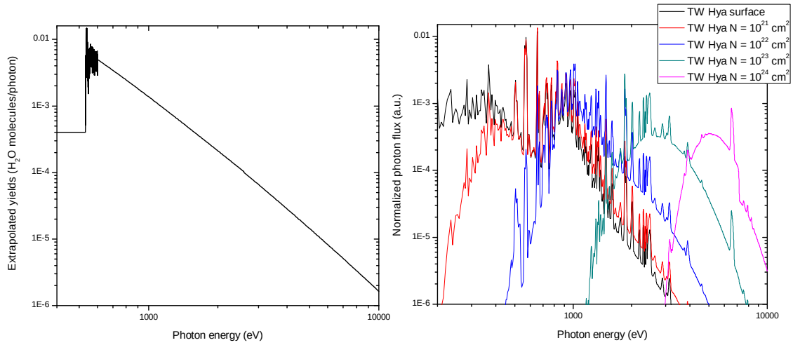
Figure VI.4: a. Photodesorption yield of \text{H}_2\text{O} from c-ASW at 15 K extrapolated up to 10 keV and down to 200 eV. b. X-ray emission spectrum of TW Hya adapted from [30] and spectra of the same spectrum after attenuation by different column densities N of dust and gas (see text). All spectra have been normalized for comparison.
