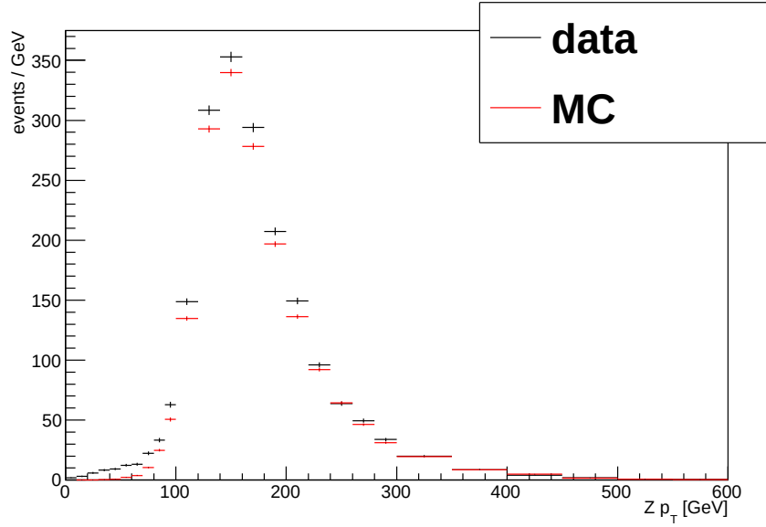
Figure 5.1: Data-MC comparison of Z boson's p_T distribution in the SHERPA Z \rightarrow ee channel.
