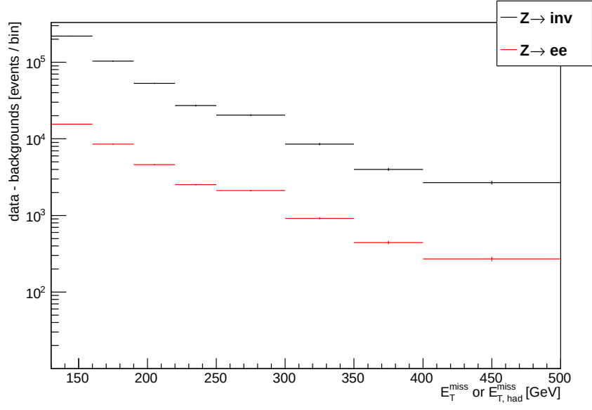
Figure 4.17: Distribution of the E_T^{\text{miss}} or E_{T,\text{had}}^{\text{miss}} measured in the data samples after the subtraction of the background estimations.
