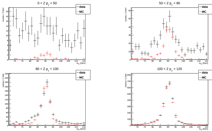
Figure 5.3: Invariant mass distributions in different bins of Z p_T .
