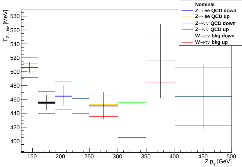
Figure 6.1: Variation in measurement of the invisible width as a function of Z boson's p_T due to systematic shifts in the background estimations.
