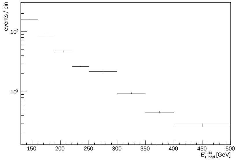
Figure 3.4: Hadronic recoil distribution in events passing the electron channel selection.
