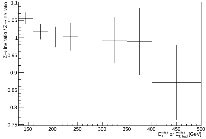
Figure 6.6: Ratio of the pileup stability as a function of E_T^{\text{miss}} or E_{T, \text{had}}^{\text{miss}} in the neutrino and electron channels.
