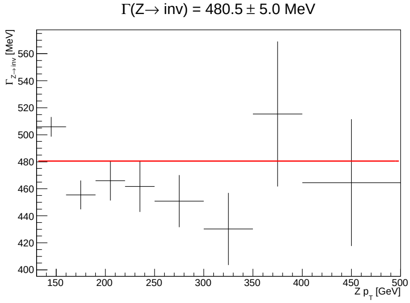
Figure 5.22: Measured invisible width as a function of Z boson p_T , with the calculated width of \Gamma(Z \rightarrow \text{inv}) = 480.5 \pm 5.0 \text{ MeV} .
