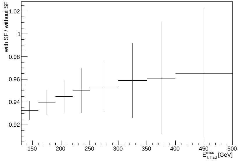
Figure 5.10: Ratio of E_{T,had}^{miss} distributions as a function of E_{T,had}^{miss} , with and without the electron efficiency scale factor applied.
