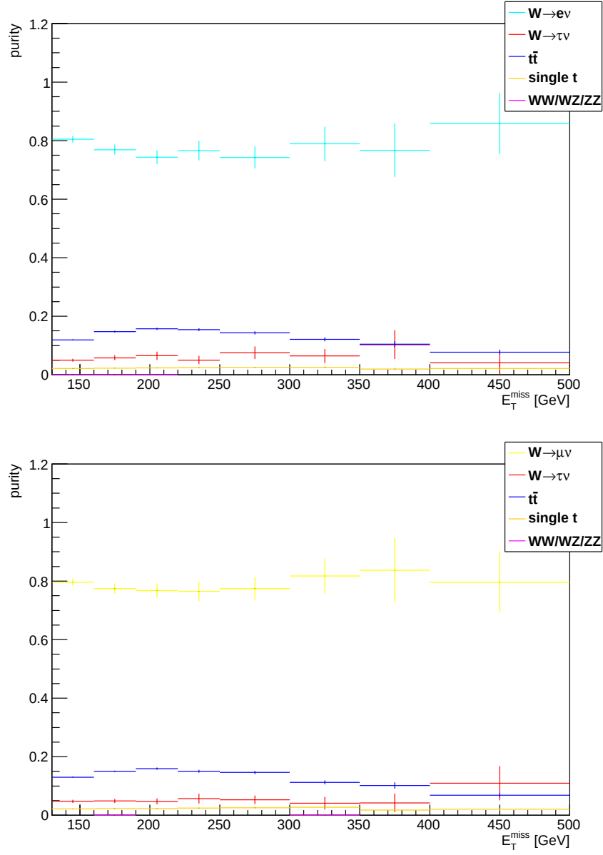
Figure 4.5: Purity of events from the MC simulations passing the W \rightarrow e\nu and W \rightarrow \mu\nu selection criteria.
