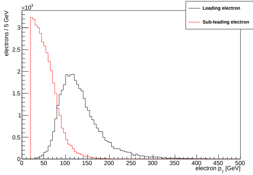
Figure 3.13: p_T distributions of the two electrons from the Z decay.
