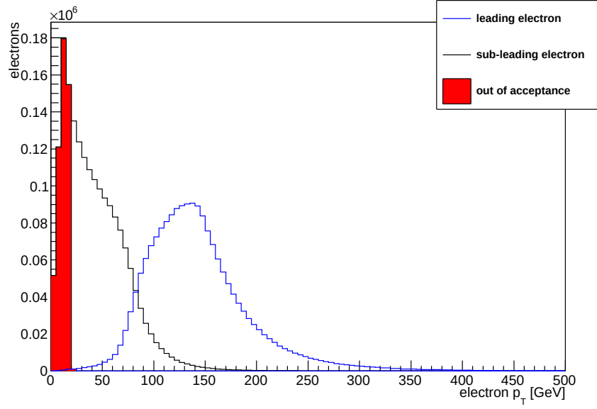
Figure 5.15: p_T distribution of electrons in \text{jet} + Z \rightarrow e^+e^- events.
