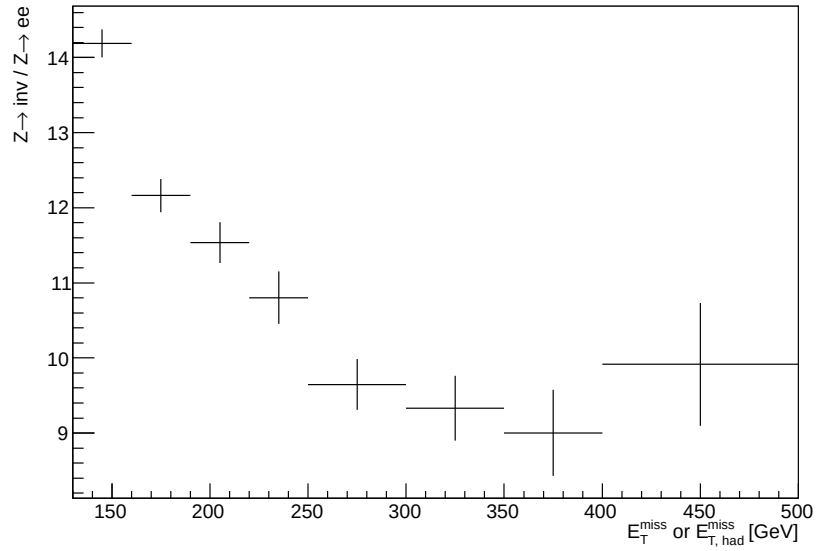
Figure 4.18: Ratio of the (background removed) E_T^{\text{miss}} / E_{T,\text{had}}^{\text{miss}} distributions measured in data.
