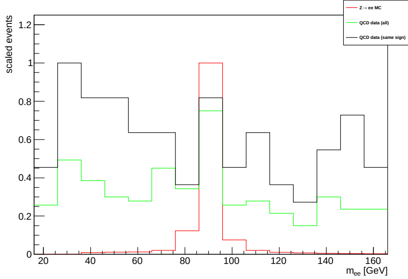
Figure 4.14: Invariant mass distributions in the jet + Z \rightarrow e^+e^- MC sample and the QCD control region data sample, with and without a same sign ‘electron’ requirement.
