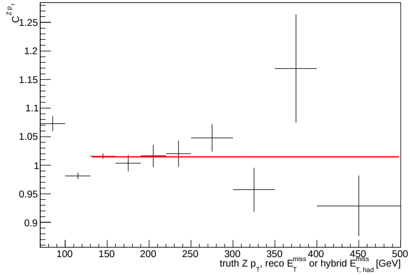
Figure 5.13: Correction for the Z momentum, jet reconstruction and background rejection cuts as a function of Z boson's p_T .
