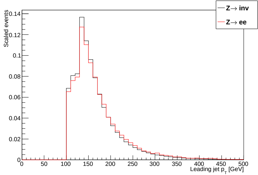
Figure 3.6: Leading jet p_T distribution in events passing the electron and invisible channel selections.
