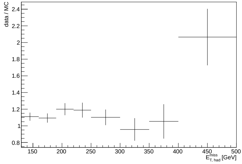
Figure 4.4: Ratio of the hadronic recoil distribution in data and MC events passing the t\bar{t} \rightarrow e\mu selection.
