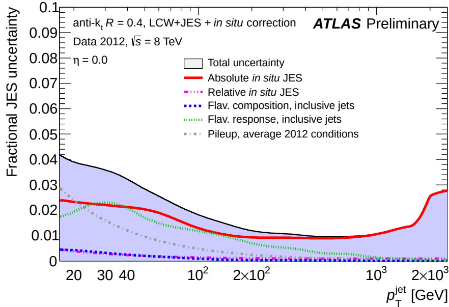
Figure 2.2: Fractional uncertainty on the Jet Energy Scale for central jets measured in 2012 data as a function of the jet p_T [19].
