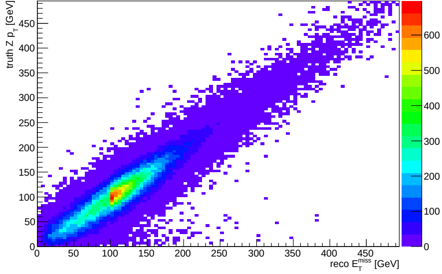
(a) E_T^{\text{miss}}
