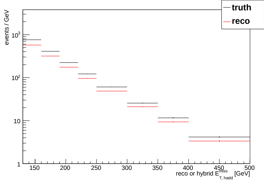
Figure 5.11: Hadronic recoil distributions using truth and reco electron selections.
