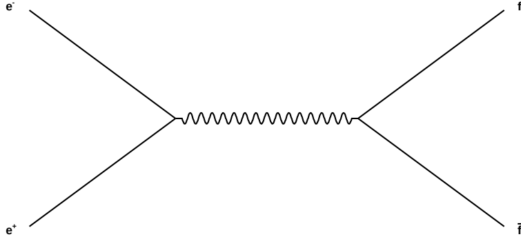
Figure 1.1: Feynman diagram of e^+e^- \rightarrow Z \rightarrow f\bar{f} interaction, measured at LEP.
