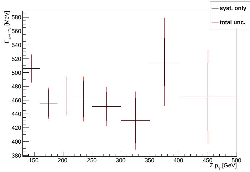
Figure 6.7: Measured invisible width of the Z boson as a function of its p_T .
