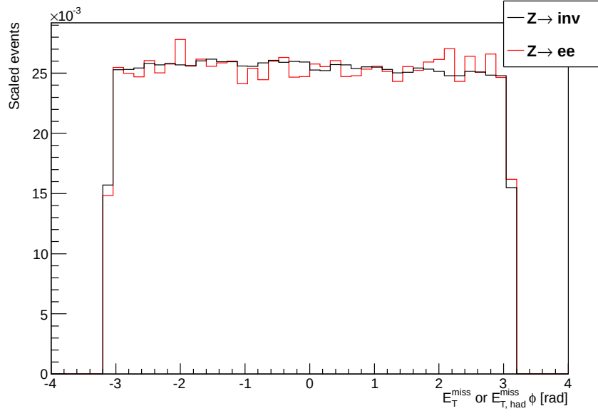
Figure 3.5: Hadronic recoil and missing transverse energy \phi distributions in events passing the electron and invisible channel selections.
