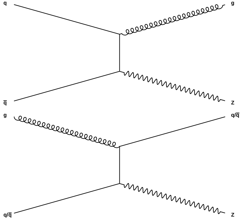
Figure 1.3: Feynman diagrams of Z + \text{jet} production at the LHC.
