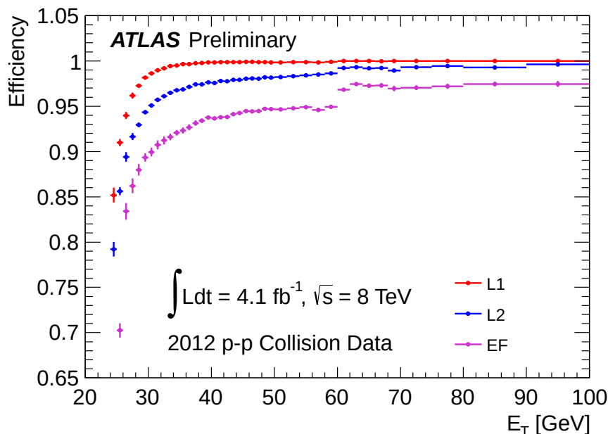
Figure 3.2: Measured electron trigger efficiency as a function of the electron's transverse energy [25]
