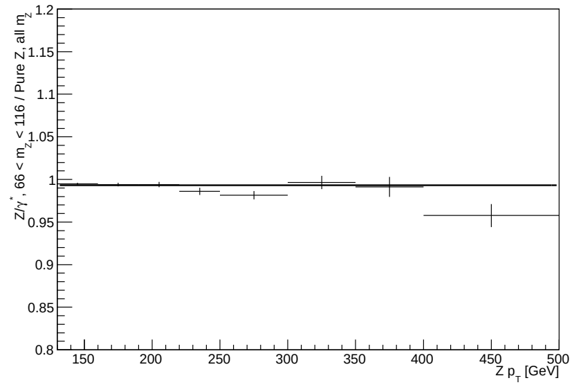
Figure 5.20: Correction factor, \delta_\gamma , as a function of the Z boson's p_T .
