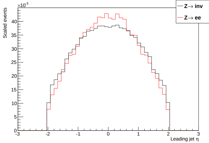
Figure 3.8: Leading jet \eta distribution in events passing the electron and invisible channel selections.
