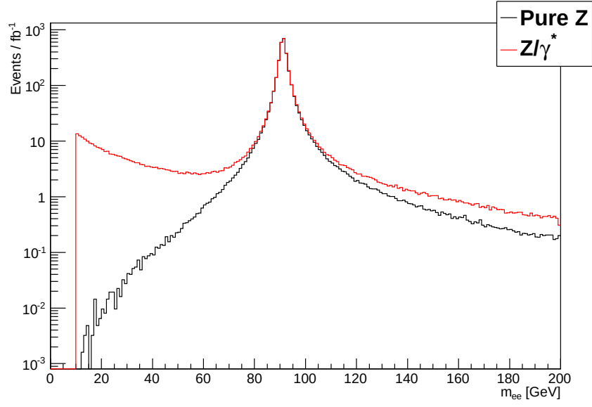
Figure 5.19: Invariant mass distribution in both channels, scaled to the same luminosity.
