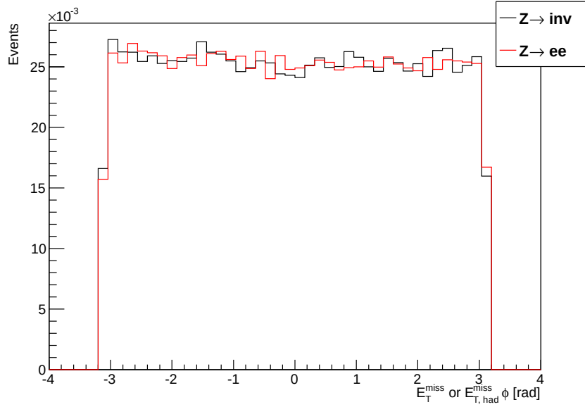
Figure 4.19: Hadronic recoil and missing transverse energy \phi distributions in events passing the electron and invisible channel selections after background subtraction.
