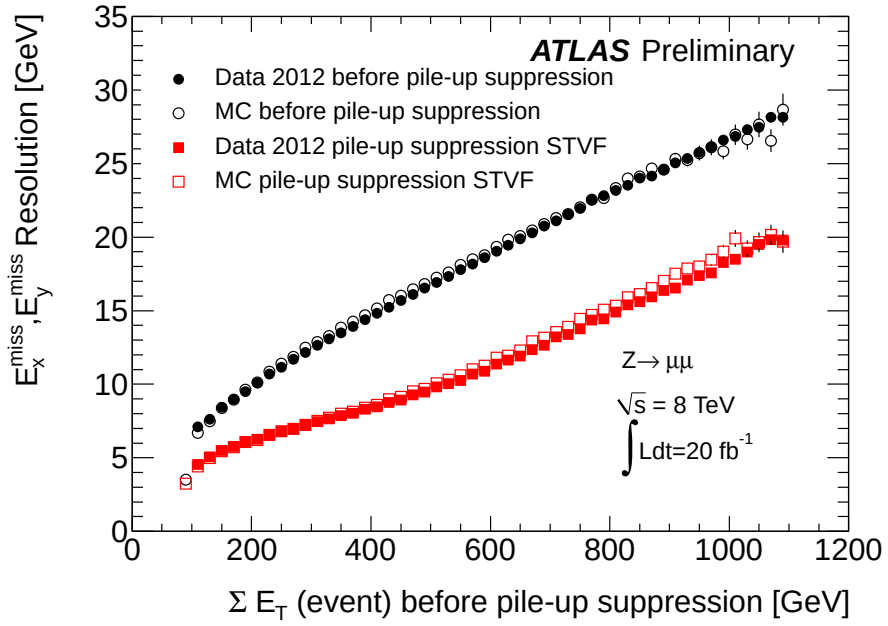
Figure 2.4: Measured and simulated E_T^{\text{miss}} resolution as a function of the scalar sum of the transverse energy, using Z \rightarrow \mu\mu events.
