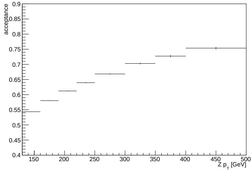
Figure 5.18: Acceptance correction as a function of Z boson's p_T .
