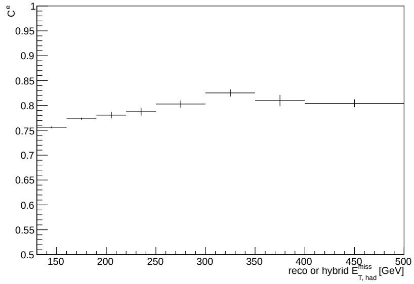
Figure 5.12: The electron selection correction as a function of E_{T, \text{had}}^{\text{miss}} .
