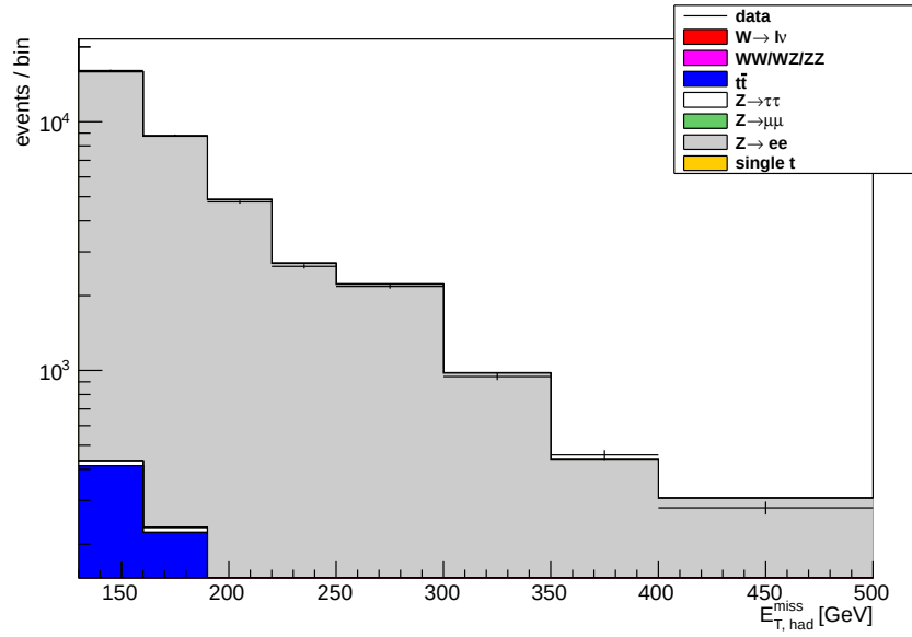
Figure 4.13: E_{T, \text{had}}^{\text{miss}} distribution in Monte Carlo estimated backgrounds to the electron channel.
