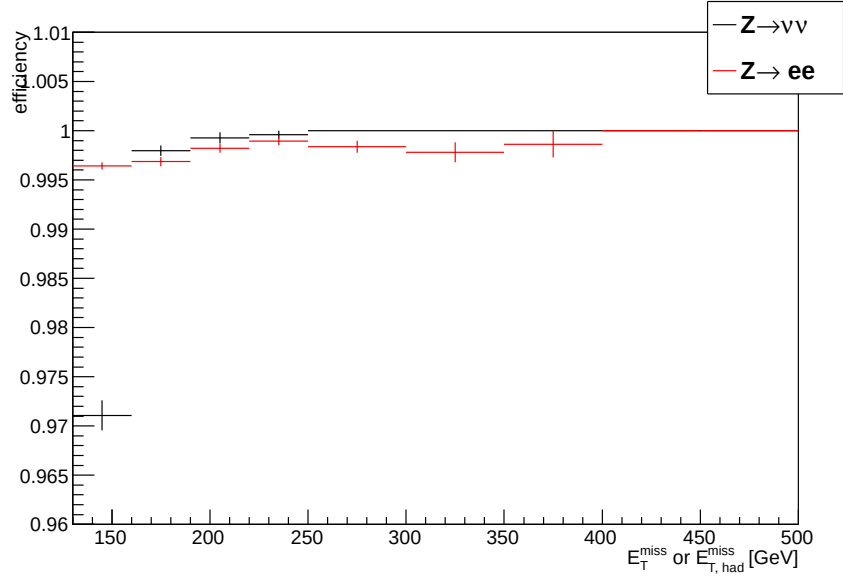
Figure 5.7: Estimated E_T^{\text{miss}} and electron trigger efficiencies as a function of E_T^{\text{miss}} or E_{T, \text{had}}^{\text{miss}} in events used in this analysis.
