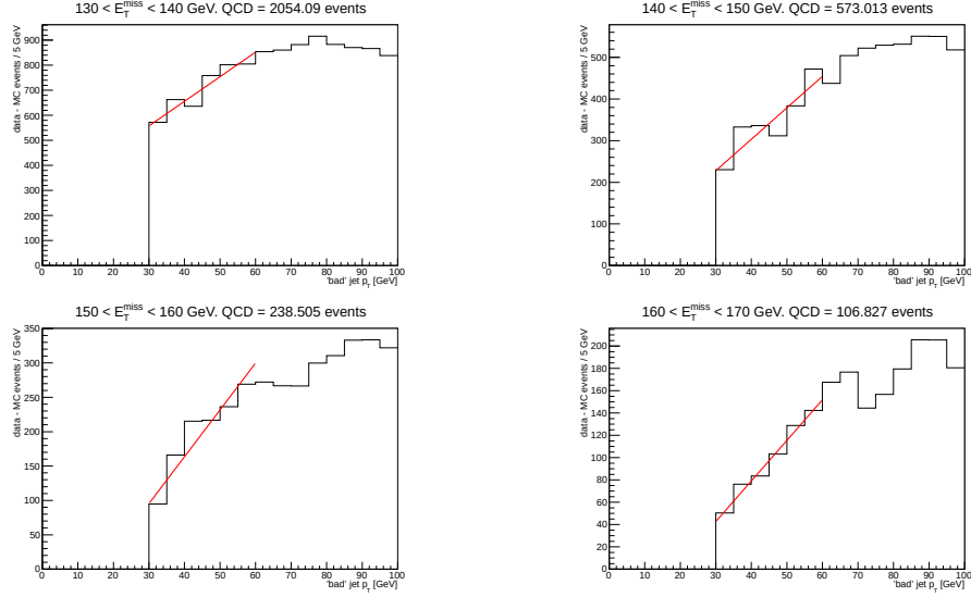
Figure 4.12: p_T distribution of the jet pointing towards the E_T^{\text{miss}} in the QCD control region with the MC background estimations removed, in the sections of the lowest E_T^{\text{miss}} bin.
