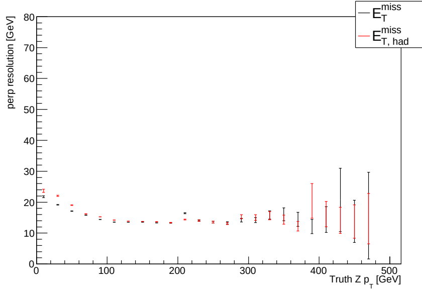
(b) perpendicular
