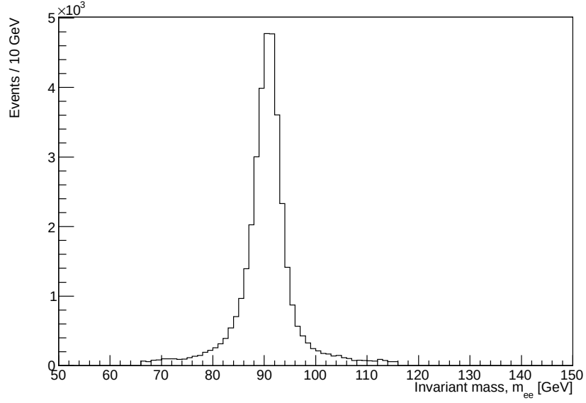
Figure 3.12: Invariant mass of the electrons from the Z decay in events passing the \text{jet} + Z \rightarrow e^+e^- selection.
