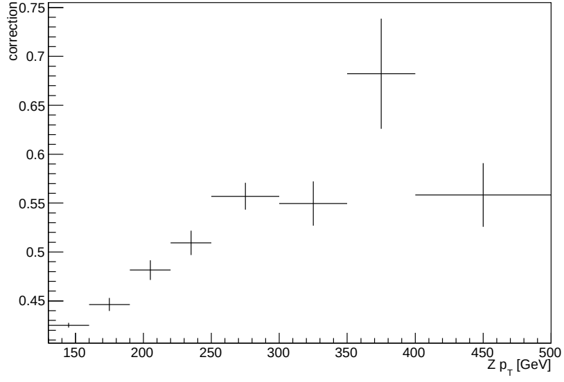
Figure 5.21: Product of different corrections as a function of Z boson's p_T .
