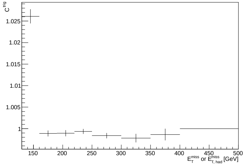
Figure 5.8: Trigger efficiency correction as a function of E_T^{\text{miss}} or E_{T, \text{had}}^{\text{miss}} .
