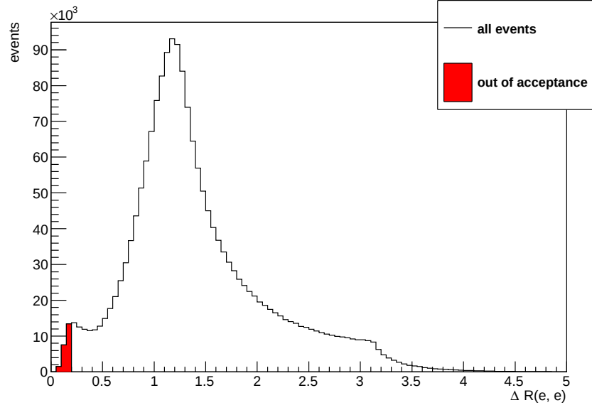
Figure 5.17: \Delta R(e, e) distribution in \text{jet} + Z \rightarrow e^+e^- events.
