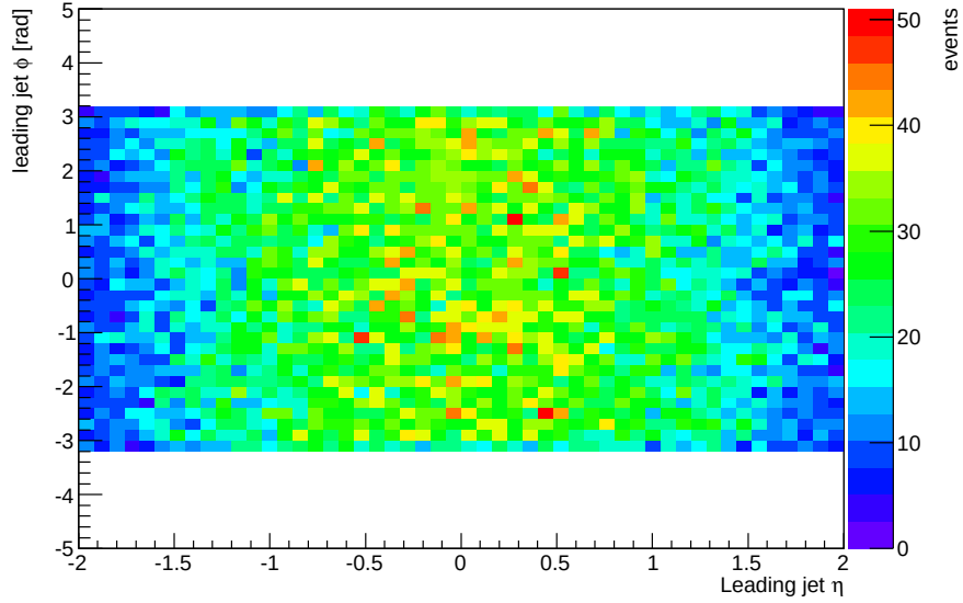
Figure 3.10: Leading jet \eta - \phi distribution in events passing the electron channel selection.
