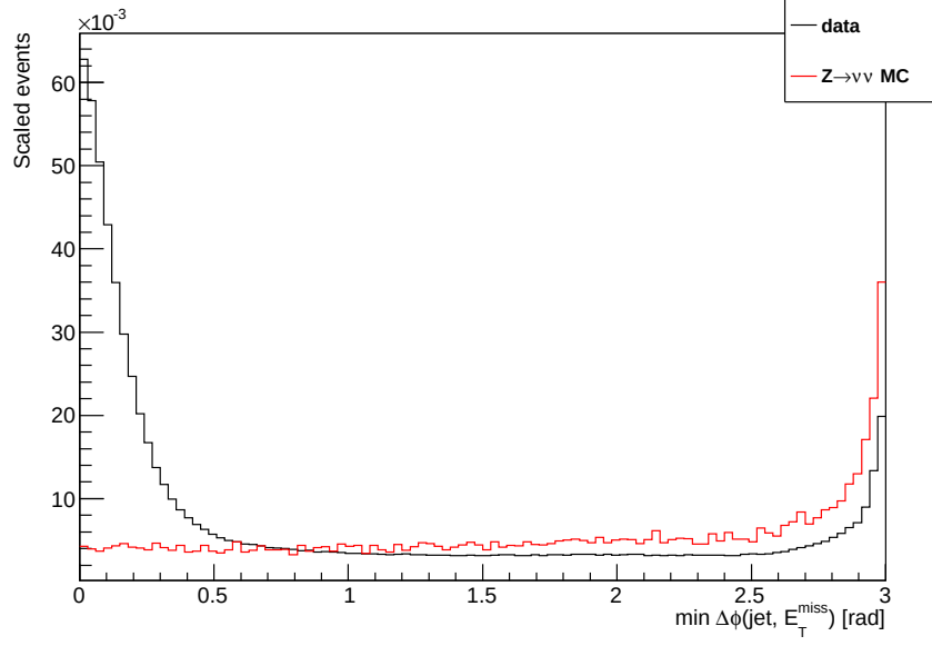
Figure 4.7: \Delta\phi(\text{jet}, E_T^{\text{miss}}) distribution for the jet closest to the E_T^{\text{miss}} in the data and Z \rightarrow \nu\nu MC samples with the \Delta\phi veto relaxed.
