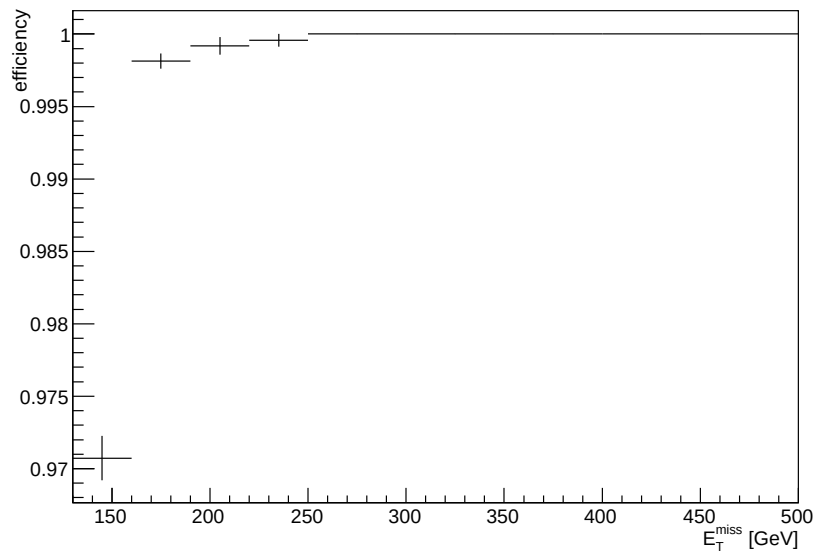
Figure 3.1: Estimated E_T^{\text{miss}} trigger efficiency as a function of E_T^{\text{miss}} found from Monte Carlo simulation.
