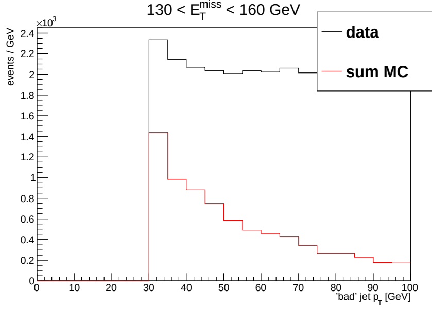
Figure 4.9: p_T distribution of the jet pointing towards the E_T^{\text{miss}} in the QCD control region in data and MC background estimations in the lowest E_T^{\text{miss}} bin.
