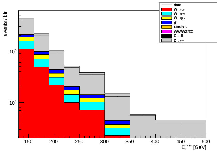
Figure 4.1: Monte Carlo estimated E_T^{\text{miss}} distributions in the invisible channel.
