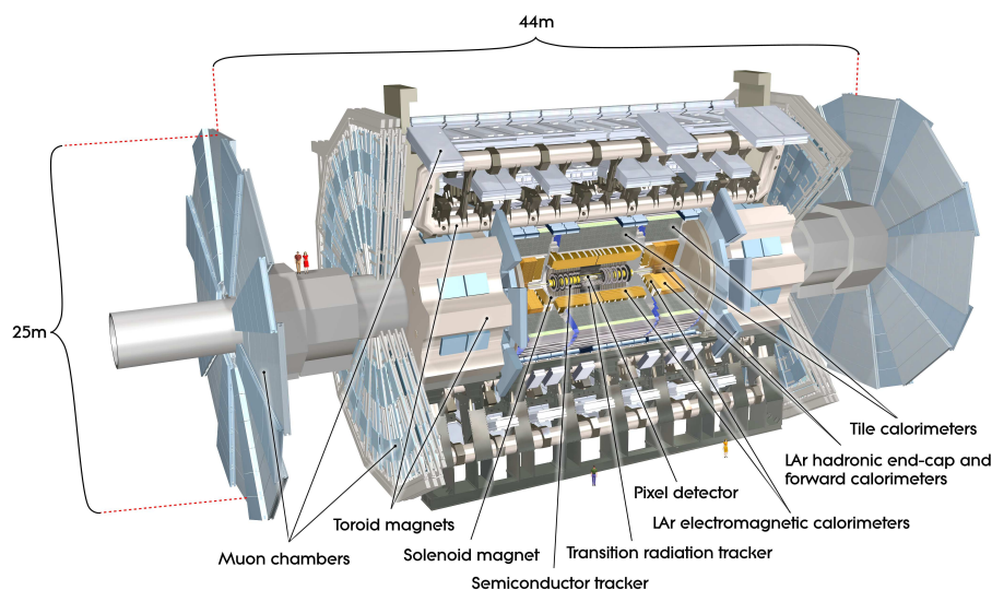
Figure 2.1: Diagram of the ATLAS detector [15].
