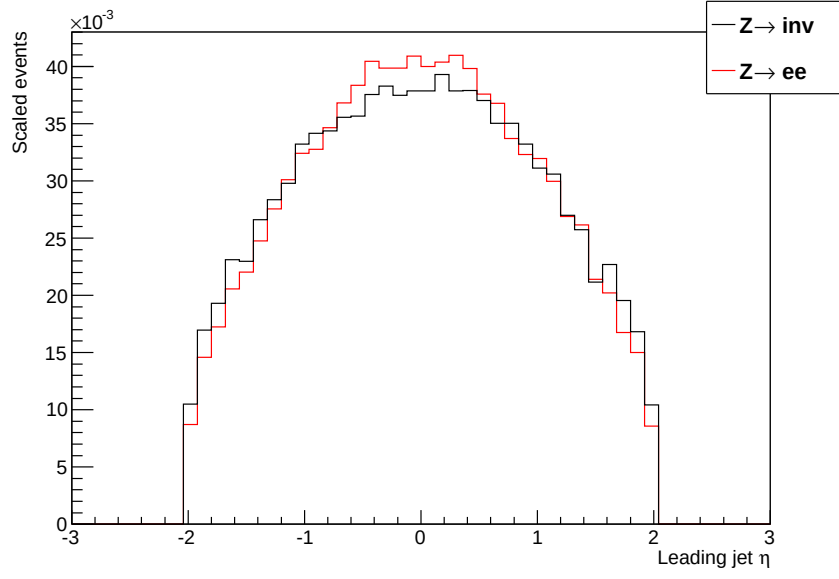
Figure 4.22: Leading jet \eta distribution in events passing the electron and invisible channel selections after background subtraction.
