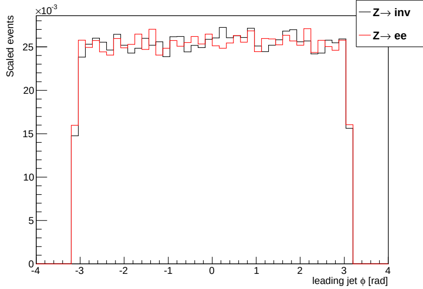
Figure 4.23: Leading jet \phi distribution in events passing the electron and invisible channel selections after background subtraction.
