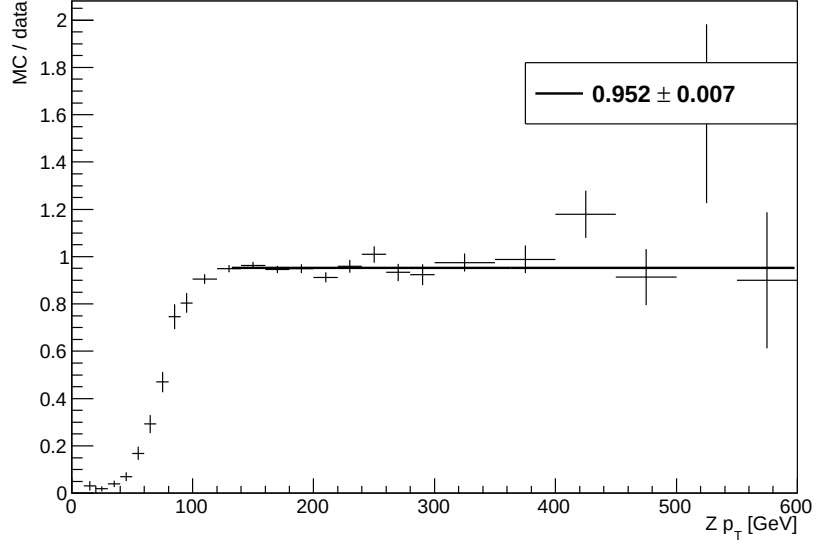
Figure 5.2: Ratio of data and SHERPA MC Z boson's p_T distributions.
