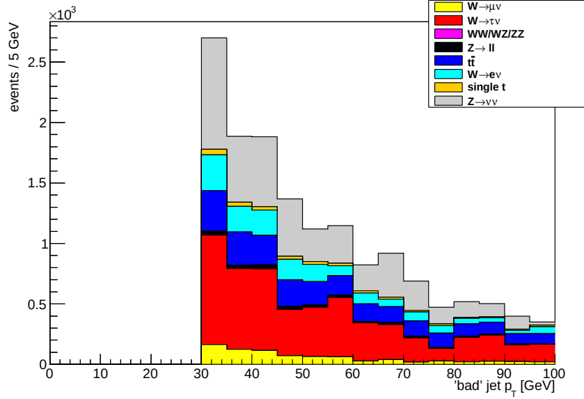
Figure 4.8: p_T distribution of the jet pointing towards the E_T^{\text{miss}} in the MC background estimations in the lowest E_T^{\text{miss}} bin.
