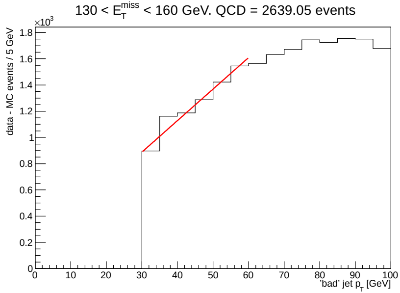
Figure 4.10: p_T distribution of the jet pointing towards the E_T^{\text{miss}} in the QCD control region with the MC background estimations removed, in the lowest E_T^{\text{miss}} bin.
