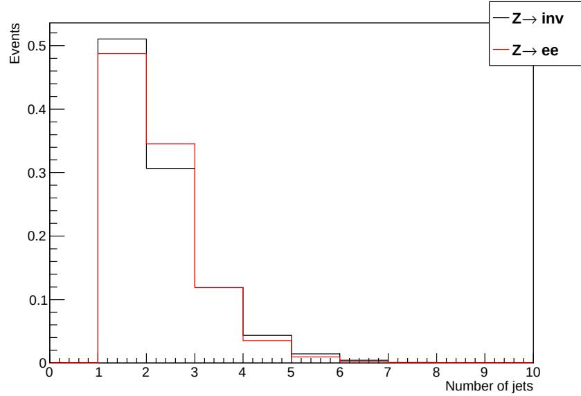
Figure 4.21: The number of jets in events passing the jet + Z \rightarrow inv and jet + Z \rightarrow e^+e^- selections after background subtraction.
