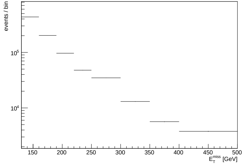
Figure 3.3: Missing transverse energy distribution in events passing the invisible channel selection.
