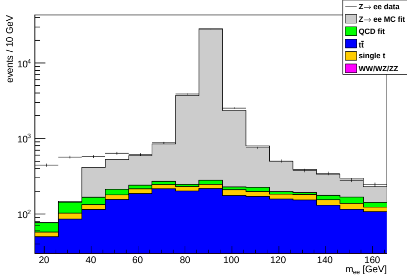
Figure 4.15: Result of fitting QCD and jet + Z \rightarrow e^+e^- m_{ee} templates to the m_{ee} distribution of events passing the jet + Z \rightarrow e^+e^- channel selection, where the scale of the Z \rightarrow ee MC and QCD template distributions has been set by the fitting procedure.
