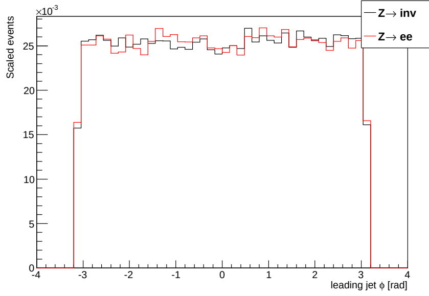
Figure 3.9: Leading jet \phi distribution in events passing the electron and invisible channel selections.
