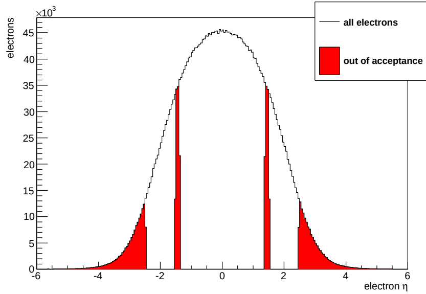
Figure 5.16: \eta distribution of electrons in \text{jet} + Z \rightarrow e^+e^- events.
