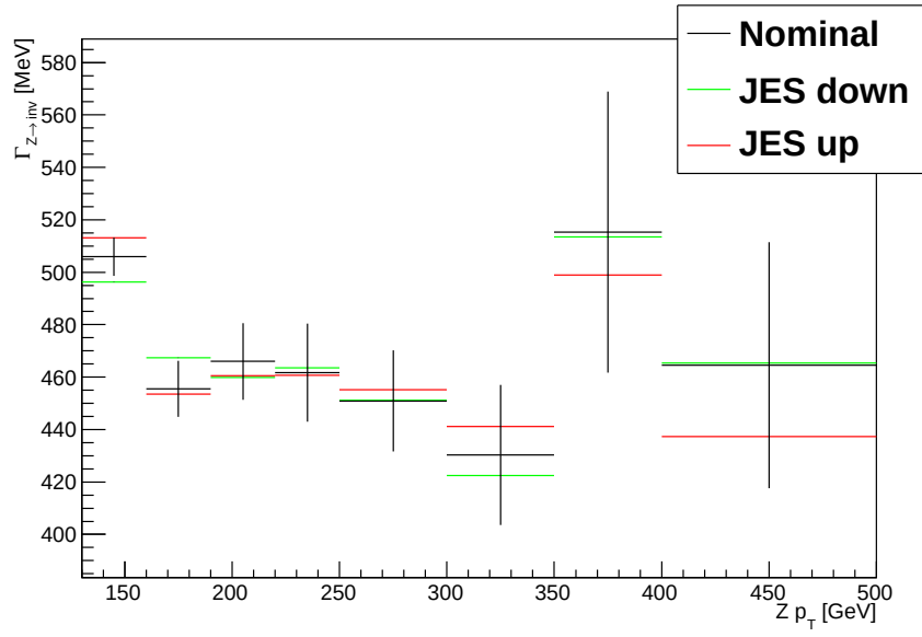
Figure 6.3: Variations in the measured invisible width as a function of Z boson's p_T due to systematic shifts in the Jet Energy Scale.
