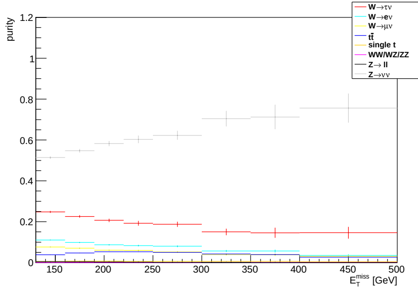
Figure 4.2: Proportion of Monte Carlo estimated backgrounds from different sources as a function of E_T^{\text{miss}} in the invisible channel.
