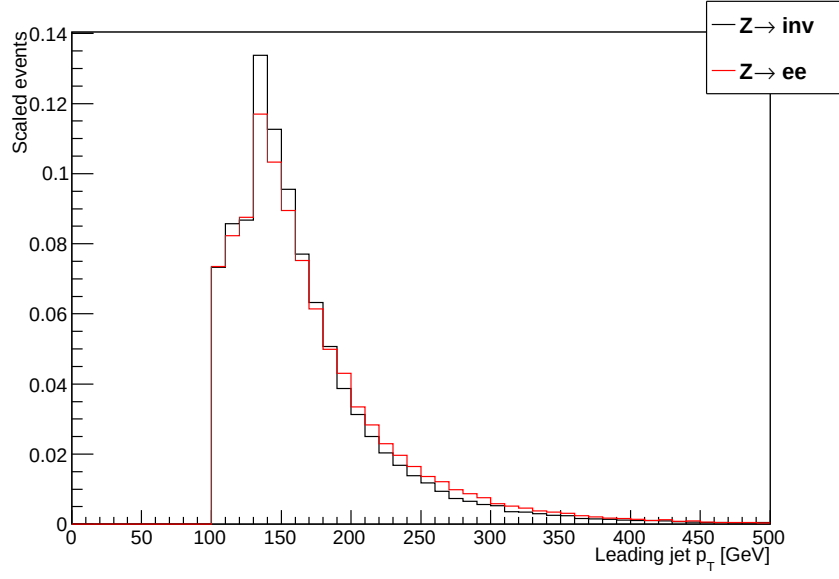
Figure 4.20: Leading jet p_T distribution in events passing the electron and invisible channel selections after background subtraction.
