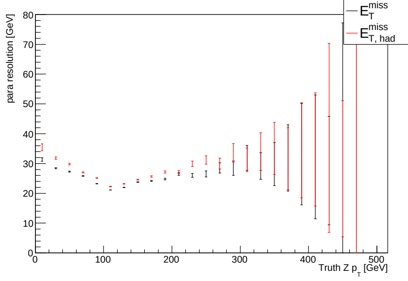
(a) parallel
