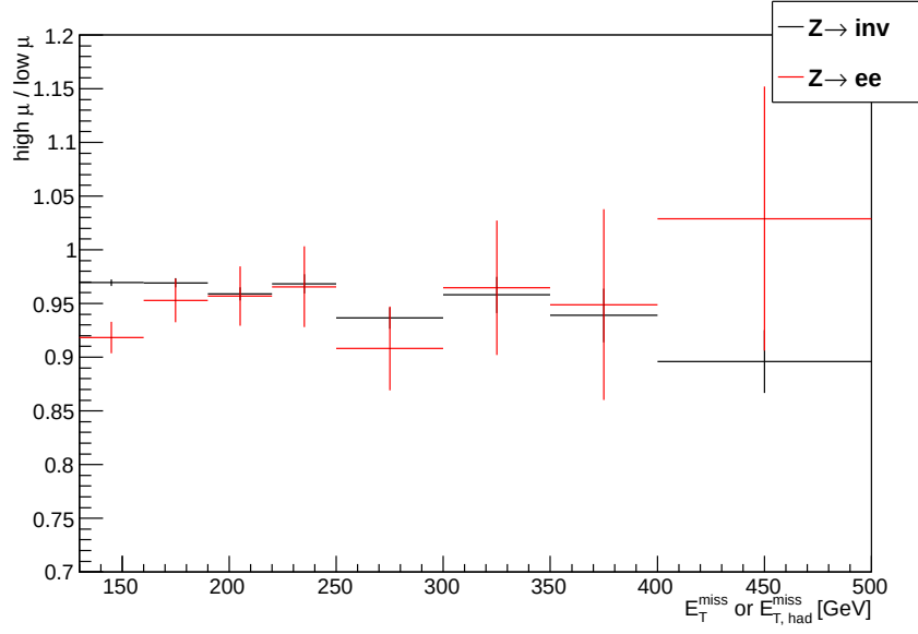
Figure 6.5: Ratios of measured E_T^{\text{miss}} or E_{T, \text{had}}^{\text{miss}} distributions in low- and high-pileup conditions.
