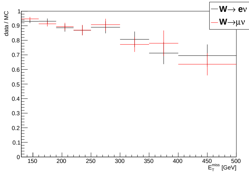
Figure 4.6: The ratios of data and MC E_T^{\text{miss}} distributions in events passing the W \rightarrow e\nu or W \rightarrow \mu\nu selection criteria.
