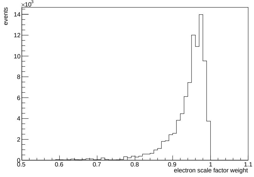
Figure 5.9: Electron reconstruction efficiency scale factor distribution.
