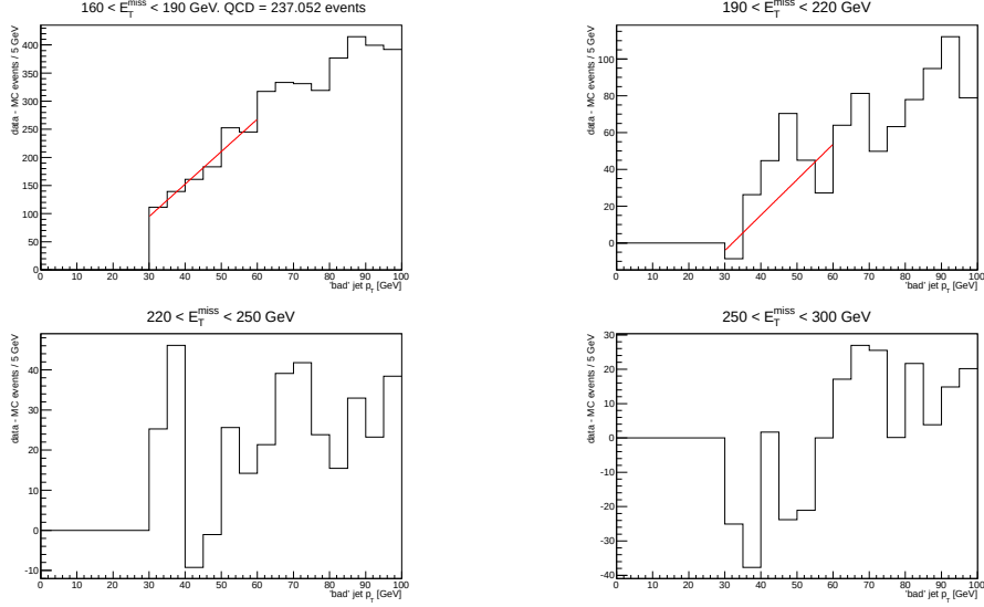
Figure 4.11: p_T distribution of the jet pointing towards the E_T^{\text{miss}} in the QCD control region with the MC background estimations removed, in higher E_T^{\text{miss}} bin.
