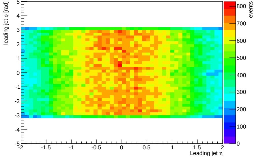
Figure 3.11: Leading jet \eta - \phi distribution in events passing the invisible channel selection.
