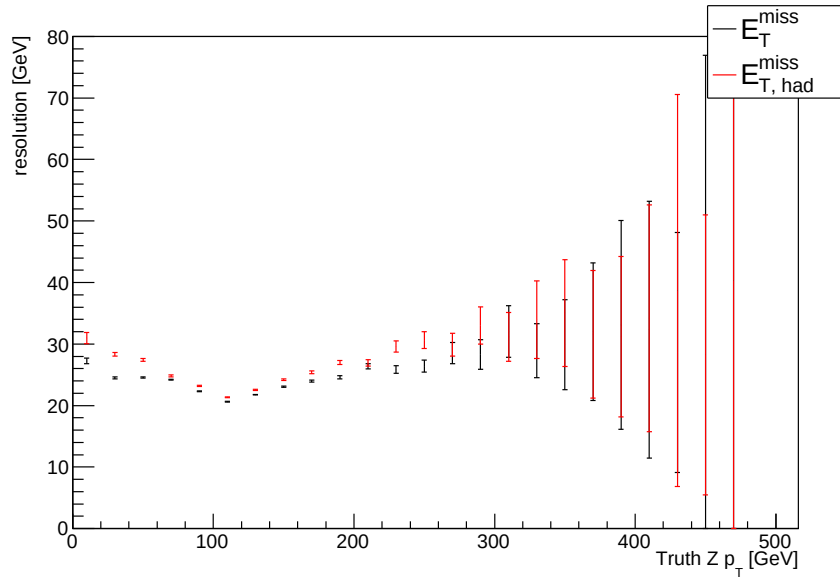
Figure 5.5: E_T^{\text{miss}} and E_{T, \text{had}}^{\text{miss}} resolutions as a function of truth Z boson's p_T .
