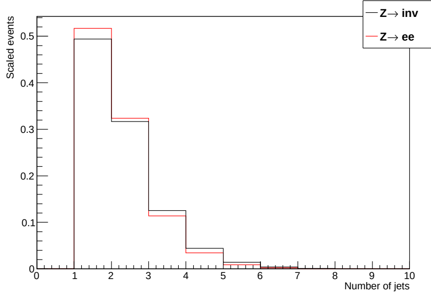
Figure 3.7: The number of jets in events passing the \text{jet}+Z \rightarrow \text{inv} and \text{jet}+Z \rightarrow e^+e^- selections.
