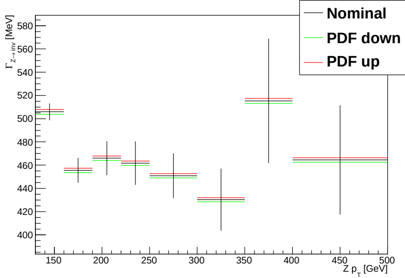
Figure 6.2: Variation in measurement of the invisible width as a function of Z boson's p_T due to systematic shifts in the PDF.
