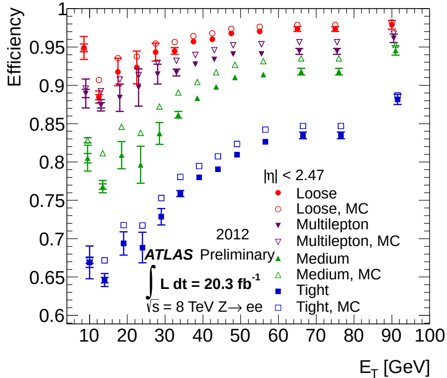
Figure 2.3: Measured and simulated efficiencies for electron identification as a function of the electron’s transverse energy [21].
