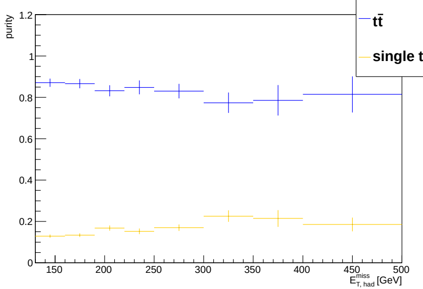
Figure 4.3: Proportion of the MC estimated events passing the t\bar{t} \rightarrow e\mu selection coming from t\bar{t} or single top samples as a function of E_{T, \text{had}}^{\text{miss}} .
