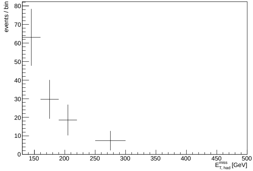
Figure 4.16: E_{T, \text{had}}^{\text{miss}} distribution of estimated QCD background to the jet + Z \rightarrow e^+e^- channel.
