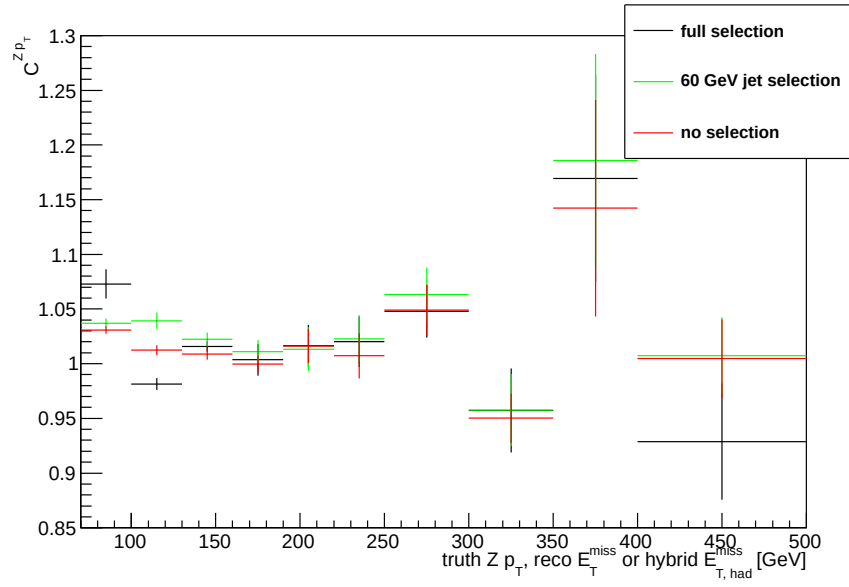
Figure 5.14: Comparison of Z boson's p_T correction as a function of truth Z boson's p_T with different selection criteria.
