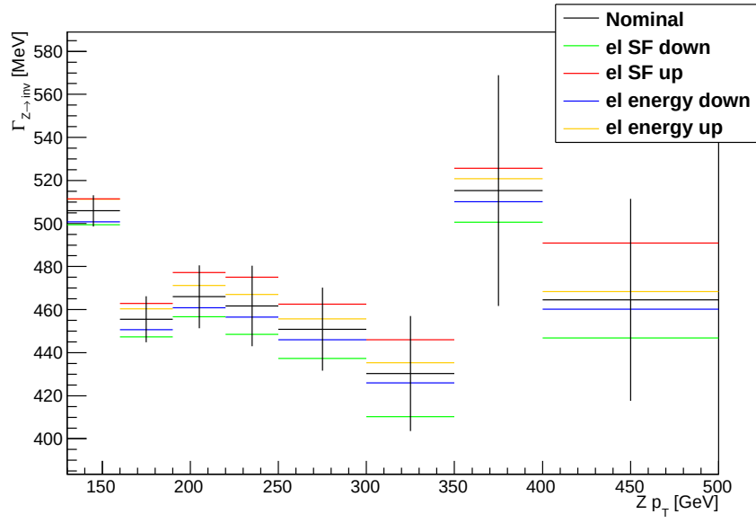
Figure 6.4: Variations in the measured invisible width as a function of Z boson's p_T due to systematic shifts of the electron energy or identification scale factors.
