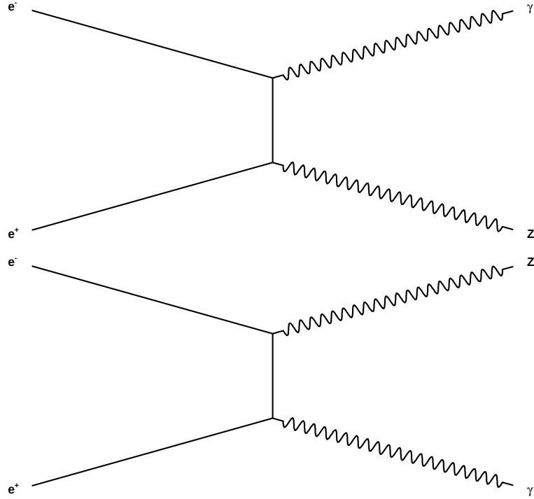
Figure 1.2: Feynman diagrams of e^+e^- \rightarrow Z\gamma interaction, used for the direct measurement at LEP.
