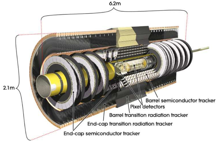
Figure 2.3: Cut-away sketch of the Inner Detector. The outermost part shows the Transition Radiation Tracker, the gray wheels and the barrel part with same diameter are the disks and the barrel of the Semiconductor Tracker. The Pixel Detector sits as the innermost part in the center and is detailed in Figure 2.4 [102].
