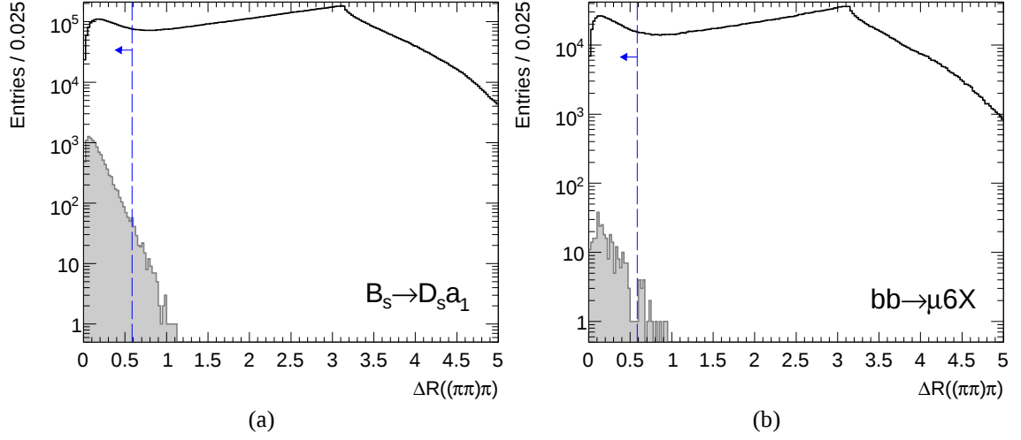
Figure 6.11: Opening angle in \Delta R((\pi\pi)\pi) between the directions of selected \rho candidates and a third track obtained from the B_s^0 \rightarrow D_s^- a_1^+ (a) and bb \rightarrow \mu 6X (b) data samples. The open histograms show the opening angle for all track triplets, whereas the gray filled areas correspond to triplets with truth matched tracks.
