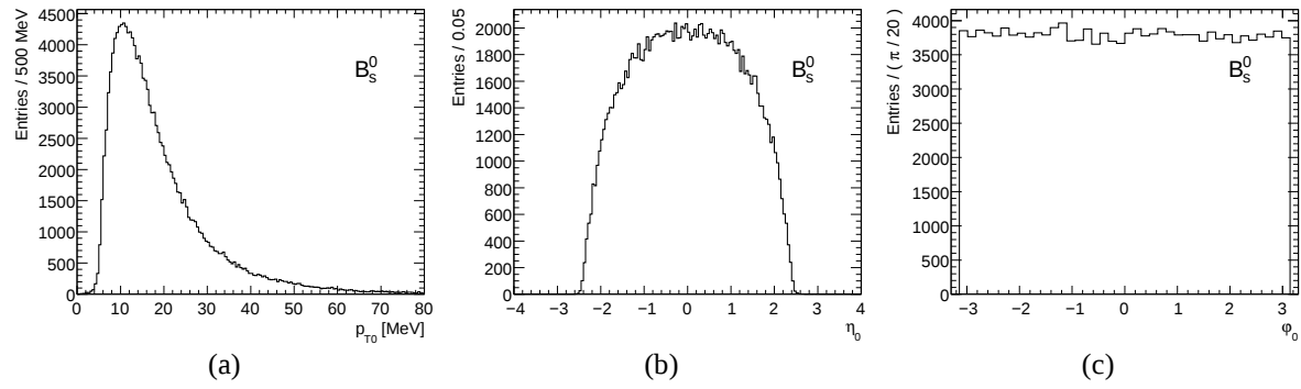
Figure B.4: For the B_s^0 meson, the transverse momentum ( p_{T0} ) (a), the \eta_0 (b) and the \phi_0 (c) distributions obtained from the MC truth information are shown.
