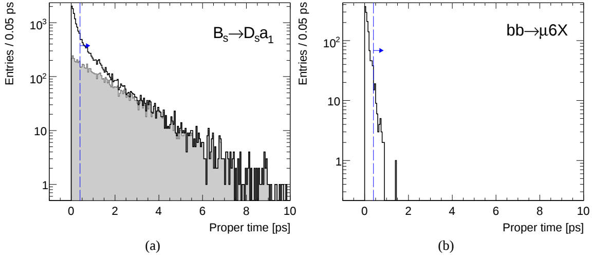
Figure 6.14: Proper time distribution of the \bar{B}_s^0 meson for track sextuplets passing the \chi^2 cut (6.24) of the vertex fit obtained from the B_s^0 \rightarrow D_s^- a_1^+ (a) and bb \rightarrow \mu 6X (b) data samples. The open histogram shows all combinations, whereas the gray filled area represents truth matched track sextuplets.
