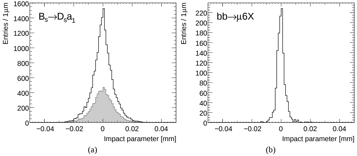
Figure 6.21: Impact parameter of the B_s^0 meson for track sextuplets passing the \chi^2 cut (6.24) obtained from the B_s^0 \rightarrow D_s^- a_1^+ (a) and bb \rightarrow \mu 6X (b) data samples. The shaded histogram is obtained from truth matched candidates. The difference in (a) between the open and shaded histogram shows the contribution by the combinatorial background in the signal sample.
