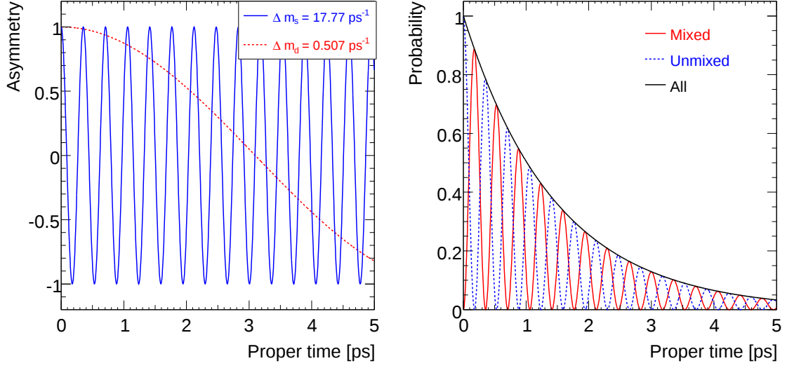
Figure 1.7a: Asymmetry of neutral B_q^0 mesons versus the proper lifetime. The B_s^0 - \bar{B}_s^0 oscillation frequency \Delta m_s is a factor of about 35 larger than the B_d^0 - \bar{B}_d^0 oscillation frequency \Delta m_d .
