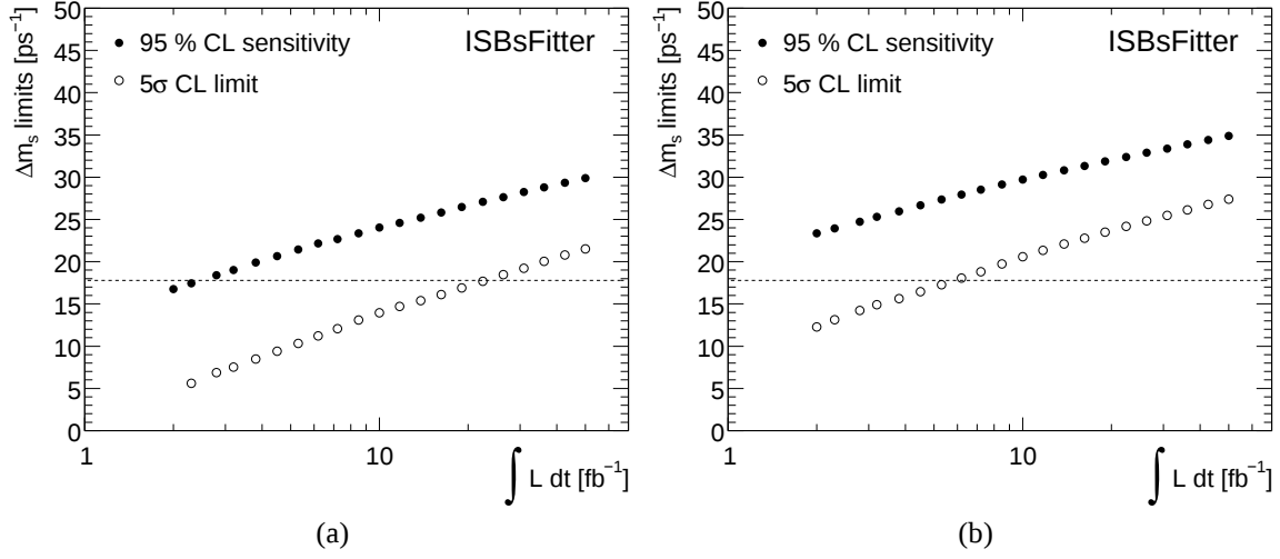
Figure 7.9: Dependence of the 95 % CL sensitivity and the 5 \sigma CL limit on the integrated luminosity for the B_s^0 \rightarrow D_s^- a_1^+ decay channel (a) and for a combination of the B_s^0 \rightarrow D_s^- a_1^+ and B_s^0 \rightarrow D_s^- \pi^+ decay channels (b). The horizontal line at \Delta m_s^{\text{meas}} = 17.77 ps -1 corresponds to the value measured by CDF [66]. The statistical errors are smaller than the dot size.
