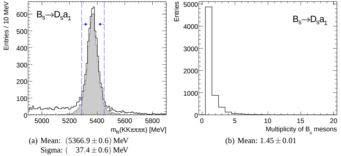
Figure 6.17: Reconstructed invariant mass distribution (a) of track sextuplets passing the p_T cut (6.27) and number of B_s^0 candidates per event. The values are obtained from a fit of a Gaussian function to truth matched candidates within a 2\sigma range around the mean value.
