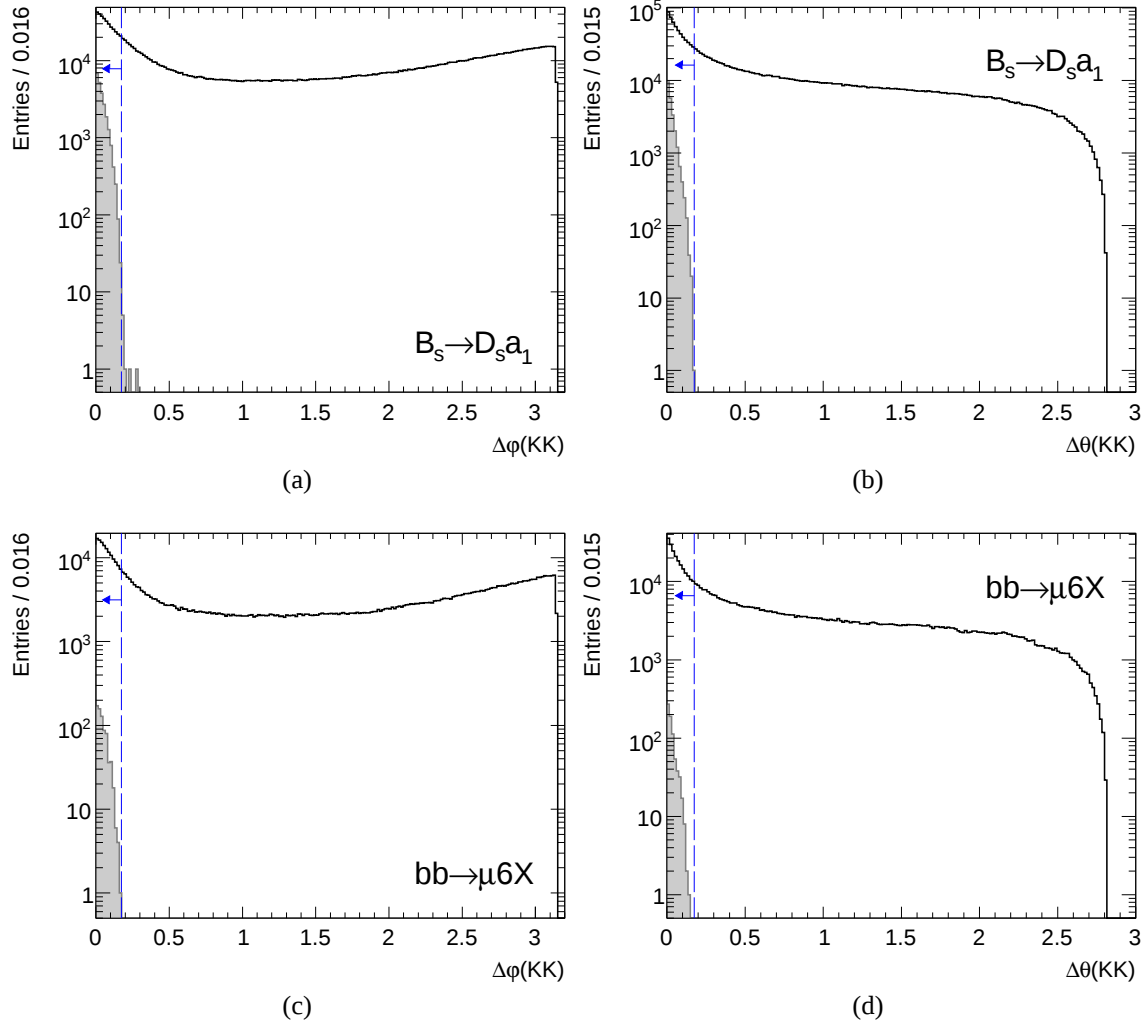
Figure 6.4: Distribution of the opening angles \Delta\phi (a,c) and \Delta\theta (b,d) for all reconstructed track pairs with oppositely charged tracks for the signal sample (a,b) and the bb \rightarrow \mu 6X data sample (c,d). The open black histograms show all combinations within the sample, whereas the gray filled histograms correspond to reconstructed tracks matching the MC truth particles from the \phi meson decay.
