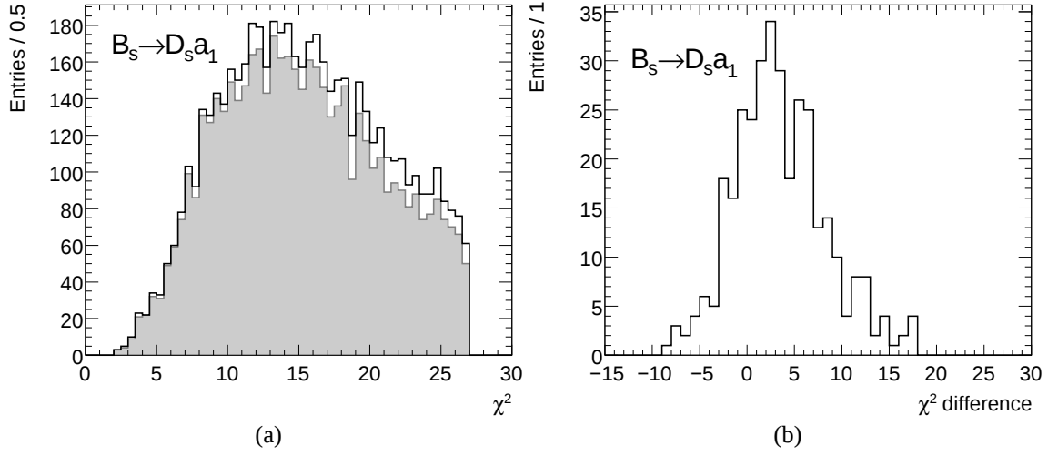
Figure 6.18: The left hand side plot (a) shows the \chi^2 distribution for all \bar{B}_s^0 candidates (black) and truth matched candidates (gray filled area). For events with more than one \bar{B}_s^0 candidate (including a truth matched candidate), the difference (6.30) of the \chi^2 to the truth matched candidate (b) is shown.
