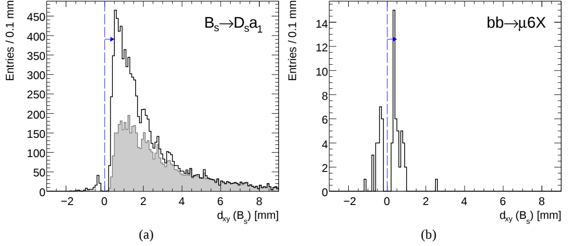
Figure 6.15: Transverse decay length d_{xy} distribution of the \bar{B}_s^0 meson for track sextuplets passing the proper time cut (6.25) obtained from the B_s^0 \rightarrow D_s^- a_1^+ (a) and bb \rightarrow \mu 6X (b) data samples. Entries around d_{xy}(B_s^0) = 0 are already rejected by the proper time cut.
