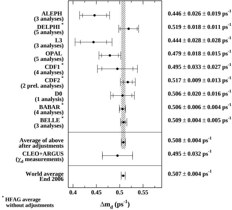
Figure 1.5: The current status of B^0\text{-}\bar{B}^0 oscillation frequency measurements \Delta m_d as provided by the Heavy Flavor Averaging Group (HFAG) [48].
