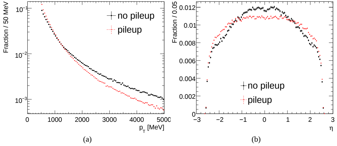
Figure 7.17: Normalized reconstructed transverse momentum spectrum (a) and \eta distribution (b) of all reconstructed tracks overlayed for the sample including effects of pileup (red, dashed line) and without (black, solid line).
