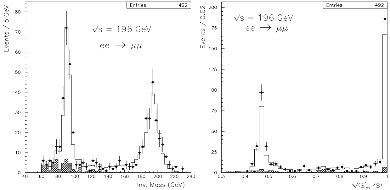
Figure 5.1: Distributions of data (dots), signal MC (open histogram) and background (hatched histogram) in the variables invariant mass M_{inv} and \sqrt{s'_m/s} for E_{CM} = 196 GeV.
