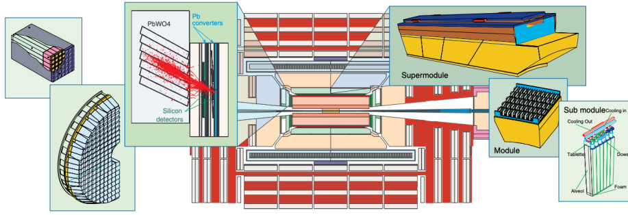
Figure 3.11 A schematic view of the ECAL of CMS [82] .
