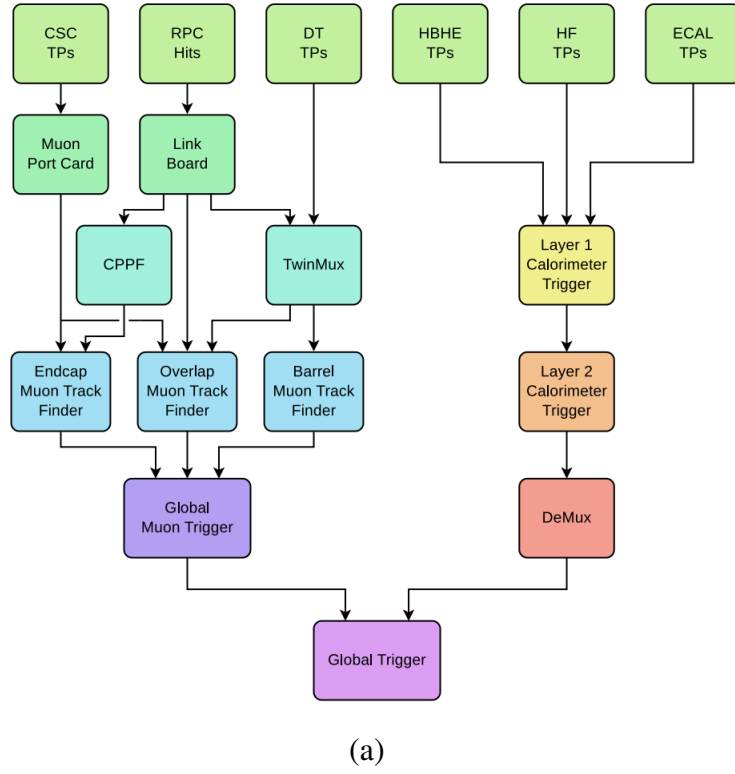
Figure 3.18 Schematic of the upgraded CMS Level-1 trigger system during Run 2 [90] .
