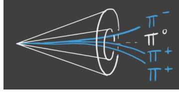
Figure 4.11 Schematic diagram of hadronic tau lepton decays.
