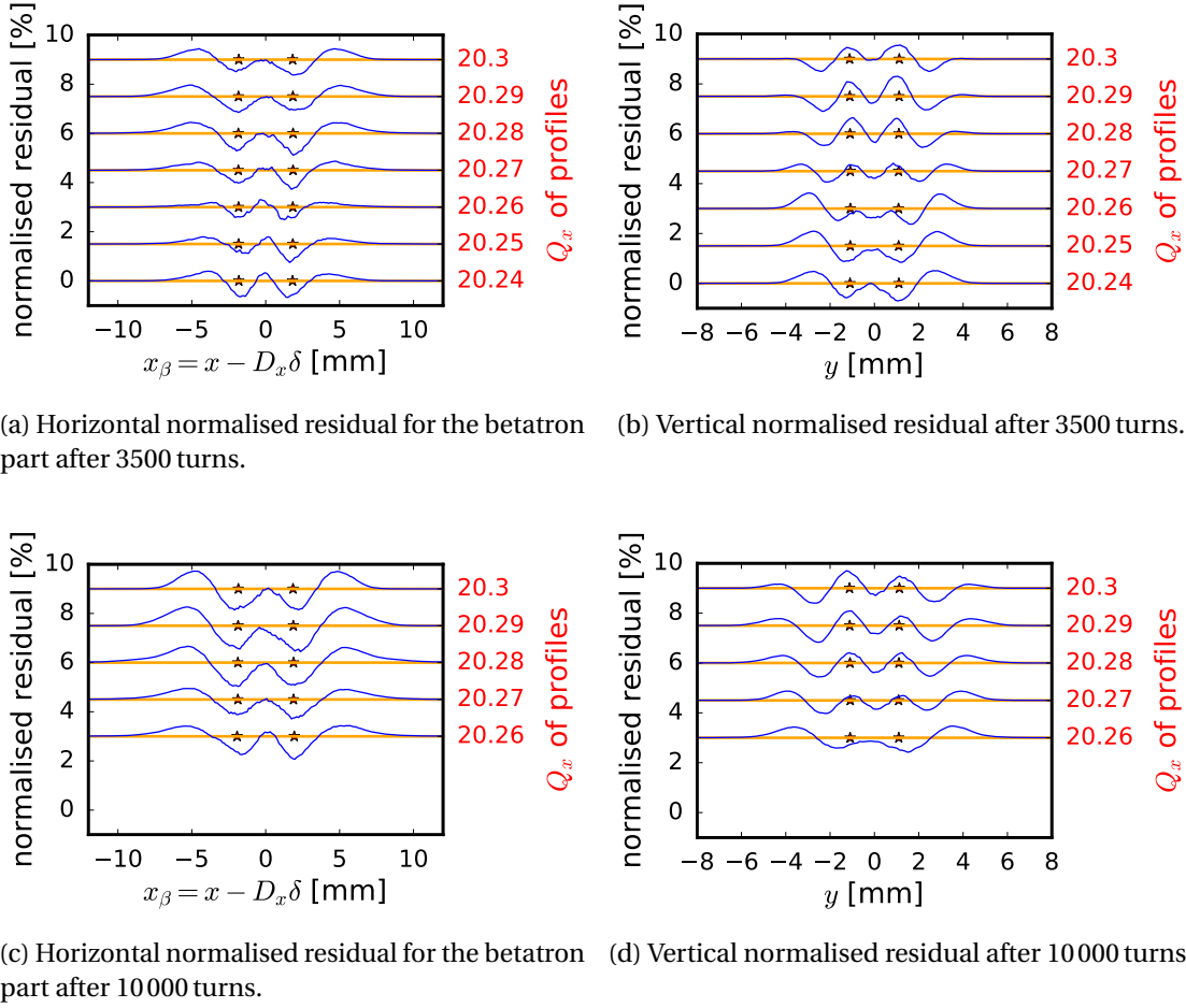
Figure 4.21 – Residuals of the transverse beam profiles via subtraction of the Gaussian fits show the created tails. The red stars indicate the Gaussian 1\sigma widths.
