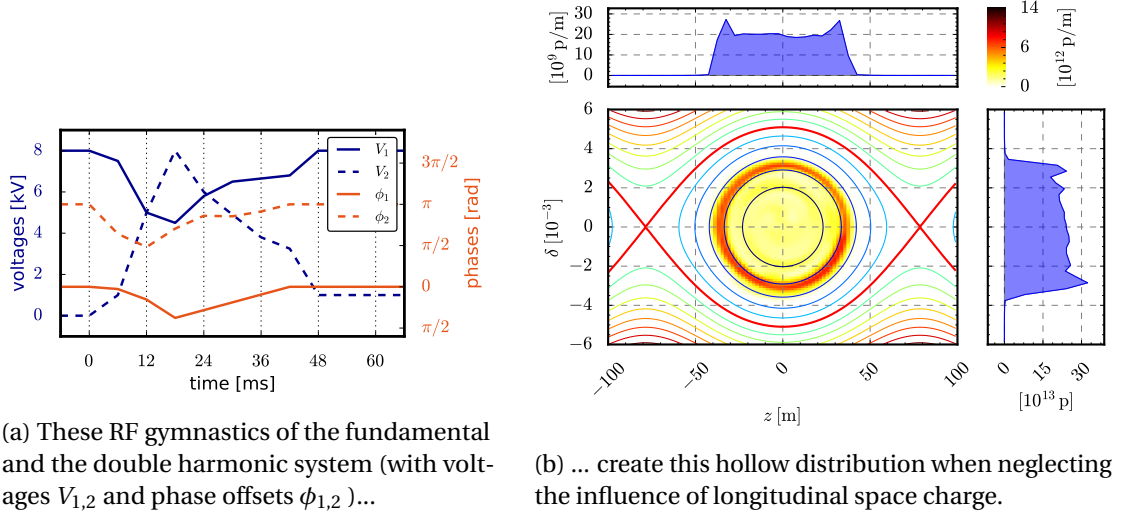
Figure 5.2 – Insertion of empty phase space into the longitudinal distribution.
