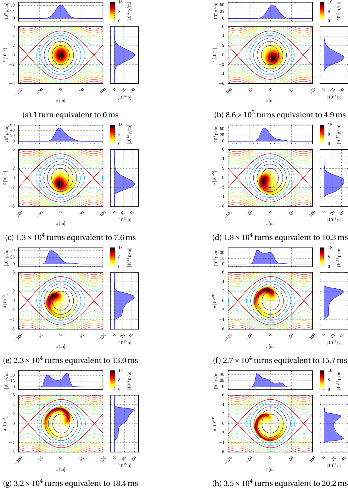
Figure 5.7 – Longitudinal phase space (z, \delta) during the RF phase modulation. The excitation of a longitudinal dipolar parametric resonance at \hat{\phi}_{\text{drive}} = 18^\circ is shown for a duration of nine synchrotron periods. The simulation includes longitudinal space charge effects.
