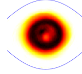
(c) Second (central) triplet bunch.
