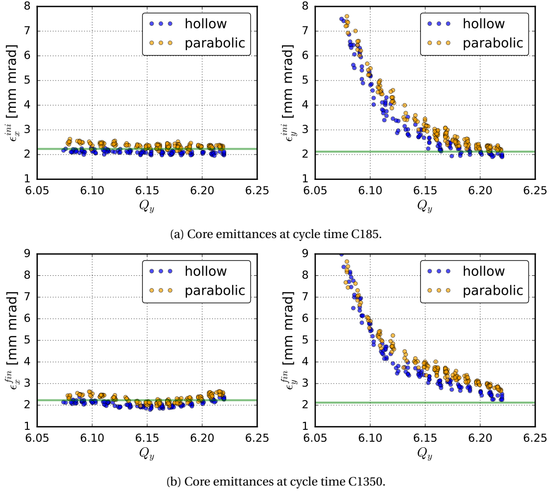
Figure 5.25 – Measured transverse core emittances versus the vertical tune. The green line shows the PS Booster emittance measured for a parabolic bunch at extraction using expression (2.35).
