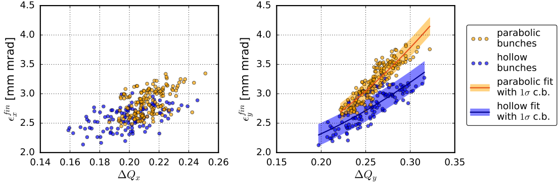
Figure 5.24 – Final core emittances versus Gaussian reference space charge detuning (based on assuming a 6D Gaussian distributed bunch). A quadratic fit is superimposed with its 1\sigma confidence band.
