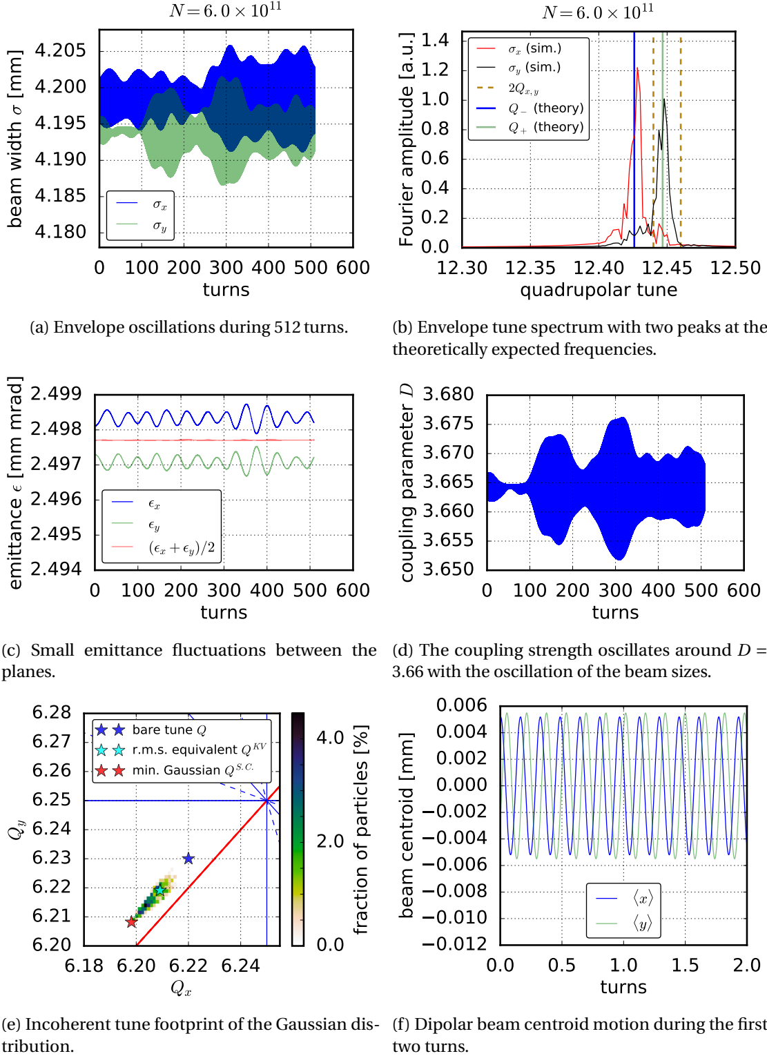
Figure 3.19 – Envelope oscillations for a Gaussian distribution with r.m.s. equivalent KV tune shift \Delta Q^{\text{KV}} = 0.011 at transverse betatron tunes Q_x = 6.22 and Q_y = 6.23 . With the approximately round beam of 2\sigma_x \approx 2\sigma_y \approx 8.4 mm, the coupling strength amounts to D = 3.66 .
