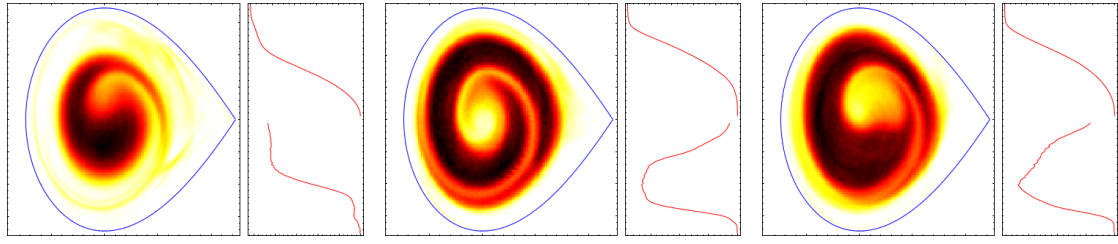
(a) 5 synchrotron periods
