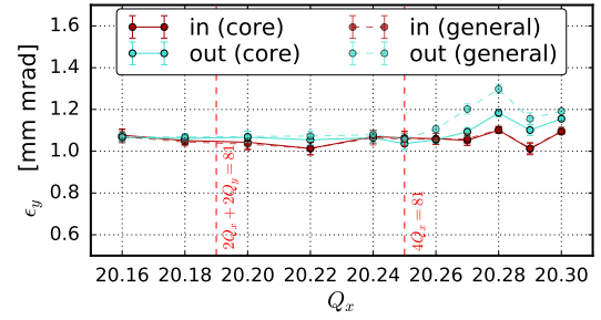
(b) Vertical emittance from core and general Gaussian fit vs. horizontal tune
