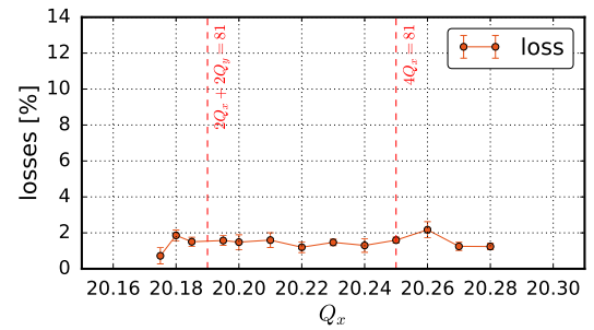
(b) Relative beam losses vs. horizontal tune
