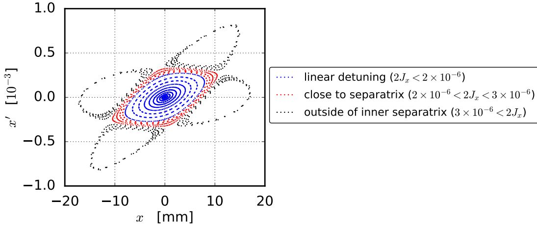
Figure 4.17 – Poincaré section for horizontal phase space (x, x') plotting particles of various amplitudes J_x during 128 turns at the horizontal wire scanner location. The extraction octupole L0E . 10402 imprints with resonant islands on the phase space at a bare machine tune of Q_x = 20.24 .
