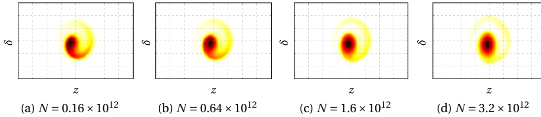
Figure 5.9 – Longitudinal phase space (z, \delta) for different intensities N after 25T_S of excitation at a very weak driving amplitude of \hat{\phi}_{\text{drive}} \approx 0.7^\circ . The simulation shows for increasing intensities how the bunch core ceases to decohere during the resonant centroid motion. Longitudinal space charge prevents the azimuthal spreading and hence works against the hollowing mechanism. The numeric experiment is conducted at 2 GeV, the future PS Booster extraction energy where space charge is expected to play a minor role compared to lower energies.
