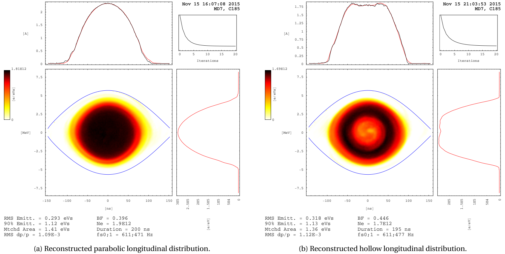
Figure 5.18 – Tomograms of typical candidates for the two compared beam types show the charge density in phase space ( t, \Delta E ) along with the projected beam profile and energy distribution. Both measurements have been taken in the PS at cycle time C185.
