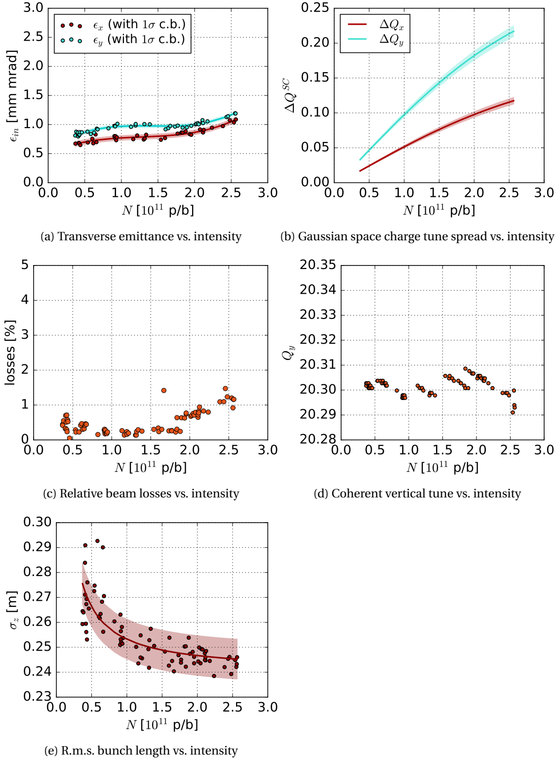
Figure 4.7 – Intensity scan for constant emittance keeping the coherent dipolar tunes fixated around (Q_x, Q_y) \approx (20.22, 20.30) .
