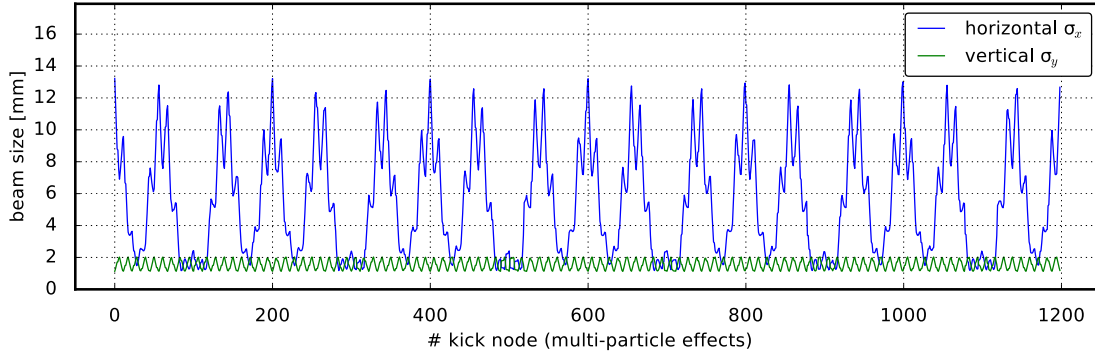
Figure 3.1 – Transverse beam sizes around the SPS ring (using the “Q20” optics, cf. chapter 4) for a low-emittance beam. The SPS ring has been split into 1200 nodes to sufficiently resolve the beam size for space charge simulations.
