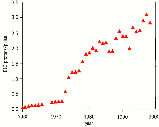
Figure 1.2 – Annual PS peak intensity in protons per pulse from 1960 till 2000 [PS Staff 1999].
