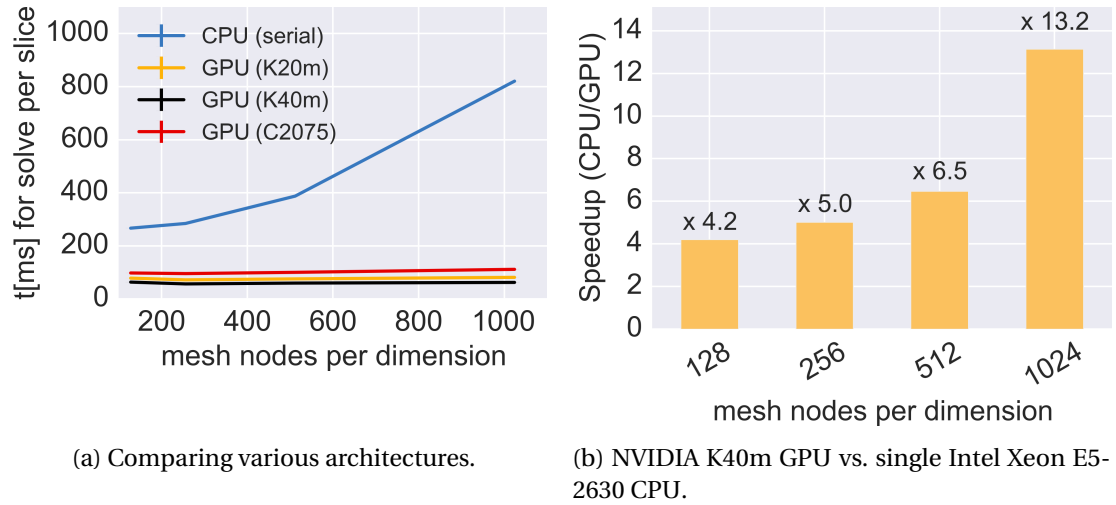
Figure 3.7 – Overall 2.5D PIC speed-up achieved (for a single slice) vs. number of mesh nodes per transverse dimension [Oeftiger and Hegglin 2016].
