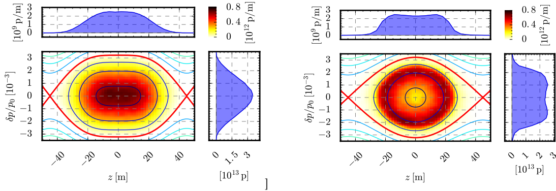
(a) Double-harmonic bucket in bunch lengthening mode (i.e. 180^\circ relative phase and V_{h=2} = V_{h=1}/2 ) populated with a matched distribution (note the quasi-Gaussian distribution in the momentum projection).
