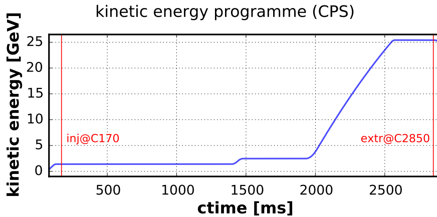
Figure 5.16 – Kinetic energy along the double batch injection PS cycle [Damerau 2011].
