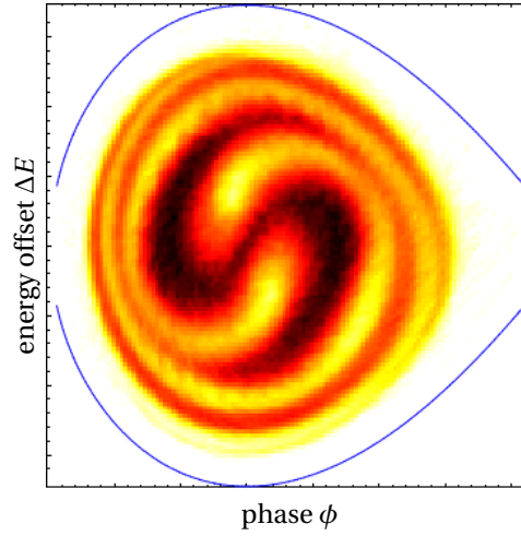
Figure 5.6 – Longitudinal phase space ( \phi, \Delta E ) via phase space tomography measured in the PS Booster (with \phi = -hz/R and \Delta E = \delta p_0 c / \beta to relate to the variables used in the simulations). The distribution resulted from a 1 : 2 dipolar parametric resonance which has been excited during seven synchrotron periods. The corresponding two filaments spiralling outwards from the core are clearly visible.
