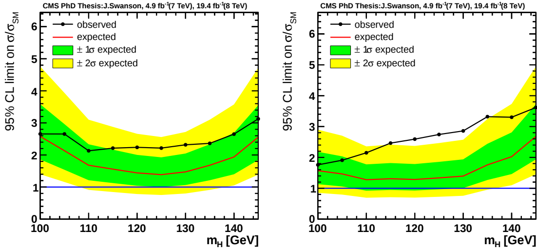
Figure 7.4: Observed and expected upper limit exclusions on the standard model Higgs cross section at at 95% C.L. as a function of Higgs boson mass. Green and yellow bands correspond to 1 and 2 sigma expected uncertainty in the absence of signal. The plots correspond to the 1-jet (left) and VBF (right) categories individually combined.
