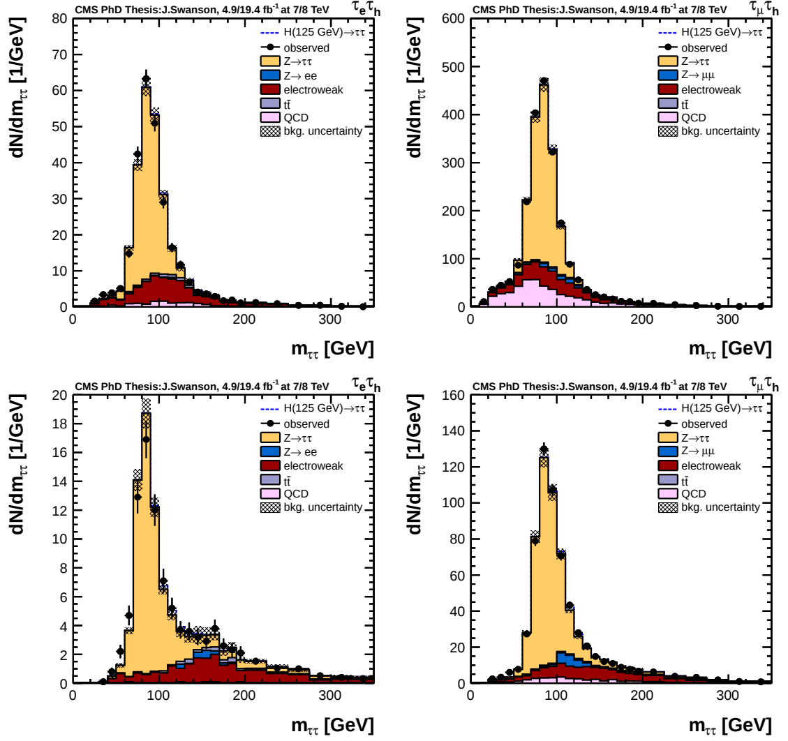
Figure 7.2: Post fit SVFit mass distributions of \tau\tau events from the 1-jet categories. The 7 TeV and 8 TeV distributions are combined. The distribution are for the \tau_e\tau_h (left) and \tau_\mu\tau_h (right) channel and low (top) and high (bottom) \tau_h p_T categories respectively. The uncertainty on the background is represented in the shaded region and comes from the fitted nuisances.
