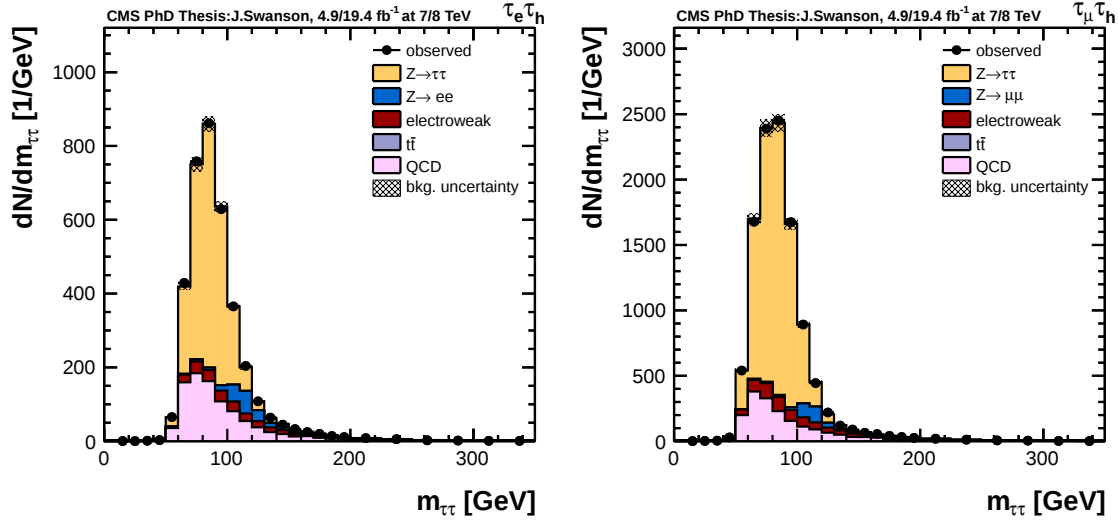
Figure 7.1: Post fit SVFit mass distributions of \tau\tau events from the 0-Jet category. The low and high \tau_h p_T categories and 7 TeV and 8 TeV are combined. The distributions are for the \tau_e\tau_h (left) and \tau_\mu\tau_h (right) channel respectively. The uncertainty on the background is represented in the shaded region and comes from the fitted nuisances.
