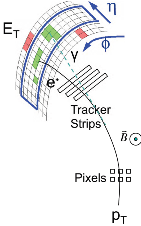
Figure 5.1: A graphical representation of an electron produced in the CMS detector. Notice the bending of the electron inside the magnetic field and the subsequent energy lost due to bremsstrahlung radiation which spreads the ECAL supercluster in the \phi direction.
