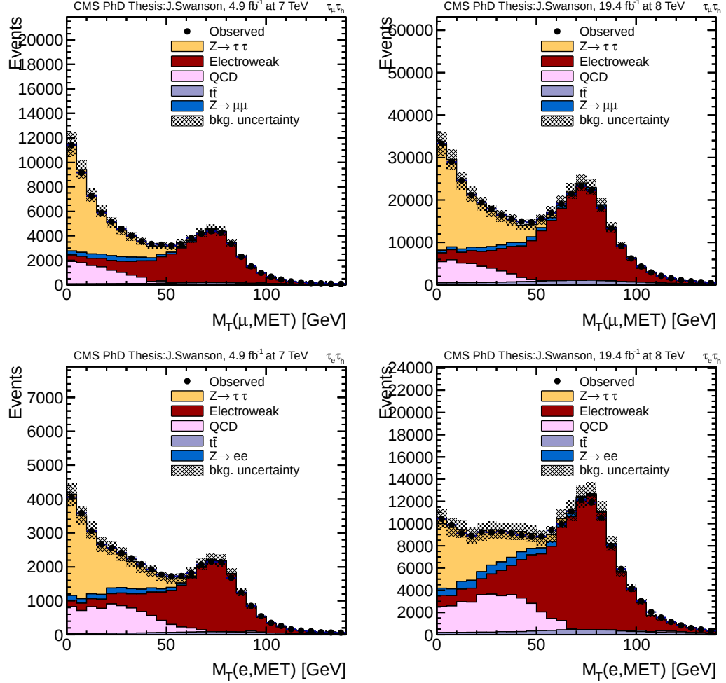
Figure 6.1: Distribution of the transverse mass from the \tau_\mu\tau_h (top) and \tau_e\tau_h (bottom) channels. The plots on the left and right correspond to the 7 TeV and 8 TeV periods respectively. The background components (except W^\pm ) are scaled relative to the results of a fit to the inclusive mass distribution. The uncertainty on the background is represented in the shaded region and comes from the fitted nuisances.
