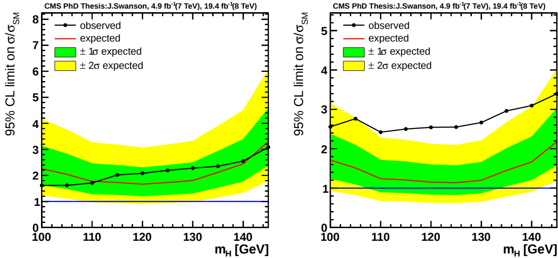
Figure 7.5: Observed and expected upper limit exclusions on the standard model Higgs cross section at at 95% C.L. as a function of Higgs boson mass. Green and yellow bands correspond to 1 and 2 sigma expected uncertainty in the absence of signal. The plots correspond to the limit set in the \tau_e \tau_h (left) and \tau_\mu \tau_h (right) channels separately.
