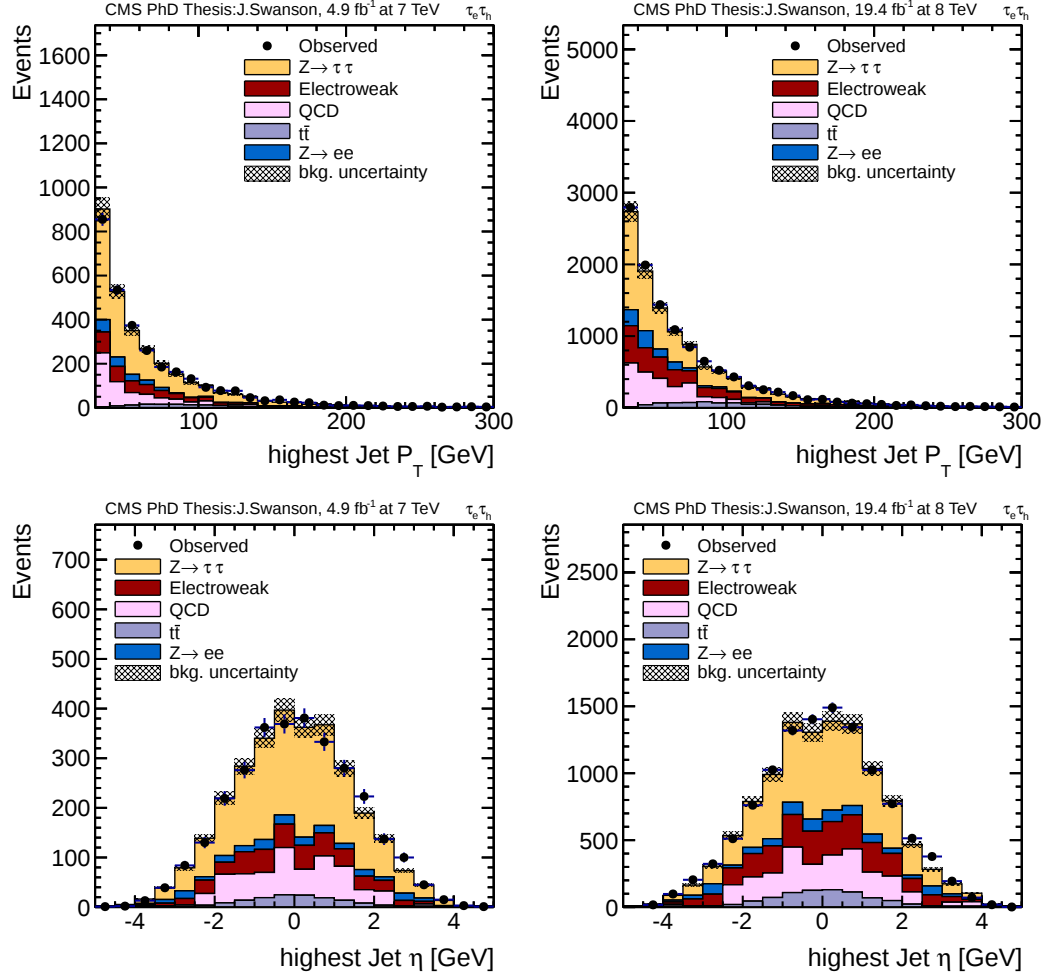
Figure 5.6: Distribution of the leading jet transverse momentum and pseudorapidity from the \tau_e \tau_h channel for events containing at least one jet. The background components are scaled relative to the results of a fit to the 1 jet mass distribution. The uncertainty on the background is represented in the shaded region and comes from the fitted nuisances.
