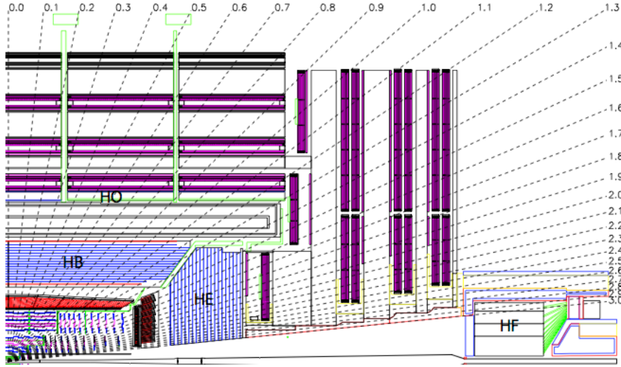
Figure 3.6: A longitudinal diagram of the CMS HCAL system. Dashed lines are at fixed \eta values.
