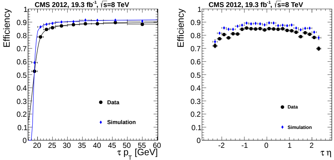
Figure 5.11: Efficiency of the L3 \tau algorithm from the \mu\tau cross object trigger plotted as a function of transverse momentum (left) and pseudorapidity (right).
