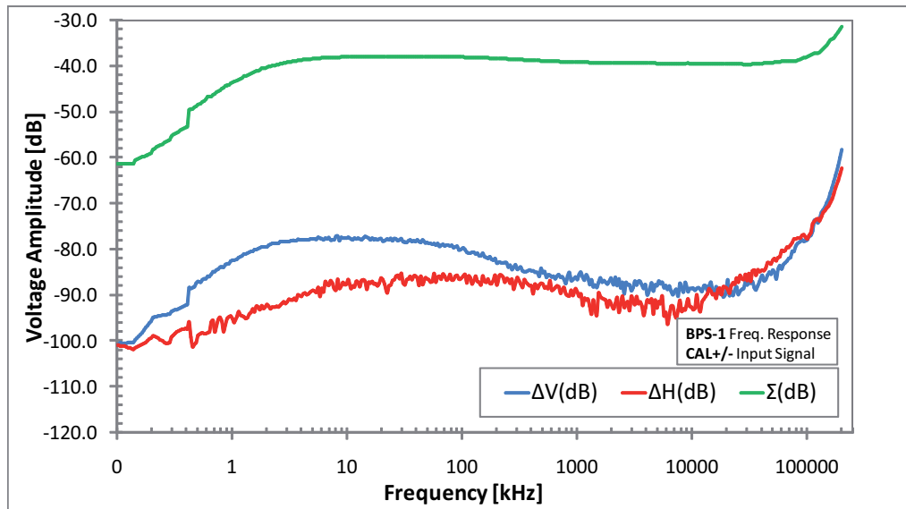
Figure 4.12: BPS1 frequency response for the \Delta V , \Delta H and \Sigma signals when exciting the positive (Cal+) and negative (Cal-) calibration input at the same time.
