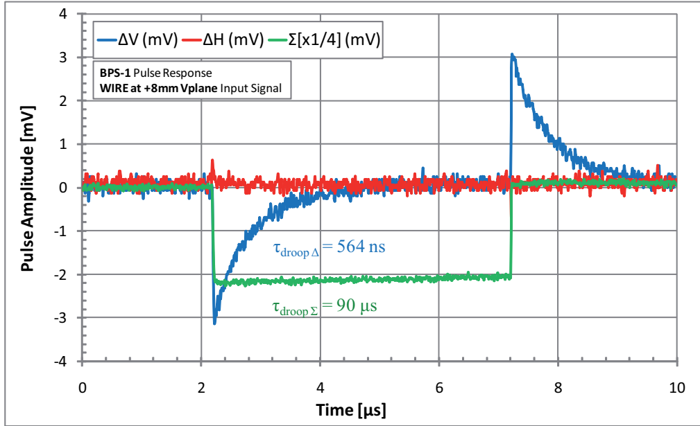
Figure 4.13: BPS1 transmitted pulse for \Delta and \Sigma signals at +8 mm wire position in the vertical plane, and positive input pulse of 5 V and 5 \mu s.
