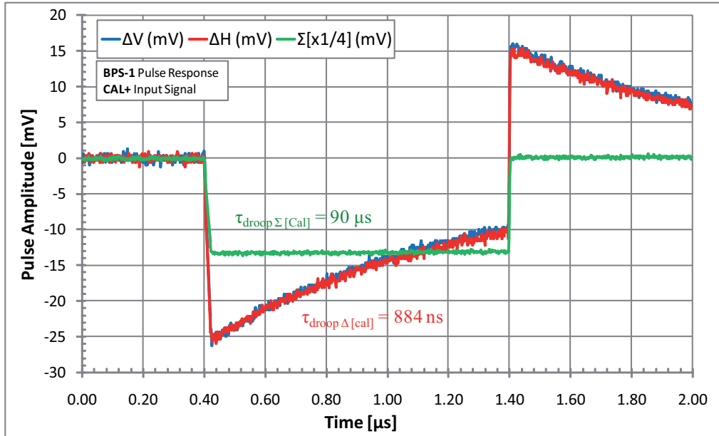
Figure 4.14: BPS1 transmitted pulse for \Delta and \Sigma signals with positive calibration input excitation (Cal+), and positive input pulse of 5 V and 1 \mu s.
