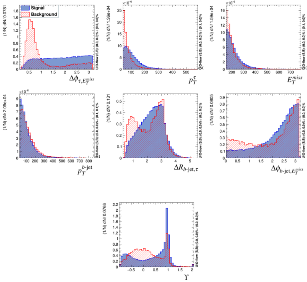
FIGURE 6.2: Distributions of input variables for BDT training within 200-400 GeV. Signal is presented as a blue, solid histogram; top production background (as estimated from MC) is presented as a red, dashed histogram. Histograms are arbitrarily normalized.
