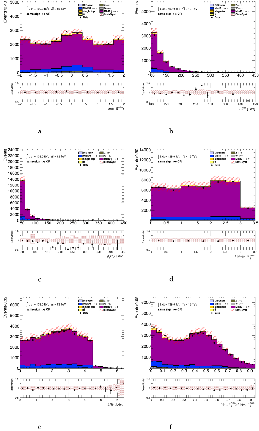
FIGURE B.1: Distributions of input variables for BDT-training for \tau_{\text{had-vis}} + \text{lep} channel in \tau +electron same sign control region (a) \Delta\phi_{\tau, \text{miss}} (b) E_T^{\text{miss}} (c) p_T^\tau (d) \Delta\phi_{bjet, \text{miss}} (e) \Delta R_{bjet, \tau} (f) \Delta\phi_{\tau, \text{miss}} / \Delta\phi_{jet, \text{miss}} where the jets are two hardest jets, the distribution of Y is already shown in Figure 7.31 (a).
