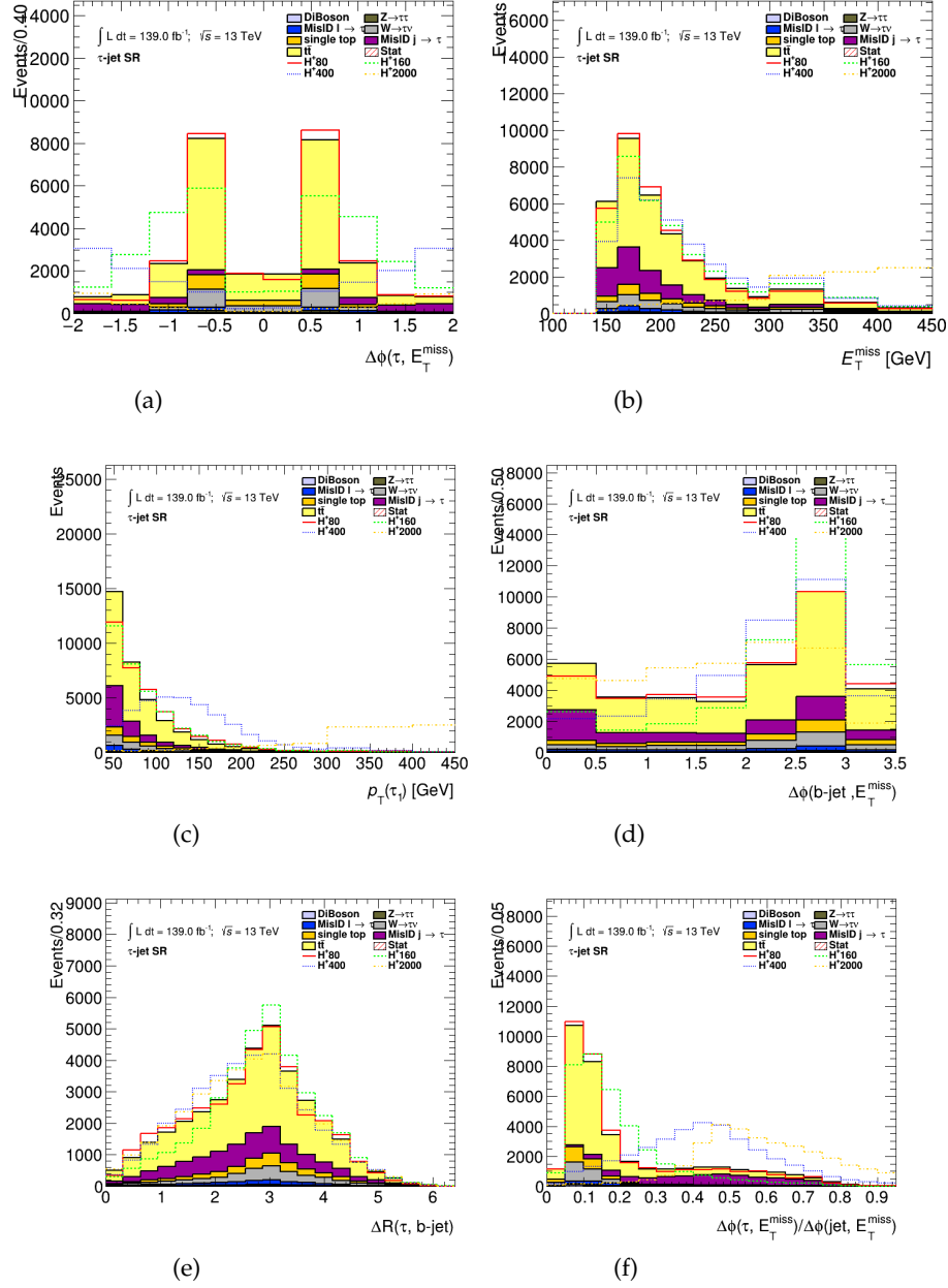
FIGURE B.3: Distributions of input variables for BDT training for \tau_{\text{had-vis}} + \text{jet} signal region, \Delta\phi_{\tau, \text{miss}} (a) E_T^{\text{miss}} (b), p_T^\tau (c) \Delta\phi_{\text{bjet}, \text{miss}} (d) \Delta R_{\text{bjet}, \tau} (e) \Delta\phi_{\tau, \text{miss}} / \Delta\phi_{\text{jets}, \text{miss}} (f) where the jets are two hardest jets.
