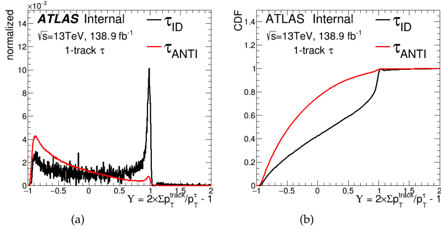
FIGURE 7.30: Distribution of the Y for \tau_{\text{had-vis}} (black) and anti- \tau_{\text{had-vis}} (red) candidates in the W+jets control region (a). CDF of Y for \tau_{\text{had-vis}} (black) and anti- \tau_{\text{had-vis}} (red) candidates in the W+jets control region (b).
