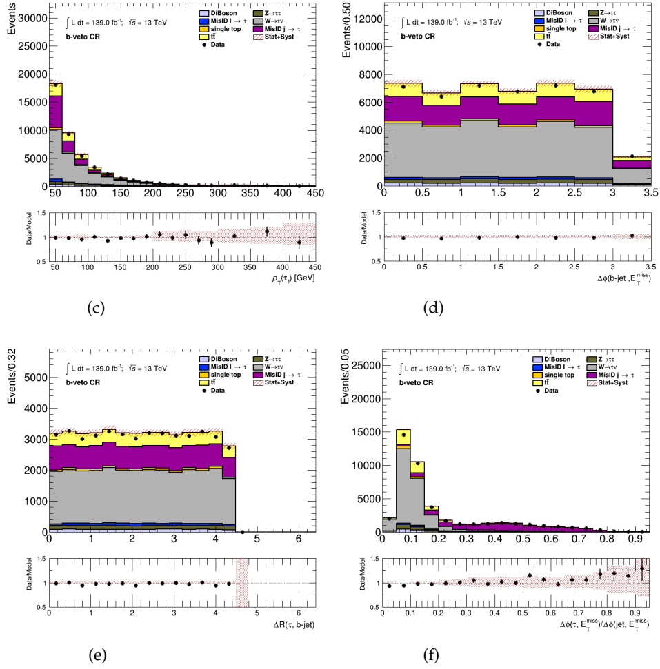
FIGURE 7.33: Distributions of input variables for BDT training for \tau_{\text{had-vis}} + \text{jet} channel in the b -veto control region, p_T^\tau (c) \Delta\phi_{b\text{jet},\text{miss}} (d) \Delta R_{b\text{jet},\tau} (e) \Delta\phi_{\tau,\text{miss}} / \Delta\phi_{\text{jets},\text{miss}} (f) where the jets are two hardest jets, the distribution of Y is shown in Figure 7.31 (a). The uncertainty band in the ratio plots includes both statistical and fake factor method systematic uncertainty.
