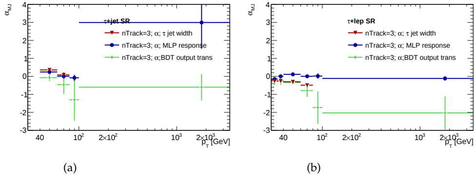
FIGURE 7.17: \alpha_{MJ} as a function of p_T^\tau for 3-prong \tau_{\text{had-vis}} candidates estimated by the template fit method using \chi^2 with the \tau jet width, the MLP response and the transformed BDT score (red, blue and green lines respectively) for (a) \tau_{\text{had-vis}}+\text{jet} signal region and (b) \tau_{\text{had-vis}}+\text{lepton} signal region.
