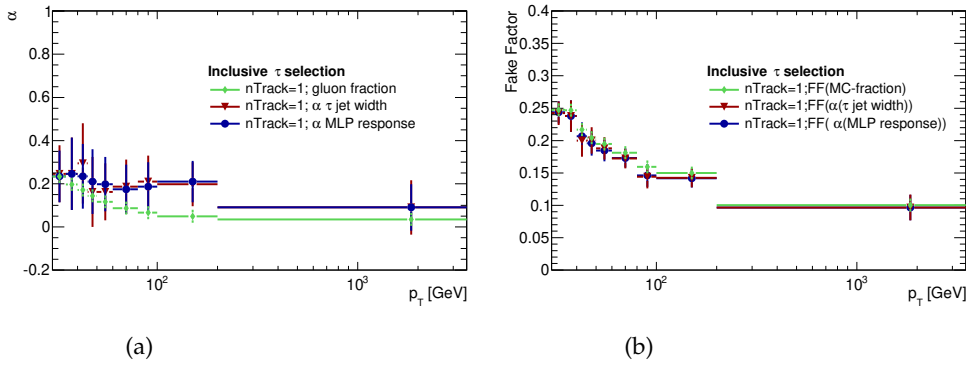
FIGURE 7.28: The distribution of \alpha_g estimated by the template fit from \tau jet width and the MLP response in comparison with the real number of gluons in the \tau_{\text{had-vis}} + \text{lepton} signal region (a) and the combined fake factors estimated by corresponding \alpha_g estimation (b).
