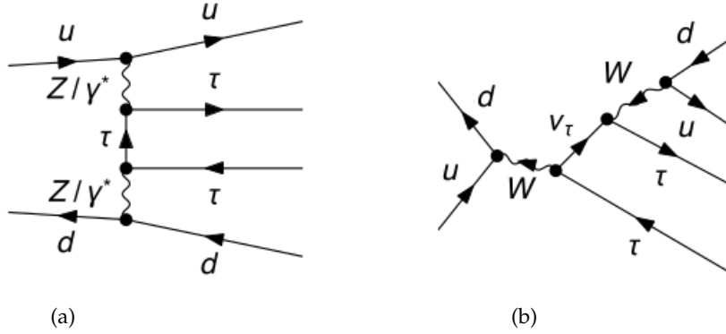
FIGURE 3.1: Typical topologies of diagrams contributing to the Drell-Yan-type SM process in u\bar{d} \rightarrow \tau^+ \tau^- u\bar{d} : multi-peripheral (a), t-cascade (b)
