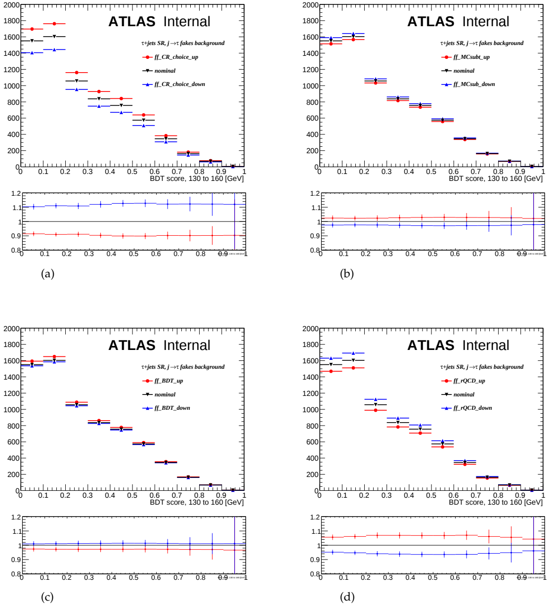
FIGURE 7.29: Effect of systematic variations on the BDT score in the H^+ mass range 130–160 GeV in the \tau_{\text{had-vis}} +jets signal region: choice of control region (a) true \tau contamination in the anti- \tau_{\text{had-vis}} control region (b), lower cut of the transformed \tau_{\text{had-vis}} BDT score (c) and \alpha_{MJ} uncertainty (d).
