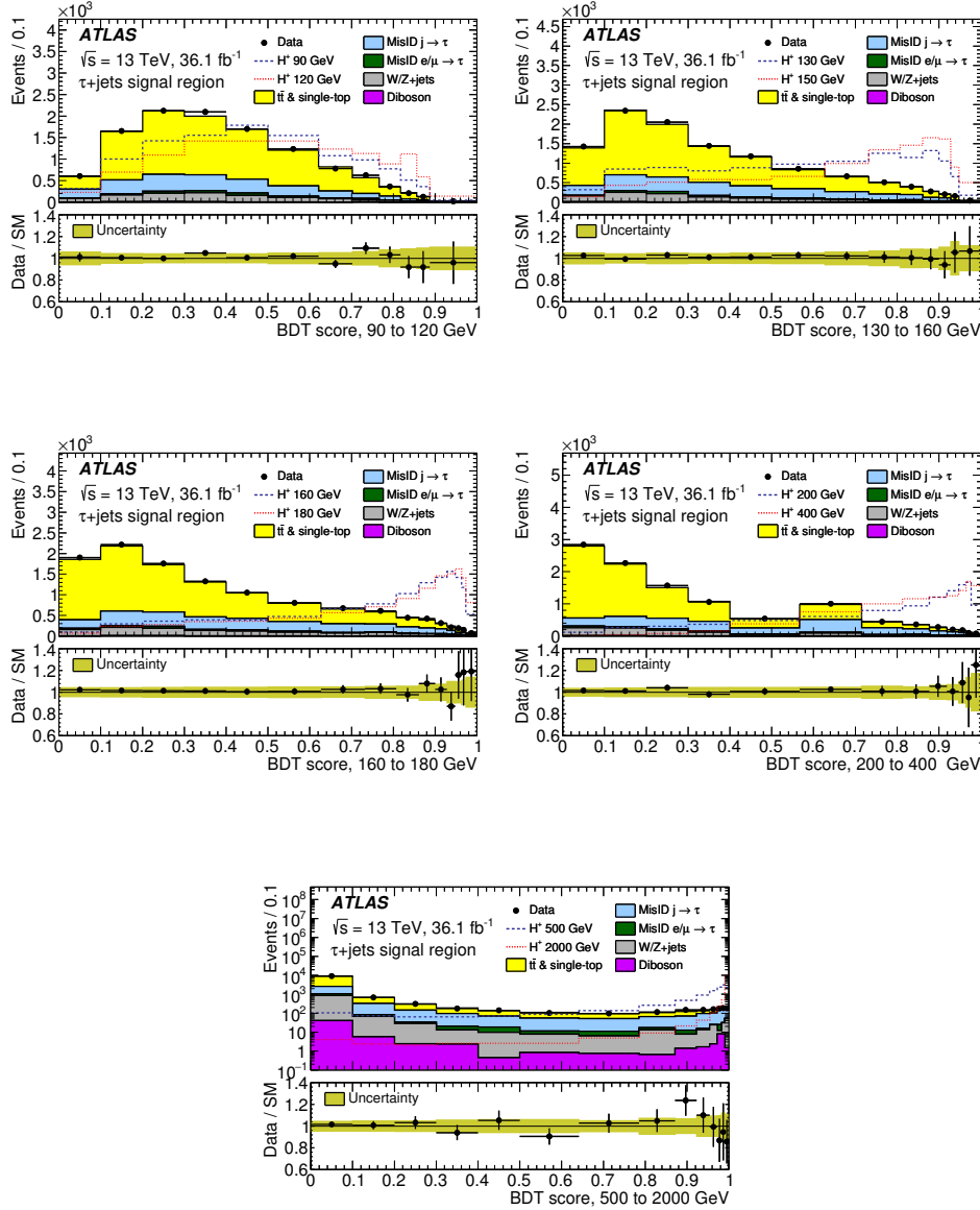
FIGURE 6.16: Distributions of the BDT score in the \tau_{\text{had-vis}}+\text{jets} signal region, in the five mass ranges used for BDT training, after a fit to the data with the background-only hypothesis. The lower panel of each plot shows the ratio of data to the SM background prediction. The uncertainty bands include all statistical and systematic uncertainties. The normalization of the signal (shown for illustration) corresponds to the integral of the background [6].
