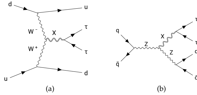
FIGURE 3.3: Topologies of Feynman diagrams for X production through its coupling to gauge bosons VBF process (a) and X -Strahlung process (b). Similar diagrams, with different combinations of W^\pm 's, Z 's, photons and quark flavours also exist.
