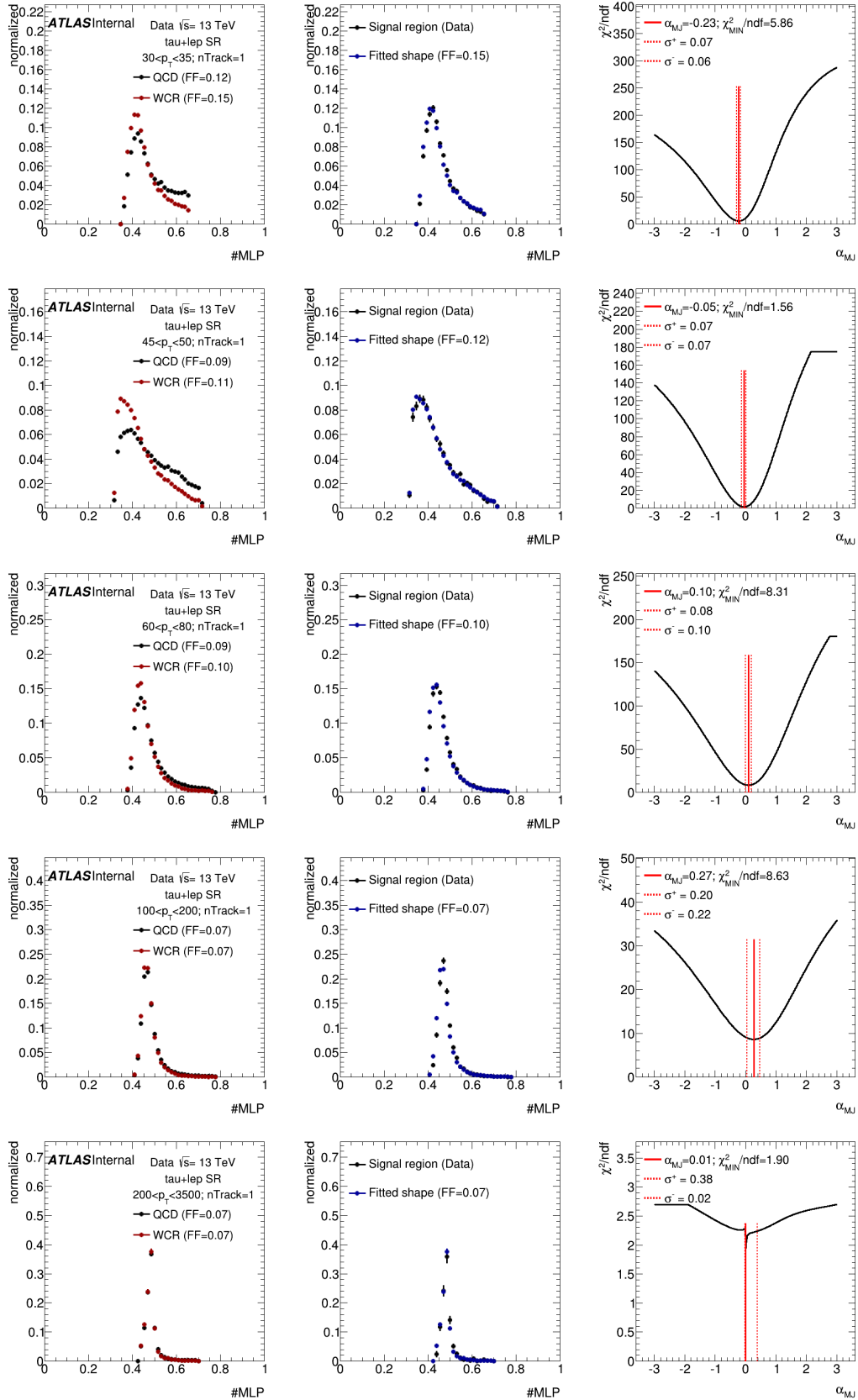
FIGURE 7.14: Estimation of \alpha_{MJ} in the \tau_{\text{had-vis}} + \text{lepton} signal region and in the anti- \tau_{\text{had-vis}} region defined with not-loose working point for 1-prong \tau_{\text{had-vis}} candidates. Left: templates of discriminating variables MLP for different p_T^\tau slices. Middle: shape of the discriminating variable obtained in the signal region and fitted shape using the templates measured in the control regions. Right: \chi^2/ndf of the fit as a function of \alpha_{MJ} , the error on \alpha_{MJ} is defined by the band at \chi^2_{\min}/ndf + \sqrt{\frac{2}{ndf}} .
