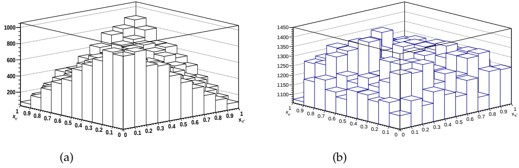
FIGURE 3.11: Distribution of x_{\tau}^{+} versus x_{\tau}^{-} before (a) and after (b) reweighting for Sherpa 2.2.
