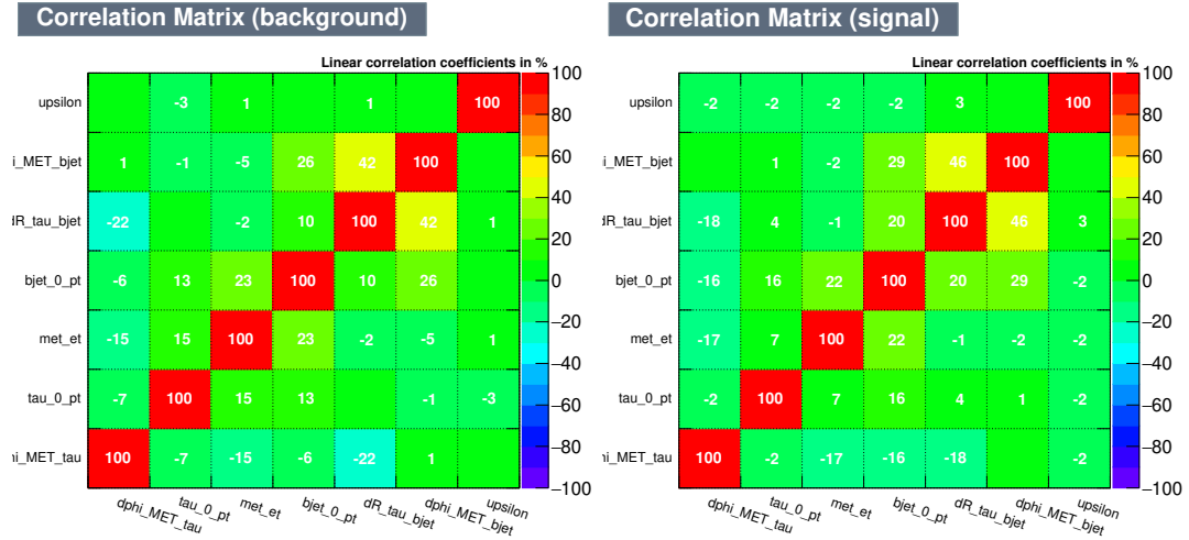
FIGURE 6.3: Correlation matrix of BDT input variables for the background (left plot) and signal (right plot), the H^+ mass range, 90-120 GeV. Here: \epsilon = \Upsilon ; dphi\_MET\_bjet = \Delta\phi_{b-jet, E_T^{miss}} ; dR\_tau\_bjet = \Delta R_{b-jet, \tau} ; bjet\_0\_pt = p_T ; met\_et = E_T^{miss} ; tau\_0\_pt = p_T^\tau and dphi\_MET\_tau = \Delta\phi_{\tau, E_T^{miss}} .
