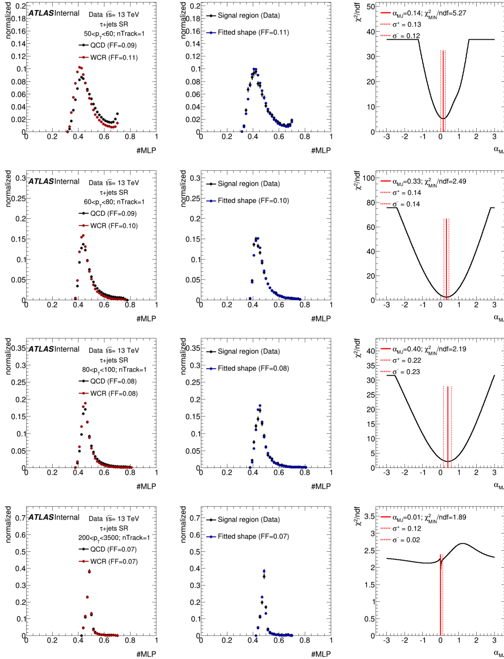
FIGURE 7.13: Estimation of \alpha_{MJ} in the \tau_{\text{had-vis}} + \text{jets} signal region and in the anti- \tau_{\text{had-vis}} region defined with not-loose working point for 1-prong \tau_{\text{had-vis}} candidates. Left: templates of the MLP response for different p_T slices. Middle: shape of the discriminating variable obtained in the signal region and fitted shape using the templates measured in the control regions. Right: \chi^2/ndf of the fit as a function of \alpha_{MJ} , the error on \alpha_{MJ} is defined by the band at \chi^2_{\text{min}}/ndf + \sqrt{\frac{2}{ndf}} .
