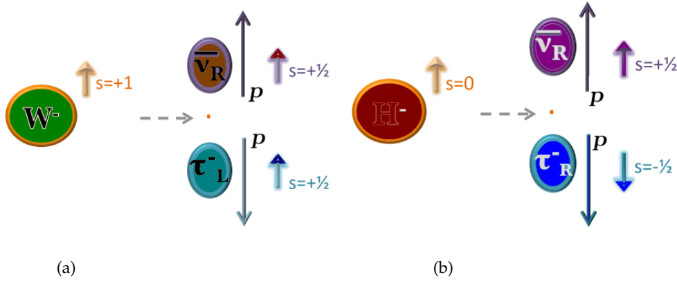
FIGURE 2.8: The W^- \rightarrow \tau_L^- \nu (a) and H^- \rightarrow \tau_R^- \nu (b), in the rest frame of the bosons. Since W boson has spin 1, the \frac{1}{2} -spin directions of the subsequent leptons must be compensated. Moreover, since the state of the \nu is fixed by nature, the spin of the \tau lepton has to be oriented opposite to the direction of flight. However, the H^- spin=0 causes the spin vectors of the subsequent leptons to be in opposite directions [39].
