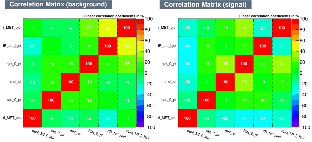
FIGURE 6.5: Correlation matrix of BDT input variables for back-grounds (left plot) and signal (right plot), the H^+ mass ranges 500-2000 GeV. Here: upsilon = Y ; dphi\_MET\_bjet = \Delta\phi_{b-jet, E_T^{miss}} ; dR\_tau\_bjet = \Delta R_{b-jet, \tau} ; bjet\_0\_pt = p_T ; met\_et = E_T^{miss} ; tau\_0\_pt = p_T^\tau and dphi\_MET\_tau = \Delta\phi_{\tau, E_T^{miss}} .
