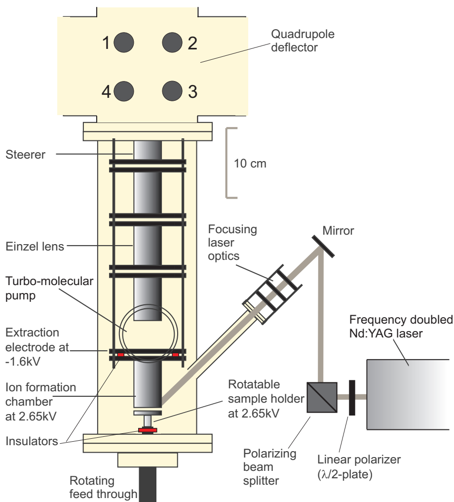
Figure 5.5: The present laser ion source layout. Steerers were implemented and the insulating material was changed to avoid shortcuts in the ion optics system. The laser system was modified by adding an attenuator, which works via polarization selective elements (linear polarizer and polarizing beam splitter).
