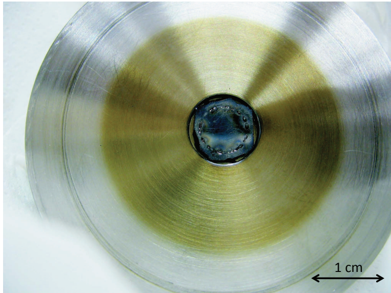
Figure 5.2: Photograph of an ISOLTRAP Sigradur pellet glued on a stainless steel sample holder. A circle on the target material formed by many craters is the result of many hours of the laser ablation process. The pellet is continuously rotating (with about 2 Hz) to ensure that the beam is hitting different positions on the Sigradur surface. The surrounding of the solid target is coated by carbon dust.
