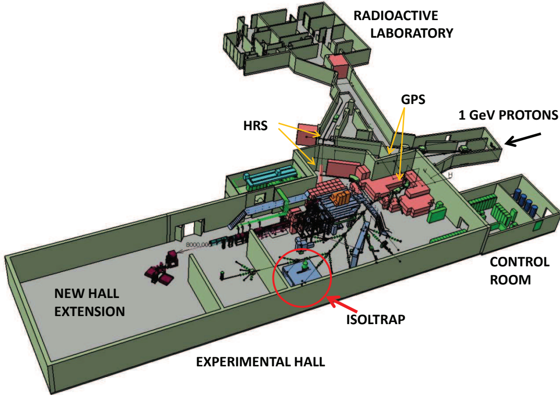
Figure 3.3: Experimental hall of the ISOLDE facility [Kug00]. On the upper right the protons coming from the Proton Synchrotron Booster enter the hall and are impinged on a thick target, typically \text{UC}_x or \text{ThC}_x , to create radioactive nuclides. Two target stations, GPS or HRS, are available. After extraction and ionization the radionuclides are mass separated by one of the mass filters and pass ion optics before they enter ISOLTRAP via the central beamline.
