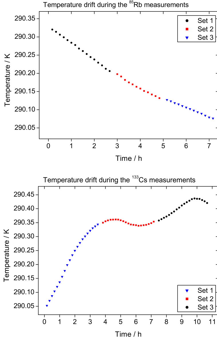
Figure 6.8: Temperature changes close to the precision trap, recorded during the measurements on ^{85}\text{Rb} (top) and ^{133}\text{Cs} (bottom). The duration of the measurement for one set corresponds to a temperature drift of \Delta T_{\min} \approx 20 mK and \Delta T_{\max} \approx 300 mK. Error bars are not presented since they are smaller than the symbol size.
