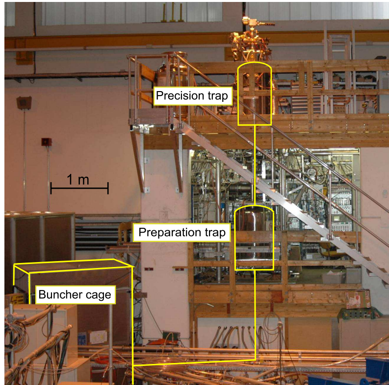
Figure 3.1: Photograph of the ISOLTRAP experiment with the three ion traps dedicated to preparation, purification and mass determination of radioactive ions [Muk08]. For more details see text.
