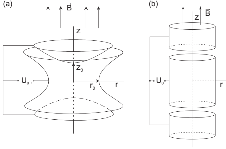
Figure 2.1: Sketch of Penning traps with conventional shapes. Applying a DC voltage between the endcaps and the ring electrode, both the a) hyperbolic as well as b) the cylindrical Penning trap, create a trapping potential in axial direction. The homogeneous magnetic field \vec{B} defines the z -axis and confines the ions in radial direction.
