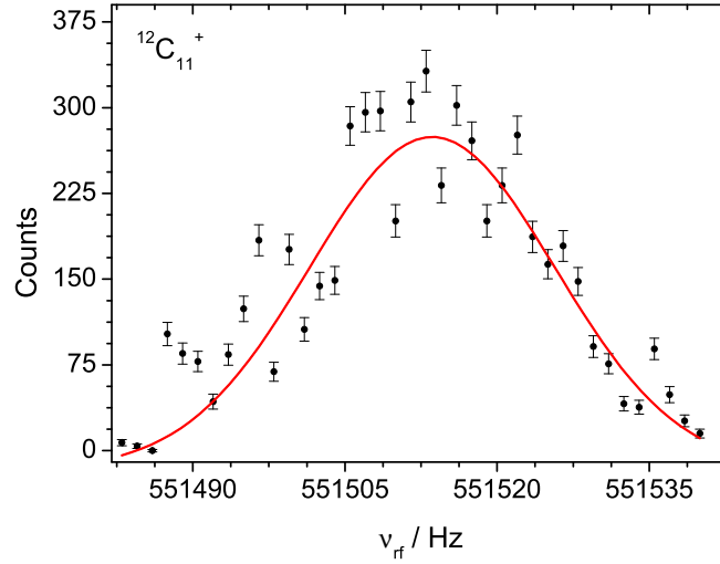
Figure 5.8: Cooling resonance of ^{12}\text{C}_{11}^+ with excitation time T_{\text{rf}} = 200 ms. The solid line is a Gaussian fit to the data. The center frequency is at \nu_c = 551513.6(2) Hz and the FWHM is 28.5(6) Hz. A resolving power of R \approx 19400 is obtained.
