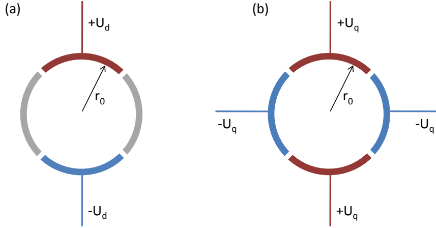
Figure 2.4: For a dipolar excitation voltages with 180^\circ phase-shift are applied to two diametral electrodes (a) while a quadrupolar excitation requires an rf voltage at all electrodes (b). The dipole excitation addresses single eigenmotions while the quadrupolar excitation with an adequate frequency transfers the energy of one eigenmotion into another.
