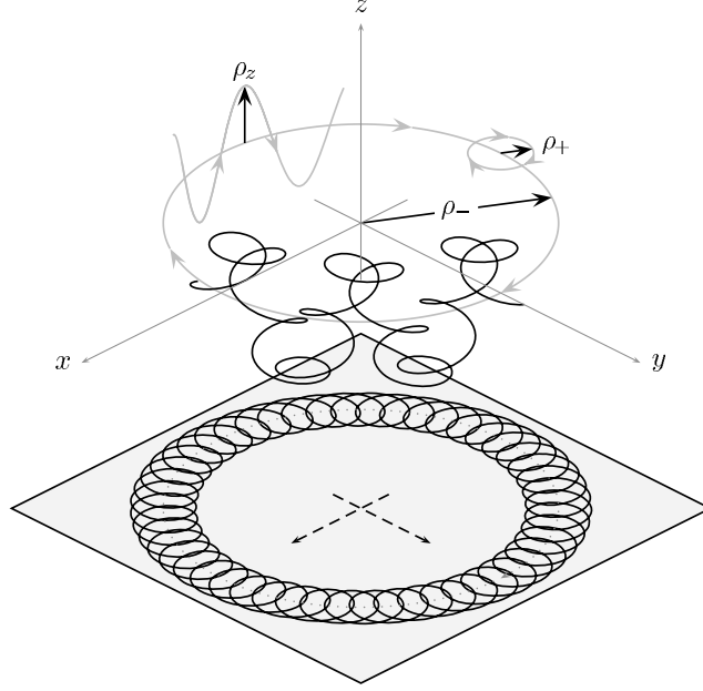
Figure 2.2: Ion motions in a Penning trap. \rho_+ , \rho_z and \rho_- are the radii of the modified cyclotron, the axial and the magnetron motion, respectively. The black solid line (top) shows the superposition of all three eigenfrequencies, whereas the solid line below represents the superposition of the radial eigenfrequencies. The frequencies and amplitudes are not to scale.
