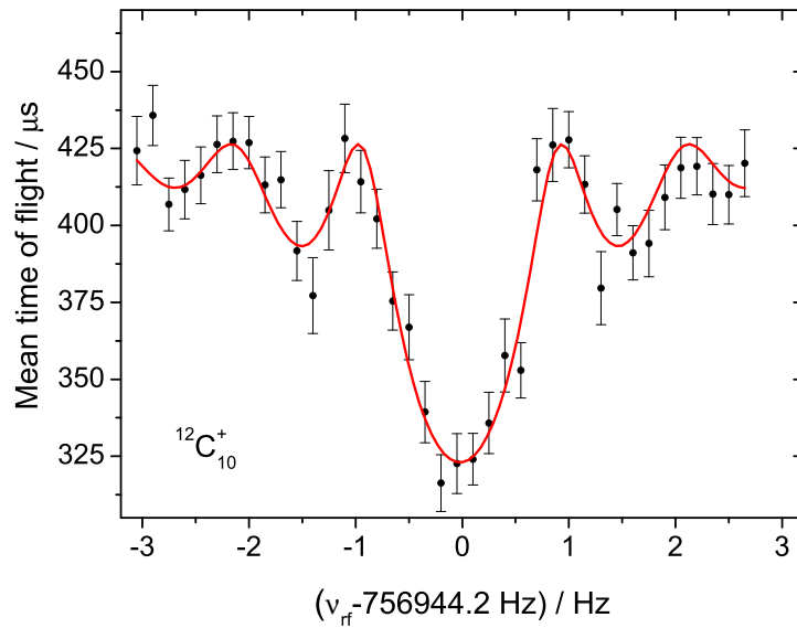
Figure 3.9: Time-of-flight spectrum of ^{12}\text{C}_{10}^+ with an excitation time of T_{\text{rf}} = 900 ms. The lineshape reflects the Fourier transform of the applied rectangular excitation signal. The solid line is a fit of the theoretical lineshape to the data [Kön95a].
