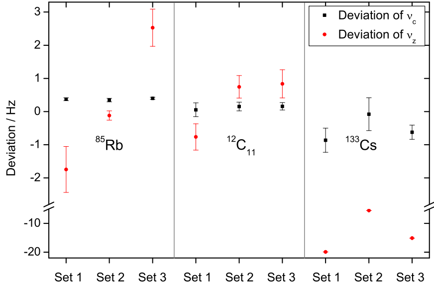
Figure 6.7: Deviation of the conversion frequency (black) and axial frequency (red) according to the values listed in Tab. 6.3.
