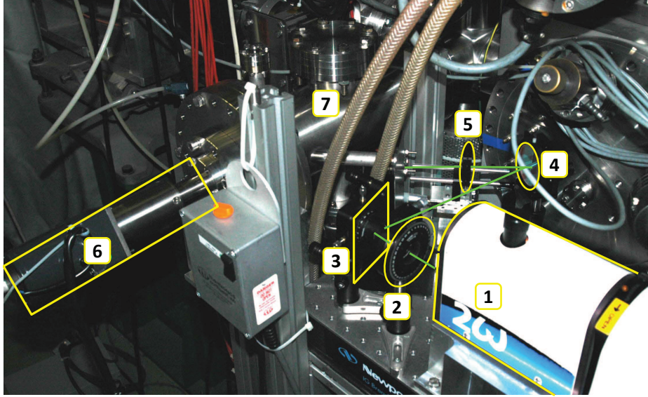
Figure 5.4: The close-to-linear polarization of the Nd:YAG laser beam (1) is rotated by a \lambda/2 -plate (2) and enters then the polarization sensitive beam splitter (3). Next, the laser beam is reflected by a mirror (4) and passes through a focusing lens (5). Afterwards the laser light hits a Sigradur pellet which is rotated by a motor (6) in order to ablate clusters at different pellet positions. The vacuum chamber (7) including the ion optics is attached to the ISOLTRAP beamline.
