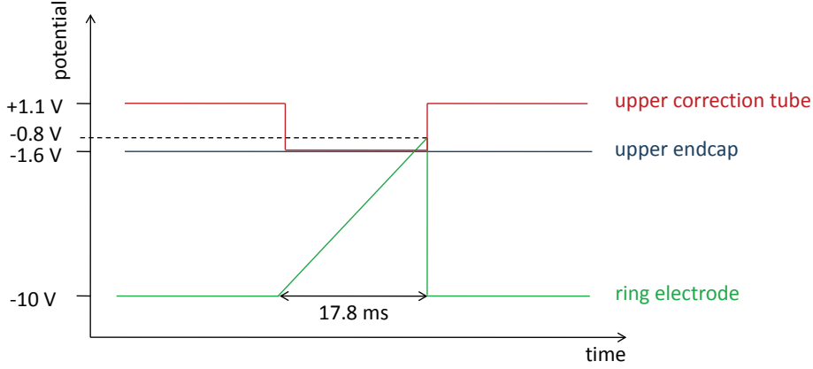
Figure 6.5: The potential of the ring electrode is ramped from -10 V to -0.8 V. Therefore, resonantly excited ions with enough axial energy leave the trap earlier than nonresonantly excited ions. In order to avoid the potential wall caused by the upper correction tube, this electrode is adjusted to the potential of the upper endcap while the ramp is applied to the ring electrode.
