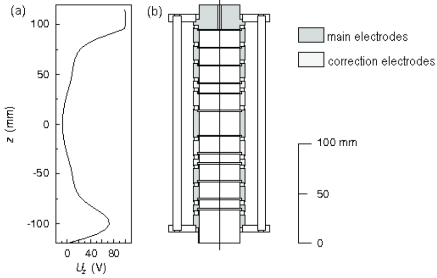
Figure 3.6: The harmonic trapping potential (a) in the center of the trap can only be realized by additional correction electrodes, which are shown in the detailed sketch (b) of the preparation trap.
