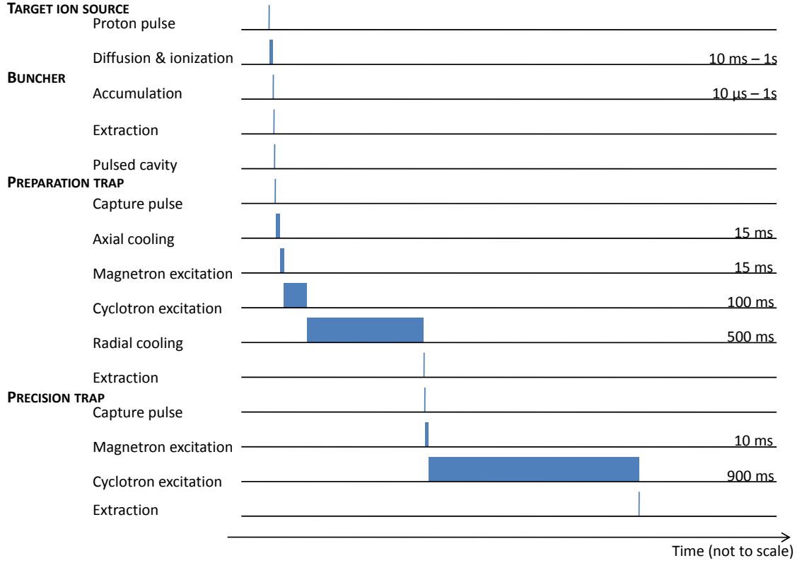
Figure 3.10: The timing of the signals for the measurement procedure is depicted. Each cycle is triggered by the proton pulse. After the ionization the quasi-continuous ion beam is passing the buncher. After an accumulation time ion bunches are guided to the tandem Penning trap system. For more details see text.
