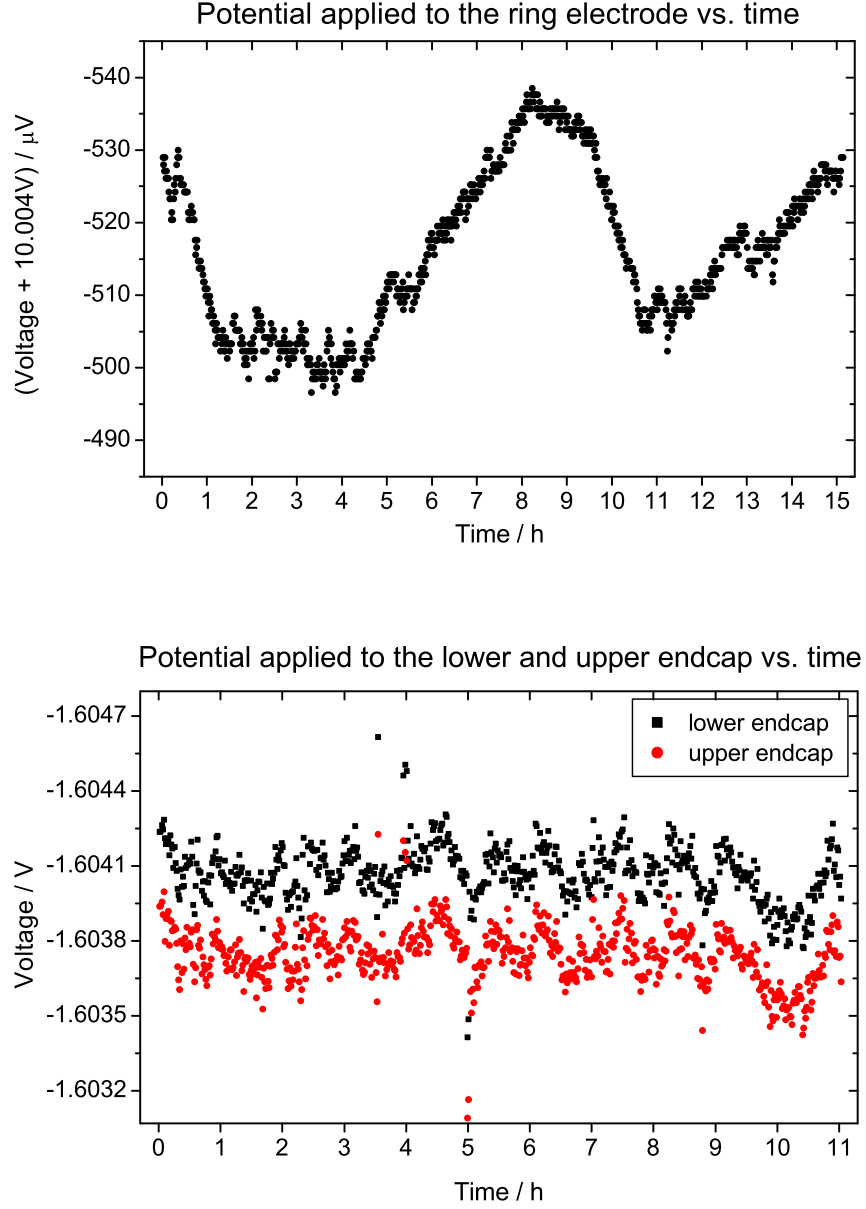
Figure 6.9: Fluctuations of the voltages applied to the main electrodes of the precision trap versus time. The potential of the ring electrode (top) shows a relative fluctuation of \delta U/U \approx 3.4 \cdot 10^{-6} within 3 hours (corresponding to the duration of the measurement of one set). Below the voltages applied to the upper (red) and lower (black) endcap versus time are presented with a relative fluctuation of \delta U/U \approx 2 \cdot 10^{-4} (during 3 hours). Error bars are not indicated since they are smaller than the symbol size.
