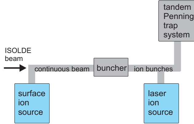
Figure 5.1: Two off-line ion sources used at ISOLTRAP produce stable ions required for test measurements, optimization of the ion transport and measurement process, as well as for the calibration of the magnetic field strength. On the one hand the surface ion source installed in front of the buncher provides a continuous alkali ion beam and on the other hand bunches of carbon cluster ions are generated by the laser ion source.
