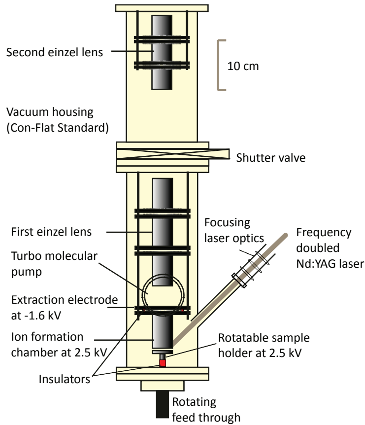
Figure 5.3: The previous setup was installed in the year 2004 at the ISOLTRAP experiment [Muk04]. Because the shutter valve was too heavy and caused mechanical instability it was taken out, together with the second einzel lens.
