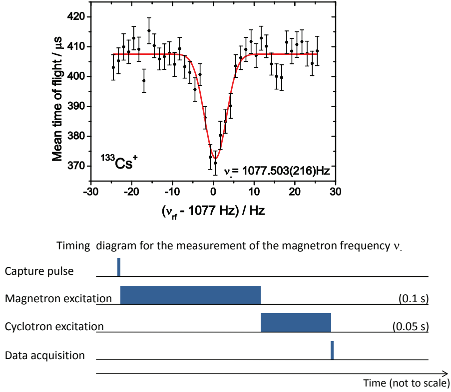
Figure 6.3: Time-of-flight spectrum (top) of the ^{133}\text{Cs}^+ magnetron frequency with an excitation time of T_{\text{rf}} = 0.1 \text{ s} . The solid line is a fit to the data points based on a Gaussian function ( \chi^2_{\text{red}} \approx 1.01 ). The excitation scheme (bottom) for the determination of the magnetron frequency contains, apart from the capture and the extraction pulse, two excitations. First, a dipolar excitation is applied with T_{\text{rf}} = 0.1 \text{ s} where \nu_{\text{rf}} is varied around the magnetron frequency \nu_- . Afterwards a quadrupolar cyclotron excitation converts the magnetron motion of the ions into a modified cyclotron motion within 0.05 s using an excitation amplitude of a_{\text{rf}} = 4.3 \text{ V}_{pp} . Therefore a full conversion is achieved. The data acquisition starts with the extraction of the ions.
