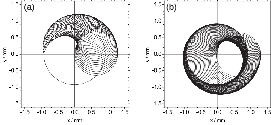
Figure 2.6: The conversion of a pure magnetron into a pure modified cyclotron motion is performed by applying a quadrupole excitation with \omega_{\text{rf}} = \omega_+ + \omega_- . a) shows the ion trajectories for the first half and b) for the second half of the conversion. The circle in a) with a radius r \approx 0.9 mm indicates the initial magnetron radius.
