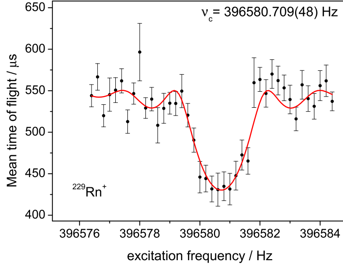
Figure 4.2: Time-of-flight spectrum of ^{229}\text{Rn}^+ with an excitation time T_{\text{rf}} = 600 ms. The half-life of ^{229}\text{Rn} was determined using the ISOLDE tape station to t_{1/2} = 12.0 \pm 1.2 s. The solid line is a fit to the theoretical line shape to the data [Kön95a].
