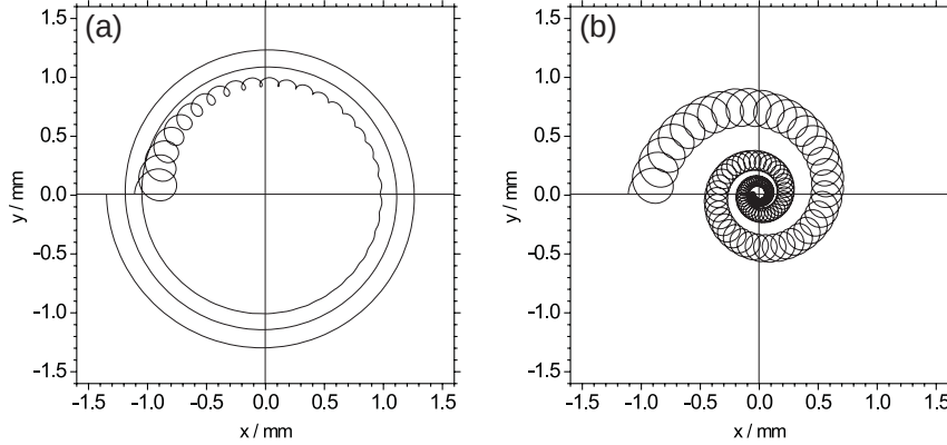
Figure 2.7: Calculated ion trajectories in a buffer gas filled trap. The buffer gas causes a velocity dependent damping force which lowers the cyclotron radius while the magnetron radius is increasing (a). Part (b) shows the effect of an additional applied azimuthal quadrupole excitation, which is responsible for centering due to the coupling of \omega_+ and \omega_- . Since \omega_+ is mass dependent the combination of buffer gas cooling and an azimuthal quadrupole excitation is mass selective.
