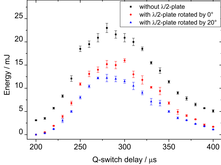
Figure 5.6: Laser energy versus Q-switch delay for different settings of the linear polarizer, which is implemented to tune the attenuation of the laser output. The linear polarizer can be rotated continuously. Examples for two rotation angles are shown in red and blue. For the present carbon cluster measurements a Q-switch delay of 355 \mu\text{s} and a rotation angle of 0^\circ was chosen.
