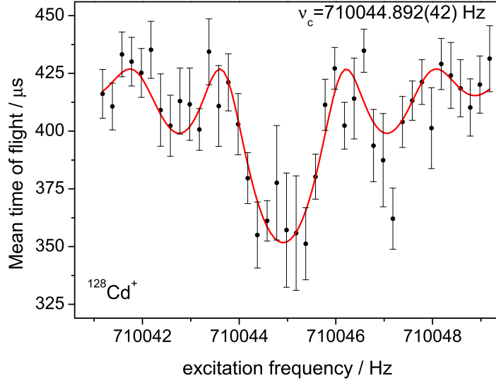
Figure 4.1: Time-of-flight spectrum of ^{128}\text{Cd}^+ with an excitation time of T_{\text{rf}} = 600 ms. ^{128}\text{Cd} is a \beta -emitter 16 neutrons away from stability with a half-life of only t_{1/2} = 280 ms. The solid line is a fit to the theoretical line shape to the data [Kön95a].
