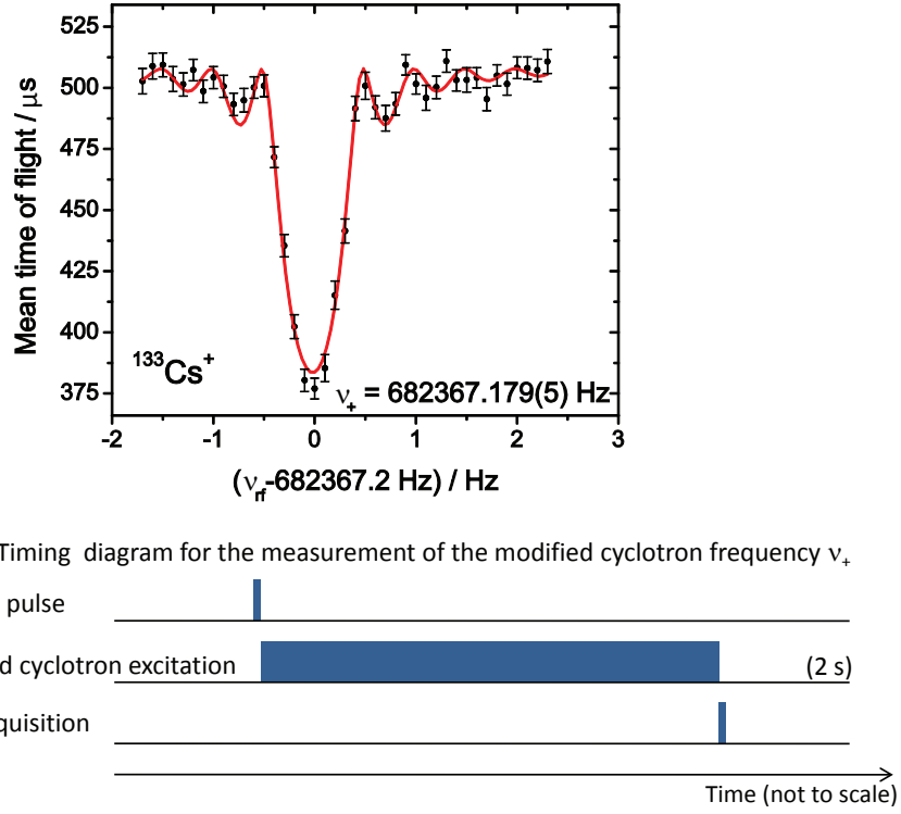
Figure 6.2: Time-of-flight spectrum (top) of the ^{133}\text{Cs}^+ modified cyclotron frequency with an excitation time of T_{rf} = 2 \text{ s} . The solid line shows a fit of the data points with \chi^2_{red} \approx 1.07 [Kön95b]. The timing diagram below (example for ^{133}\text{Cs} ) shows the capture pulse followed by a radial dipole excitation where \nu_{rf} is varied around the modified cyclotron frequency \nu_+ . Finally, the ions are extracted and the data acquisition starts simultaneously.
