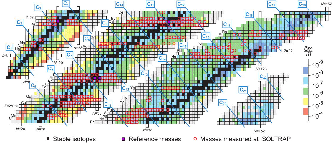
Figure 1.1: Nuclear chart with nuclides measured at ISOLTRAP (red circles), as well as the alkali reference ions (purple) and isobaric lines of carbon cluster ions [Bla05]. Further masses are shown with a color code indicating the relative precision of the mass data.
