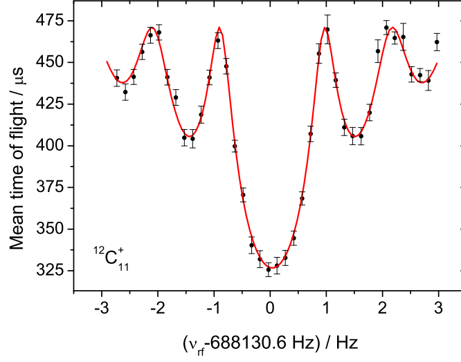
Figure 5.9: Time-of-flight ion cyclotron resonance curve for ^{12}\text{C}_{11}^+ with an excitation time of T_{\text{rf}} = 900 ms. About 3200 ions were recorded. The solid line shows a fit of the theoretical lineshape to the data [Kön95a].
