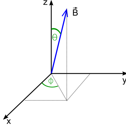
Figure 2.3: The magnetic field in an ideal Penning trap defines the z -axis. In a real Penning trap it is tilted by an angle \theta . Assuming cylindric symmetry \phi can be set to zero.
