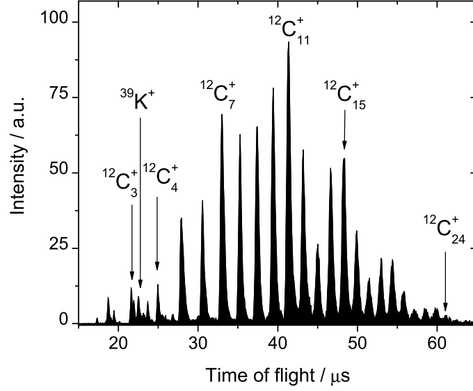
Figure 5.7: Time-of-flight spectrum of carbon cluster ions recorded in front of the preparation trap (about 2 m away from the cluster source) on an MCP detector. In this spectrum carbon cluster ions ^{12}\text{C}_n from n = 3 up to n = 24 are identified.
