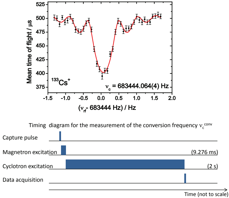
Figure 6.1: Time-of-flight spectrum for ^{133}\text{Cs}^+ (top) to determine the conversion frequency with an excitation time of T_{\text{rf}} = 2 \text{ s} . The solid line is a fit to the data points with \chi_{\text{red}}^2 \approx 1.06 [Kön95b]. At the bottom the corresponding timing diagram is presented. The capture pulse is followed by a phase-locked dipolar magnetron excitation to bring the ions on a defined radius. Afterwards a quadrupolar excitation with \nu_{\text{rf}} varied around the cyclotron frequency \nu_c is applied. Finally, the ions are extracted and the data acquisition starts simultaneously.
