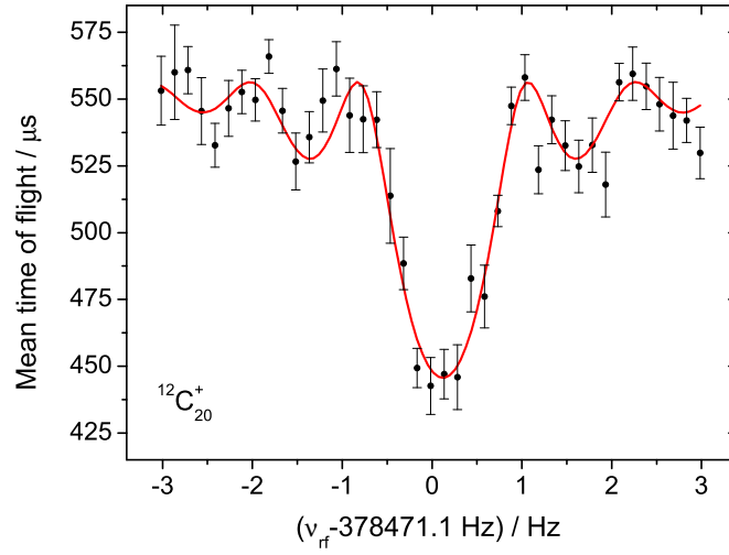
Figure 5.10: Same as in Fig. 5.9 but for the carbon cluster ^{12}\text{C}_{20}^+ . In total only 1300 ions have been recorded.
