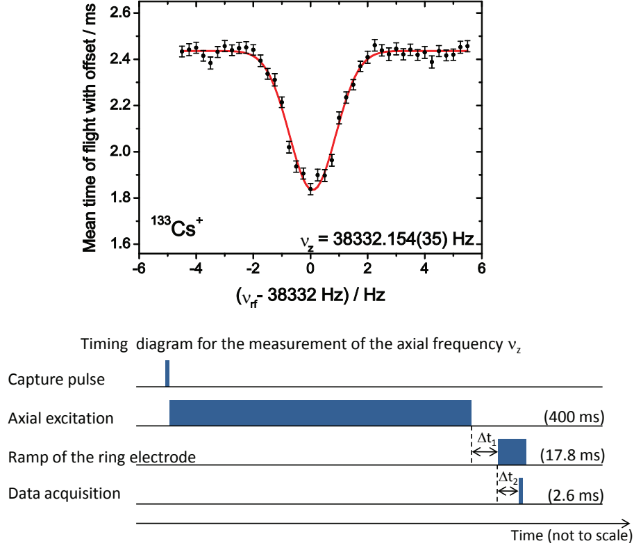
Figure 6.4: Time-of-flight spectrum (top) of the ^{133}\text{Cs}^+ axial frequency with an excitation time of T_{\text{rf}} = 400 \text{ ms} . The solid line shows a fit of the data points based on a Gaussian function ( \chi^2_{\text{red}} \approx 0.93 ). The timing diagram (bottom) shows the capture pulse followed by an axial dipole excitation with \nu_{\text{rf}} varying around \nu_z . After a delay of \Delta t_1 = 16.6 \text{ ms} a ramp potential is applied to the ring electrode in order to allow resonantly excited ions with sufficient energy to leave the trap earlier than nonresonantly excited ions. The data acquisition starts with a delay of \Delta t_2 = 12.4 \text{ ms} after the start of the ramp and takes place for 2.6 ms.
