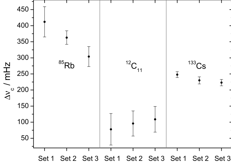
Figure 6.6: Cyclotron frequency shifts according to Eq. (6.1) for all three sets recorded for ^{85}\text{Rb} , ^{12}\text{C}_{11} and ^{133}\text{Cs} . The values are extracted from Tab. 6.2.
