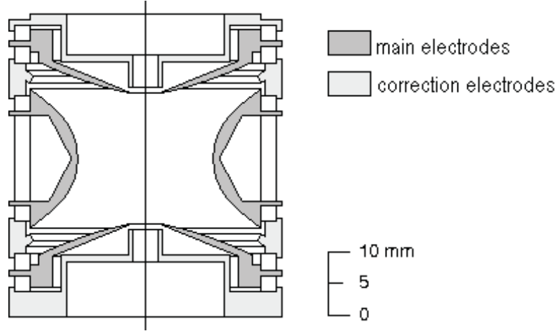
Figure 3.7: Detailed sketch of the hyperbolical precision trap. The correction electrodes are necessary to compensate the deformation of the potential due to the segmentation and boreholes in the electrodes.
