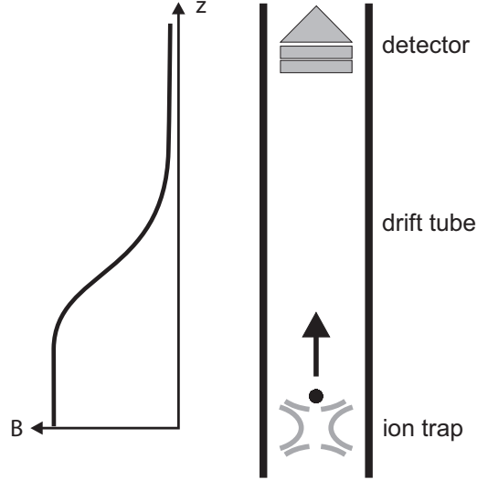
Figure 3.8: Principle of the time-of-flight ion cyclotron resonance detection technique [Grä80]. The magnetic field gradient (left) and the drift section (right) are shown.
