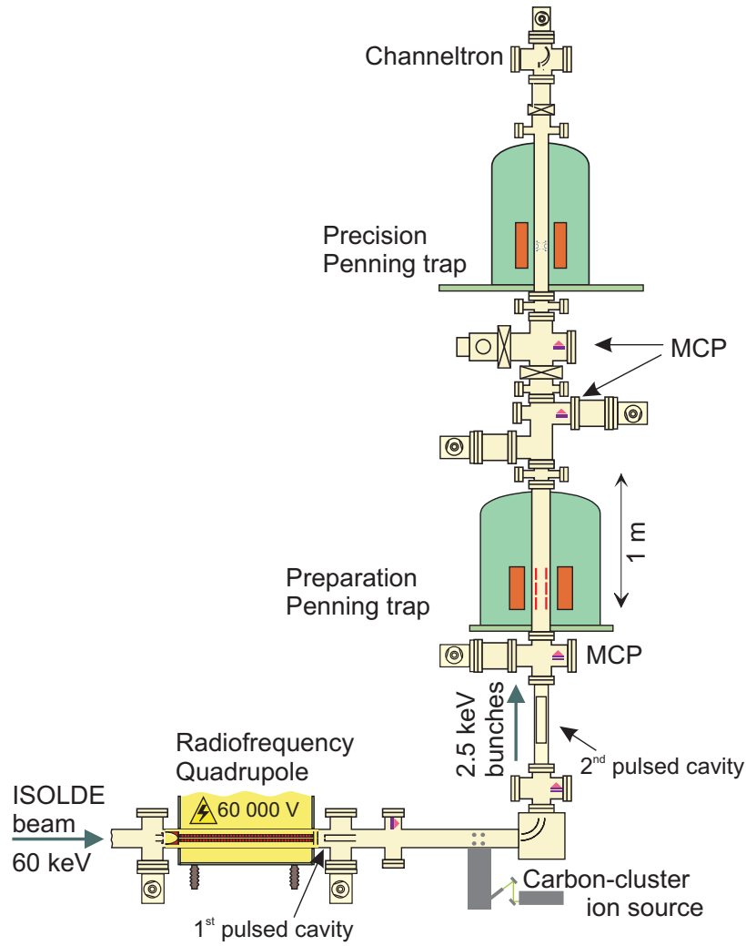
Figure 3.5: The short-lived radionuclides reach the buncher with a kinetic energy of up to 60 keV where they are accumulated, cooled and bunched. After ejection the potential energy is lowered in a pulsed drift tube down to about 2.5 keV. After a second deceleration step the ion cloud is injected into the preparation trap where contaminants are removed by a mass selective buffer gas cooling technique. Finally, they are fed into the upper trap for precision mass measurements via the determination of the cyclotron frequency employing the time-of-flight ion cyclotron resonance detection technique.
