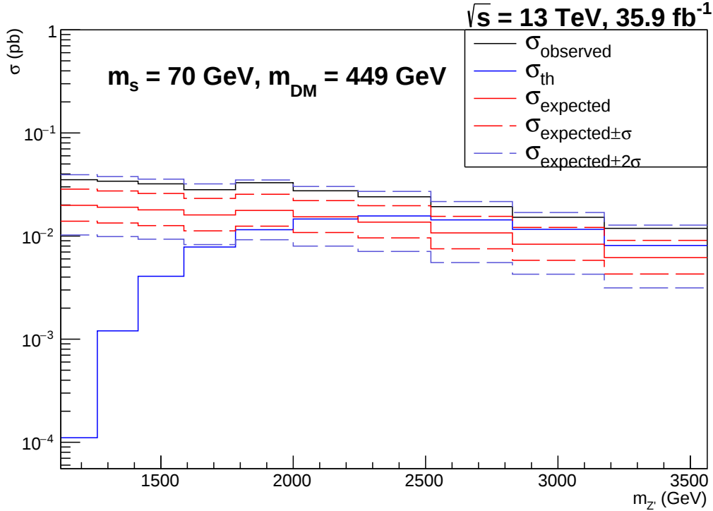
(b) m_s = 70 GeV, m_{DM} = 449 GeV, g_x < (4\pi)^{1/2} and g_q = 0.25
