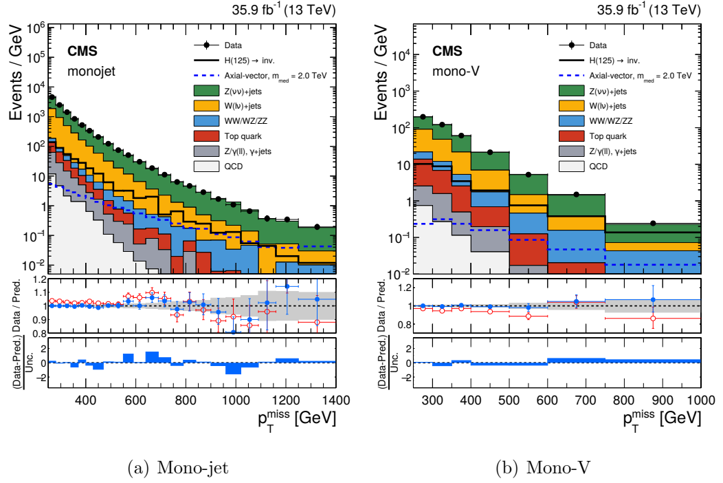
Figure 1.6: Observed MET distribution in mono-jet and mono-V signal regions with an integrated luminosity of 35.9 fb -1 . Left: the mono-jet search. Right: the mono-V search. MET > 1250 (750) GeV for the mono-jet (mono-V) search has been applied for the last bin. Two signal events are drawn here: one from 125 GeV Higgs boson decaying to invisible particles and the other from 2 TeV axial-vector mediator decaying to 1 GeV dark matter particles. Ratios of data with pre-fit background distributions (red points) and postfit expected background distributions (blue points) are performed. The gray bands refer uncertainties. The difference between data and prediction over the sum of uncertainties is also shown at the bottom. Figure taken from [24].
