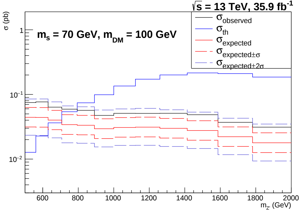
(a) m_s = 70 GeV, m_{DM} = 100 GeV, g_x < (4\pi)^{1/2} and g_q = 0.25
