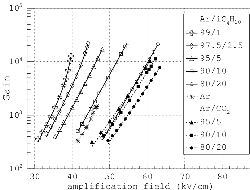
Figure 6.6: Gain and amplification field in some argon-based mixtures. The amplification gap size is equal to 86\text{ }\mu\text{m} .
