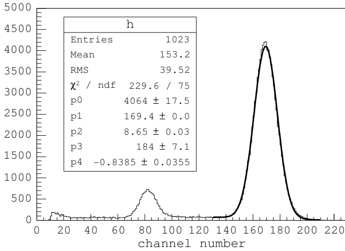
Figure 6.14: ^{55}\text{Fe} spectrum recorded in a P10 mixture. The K_\beta line was strongly absorbed by a 10\text{ }\mu\text{m} thin Cr foil. The parameters of a gaussian ( p_0 – p_2 ) and a linear ( p_3 , p_4 ) function were adjusted to the photo-peak.
