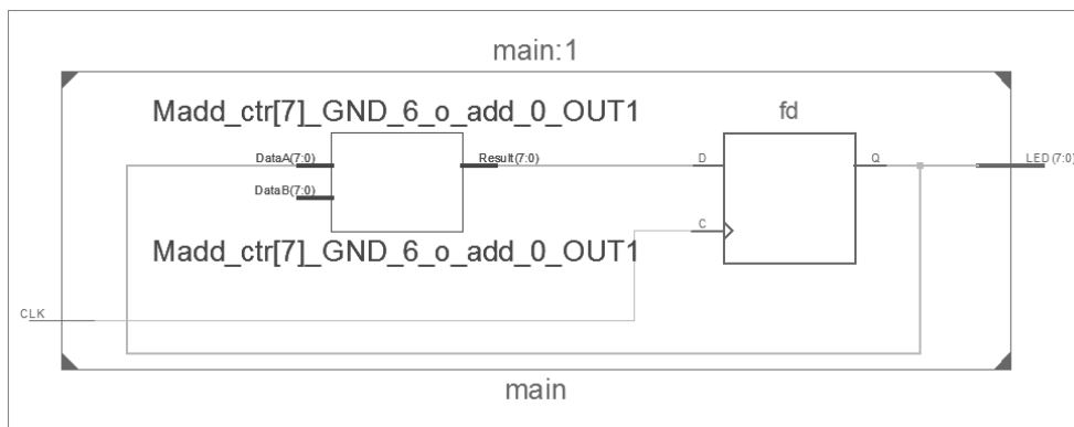
Figure 12: Netlist of a counter running on input clock CLK and presenting the output on LEDs, the code has been synthesized into an adder module and a flip flop with feedback connection.
