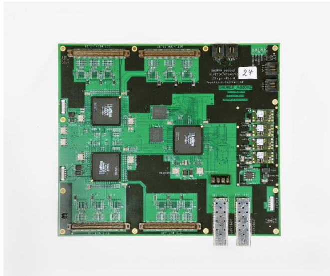
Figure 38: Photo of Shower Add-on board. Four brown connectors deliver analog signals to ADCs which are controlled and read out by the FPGAs. One central FPGA is a controller and an interface to both TrbNet and Gigabit Ethernet network, through the optical connectors.
