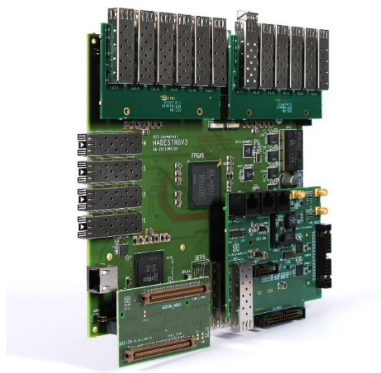
Figure 23: Photo of TRB3 equipped with different extension modules. On top there are two SFP mezzanine Add-ons plugged, down left is an ADA mezzanine Add-on and on the down right Multi-test mezzanine Add-on. [trb.gsi.de]
