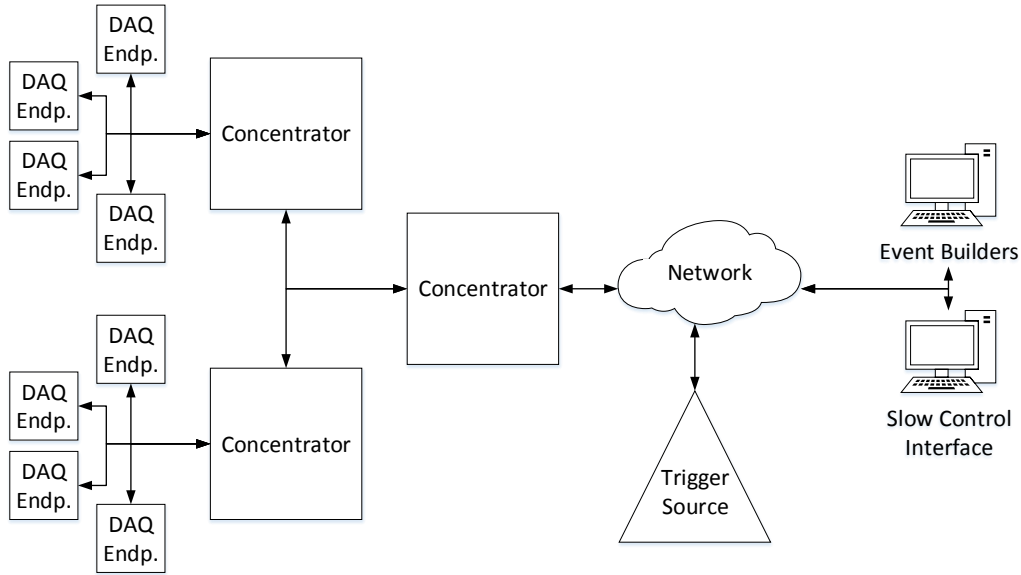
Figure 4: Scheme of the DAQ components interconnections with subsystems. DAQ Endpoints (digitizers, active FEEs, etc.) communicate through several layers of concentrators and network with Event Building machines, Slow Control computers and a Trigger System.
