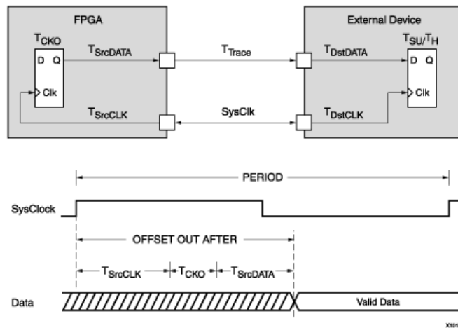
Figure 14: Visualization of timing requirements for output signals. Valid data offsets in respect of clock signal provided to an external device has to be constrained for proper operation of PAR algorithm and production of design with secured timing. [xilinx.com]
