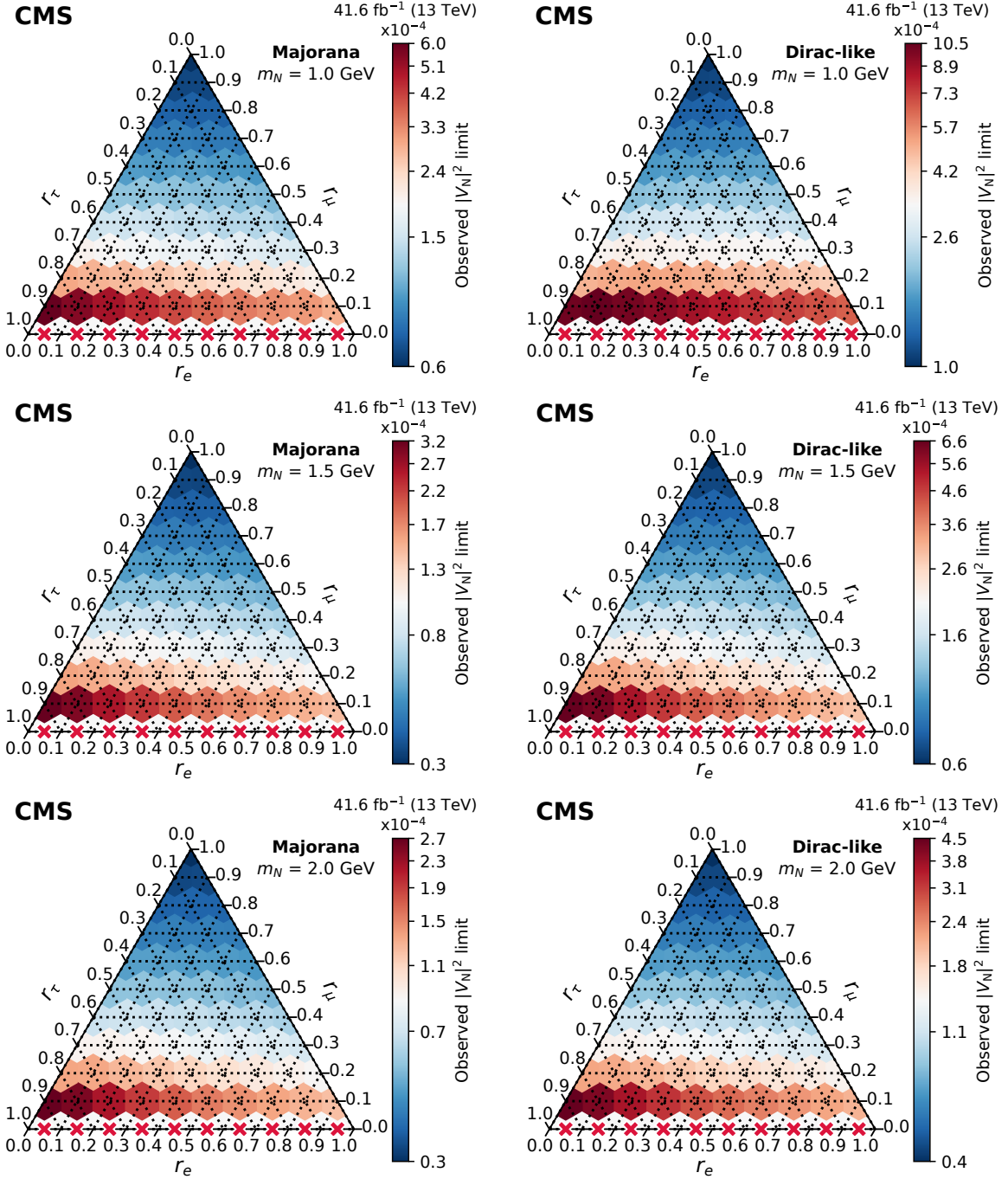
Figure 6.26: Observed 95% CL upper limits on |V_N|^2 as functions of the mixing ratios ( r_e , r_\mu , r_\tau ) for fixed HNL masses of 1 GeV ( upper ), 1.5 GeV ( middle ), and 2 GeV ( lower ), in the Majorana ( left ) and Dirac-like ( right ) scenarios. The range of values on the z -axis is not kept fixed across the different plots. The red crosses indicate that there is no exclusion for that point. The orientation of the value markers on each axis indicates the direction of reading.
