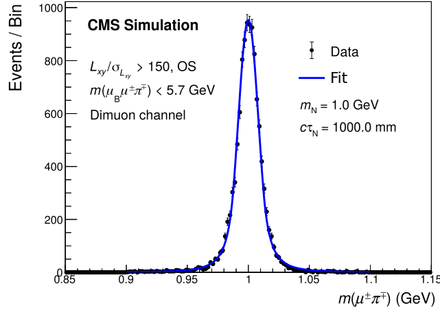
Figure 6.18: Distribution of m(\ell^\pm \pi^\mp) for simulated events with m_N = 1 GeV and c\tau_N = 1000 mm in the high L_{xy}/\sigma_{L_{xy}} , OS, and low m(\ell_B \ell^\pm \pi^\mp) category in the dimuon channel. The blue curve corresponds to the fit to the data using a double-sided Crystal Ball function.
