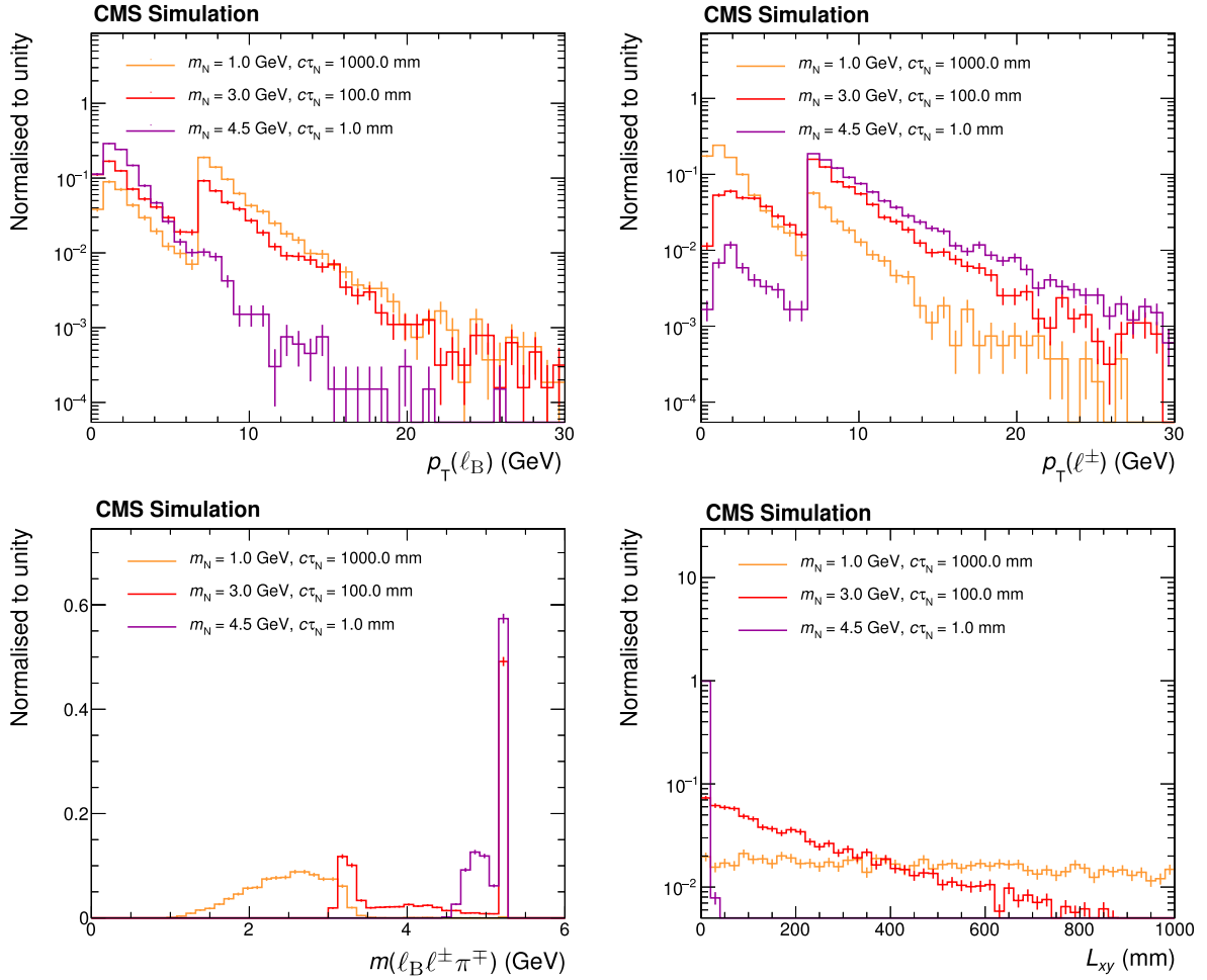
Figure 6.7: Distribution of the primary lepton p_T (upper left), displaced lepton p_T (upper right), invariant mass of the \ell_B^\pm \pi^\mp system (lower left), and L_{xy} of the DV (lower right). The distributions are shown for generator-level events from the ( B_u , B_d , B_s ) samples simulated with (i) m_N = 1 GeV, c\tau_N = 1000 mm, (ii) m_N = 3 GeV, c\tau_N = 100 mm, and (iii) m_N = 4.5 GeV, c\tau_N = 1 mm. No corrections are applied on the simulated events. The distributions are normalised to unit area.
