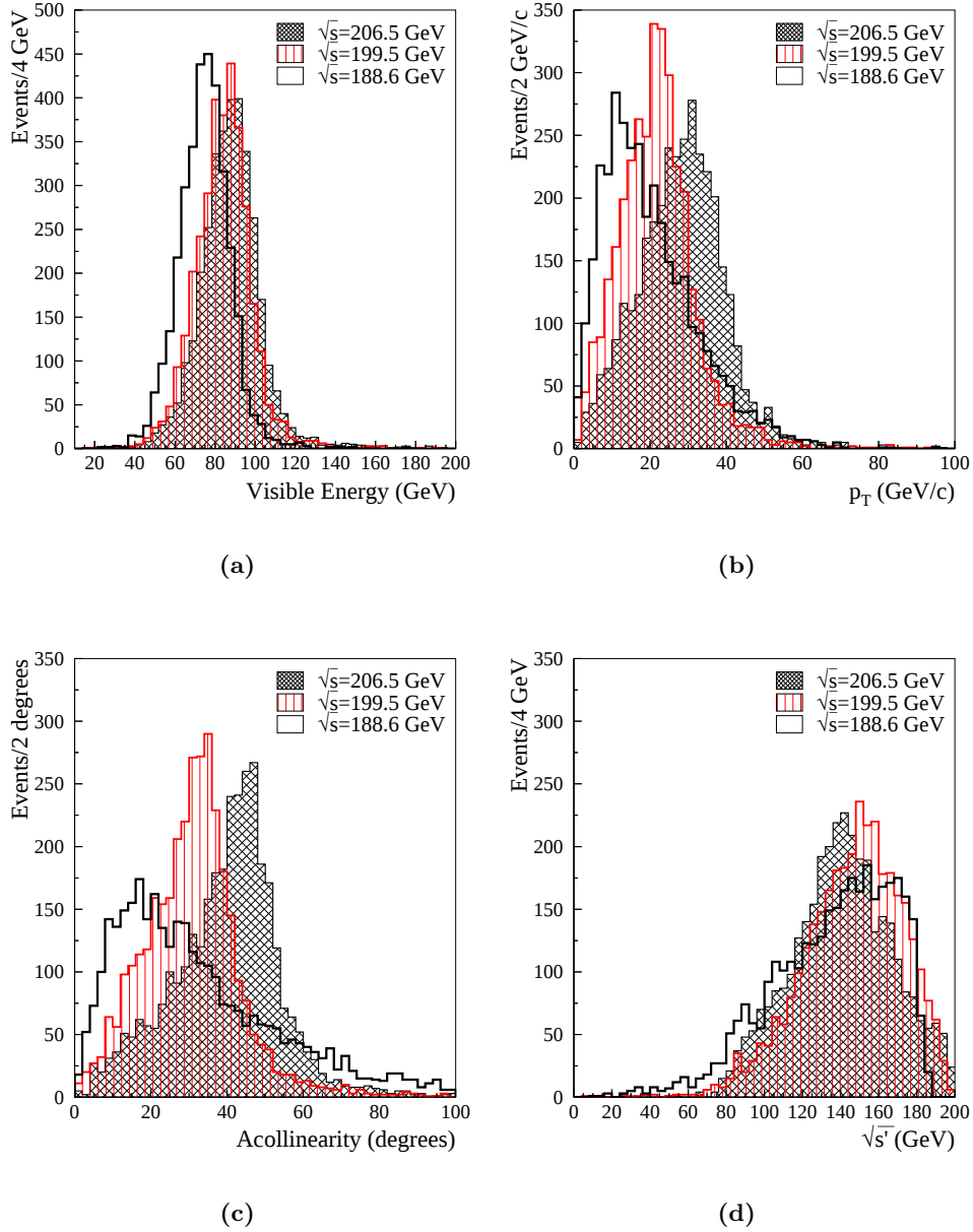
Figure 6.3: The \sqrt{s} dependence of the event signatures for m_H = 100 GeV/ c^2 for three different centre-of-mass energies: 206.5 GeV (hatched), 199.5 GeV (lines) and 188.6 GeV (white). The distributions shown are the same as in Fig. 6.2.
