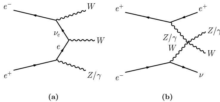
Figure 8.13: Two Feynman graphs contributing to electroweak six-fermion production at LEP: The three boson production (a) and the vector boson scattering (b).
