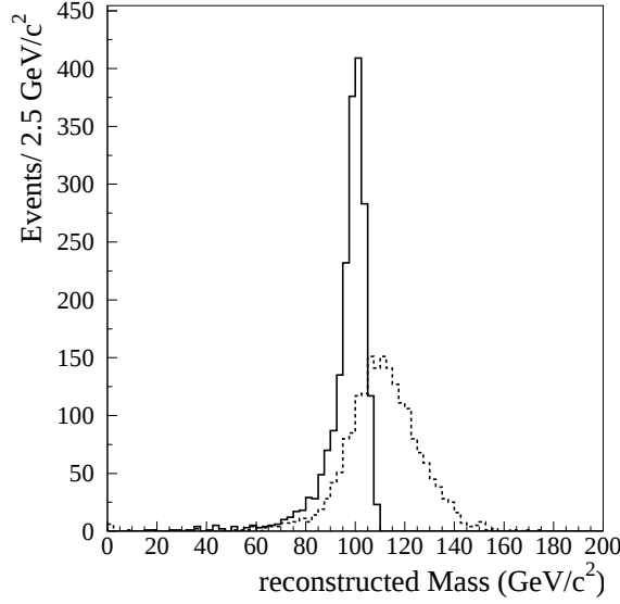
Figure 6.8: The mass of the invisible Higgs boson (dotted line) and the constrained mass of the invisible Higgs boson (continuous line). The constrained mass gives a greatly improved mass resolution for the case of invisibly decaying Higgs boson with a mass of 100 \text{GeV}/c^2 .
