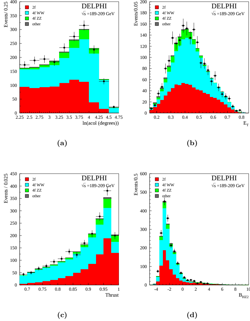
Figure C.2: Distributions for some of the preselection variables of the medium mass analyses as described in chapter 7.4.2: (a) \ln(\text{acollinearity}) (b) E_T/\sqrt{s} (c) Thrust (d) B-Tagging B_{HZ2} .
