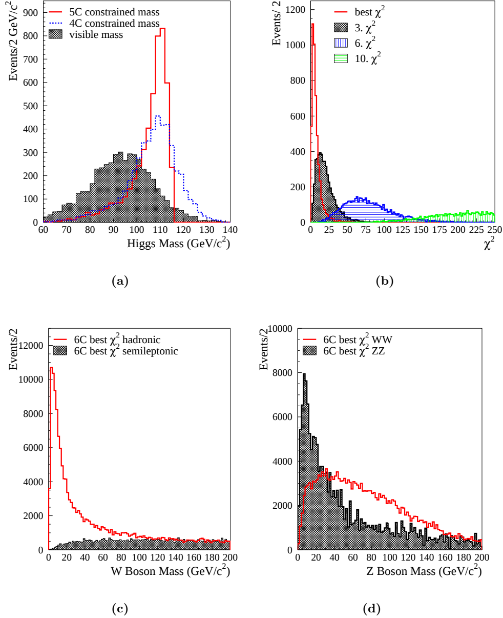
Figure 8.3: Mass reconstruction using PUFIT. First, the reconstructed mass for a Higgs boson of 110 \text{GeV}/c^2 mass decaying into WW^* using the paring with the best \chi^2 is shown in (a). Plotted are the raw visible mass, the visible mass after a 4C fit and the visible mass after the 5C fit. In (b) four of the 15 \chi^2 values for the 5C fit with 6 jets are shown. Second, the reconstructed masses of W and Z pairs after a 6C fit with 4 jets are shown. Plotted in (c) is the best \chi^2 for the WW \rightarrow 4 jets hypothesis, both for the fully hadronic and semileptonic decays after a 6 C fit assuming the W mass for the two di-jet pairs. In (d), the same is shown for fully hadronic Z and W bosons after a 6 C fit assuming the Z mass for the two di-jet pairs.
