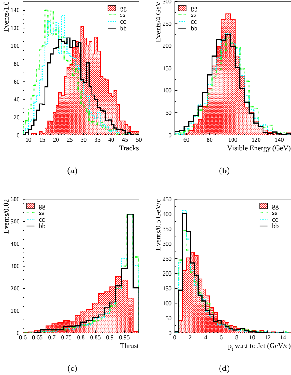
Figure 7.2: The decay flavour dependence of the event signatures for m_H=100 GeV/ c^2 at a centre-of-mass energy of 206.5 GeV for the four different flavours: gluons (hatched), strange quarks (light grey dashed line), charm quarks (light grey dotted line) and bottom quarks (black solid line). Shown are the charged multiplicity (a), the visible energy (b), the thrust of the event (c) and the largest transverse momentum of a particle with respect to the jet axis (d).
