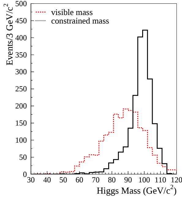
Figure 7.5: The mass reconstruction for a hadronic Higgs decay with m_H=100 \text{GeV}/c^2 using only the visible mass (hatched line) or the constrained mass (solid line).
