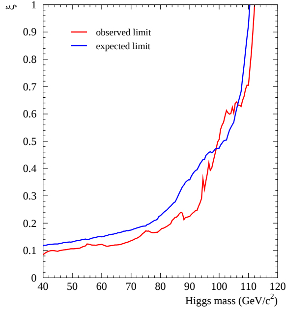
Figure 6.14: The 95% CL upper limit on the \xi factor in e^+e^- \rightarrow HZ ( H \rightarrow invisible)( Z \rightarrow anything) as a function of the Higgs boson mass. The region above the line for an observed limit is excluded.
