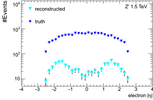
(c) Electron \eta
