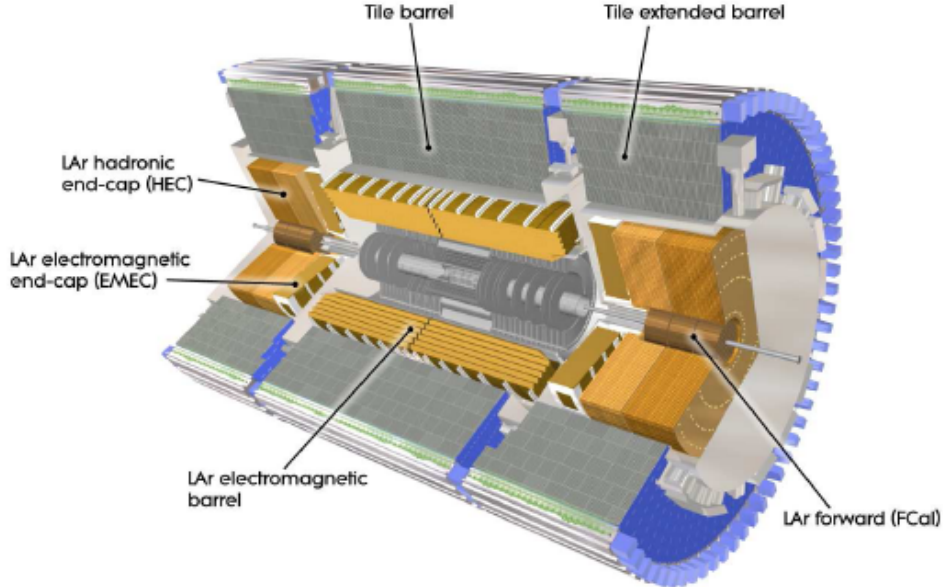
Figure 4.7: The ATLAS calorimeter system [23]
