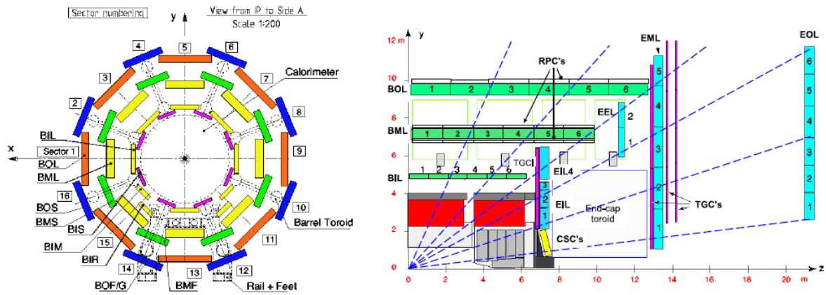
Figure 7.2: Left: Cross-section of the barrel part of the MS in the transverse plane[23], with three concentric cylindrical layers with eight large and eight small chambers. Right: Cross-section of the muon system in the longitudinal plane[23].
