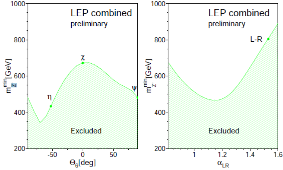
Figure 2.3: The 95% confidence limits on M'_{Z'} as a function of the model parameter \theta_{E_6} for the E_6 models and \alpha_{LR} for the LRM[18].
