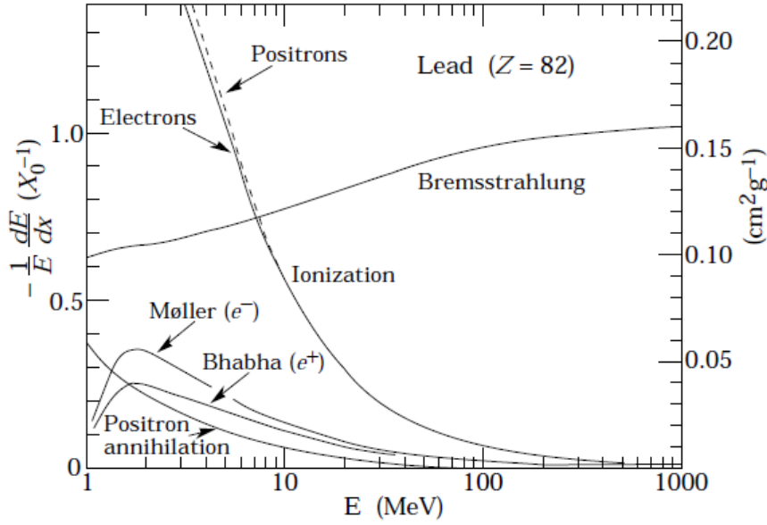
Figure 3.2: The fraction of the energy loss per radiation length in lead as a function of the electron (positron) energy[2]. A radiation length is the mean distance over which an electron (positron) travels before it is left with only 1/e of its starting energy.
