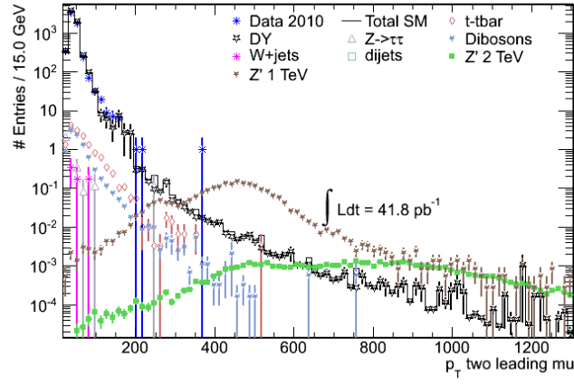
(c) Muon p_T . The SM background is divided into its constituents and two Z' s are shown (1.0 and 2.0 TeV).
