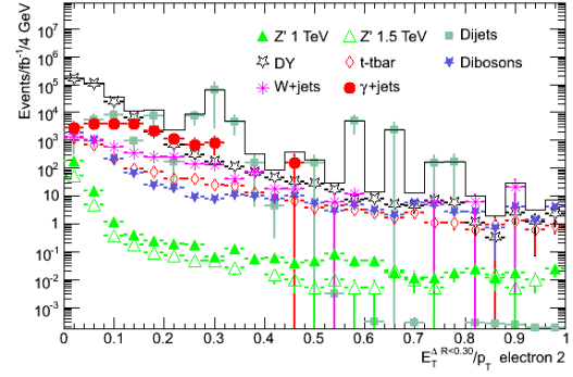
(b) E_T\text{-cone30}/p_T - electron 2
