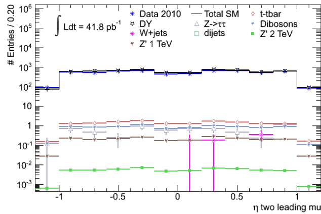
(d) Muon \eta . The SM background is divided into its constituents and two Z' s are shown (1.0 and 2.0 TeV).
