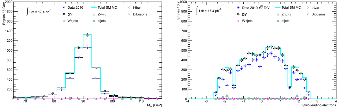
(a) Dielectron invariant mass M_{ee}
