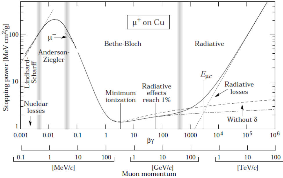
Figure 3.1: The Bethe-Bloch formula for positive muons in copper as a function of \beta\gamma [2] (shown between the second and third grey band. The rest is described by other models.)
