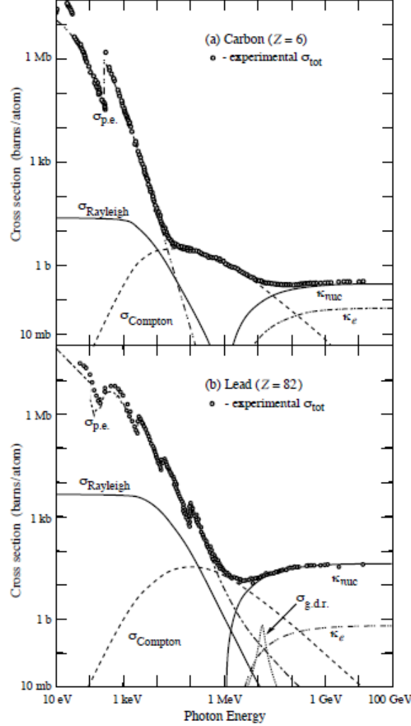
Figure 3.3: Photon total cross-sections as a function of the photon energy. [2] “p.e” stands for “photoelectric effect”, “nuc” means pair production in nuclear field and “e” pair production in electron field.
