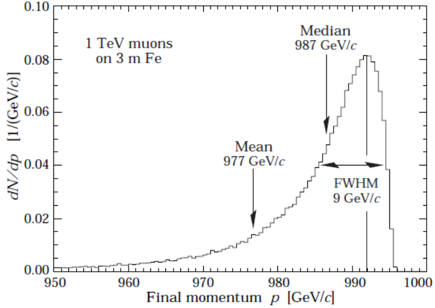
Figure 3.5: The momentum distribution of 1 TeV muons after passing through 3 meters of iron [2].
