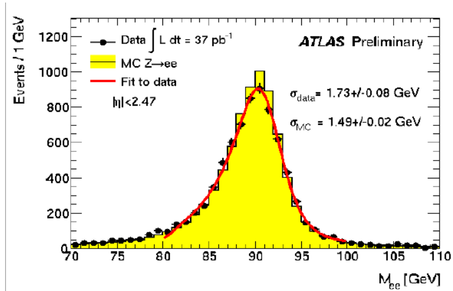
Figure C.5: The dielectron invariant mass distribution is fitted with a convolution of a Breit-Wigner convoluted with a Crystal Ball[41]. The obtained resolution ( \sigma of the Crystal Ball) is 1.73 \pm 0.08 . 36.6 \text{ pb}^{-1} of data is used. Electrons are required to be identified as medium, have E_T > 20 \text{ GeV} and |\eta| < 2.47 (excluding the crack 1.37 < |\eta| < 1.52 ). Dielectrons with opposite sign and invariant mass between 80 GeV and 100 GeV are used in the fit.
