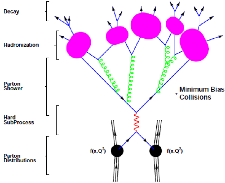
Figure 5.8: Schematic view of the Parton Shower technique[30], showing (from bottom up) the hard collision of two partons, the parton shower followed by hadronization, and finally decay of the colorless hadrons.
