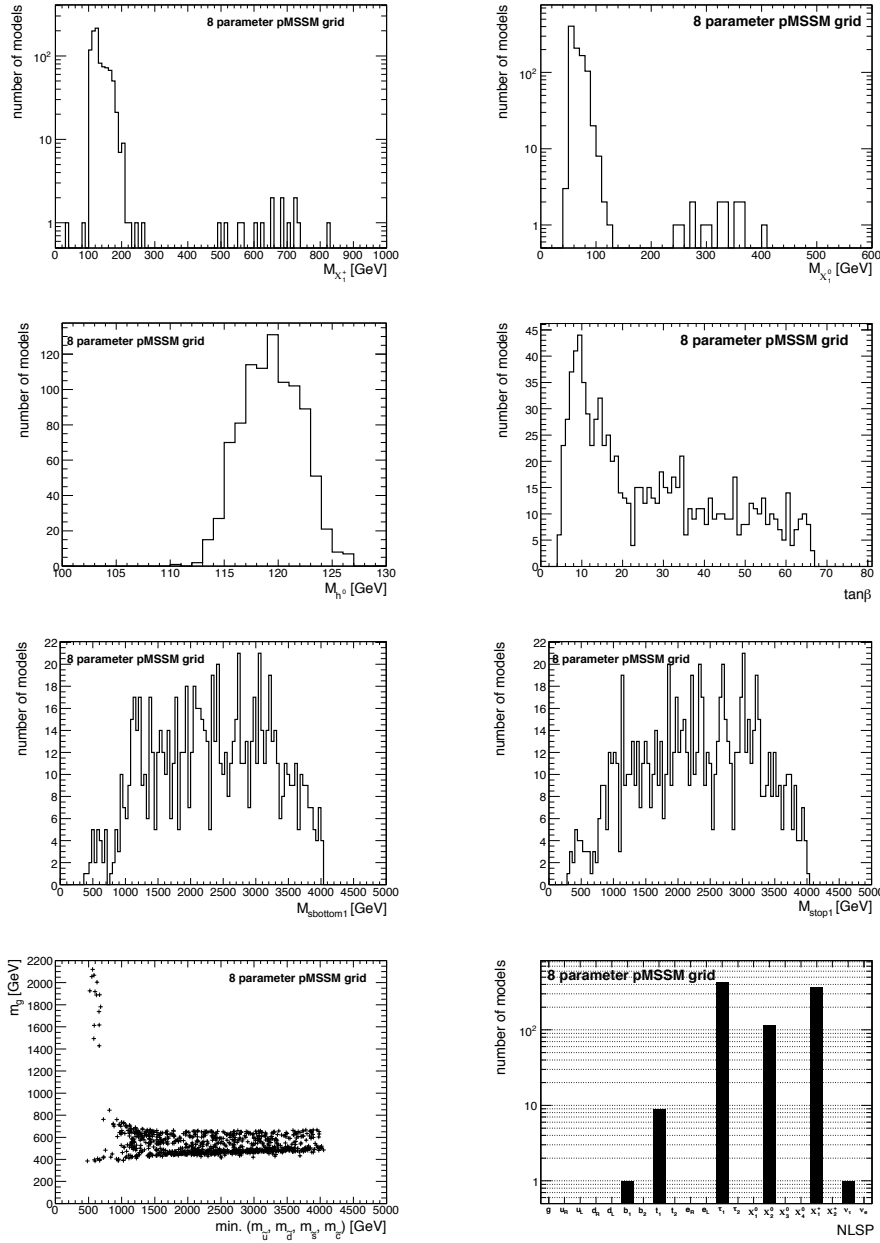
Figure 4.9: Parameters of the 8 parameter pMSSM grid. The mass of the chargino \chi_1^\pm (top left plot), the mass of the neutralino \chi_1^0 (top right plot), the mass of the lightest higgs (2nd row left plot), the distribution of \tan\beta (2nd row right plot), the mass of the lightest sbottom (3rd row left plot), the mass of the lightest stop (3rd row right plot), the distribution gluino versus minimal mass of the 1st and 2nd family squarks (bottom left plot) and next LSP type (NLSP) for the selected SUSY models (bottom right plot).
