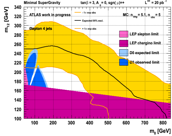
Figure 13.5: Expected 95% C.L. ATLAS exclusion limit for the 4 jet 0-lepton SUSY analysis in the mSUGRA \tan\beta = 3 , A_0 = 0 and \text{sgn}(\mu) > 0 parameter space assuming \mathcal{L} = 20 \text{ pb}^{-1} . Figure is taken from Ref. [364].
