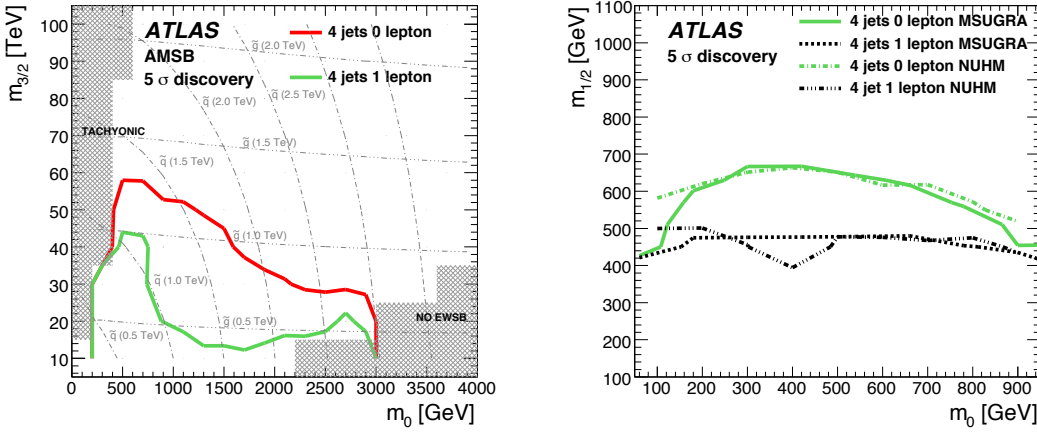
Figure 8.8: Discovery potential for the 4 jet 0 and 1-lepton channel in the AMSB (left plot) and NUHM (right plot) parameter space. The horizontal and curved grey lines indicate the gluino and squark masses respectively in steps of 500 GeV.
