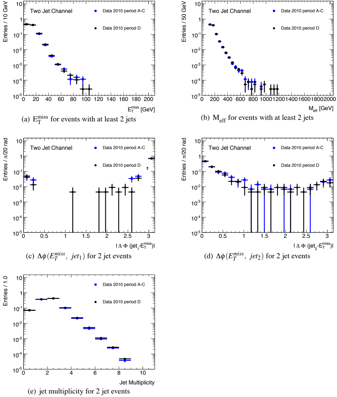
Figure E.12: Pile up studies for collision events of \mathcal{L} = 70 \text{ nb}^{-1} . E_T^{\text{miss}} (top left plot, figure (a)), effective mass before E_T^{\text{miss}} selection (top right plot, figure (b)), \Delta\phi(E_T^{\text{miss}}, \text{jet}_{1,2}) distributions after the E_T^{\text{miss}} > 40 \text{ GeV} selection (2nd row, figure (c) and figure (d)) for 2 jet 0-lepton events. The bottom plot (figure (e)) shows the jet multiplicity for jets with p_T > 20 \text{ GeV} and |\eta| < 2.5 . Events of high (black line) and low (blue line) pile-up runs are compared.
