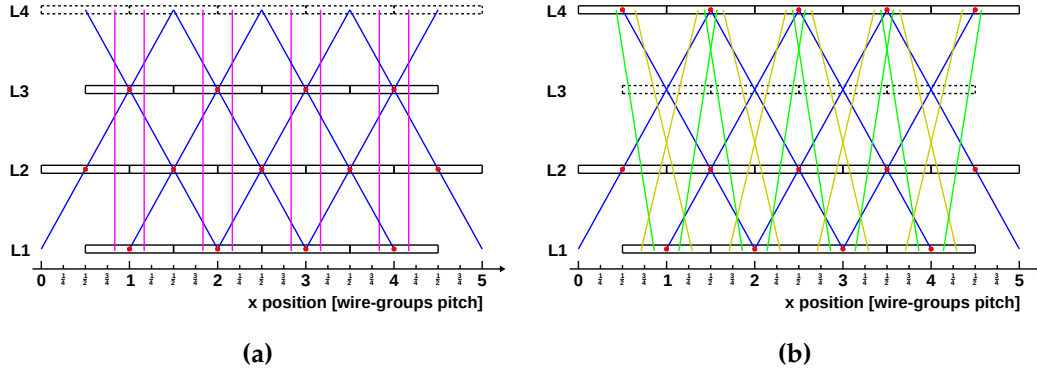
Figure D.3: Sketch of the possible x positions of a reference track reconstructed with wire hits in the x - z plane on the tested layer of a sTGC built with half staggering of the wire groups and equal distance between detector planes. The special cases for an (a) outer tested layer (layer 4) and (b) inner tested layer (layer 3) are shown. The wire groups are identified by rectangles. The wire groups of the tested layer have dotted lines. The position of the reconstructed wire space points is marked by a red dot in the middle of the wire groups. The tracks are displayed using lines of different colours. Each colour is associated with a different value of the x - z track polar angle |\theta_{xz}| .
