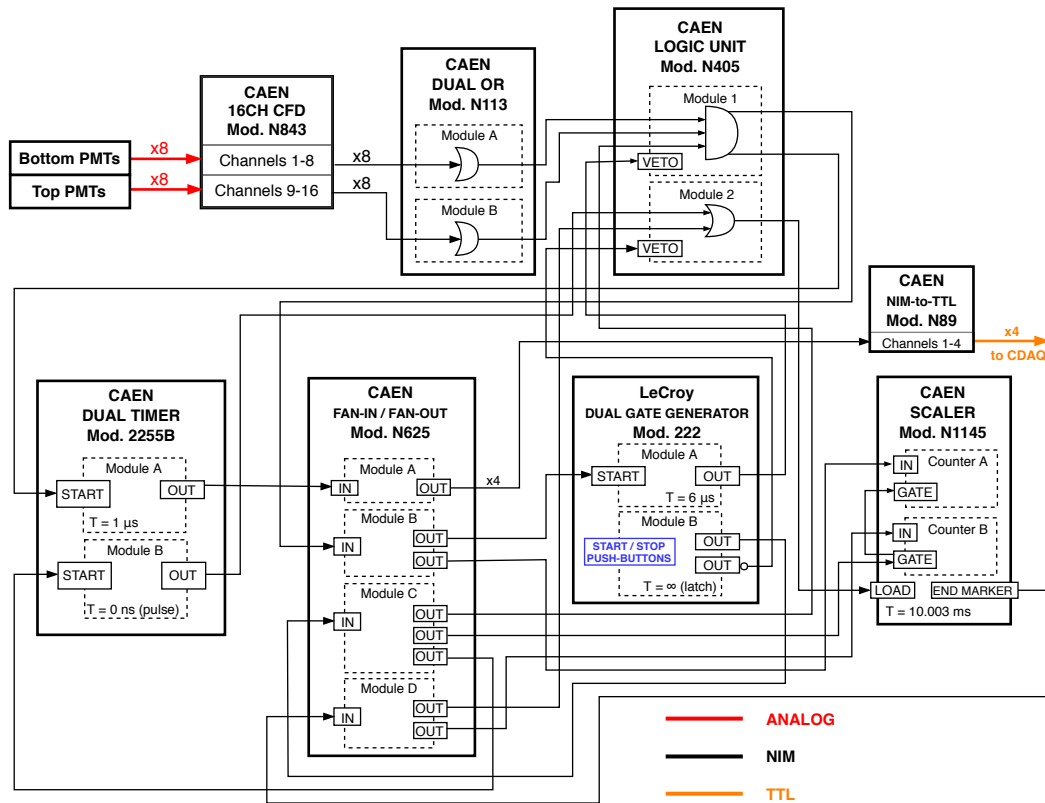
Figure 6.2: Block diagram of the cosmic-ray hodoscope trigger system. The bold rectangles indicate individual NIM modules. The arrows indicate the direction of the signal. The colour of the arrows is associated with the logic levels of the signal lines. The CAEN N89 NIM-to-TTL module is used only for the CDAQ prototype boards which require TTL levels. More than 4 independent trigger lines can be used if additional fan-out modules are daisy-chained to the first one.
