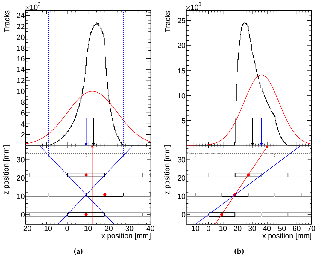
Figure C.1: Results of the wire track extrapolation simulation for the two track types considered.
