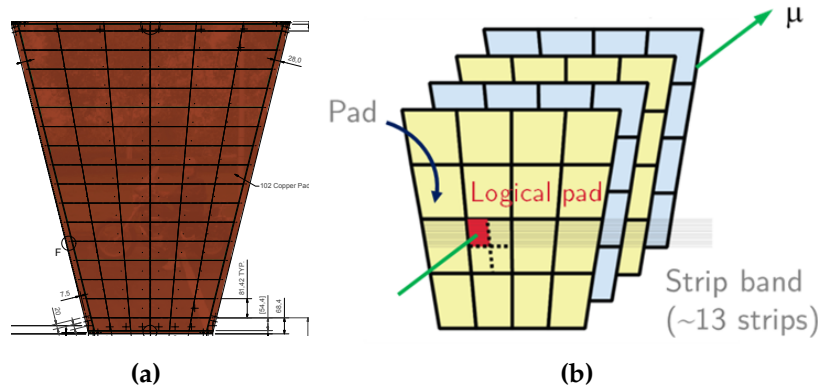
Figure 3.10: (a) Physical readout pads geometry of layer 1 of the QL1 pivot quadruplet [99] and (b) schematic of the readout pads staggering between different sTGC layers of a quadruplet [97]. The area corresponding to a logical pad on a detector plane is approximately four times smaller than the area of a physical pad.
