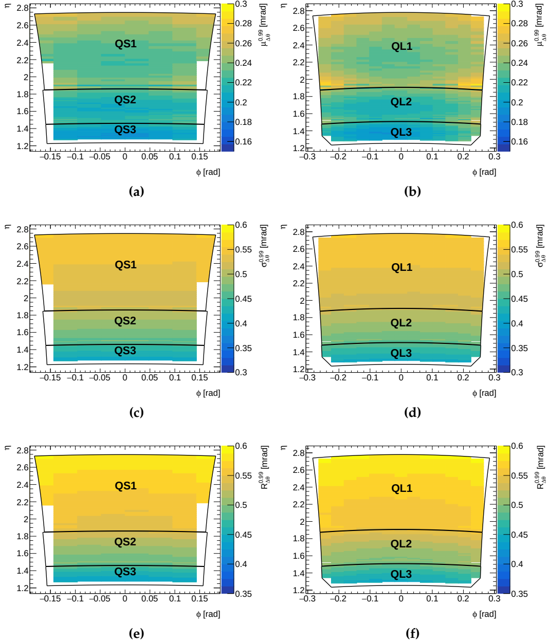
Figure 4.7: Values of (a)-(b) \mu_{\Delta\theta}^{0.99} , (c)-(d) \sigma_{\Delta\theta}^{0.99} and (e)-(f) R_{\Delta\theta}^{0.99} as a function of the logical pad. Values for the small sector are shown in (a)-(c)-(e) and for the large sector in (b)-(d)-(f). The black overline highlights the limits of the sector first layer when projected in the \eta - \phi space. The orientation of the quadruplets in the \eta - \phi space is inverted with respect to the orientation in the x - y space shown in Fig. 4.2.
