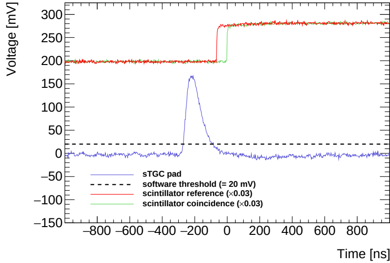
Figure 5.19: Oscilloscope segment of a representative pad analog signal from a cosmic-ray muon amplified and shaped by the VMM3 ASIC. The scintillator detector reference and coincidence signals are digital TTL logic pulses. The digital pulses are scaled by a factor \times 0.03 and offset on the voltage scale for display purposes. The origin of the time axis is the leading edge of the scintillator detector coincidence pulse, which triggers the oscilloscope. The sTGC pulse time measurement is taken as the time when the pulse leading edge crosses the offline software threshold. The reference scintillator detector time measurement is taken as the leading edge of the scintillator detector discriminated pulse (red line).
