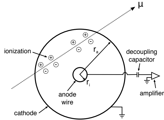
Figure 2.8: Cross-section schematic of a cylindrical ionization detector.
