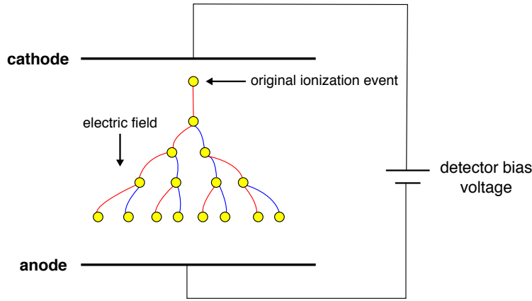
Figure 2.6: Schematic diagram of a Townsend avalanche. A strong electric field permeates the gaseous medium between the anode and the cathode. The yellow disks represent ionization events caused by an incident electron (red lines). Freed electrons (blue lines) produce more ionization events as they drift in the electric field. The total ionization approximately doubles at each step of the avalanche.
