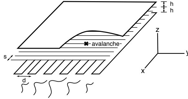
Figure 2.12: Schematic of a multiwire chamber with a segmented cathode. The cross highlights the avalanche position on one of the anode wires. The signal induction on each cathode strip is sketched [57].
