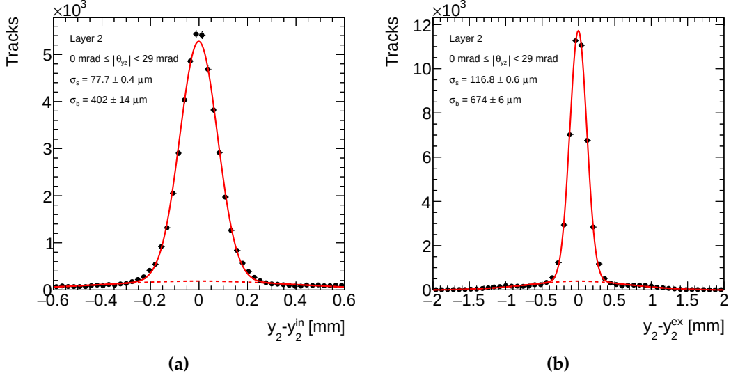
Figure 5.9: Distributions of reference track y -residuals on layer 2 for the (a) inclusive and (b) exclusive cases. The double Gaussian function fitted to the data is drawn on the distributions as a continuous red line. The background term of the fit function is drawn with a dashed line. The signal term accounts for about A_s/(A_s + A_b) = 85\% of the events for both distributions. The signal fraction is approximately constant as a function of the reference track angle.
