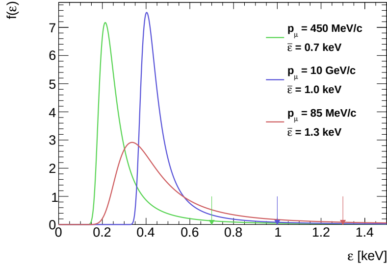
Figure 2.2: Fluctuations of energy loss predicted by Landau's theory for muons traversing a sTGC gas volume. The arrows indicate the mean energy loss \bar{\epsilon} obtained by the Bethe-Bloch formula.
