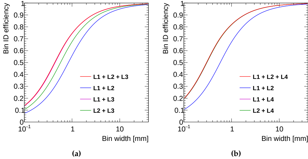
Figure D.2: Calculated BIDA values for (a) an outer tested layer (layer 4) and (b) an inner tested layer (layer 3) based on the parameters of the double Gaussian function fitted to the exclusively reconstructed track y -residual distributions shown in Fig. D.1. The layers used for the exclusive track reconstruction are indicated in the legend. The purple and red line coincide for the outer layer case (a). The red, purple and green curves coincidence for the inner layer case (b).
