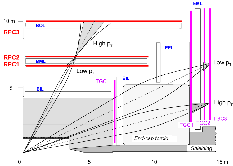
Figure 3.5: Schematic diagram of the TGC and RPC modules shown on a quadrant cross-section of the ATLAS muon spectrometer in the z - r plane.
