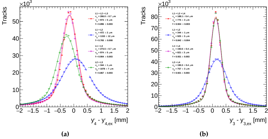
Figure D.1: Exclusive y -residual distributions for (a) an outer tested layer (layer 4) and for (b) an inner tested layer (layer 3). The full red markers denote the track y -residuals from a track reconstructed with all 3 exclusive layers. The other markers indicate tracks reconstructed with only 2 exclusive layers. The distributions have the same normalization. The distributions are fitted to a double Gaussian function. The width of the signal ( \sigma_s ) and background ( \sigma_b ) Gaussians and the signal fraction f are shown.
