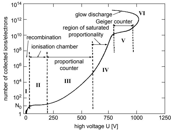
Figure 2.7: Ionization yield as a function of voltage for a typical ionization detector following the passage of a mip with a primary ionization N_0 \sim 10 [32].
