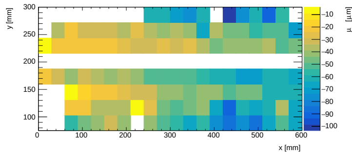
Figure 6.8: Value of the mean obtained from the fitted double Gaussian function to the exclusive y -residual distribution for layer 4 of the 40 \times 60 \text{ cm}^2 sTGC prototype.
