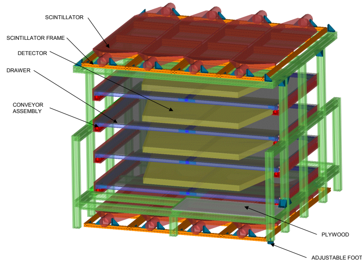
Figure 6.1: Schematic of the cosmic-ray hodoscope. The extruded aluminum parts are coloured green and orange. The assemblies of scintillators, waveguides and PMTs are coloured red and are located over and under the structure. The flat trapezoid sTGC modules are coloured olive and are located over the blue drawers where they are partially seen.
