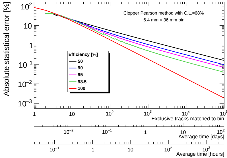
Figure 6.6: Absolute statistical error on the hit efficiency measurement obtained using the Clopper Pearson method with a confidence interval of 68% for different measured hit efficiencies. The calculated error is the maximum deviation from the measured efficiency within a confidence interval width of 68%. The corresponding average data taking time is indicated assuming bins of dimensions 6.4 \times 36 \text{ mm}^2 and the reference track density of a typical cosmic-ray run using the 40 \times 60 \text{ cm}^2 prototype sTGC.
