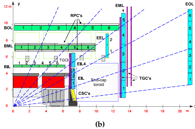
Figure 3.4: Projection of the current ATLAS muon detector system [3] (a) on the x - y plane and (b) on the y - z plane. The muon stations and module size are denoted using 3-letter acronyms. The first letter indicates a Barrel (B) or End-cap (E) station. The second letter indicates the position of the station relative to the interaction point. Four layers of stations are defined: Inner (I), Middle (M), Outer (O) and transition end-cap (E). Finally, the third letter indicates the module size typically named Small (S) or Large (L). End-cap small modules are not seen in the y - z projection because they are located at a different \phi position. Special modules are positioned around the support structures, or “feet”, of the muon spectrometer to minimize the loss of coverage in these regions. The special modules are denoted with the letters M, R, F or G depending on their exact dimensions and location.
