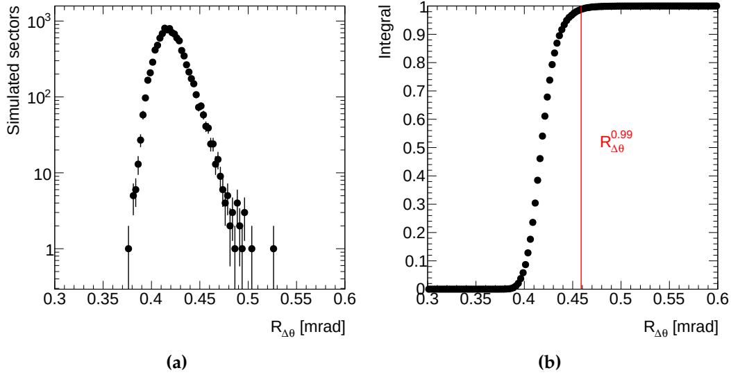
Figure 4.6: (a) Distribution of R_{\Delta\theta} values for one logical pad after simulating 10^4 small sectors and (b) the same distribution, but integrated and normalized with the value at which the integral is above 99%, R_{\Delta\theta}^{0.99} , highlighted.
