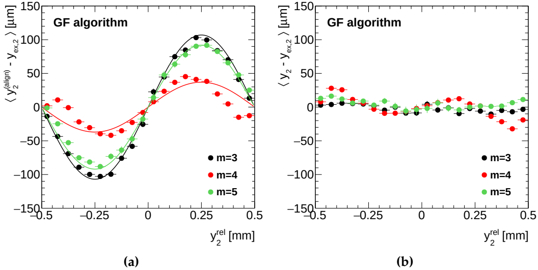
Figure 5.8: Mean of the layer 2 y -residuals as a function of y_2^{\text{rel}} for different cluster strip multiplicities m (a) without and (b) with the differential non-linearity correction applied on the space points of layer 2. The exclusively reconstructed reference track space points are corrected for differential non-linearity effects in (a) and (b). The space points of all layers are corrected for inter-layer misalignments. The differential non-linearity corrections obtained at convergence of the iterative procedure are drawn as continuous lines in (a).
