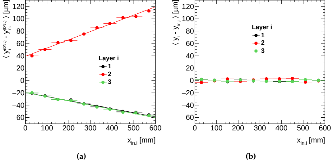
Figure 5.7: Mean of the inclusive reference track y -residuals for each tested layer i as a function of the reference track x -coordinate on the layer (a) without and (b) with inter-layer misalignments correction. The differential non-linearity corrections are applied in both cases to all space points. The non-corrected y -residuals are fitted to a first order polynomial.
