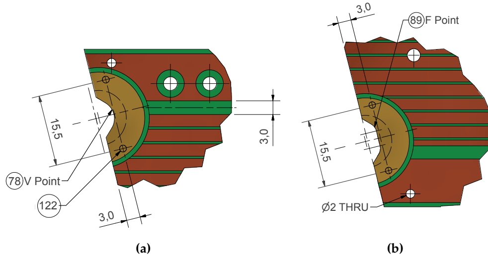
Figure 4.4: Drawing of the strip-board brass inserts as seen in the QL1 quadruplet technical drawings [99]. Units are millimetres. The brass inserts can be either of (a) triangular or (b) trapezoidal type. One brass insert of each type is crimped on one of the angled sides of the strip-boards. The triangular brass insert is located on the long-base side and the trapezoid brass insert on the short-base side.
