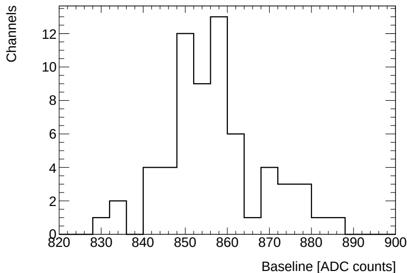
Figure 5.4: Baseline value distribution for the 64 channels of a representative VMM1 ASIC.
