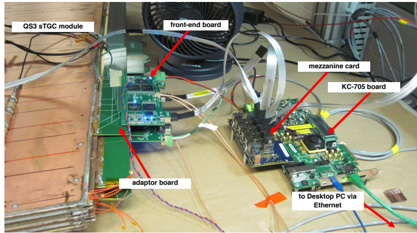
Figure 5.17: Picture of the VMM3 DAQ system used for the pad time jitter measurement. The KC-705 board communicates with a desktop computer via Ethernet for the configuration and control of the DAQ system. The mezzanine card provides the necessary connectivity between the front-end board and the KC-705 board. The adaptor board is soldered to the QS3 sTGC module and provides the connectivity between the front-end board and the sTGC pad readout channel under test.
