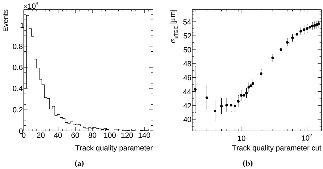
Figure 5.12: (a) Distribution of the track quality parameter for reconstructed tracks from the pixel telescope. (b) Measured spatial resolution as a function of the cut on the pixel telescope track quality parameter.
