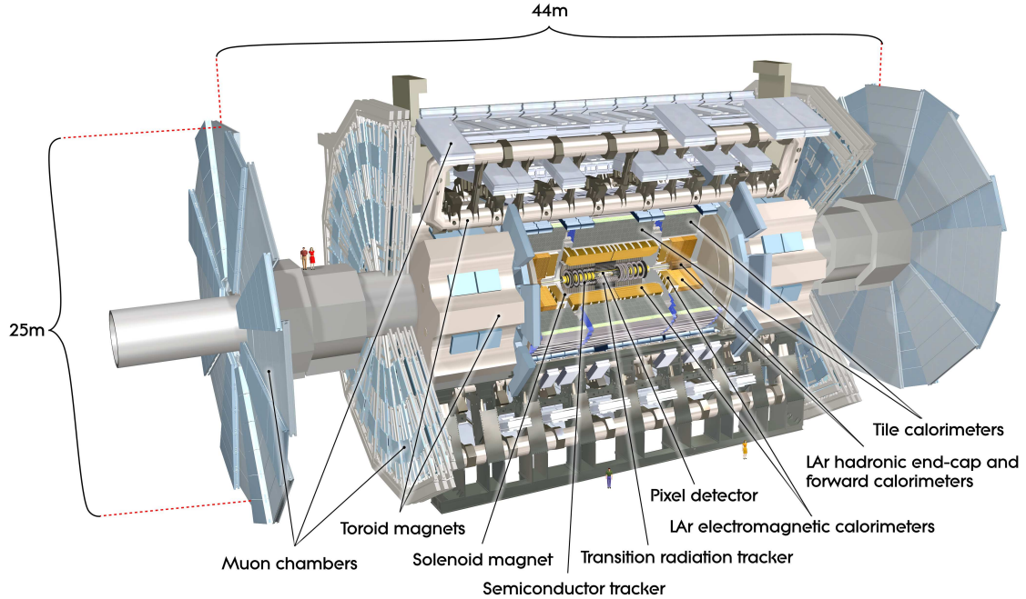
Figure 3.3: Cut-away view of the ATLAS detector. The major detector subsystems are identified.
