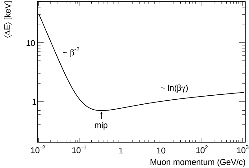
Figure 2.1: Mean energy loss from electronic interactions of a muon traversing the gas volume of a sTGC detector. The energy loss is computed assuming a gas volume with a thickness of 2.8 mm filled with a mixture of n-pentane and \text{CO}_2 in the ratio 45:55.
