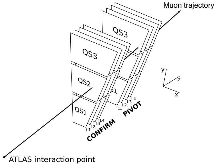
Figure 4.2: Schematic diagram of the simulated detector layout for the small sector. The confirm wedge of the small sector is positioned closer to the ATLAS interaction point than the pivot wedge while the inverse is true for large sectors. A simulated muon trajectory is shown. This schematic is not to scale.
