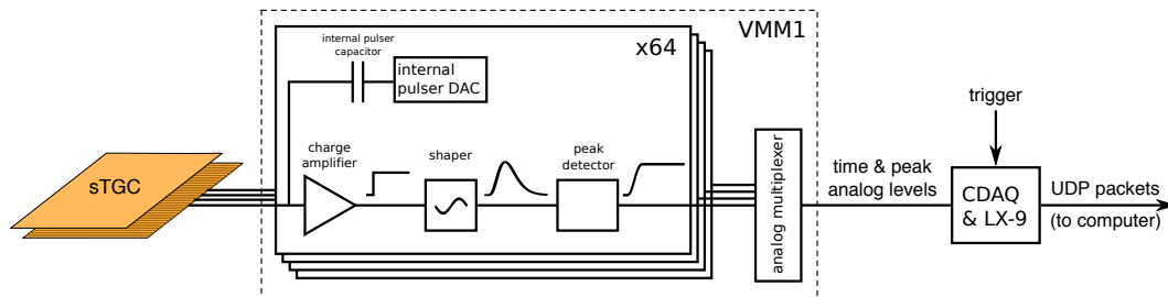
Figure 5.3: Schematic diagram of the VMM1 signal processing chain. The signal from sTGC electrodes (strips on the schematic diagram) is transmitted to one of the 64 VMM1 readout channels. Elements that are part of the VMM1 ASIC are enclosed in the dashed rectangle.
