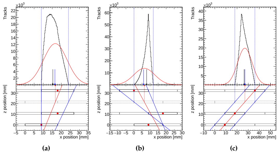
Figure C.2: Results of the wire track interpolation simulation for the three track types considered.
