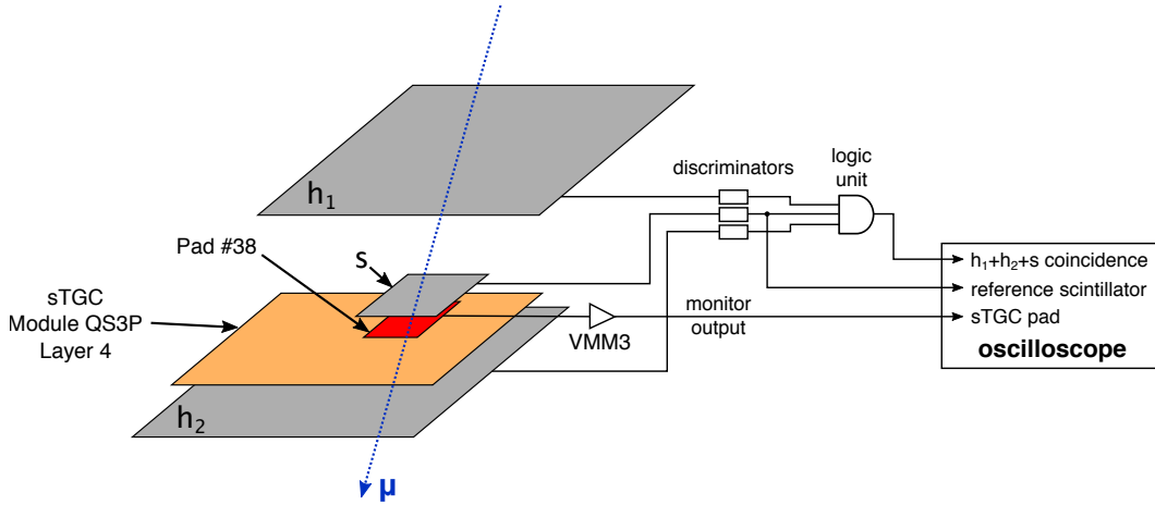
Figure 5.16: Schematic diagram of the experimental setup used for the pad time jitter measurement. The signals from the s , h_1 and h_2 scintillator detectors are processed by discriminators. The coincidence between the three scintillators is provided by a NIM logic unit. Signals from the VMM3 monitor output, the reference scintillator s and the triple coincidence are recorded by the oscilloscope.
