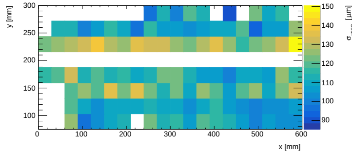
Figure 6.7: Strip intrinsic spatial resolution as a function of position for layer 4 of the 40 \times 60 \text{ cm}^2 sTGC prototype.
