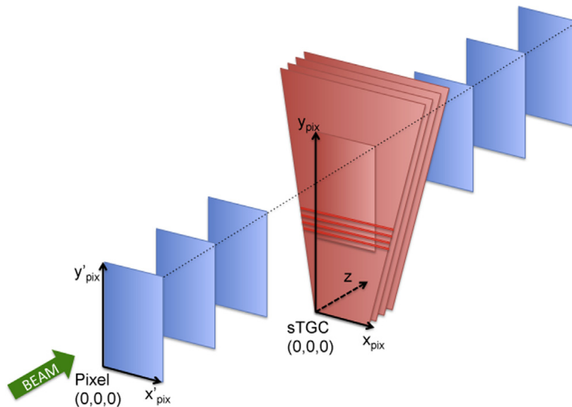
Figure 5.11: Schematic diagram of the experimental setup used for the intrinsic strip spatial resolution measurement with a pion beam. The blue planes indicate the pixel telescope sensor planes. The red trapezoid shapes indicate the sTGC quadruplet gas volumes. The orientation of the sTGC readout strips is shown on the first gas volume. The pixel and sTGC coordinate systems are indicated. The scintillator detectors used for trigger are not shown. The schematic diagram is not to scale.
