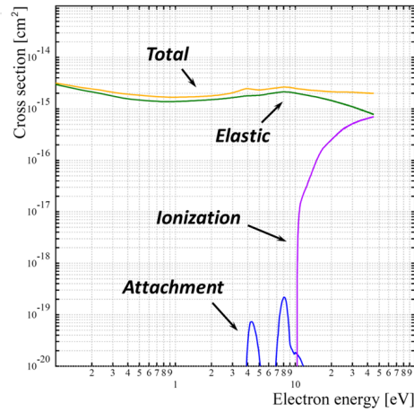
Figure 2.5: Cross-section of the main electron processes as a function of the electron kinetic energy in the operating gas of a sTGC detector, a mixture of n-pentane and \text{CO}_2 in the ratio 45:55. The total cross-section (yellow) is the sum of elastic collision, ionization and attachment processes. The cross-section for ionization is comparable to the cross-section for elastic scattering for electrons with a kinetic energy higher than 50 eV. The cross-sections are obtained from simulation [33].
