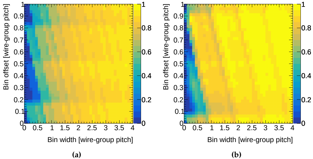
Figure D.4: Simulated bin identification accuracy as a function of the bin width and the bin offset when the tested layer is (a) an outer layer and (b) an inner layer.
