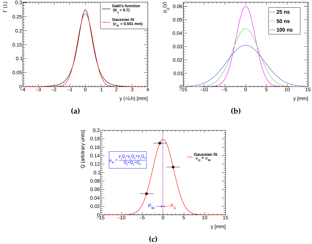
Figure 2.13: (a) Charge induction on the cathode of a sTGC detector predicted by Gatti's formula. (b) The effect of the resistive coating on the charge distribution as a function of time for a graphite time constant of 10 ns. (c) Example of the charge induced on three consecutive readout strips in a sTGC detector as a function of the strip position. The centroid positions obtained using the Gaussian fit ( \mu_G ) and weighted average ( \mu_W ) algorithms, described in Chapter 5, are shown. The charge cluster nominal position is at y = 0 and the strip pattern is shifted by 1.6 mm. The difference between the nominal cluster position and the reconstructed positions is due to the differential non-linearity.
