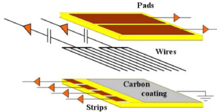
Figure 3.9: Schematic of the pad, strip and wire electrodes of a sTGC gas volume used in the NSW. The wires are ganged in groups of 20 and capacitively coupled to the readout electronics. The strip and pad electrodes are capacitively coupled to the graphite coating.
