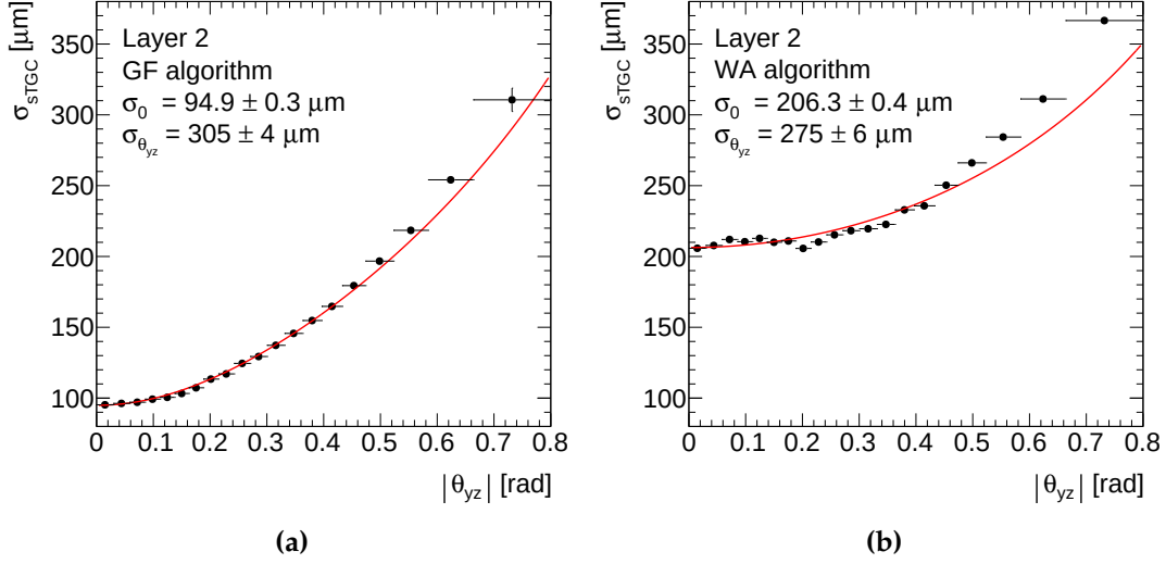
Figure 5.10: Intrinsic strip spatial resolution as a function of the reference track angle \theta_{yz} . The y -coordinate of the space points on all layers is obtained using the (a) GF and (b) WA cluster reconstruction algorithms. The red line is a fit of the expected spatial resolution using the parameterization described in the text.
