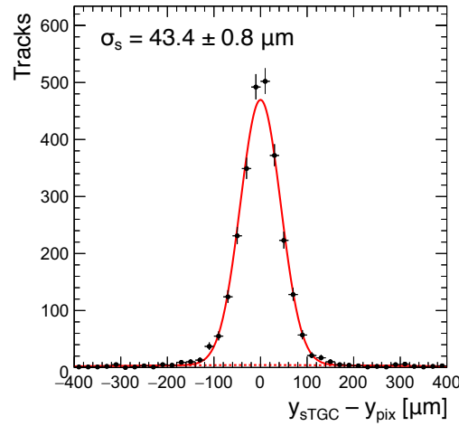
Figure 5.15: Distribution of the reference track y -residual obtained after both differential non-linearity and misalignment corrections are applied. The red line shows the results of the global model fit to the data based on a double Gaussian function. The red dashed line indicates the resulting contribution from the background Gaussian distribution. The value of the fitted \sigma_s parameter, which corresponds to the width of the signal Gaussian function and interpreted as the spatial resolution, is indicated.
