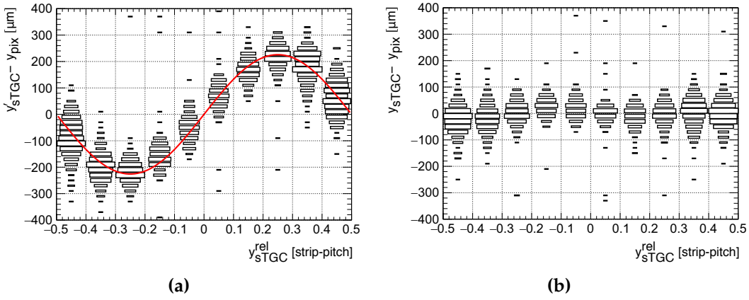
Figure 5.13: Two dimensional distributions of the y -residuals as a function of the the cluster position y_{\text{STGC}}^{\text{rel}} relative to the inter-strip spacing for a representative data acquisition run. The differential non-linearity correction has been omitted in (a). The red line highlights the universal differential non-linearity correction used for correcting all cluster strip multiplicities. The corrected y -residuals are shown in (b).
