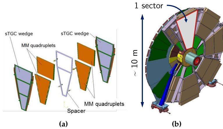
Figure 3.8: (a) Schematic of a disassembled large sector combining sTGC and Micromegas wedges and (b) cutaway drawing of the finished NSW as seen looking towards the interaction point. The sTGC wedges combine 3 modules while Micromegas wedges have 2 modules. The detector modules are made of 4 detector layers. Wedges can be of “large” or “small” type making large and small sectors respectively. The NSW is made of 8 large and 8 small sectors.
