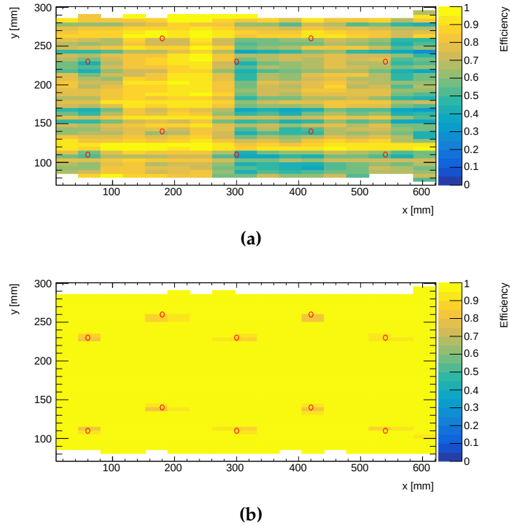
Figure 6.5: Strip efficiency maps for layer 1 of the 40 \times 60 \text{ cm}^2 sTGC prototype at an operating voltage of (a) 2.9 kV and (b) 3.1 kV. The position of button supports in the gas volume of the tested layer is indicated by red circles.
