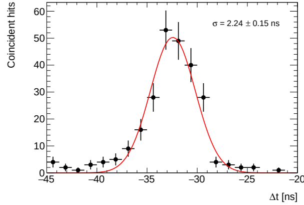
Figure 5.18: Time difference between the coincident hits of the scintillator detector s and another reference scintillator detector of similar size. The Gaussian function fitted to the distribution is shown as a red line. The horizontal axis of the plot has an arbitrary offset.
