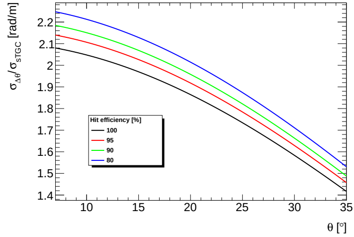
Figure A.2: Angular resolution of a NSW sTGC sector scaled to the intrinsic spatial resolution as a function of the track angle for different values of the hit efficiency. The angular acceptance of a sTGC sector is approximately between 7^\circ and 35^\circ .
