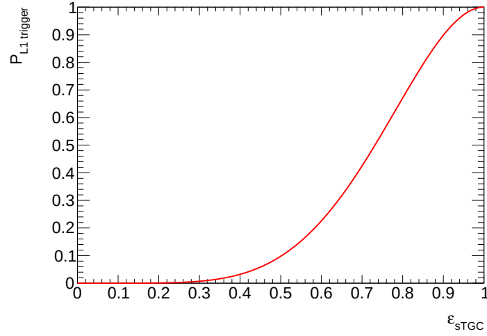
Figure A.1: Trigger efficiency as a function of the single plane sTGC hit efficiency
