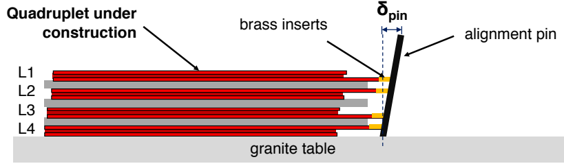
Figure 4.5: Gluing of doublets into a quadruplet on a granite table. The brass inserts are moved away from their nominal positions because of tilted alignment pins.
