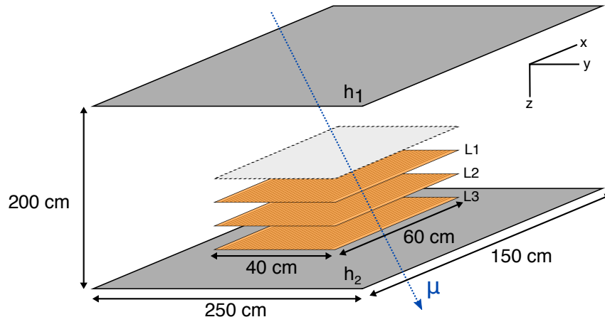
Figure 5.1: Schematic diagram of the experimental setup used for the strip intrinsic spatial resolution measurement performed with cosmic-ray muons. The plastic scintillator detector planes used to provide a data acquisition trigger signal are represented by the areas identified as h_1 and h_2 . Three out of four gas volumes of the sTGC module prototype are read out. Layers under test are denoted L1, L2 and L3. The right-handed Cartesian coordinate system used to define the track space point coordinates is shown. The x -axis is parallel to the readout strips, drawn on each tested layer. The y -axis is perpendicular to the strips. The z -axis is perpendicular to the detector planes. The z -spacing between the gas volume is approximately 10.8 mm. The schematic diagram is not to scale.
