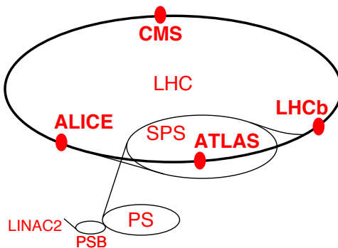
Figure 3.1: Schematic diagram of the LHC and its injectors [72]. The approximate location of the main CERN experiments that are using the LHC beams is also shown. The accelerator complex includes the Linear Accelerator 2 (LINAC2), the Proton Synchrotron Booster (PSB), the Proton Synchrotron (PS), the Super Proton Synchrotron (SPS) and the Large Hadron Collider (LHC).
