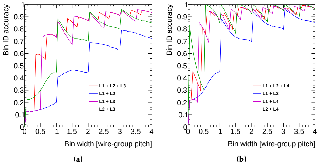
Figure D.5: Simulated BIDA as a function of the bin width for a fixed bin offset equal to half the wire group width when the tested layer is (a) an outer layer and (b) an inner layer. The detector planes used for the reference track reconstruction are indicated in the legend.
