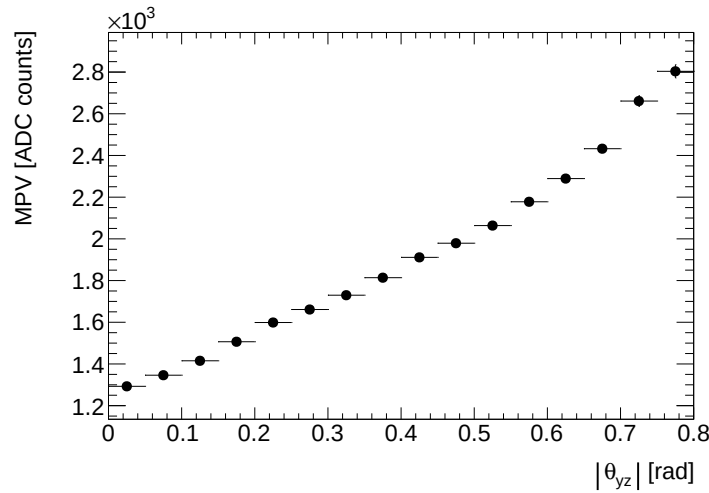
Figure 6.11: Most probable value of the fitted Landau function of the strip Q values as a function of the muon track angle |\theta_{yz}| .
