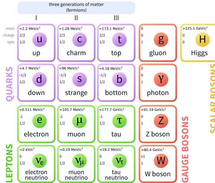
Figure 1.1: Schematic diagram [4] showing the different types of elementary particles observed in nature and described by the Standard Model of particle physics. Particles are arranged in different categories according to their properties. The mass, electric charge and spin of the particles are also indicated using values taken from [5].
