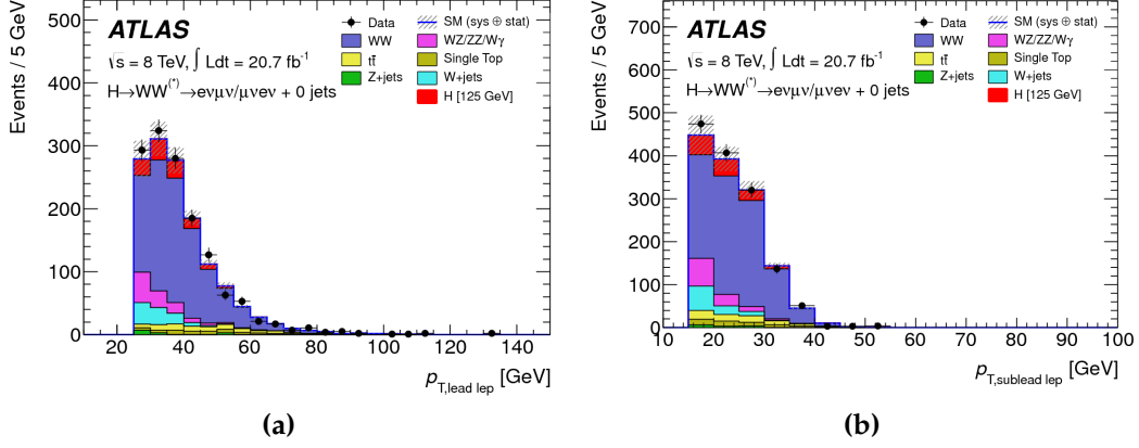
Figure 3.6: Distribution of the (a) leading and (b) subleading lepton p_T for candidate events of the H \rightarrow WW^{(*)} \rightarrow l\nu l\nu decay channel [93]. The red region highlights the simulated yield originating from Higgs boson decays. The efficiency for identifying this particular type of process is very sensitive to an increase in the p_T threshold.
