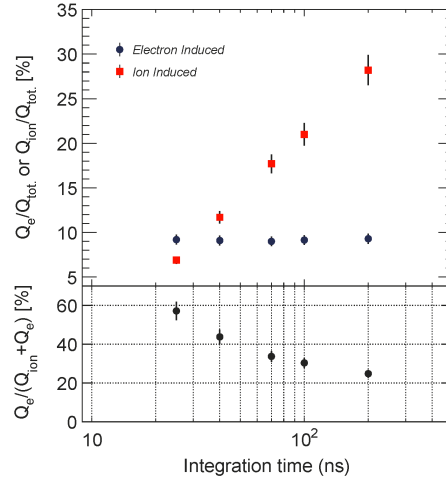
Figure 2.10: Signal contribution of ions and electrons for a sTGC detector as a function of the integration time [33]. The bottom plot highlights that the electron contribution is dominant only for very short integration times. The resulting voltage signal is v = (Q_e + Q_{ion})/C where C is the detector capacitance.
