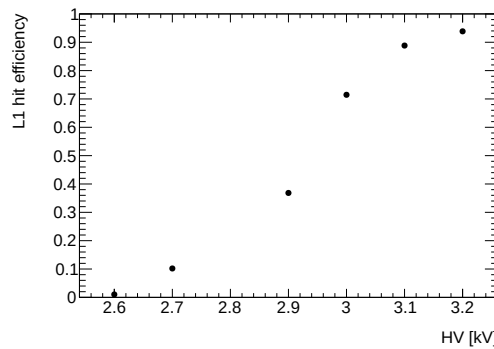
Figure 6.4: Average hit efficiency for layer 1 of the 40 \times 60 \text{ cm}^2 sTGC prototype as a function of the operating voltage.
