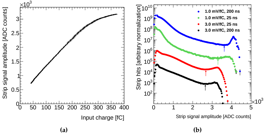
Figure 5.5: (a) Charge response calibration of a VMM1 channel using a gain of 3.0 mV/fC and an integration time of 25 ns. The amplifier linearity is lost at an input charge of approximately 250 fC. (b) Distributions of strip signal amplitude in cosmic-ray muon data obtained with different VMM1 configurations. The arrows indicate the onset of saturation effects and are positioned at the approximate value of P_{\text{sat}} used for charge cluster reconstruction.
