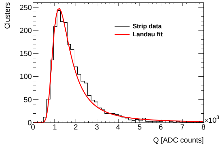
Figure 6.9: Distribution of the strip cluster charge with Landau fit for a single measurement bin of the gain uniformity map located at 280 \text{ mm} \leq x < 300 \text{ mm} and 270 \text{ mm} \leq y < 280 \text{ mm} . Measurements were performed on layer 2 of the 40 \times 60 \text{ cm}^2 sTGC prototype.
