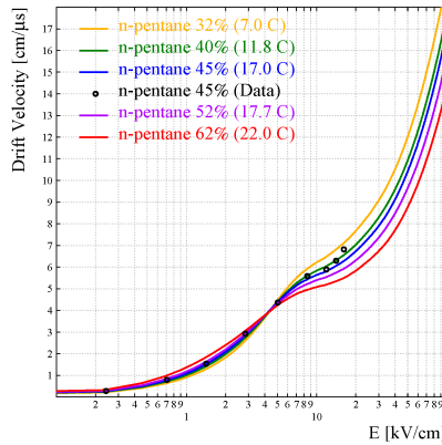
Figure 2.4: Drift velocity of electrons as a function of the electric field for various concentrations of n-pentane in \text{CO}_2 [33]. The x -axis covers the possible E field values within the gas volume of a sTGC operating at 2.9 kV.
