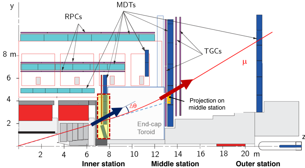
Figure 3.7: Projection of the current ATLAS muon spectrometer on the y - z plane [97]. The yellow shaded rectangle highlights the inner station modules that will be replaced by the NSW as part of the muon spectrometer upgrade. A visual representation of the Level-1 muon trigger algorithm, based on information from the NSW, is shown. A muon originating from the interaction point (red line) traverses the NSW resulting in the reconstruction of a track segment. The NSW measurement is used to confirm whether the reconstructed track segment comes from a particle originating from the interaction point by measuring the angle difference \Delta\theta between the reconstructed track segment and a track segment that would be expected from a muon originating from the interaction point. Then, the NSW track segment is required to be consistent with a second track segment reconstructed by the middle station. Finally, if the NSW trigger conditions are met, the central trigger processor determines if a Level-1 trigger accept shall be issued based on the track segments. The muon transverse momentum p_T is estimated from the muon deviation in the magnetic field of the end-cap toroid which corresponds to angle difference of the track segments of the inner and middle stations.
