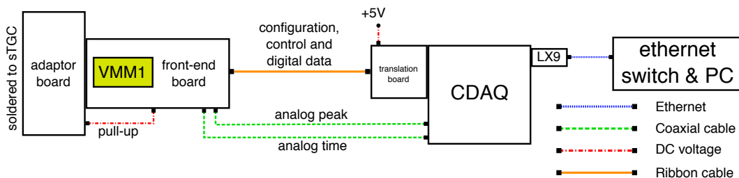
Figure 5.2: Schematic diagram of the data acquisition system associated with a single VMM1 ASIC used to read out wire and strip electrodes. The translation board is used to convert the digital voltage levels for communication between the CDAQ and the front-end board. The translation board also provides power to the CDAQ and the front-end board through the +5V input. The pull-up is a DC voltage level used to bias the signal from sTGC strips and is required by the VMM1 to read out a signal of positive polarity.
