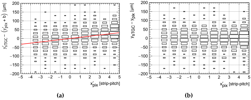
Figure 5.14: Two-dimensional distributions of y -residuals as a function of x'_{\text{pix}} for a representative data acquisition run. The rotation correction (red line) has been omitted in (a) for computing the residuals, whereas the corrected y -residual distribution is shown in (b).
