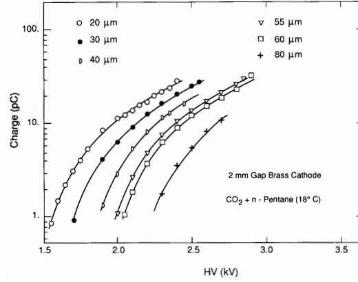
Figure 2.9: Impact of the wire diameter on the signal response of a TGC [50]. The charge saturation as a function of the operational high voltage (HV) is explained by space charge effects [51].
