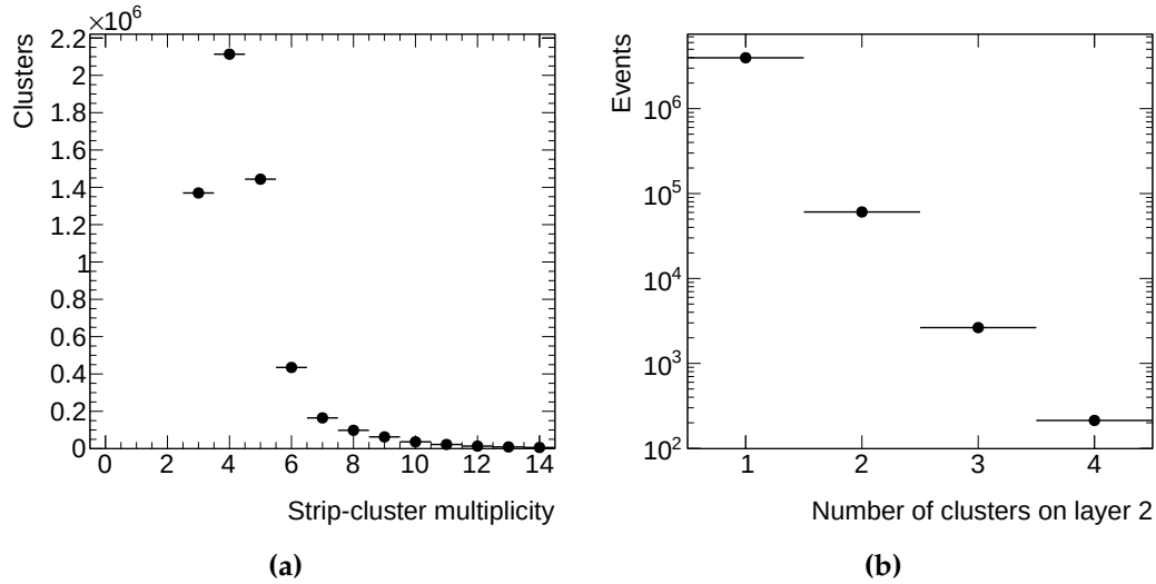
Figure 5.6: (a) Distribution of the charge cluster strip multiplicity for layer 2 and (b) distribution of the number of clusters for the same layer. The VMM1 gain is 3.0 mV/fC and the integration time is 25 ns.
