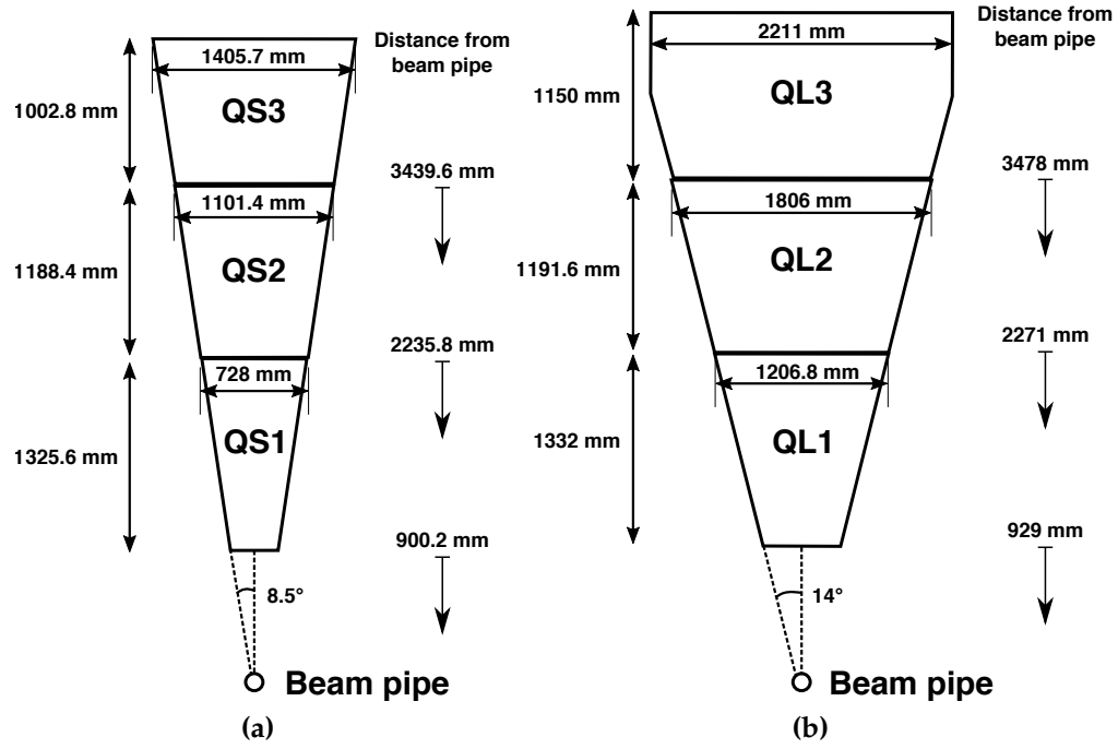
Figure 4.3: Dimensions of the (a) small and (b) large sTGC wedges projected in the x-y plane. The schematics are to scale. The height, width and distance from the beam pipe of each sTGC quadruplet are displayed. The wedges angular coverage in \phi is also shown. There are small gaps between the quadruplets of the order of 1 cm that cannot be resolved on the figure.
