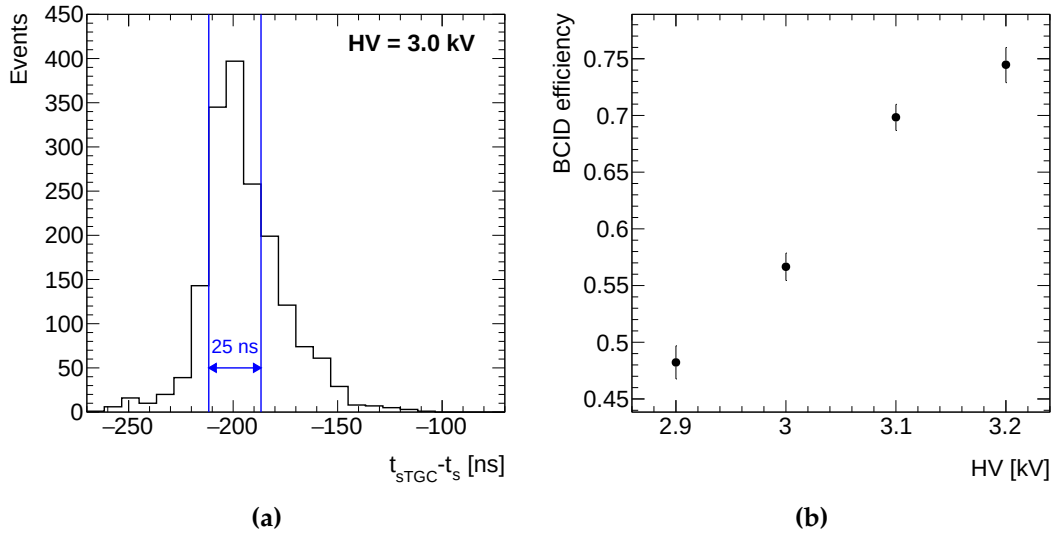
Figure 5.20: (a) Pad time jitter at an operating voltage of 3.0 kV and (b) fraction of hits contained in an optimal 25 ns time-window as a function of the operating voltage. The optimal 25 ns time-window, used to calculate the BCID efficiency, is highlighted with blue lines on the (a) distribution.
