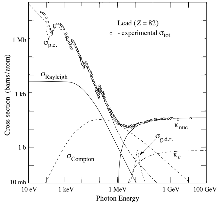
Figure 2.3: Interaction cross-section of photons in lead [5]. The contribution of individual photon processes, including the photoelectric effect ( \sigma_{p.e.} ), Compton effects ( \sigma_{Compton} ) and pair production (in the nuclear field, \kappa_{nuc} , and in the electron field, \kappa_e ) is shown. The contribution of Rayleigh scattering ( \sigma_{Rayleigh} ) and photonuclear interactions ( \sigma_{g.d.r.} ) to the photon cross-section is also shown. These processes were not mentioned in the text because they are not dominant.
