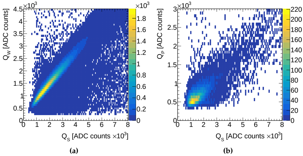
Figure 6.12: Two-dimensional distributions of Q for (a) layer 2 strips and wires and (b) layer 3 strips and pads measured with the 40 \times 60 \text{ cm}^2 sTGC prototype.
