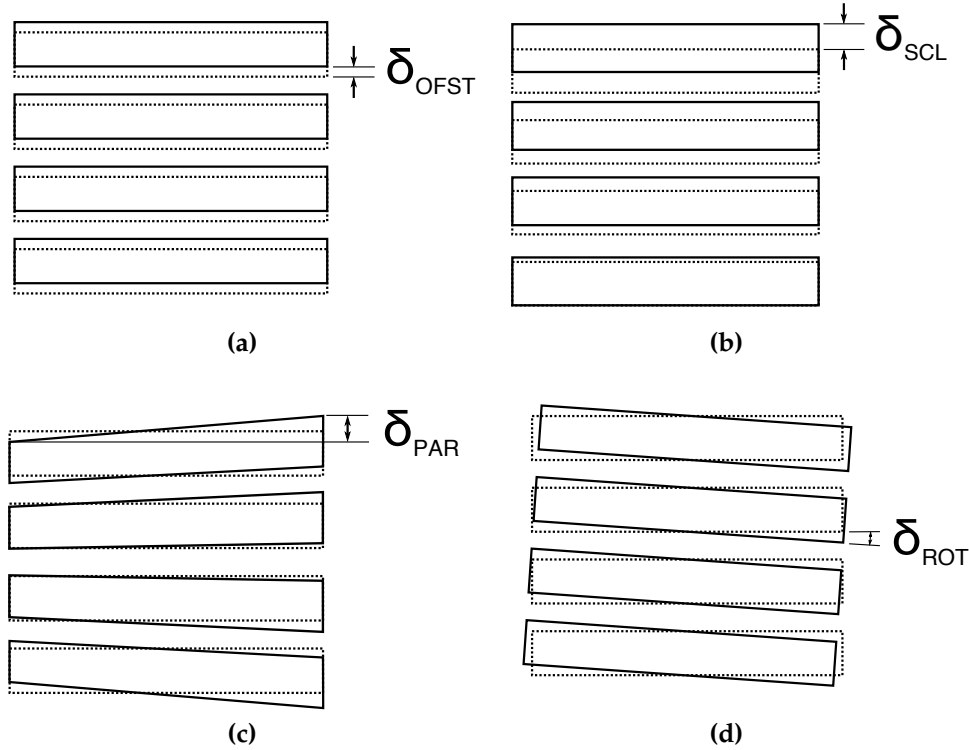
Figure 4.1: Sketch of the strip-board non-conformities considered compared to the nominal strip pattern (dotted lines): (a) constant offset, (b) pitch scale, (c) non-parallelism and (d) rotation. The measurement performed during strip-board dimensional control is shown on each diagram. The values of \delta_{\text{OFST}} , \delta_{\text{SCL}} and \delta_{\text{PAR}} are in units of length while the value of \delta_{\text{ROT}} is an angle. The strip dimensions are not to scale.
