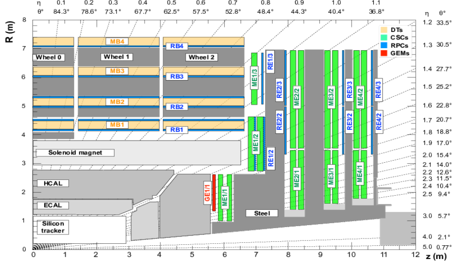
Figure 1.11: Quadrant of the CMS detector showing the present muon system including RPCs, DTs and CSCs. The first GEM detectors in the inner endcap stations is indicated by the red box. The full implementation of the GEM detectors will be carried on going towards the HL-LHC [30].
