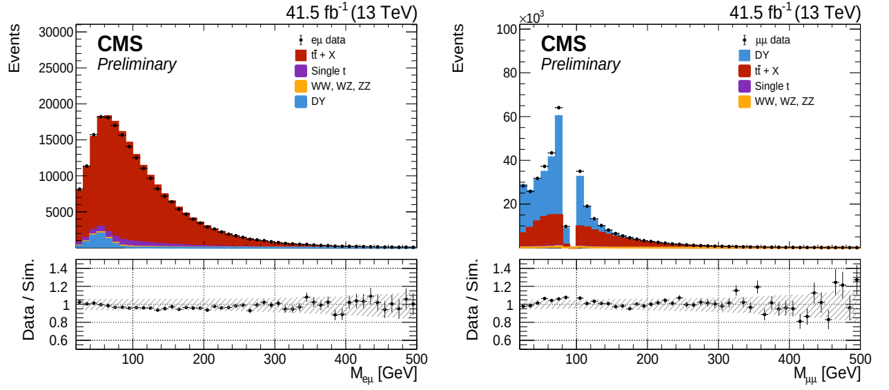
Figure D.17: For 2017 data and MC, invariant mass of the lepton pair in the (left) e\mu and (right) \mu\mu samples. The hatched bands represent the systematic uncertainties.
