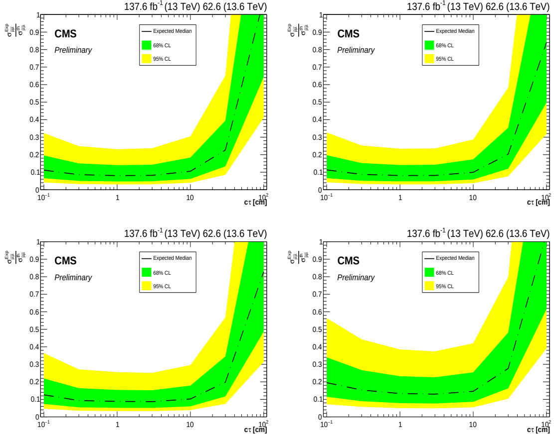
Figure G.8: \sigma_{\mu\tilde{\mu}} \times B_r(\tilde{\mu} \rightarrow \mu\tilde{\chi}_1^0)^2 assuming different mass combinations between the smuon and the neutralino S_{m_{\tilde{\chi}_1^0}}^{m_{\tilde{\mu}}} : (upper left) S_{300}^{500} (upper right) S_{350}^{500} (lower left) S_{400}^{500} (lower right) S_{450}^{500} . Signal samples for which the ratio of the cross sections is below 1 are excluded.
