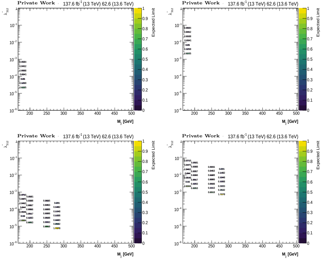
Figure 5.30: \lambda''_{312} vs M_{\tilde{\chi}_1^0} expected limits at a 95% confidence level assuming different stop masses of (left) 1 TeV and (right) 10 TeV and smuon masses (upper) 200 GeV (lower) 300 GeV. The z -axis is the ratio of the expected cross section over the theoretical one. Signal samples with z -axis values below 1 are excluded. The center of each bin corresponds to a specific signal sample. The upper and lower values of \lambda'' correspond to the tracker bounds of CMS following Eq.3.48.
