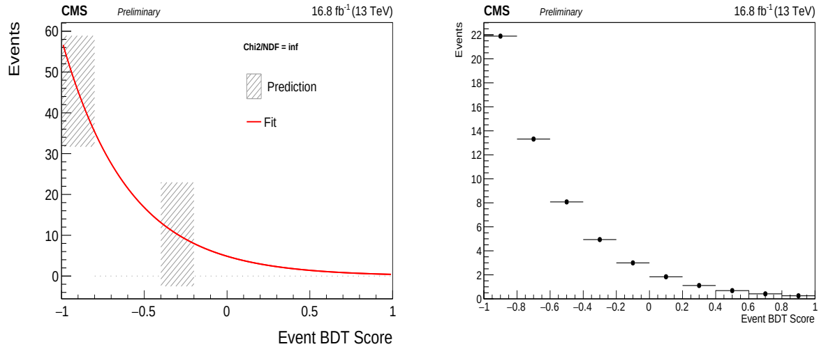
Figure F.2: (left) Fit of the background estimate in the signal region for 2016-post \mu\mu data. (right) Toy experiments generated injected in the COMBINE tool to extract expected limits.
