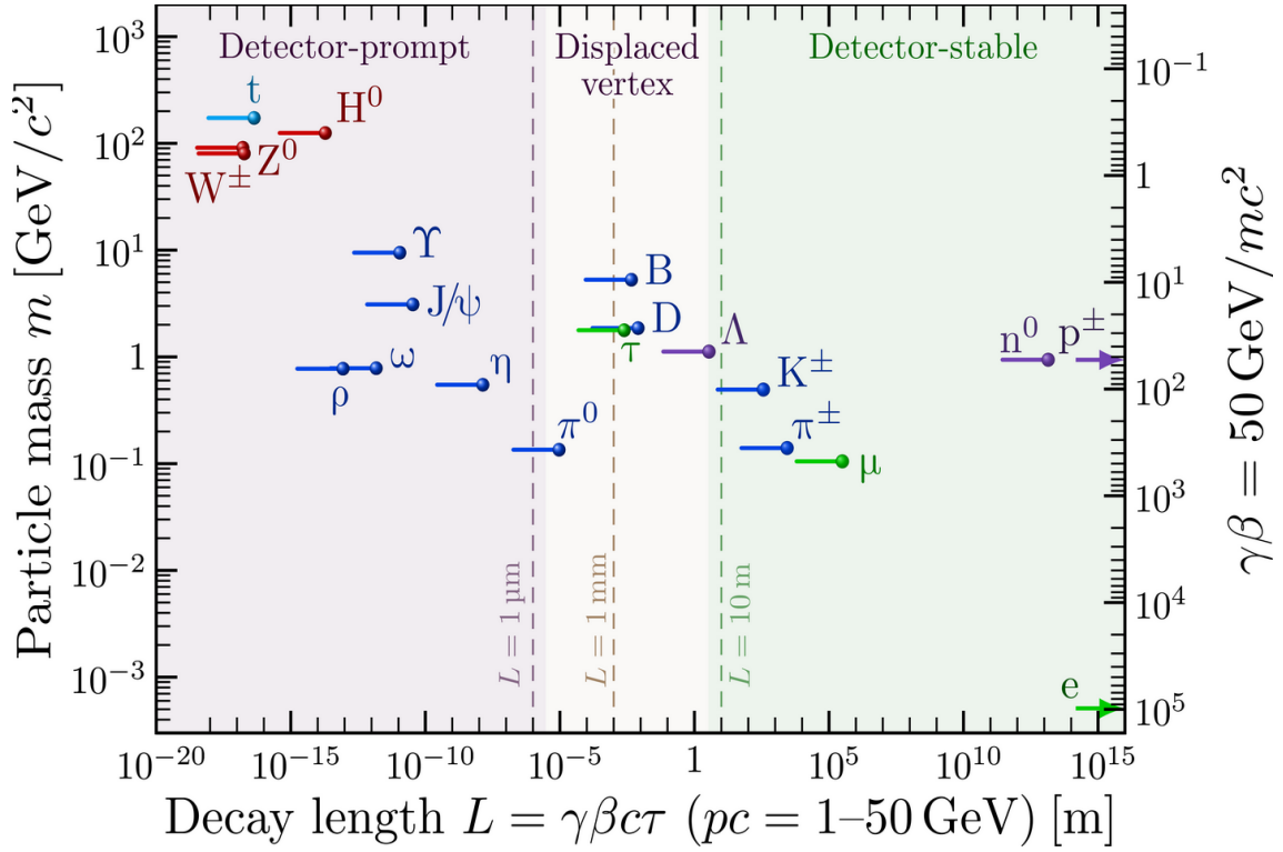
Figure 3.8: Standard Model particles decay length for a momentum range from 1 to 50 GeV [25]. Particles highlighted in green (red) are the SM fermions (bosons). The top quark (light blue) is the only quark that decays, the other quarks follow the process of hadronization. Dark-blue (purple) particles are bound states made of 2 (3) quarks referred as mesons (baryons).
