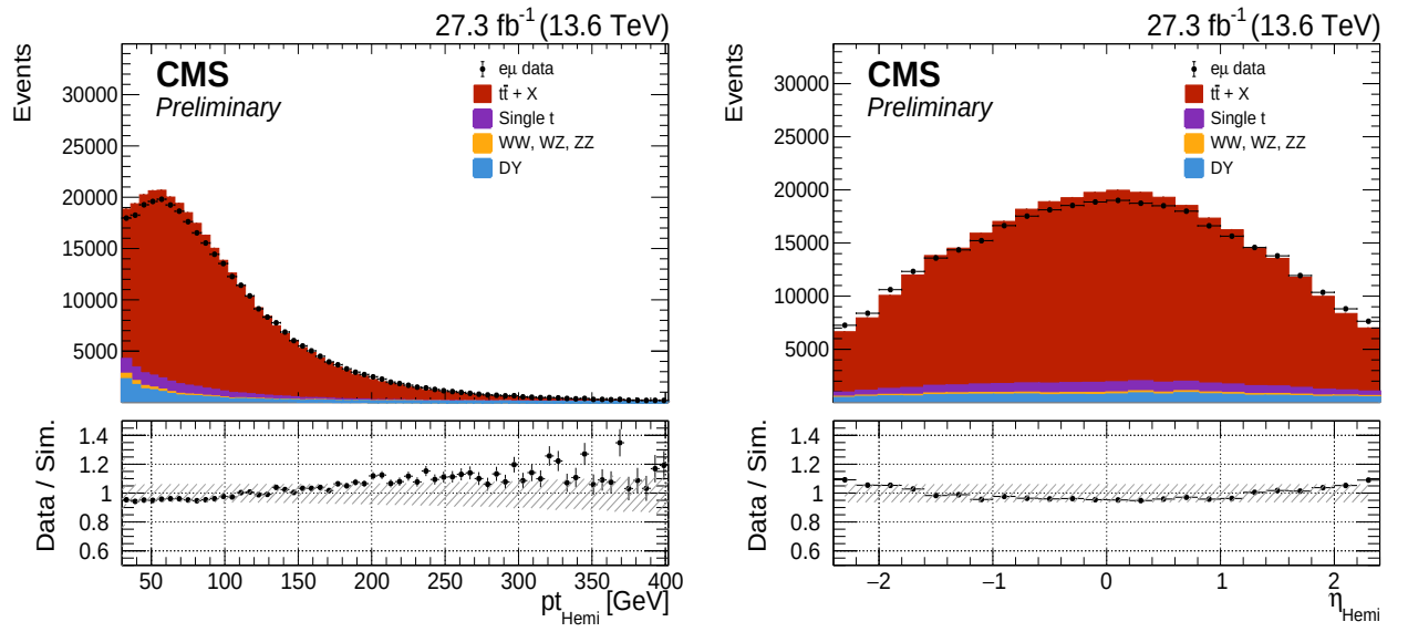
Figure D.37: p_T and \eta of the hemispheres in the 2023 e\mu data and MC. The hatched bands represent the systematic uncertainties.
