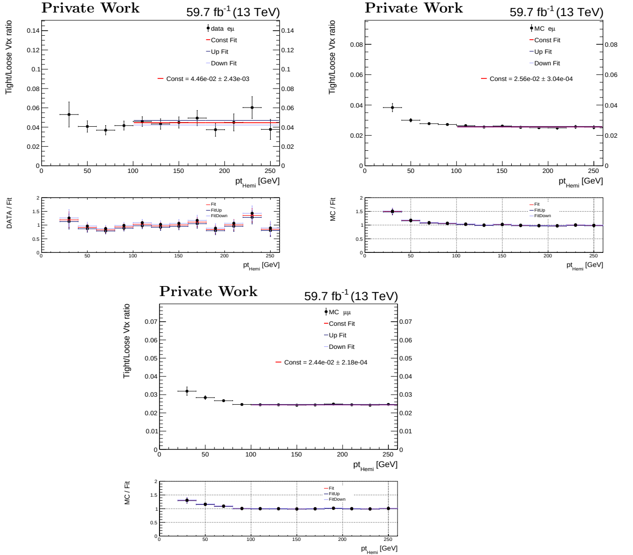
Figure 5.17: Ratio of the number of tight over loose vertices as a function of the p_T of the hemispheres in the 2018 (upper left) e\mu data, (upper right) e\mu MC and (lower) \mu\mu MC.
