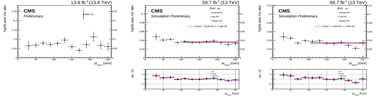
Figure D.30: Ratio of the number of tight over loose vertices as a function of the p_T of the hemispheres in the 2022-pre (left) e\mu data, (middle) e\mu MC and (right) \mu\mu MC.
