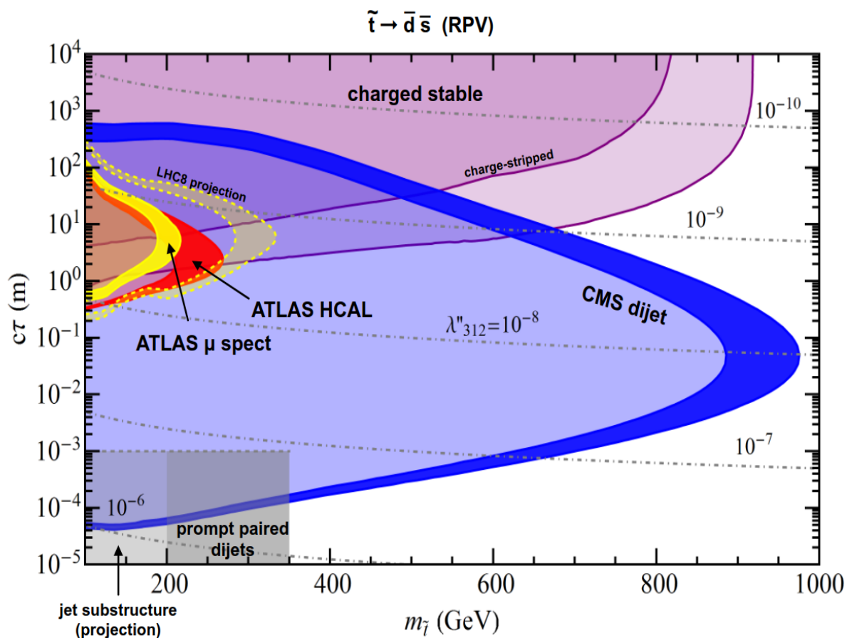
Figure 3.13: Recast constraints on displaced stop via baryonic RPV based on Run 1 results. Colored bands indicate acceptance variations up/down by 1.5. The dot-dashed lines indicate contours of \lambda_{312}'' , assumed to be the only contributing RPV coupling. [127]
