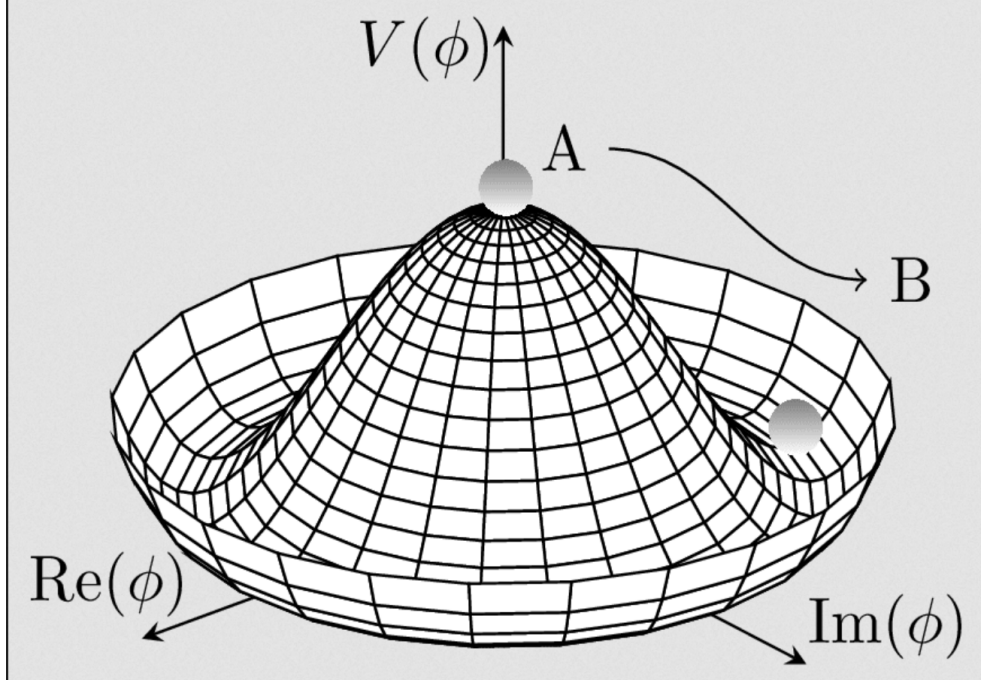
Figure 3.3: Shape of the scalar potential V with positive value for \mu and \lambda [25].
