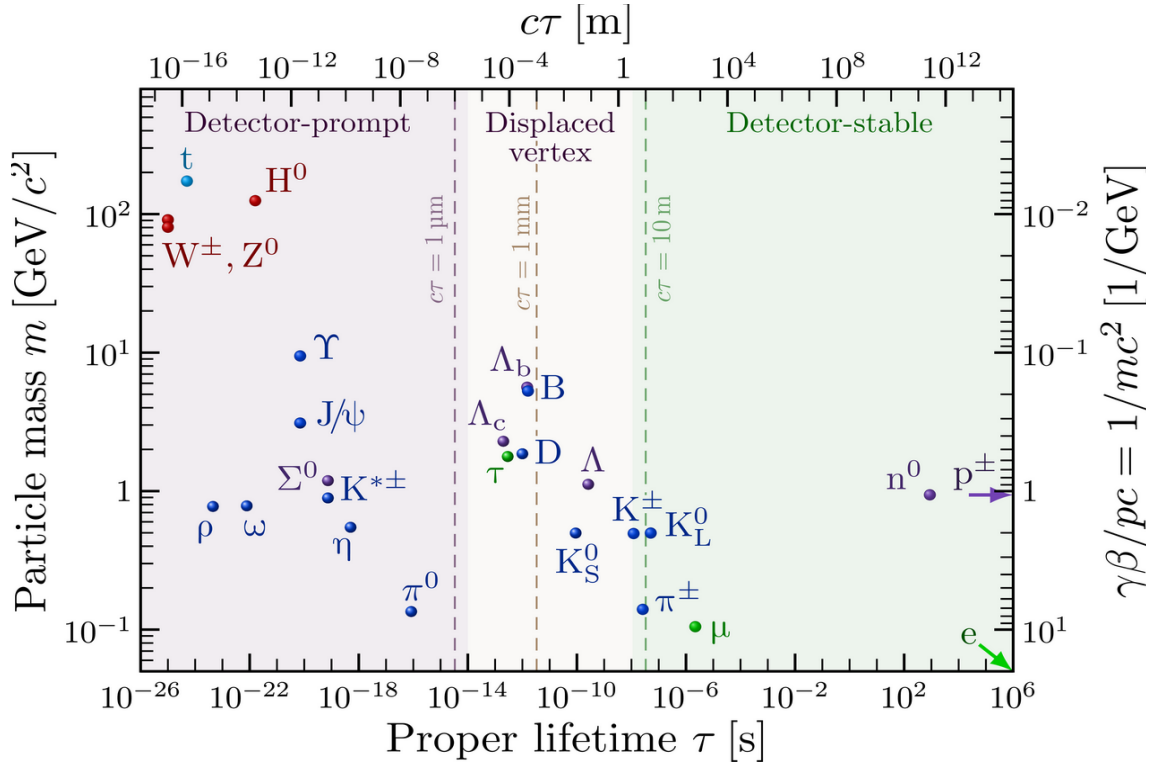
Figure 3.2: Standard Model particles proper lifetime [25]. Particles highlighted in green (red) are the SM fermions (bosons). The top quark (light blue) is the only quark that decays, the other quarks follow the process of hadronization. Dark-blue (purple) particles are bound states made of 2 (3) quarks referred as mesons (baryons).
