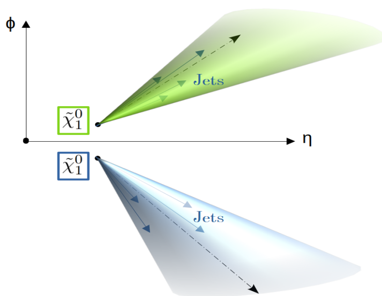
Figure 4.8: Schematic view of the decay of the two neutralinos. The dashed black arrow displays the direction of the generated neutralino momentum.
