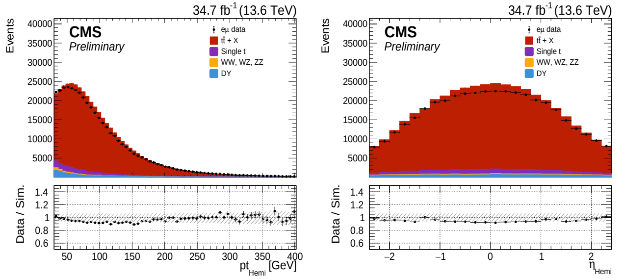
Figure D.26: p_T and \eta of the hemispheres in the 2022 e\mu data and MC. The hatched bands represent the systematic uncertainties.
