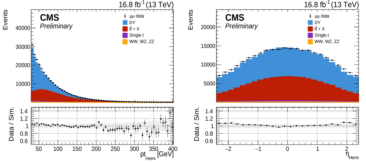
Figure D.12: p_T and \eta of the hemispheres in the 2016-post \mu\mu data and MC. The hatched bands represent the systematic uncertainties.
