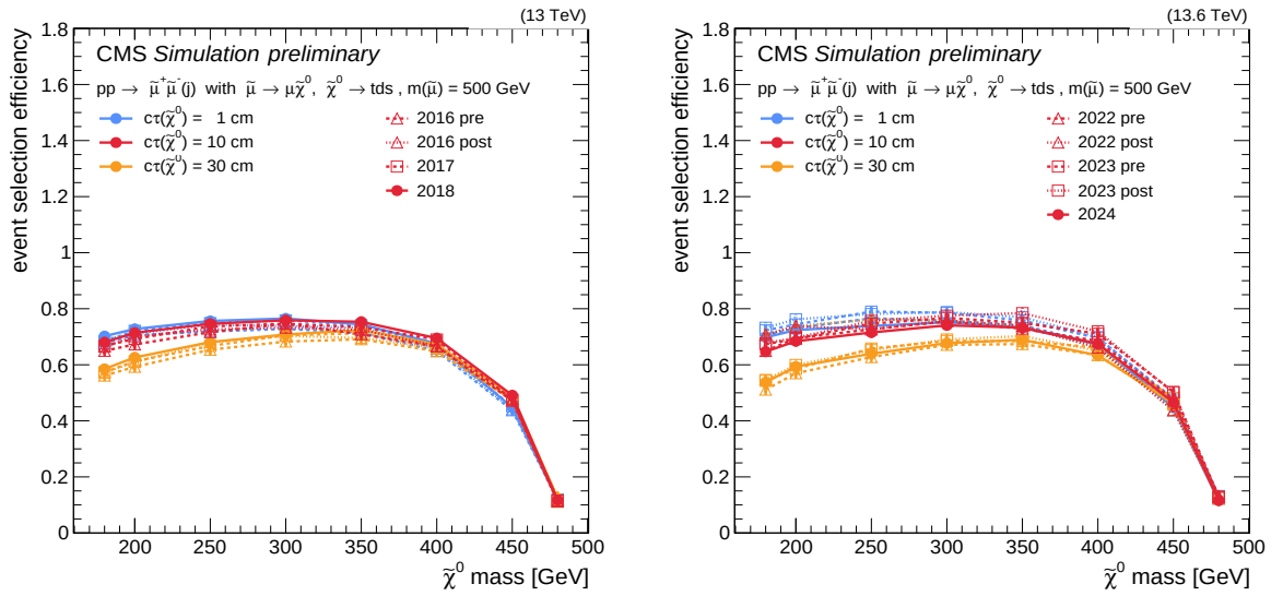
Figure C.1: Event selection efficiency in signal events as a function of the neutralino and smuon masses and neutralino c\tau_{\tilde{\chi}} in each MC year period of (left) Run 2 and (right) Run 3.
