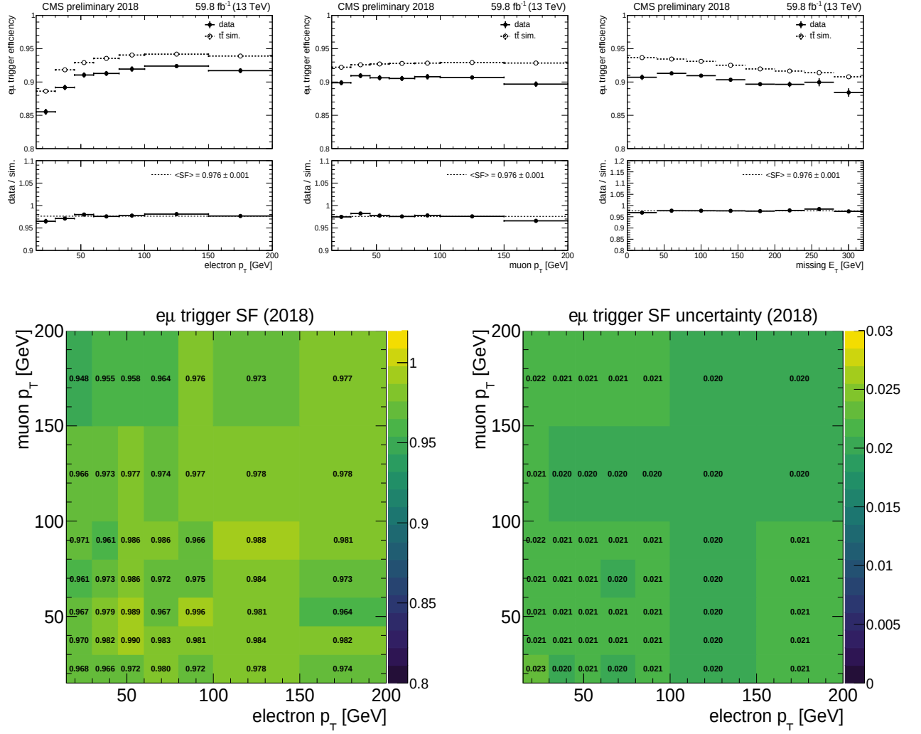
Figure E.3: Same as Fig.E.1 for the 2018 datasets.
