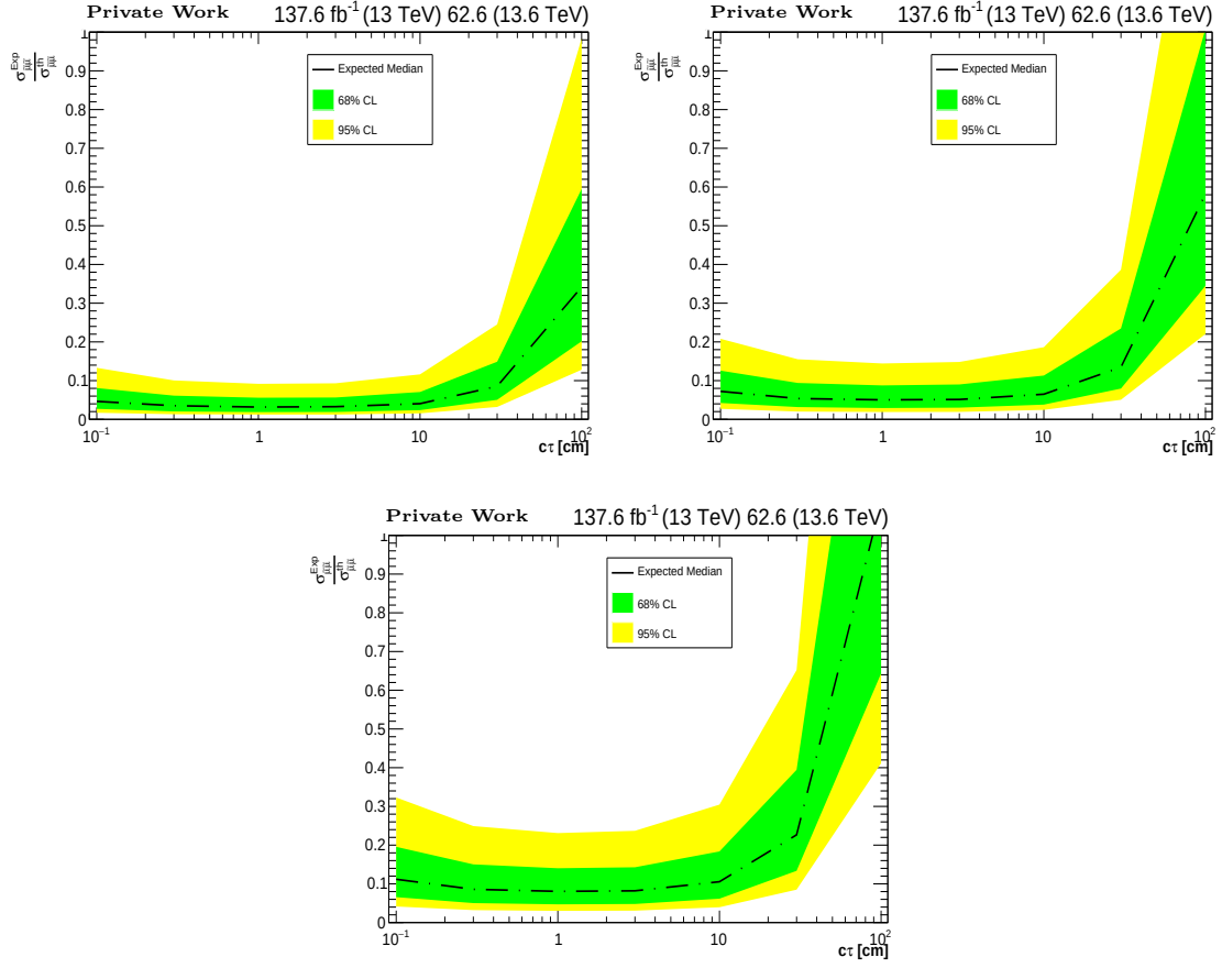
Figure 5.29: \sigma_{\tilde{\mu}\tilde{\mu}} \times B_r(\tilde{\mu} \rightarrow \mu\tilde{\chi}_1^0)^2 assuming different mass combinations between the smuon and the neutralino S_{m_{\tilde{\chi}_1^0}}^{m_{\tilde{\mu}}} : (upper left) S_{300}^{400} (upper right) S_{300}^{450} (lower) S_{300}^{500} . Signal samples for which the ratio of the cross sections is below 1 are excluded.
