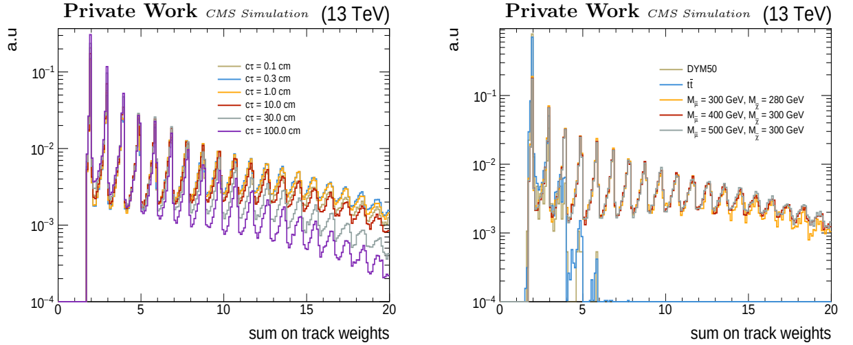
Figure 5.10: Example of the distribution of \sum w (left) as a function of the signal c\tau_{\tilde{\chi}} and (right) for different backgrounds and signals. Peaks are observed around integers values when the number of tracks at vertex N = \lceil \sum w \rceil .
