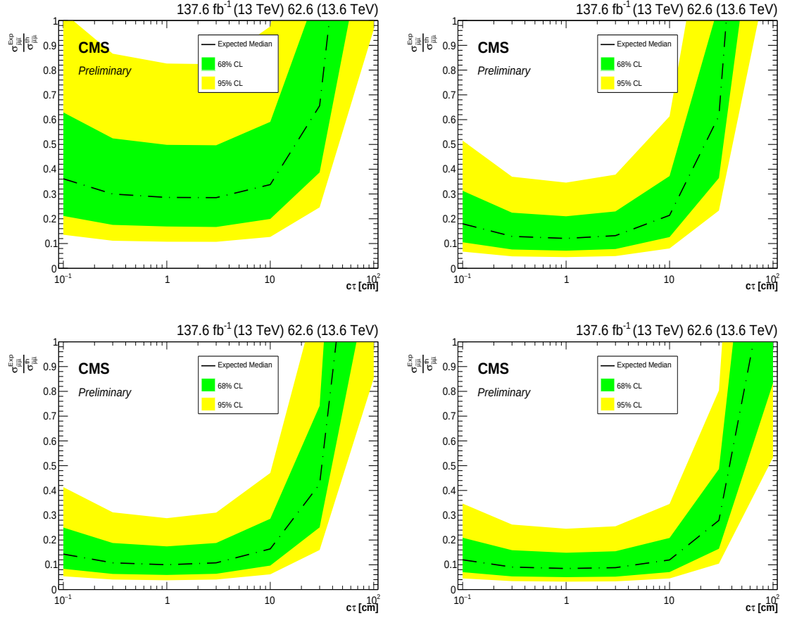
Figure G.7: \sigma_{\mu\tilde{\mu}} \times B_r(\tilde{\mu} \rightarrow \mu\tilde{\chi}_1^0)^2 assuming different mass combinations between the smuon and the neutralino S_{m_{\tilde{\chi}_1^0}^{m_{\tilde{\mu}}}} : (upper left) S_{430}^{450} (upper right) S_{180}^{500} (lower left) S_{200}^{500} (lower right) S_{250}^{500} . Signal samples for which the ratio of the cross sections is below 1 are excluded.
