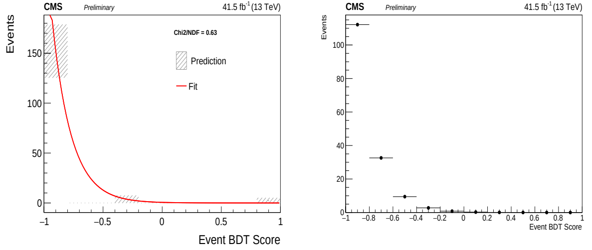
Figure F.3: (left) Fit of the background estimate in the signal region for 2017 \mu\mu data. (right) Toy experiments generated injected in the COMBINE tool to extract expected limits.
