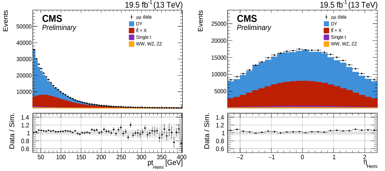
Figure D.4: p_T and \eta of the hemispheres in the 2016-pre \mu\mu data and MC. The hatched bands represent the systematic uncertainties.
