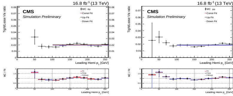
Figure D.15: Ratio of the number of tight over loose vertices as a function of the p_T of the leading hemisphere in the 2016-post (left) e\mu MC and (right) \mu\mu MC.
