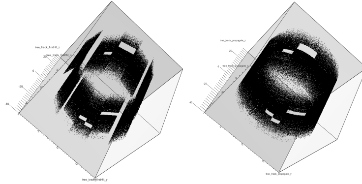
Figure 4.3: First hit of the tracks in the BPIX L1 in the (left) RECO data tier and (right) MINIAOD data tier. Layers in MINIAOD are approximated as cylinders in the barrel region and as planes in the endcap regions. The cylinder has a radius that is defined by the mean position of the first hit of tracks in RECO. Masked modules that can be identified in RECO are still clearly visible in MINIAOD.
