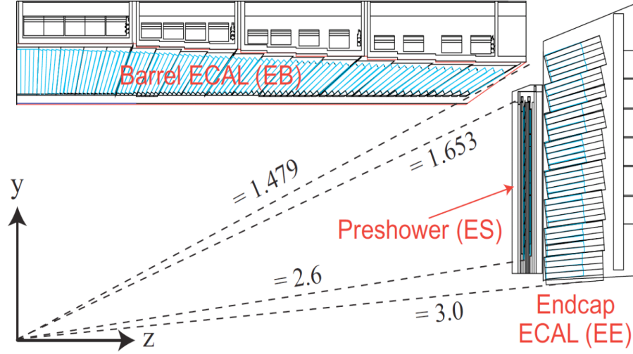
Figure 1.9: Sketch of one quarter of the ECAL in the r-z view [23].
