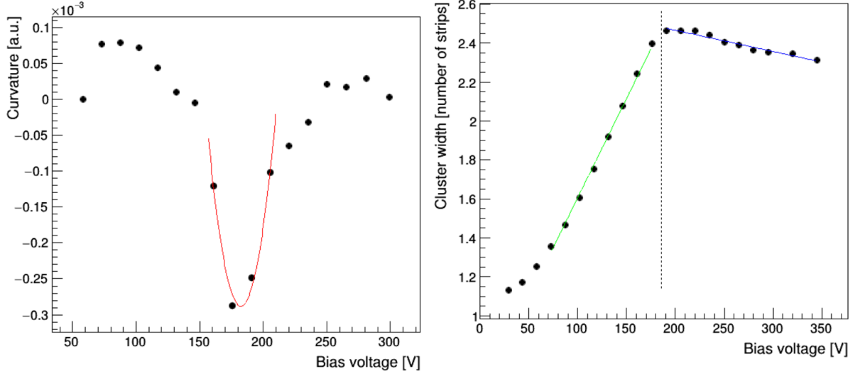
Figure 2.19: (Left) Fit of the curvature of the leakage current as a function of the bias voltage. The V_{FD} value is defined as the minimum of the parabola. (Right) Linear fit of the two regimes with the black dashed line being V_{FD} . The figures are shown for a TIB L1 module during the scan of August 2012 [85].
