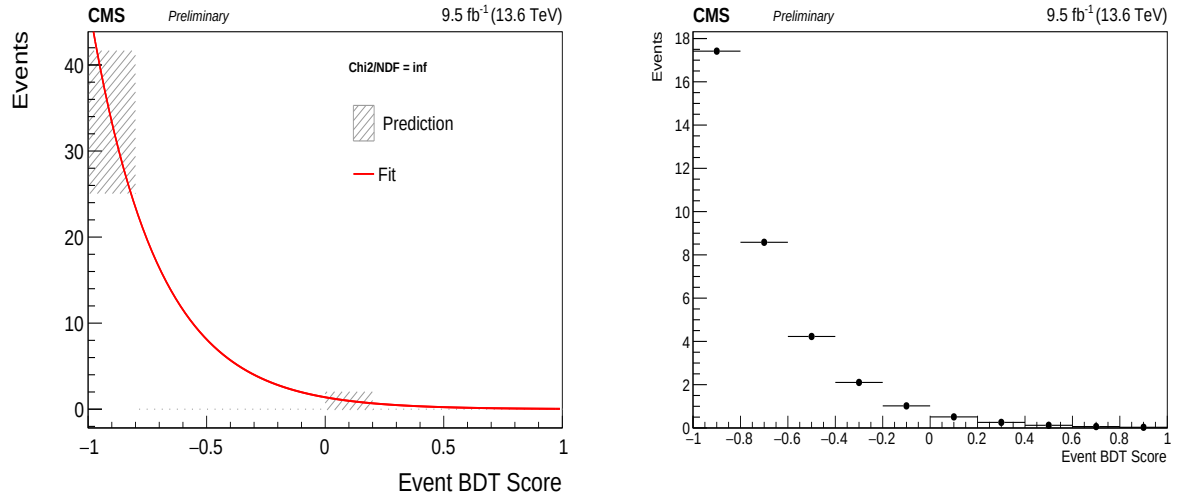
Figure F.7: (left) Fit of the background estimate in the signal region for 2023-post \mu\mu data. (right) Toy experiments generated injected in the COMBINE tool to extract expected limits.
