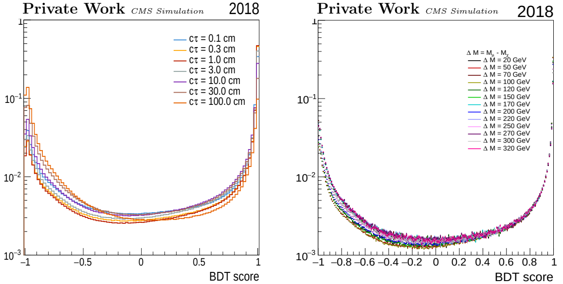
Figure 4.33: Track BDT score for (left) different neutralino c\tau_{\tilde{\chi}} for any mass combination between the neutralino and the smuon and (right) for different \Delta m_{\tilde{\mu}\tilde{\chi}} for any c\tau_{\tilde{\chi}} .
