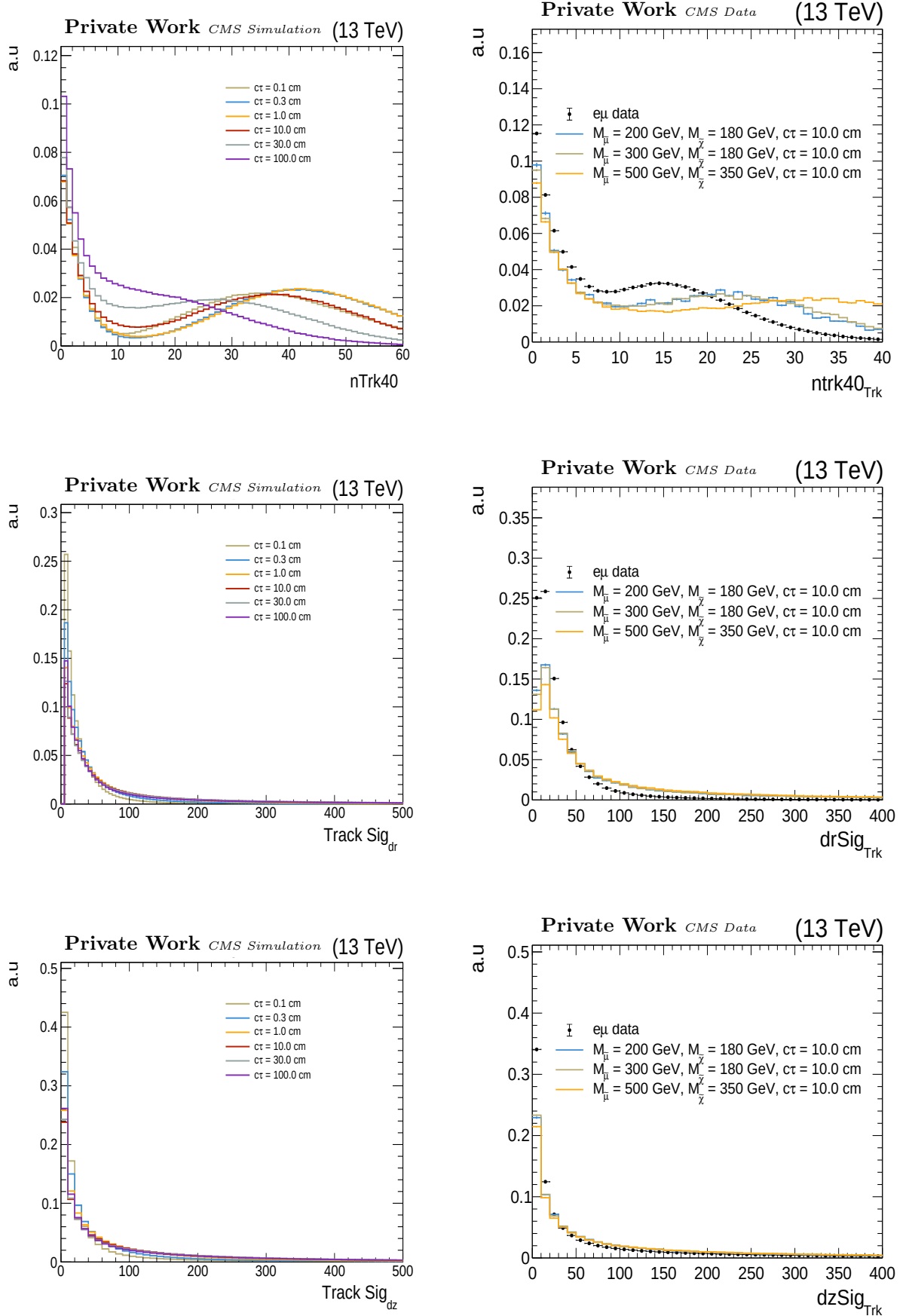
Figure 4.28: Input variables to the BDT. The left column shows the signal distribution for different c\tau_{\tilde{\chi}} while the right column shows the comparison between signal and e\mu data.
