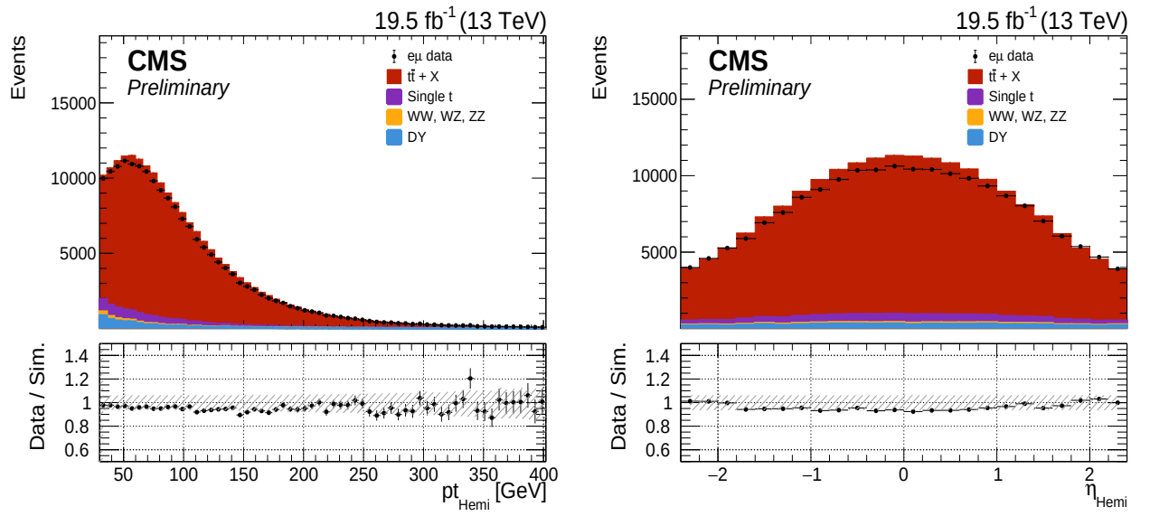
Figure D.2: p_T and \eta of the hemispheres in the 2016-pre e\mu data and MC. The hatched bands represent the systematic uncertainties.
