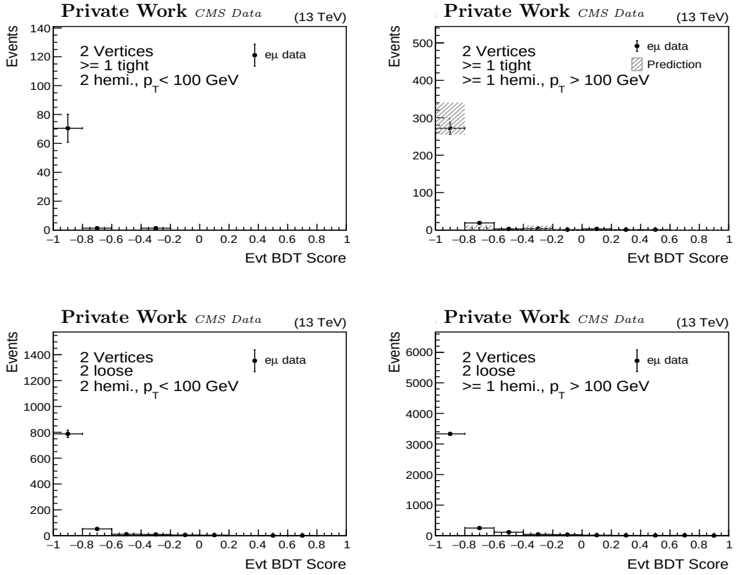
Figure 5.20: Background estimation method applied to the 2018 e\mu data sample, taking into account the correction associated with the correlation.
