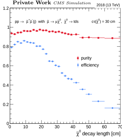
Figure 5.6: Tight vertex reconstruction efficiency (blue) and purity (red) as a function of the decay length of the neutralino. Signal events are simulated in the 2018 conditions for a broad range of smuon and neutralino masses and neutralino c\tau_{\tilde{\chi}} = 30 cm.
