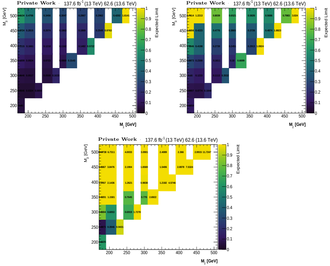
Figure 5.27: M_{\tilde{\mu}} vs M_{\chi_1^0} expected limits at a 95% confidence level assuming a mean c\tau_{\tilde{\chi}} of (upper left) 10.0 cm (upper right) 30.0 cm (lower) 100.0 cm. The z -axis is the ratio of the expected cross section over the theoretical one. Signal samples with z -axis values below 1 are excluded. The center of each bin corresponds to a specific signal sample.
