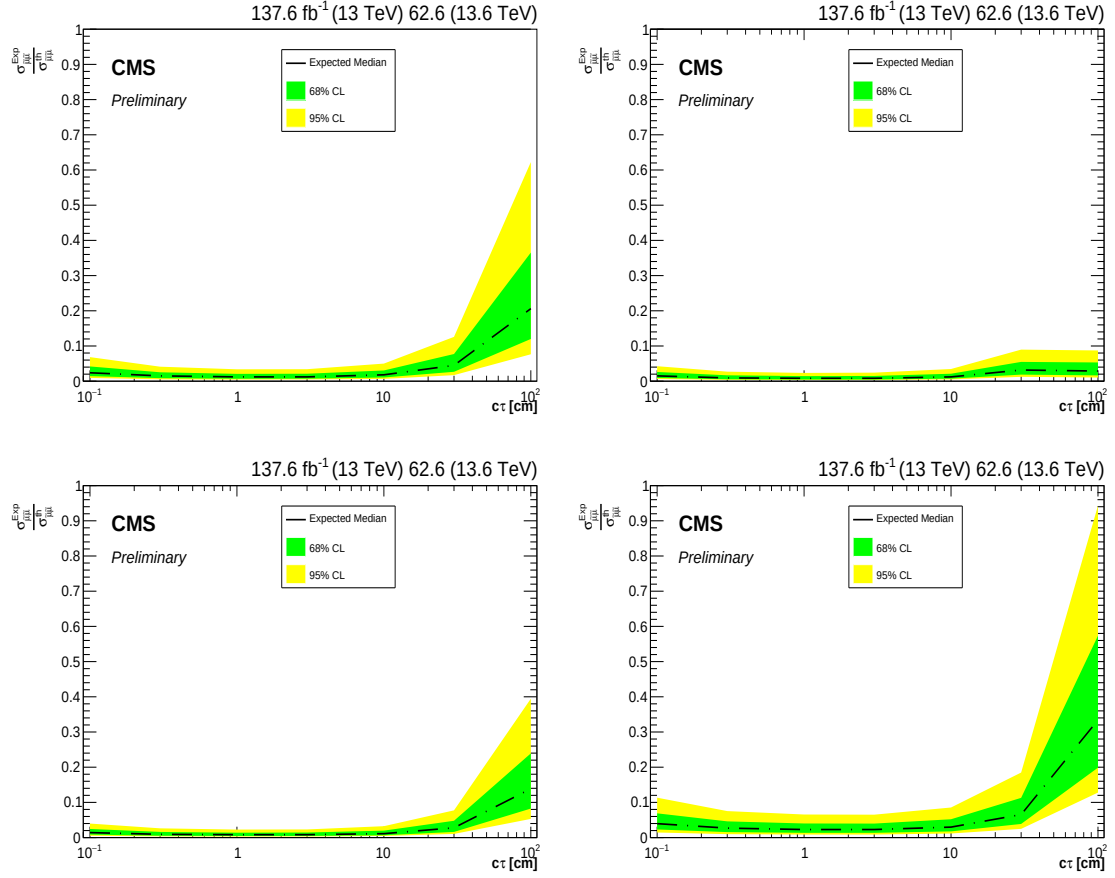
Figure G.1: \sigma_{\mu\tilde{\mu}} \times B_r(\tilde{\mu} \rightarrow \mu\tilde{\chi}_1^0)^2 assuming different mass combinations between the smuon and the neutralino S_{m\tilde{\chi}_1^0}^{m\tilde{\mu}} : (upper left) S_{180}^{200} (upper right) S_{180}^{250} (lower left) S_{200}^{250} (lower right) S_{230}^{250} . Signal samples for which the ratio of the cross sections is below 1 are excluded.
