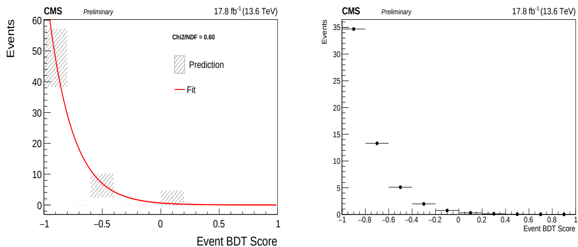
Figure F.6: (left) Fit of the background estimate in the signal region for 2023-pre \mu\mu data. (right) Toy experiments generated injected in the COMBINE tool to extract expected limits.
