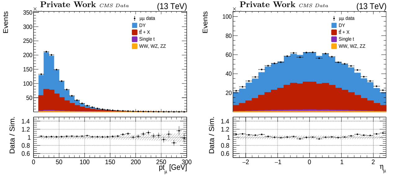
Figure 4.17: p_T and \eta of the muons in the 2018 \mu\mu data and MC. The hatched bands represent the systematic uncertainties.
