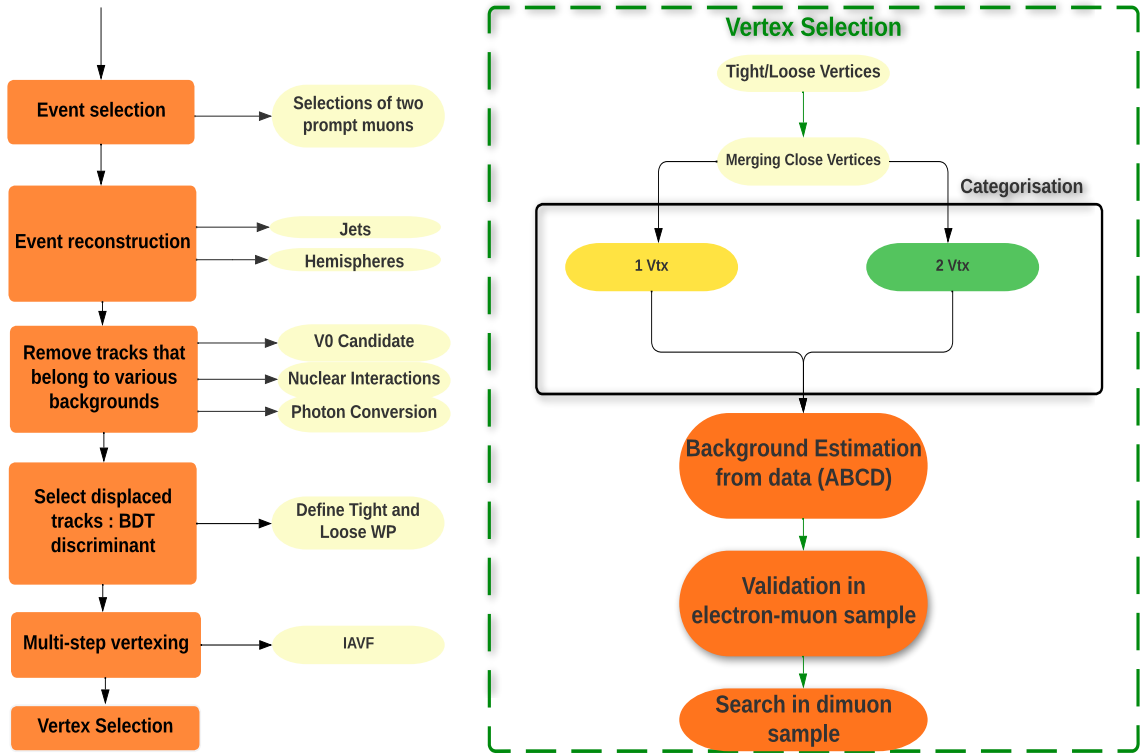
Figure 4.1: Schematic view of the analysis strategy.
