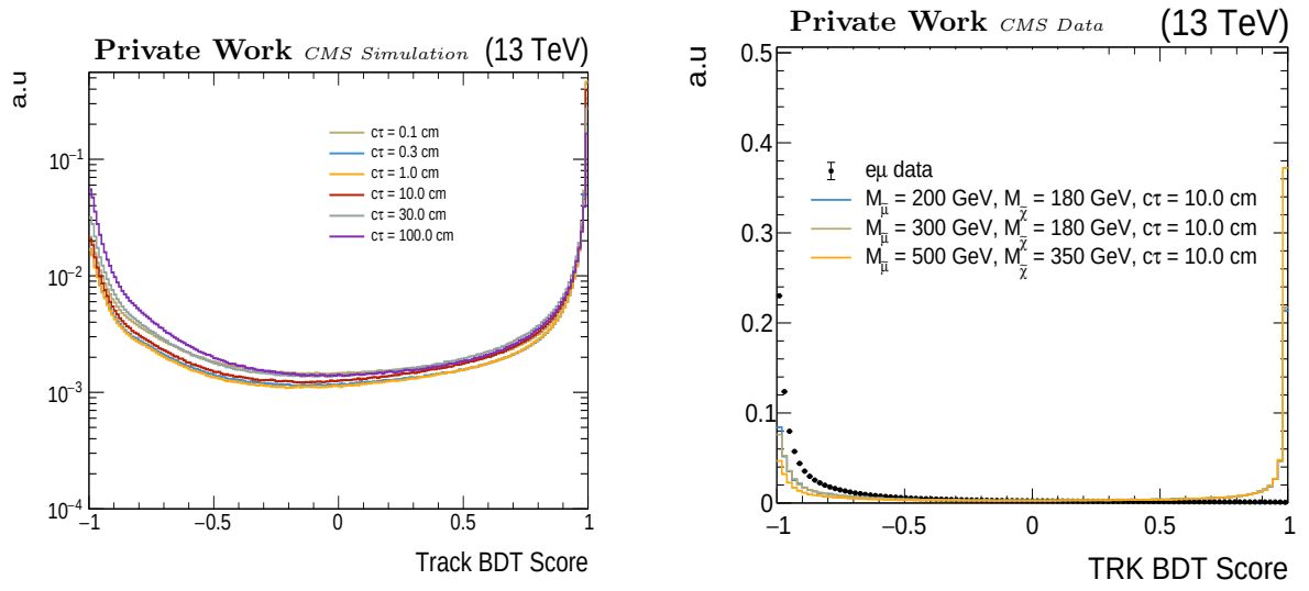
Figure 4.32: Track selection BDT output for all selected tracks in (left) signal events with different c\tau_{\tilde{\chi}} and (right) by comparing signal events and e\mu data.
