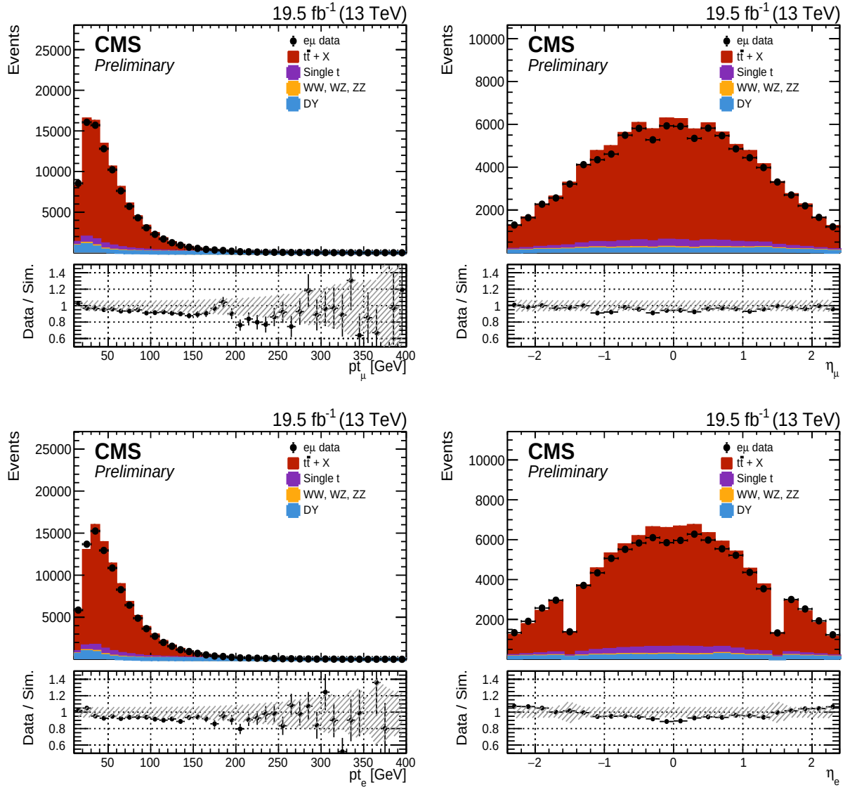
Figure D.3: p_T and \eta of the muons and electrons in the 2016-pre e\mu data and MC. The hatched bands represent the systematic uncertainties.
