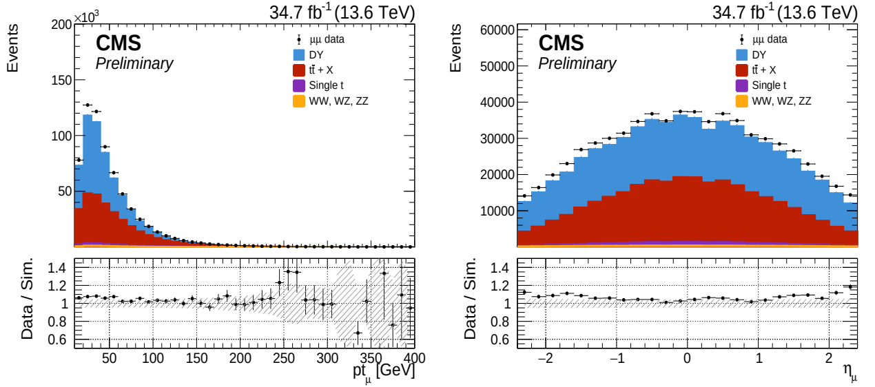
Figure D.29: p_T and \eta of the muons in the 2022 \mu\mu data and MC. The hatched bands represent the systematic uncertainties.
