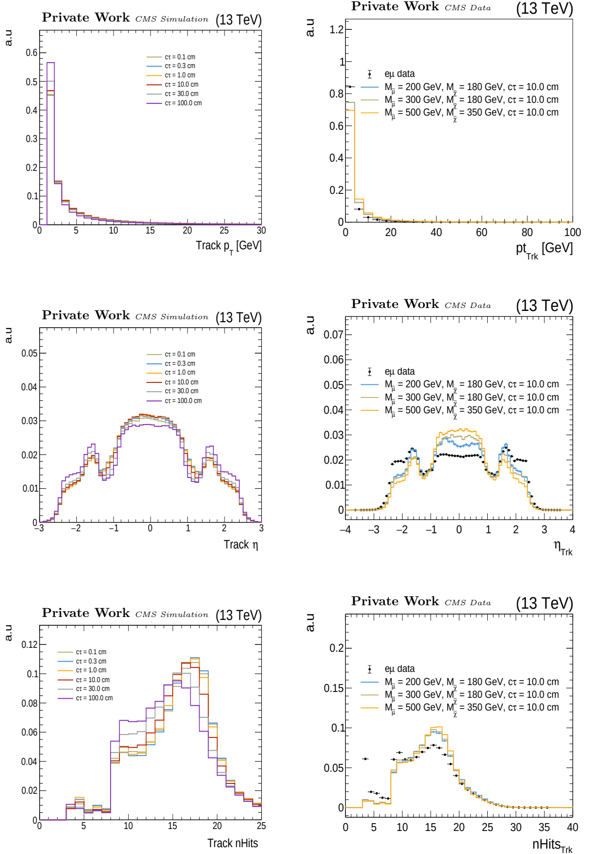
Figure 4.26: Input variables to the BDT. The left column shows the signal distribution for different c\tau_{\tilde{\chi}} while the right column shows the comparison between signal and e\mu data.
