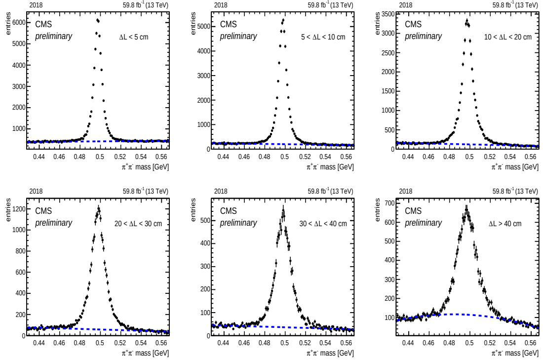
Figure E.6: Invariant mass of K_S candidates from the e\mu data sample in 2018 for various vertex displacements. The dashed line is the background fit from the tails.
