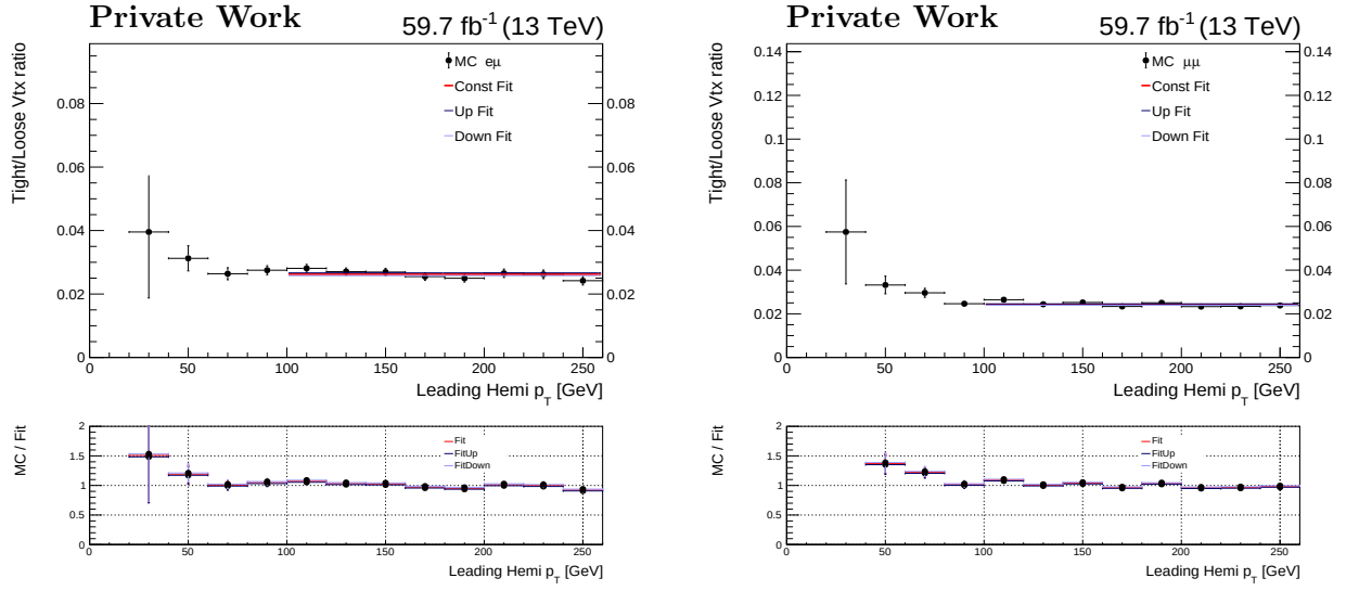
Figure 5.18: Ratio of the number of tight over loose vertices as a function of the p_T of the leading hemisphere in the 2018 (left) e\mu MC and (right) \mu\mu MC.
