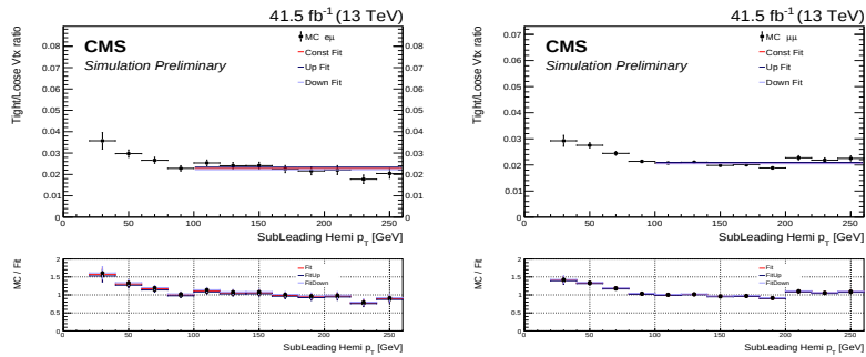
Figure D.24: Ratio of the number of tight over loose vertices as a function of the p_T of the sub-leading hemisphere in the 2017 (left) e\mu MC and (right) \mu\mu MC.
