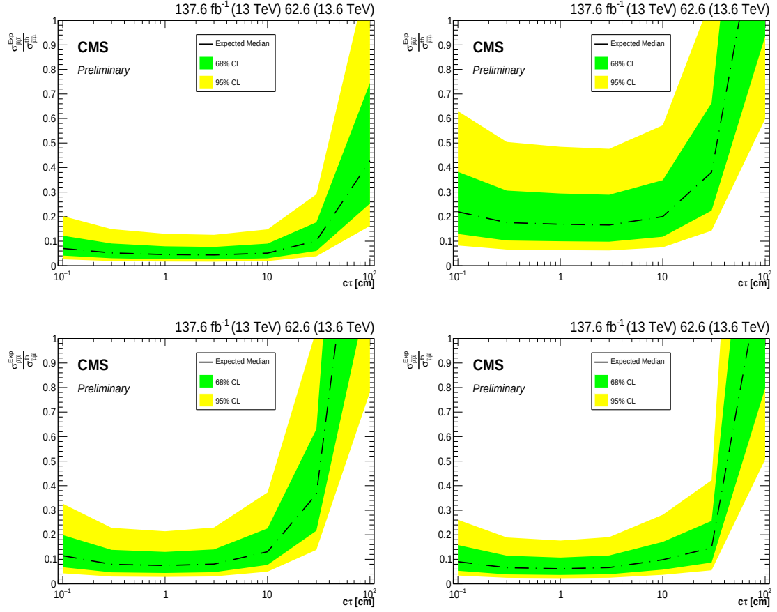
Figure G.5: \sigma_{\tilde{\mu}\tilde{\mu}} \times B_r(\tilde{\mu} \rightarrow \mu\tilde{\chi}_1^0)^2 assuming different mass combinations between the smuon and the neutralino S_{m\tilde{\chi}_1^0}^{m\tilde{\mu}} : (upper left) S_{350}^{400} (upper right) S_{380}^{400} (lower left) S_{180}^{450} (lower right) S_{200}^{450} . Signal samples for which the ratio of the cross sections is below 1 are excluded.
