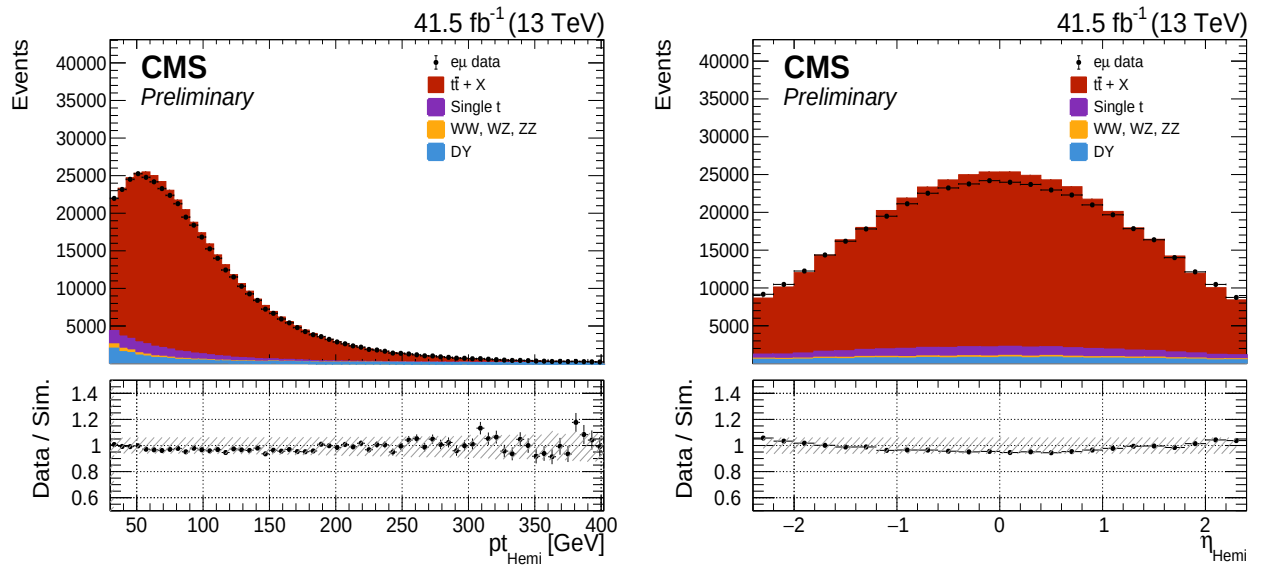
Figure D.18: p_T and \eta of the hemispheres in the 2017 e\mu data and MC. The hatched bands represent the systematic uncertainties.
