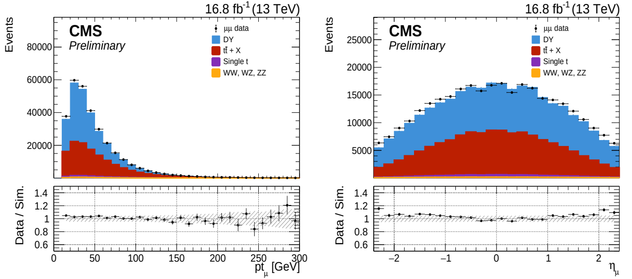
Figure D.13: p_T and \eta of the muons in the 2016-post \mu\mu data and MC. The hatched bands represent the systematic uncertainties.
