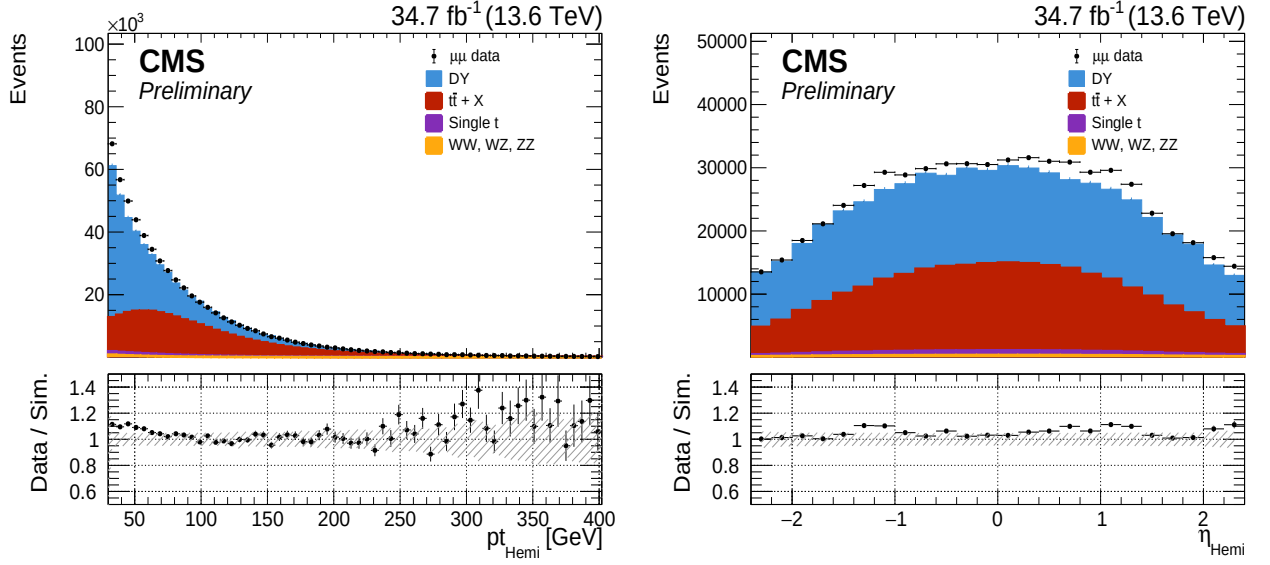
Figure D.28: p_T and \eta of the hemispheres in the 2022 \mu\mu data and MC. The hatched bands represent the systematic uncertainties.
