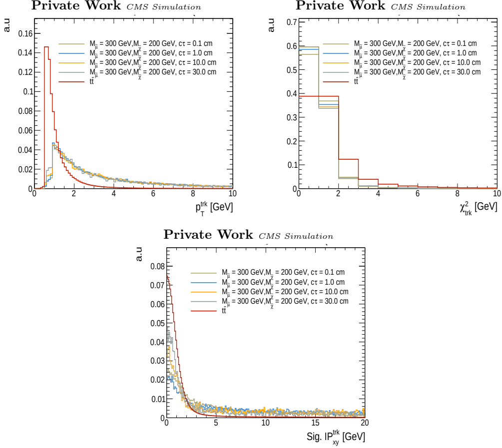
Figure 4.23: Track (upper left) p_T , (upper right) \chi^2_{\text{trk}}/\text{dof} and (lower) impact parameter significance for displaced signal tracks and tracks from t\bar{t} events in 2018 MC conditions. Distributions are normalized to unit area.
