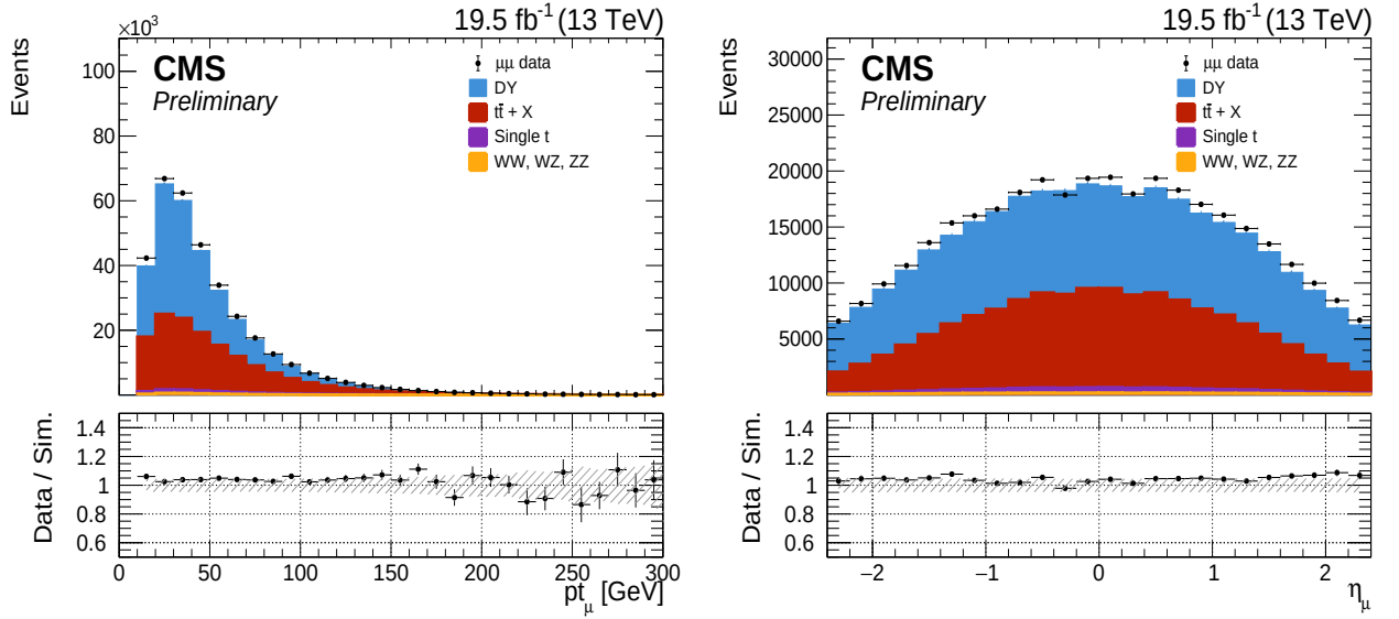
Figure D.5: p_T and \eta of the muons in the 2016-pre \mu\mu data and MC. The hatched bands represent the systematic uncertainties.
