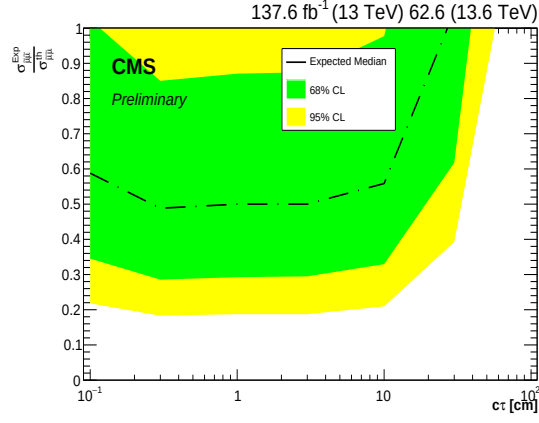
Figure G.9: \sigma_{\tilde{\mu}\tilde{\mu}} \times B_r(\tilde{\mu} \rightarrow \mu\tilde{\chi}_1^0)^2 assuming a mass combination between the smuon and the neutralino S_{m_{\tilde{\chi}_1^0}}^{m_{\tilde{\mu}}}: S_{480}^{500} . Signal samples for which the ratio of the cross sections is below 1 are excluded.
