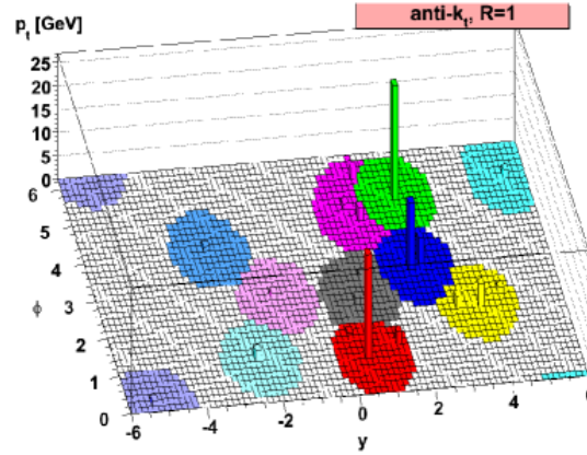
Figure 1.22: Output of the anti- k_t algorithm in the rapidity-azimuth plane as a function of the transverse momentum of the jets [51].
