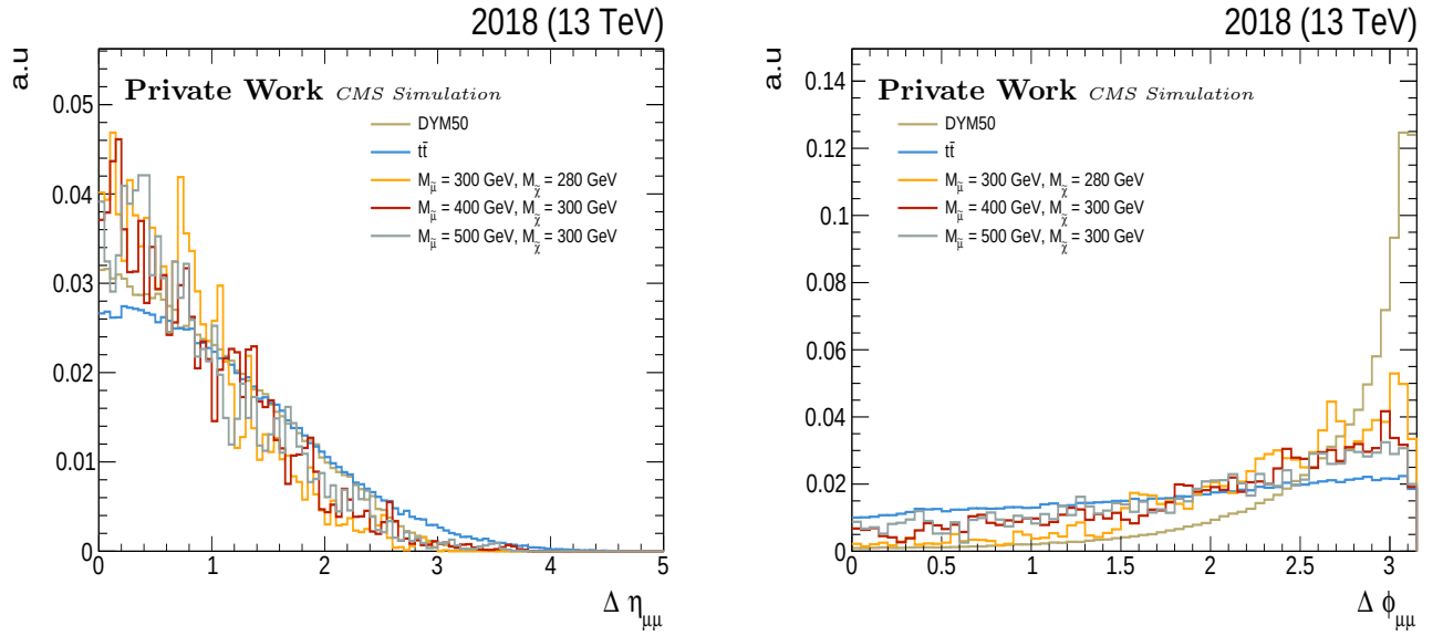
Figure 4.5: \Delta\eta and \Delta\phi distributions between the leading and sub-leading muon in MC signal events, Drell-Yan and t\bar{t} events in 2018 conditions.
