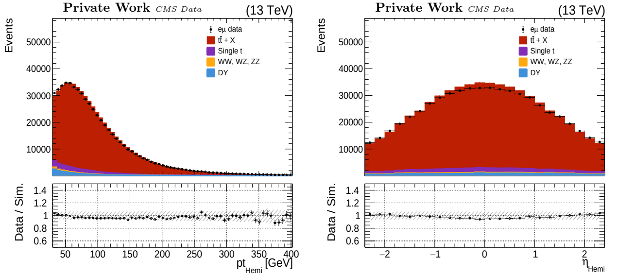
Figure 4.14: p_T and \eta of the hemispheres in the 2018 e\mu data and MC. The hatched bands represent the systematic uncertainties.
