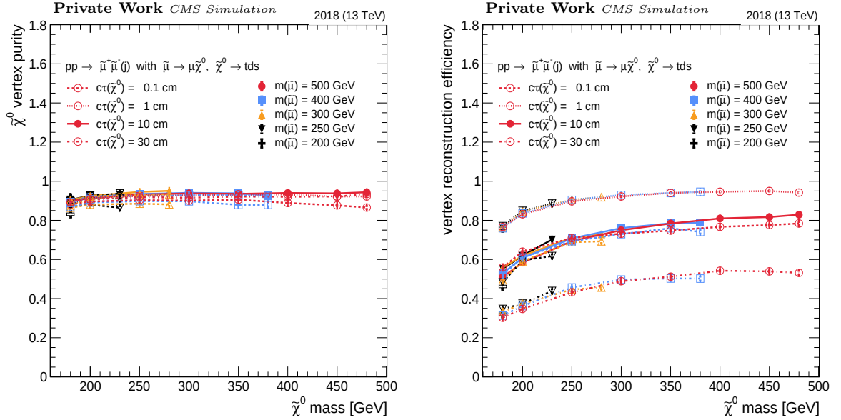
Figure 5.7: The (left) purity and (right) efficiency of the tight reconstructed displaced vertices as a function of the masses of the neutralino and smuon for different neutralino c\tau_{\tilde{\chi}} in the 2018 MC conditions.
