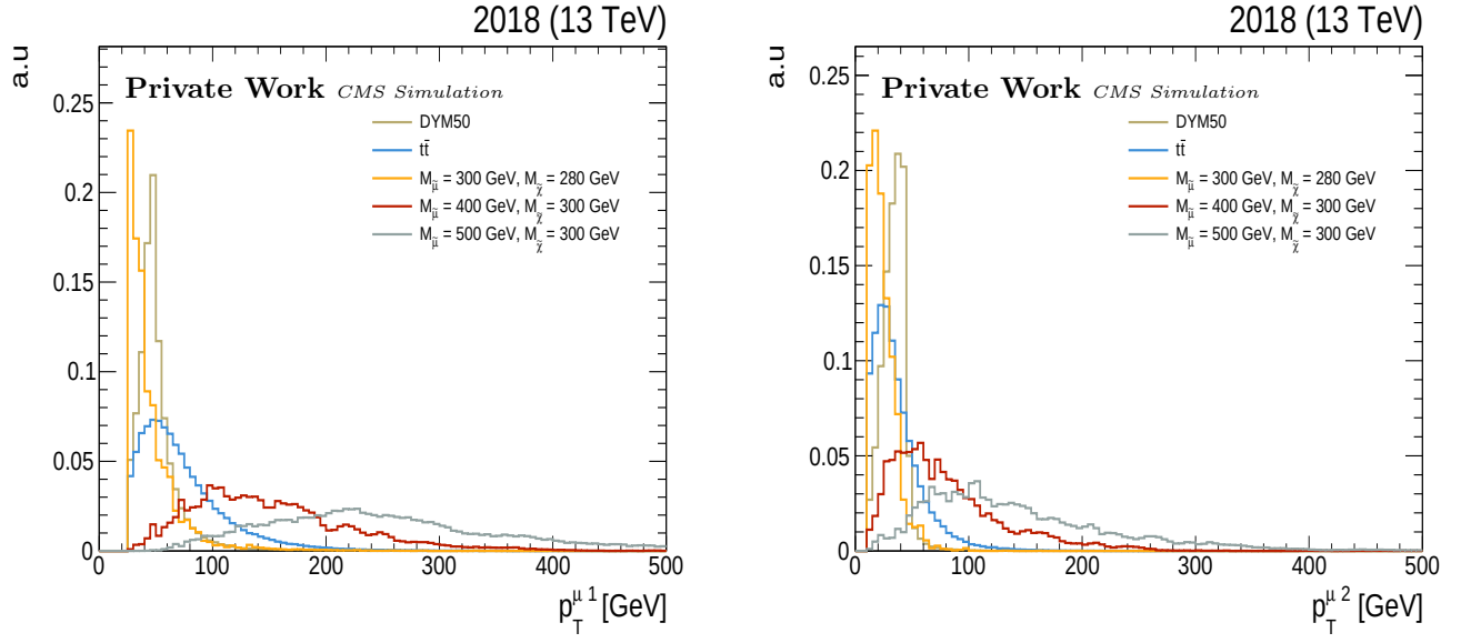
Figure 4.4: Distributions of the leading and sub-leading muon p_T in MC signal events, Drell-Yan and t\bar{t} events in the 2018 conditions.
