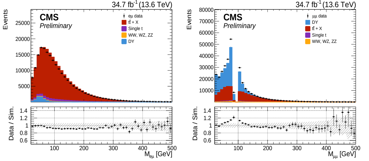
Figure D.25: For 2022 data and MC, invariant mass of the lepton pair in the (left) e\mu and (right) \mu\mu samples. The hatched bands represent the systematic uncertainties.
