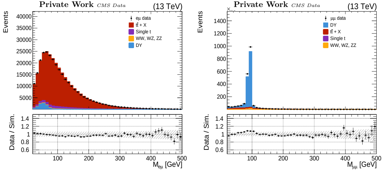
Figure 4.13: For 2018 data and MC, invariant mass of the lepton pair in the (left) e\mu and (right) \mu\mu samples. The hatched bands represent the systematic uncertainties.
