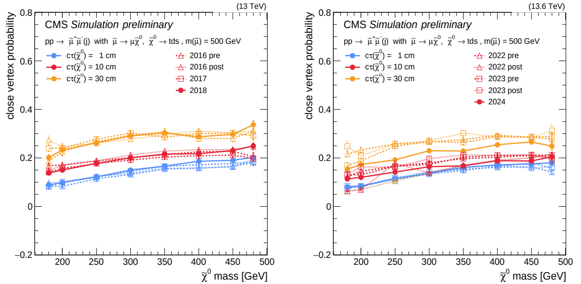
Figure C.3: Probability of having two close (below their resolution) vertices, one being tight, as a function of the neutralino and smuon masses and c\tau_{\tilde{\chi}} in each MC year period of (left) Run 2 and (right) Run 3.
