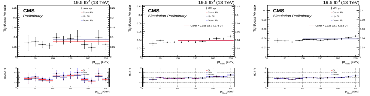
Figure D.6: Ratio of the number of tight over loose vertices as a function of the p_T of the hemispheres in the 2016-pre (left) e\mu data, (middle) e\mu MC and (right) \mu\mu MC.
