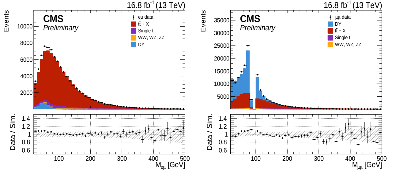
Figure D.9: For 2016-post data and MC, invariant mass of the lepton pair in the (left) e\mu and (right) \mu\mu samples. The hatched bands represent the systematic uncertainties.
