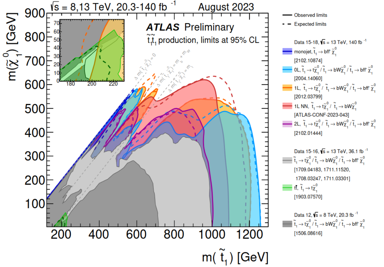
Figure 3.14: A summary of the 95% CL. exclusion contours in the stop-neutralino mass plane for various possible decay chains, including two-, three- and four-body decays, as obtained in dedicated analyses by ATLAS, see Section 89.6 of [68]. The results are combining Run 1 and Run 2 results.
