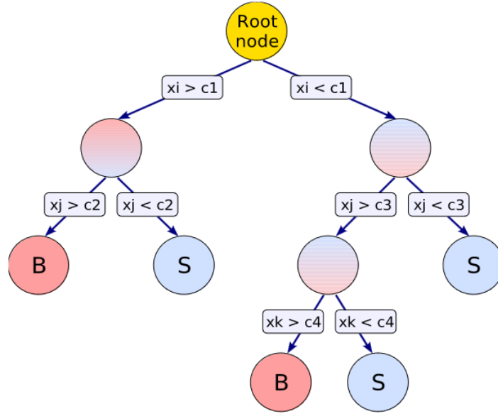
Figure 4.24: Example of a Boosted Decision Tree with the final leaves labeled as "S" for signal and "B" for background, borrowed from [169]. The x_i and x_j are variables used as an input to the BDT.
