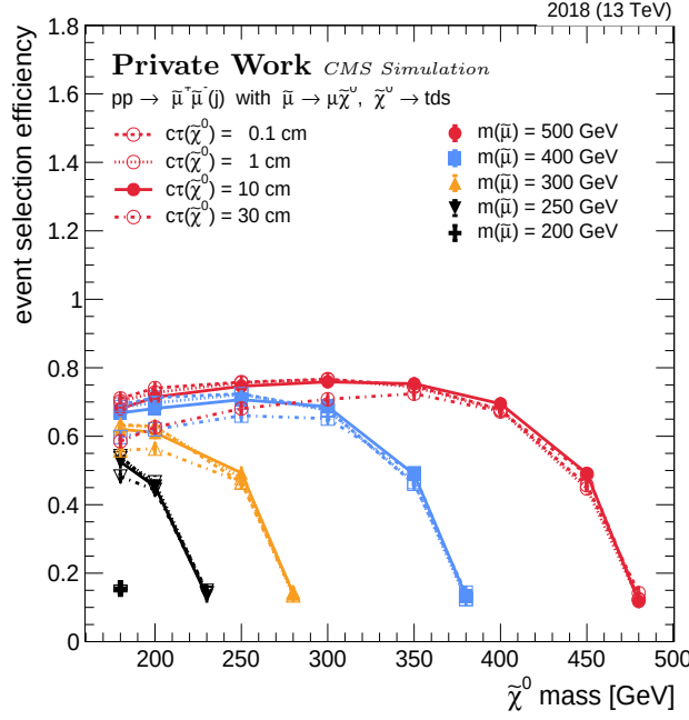
Figure 4.12: Efficiency for signal events to pass the event selection as a function of the neutralino and smuon masses and neutralino lifetime in the 2018 MC conditions.
