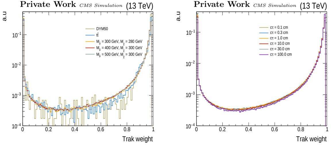
Figure 5.9: Example of the distribution (left) of the track weight for three MC signal sample, the DY and t\bar{t} background. Same distribution (right) for signal samples with different c\tau_{\tilde{\chi}} .
