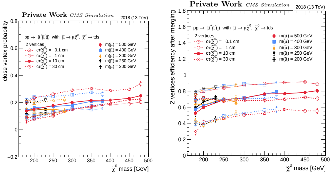
Figure 5.5: Left: probability of having two close (below their resolution) vertices, one being tight. Right: probability to reconstruct another tight displaced vertex. Figures are shown as a function of the neutralino mass for different values of the neutralino c\tau_{\tilde{\chi}} and smuon mass in the 2018 MC conditions.
