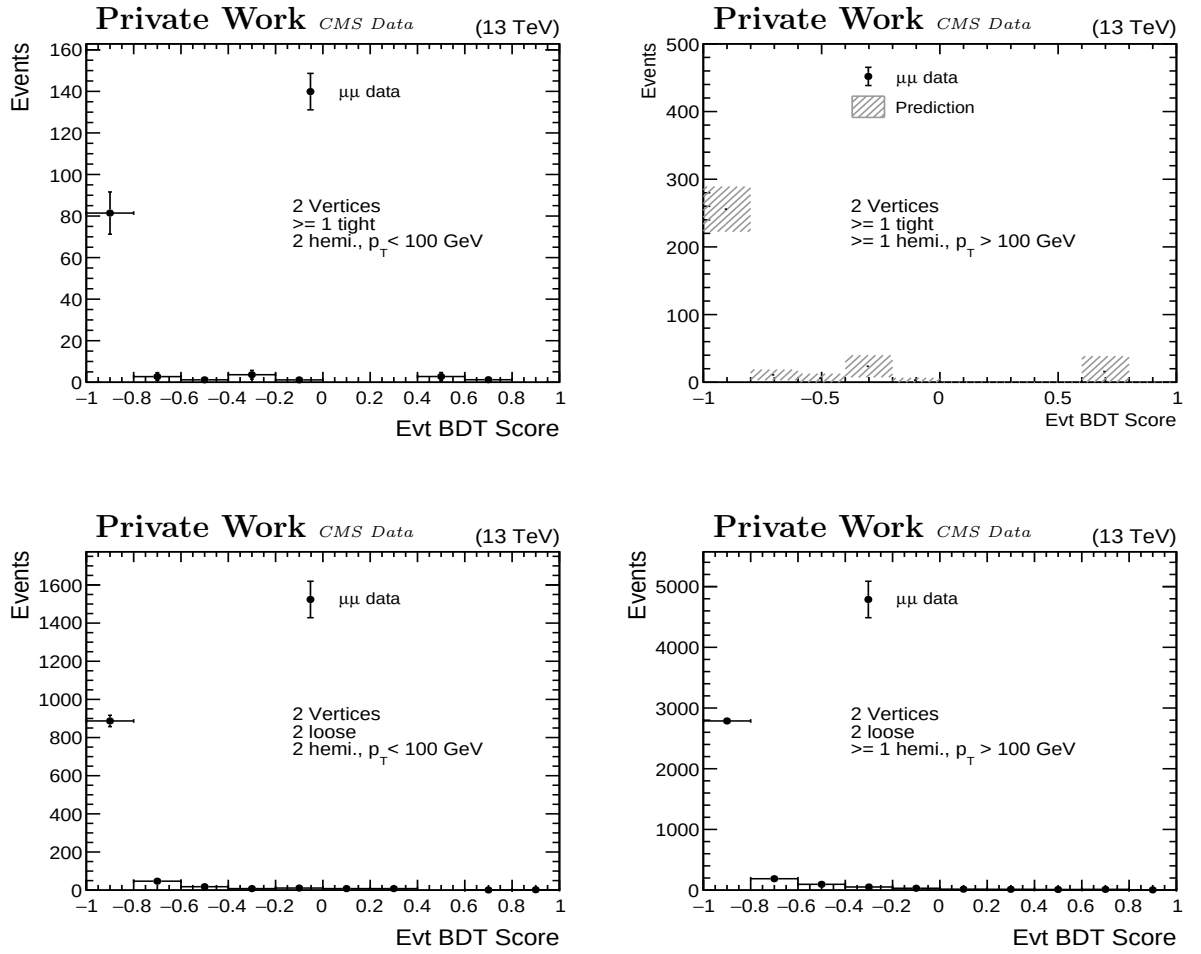
Figure 5.22: Background estimation method applied to the 2018 \mu\mu sample, with blinded SR, taking into account the correction associated with the correlation.
