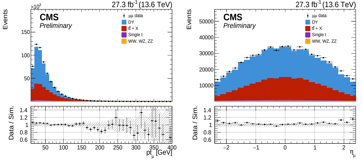
Figure D.40: p_T and \eta of the muons in the 2023 \mu\mu data and MC. The hatched bands represent the systematic uncertainties.
