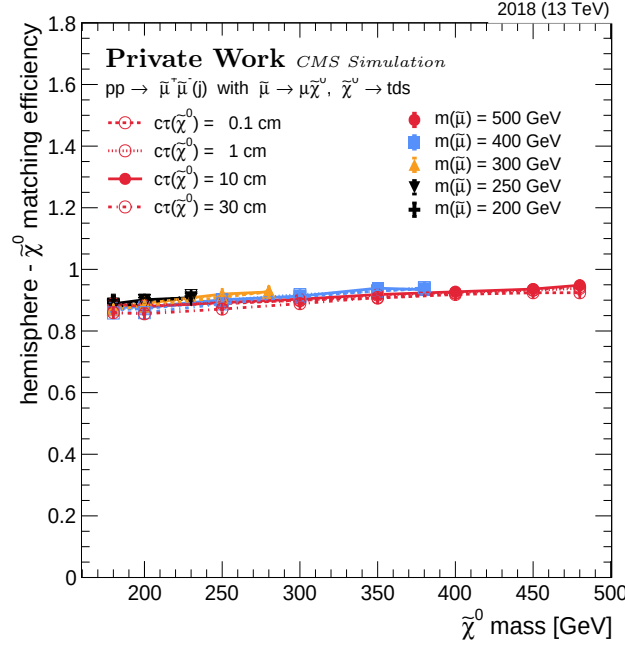
Figure 4.11: Efficiency to match the reconstructed hemisphere axis and the nearest generated neutralino direction ( \Delta R < 1.5 ) as a function of the neutralino and smuon masses and neutralino lifetime in the 2018 MC conditions.
