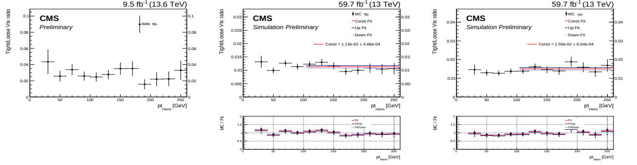
Figure D.44: Ratio of the number of tight over loose vertices as a function of the p_T of the hemispheres in the 2023-post (left) e\mu data, (middle) e\mu MC and (right) \mu\mu MC.
