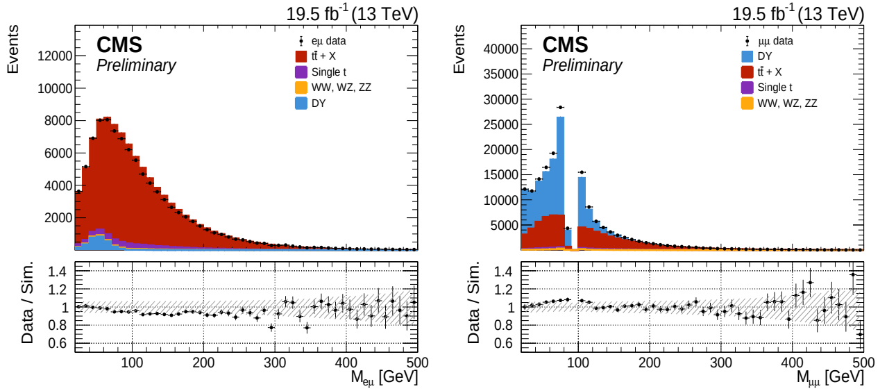
Figure D.1: For 2016-pre data and MC, invariant mass of the lepton pair in the (left) e\mu and (right) \mu\mu samples. The hatched bands represent the systematic uncertainties.
