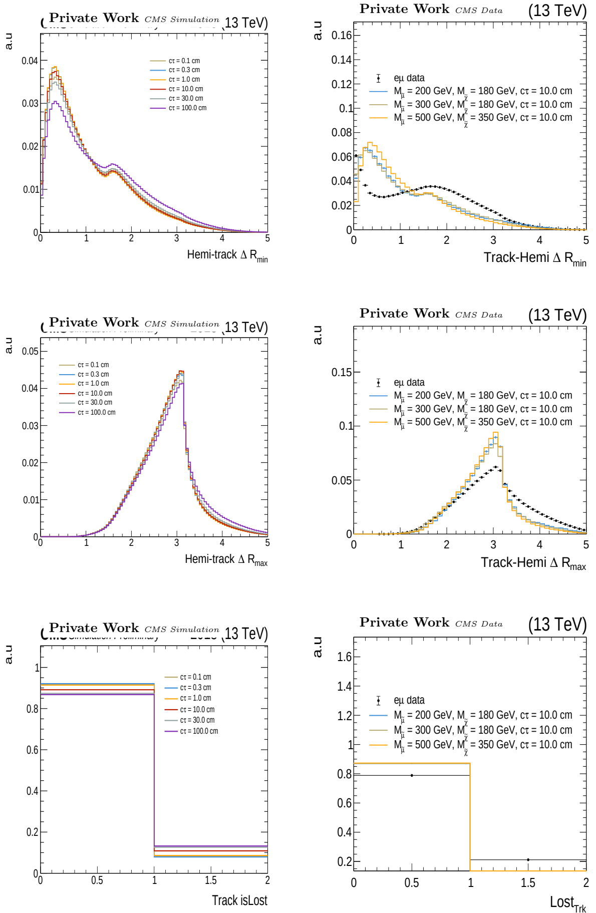
Figure 4.29: Input variables to the BDT. The left column shows the signal
