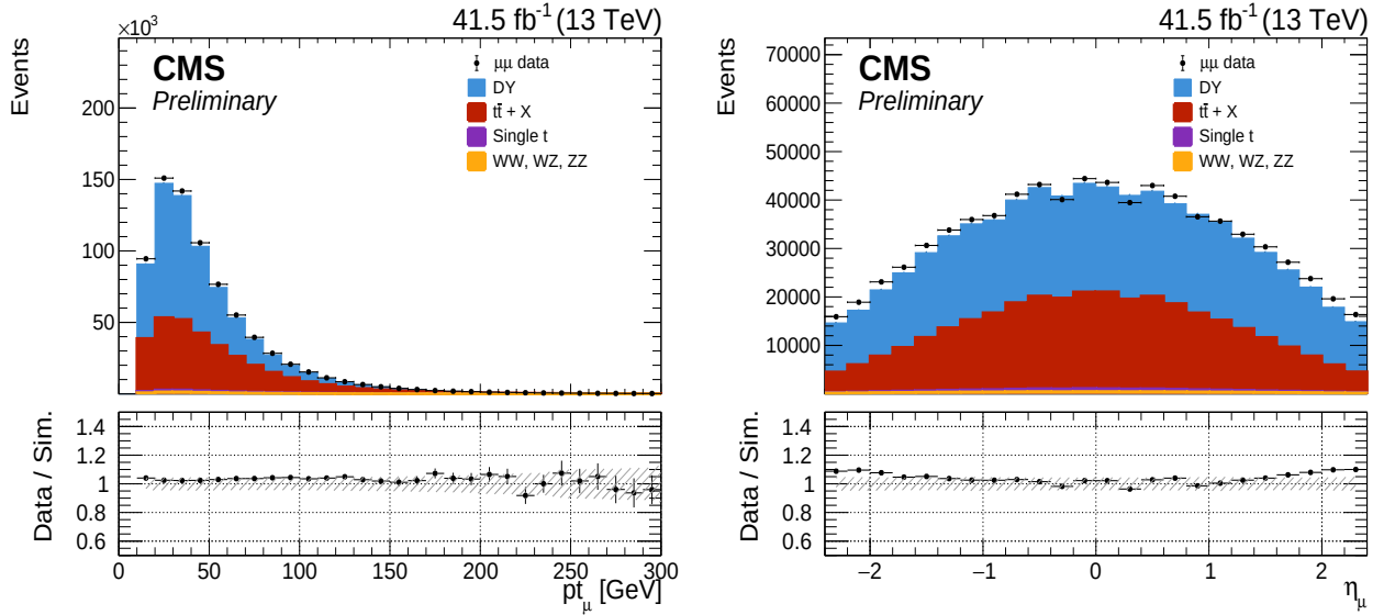
Figure D.21: p_T and \eta of the muons in the 2017 \mu\mu data and MC. The hatched bands represent the systematic uncertainties.
