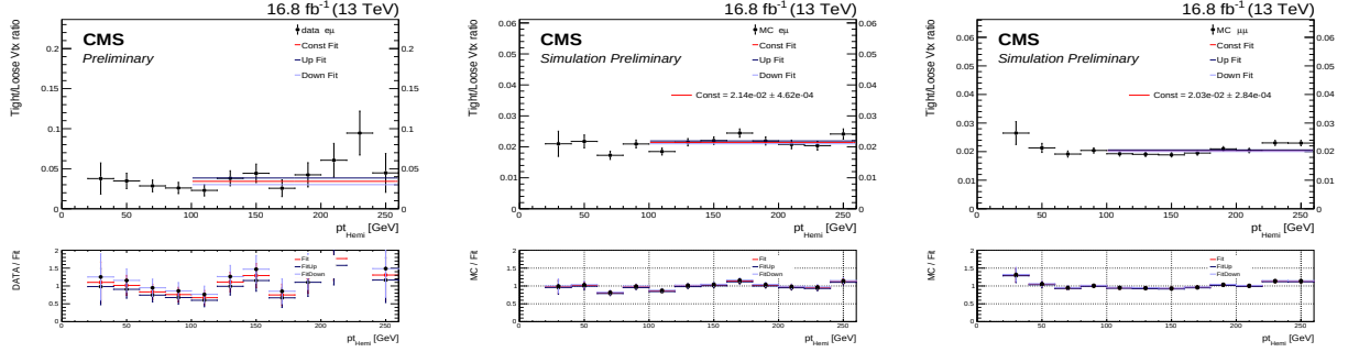
Figure D.14: Ratio of the number of tight over loose vertices as a function of the p_T of the hemispheres in the 2016-post (left) e\mu data, (middle) e\mu MC and (right) \mu\mu MC.
