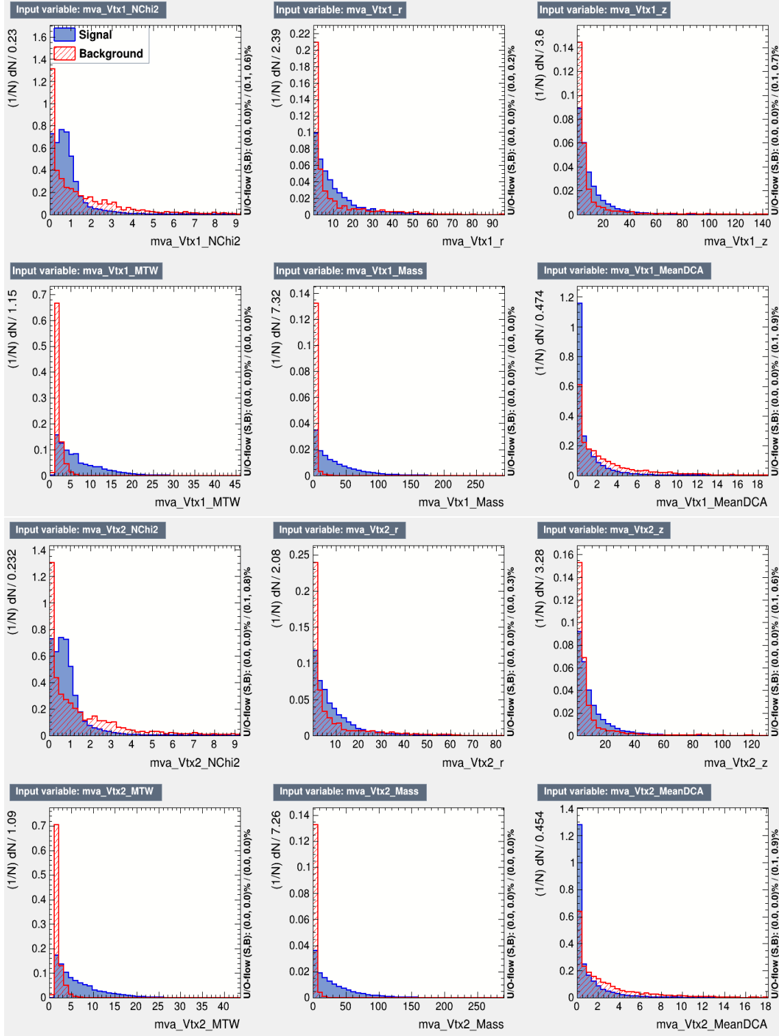
Figure 5.12: Input variables of the vertex BDT for 2018. The signal vertices are from the c\tau_{\tilde{\chi}} = 10 cm sample, while the background vertices are from the e\mu data sample. The MTW variable refers to the sum of the weight of the tracks at vertex.
