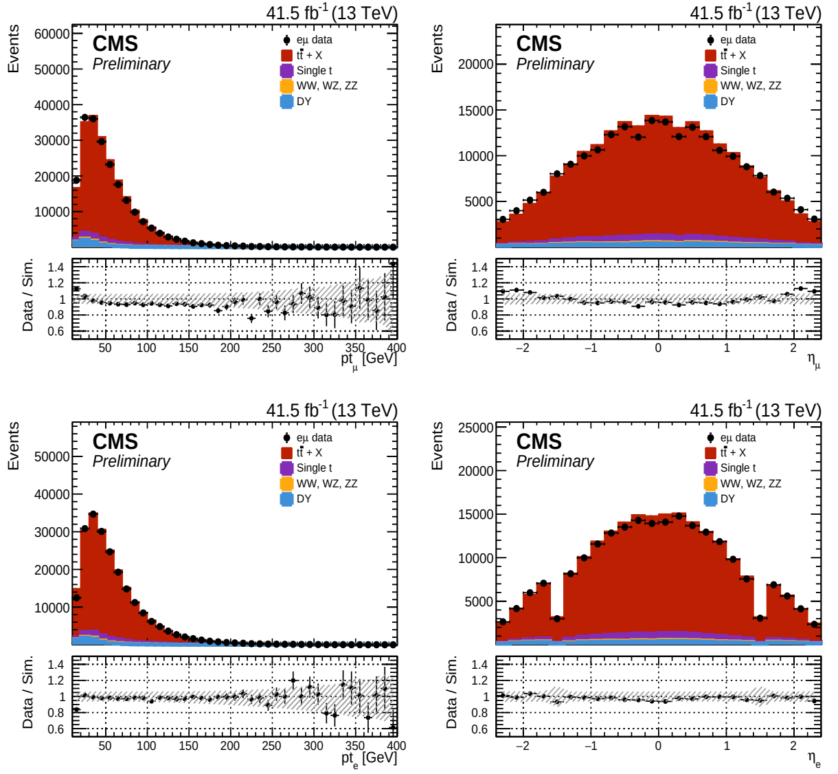
Figure D.19: p_T and \eta of the muons and electrons in the 2017 e\mu data and MC. The hatched bands represent the systematic uncertainties.
