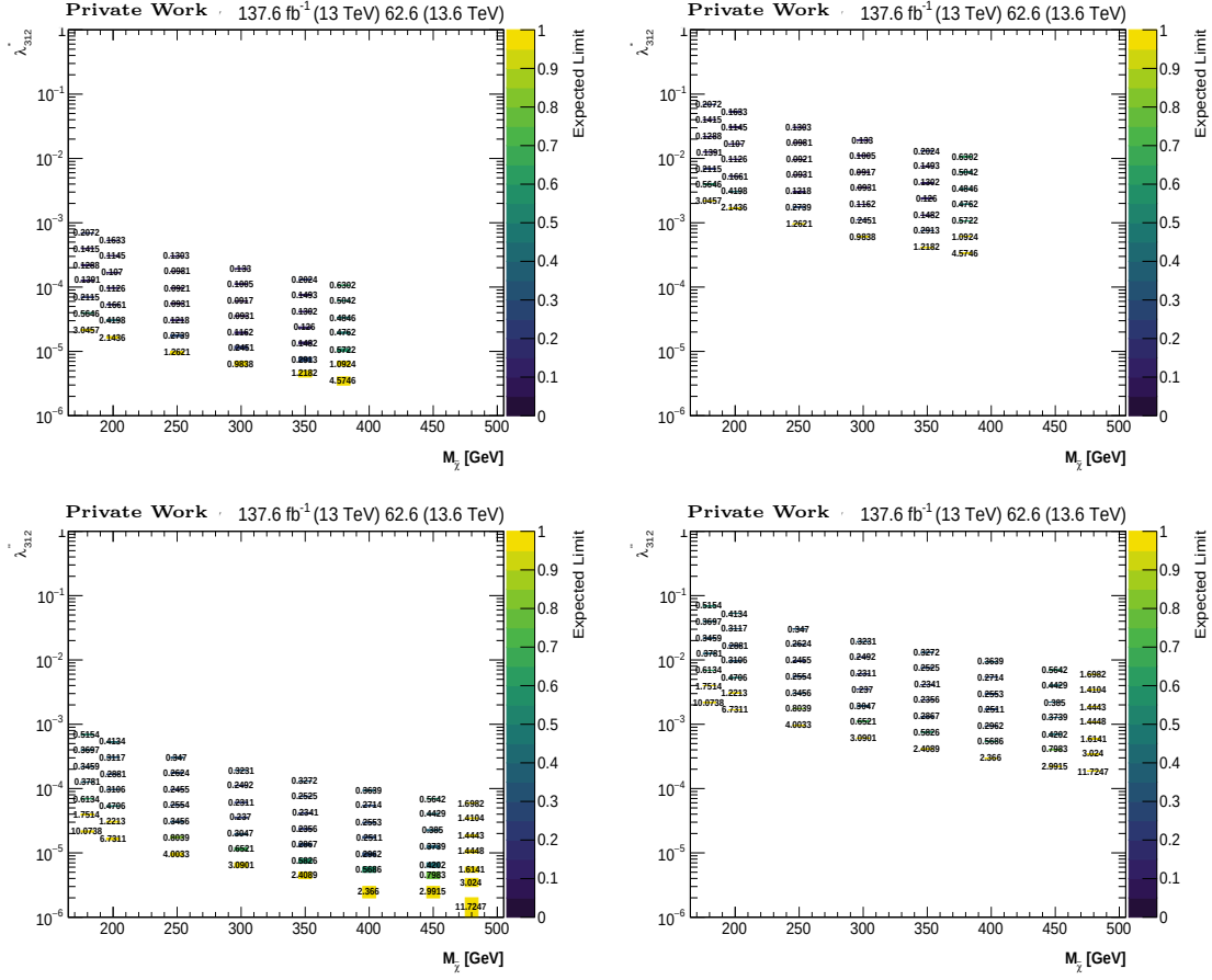
Figure 5.31: \lambda''_{312} vs M_{\tilde{\chi}_1^0} expected limits at a 95% confidence level assuming different stop masses of (left) 1 TeV and (right) 10 TeV and smuon masses (upper) 400 GeV (lower) 500 GeV. The z -axis is the ratio of the expected cross section over the theoretical one. Signal samples with z -axis values below 1 are excluded. The center of each bin corresponds to a specific signal sample. The upper and lower values of \lambda'' correspond to the tracker bounds of CMS following Eq.3.48.
