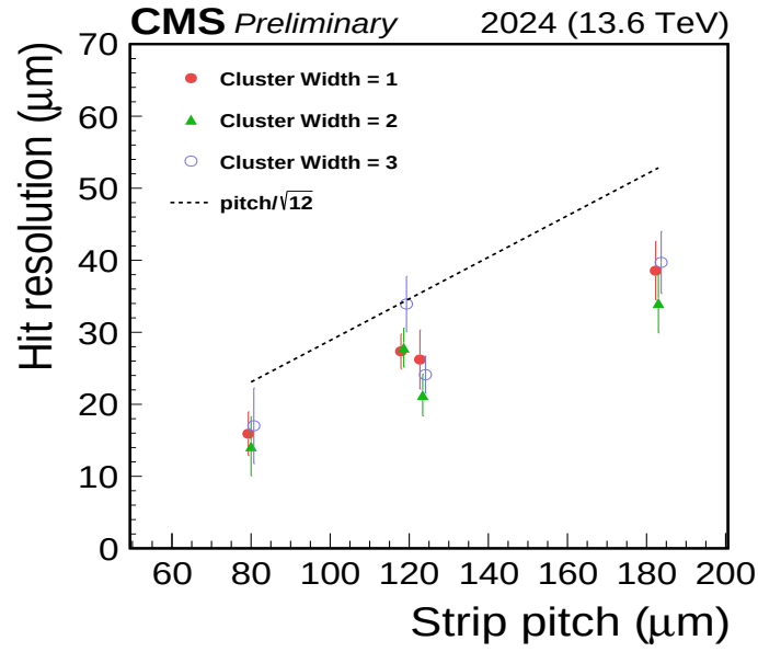
Figure 1.17: Strip hit resolution is shown for an early 2024 13.6 TeV pp collisions run where the silicon strip tracker was operated in nominal conditions and cooled down to -22^{\circ}\text{C} . The strip hit resolution is derived by selecting pairs of hits in different types of overlapping sensors and for different cluster widths expressed in units of number of strips. The theoretically expected resolution from a binary readout tracking detector (i.e., hit or no hit) is also displayed. By measuring the fraction of charge collected by adjacent strips, the hit position can be interpolated more precisely, leading to a resolution significantly better than the binary limit [43].
