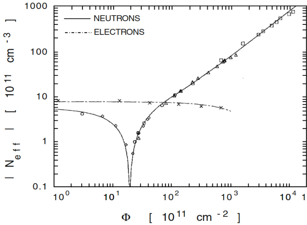
Figure 2.5: Fluence dependence of the magnitude of the effective doping for an n-type silicon wafer irradiated with 1 MeV neutrons equivalent. Also shown is the much smaller effect of irradiation with 1.8 MeV electrons also scaled to 1 MeV neutron equivalent NIEL. [69] .
