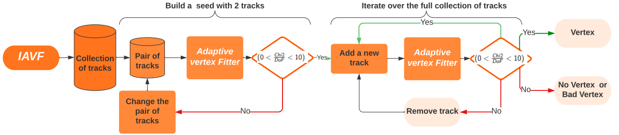
Figure 5.2: Visual representation of the IAVF algorithm
