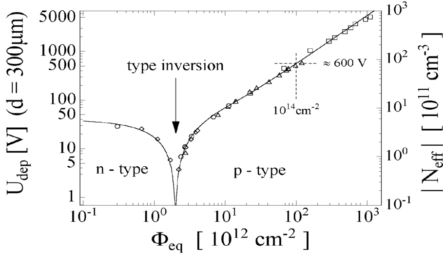
Figure 2.7: Change in the depletion voltage and in the absolute effective doping concentration as measured immediately after irradiation for a 300 \mu m -wide sensor [73].
