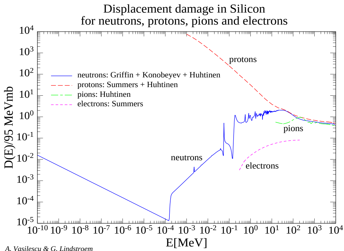
Figure 2.4: NIEL cross sections normalized to 95 \text{ MeV} \cdot \text{mb} for protons, neutrons, electrons and pions [72].
