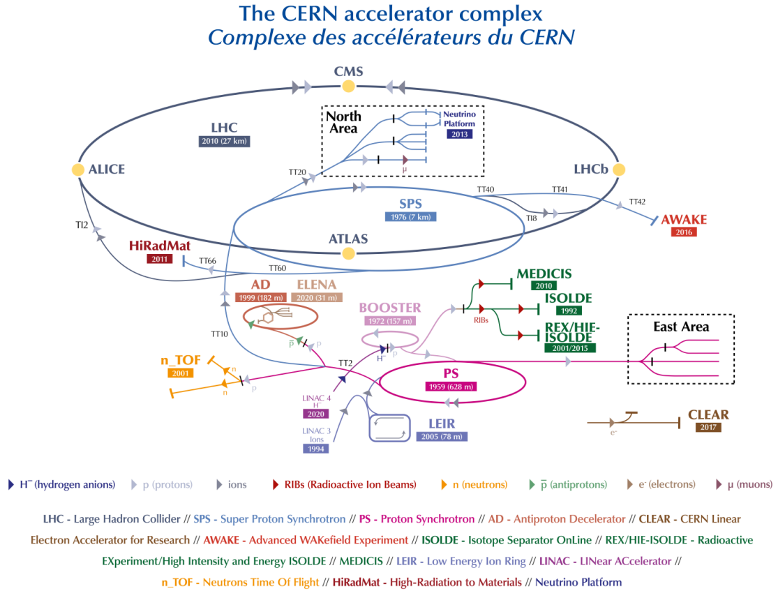
Figure 1.1: CERN accelerator complex [2].
