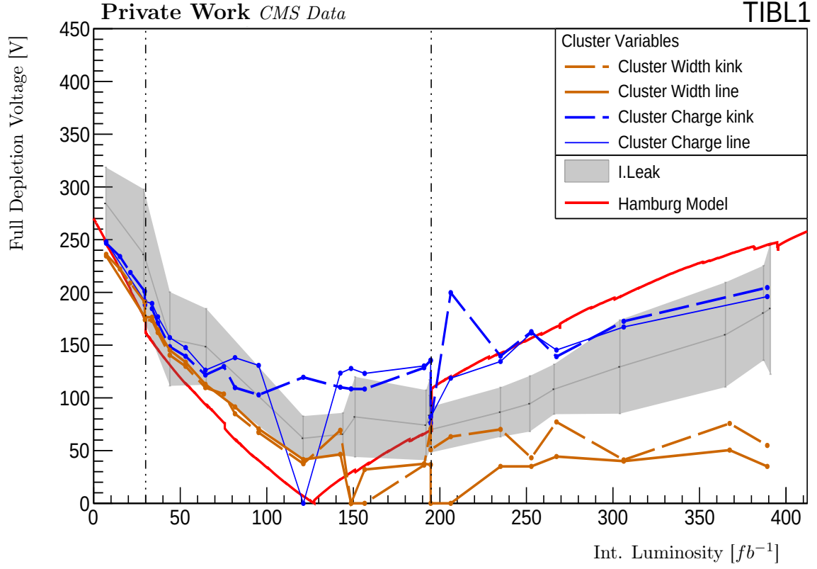
Figure 2.26: Full depletion voltage as a function of the integrated luminosity from the beginning of the operations of the LHC up to the end of 2024 in small scans. The values extracted from the three observables are shown with the cluster width and the cluster charge displayed with both extraction methods. The gray band corresponds to the extrema of the ten different fit functions on the leakage current curves. The predicted behavior from the Hamburg model is shown in red. The cluster curves reach 0 when the extraction method could not converge. The black dashed vertical lines show the LS1 ( \sim 30 \text{ fb}^{-1} ) and the LS2 ( \sim 200 \text{ fb}^{-1} ). The final data point corresponds to the last scan before 2025 operations. The see-saw effects observed around LS2 is not clearly understood. The uncertainty on the cluster curves is about 20-30 V as it arises from the statistical limitations of the small scans.
