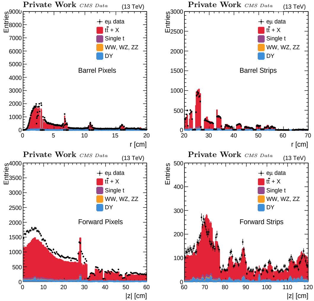
Figure 4.22: After veto on tracker material, remaining reconstructed secondary interactions in (upper) barrel ( |\eta| < 1.5 ) and (lower) endcaps ( |\eta| > 1.5 ) for 2018 data and MC e\mu samples.
