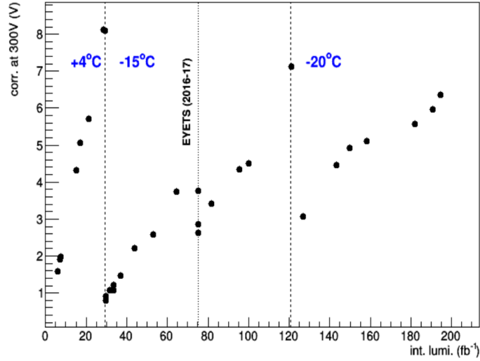
Figure 2.22: Evolution of the value of the voltage drop induced by the leakage current at 300 V for module 369121381 in TIB layer 1. The integrated luminosity at temperature transition time is shown by a dashed vertical line. The dotted vertical line points to the time of the extended year end technical stop of 2016 where the detector was at ambient temperature and annealing occurred [85].
