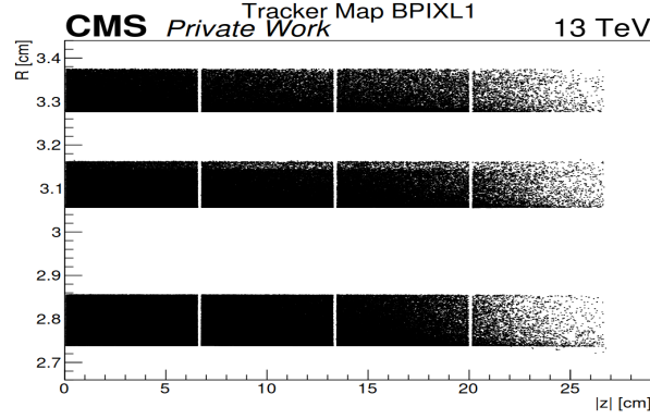
Figure 4.2: Example of the tracker BPIX L1 geometry built using the RECO data tier with the first hit of the tracks
