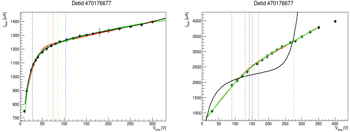
Figure 2.35: Leakage current curve of (left) 2018 and (right) end of 2024. The 2024 curve is almost non-exploitable as the shape is almost linear and fits start to fail.
