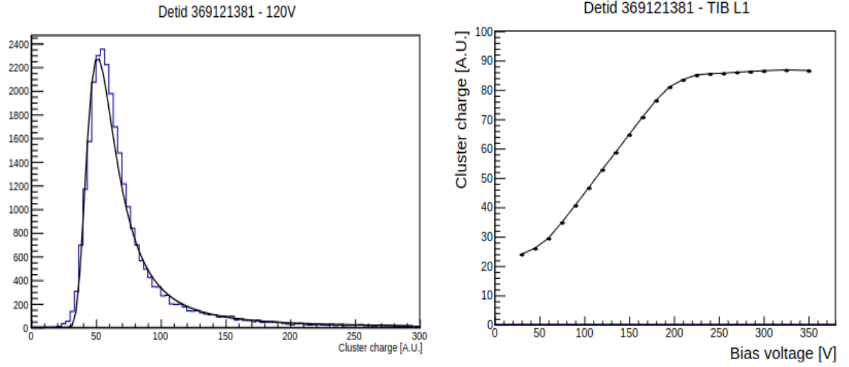
Figure 2.15: (Left) Distribution of the cluster charge at the step 120 V of the scan, (Right) Cluster charge curve as a function of the bias voltage. Both figures come from the same scan of August 2012 for a single TIB L1 module. The full depletion voltage is about 200 V [85].
