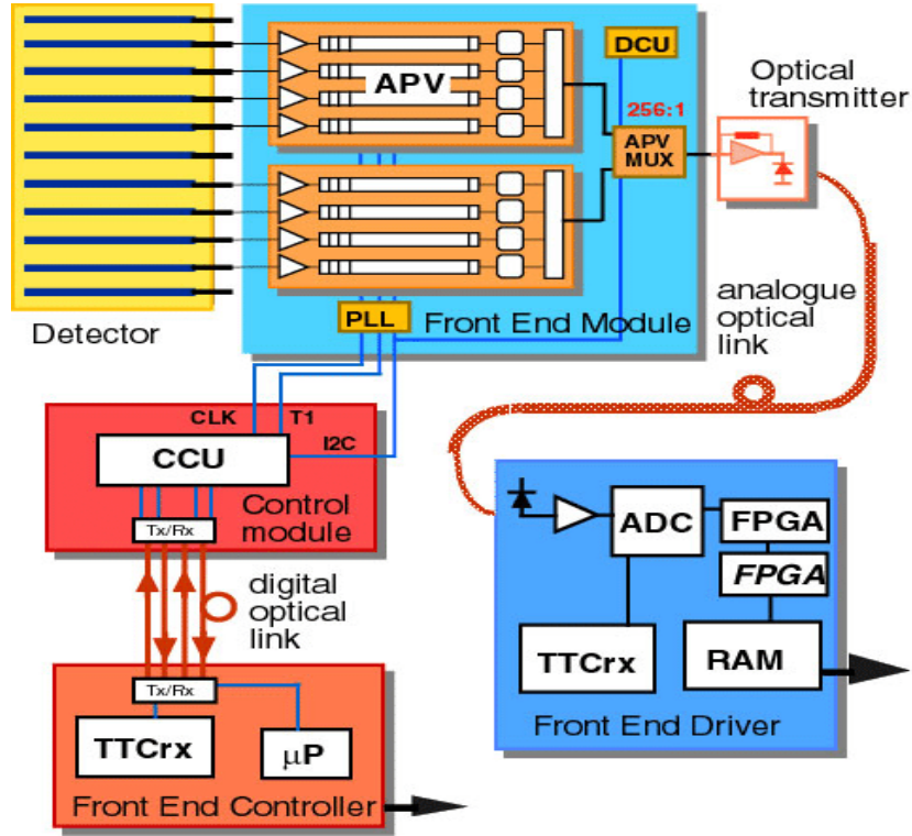
Figure 2.12: Scheme of the front end electronics of the silicon strip modules. [81].
