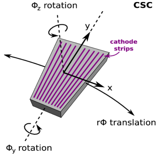
Figure 1.13: Coordinates and alignment parameters for a CSC chamber [32].
