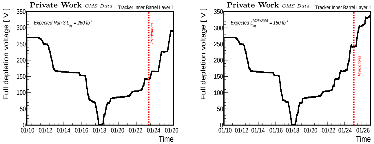
Figure 2.31: The CMS Strip Tracker full depletion voltage plot for Tracker Inner Barrel layer 1 (TIBL1) as a function of time. Predictions are given for an hypothetical module with characteristics (initial full depletion voltage and temperature) representative of all the modules of the layer. The doping type inversion from n to p is observed at the end of Run 2 for TIB L1. After data-taking periods when the full depletion voltage increases, a small reduction of the full depletion voltage is observed due to the beneficial annealing before the reverse annealing takes over.
