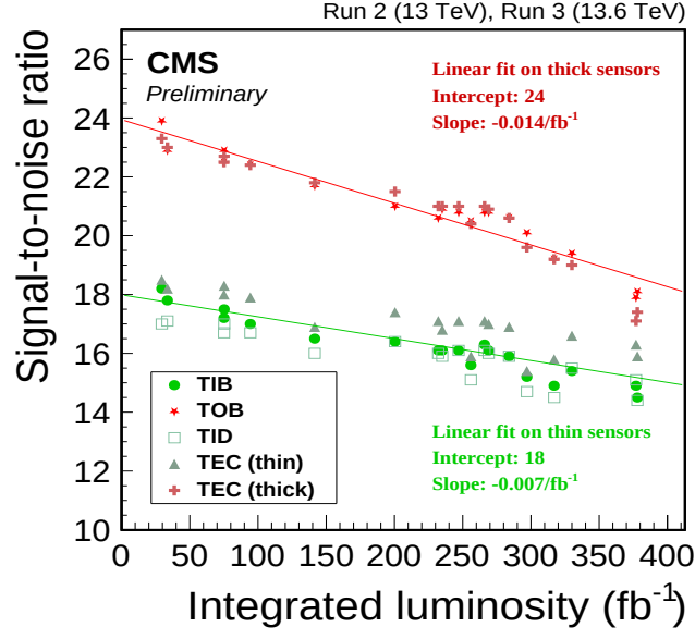
Figure 1.16: The overall signal-to-noise ratio of clusters ( S/N ) measured in pp collisions since Run 2 is reported as a function of the integrated delivered luminosity. Measurements have been performed split per sensor thickness in the Tracker endcaps ( 320 \mu\text{m} or 500 \mu\text{m} ). The S/N scales with integrated luminosity. The data were fitted with a linear function [43].
