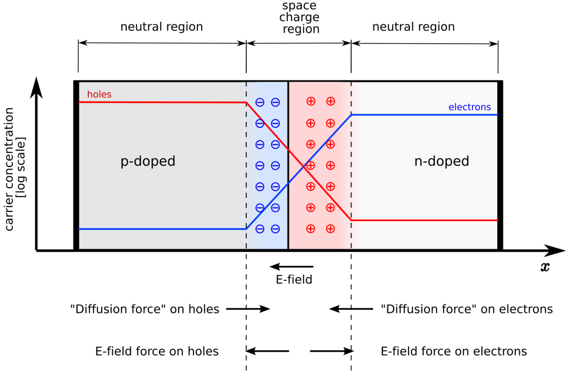
Figure 2.3: A p-n junction in thermal equilibrium with zero-bias voltage applied. Electron and hole concentrations are reported with blue and red lines, respectively. Gray regions are charge-neutral. Light-red zone is positively charged. Light-blue zone is negatively charged. The electric field is shown on the bottom, with the electrostatic force on electrons and holes and the direction in which the diffusion tends to move electrons and holes [70].
