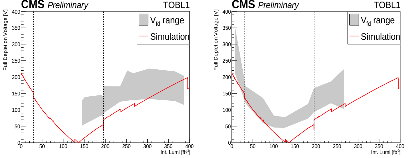
Figure B.4: Leakage current method applied to (left) small scan modules and (right) all the modules of the TOB L1 layer. The TOB L1 modules were included in 2017 in small scans. On the right plot, the last data point is the full scan of March 2024, no other full scan were performed this year and the fit results were not good enough to extract a value of the noise scan at the end of 2024. The red line is the prediction made by the Hamburg Model.
