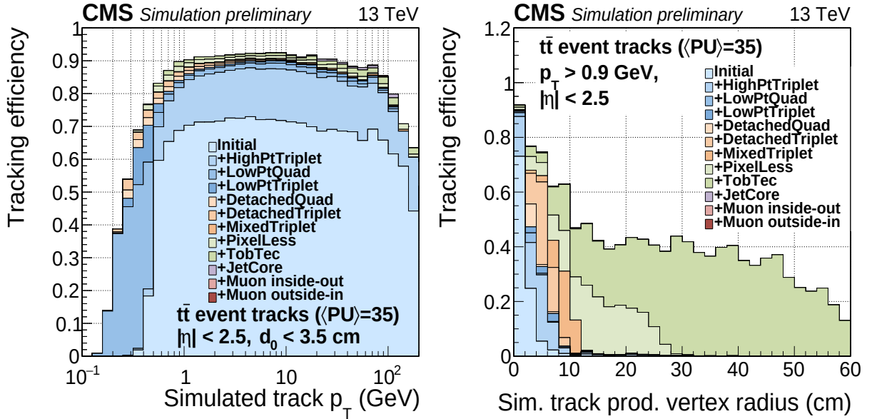
Figure 1.19: (Left) Track reconstruction efficiency per tracking iteration as a function of simulated track transverse momentum p_T for the Phase I tracker. (Right) Track reconstruction efficiency per tracking iteration as a function of simulated track production vertex radius for the Phase I tracker [47].
