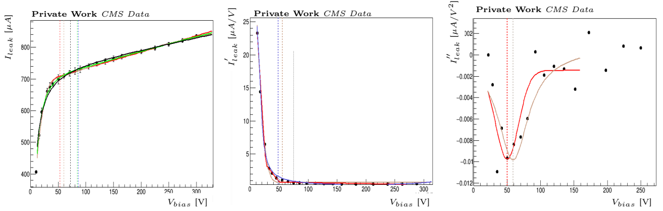
Figure 2.20: (Left) Leakage current curve with the five different fits. The red and brown curves are the sigmoid with the first-order and second-order polynomials respectively. The blue and the green curves are the arctangent with the first-order and second-order polynomials respectively. The black curve is the general purpose fit. (Middle) Leakage current slope as a function of the bias voltage with three different fits. The Gaussian/exponential fit is brown, the linear fit is red and the the general purpose fit is in blue. (Right) Leakage current curvature as a function of the bias voltage with two different fits. The Gaussian fit is in red while the general purpose function is brown. The extracted V_{FD} values are shown by the vertical dashed lines. The curves are shown for a TIB L1 module of a 2018 scan around type inversion.
