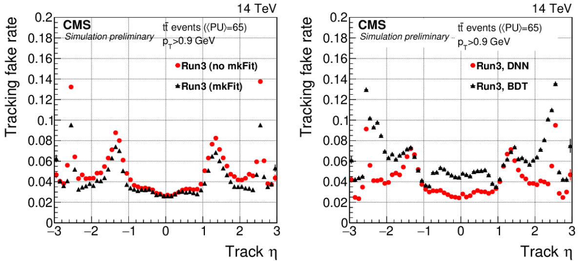
Figure 1.20: (Left) Comparison of tracking fake rate as a function of the track pseudorapidity \eta between mkFit and CTF. (Right) Comparison of the tracking fake rates for tracks selected by DNN (red) and BDT (black) [50].
