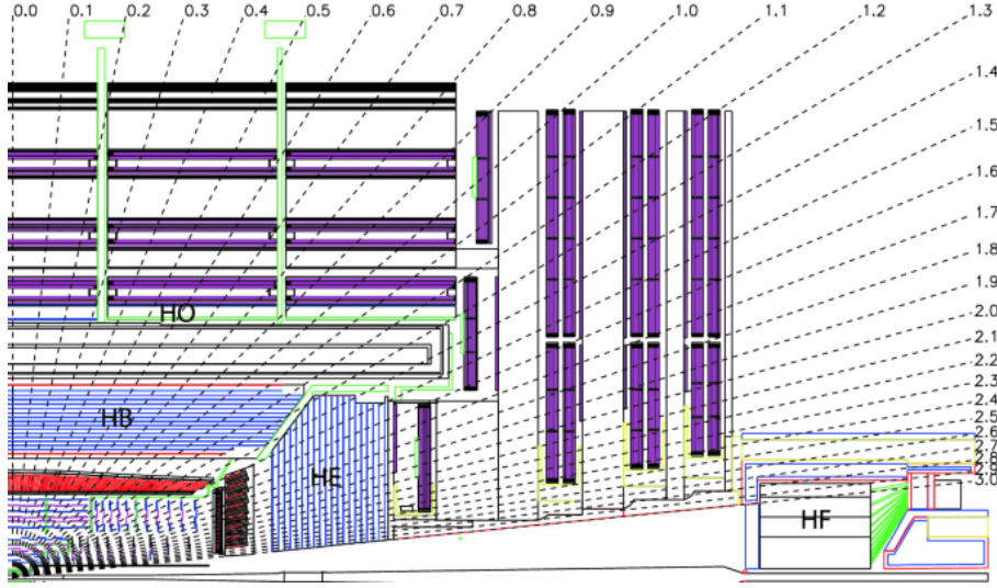
Figure 1.10: Longitudinal view of the CMS detector showing the locations of the hadron barrel (HB), endcap (HE), outer (HO) and forward (HF) calorimeters.[5]
