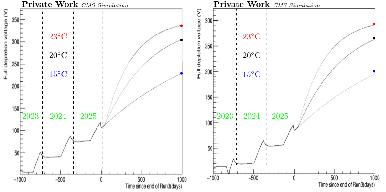
Figure 2.33: Evolution of the full depletion voltage value as a function of time since the end of Run 3 in days. Negative x-axis values meaning the Run 3 is on-going while positive x-axis value corresponding to the dismantling of the tracker. The results are shown for (left) TOB L5 and (right) TOB L6 for different exposure temperature of the tracker. The predictions are made based on the average behavior of a module of each layer.
