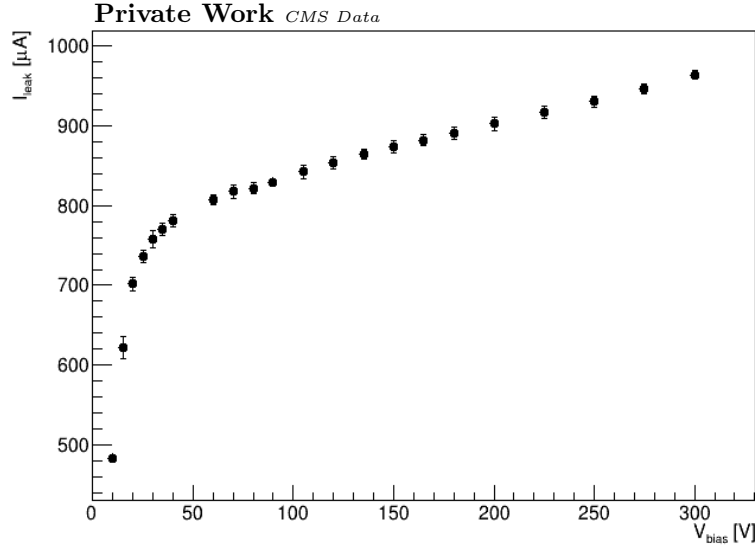
Figure 2.18: Distribution of the leakage current as a function of the bias voltage of a TIB L1 module during a scan of 2018 close to type inversion of the module [85].
