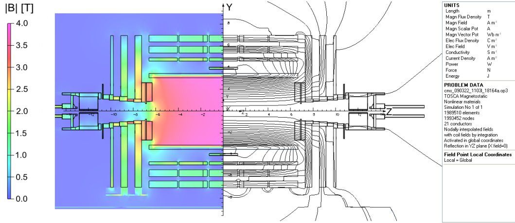
Figure 1.6: Simulation of the CMS magnetic field [26]
