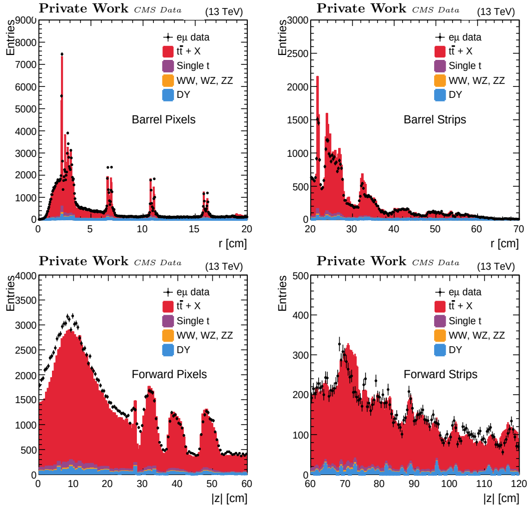
Figure 4.21: Reconstructed secondary interactions in (upper) barrel ( |\eta| < 1.5 ) and (lower) endcaps ( |\eta| > 1.5 ) for 2018 data and MC e\mu samples.
