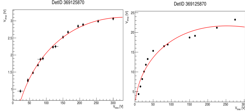
Figure 2.21: Curves of the voltage drop as a function of the bias voltage for the TIB layer 1 module 369125870 at different dates: (left) May 2015, (Right) August 2018. Increasing values with time are related to leakage current increase. Horizontal bars are drawn when the current measurement took place in-between two voltage steps (in this case the exact voltage value for a module is not known) [85].
