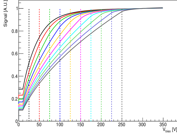
Figure 2.16: Simulated curves in arbitrary units of the cluster charge evolution at different bias voltage. The curves are shown for different full depletion voltage values represented by the vertical lines for a sensor with a thickness of 320 \mu\text{m} [85]. The curves are only valid in the case of no radiation damage.
