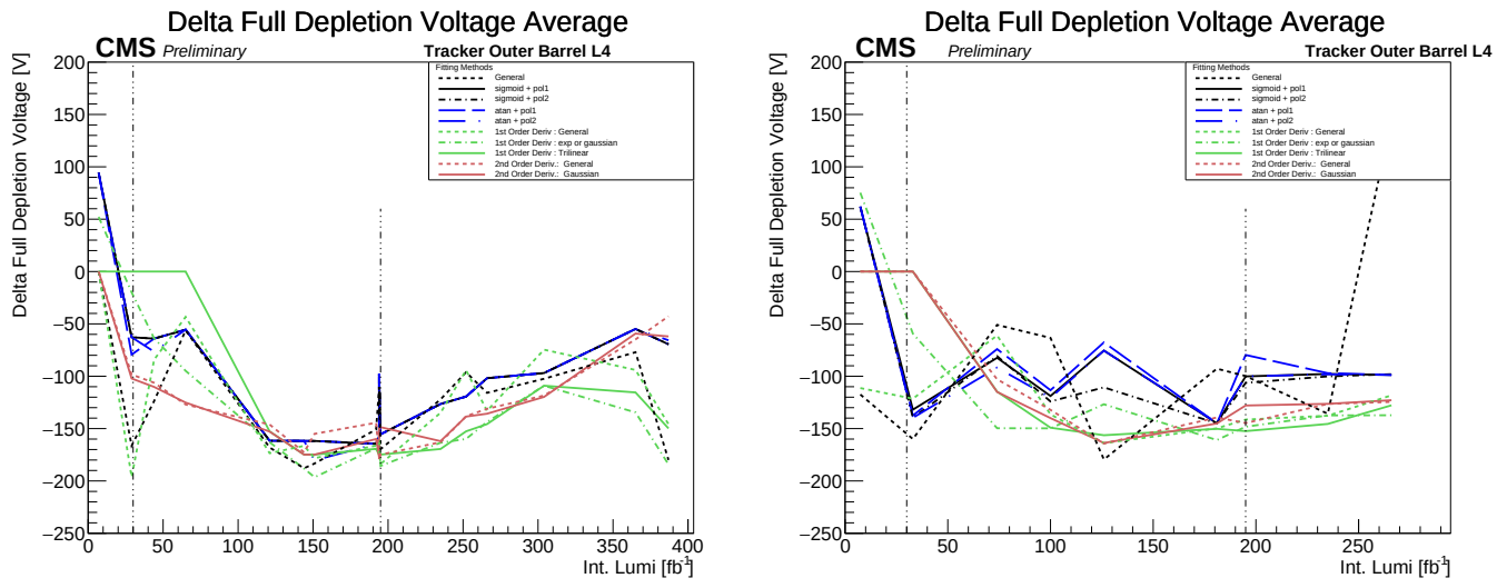
Figure B.7: Leakage current method applied to (left) small scan modules and (right) all the modules of the TOB L4 layer showing the \Delta V_{FD} . The last point of the right plot comes from the noise scan performed at the end of the 2024 operations. The black dashed lines are the LS1 and LS2.
