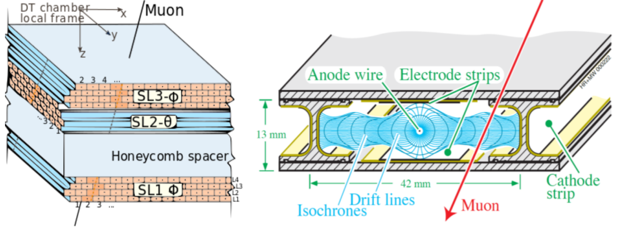
Figure 1.12: (Left) Structure of a DT chamber with three superlayers, each composed of 4 layers of drift cells. (Right) Layout of a drift cell showing the electric field lines in the gas volume [31].
