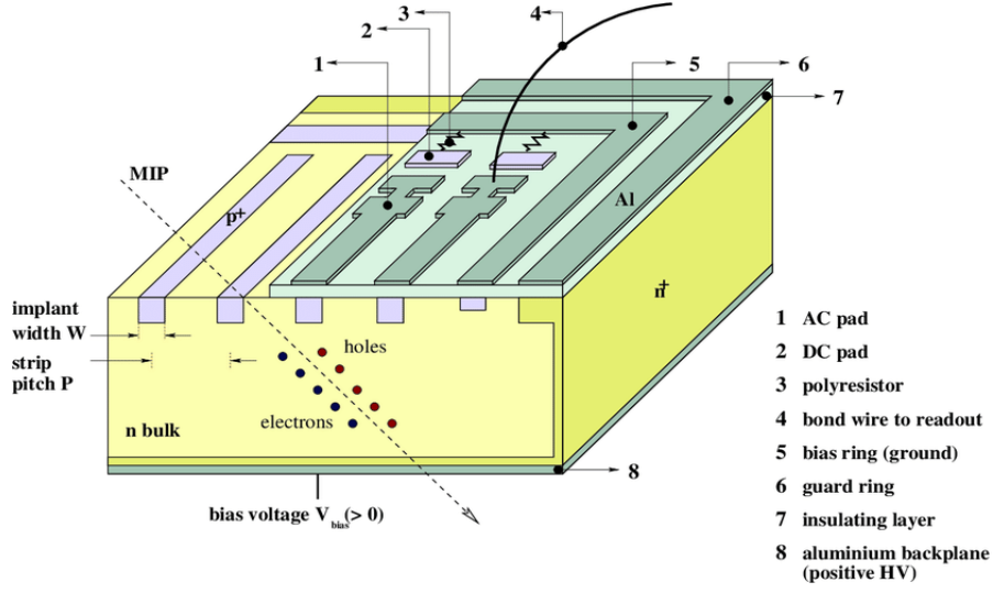
Figure 2.8: Schematic structure of a CMS silicon microstrip sensor with a n-type bulk, p + strip implants and a n + backplane. A MIP crossing the sensor and producing electron-hole pairs is also displayed [75].
