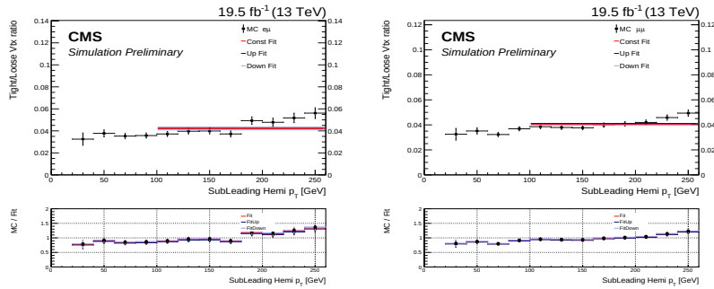
Figure D.8: Ratio of the number of tight over loose vertices as a function of the p_T of the sub-leading hemisphere in the 2016-pre (left) e\mu MC and (right) \mu\mu MC.
