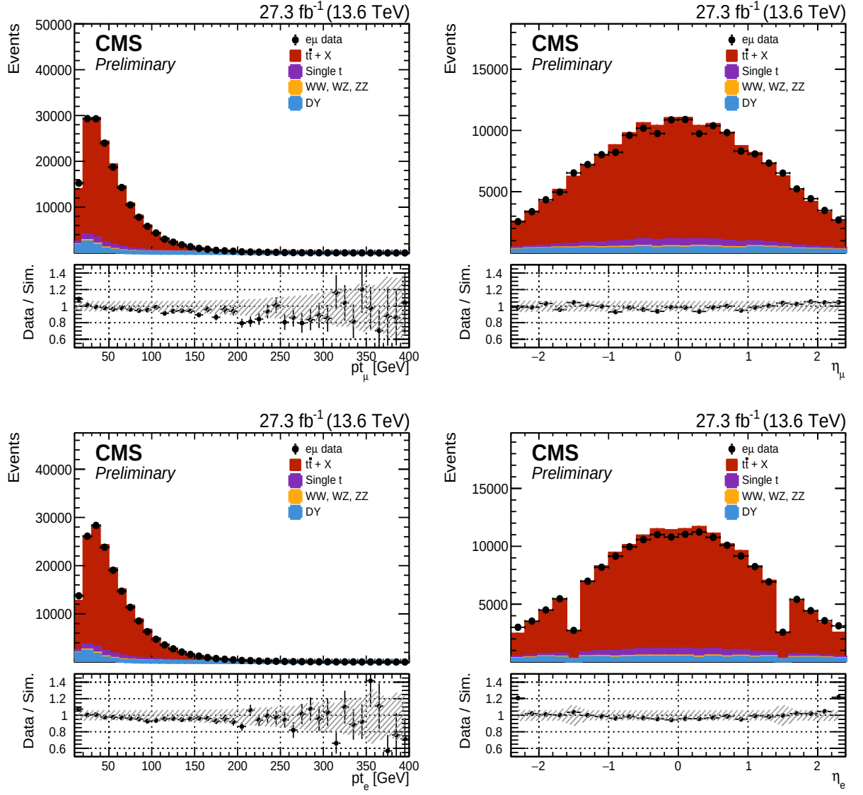
Figure D.38: p_T and \eta of the muons and electrons in the 2023 e\mu data and MC. The hatched bands represent the systematic uncertainties.
