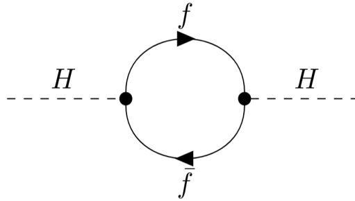
Figure 3.5: Example of a virtual fermion loop correction to the Higgs boson mass.
