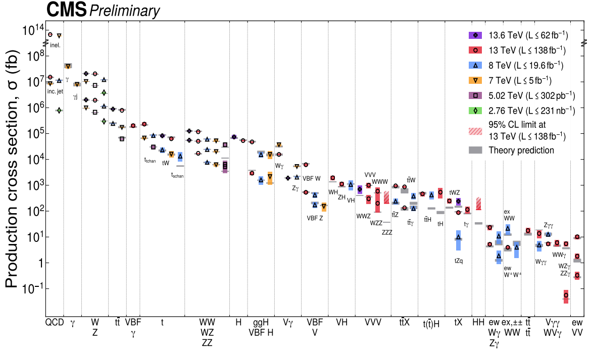
Figure 3.4: Production cross sections measured by CMS for various processes. Measurements performed at different LHC pp collision energies are marked by unique symbols and the colored bands indicate the combined statistical and systematic uncertainty of the measurement. Grey bands indicate the value with uncertainty of the corresponding SM theory predictions. Shaded hashed bars indicate the excluded cross section region for a production process with the measured 95% CL upper limit on the process indicated by the solid line of the same color [97].
