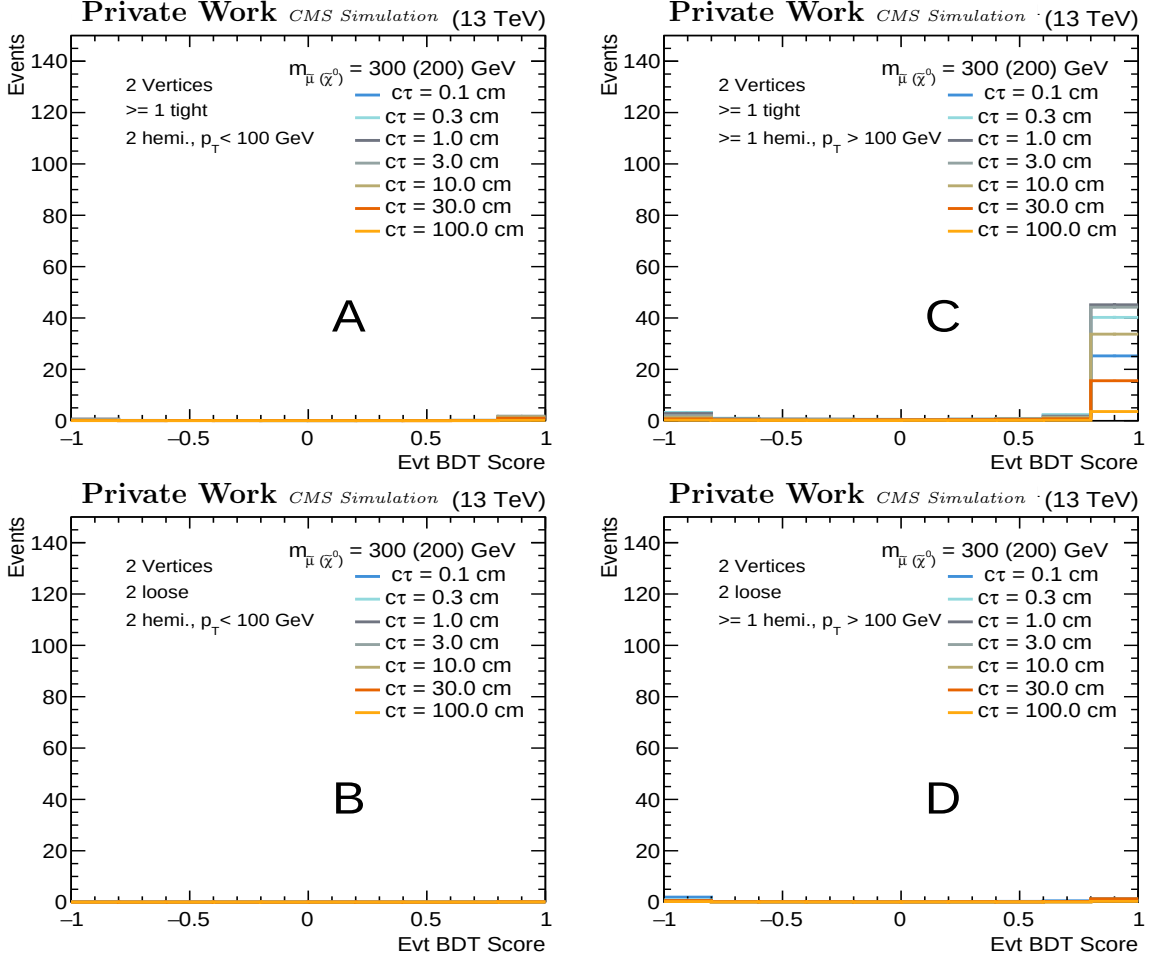
Figure 5.16: Event BDT score of two vertices in signal events with S_{m_{\tilde{\chi}_0^1}^{m_{\tilde{\mu}}}} = S_{200}^{300} in the 2018 MC conditions for various c\tau_{\tilde{\chi}} values.
