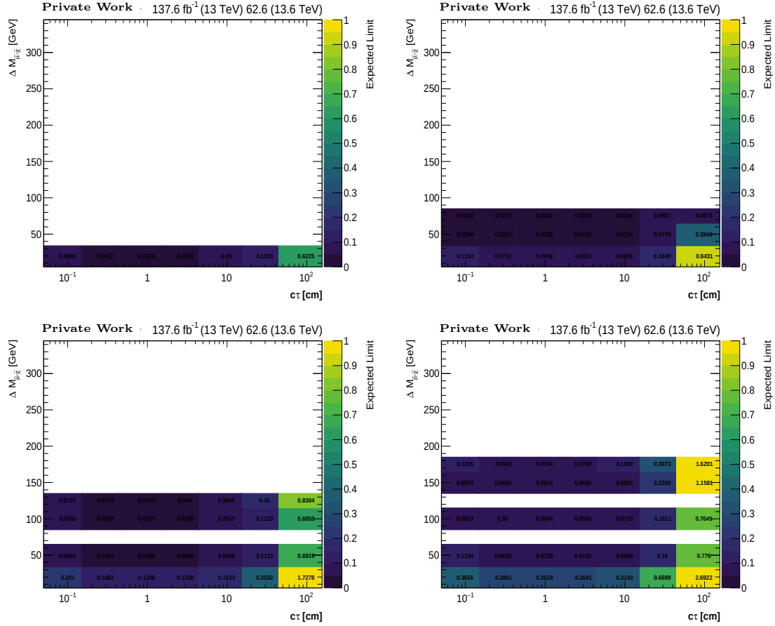
Figure 5.24: \Delta m_{\tilde{\mu}\tilde{\chi}} vs c\tau_{\tilde{\chi}} expected limits at a 95% confidence level assuming a smuon mass of (upper left) 200 GeV (upper right) 250 GeV (lower left) 300 GeV (lower right) 350 GeV. The z -axis is the ratio of the expected cross section over the theoretical one. Signal samples with z -axis values below 1 are excluded. The center of each bin corresponds to a specific signal sample.
