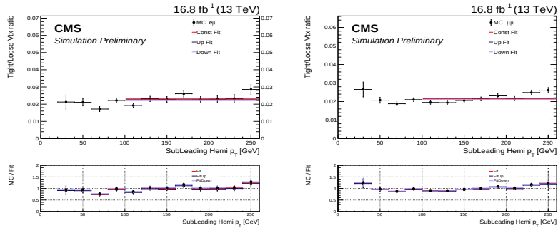
Figure D.16: Ratio of the number of tight over loose vertices as a function of the p_T of the sub-leading hemisphere in the 2016-post (left) e\mu MC and (right) \mu\mu MC.
