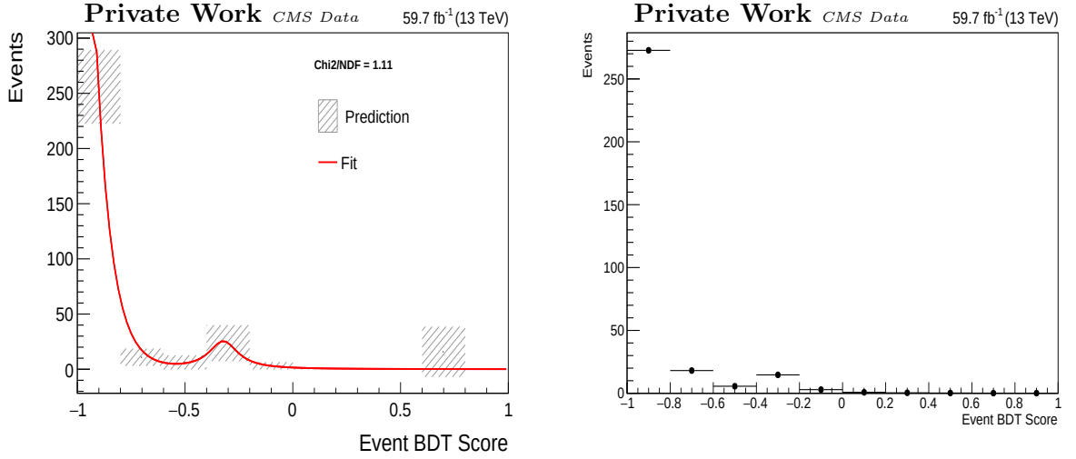
Figure 5.23: (left) Fit of the background estimate in the signal region for 2018 \mu\mu data. (right) Toy experiments generated injected in the COMBINE tool to extract expected limits.
