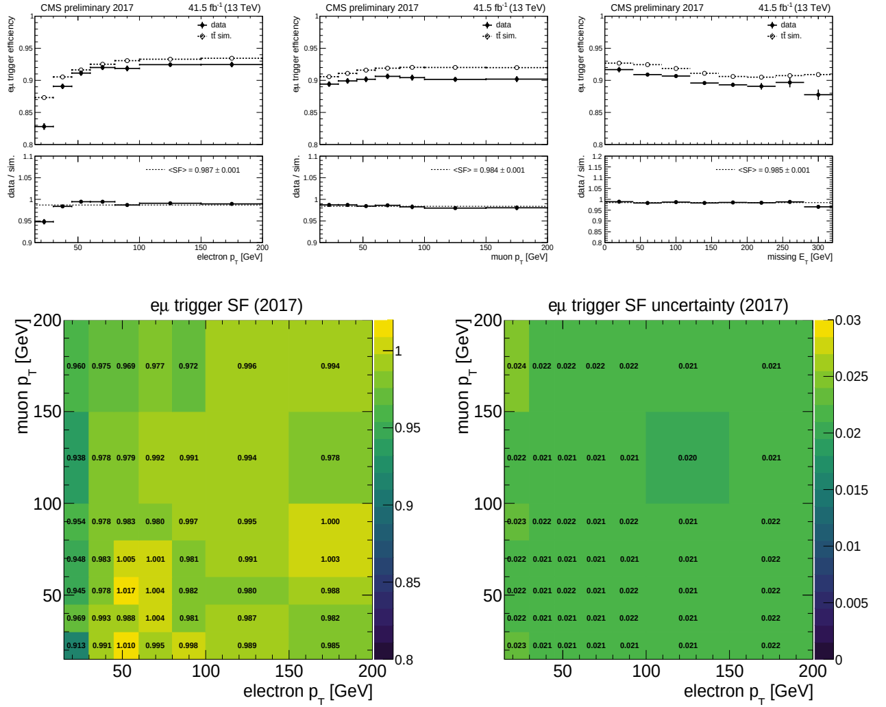
Figure E.2: Same as Fig.E.1 for the 2017 datasets.
