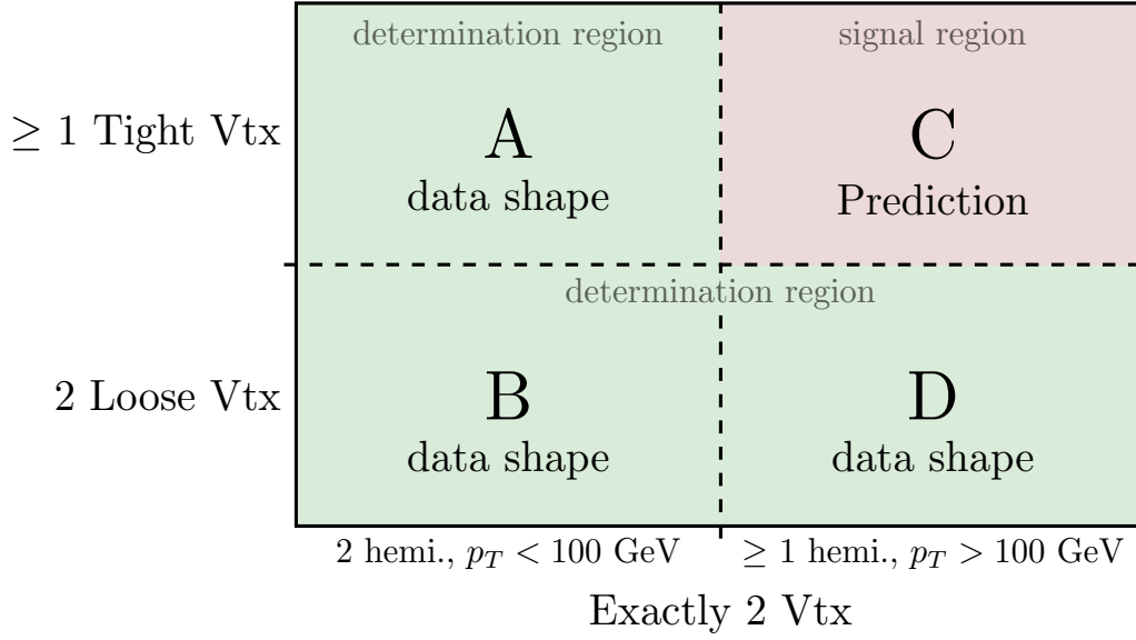
Figure 5.8: Schematic overview of the background estimation method. The background shape within the signal region C is defined using data from the A,B and D regions. The bin-by-bin evaluation of the background shape within the signal region is defined by the relation n_C = n_A n_D / n_B .
