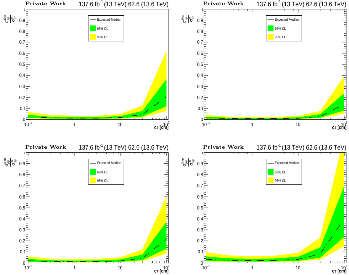
Figure 5.28: \sigma_{\tilde{\mu}\tilde{\mu}} \times B_r(\tilde{\mu} \rightarrow \mu\tilde{\chi}_1^0)^2 assuming different mass combinations between the smuon and the neutralino S_{m_{\tilde{\chi}_1^0}}^{m_{\tilde{\mu}}} : (upper left) S_{180}^{200} (upper right) S_{200}^{250} (lower left) S_{200}^{300} (lower right) S_{200}^{350} . Signal samples for which the ratio of the cross sections is below 1 are excluded.
