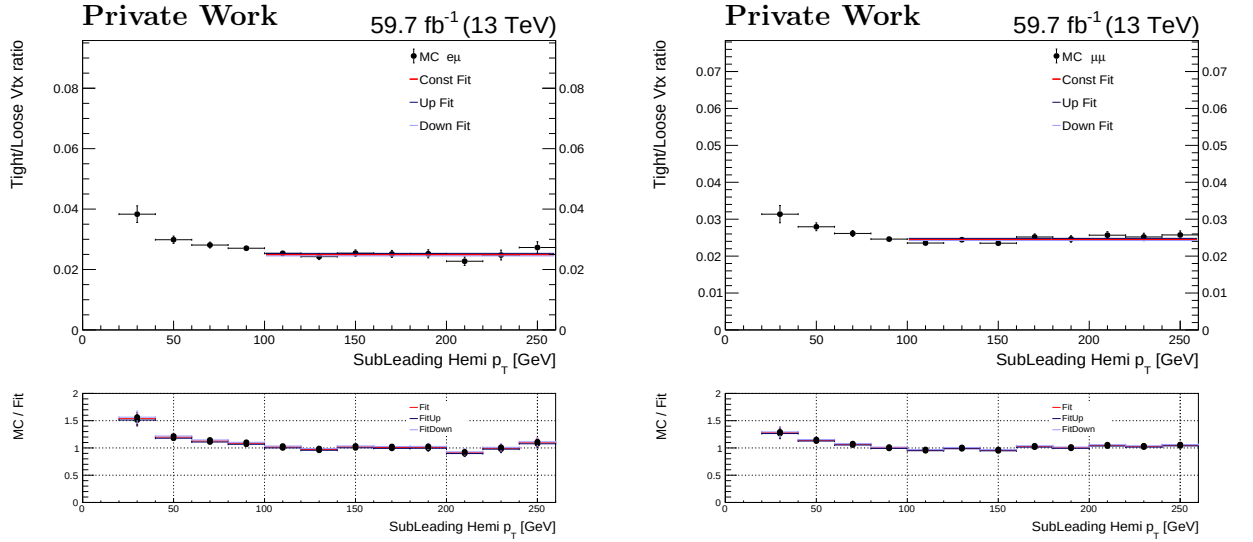
Figure 5.19: Ratio of the number of tight over loose vertices as a function of the p_T of the sub-leading hemisphere in the 2018 (left) e\mu MC and (right) \mu\mu MC.
