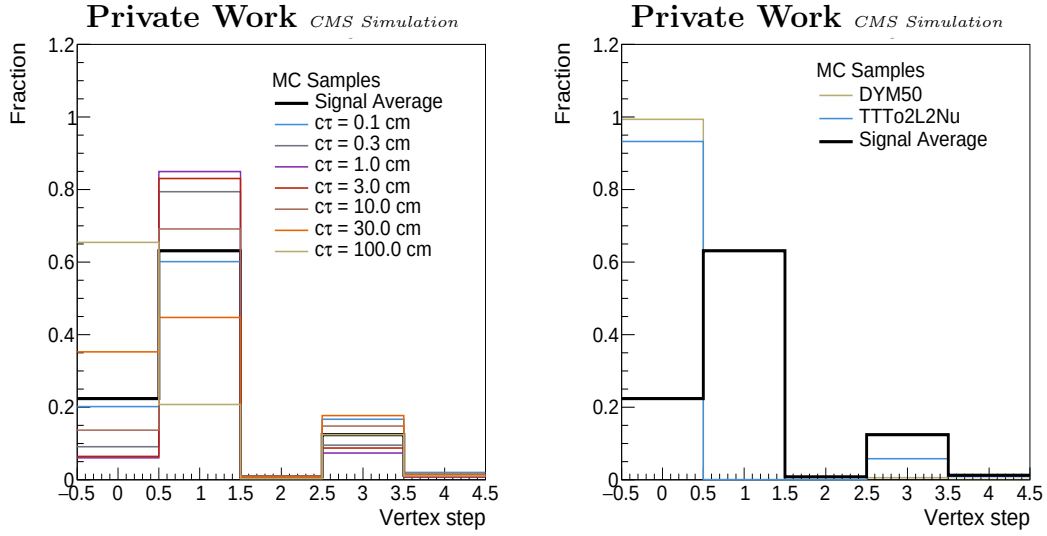
Figure 5.3: Relative contribution of each step of the displaced vertex reconstruction (before merging), in 2018 MC conditions, for (left) various neutralino c\tau_{\tilde{\chi}} values and any mass of the \tilde{\chi}_0^1 or \tilde{\mu} and (right) two different background samples. The signal average contribution is shown in black in both figures. Bin 0 corresponds to vertices not reconstructed due to either, no track available or the AVF not converging or \chi_{vtx}^2/\text{dof} being above 10 or below 0.
