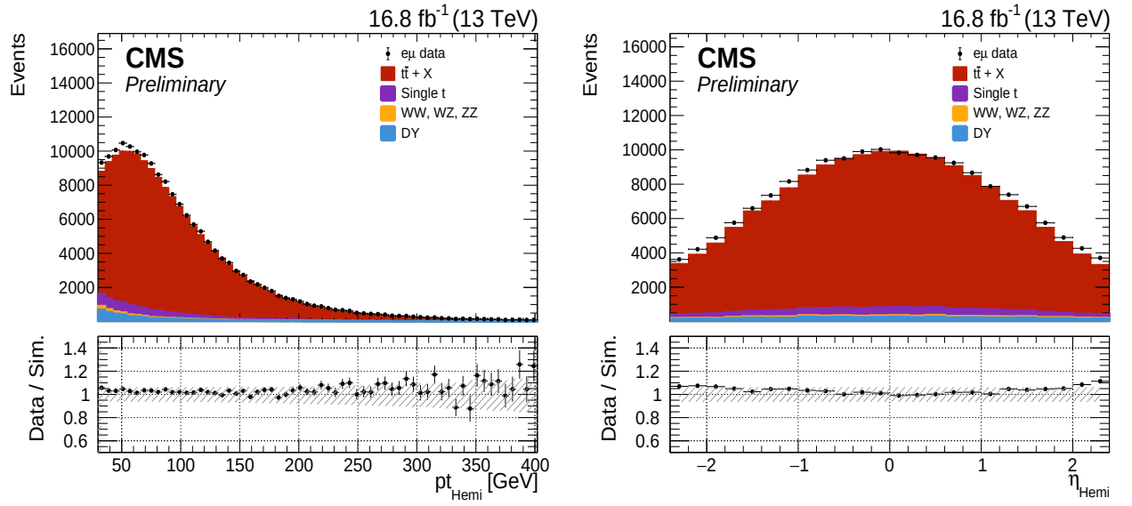
Figure D.10: p_T and \eta of the hemispheres in the 2016-post e\mu data and MC. The hatched bands represent the systematic uncertainties.
