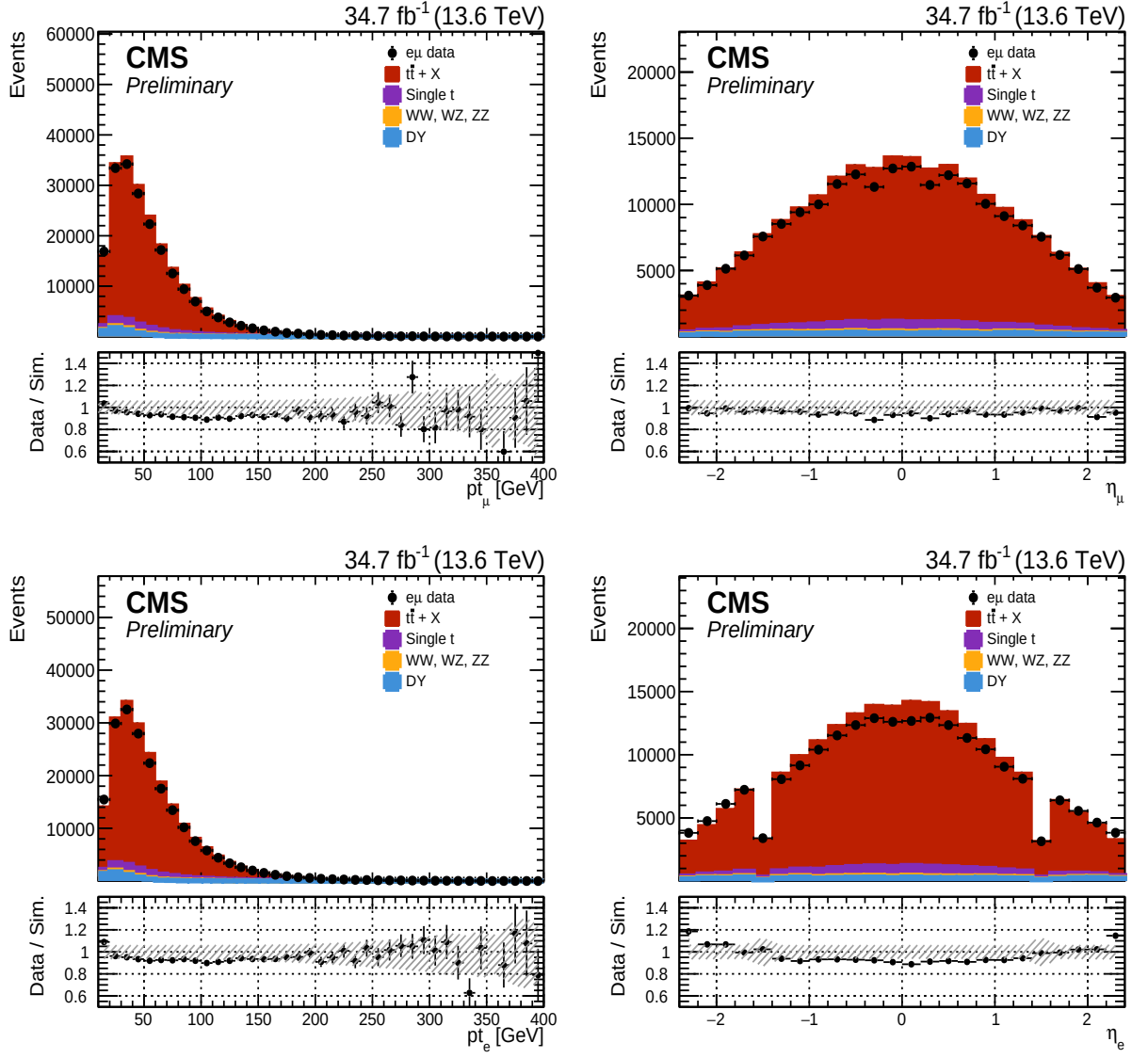
Figure D.27: p_T and \eta of the muons and electrons in the 2022 e\mu data and MC. The hatched bands represent the systematic uncertainties.
