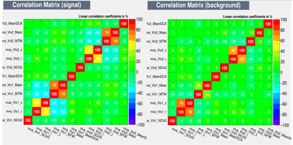
Figure 5.13: Input variables correlation of the vertex BDT for (left) signal and (right) background vertices. The signal vertices are from the c\tau_{\tilde{\chi}} = 10 cm sample, while the background vertices are from the e\mu data sample. The MTW variable refers to the sum of the weight of the tracks at vertex.
