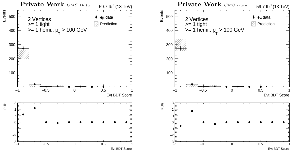
Figure 5.21: Signal region in the 2018 e\mu data sample (left) without taking into account the correlation and (right) with the correlation comparing the data and the predictions. The pulls are defined as: \frac{\text{data} - \text{prediction}}{\sqrt{\text{data} + \sigma_{\text{predi}}^2}} where \sigma_{\text{predi}} is the uncertainty associated to the prediction.
