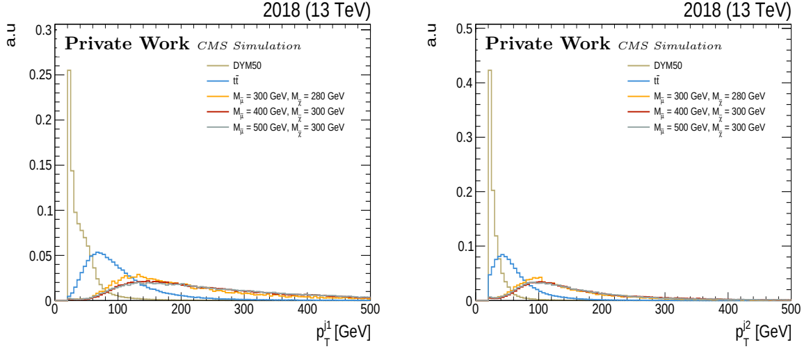
Figure 4.6: Distributions of the leading and sub-leading jet p_T in signal, Drell-Yan and t\bar{t} MC events in 2018 conditions.
