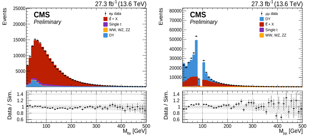
Figure D.36: For 2023 data and MC, invariant mass of the lepton pair in the (left) e\mu and (right) \mu\mu samples. The hatched bands represent the systematic uncertainties.
