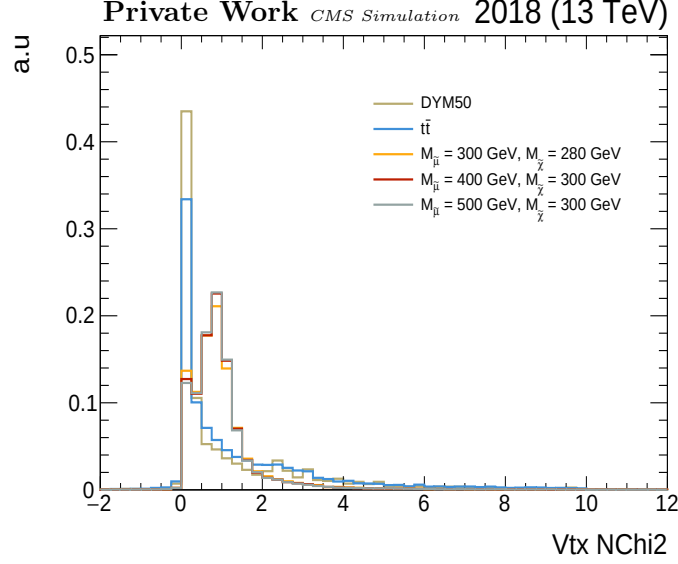
Figure 5.1: \chi^2_{vtx}/\text{dof} distribution for signal, Drell-Yan and t\bar{t} vertices.
