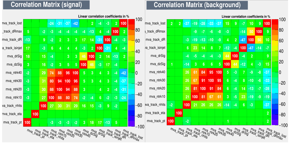
Figure 4.30: Correlation matrices between input variables of the track selection BDT for (left) signal and (right) background.
