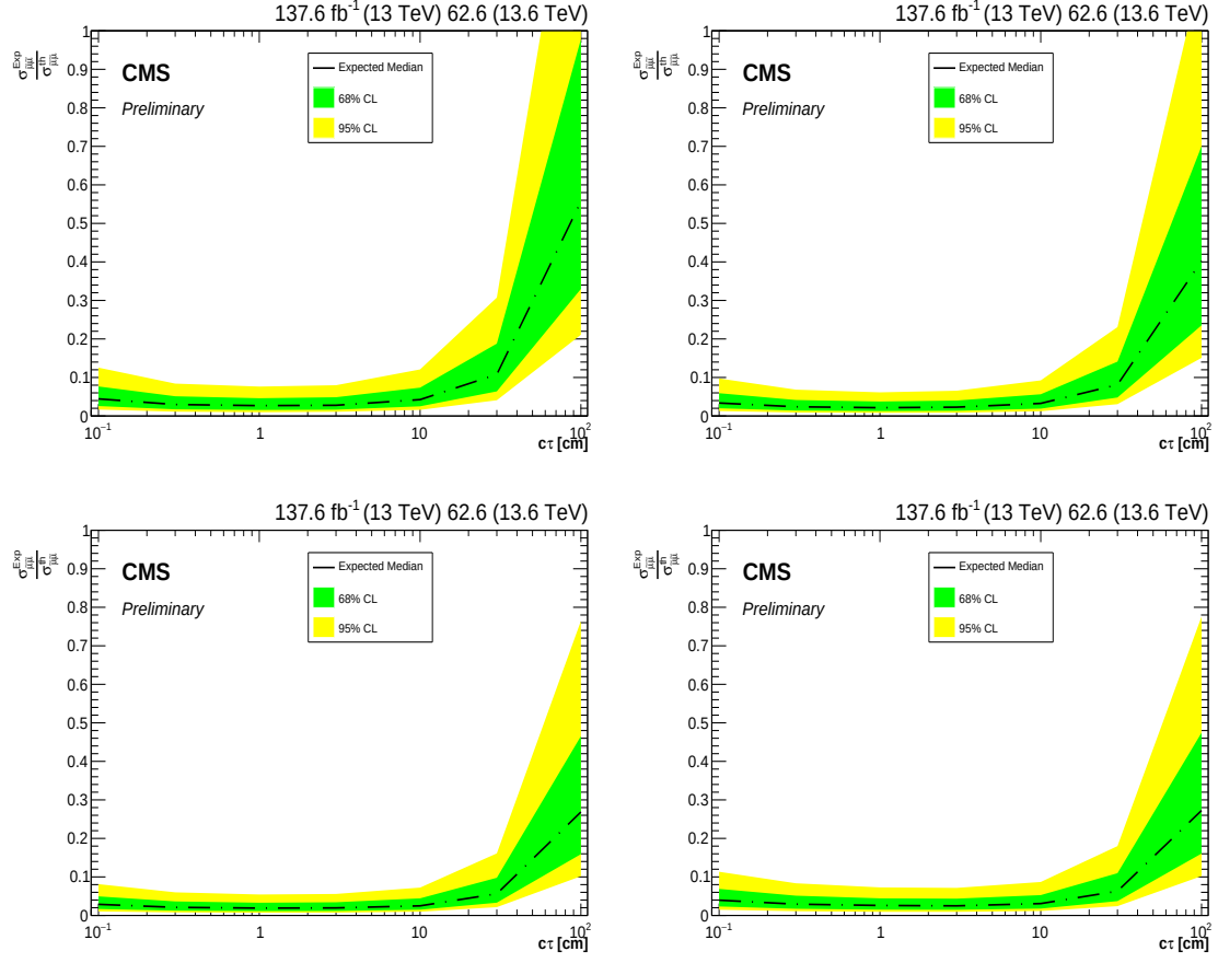
Figure G.3: \sigma_{\tilde{\mu}\tilde{\mu}} \times B_r(\tilde{\mu} \rightarrow \mu \tilde{\chi}_1^0)^2 assuming different mass combinations between the smuon and the neutralino S_{m\tilde{\chi}_1^0}^{m\tilde{\mu}} : (upper left) S_{180}^{350} (upper right) S_{200}^{350} (lower left) S_{250}^{350} (lower right) S_{280}^{350} . Signal samples for which the ratio of the cross sections is below 1 are excluded.
