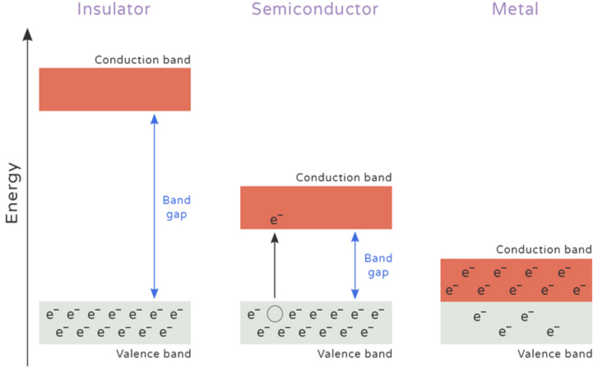
Figure 2.1: Scheme representation of the band gap for insulators (left), semiconductors (middle) and metals (right) [67].
