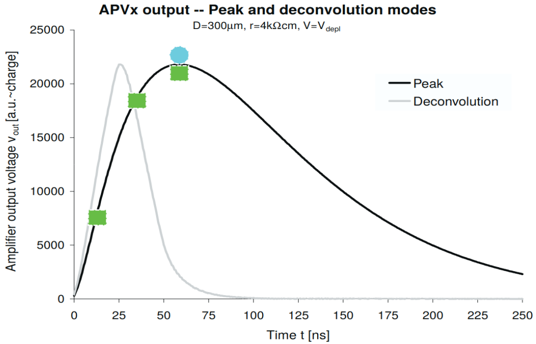
Figure 2.10: Amplifier output voltage in the peak (black) and deconvolution (gray) mode. Actually, the shaper output is sampled in the APV25 to obtain only maxima of the two curves. An example of the sampling points for the deconvolution mode is shown in green rectangles, the sampling point for the peak mode is represented by a blue circle [79].
