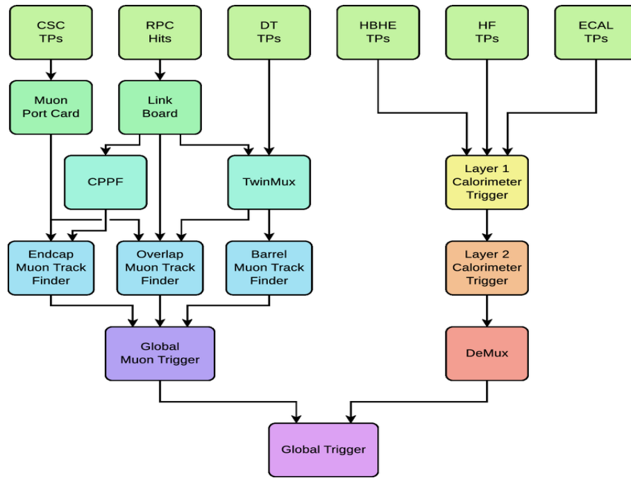
Figure 1.15: Flow chart of the L1 trigger system using the information of the calorimeters and the muon chambers (at the top) to make the final decision (at the bottom) [35]
