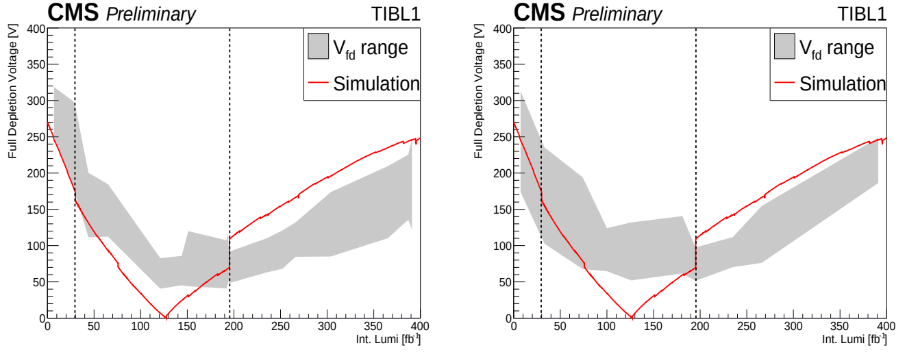
Figure B.1: Leakage current method applied to (left) small scan modules and (right) all the modules of the TIB L1 layer. The last point of the right plot comes from the noise scan performed at the end of the 2024 operations. The red line is the prediction made by the Hamburg Model.
