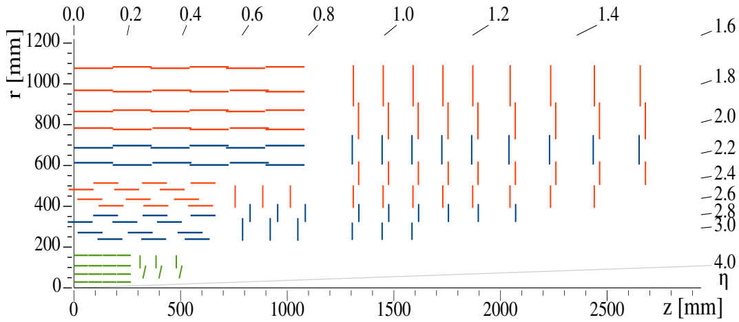
Figure 1.7: Sketch of one quarter of the Phase-1 CMS tracking system in r - z view. The pixel detector is shown in green, while single-sided and double-sided strip modules are depicted as red and blue segments, respectively [27].
