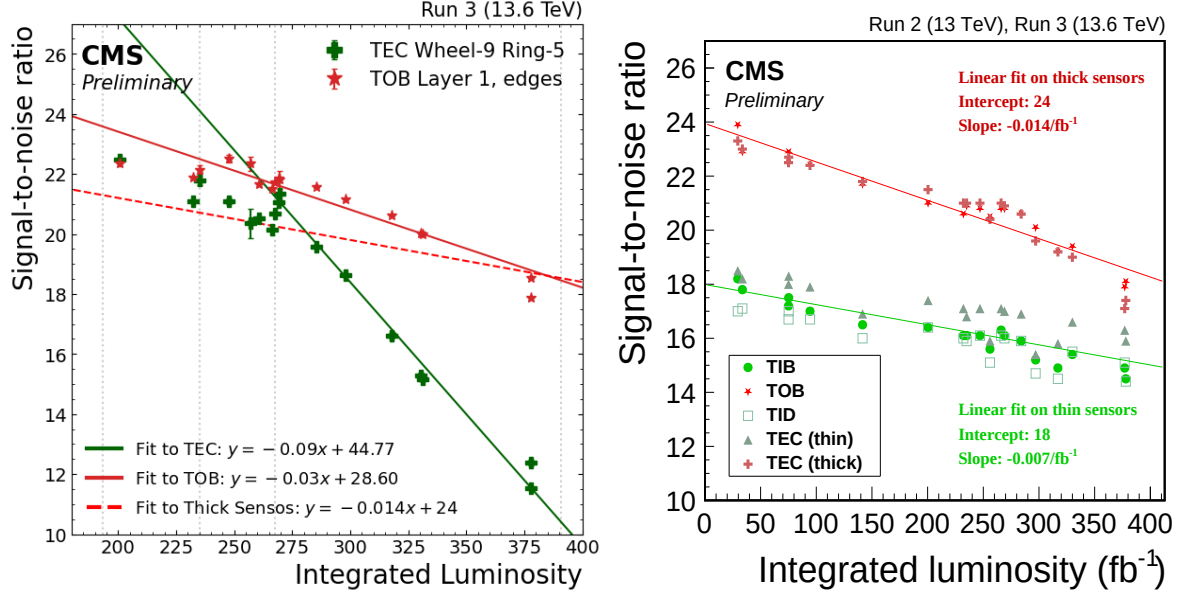
Figure 2.34: Signal-to-noise ratio plots (left) for the TEC W9 R5 and TOB L1 modules and (right) for all sub-detectors. Linear fits are performed with a steeper slope for the TEC W9 R5 potentially meaning loss of charge collection due to under depletion. The effect can not be seen when looking at the average behavior of the TEC modules, for both thin and thick sensors [88].
