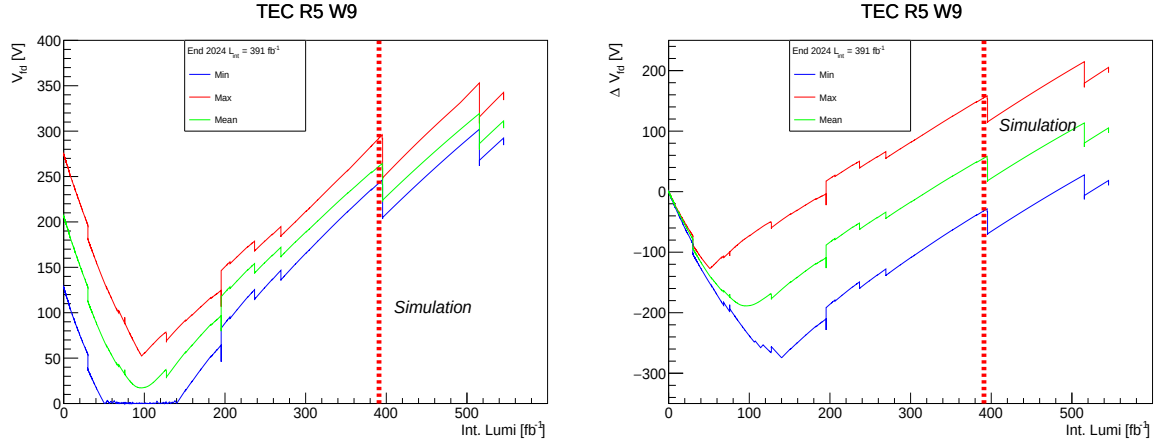
Figure 2.36: Distribution of the (left) full depletion voltage and (right) the difference between the full depletion voltage and the initial measured value referred as \Delta V_{FD} for the TEC W9 R5 modules. In both plots, the maximum, mean and minimum values are shown based on data before the red-dashed line and based on the expected schedule after the red dashed line.
