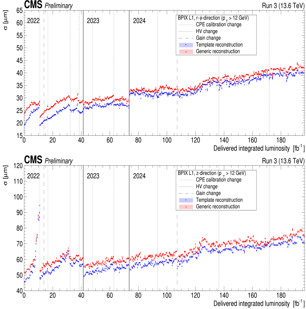
Figure 1.18: (Upper) Hit resolution in the r - \phi coordinate for the BPIX Layer 1 in Run 3 data and (Lower) in the z coordinate [44]. The increase in offset and the degradation of resolution, caused by radiation damage, are recovered by the increase in sensor high voltage bias and the update of the Lorentz angle.
