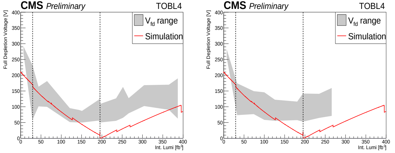
Figure B.6: Leakage current method applied to (left) small scan modules and (right) all the modules of the TOB L4 layer. On the right plot, the last data point is the full scan of March 2024, no other full scan were performed this year and the fit results were not good enough to extract a value of the noise scan at the end of 2024. The red line is the prediction made by the Hamburg Model.
