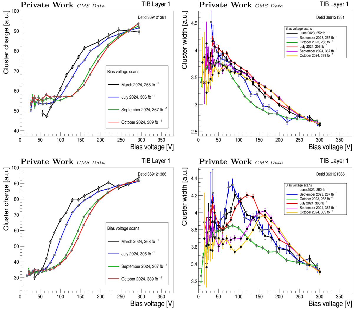
Figure 2.23: (Left) Cluster charge curves from four scans of 2024 for two TIB L1 modules. (Right) Cluster width curve from six scans for the same TIB L1 modules. More scans are shown for the cluster width to show the evolution of the non-expected behavior of the bottom right plot. Grey data points have been corrected for the voltage drop while black data points are not corrected for that effect.
