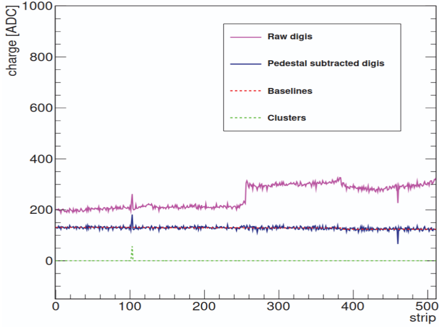
Figure 2.11: Example of data from one tracker module undergoing zero suppression and clustering. The raw digis are shown in pink. From the raw digis the pedestals are subtracted and the resulting digis are shown in blue. From pedestal subtracted digis the baselines shown in red are computed and subtracted. The final output of each channel is shown ingreen. [80].
