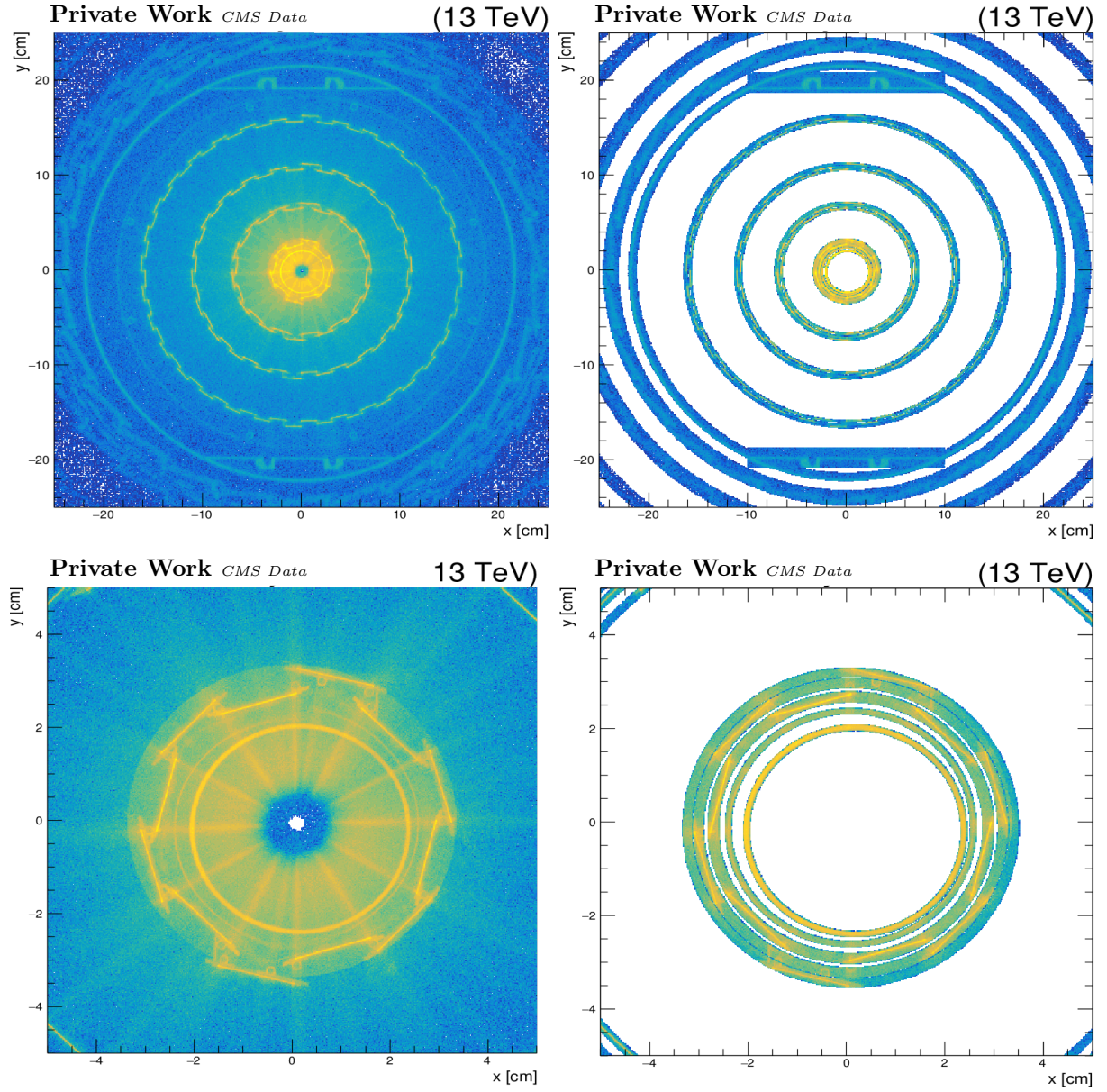
Figure 4.20: Transverse distribution of secondary interactions in the (upper) tracker and (lower) inner pixel layer for the 2018 \mu\mu data sample: (left) all reconstructed vertices, (right) vetoed vertices. For clarity purpose, secondary vertices are requested to be within |\eta| < 1.4 to focus on the barrel region.
