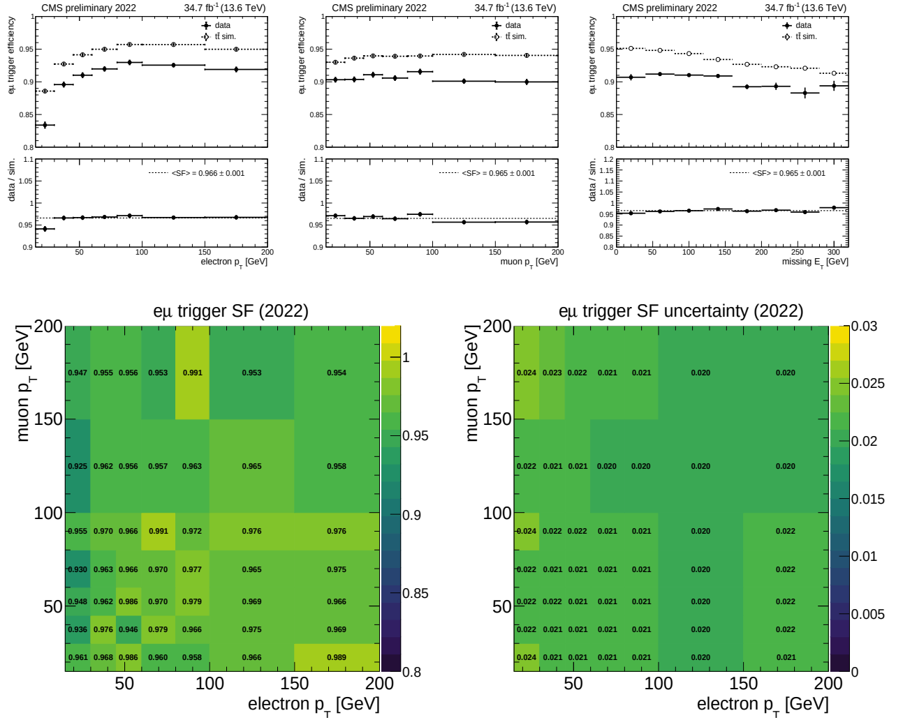
Figure E.4: Same as Fig.E.1 for the 2022 datasets.
