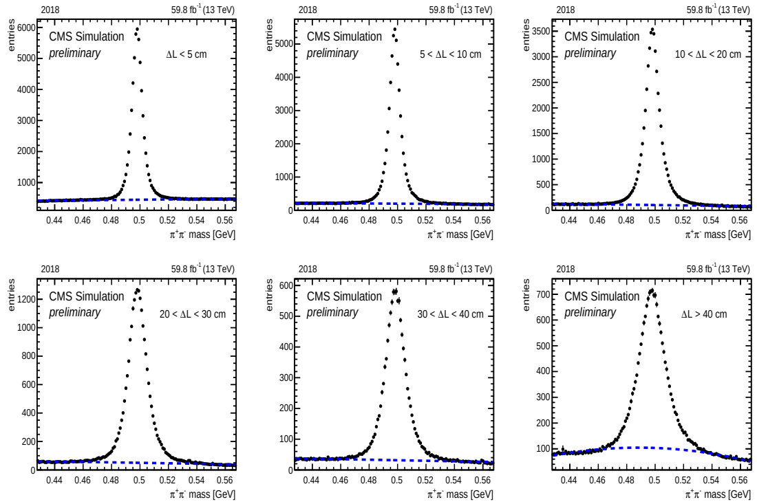
Figure E.7: Invariant mass of K_S candidates from the e\mu MC sample in 2018 for various vertex displacements. The dashed line is the background fit from the tails.
