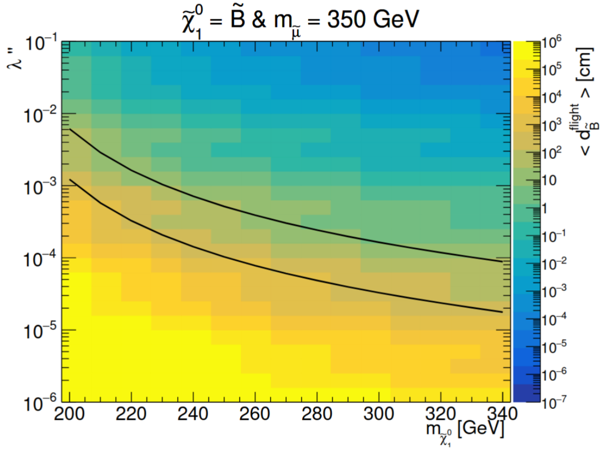
Figure 3.17: Average flight distance \langle d_{\tilde{B}}^{flight} \rangle of the neutralino Bino-like in the laboratory frame as a function of \lambda'' and the neutralino mass m_{\tilde{\chi}_1^0} . A smuon mass of m_{\tilde{\mu}} = 350 \text{ GeV} is assumed. The black lines represent the geometrical limits of the tracker volume [121].
