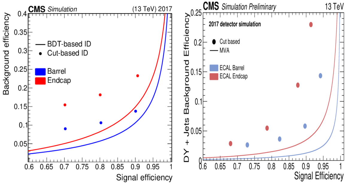
Figure 1.21: (Left) Performance of photon identification algorithms in 2017 Monte-Carlo simulation [59] (Right) Performance of electron identification algorithms in Drell-Yan Monte-Carlo simulation [60].
