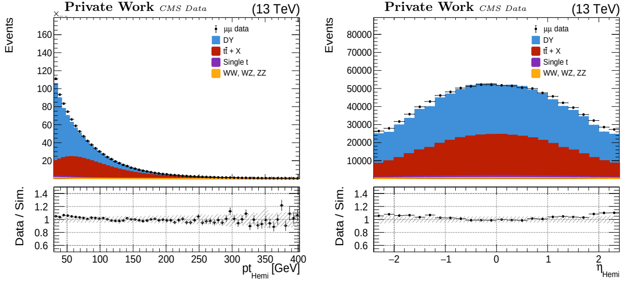
Figure 4.16: p_T and \eta of the hemispheres in the 2018 \mu\mu data and MC. The hatched bands represent the systematic uncertainties.
