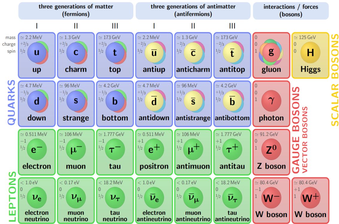
Figure 3.1: Standard Model of elementary particles[25].
