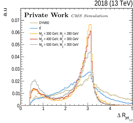
Figure 4.7: \Delta R distribution between the leading and sub-leading jets in signal, Drell-Yan and t\bar{t} MC events in 2018 conditions.
