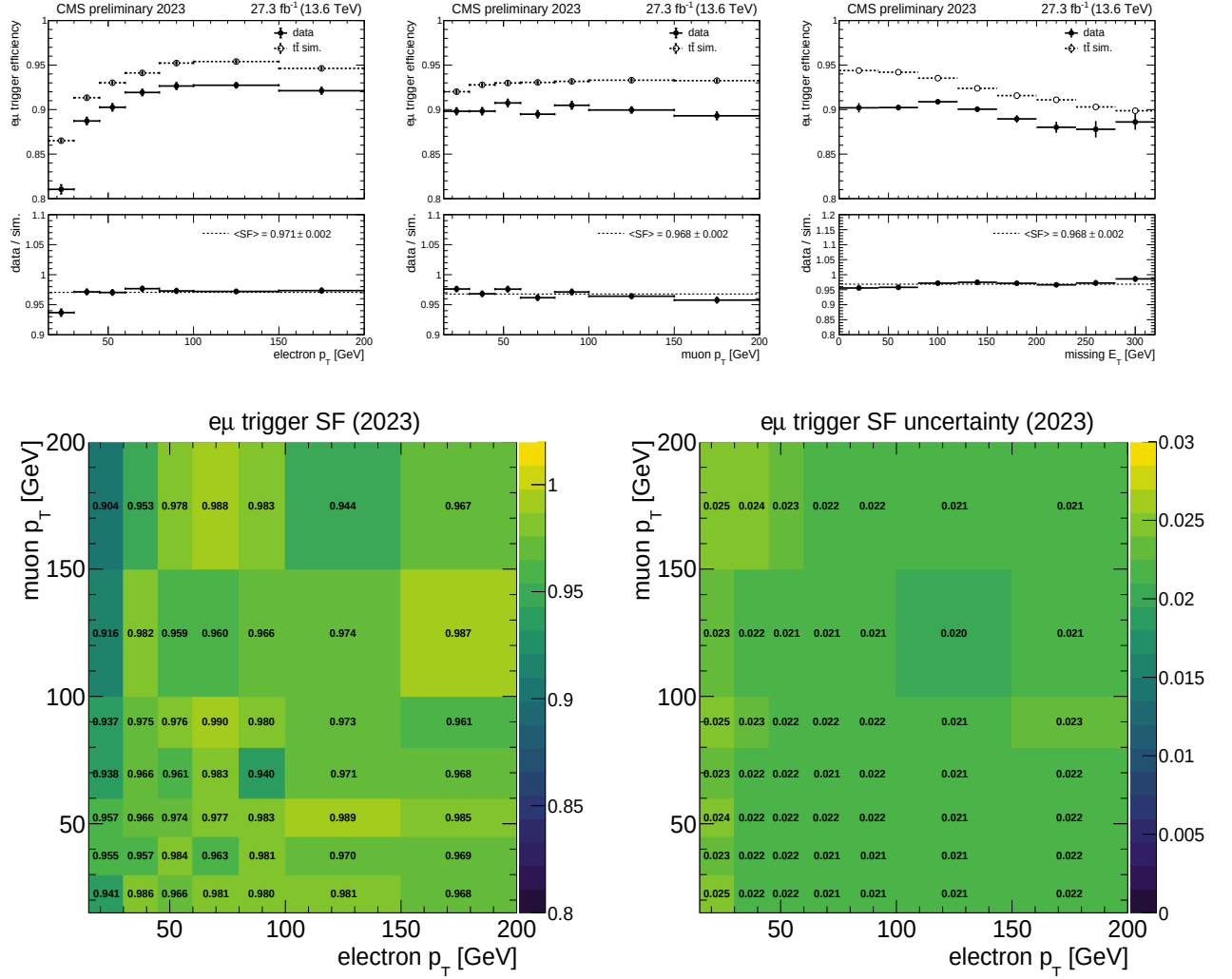
Figure E.5: Same as Fig.E.1 for the 2023 datasets.
