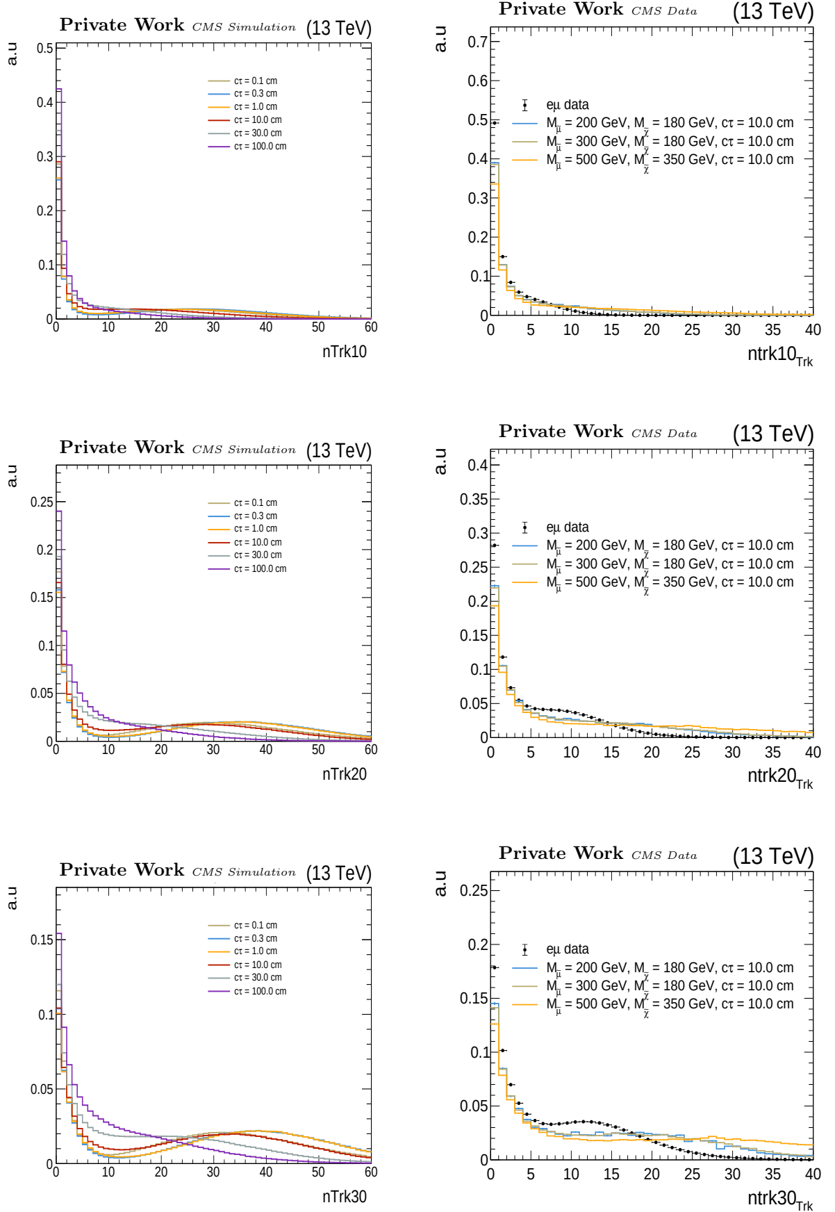
Figure 4.27: Input variables to the BDT. The left column shows the signal distribution for different c\tau_{\tilde{\chi}} while the right column shows the comparison between signal and e\mu data.
