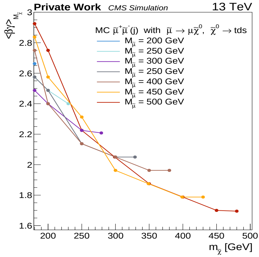
Figure 3.16: Average Lorentz boost of the neutralino as a function of the neutralino mass and smuon mass.
