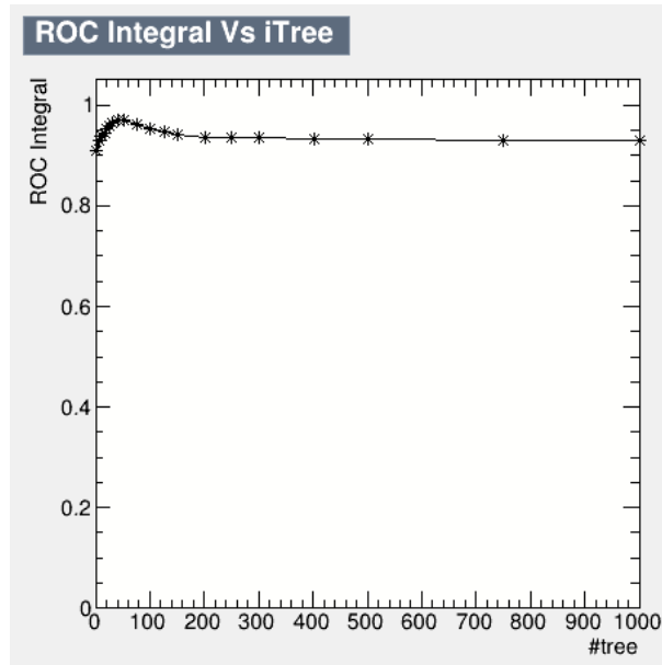
Figure 4.25: ROC Integral evolution with respect to the number of trees in the training. The ROC Integral (also called AUC for Area Under Curve depicts the overall power of the classifier.)
