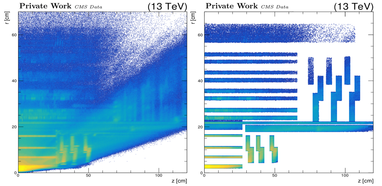
Figure 4.19: Longitudinal distribution of secondary interactions for the 2018 \mu\mu data sample: (left) all reconstructed vertices, (right) vetoed vertices.
