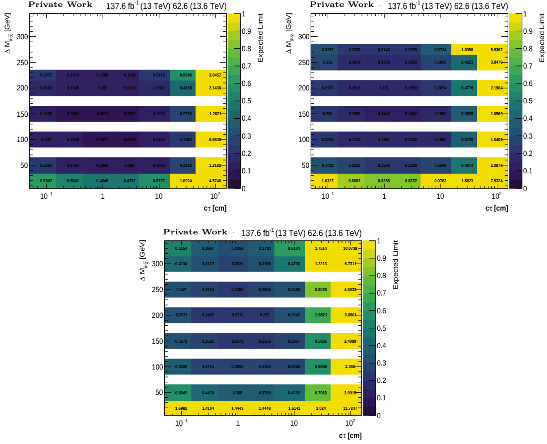
Figure 5.25: \Delta m_{\mu\tilde{\chi}} vs c\tau_{\tilde{\chi}} expected limits at a 95% confidence level assuming a smuon mass of (upper left) 400 GeV (upper right) 450 GeV (lower) 500 GeV. The z -axis is the ratio of the expected cross section over the theoretical one. Signal samples with z -axis values below 1 are excluded. The center of each bin corresponds to a specific signal sample.
