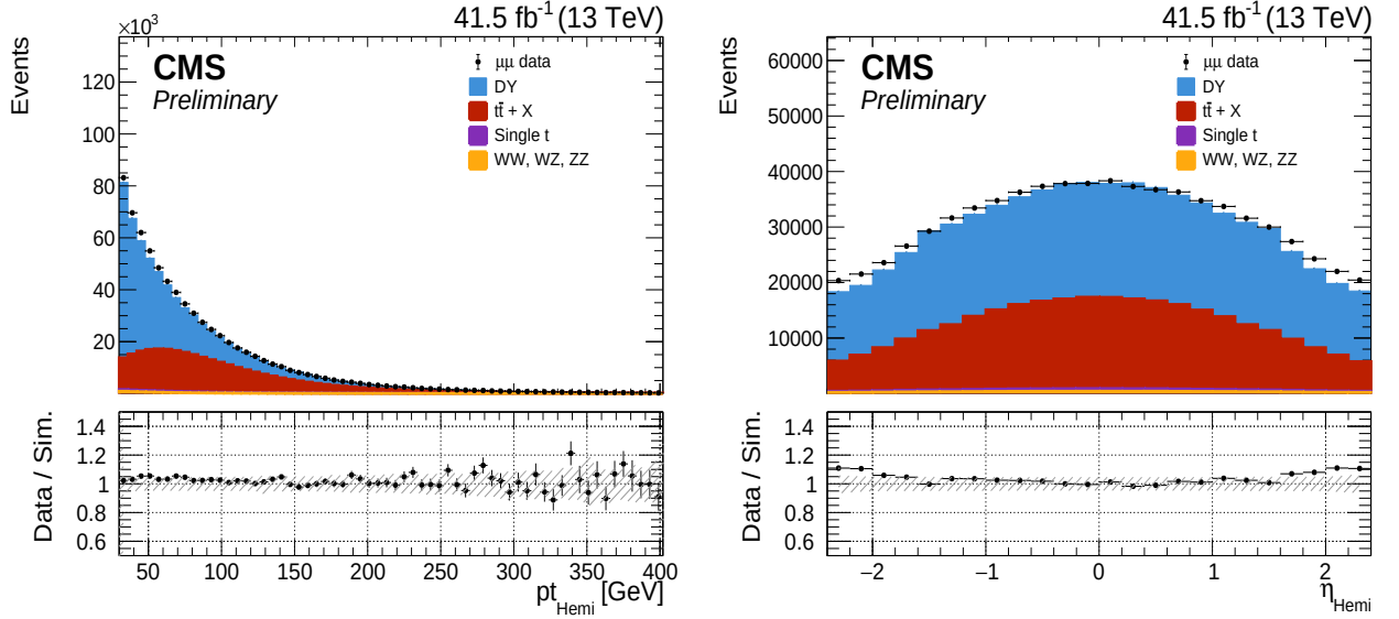
Figure D.20: p_T and \eta of the hemispheres in the 2017 \mu\mu data and MC. The hatched bands represent the systematic uncertainties.
