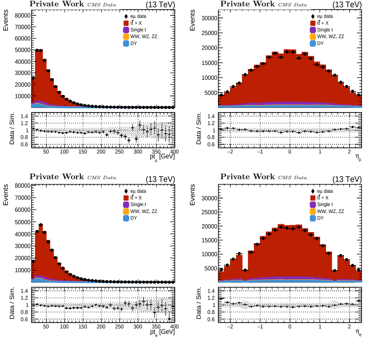
Figure 4.15: p_T and \eta of the leading muons and electrons in the 2018 e\mu data and MC. The hatched bands represent the systematic uncertainties.
