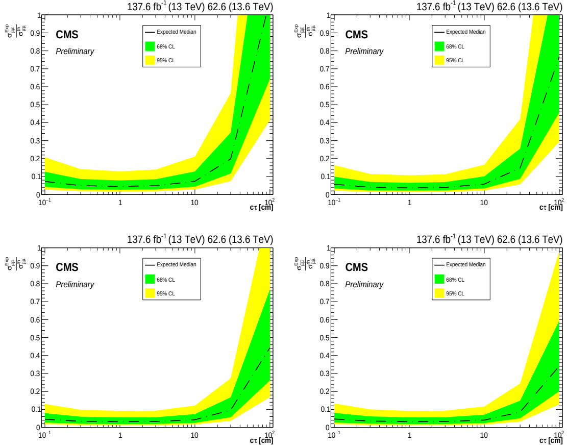
Figure G.4: \sigma_{\tilde{\mu}\tilde{\mu}} \times B_r(\tilde{\mu} \rightarrow \mu\tilde{\chi}_1^0)^2 assuming different mass combinations between the smuon and the neutralino S_{m_{\tilde{\chi}_1^0}}^{m_{\tilde{\mu}}} : (upper left) S_{180}^{400} (upper right) S_{200}^{400} (lower left) S_{250}^{400} (lower right) S_{300}^{400} . Signal samples for which the ratio of the cross sections is below 1 are excluded.
