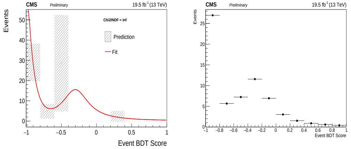
Figure F.1: (left) Fit of the background estimate in the signal region for 2016-pre \mu\mu data. (right) Toy experiments generated injected in the COMBINE tool to extract expected limits.
