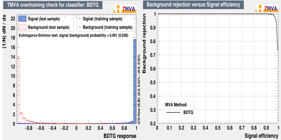
Figure 5.14: (Left) Training and test distributions for both (blue) signal and (red) background vertices. (Right) Associated ROC curve.
