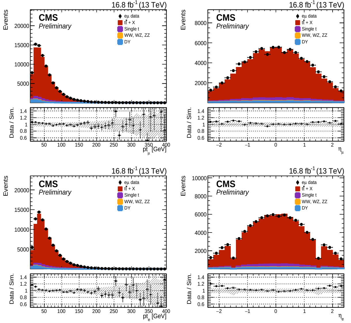
Figure D.11: p_T and \eta of the muons and electrons in the 2016-post e\mu data and MC. The hatched bands represent the systematic uncertainties.
