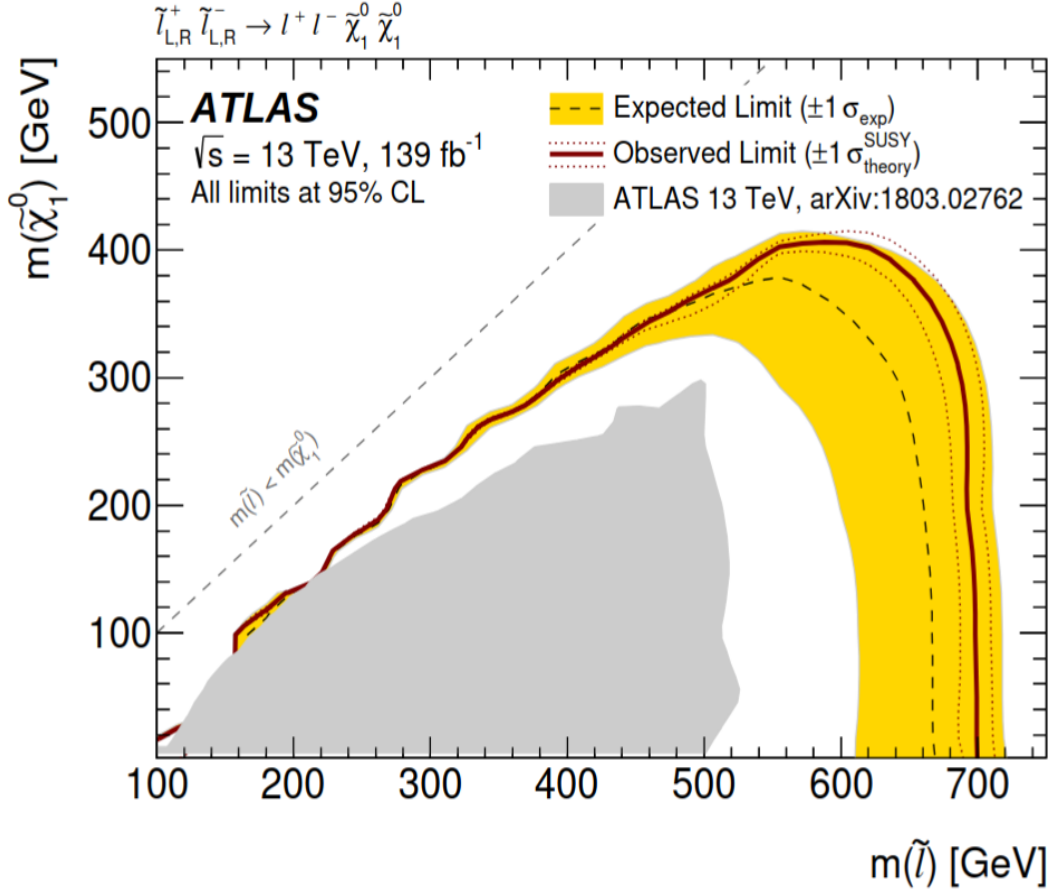
Figure 3.12: Upper limits at 95% CL on slepton pair production cross section as a function of the slepton and neutralino masses. The upper shaded band corresponds to the \pm 1\sigma variations in the expected limit, including all uncertainties except theoretical uncertainties in the signal cross section. The dotted lines around the observed limit illustrate the change in the observed limit as the nominal signal cross section is scaled up and down by the theoretical uncertainty [126]. The observed limits obtained by ATLAS in previous searches are also shown (lower shaded areas)
