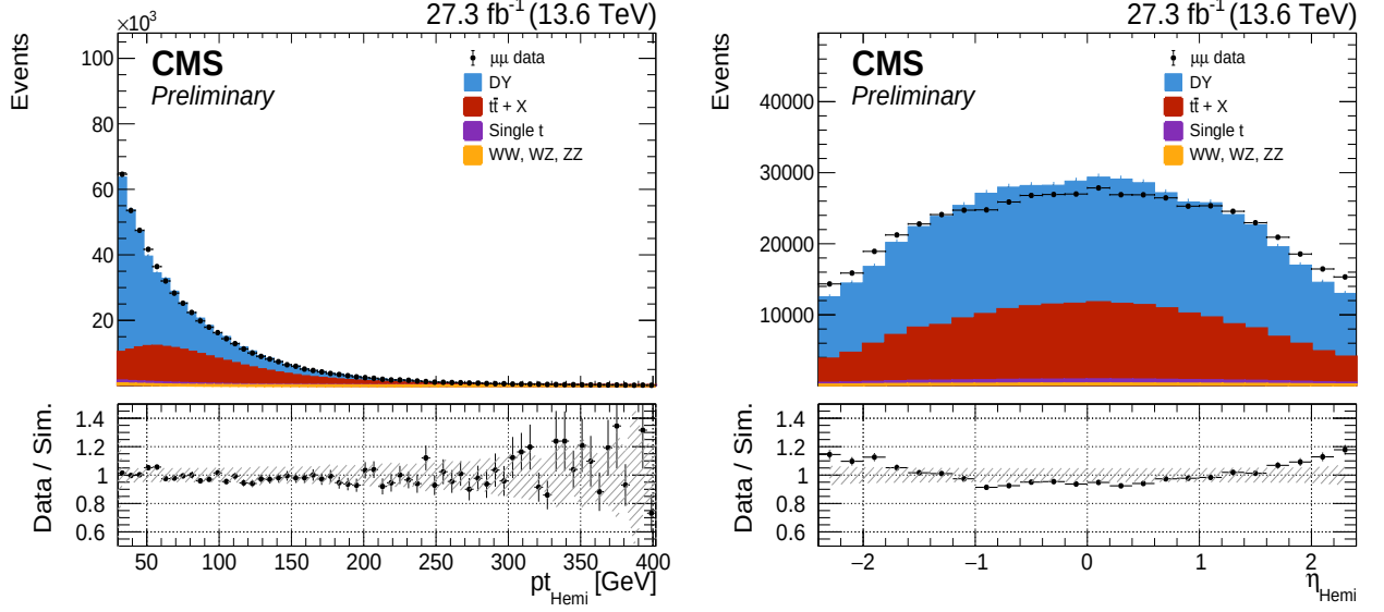
Figure D.39: p_T and \eta of the hemispheres in the 2023 \mu\mu data and MC. The hatched bands represent the systematic uncertainties.
