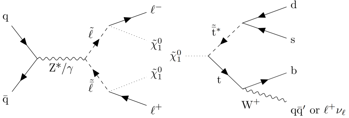
Figure 3.10: (Left) Feynman diagram (at LO QCD) related to the indirect production of neutralinos by sleptons. The electrical charge carried by the sleptons is given by the electrical charge of the associated leptons for clarity. (Right) Neutralino decay channel involving the \lambda'' coupling in the decay of the stop quark.
