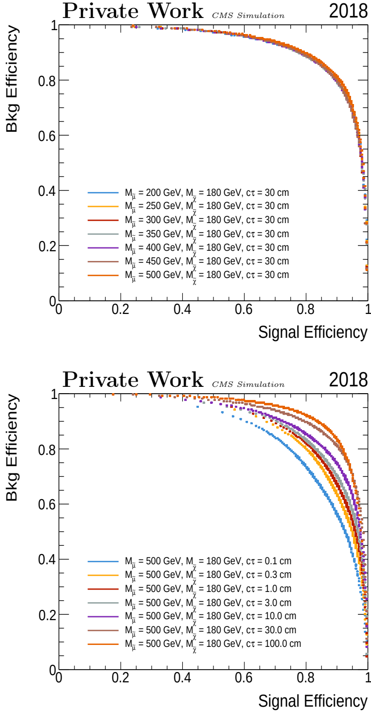
Figure 4.34: Background vs Signal efficiency for the track selection BDT for different signal samples.
