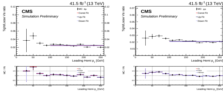
Figure D.23: Ratio of the number of tight over loose vertices as a function of the p_T of the leading hemisphere in the 2017 (left) e\mu MC and (right) \mu\mu MC.
