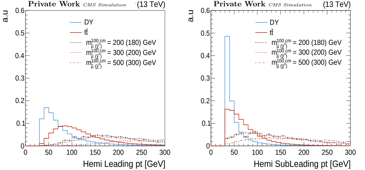
Figure 4.10: Distributions of the p_T of the leading (left) and sub-leading (right) hemispheres in the 2018 MC conditions for the DY, t\bar{t} MC background samples and three different signal samples normalized to unitary.
