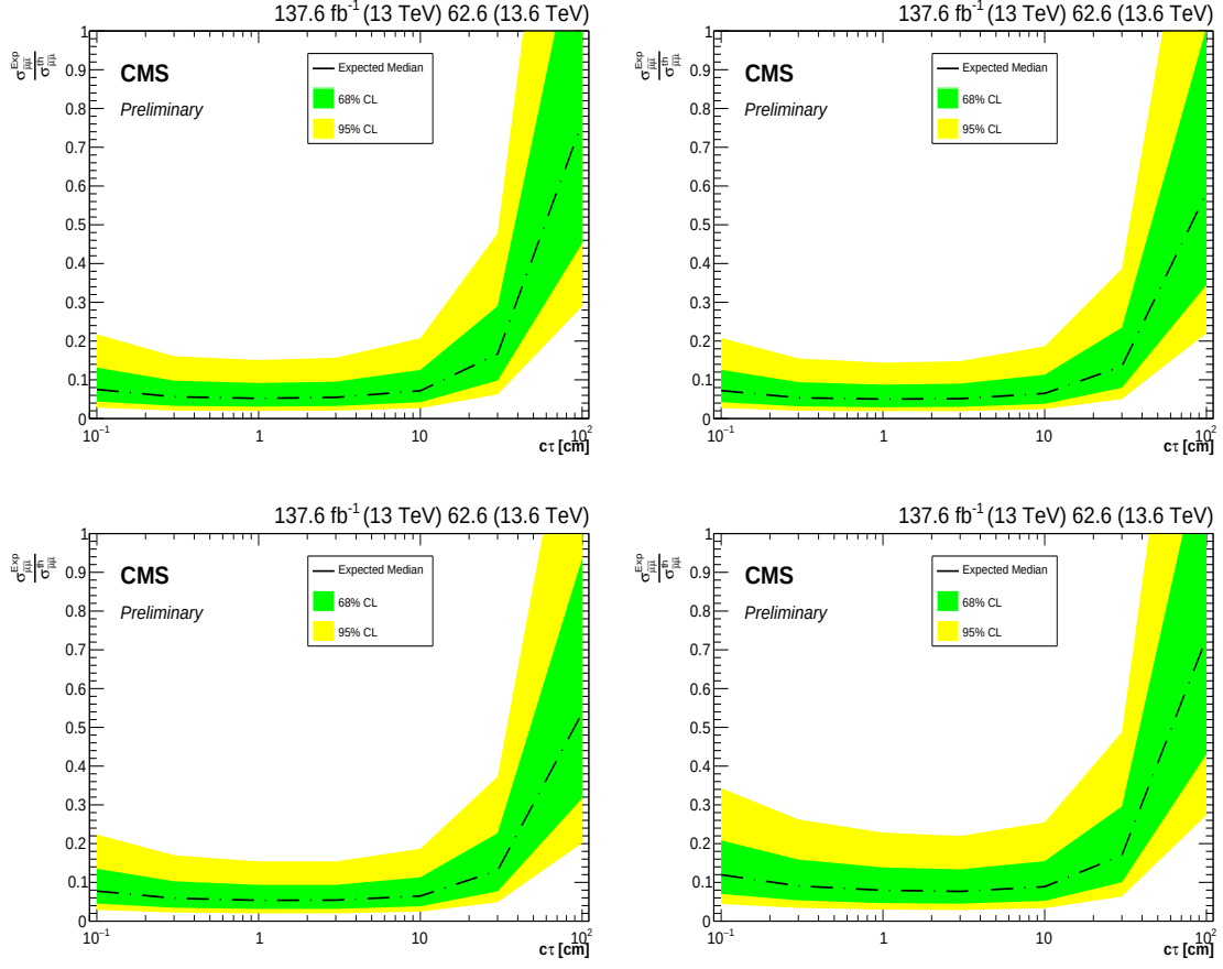
Figure G.6: \sigma_{\tilde{\mu}\tilde{\mu}} \times B_r(\tilde{\mu} \rightarrow \mu\tilde{\chi}_1^0)^2 assuming different mass combinations between the smuon and the neutralino S_{m_{\tilde{\chi}_1^0}}^{m_{\tilde{\mu}}} : (upper left) S_{250}^{450} (upper right) S_{300}^{450} (lower left) S_{350}^{450} (lower right) S_{400}^{450} . Signal samples for which the ratio of the cross sections is below 1 are excluded.
