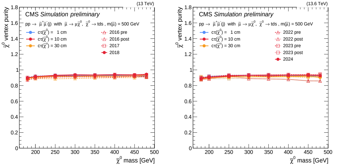
Figure C.5: Purity of the tight reconstructed displaced vertices as a function of the neutralino and smuon masses and c\tau_{\tilde{\chi}} in each MC year period of (left) Run 2 and (right) Run 3.
