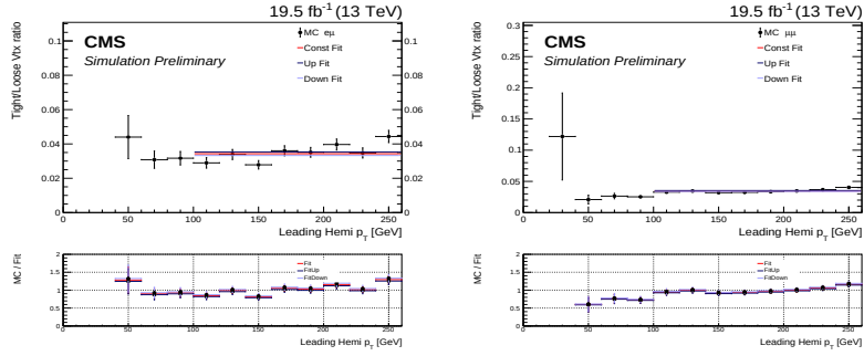
Figure D.7: Ratio of the number of tight over loose vertices as a function of the p_T of the leading hemisphere in the 2016-pre (left) e\mu MC and (right) \mu\mu MC.
