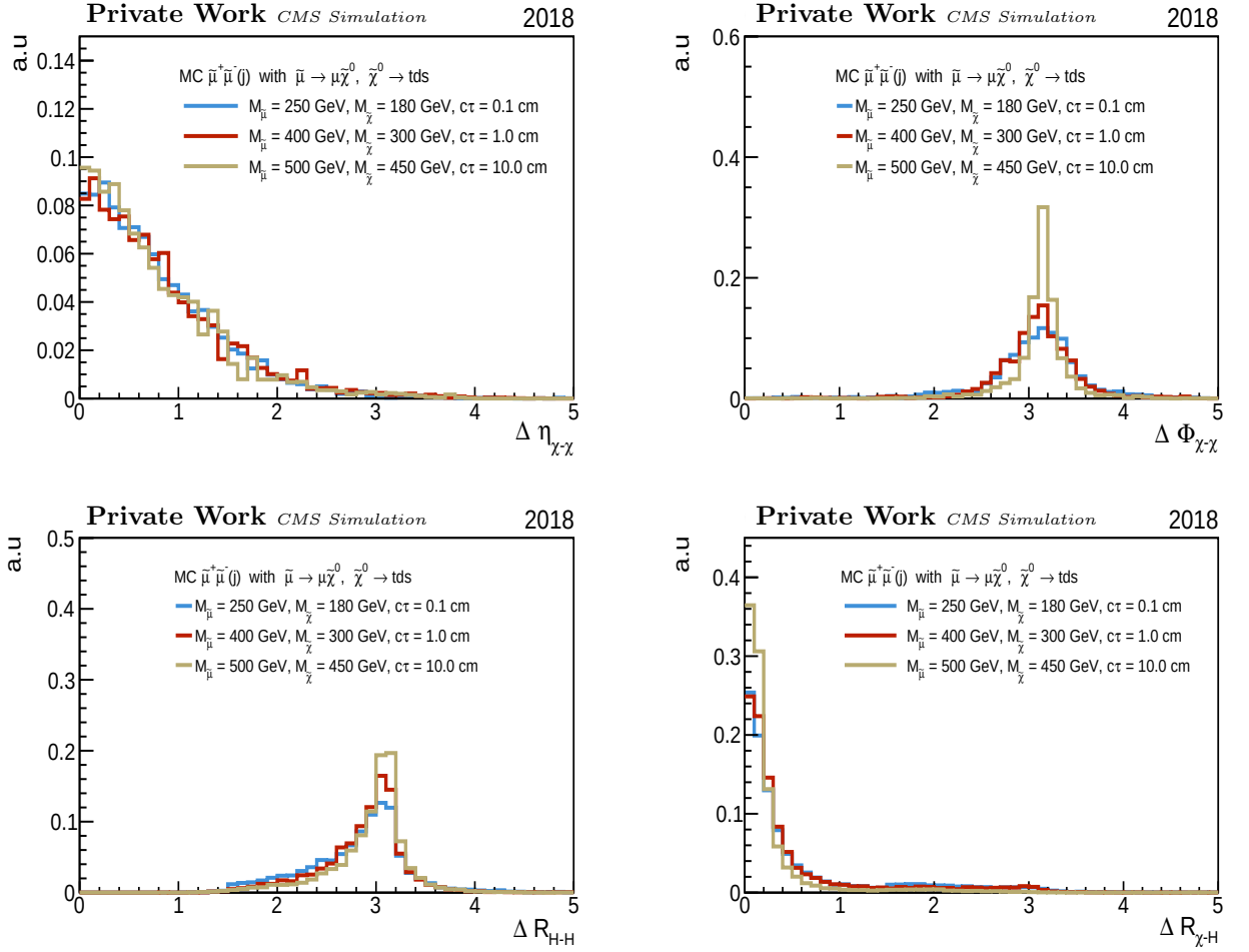
Figure 4.9: Characteristics of the generated neutralinos and reconstructed hemispheres in the 2018 MC conditions. Upper left (right): |\Delta\eta| ( |\Delta\phi| ) between the two generated neutralinos. Lower left: \Delta R between the two reconstructed hemisphere axes. Lower right: \Delta R between the generated neutralino direction and its closest hemisphere axis. Distributions are normalized to unit area.
