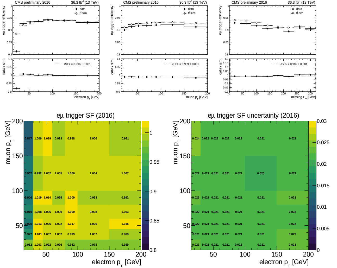
Figure E.1: The e\mu trigger efficiency and scale factor in 2016 datasets as a function of: (upper left) electron p_T , (upper middle) muon p_T , (upper right) E_T^{\text{miss}} (errors are statistical alone); and (lower left) 2D e\mu trigger scale factor and (right) its overall (stat. + syst.) uncertainty as a function of both electron and muon p_T . The last bins include the overflows.
