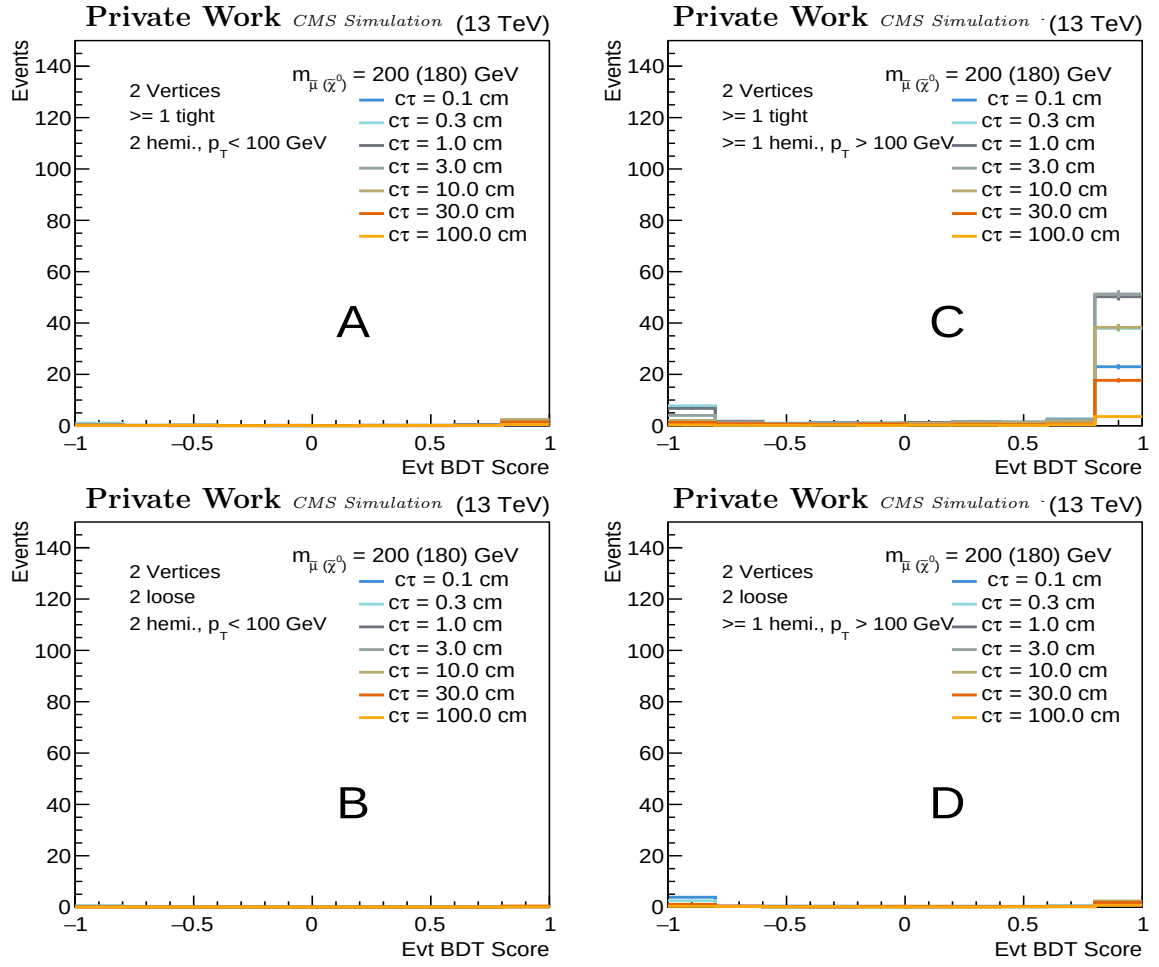
Figure 5.15: Event BDT score of two vertices in signal events with S_{m_{\tilde{\chi}_0^1}}^{m_{\tilde{\mu}}} = S_{180}^{200} in the 2018 MC conditions for various c\tau_{\tilde{\chi}} values.
