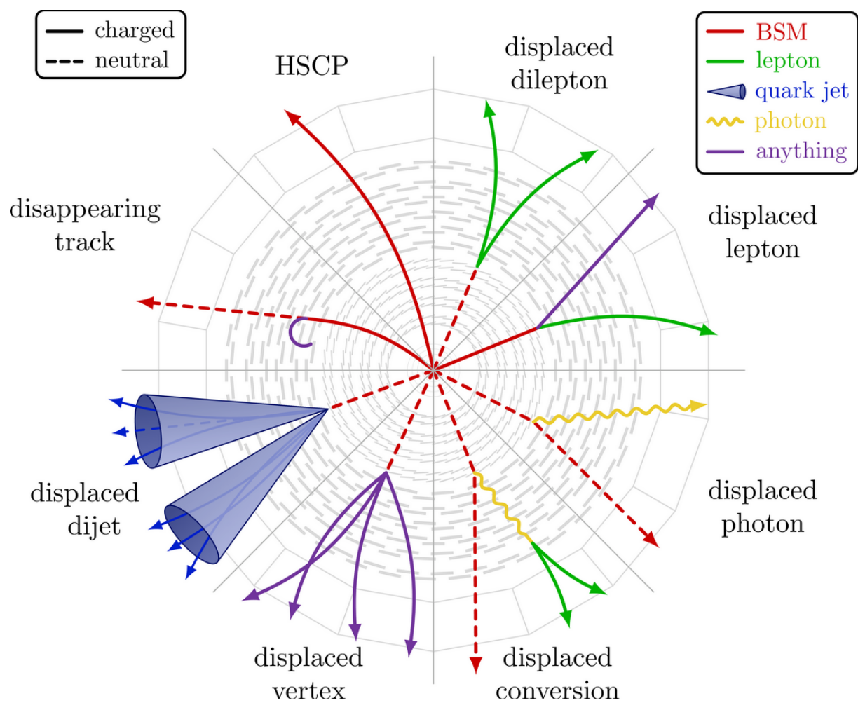
Figure 3.9: Long-lived experimental signatures within a typical LHC detector [25].
