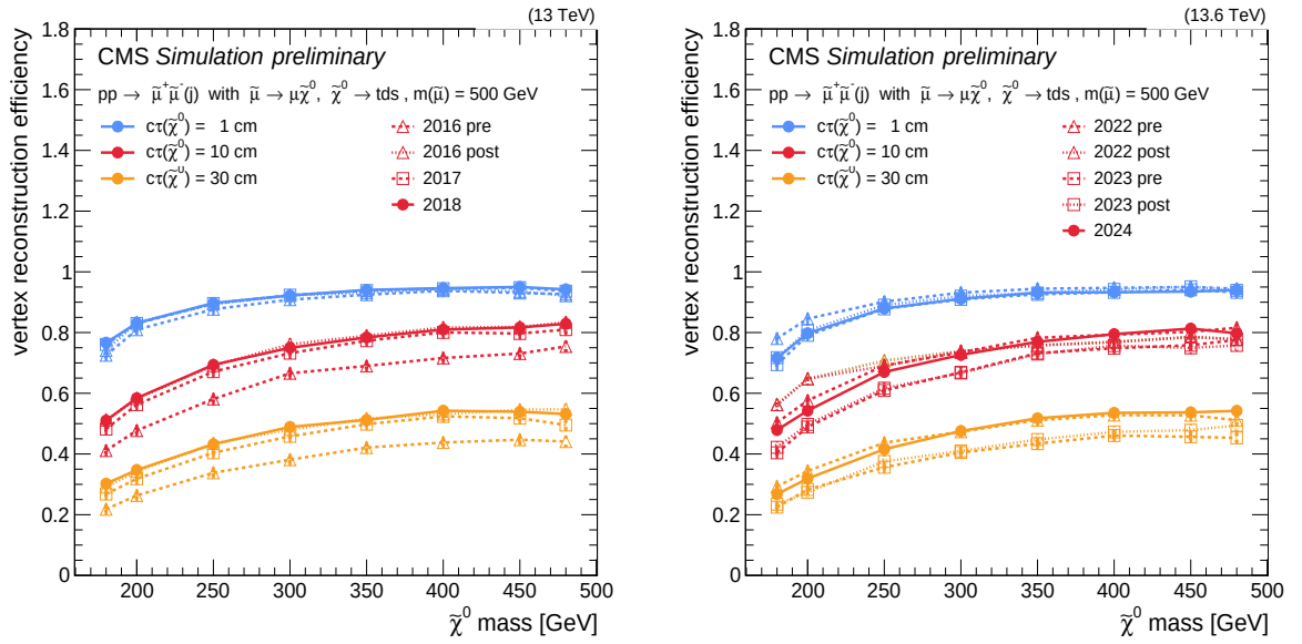
Figure C.6: Efficiency to reconstruct a tight displaced vertex as a function of the neutralino and smuon masses and c\tau_{\tilde{\chi}} in each MC year period of (left) Run 2 and (right) Run 3.
