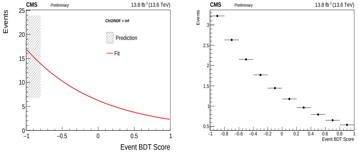
Figure F.4: (left) Fit of the background estimate in the signal region for 2022-pre \mu\mu data. (right) Toy experiments generated injected in the COMBINE tool to extract expected limits.
