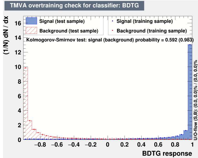
Figure 4.31: Test (histograms) and training (dots) track BDT for signal tracks (issued from neutralino decays) and background tracks.
