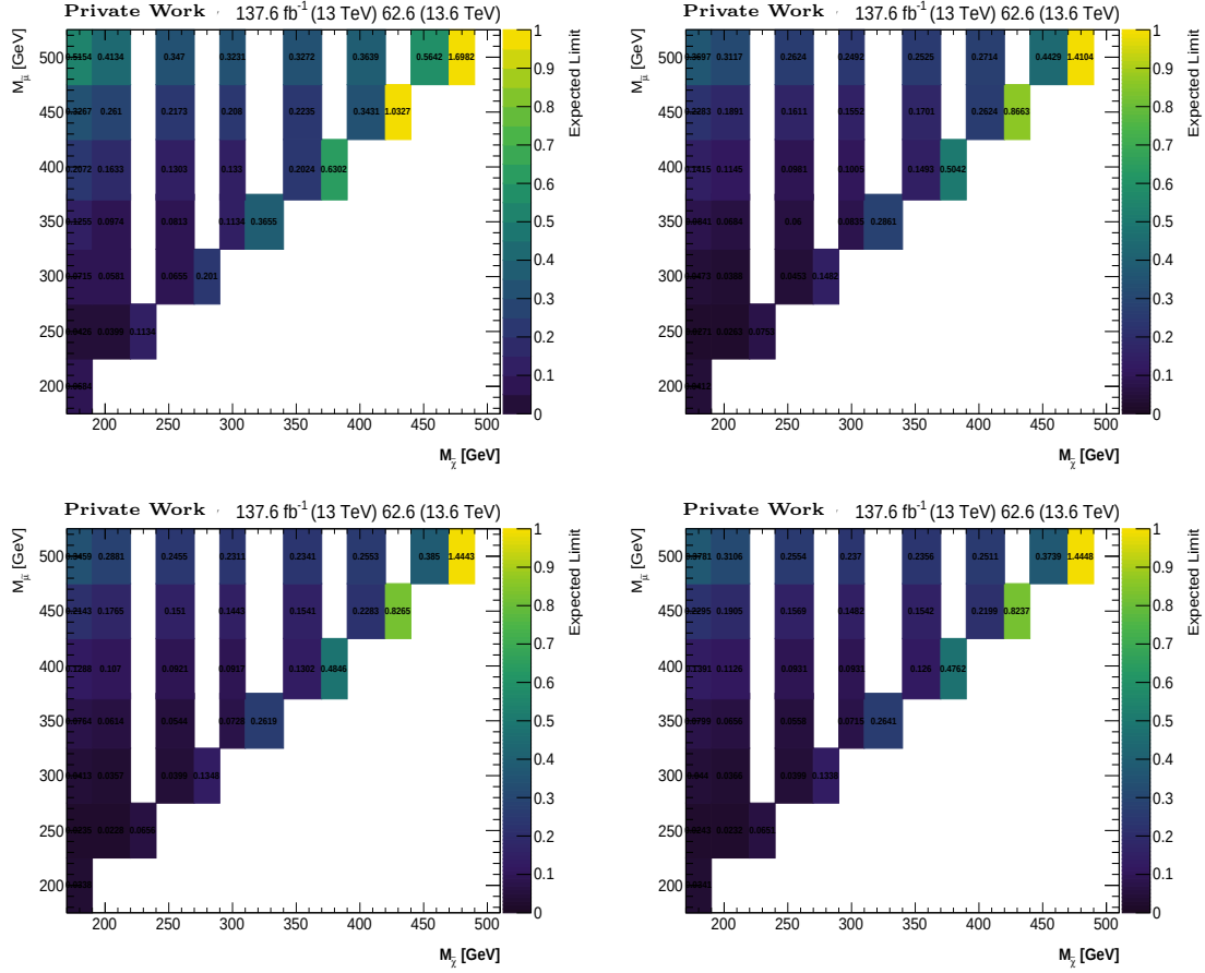
Figure 5.26: M_{\mu} vs M_{\chi_1^0} expected limits at a 95% confidence level assuming a mean c\tau_{\tilde{\chi}} of (upper left) 0.1 cm (upper right) 0.3 cm (lower left) 1.0 cm (lower right) 3.0 cm. The z -axis is the ratio of the expected cross section over the theoretical one. Signal samples with z -axis values below 1 are excluded. The center of each bin corresponds to a specific signal sample.
