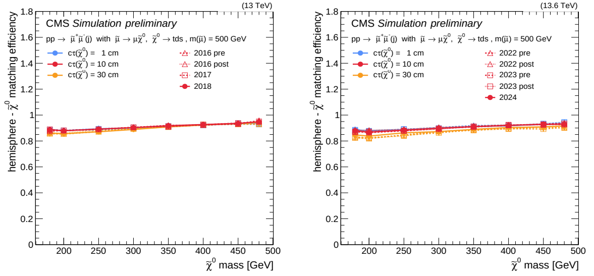
Figure C.2: Efficiency to match the reconstructed hemisphere axis and the nearest generated neutralino direction ( \Delta R < 1.5 ) as a function of the neutralino and smuon masses and c\tau_{\tilde{\chi}} in each MC year period of (left) Run 2 and (right) Run 3.
