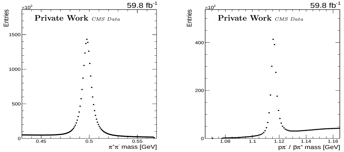
Figure 4.18: Invariant mass of (left) K_S and (right) \Lambda candidates from the \mu\mu data sample in 2018.
