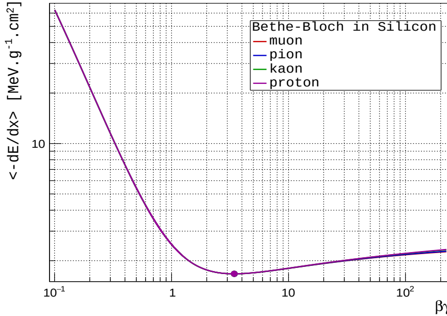
Figure 2.2: Bethe-Bloch distribution of the muon, pion, kaon and proton in silicon as a function of the Lorentz boost.
