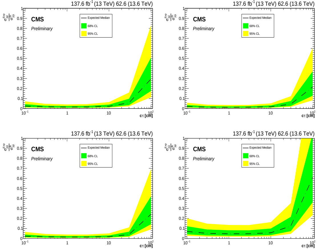
Figure G.2: \sigma_{\tilde{\mu}\tilde{\mu}} \times B_r(\tilde{\mu} \rightarrow \mu\tilde{\chi}_1^0)^2 assuming different mass combinations between the smuon and the neutralino S_{m_{\tilde{\chi}_1^0}}^{m_{\tilde{\mu}}} : (upper left) S_{180}^{300} (upper right) S_{200}^{300} (lower left) S_{250}^{300} (lower right) S_{280}^{300} . Signal samples for which the ratio of the cross sections is below 1 are excluded.
