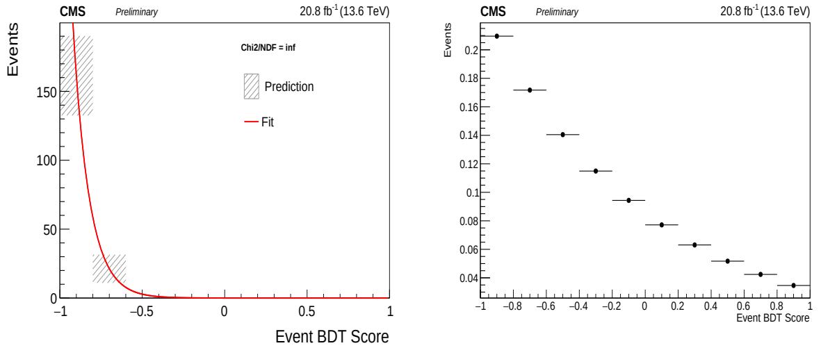
Figure F.5: (left) Fit of the background estimate in the signal region for 2022-post \mu\mu data. (right) Toy experiments generated injected in the COMBINE tool to extract expected limits.
