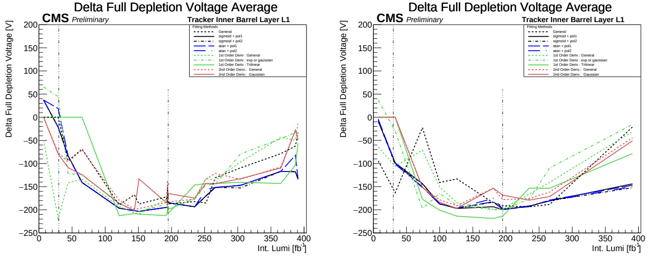
Figure B.3: Leakage current method applied to (left) small scan modules and (right) all the modules of the TIB L1 layer showing the \Delta V_{FD} . The last point of the right plot comes from the noise scan performed at the end of the 2024 operations. The black dashed lines are the LS1 and LS2.
