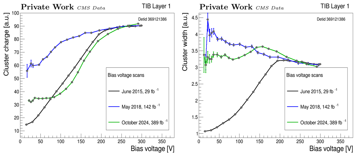
Figure 2.24: (Left) Cluster charge curves and (Right) cluster width curve. The scans were performed at the beginning of Run 2 (2015), at the end of Run 2 (2018) and at the middle of Run 3 operations (2024). The plots are shown for one TIB L1 module.
