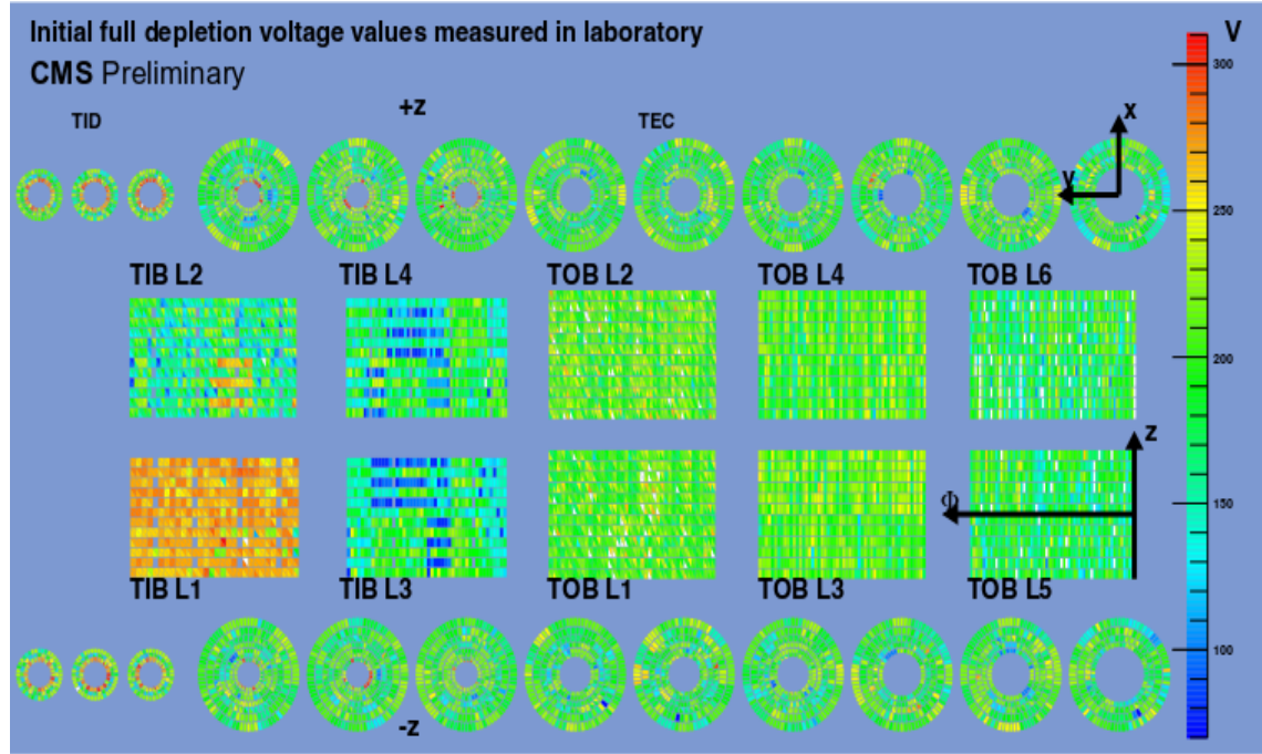
Figure 2.9: Initial full depletion voltage values measured in laboratory at the time of tracker construction. The values were extracted from the analysis of curves of the capacitance as a function of the bias voltage. For the TOB and TEC modules with two sensors, the lowest value is shown. The sensors of the most inner layer have a larger value of the initial full depletion voltage to allow a larger evolution range as they will receive a larger fluence. [77].
