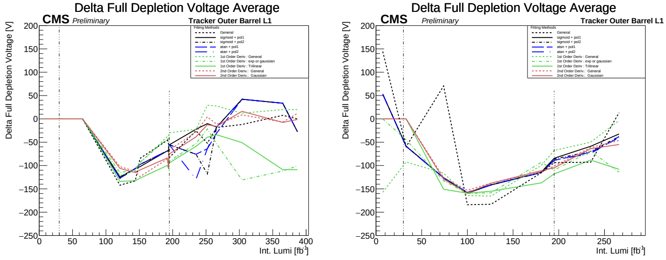
Figure B.5: Leakage current method applied to (left) small scan modules and (right) all the modules of the TOB L1 layer showing the \Delta V_{FD} . The last point of the right plot comes from the noise scan performed at the end of the 2024 operations. The black dashed lines are the LS1 and LS2.
