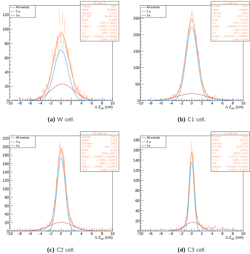
Figure A.1: Z_{\text{vtx}} resolution for the realistic hit treatment, considering a squared pixel detector.
