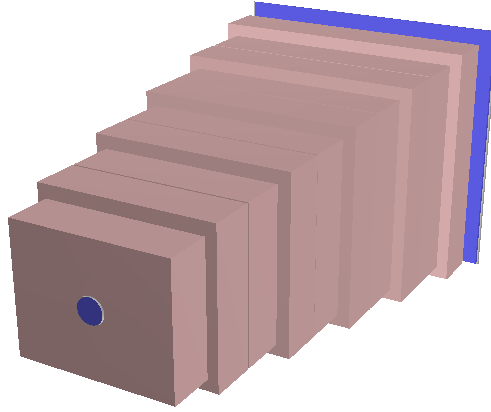
Figure 3.7: Implementation of the hadron absorber (in red Al_2O_3 and blue Fe) in TGEANT.
