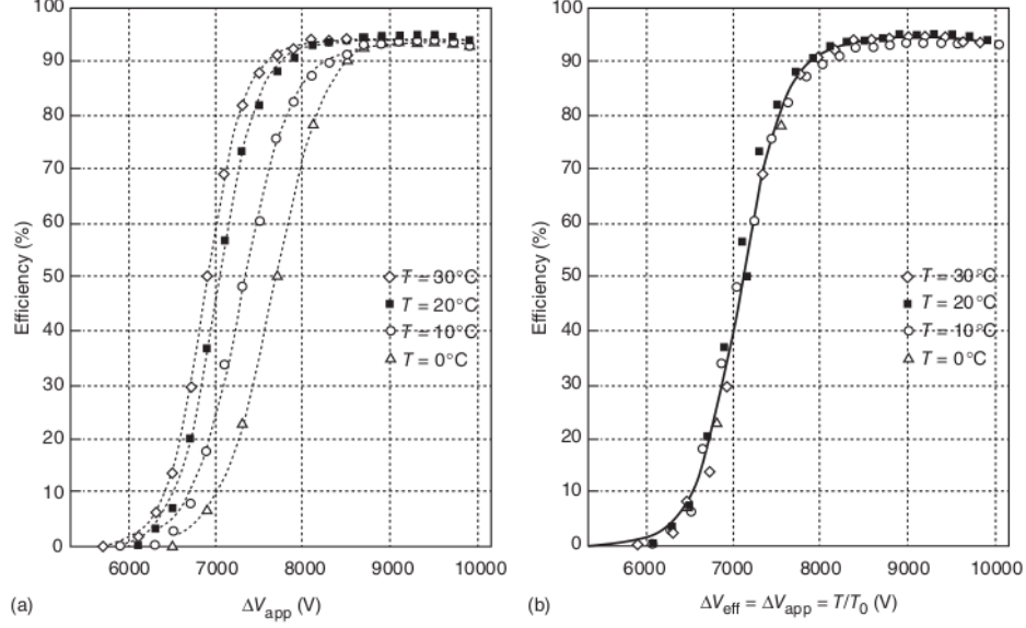
Figure 2.12: Effect of showing efficiency curves taken at different temperatures as a function of the applied high voltage (left panel) and as a function of the effective high voltage (right panel).
