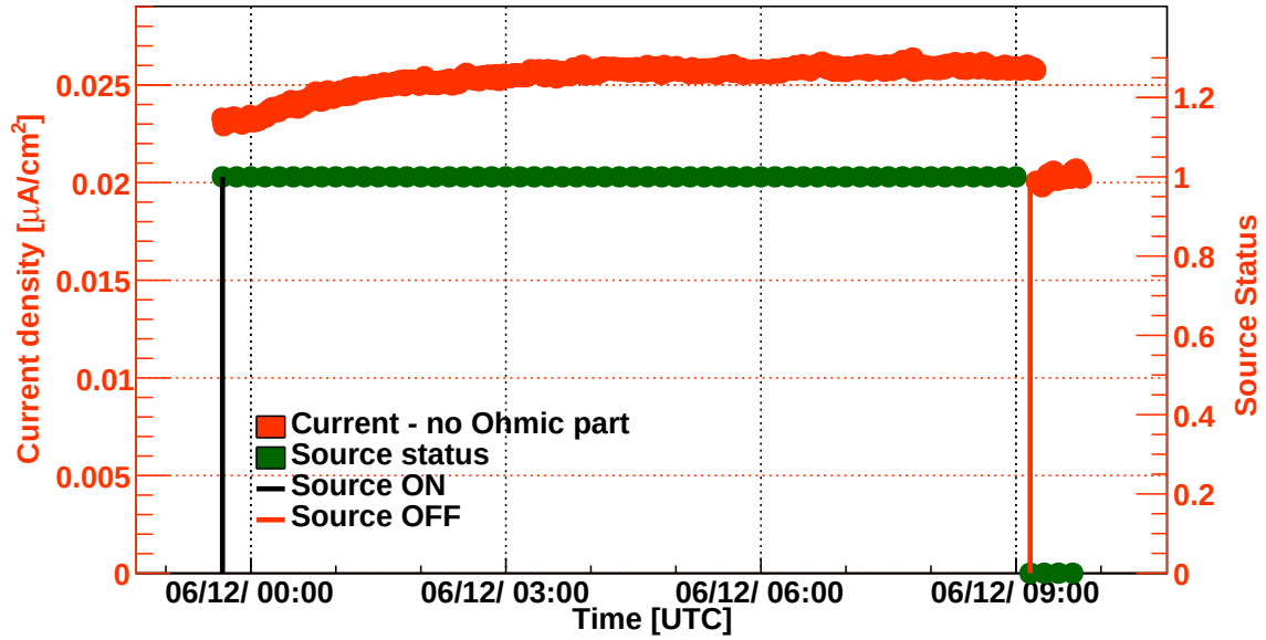
Figure 5.4: The effect of completely shielding the ^{137}\text{Cs} source during an irradiation period is a reduction of the absorbed current - example for the EP-DT detector
