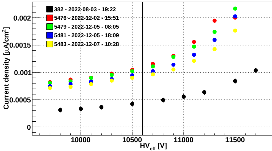
Figure 5.20: I(HV) source off scans taken with lower humidity (dew point set to 0.5 °C). The scan in black was taken before the current increase
