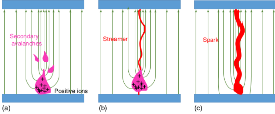
Figure 2.2: Stages of charge multiplication evolution and degeneration to a spark when the avalanche charge approaches the Raether limit. (a) field lines close to the avalanche experience a focusing effect and some secondary avalanches start moving toward the positive ions avalanche body (b) a thin plasma filament – a streamer is created (c) when the streamer reaches the electrodes, a spark happens through the channel. Figure taken from [74]
