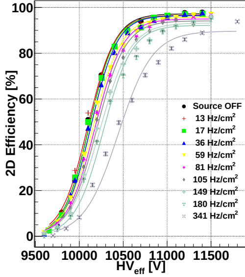
(a) Efficiency curves under irradiation for MIX5. High voltage not corrected for drop on bakelite, data from the front-end electronics
