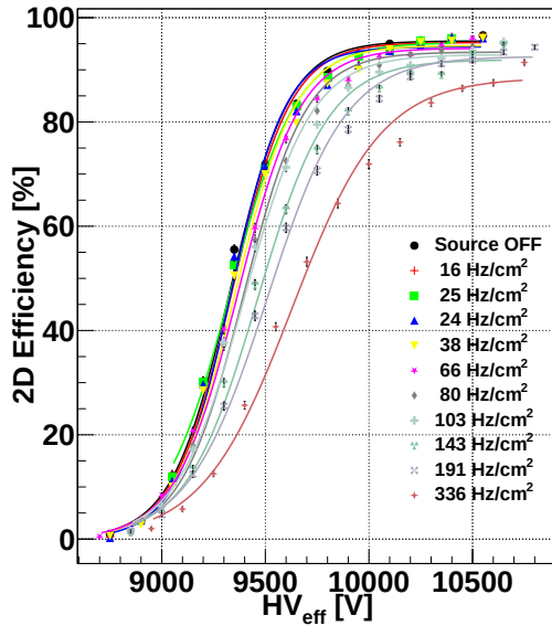
(a) MIX3 efficiency curves as a function of HV_{eff}
