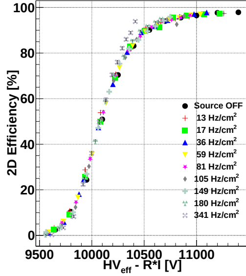
(b) Efficiency curves under irradiation for MIX5. High voltage corrected for drop on bakelite, data from the front-end electronics
