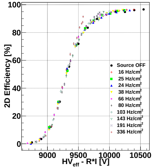
(b) MIX3 efficiency curves as a function of HV_{gas}
