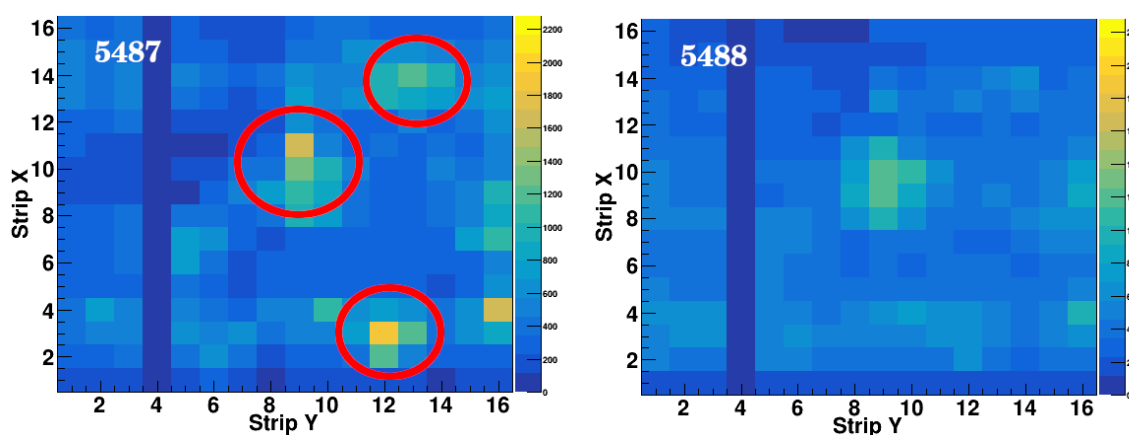
(b) Left panel: run 5487. Right panel: run 5488. Run 5487 was taken \sim 40 hours after run 5486. Hot-spots are still visible. Between run 5487 and 5488, the high voltage was kept off for \sim 8 hours, the hot-spots start to cool down
