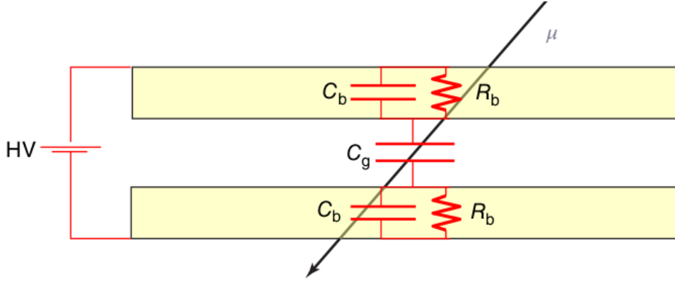
Figure 2.4: Simplified circuit representation of an RPC detector when crossed by an ionizing particle. C_b and C_g represent the capacitance of the bakelite and the gas; R_b is the resistance of the bakelite. Figure taken from [74]
