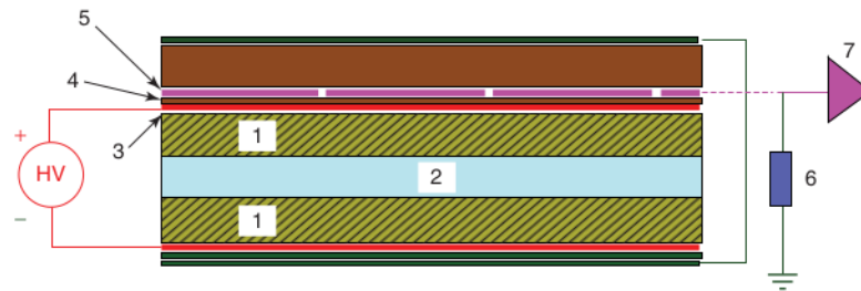
Figure 2.5: Cross section of an RPC detector. 1 = bakelite electrodes, 2 = gas gap, 3 = HV electrodes, 4 = Mylar insulating layers, 5 = readout strips, 6 = resistor, 7 = readout electronics. Figure taken from [74]
