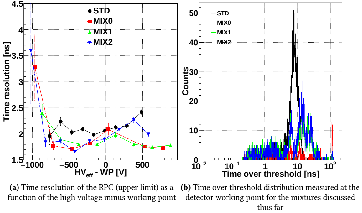
Figure 4.31: Left panel: time resolution trend as a function of the high voltage minus working point. Right panel: time over threshold distributions at working point for the mixtures tested. HFO/CO 2 : 0/95,10/85,20/75 (MIX0, MIX1, MIX2) - source off
