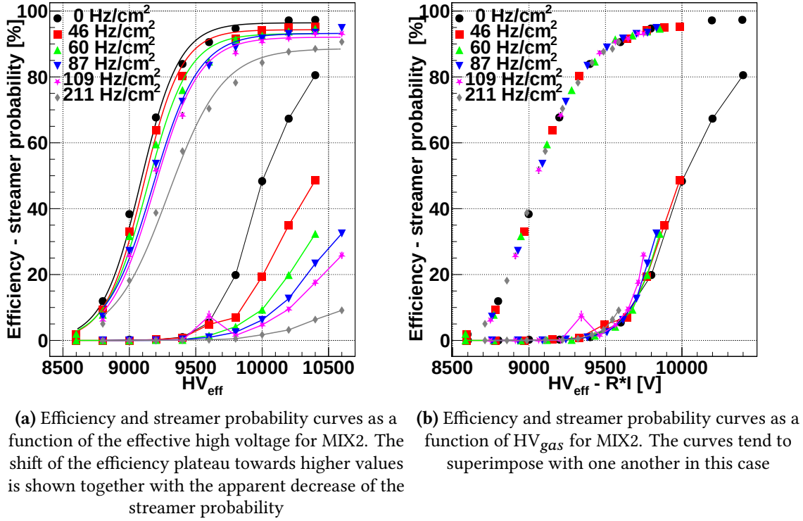
Figure 4.35: Effect of showing efficiency and streamer probability curves under irradiation as a function of the effective high voltage (left panel) and HV_{gas} (right panel).
