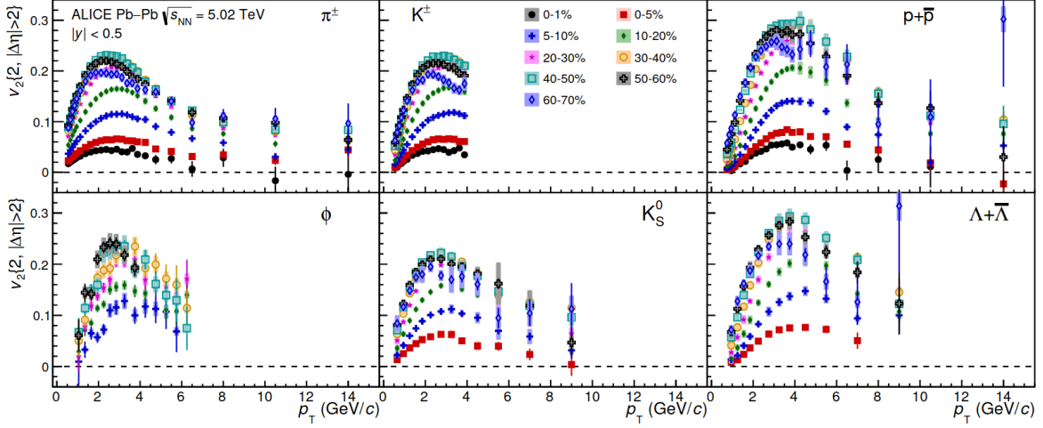
Figure 1.6: v_2 coefficient as a function of the particle p_T for different centrality classes and various particles ( \pi^\pm , K^\pm , p+\bar{p} , \phi , K_S^0 and \Lambda+\bar{\Lambda} ). Figure taken from [34]
