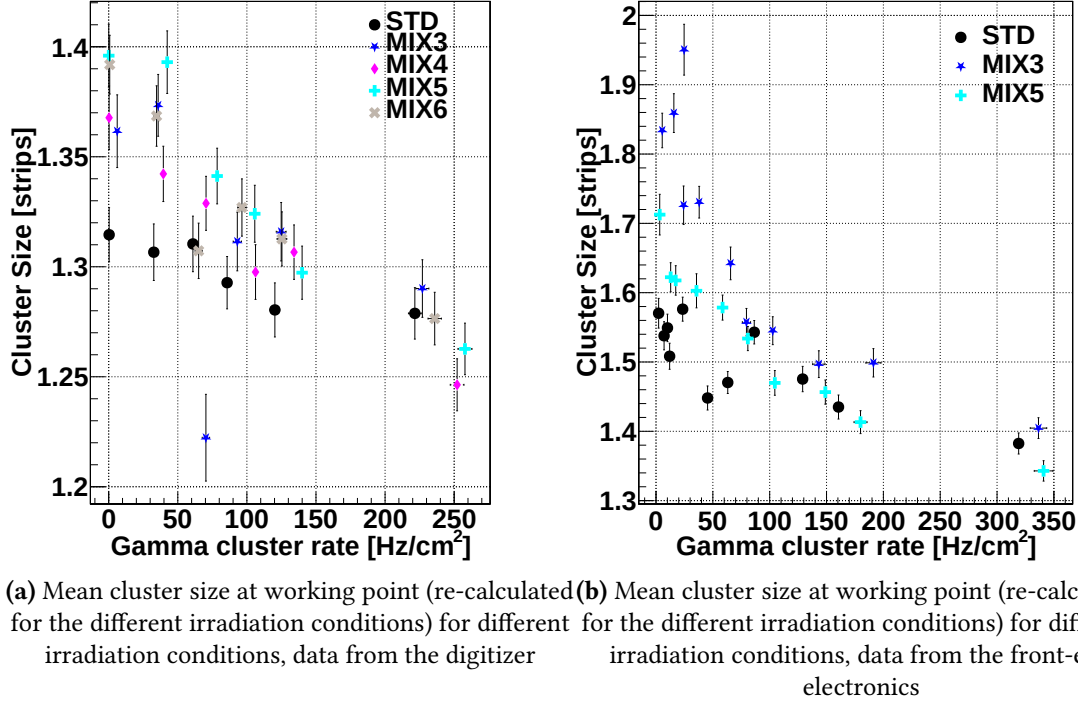
Figure 4.57: Mean cluster size as a function of the measured gamma rate
