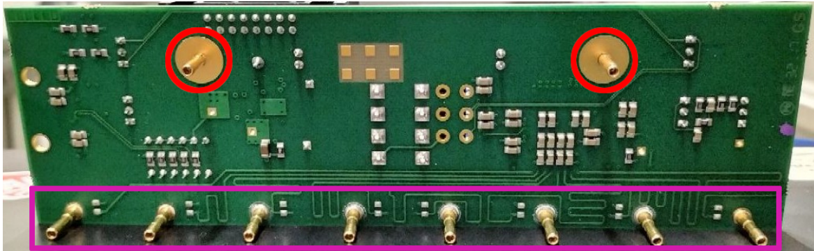
(b) Figure 4.11b Back view of the FEERIC front-end board. Circled in red are the ground pins while the pins highlighted in violet are used to couple the board to the RPC strips
