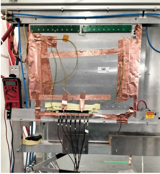
Figure 4.6: Front view of the ALICE RPC with digitizer connection
