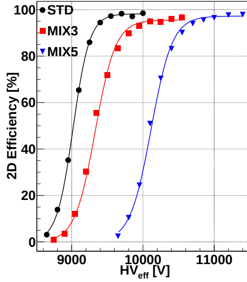
Figure 4.43: Efficiency curves obtained without irradiation, using the new ALICE front-end electronics. HFO/CO 2 : 25/69,35/60 (MIX3, MIX5)
