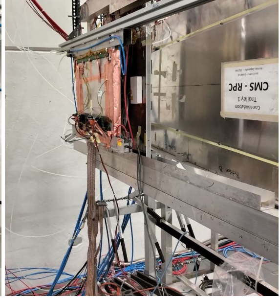
Figure 4.7: Side view of the ALICE RPC with FEERIC connections
