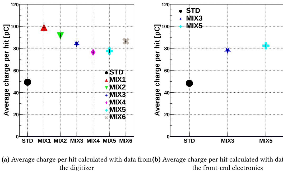
Figure 4.59: Average charge per hit obtained with the digitizer and the front-end electronics
