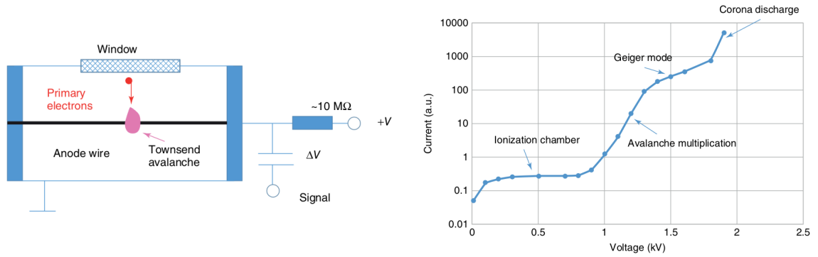
Figure 2.3: Left panel: sketch of single-wire cylindrical counter. Right panel: typical response of single-wire counter in terms of current as a function of the applied high voltage. Figures taken from [74]
