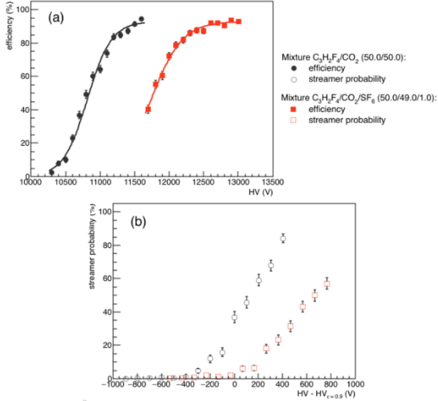
Figure 3.7: Top panel: Efficiency curves for a gas mixture based on HFO and CO_2 , with and without SF_6 . Adding 1% SF_6 shifts the working point by \sim 1 kV towards higher voltages. Bottom panel: streamer contamination curves for the same mixtures described above. The SF_6 addition greatly lowers streamer contamination, down to \sim 5\% at working point. This is compatible with the ALICE standard gas mixture performance. The working point is almost 2 kV higher with respect to the standard gas mixture. Figure taken from [125]
