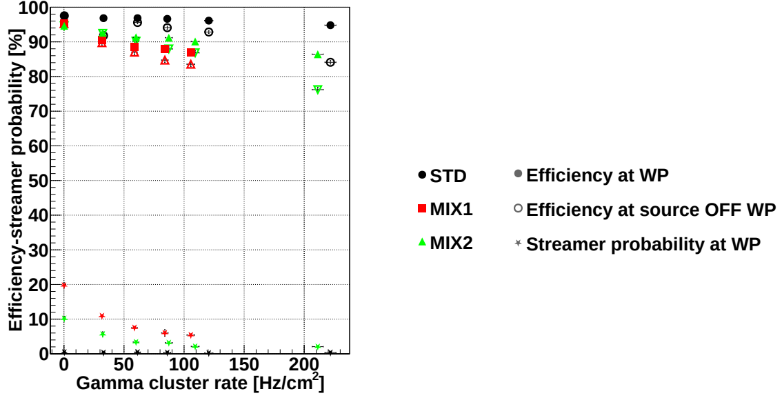
Figure 4.38: Efficiency and streamer probability computed at working point and source-off working point as a function of the gamma rate on the detector for the different mixtures. HFO/CO 2 : 10/85,20/75 (MIX1, MIX2). The source-off condition is also reported in the chart
