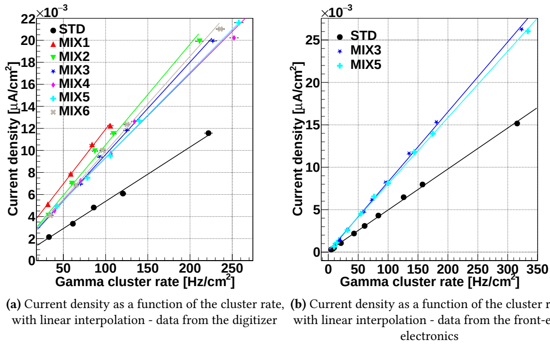
Figure 4.58: Current density vs cluster rate trends. Cluster rate measured with the digitizer and the front end electronics. The source off values have been subtracted in both cases
