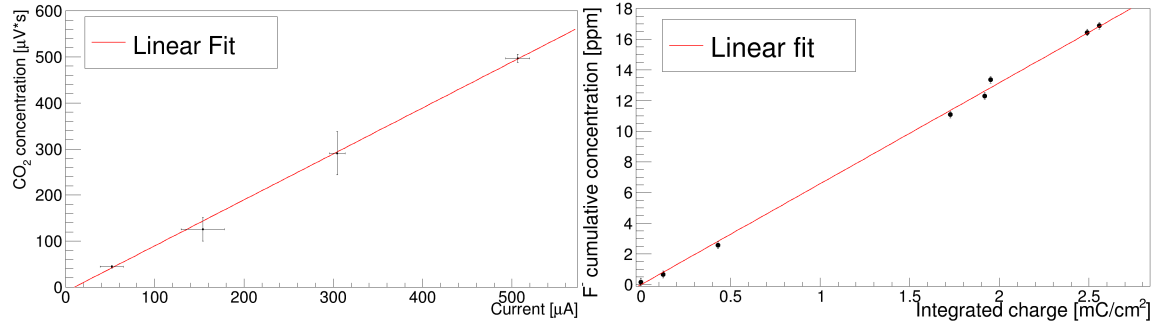
Figure 2.20: Left panel: trend of \text{CO}_2 concentration as a function of the current. Right panel: trend of \text{F}^- ions production as a function of the integrated charge during the Ar plasma test. In both cases the RPCs were flushed with Ar. Figures taken from [110]
