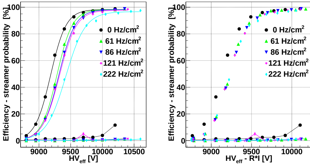
(a) STD efficiency - streamer probability curves as a function of HV_{eff} (b) STD efficiency - streamer probability curves as a function of HV_{gas}
