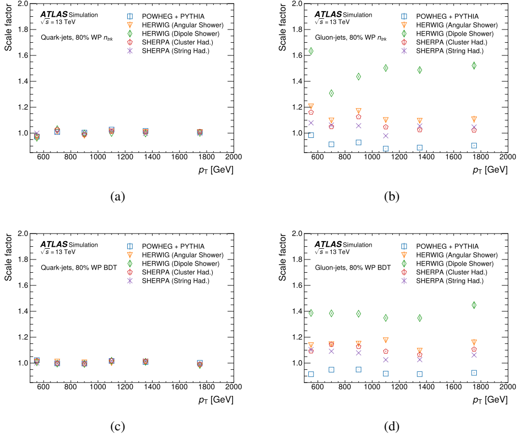
Figure 5.46 The MC-to-MC SF of the N_{\text{trk}} , (a) and (b), and BDT, (c) and (d), as a function of jet p_T for quark-jets (left) and gluon-jets (right) at the 80% WP. The vertical error bars show the statistical uncertainty.
