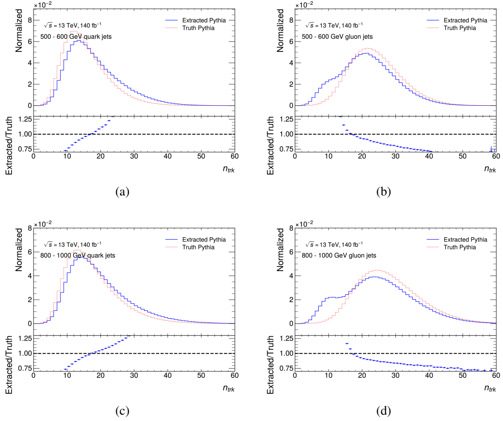
Figure 5.24 Before re-weighting: the N_{\text{trk}} distributions of quark-jet (a) (c) and gluon-jet in (b) (d) from PYTHIA 8 sample. Dashed and solid-line show the N_{\text{trk}} distributions in the truth MC and extracted MC, respectively. Bottom panels show the ratio of the extracted MC to the truth MC.
