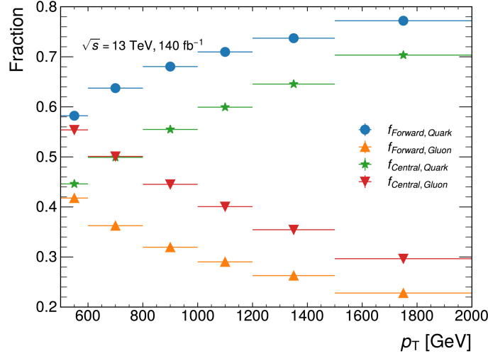
Figure 5.36 Fractions of quark jets and gluon jets in POWHEG samples.
