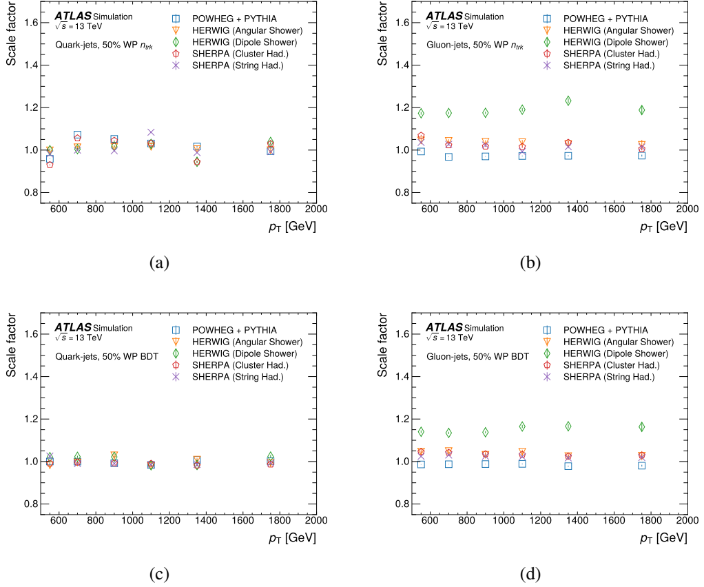
Figure 5.43 The MC-to-MC SF of the N_{\text{trk}} , (a) and (b), and BDT, (c) and (d), as a function of jet p_T for quark-jets (left) and gluon-jets (right) at the 50% WP. The vertical error bars show the statistical uncertainty.
