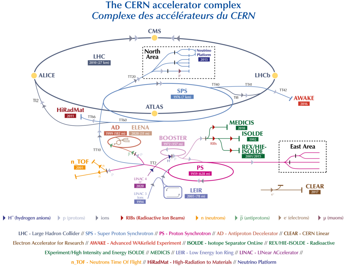
Figure 3.3 The CERN accelerator complex
