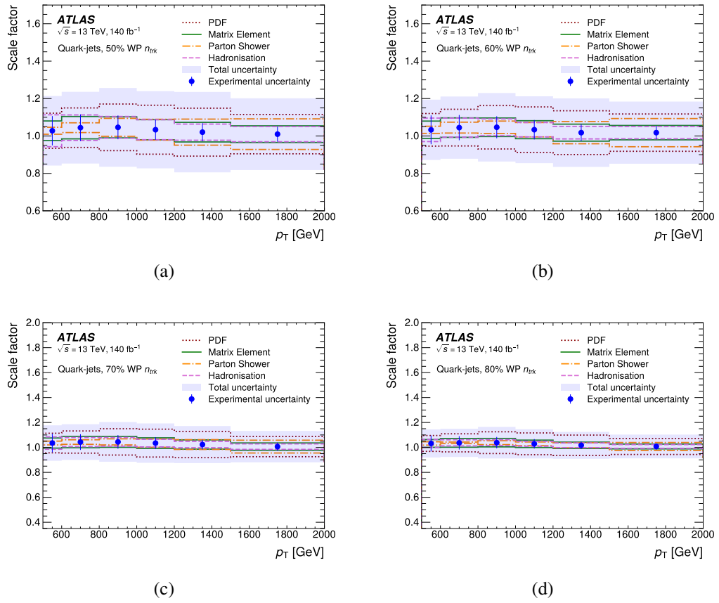
Figure 5.39 The SF with total and leading systematic uncertainty on the jet tagging variable N_{trk} obtained by PYTHIA 8 MCs as a function of jet p_T for quark-jets at each WP.
