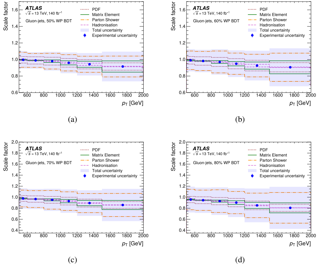
Figure 5.42 The SF with total and leading systematic uncertainty on the jet tagging variable BDT obtained by PYTHIA 8 MCs as a function of jet p_T for gluon-jets at each WP.
