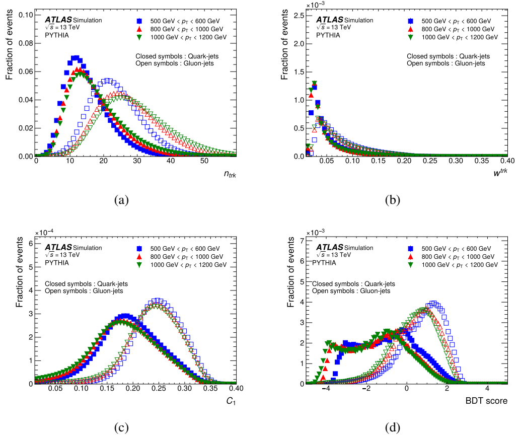
Figure 5.18 The distributions of N_{\text{trk}} (a), W_{\text{trk}} (b), C_1 (c) and BDT score (d) in the quark-jets (closed symbols) and gluon-jets (open symbols) in given p_T regions using the PYTHIA MC samples.
