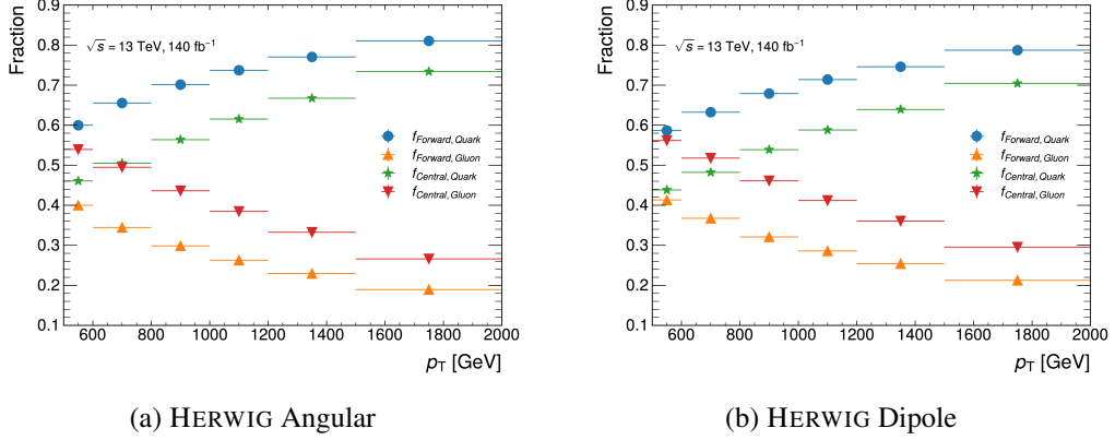
Figure 5.34 Fractions of quark- gluon-jets of HERWIG angular (a) and HERWIG dipole (b) samples.
