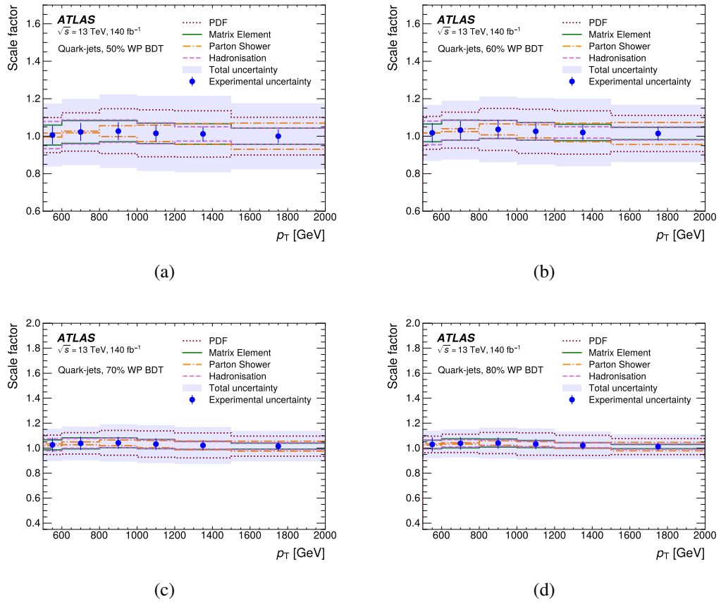
Figure 5.41 The SF with total and leading systematic uncertainty on the jet tagging variable BDT obtained by PYTHIA 8 MCs as a function of jet p_T for quark-jets at each WP.
