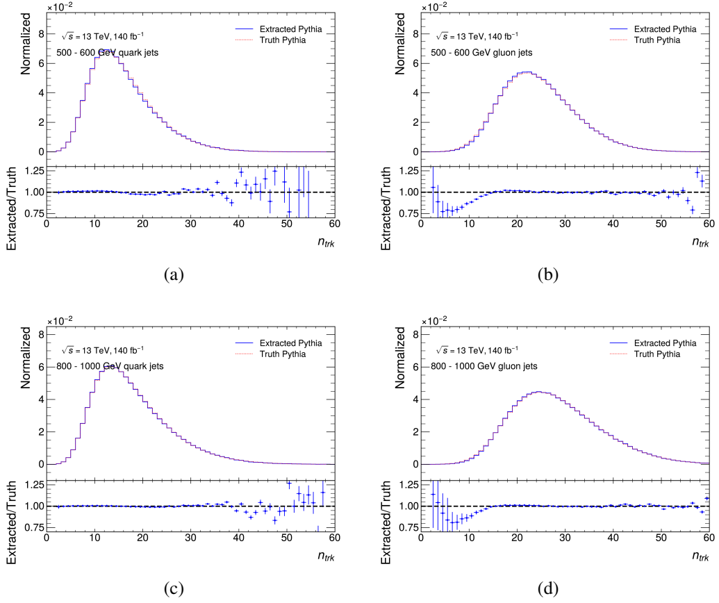
Figure 5.25 After re-weighting with quark factor: the N_{trk} distributions of quark-jet (a) (c) and gluon-jet in (b) (d) from PYTHIA 8 sample. Dashed and solid-line show the N_{trk} distributions in the truth MC and extracted MC, respectively. Bottom panels show the ratio of the extracted MC to the truth MC.
