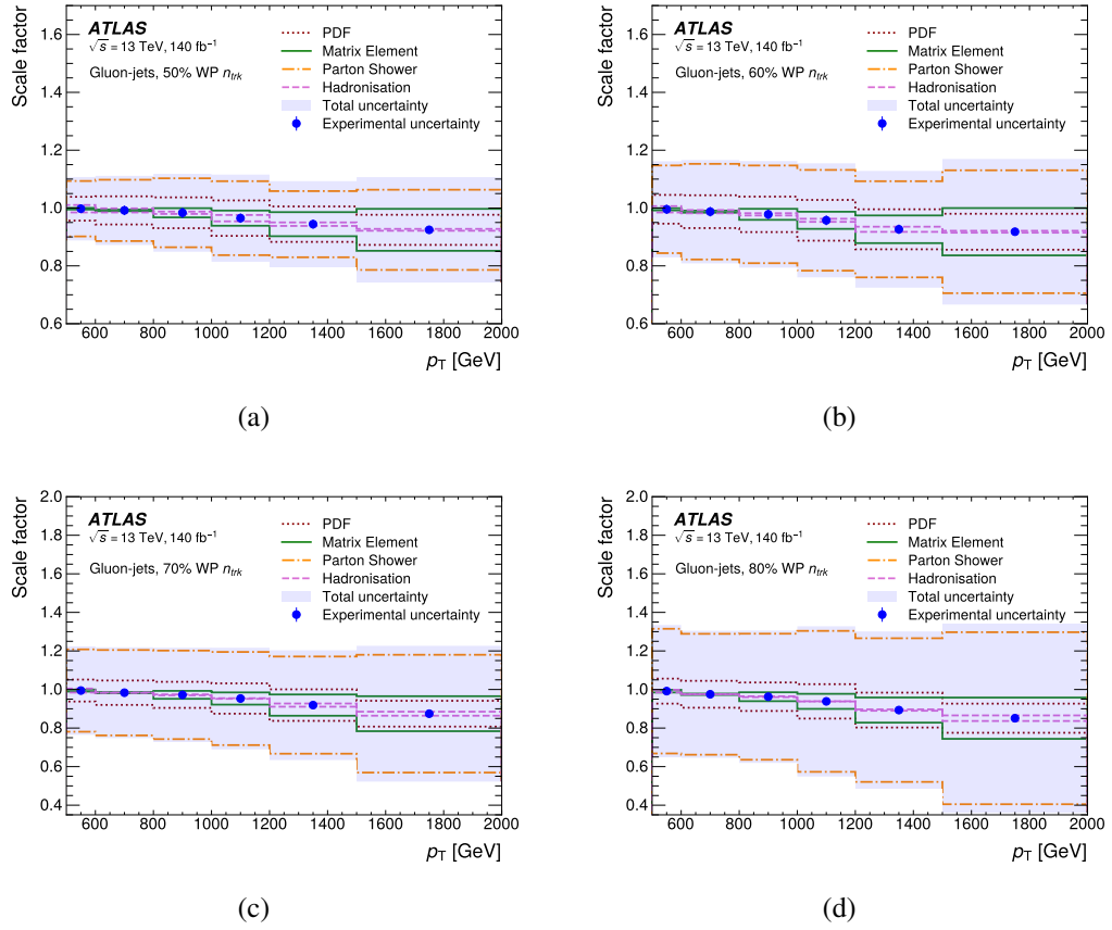
Figure 5.40 The SF with total and leading systematic uncertainty on the jet tagging variable N_{\text{trk}} obtained by PYTHIA 8 MCs as a function of jet p_T for gluon-jets at each WP.
