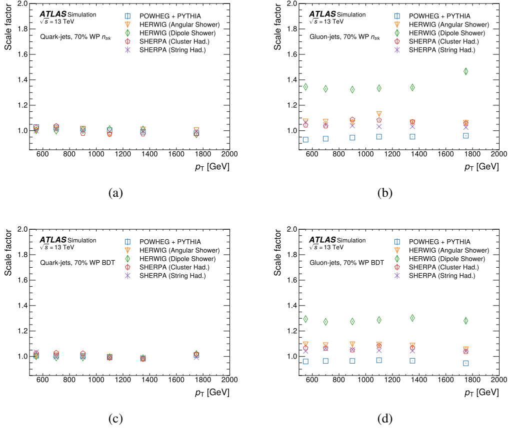
Figure 5.45 The MC-to-MC SF of the N_{\text{trk}} , (a) and (b), and BDT, (c) and (d), as a function of jet p_T for quark-jets (left) and gluon-jets (right) at the 70% WP. The vertical error bars show the statistical uncertainty.
