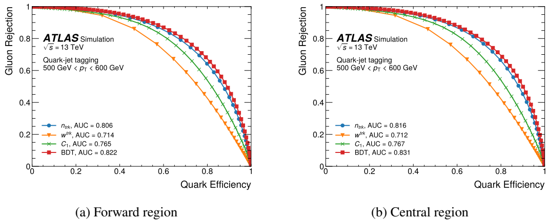
Figure 5.21 The ROC Curve for different taggers in the given jet p_T .
