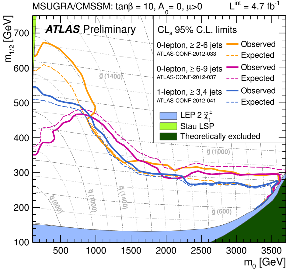
Figure 2.10: Limits in the MSUGRA/CMSSM grid [22, 15] as obtained in 5 \text{ fb}^{-1} of pp collisions at 7 TeV taken by the ATLAS experiment. The yellow solid (dashed) curve gives the observed (expected) limit for an analysis requiring between at least two and six jets [89]. The magenta curves present the observed (solid) and expected (dashed) limits for an analysis requiring between at least six and nine jets [90]. Both of these analyses veto events with electrons or muons. The third analysis [15] requires an isolated electron or muon and at least three or four jets. The observed limit (solid) and expected limit (dashed) for this analysis is shown in blue. The author has calculated the limit for the analysis requiring an isolated electron or muon and at least three or four jets.
