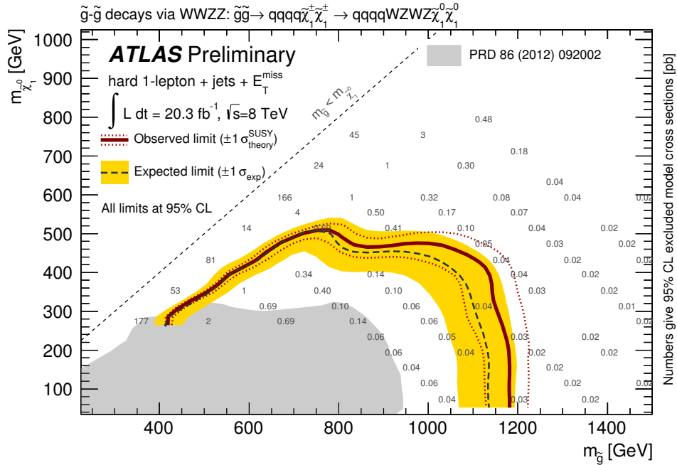
Figure 16.7: Interpretation in a simplified model with two steps and gluino pair production and the decay involving W and Z bosons. The limits are similar as in the simplified models with one step. The author contributed this plot to [179].
