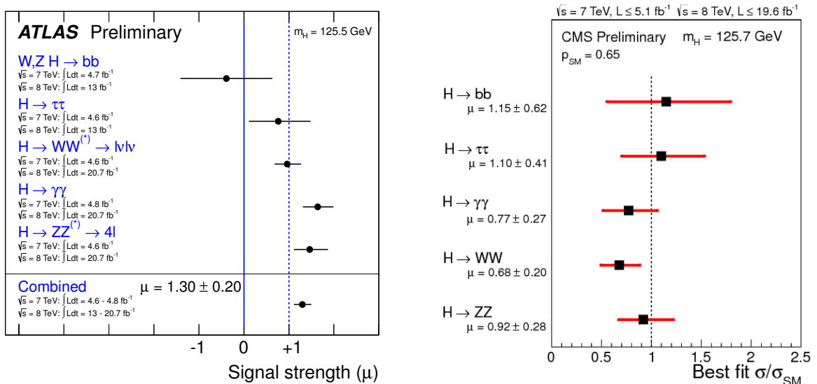
Figure 2.1: The couplings of the scalar boson recently found to other particles have been measured by the ATLAS (left, [38]) and the CMS (right, [39]) Collaborations. Within the uncertainties, the coupling strengths are as requested by a Standard Model Higgs boson.
