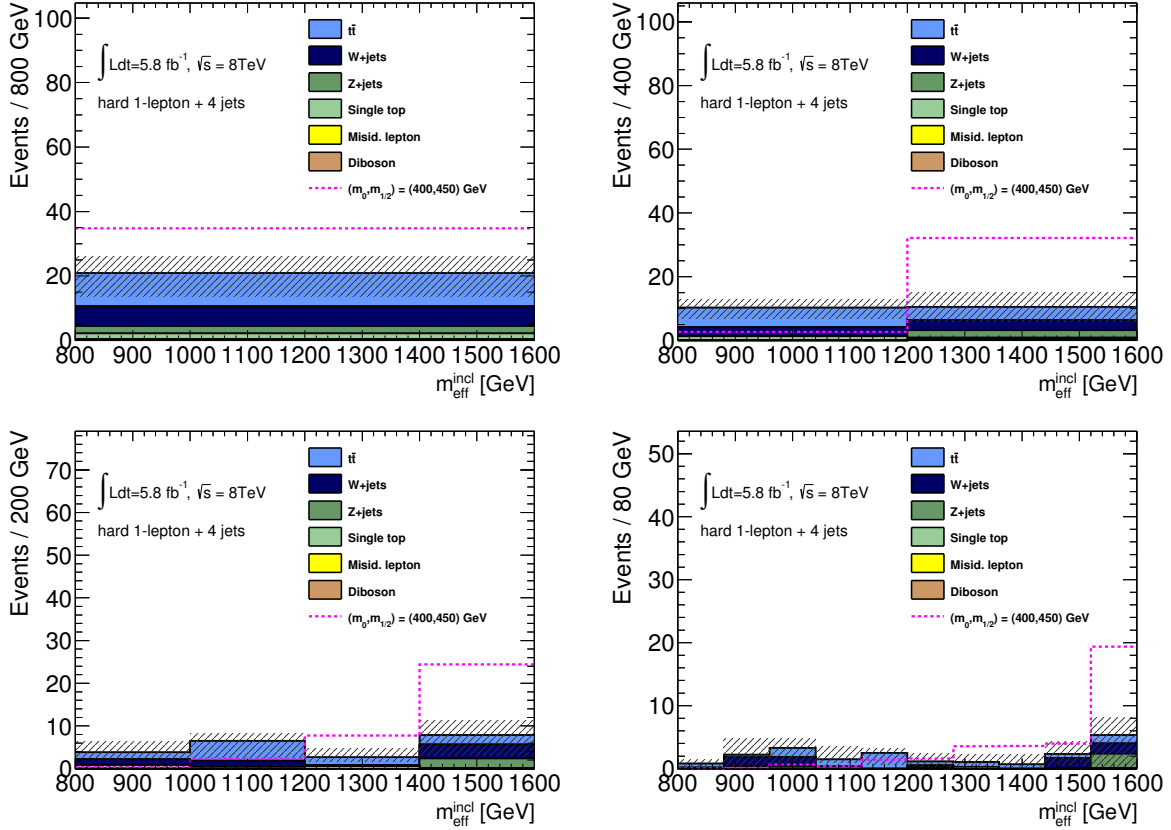
Figure 10.1: The m_{\text{eff}}^{\text{incl}} distribution is shown in a signal region in which the electron and muon channels were combined. The signal region is not sub-divided into subregions in the top left plot. This corresponds to the “cut-and-count” approach. When dividing the signal region into two subregions with m_{\text{eff}}^{\text{incl}} \in [800, 1200) GeV and m_{\text{eff}}^{\text{incl}} \in [1200, \infty) GeV, the MSUGRA/CMSSM signal model with coordinates (m_0, m_{1/2}) = (400, 450) GeV peaks in the bin with larger m_{\text{eff}}^{\text{incl}} values. The shapes of background and signal distributions are thus very distinctive (top right). This feature is more pronounced when dividing the signal region into four subregions as shown in the bottom left plot or ten subregions as shown in the plot bottom right. The relative statistical uncertainties on the background estimate however increase if choosing a finer binning. Any event having a m_{\text{eff}}^{\text{incl}} value larger than the range plotted will be added to the last bin displayed.
