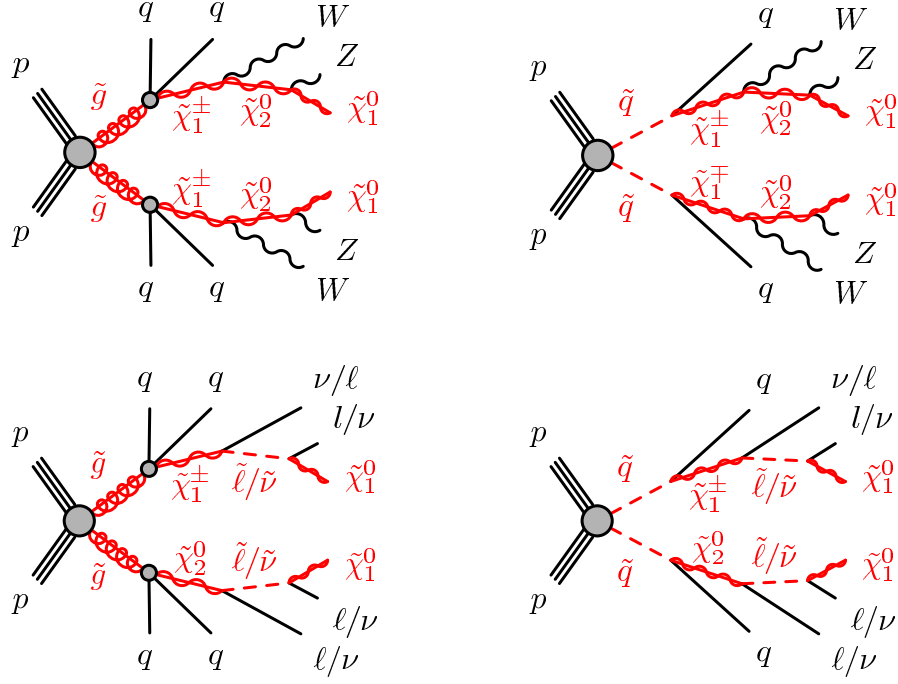
Figure 2.9: Diagrams for simplified models with two steps. The top row shows the diagrams for the simplified models with the decay involving W and Z bosons. The bottom row shows the diagrams with the decay via sleptons and sneutrinos. The diagrams with initial gluino pair production are shown left and the ones with initial squark pair production right.
