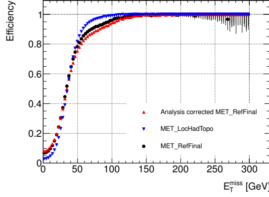
(a) Electron+ E_T^{\text{miss}} trigger based on calorimeter cells
