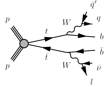
Figure 5.1: Diagram for an example t\bar{t} decay.
