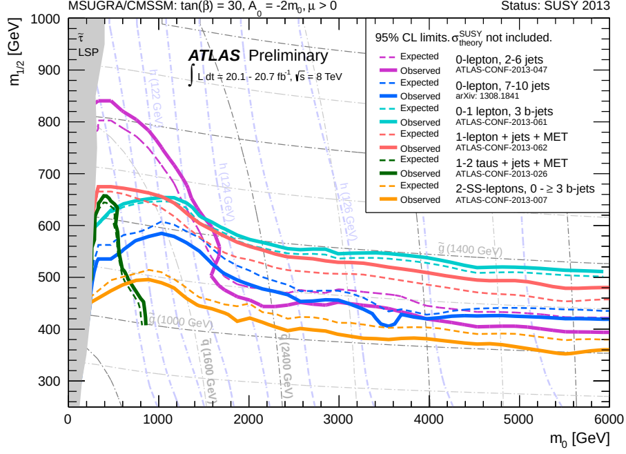
Figure 16.12: Observed and expected limits of various ATLAS analyses in the ‘Higgs aware’ MSUGRA/CMSSM grid [233]. The analysis developed in this work is shown by the red curves.
