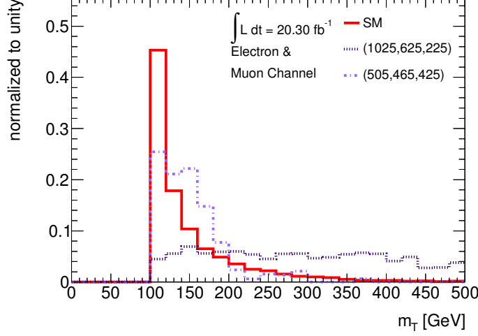
Figure 12.3: The normalised m_T distributions are shown for the total Standard Model background (in solid red) and for two signal models from the simplified models with one step and initial gluino pair production with the parameters (m_{\tilde{g}}, m_{\tilde{\chi}_1^\pm}, m_{\tilde{\chi}_1^0}) = (505, 465, 425) GeV (in dashed-dotted light blue) and (1025, 625, 225) GeV (in dotted dark blue). Preselection cuts as defined in Section 7.2.1 were applied as well as cuts on E_T^{\text{miss}} > 100 GeV, p_T^{\text{1st jet}} > 80 GeV and m_T > 100 GeV. Electron and muon channel were combined. The m_T distribution of the signal point (1025, 625, 225) GeV is flat and shows a long tail, which provides discriminating power against the Standard Model background. The other signal point with parameters (505, 465, 425) GeV shows a less dominant tail, but still peaks at larger values than the background. This analysis is more sensitive to models with a medium or large mass distance between the gluino and the \tilde{\chi}_1^0 like point (1025, 625, 225) GeV and less to models with a small mass difference like point (505, 465, 425) GeV.
