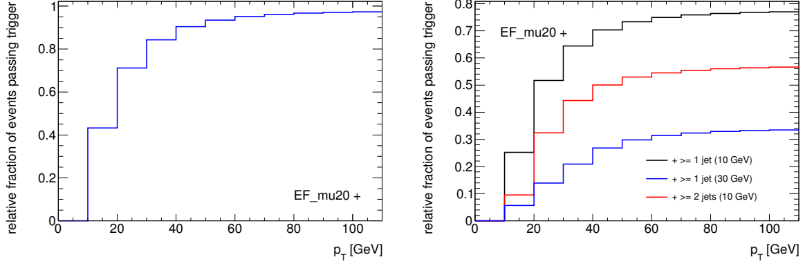
Figure 9.2: Rate reduction with respect to the single muon trigger requiring a muon with p_T(\mu) > 20 GeV when adding a geometrical isolation criterion. The left plot shows the reduction when requiring the muon to be geometrically isolated from any jet with a distance \Delta R(\mu, \text{jet}) > 0.4 . Only jets with p_T > x (as given on the x-axis) are considered in the calculation of \Delta R(\mu, \text{jet}) . Muons are required to be separated from jets by \Delta R(\mu, \text{jet}) > 0.2 in the right plot. In this plot, a further rate reduction with respect to the single muon trigger is obtained by additionally requiring the event to contain at least one jet with p_T > 10 GeV (electromagnetic scale, black curve), at least one jet with p_T > 30 GeV (electromagnetic scale, blue curve) or at least two jets with p_T > 10 GeV (electromagnetic scale, red curve).
