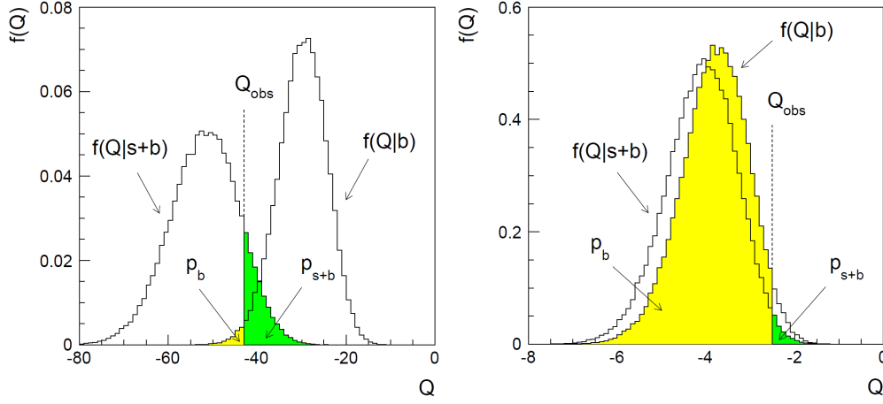
Figure 10.8: The distribution of the probability density functions for the background model ( f(Q|b) ) and signal+background model ( f(Q|s+b) ) are shown in cases where the two models can clearly be distinguished (left) or are very close together due to a very small signal contribution (right). The test statistics is denoted by Q in these plots. The plots are taken from [214].
