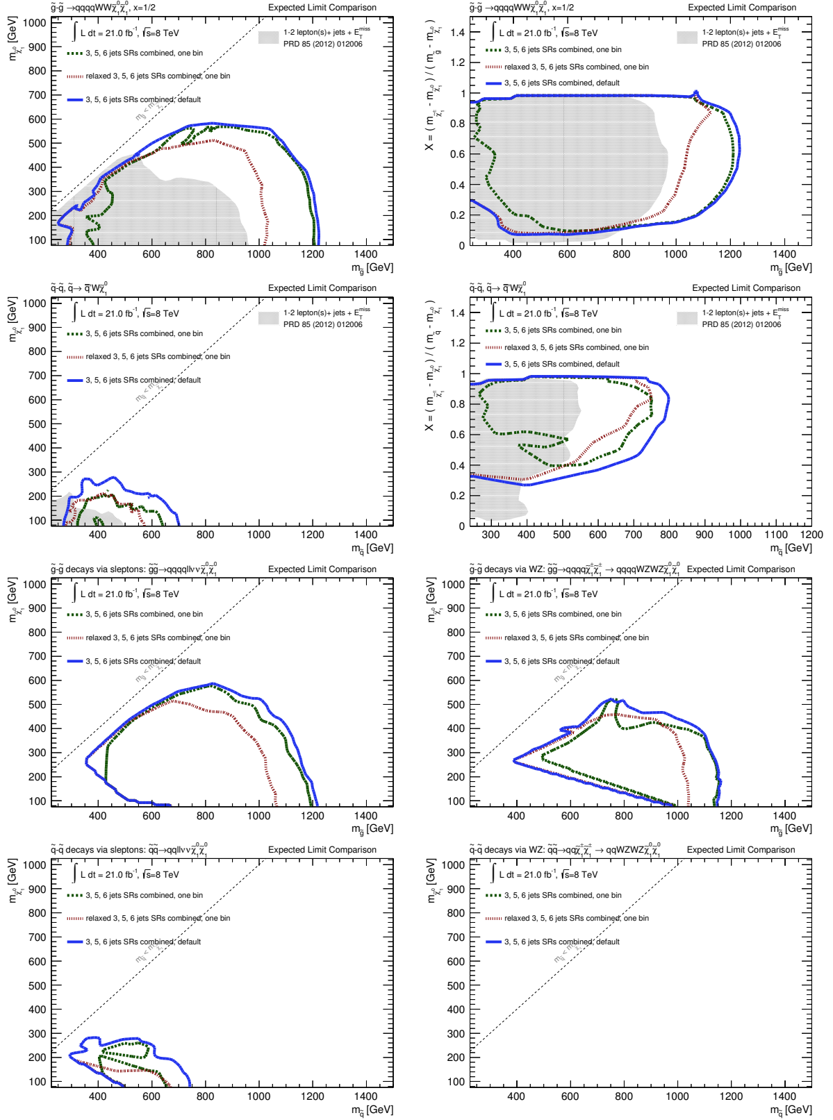
Figure 12.5: The 3-jets, 5-jets and 6-jets signal regions in the default configuration (in blue) are compared to a fit configuration with only one bin. In red dotted, the sensitivity of a version of signal regions with one bin and loose cuts in m_{\text{eff}}^{\text{incl}} for the 3-jets and 5-jets signal regions and in E_{\text{T}}^{\text{miss}} for the 6-jet signal regions is shown. In green dashed the sensitivity of signal regions with tight cuts in m_{\text{eff}}^{\text{incl}} and E_{\text{T}}^{\text{miss}} is given. The sensitivities in simplified models with one step are given in the top two rows, in simplified models with two steps in the bottom two rows. Again no sensitivity to the simplified model with two steps, initial squark pair production and the decay involving W and Z bosons is obtained.
