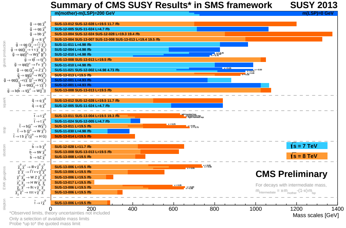
Figure F.2: Limits on Supersymmetry by the CMS Collaboration [237].
