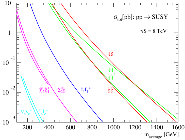
Figure 2.4: Cross sections for a center-of-mass energy of 8 TeV in pp collisions for the production of different supersymmetric particles [73]. While the cross sections for the production of squarks and gluinos are always the highest in comparison to other sparticles with the same mass, the cross sections of heavy gluinos and squarks can be significantly lower than the cross sections of lighter supersymmetric particles. The cross sections were calculated by the tool Prospino 2 [72, 73].
