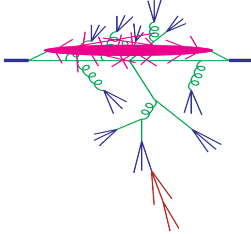
Figure 3.9: A collision event can be divided in different components due to the factorisation theorem depending on the momentum transferred (as described in the text). The middle green line indicates the hard scattering process, the outgoing green gluon and quark lines the parton shower. The hadronisation is indicated by the blue lines and the further decay of unstable hadrons by the red lines. The hard scattering is accompanied by the underlying event indicated in magenta colour. The plot is taken from [137].
