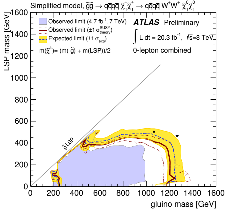
Figure 16.10: Limits by an analysis focusing on final states with two to six jets, no leptons and E_T^{\text{miss}} in the simplified model with one step, gluino pair production and fixed x = 1/2 [232].
