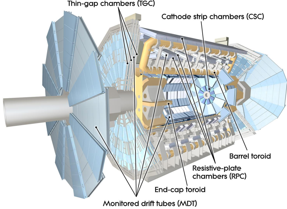
Figure 3.5: The ATLAS muon system, including the four different types of muon chambers. The magnet system surrounding the muon detectors is shown in yellow [106].
