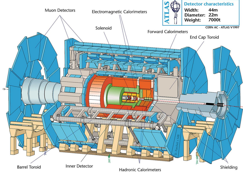
Figure 3.2: A sketch of the ATLAS detector [106].
