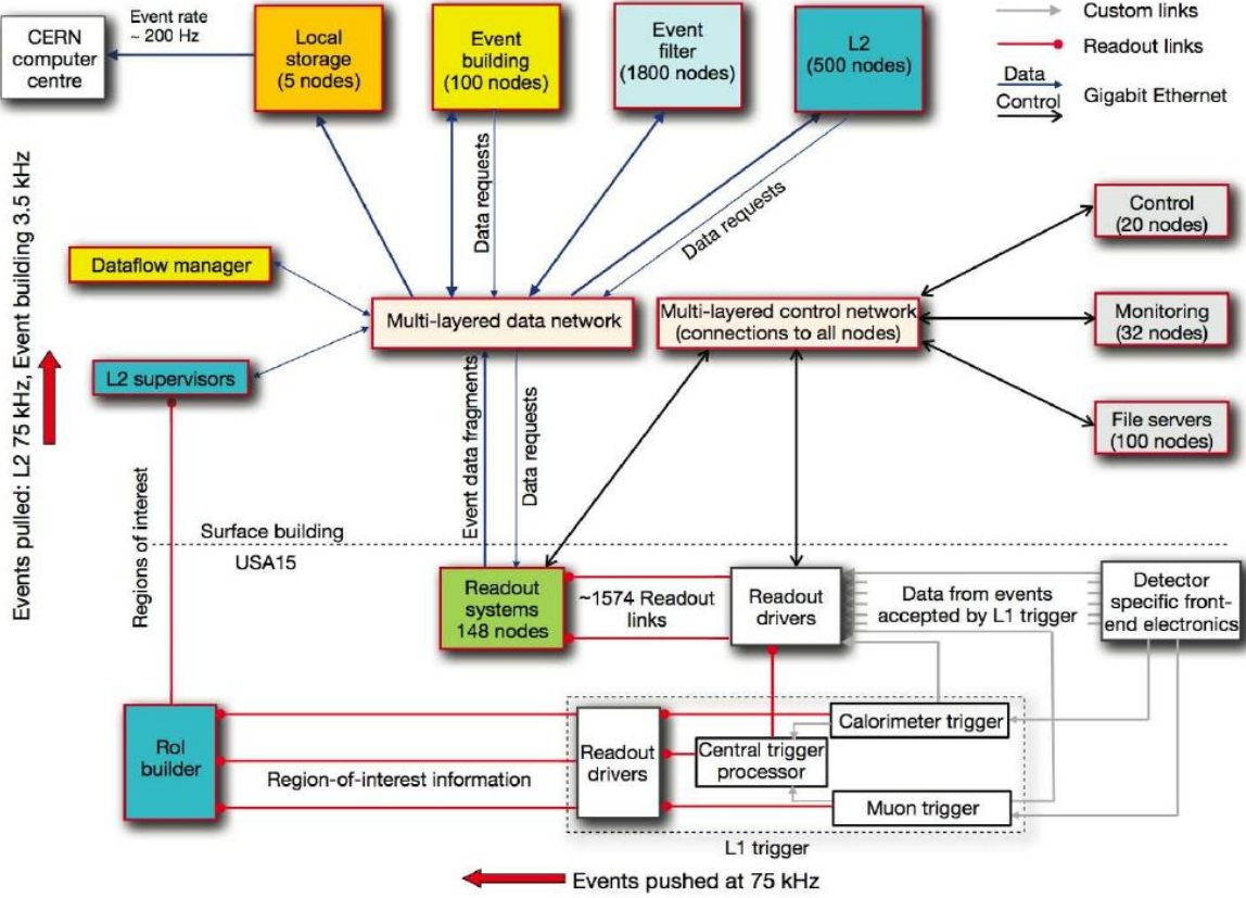
Figure 3.6: A sketch of the Trigger and Data Acquisition System (TDAQ) [106].
