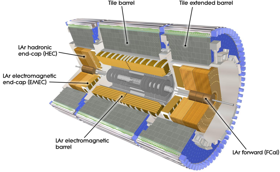
Figure 3.4: The ATLAS calorimeters in the barrel are shown schematically with the electromagnetic calorimeter closer to the beam line and enclosed by the hadronic calorimeter [106].
