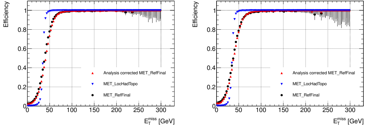
Figure 9.8: Efficiency of the electron+ E_T^{\text{miss}} trigger based on topological clusters with local cluster weighting with respect to different definitions of E_T^{\text{miss}} in events containing at least one jet (left plot) or at least two jets (right plot).
