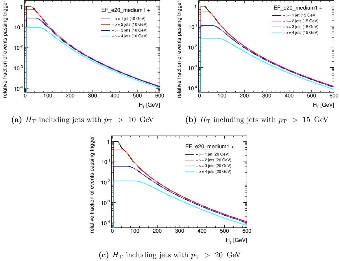
Figure 9.4: The rate of the single electron trigger with the criterion E_T(e) > 20 GeV can be further reduced when requiring the presence of H_T > x GeV (the value on the x-axis at the electromagnetic scale) in the event. Here, H_T is constructed including all jets with p_T > 10 GeV in the event (a), or including all jets with p_T > 15 GeV (b) or with p_T > 20 GeV (c). The rate can be further reduced by also requiring the presence of at least one (black curve), two (red curve), three (blue curve) or four jets(s) (cyan curve) (with p_T > 10, 15, 20 GeV depending on the jets included in the H_T calculation).
