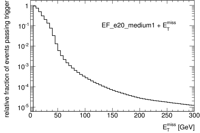
Figure 9.5: The rate reduction with respect to the single electron trigger with the criterion E_T(e) > 20 GeV when also requiring a cut on E_T^{\text{miss}} > x GeV (given by the value on the x-axis).
