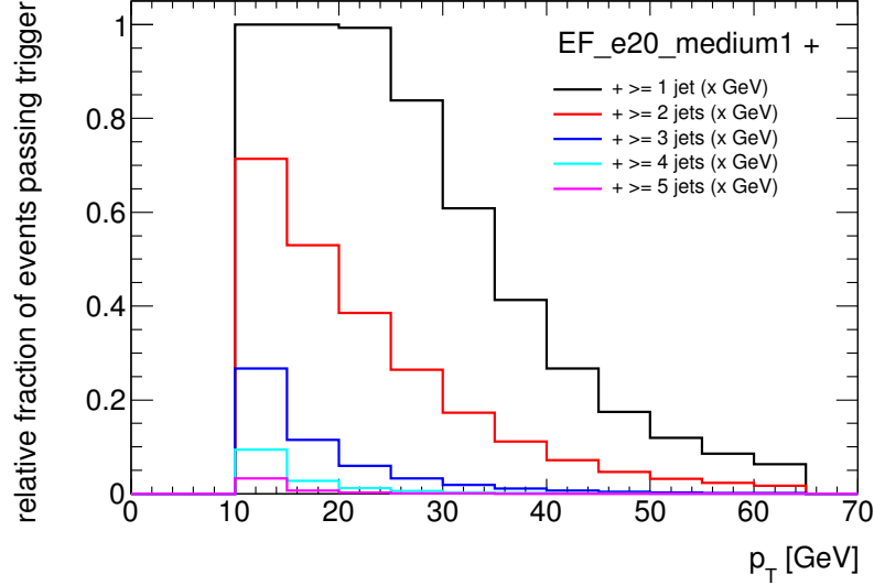
Figure 9.3: A rate reduction with respect to the single electron trigger with the criterion E_T(e) > 20 GeV can be achieved if requiring additional jets: The black curve indicates the possible rate reduction when requiring one additional jet in the event with p_T > x , where x is indicated on the x-axis. The rate can be further suppressed when requiring the event to contain at least two jets (red curve), three jets (blue curve), four jets (cyan curve) or five jets (magenta curve) with p_T > x as indicated on the x-axis. The jet p_T values are given at electromagnetic scale.
