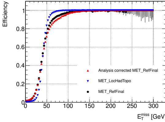
(b) Electron+ E_T^{\text{miss}} trigger based on topological clusters with electromagnetic calibration
