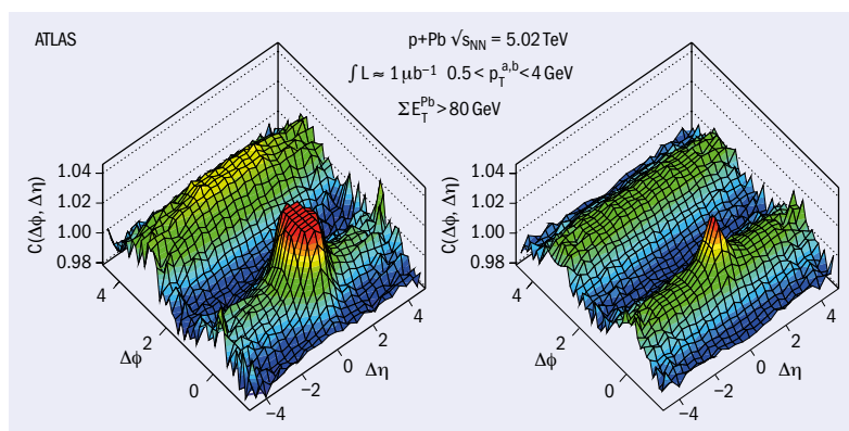
The correlation function C(\Delta\phi, \Delta\eta) for two charged particles in proton–lead collisions having \Sigma E_T > 80 GeV before (left) and after (right) background subtraction.
