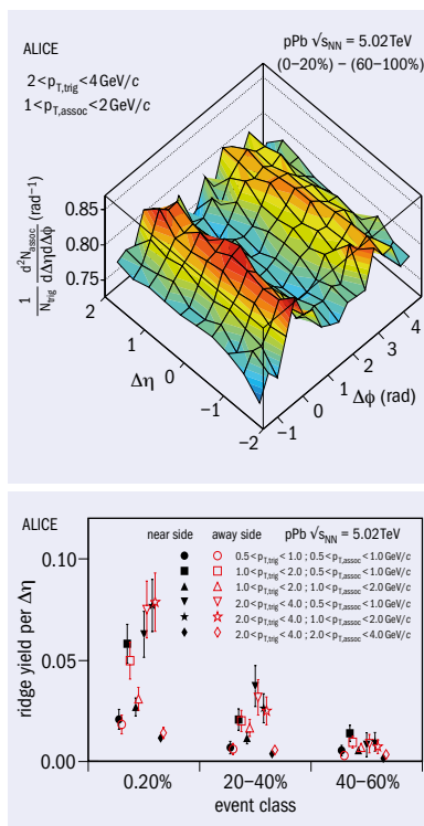
Fig. 1. Associated yield per trigger particle in \Delta\phi and \Delta\eta for pairs of charged particles with 2 < p_{T, \text{trig}} < 4 GeV/c and 1 < p_{T, \text{assoc}} < 2 GeV/c in proton–lead collisions in ALICE at \sqrt{s_{NN}} = 5.02 TeV for the 0–20% multiplicity class, after subtraction of the associated yield obtained in the 60–100% event class.
