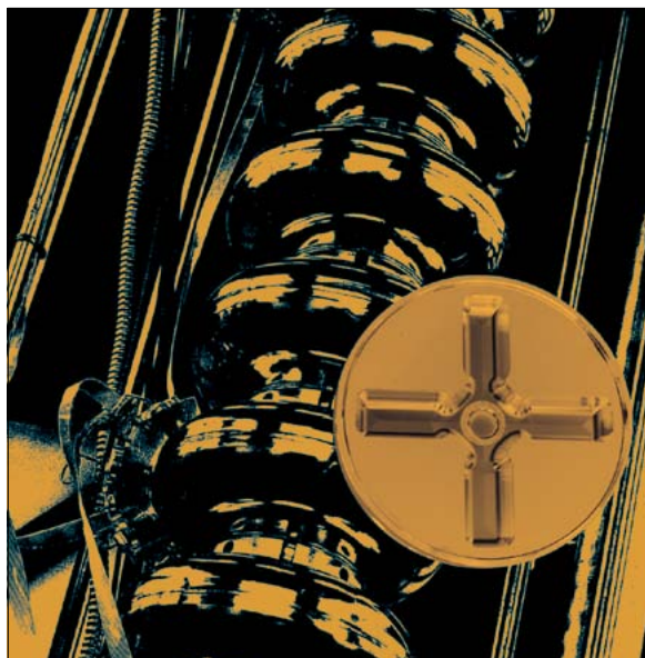
A superconducting RF accelerator structure made from the purest niobium, together with a disc of a CLIC accelerating structure prototype. (Image credit: DESY.)
