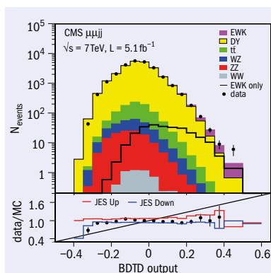
Fig. 2a. Left: Boosted decision tree output-distribution for selected Z+2jets events in the dimuon channel.
