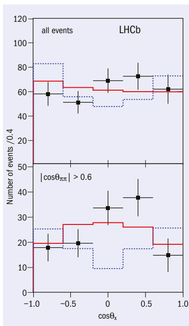
Fig. 2. Distribution of the cosine of the decay angle of the X(3872) for all candidates and for a subset with a selection on the cosine of the decay angle of the \pi^+\pi^- system. The selected shows a clearer separation between the hypotheses, coloured as in figure 1.
