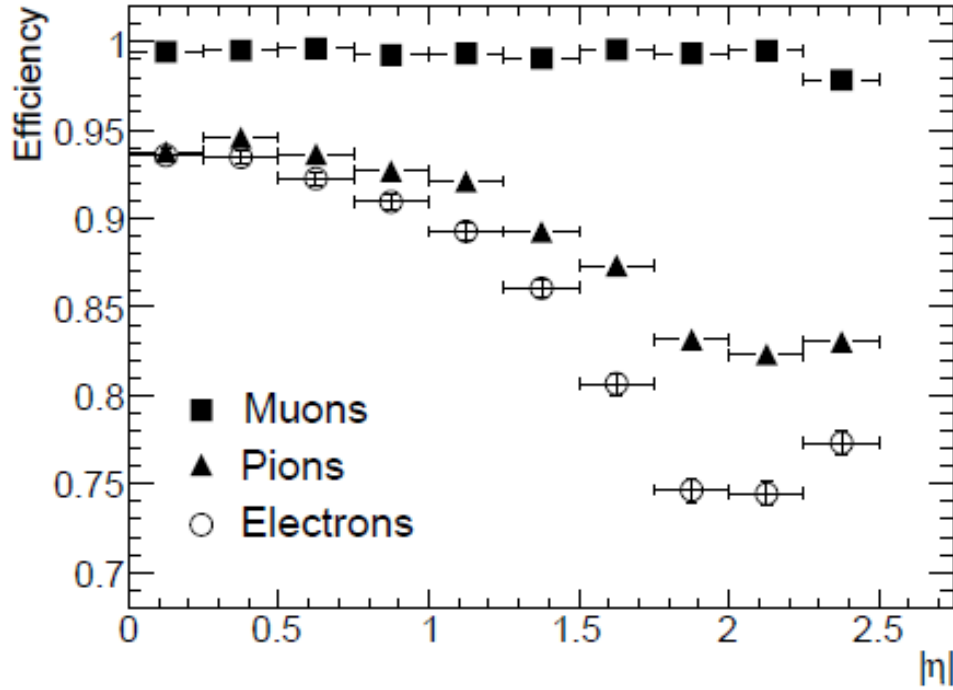
Figure 4.2: Tracking Reconstruction efficiency as a function of \eta for muons, pions, and electrons with p_T = 5 GeV.
