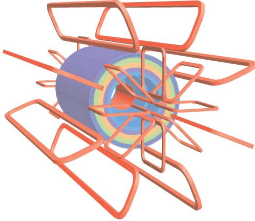
Figure 3.8: The ATLAS toroid and solenoid magnets [64].
