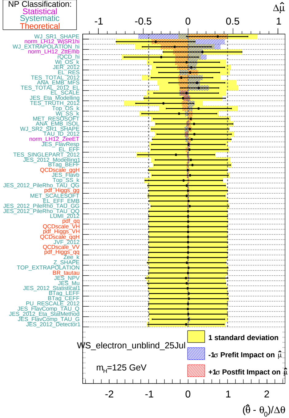
Figure B.2: Top ranked nuisance parameters in the electron measurement.
