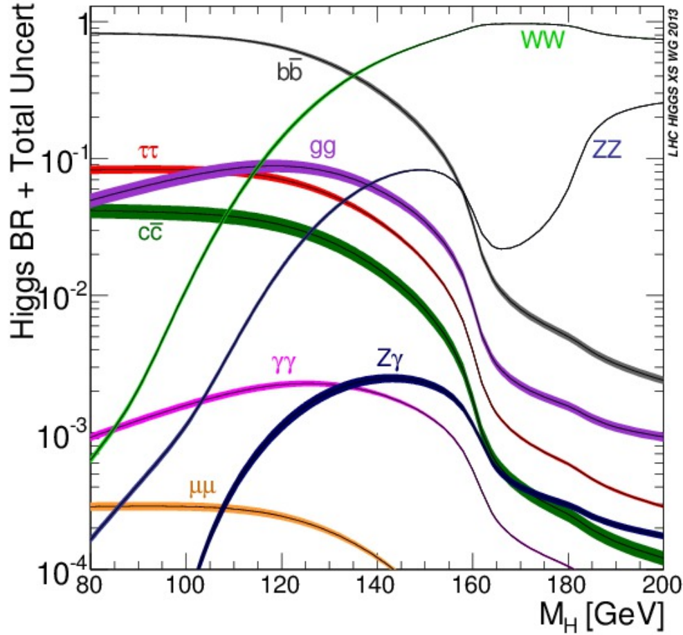
Figure 2.5: Branching ratios of the Higgs boson as a function of its mass [24].
