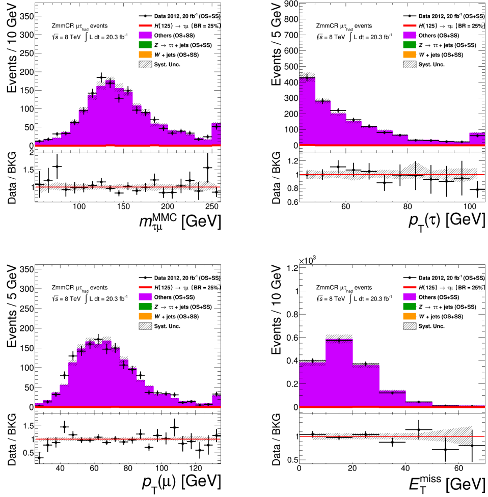
Figure 8.12: m_{\mu\tau}^{MMC} , p_T(\tau) , p_T(\mu) , and E_T^{\text{miss}} distributions in ZmmCR for the muon measurement.
