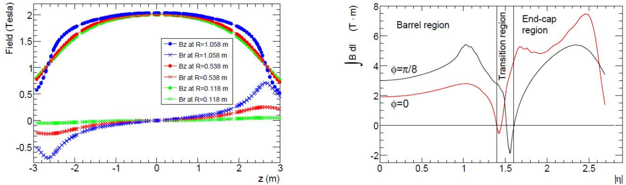
Figure 3.9: Magnetic field strength in the Inner Detector for fixed \phi (left) and in the Monitored Drift Tubes in the Muon System (right) [64].
