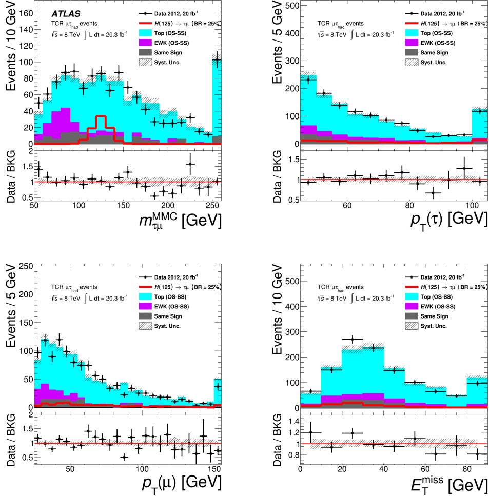
Figure 8.10: m_{\mu\tau}^{\text{MMC}} , p_T(\tau) , p_T(\mu) , and E_T^{\text{miss}} distributions in TCR for the muon measurement.
