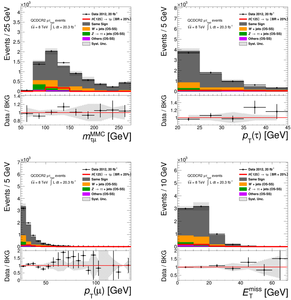
Figure 8.16: m_{\mu\tau}^{MMC} , p_T(\tau) , p_T(\mu) , and E_T^{miss} distributions in QCDCR2 for the muon measurement.
