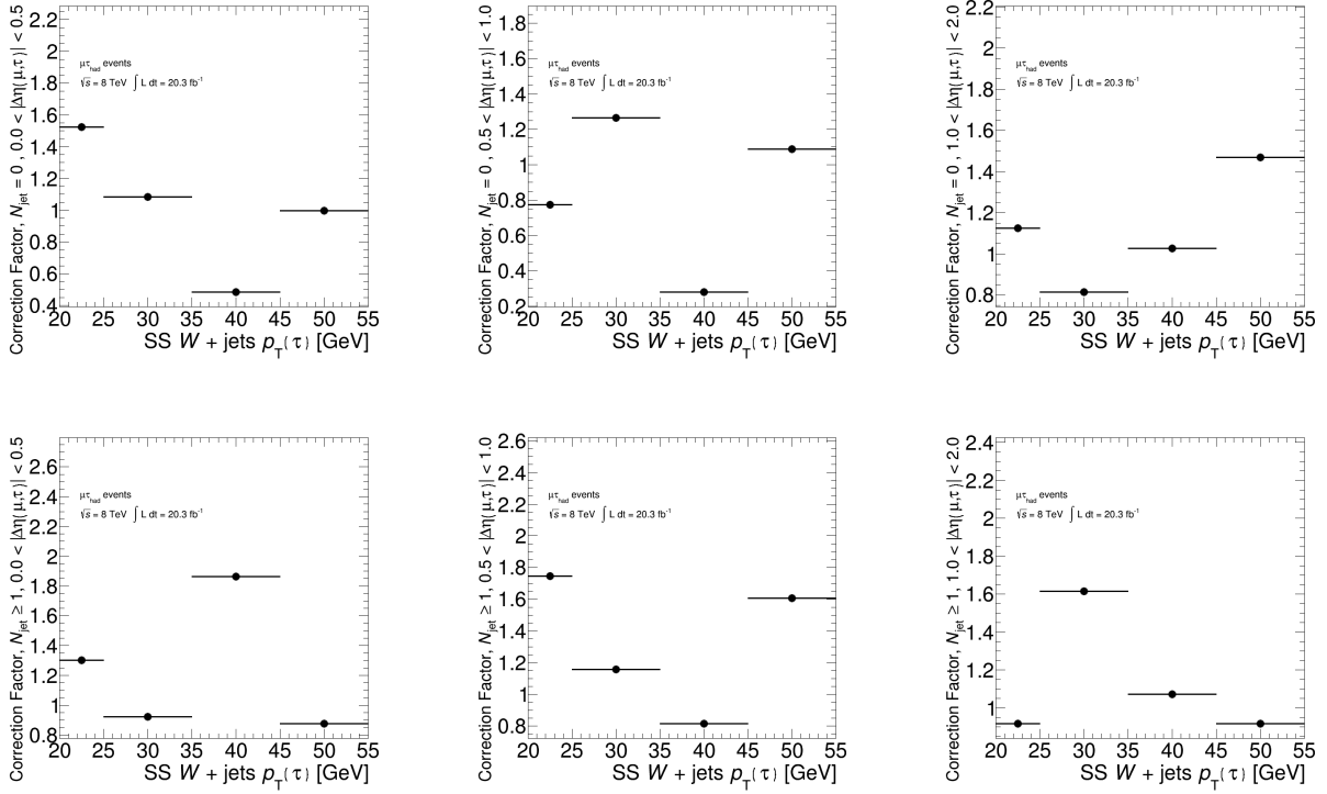
Figure A.4: Shape corrections applied to the W + \text{jets} background for SS events in WCR, TCR, and ZmmCR in the muon measurement.
