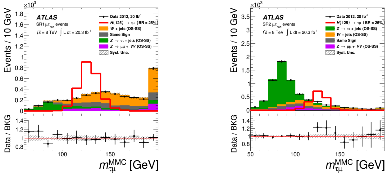
Figure 11.1: Post-fit m_{\mu\tau}^{\text{MMC}} distributions in SR1 and SR2 in the muon measurement. The red histogram indicates the predicted H \rightarrow \mu\tau distribution, assuming \text{Br}(H \rightarrow \mu\tau) = 25\% [115].
