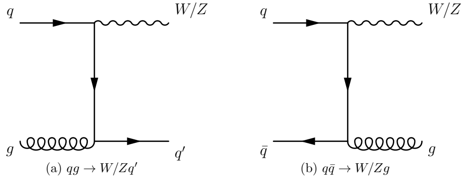
Figure 6.3: Examples of leading order diagrams for W/Z + \text{jets} production.
