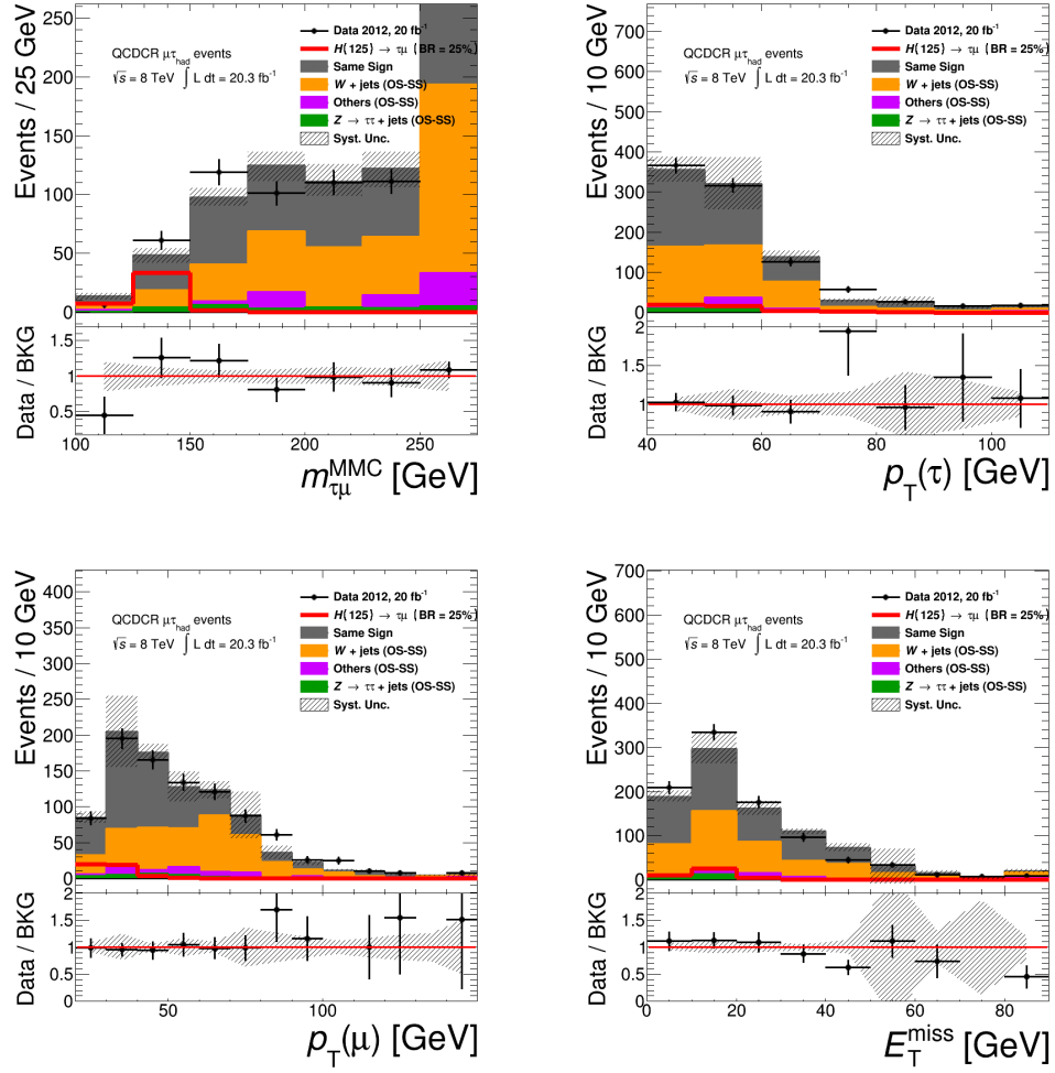
Figure 8.14: m_{\mu\tau}^{\text{MMC}} , p_T(\tau) , p_T(\mu) , and E_T^{\text{miss}} distributions in QCDCR for the muon measurement.
