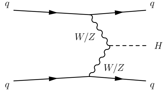
(b) Vector Boson Fusion
