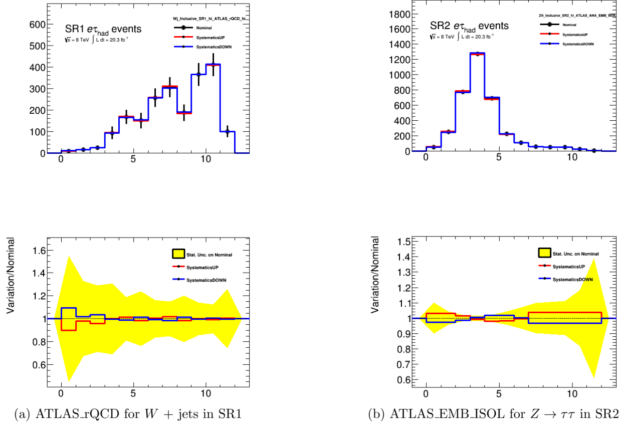
Figure 10.4: Examples of systematic variations used in the fit model, both taken from the electron measurement.
