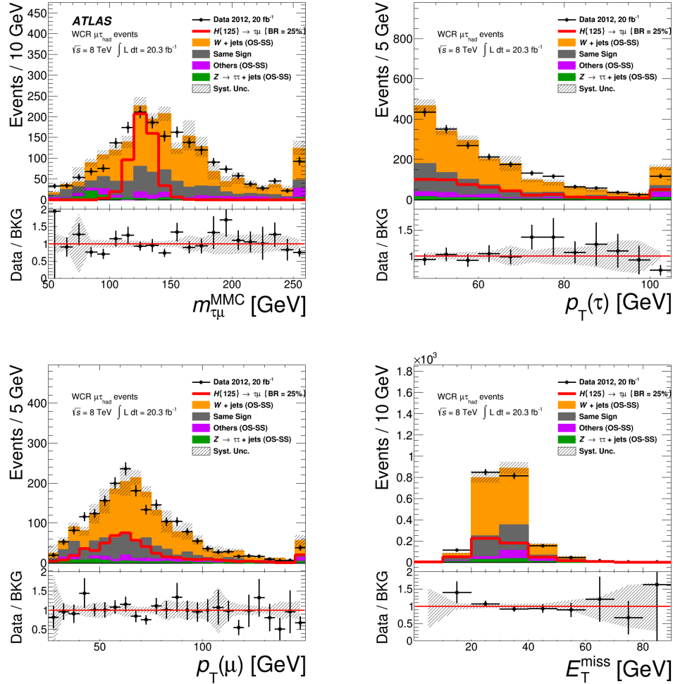
Figure 8.8: m_{\mu\tau}^{MMC} , p_T(\tau) , p_T(\mu) , and E_T^{miss} distributions in WCR for the muon measurement.
