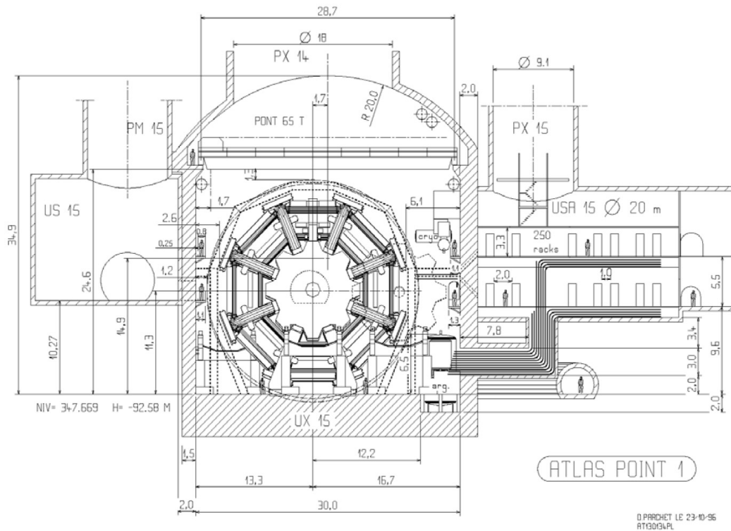
Figure B.2: Cross section of the ATLAS caverns, most important the experimental cavern UX15 and the service area USA15[92]. To get back to the Off-Detector Electronics Chapter click here .
