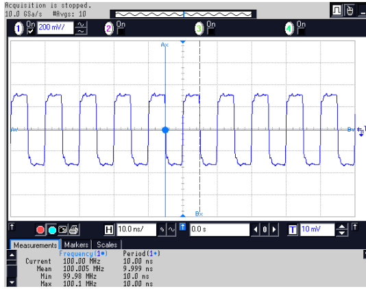
Figure 6.12: Measurement of the 100 MHz clock signal generated by a dual-frequency oscillator (Si532) on the Re-BOC (Measurement by M. Wensing).
