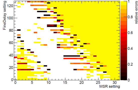
Figure 6.5: Relative error rate for the different combinations of MSR and fine delay setting[52].
