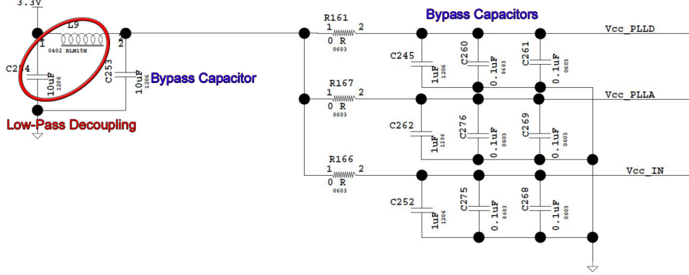
Figure 4.9: Power supply filtering circuit for the PLL handling the TTC Clock on the Re-BOC with low-pass decoupling and bypass capacitors for a wide frequency range (the 0 \Omega resistors were placed in case additional decoupling would be needed for the individual voltages of the PLL, then they would be replaced by ferrite beads).
