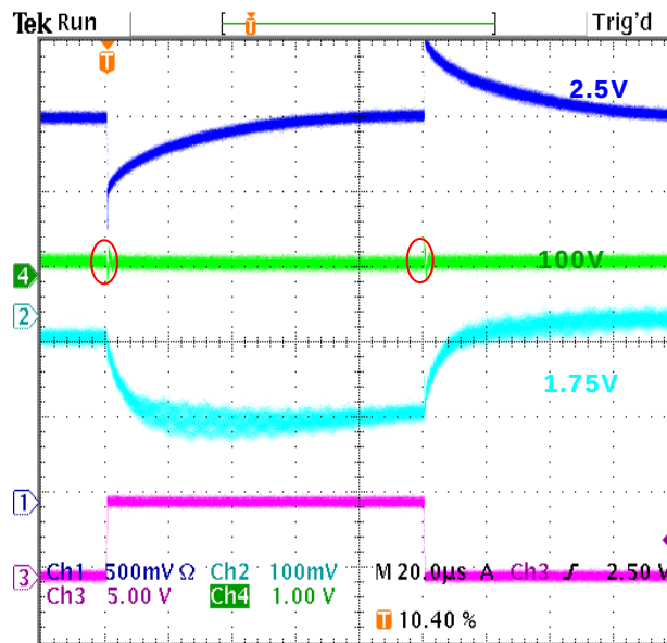
Figure 5-15. Two low voltages and one high voltage from one channel connected simultaneously using the CMS cable. The perturbation is applied to only one of the low voltage circuits. It affects the other low voltage circuit also. Small glitches are also observed in the high voltage circuit.
