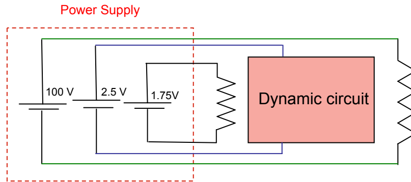
Figure 5-14. Diagram of the circuit used to test the 3 high voltage and low voltage channels at the same time.
