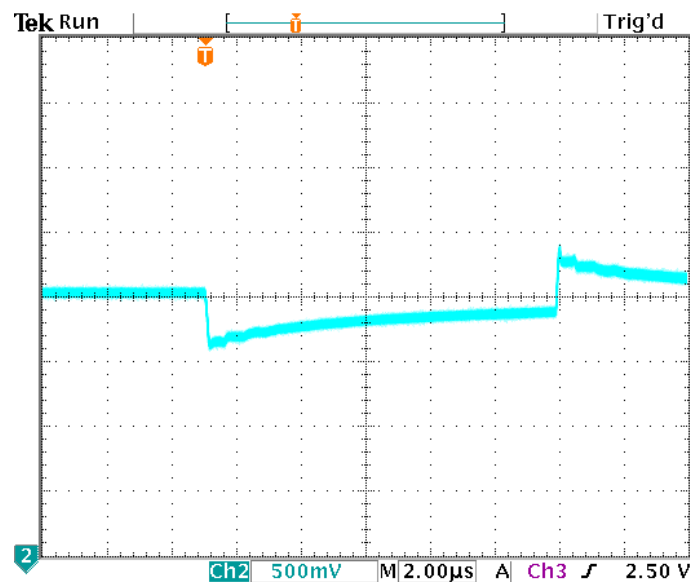
Figure 5-8 Fast and slow recoveries for a circuit without capacitor, nominal voltage of 1.8V and 11\mu\text{s} pulse width.
