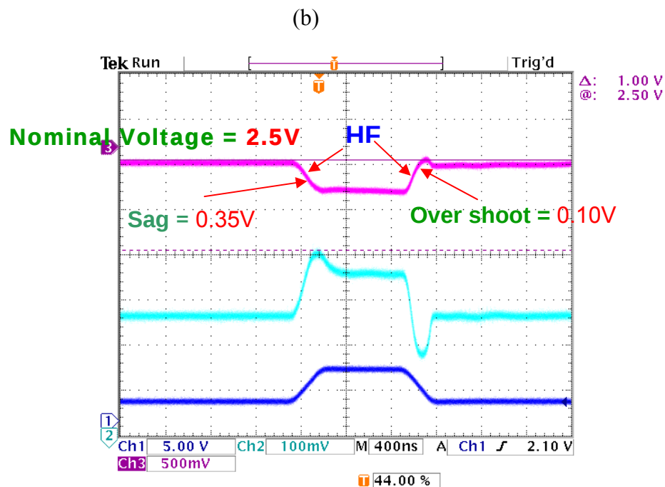
Figure 5-11. a) Signal without capacitor b) signal with capacitor of 13µF. The pulse width in the wave generator is 1µs.
