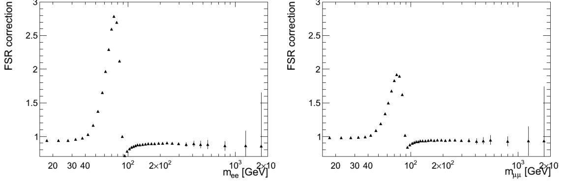
Figure 4.5. The effect of QED final state radiation on the cross section. Left: dielectron, right: dimuon channel.
