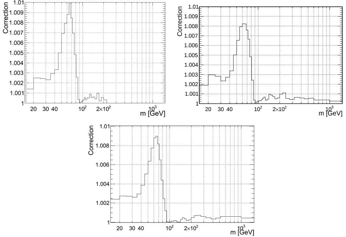
Figure 6.28. FSR correction for the type A events as a function of dilepton invariant mass for dimuon channel at 7 TeV (top left), for dimuon channel at 8 TeV (top right) and for dielectron channel at 8 TeV (bottom) simulation.
