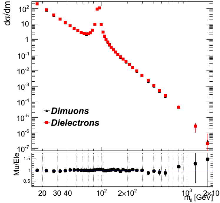
Figure 6.39. Drell–Yan pre-FSR full acceptance cross section measurement with the photon induced contribution subtracted, in the dimuon and dielectron channels at 8 TeV center-of-mass energy.
