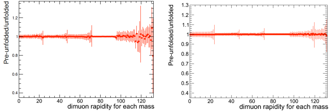
Figure 6.21. Ratio of observed yields before and after detector resolution unfolding as a function of dimuon invariant mass-absolute rapidity. Left plot: 7 TeV, right plot: 8 TeV.
