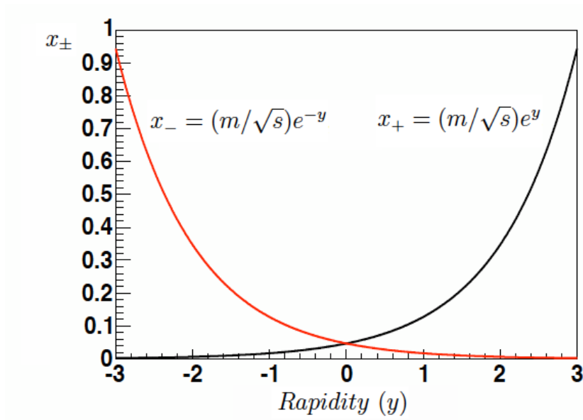
Figure 6.1. The relationship of the Bjorken scaling variables of the initial-state partons ( x_{\pm} ) and the dilepton rapidity y .
