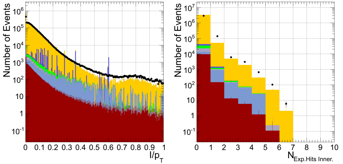
Figure 6.12. Distributions for the variables used to discriminate between signal and various backgrounds in the dielectron channel in the 8 TeV analysis (as listed in Tab. 6.4), not including the cut on the variable plotted. Peripheral pseudorapidity region ( |\eta| > 0.8 ) is plotted.
