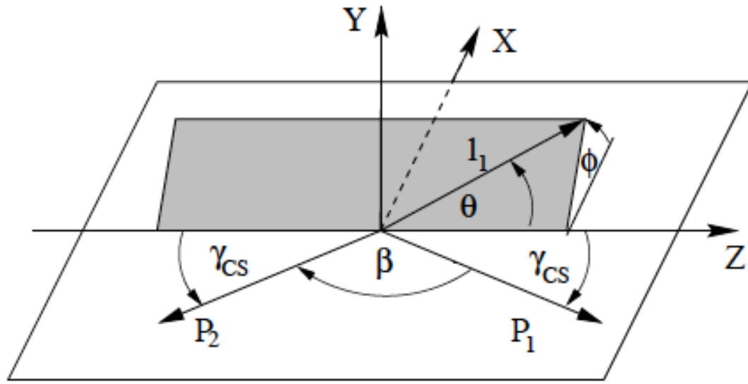
Figure A.1. The Collins-Soper frame: the z axis cuts the angle between P_1 and P_2 into halves (the half angle is called the Collins-Soper angle CS) while the x axis is perpendicular to P_1 and P_2 . The direction of one lepton momentum l_1 can then be given by the angles \phi and \theta .
