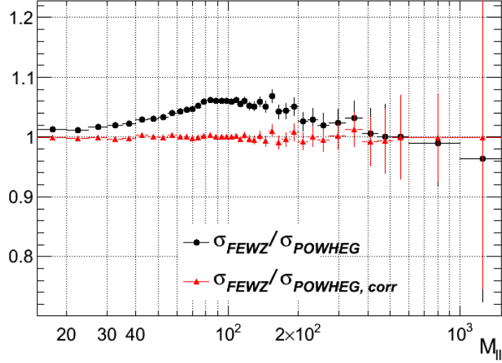
Figure D.6. The ratio of absolute cross sections calculated with POWHEG and FEWZ before and after the NNLO kinematics reweighting applied to the POWHEG MC sample.
