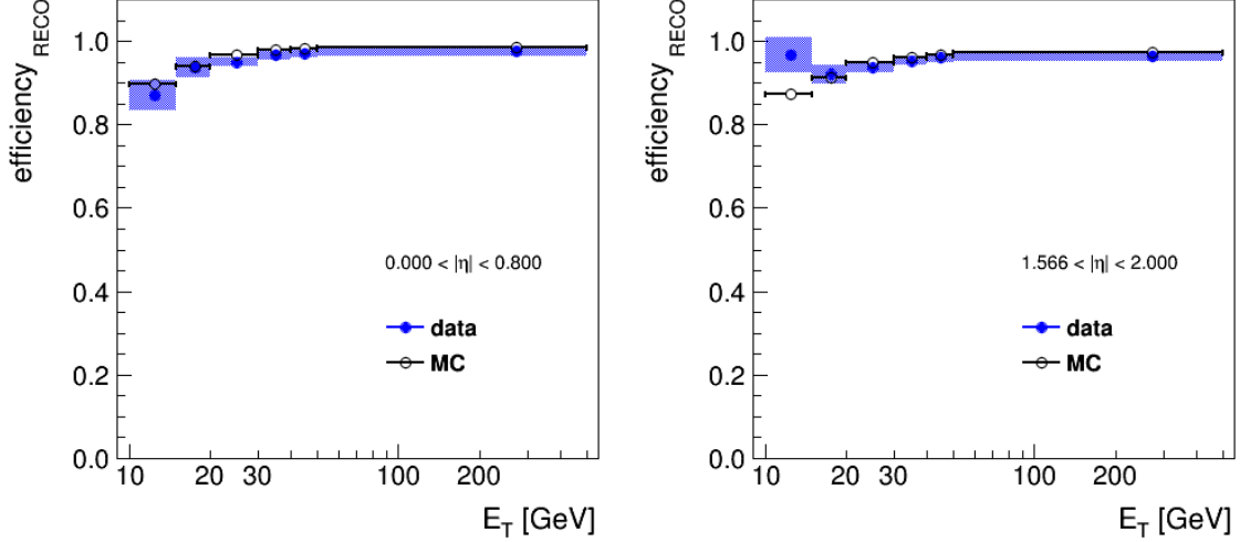
Figure F.2. Tag-and-probe electron reconstruction efficiencies.
