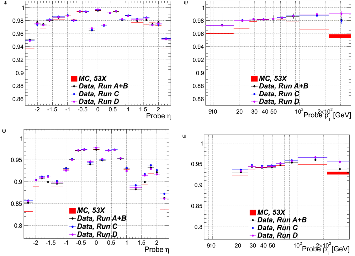
Figure F.11. Muon trigger efficiencies as a function of probe muon p_T and \eta for various data taking periods, estimated with data-driven T&P method from 8 TeV data and simulation. Top row: soft-leg efficiencies, bottom row: tight-leg efficiencies.
