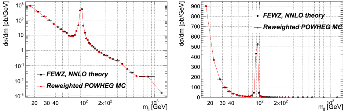
Figure D.5. The absolute cross section calculated with FEWZ compared to the signal MC truth pre-FSR cross section after reweighting, left plot: logarithmic scale on y axis, right plot: linear scale on y axis.
