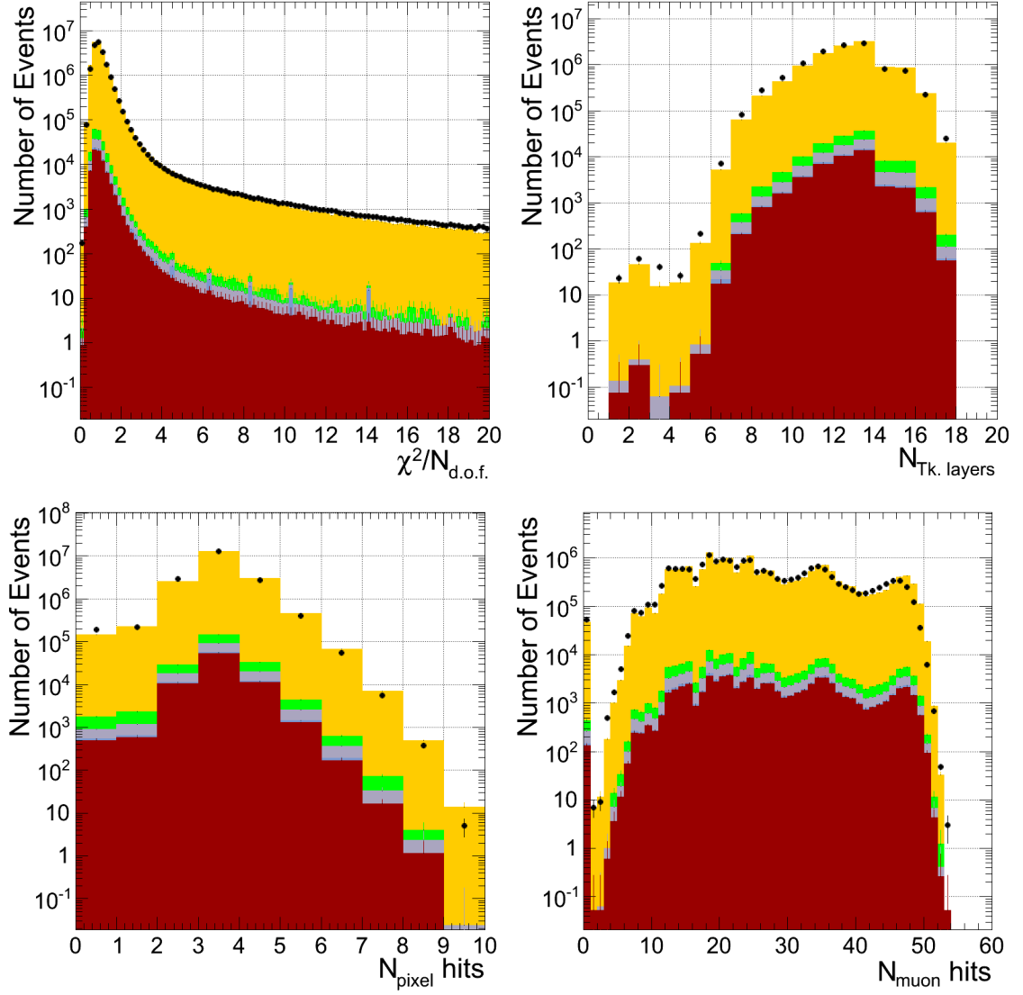
Figure 6.6. Distributions for the variables used to discriminate between signal and various backgrounds in the 8 TeV analysis (as listed in Tab. 6.3), not including the cut on the variable plotted.
