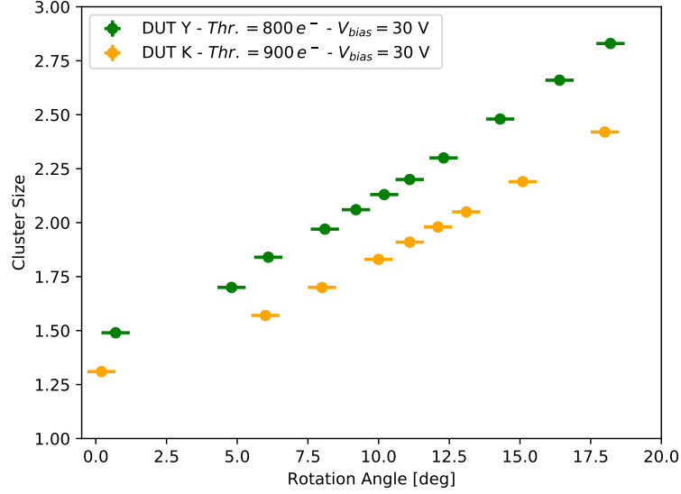
Figure 5.59: Average cluster size versus the rotation angle around the y axis (along the 25\ \mu\text{m} pitch) for DUTs K and Y, with V_{\text{bias}} = 30\ \text{V} for both DUTs.
