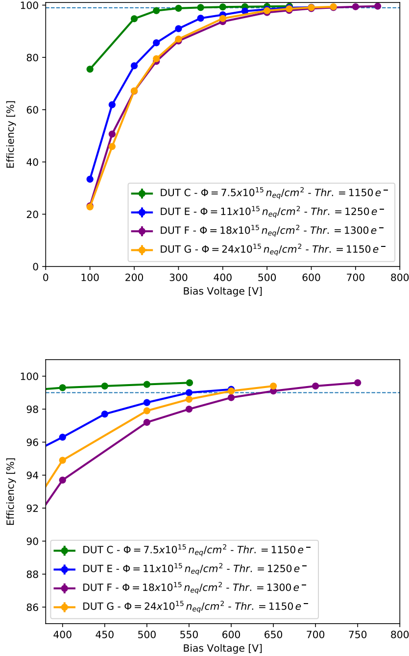
Figure 5.23: Hit detection efficiency for DUTs C, E, F and G versus the applied bias voltage with orthogonal beam incidence. The dashed line represents 99% efficiency.
