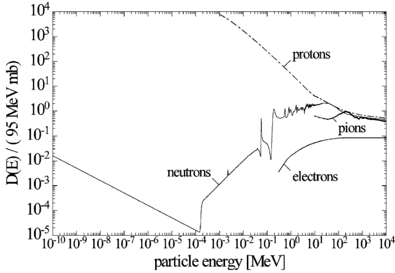
Figure 1.8: Estimation of the displacement damage cross sections for neutrons, protons, pions and electrons up to an energy of 10 GeV. [6].
