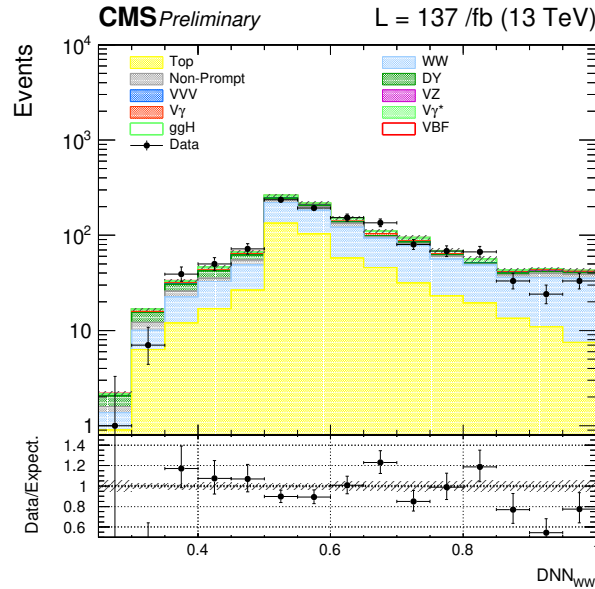
Figure 8.5: Post-fit number of events as a function of the \text{DNN}_{\text{WW}} classifier in the WW-like category of the DF VBF channel. The dashed gray band accounts for all systematic uncertainties on the signal and background yields.
