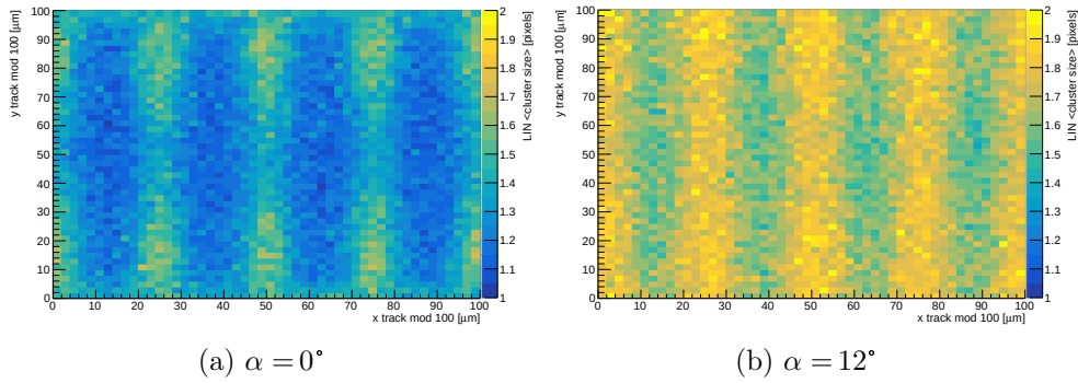
Figure 5.58: DUT K average cluster size maps for a 2 \times 2 pixel grid for different rotation angles around the y axis (along the 25 \mu\text{m} pitch), with V_{\text{bias}} = 30 \text{ V} .
