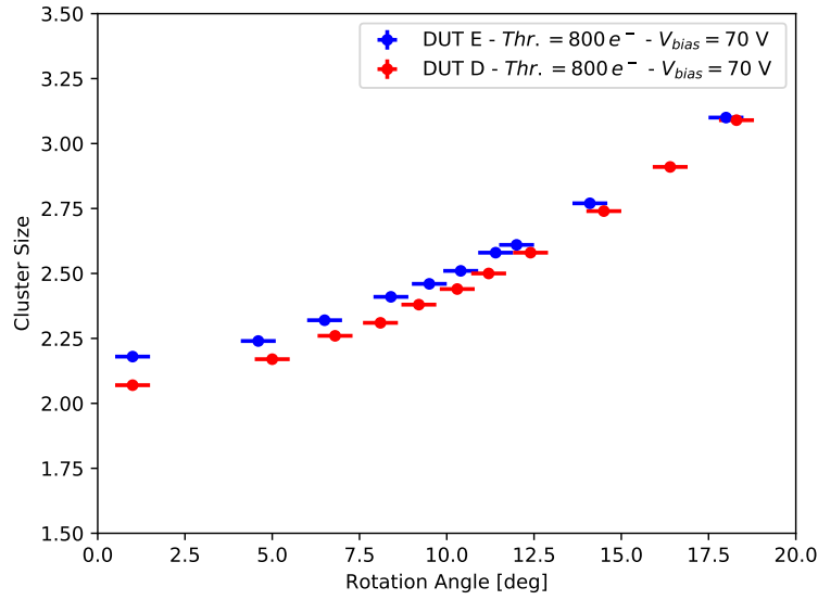
Figure 5.15: DUT D and DUT E cluster size versus the rotation angle around the y axis (along the 25 \mu m pitch), with V_{bias} = 70 V .
