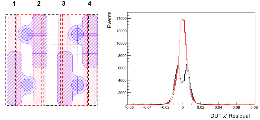
Figure 5.19: Schematic drawing of a 1 \times 4 pixel grid of the DUT E (left) and the residual distributions evaluated on the corresponding areas of the same color (right), with V_{\text{bias}} = 70 \text{ V} . See text for details.
