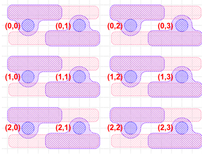
Figure 3.17: 2 \times 6 pixel matrix for a 25 \times 100 \mu\text{m}^2 planar pixel sensor. The bump pads are enumerated with the corresponding RD53A readout channel.
