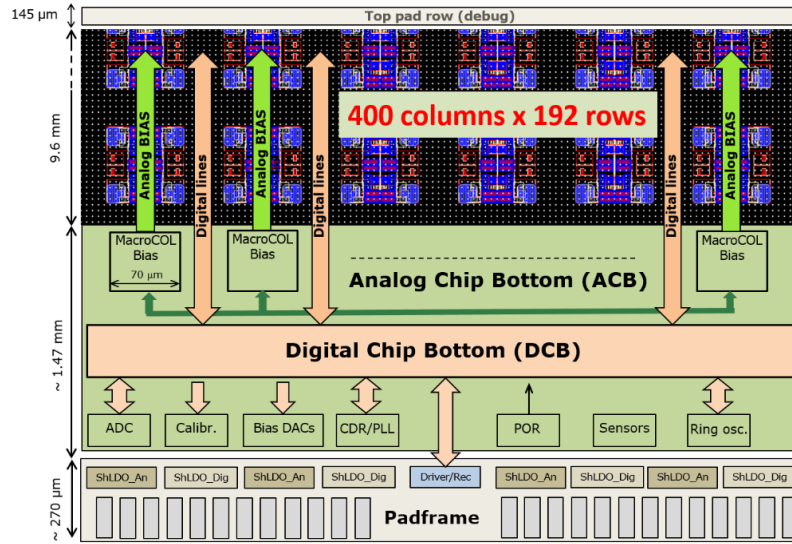
Figure 3.3: The RD53A ROC functional view. In the bottom the wire bonding pads are visible [38].
