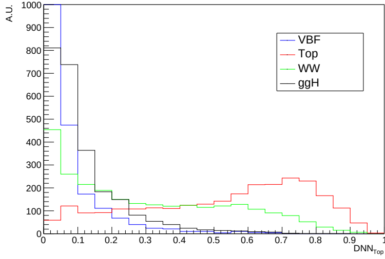
Figure 7.17: \text{DNN}_{\text{Top}} classifier distribution on the training batch.
