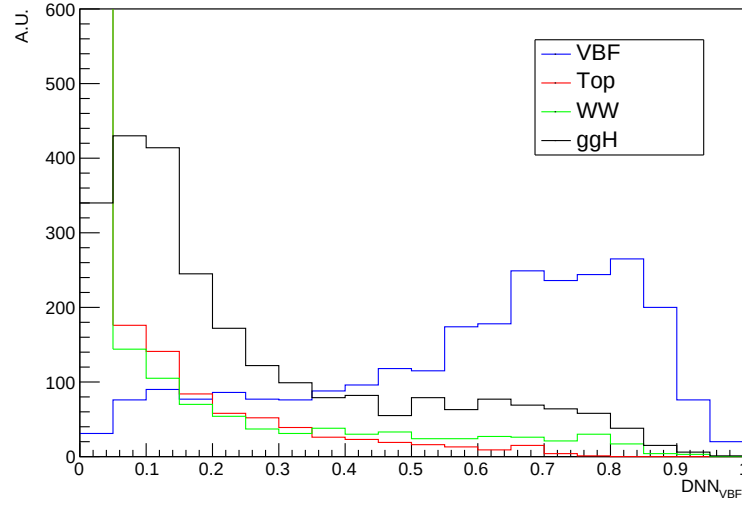
Figure 7.15: \text{DNN}_{VBF} classifier distribution on the training batch.
