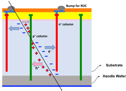
Figure 1.14: Schematic view of a 3D pixel sensor fabricated with the DWB double-sided technique. The drift path of the charge carriers is also highlighted.
