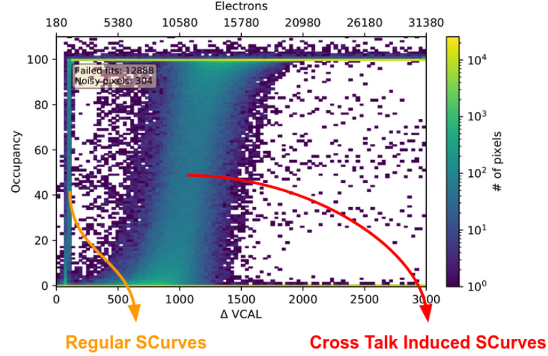
Figure 3.18: SCurve test performed by injecting up to about 30000 electrons on a 25 \times 100 \mu\text{m}^2 planar pixel sensor. Two SCurve distributions are visible: the first one is related to the injected pixels, while the second one is related to the cross-talk coupled pixels.
