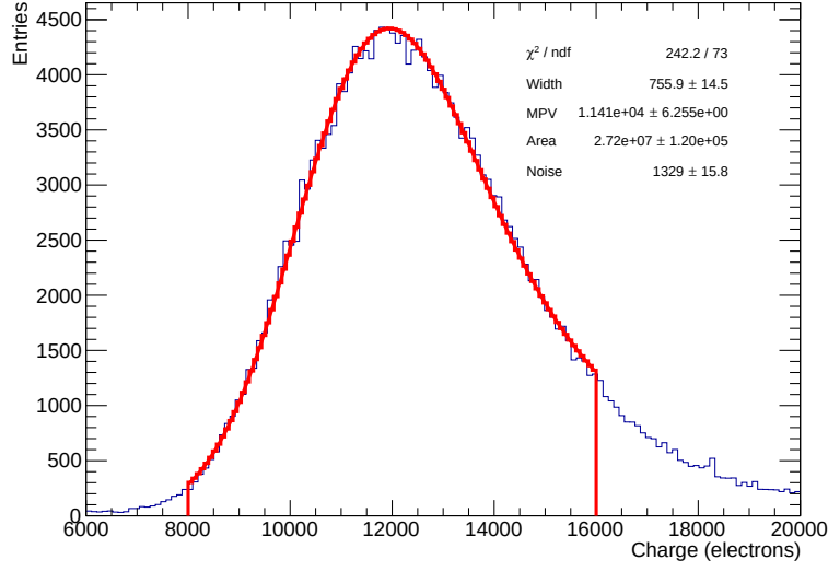
Figure 5.20: DUT D collected charge distribution with V_{\text{bias}} = 70 V. The red line represents a fit to a Landau distribution convoluted with a gaussian distribution.
