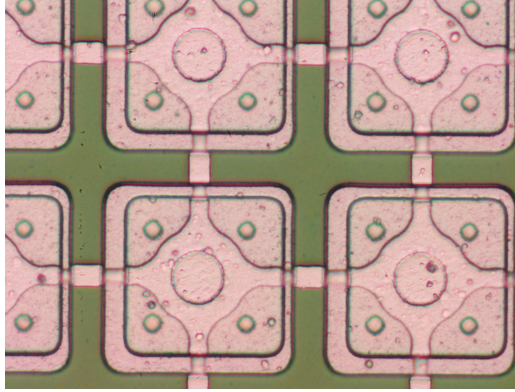
Figure 2.26: Photograph of a 50 \times 50 \mu\text{m}^2 pixel sensor from the P-1 batch, taken on wafer. The temporary metal is still present and connects all the pixels in the matrix.
