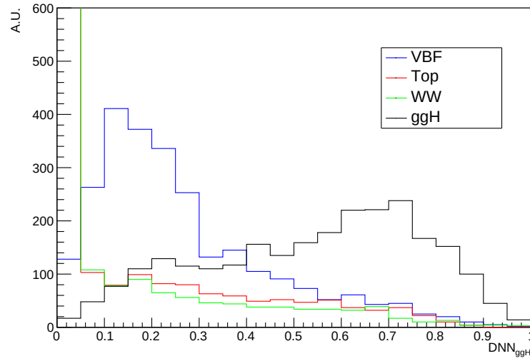
Figure 7.16: \text{DNN}_{ggH} classifier distribution on the training batch.
