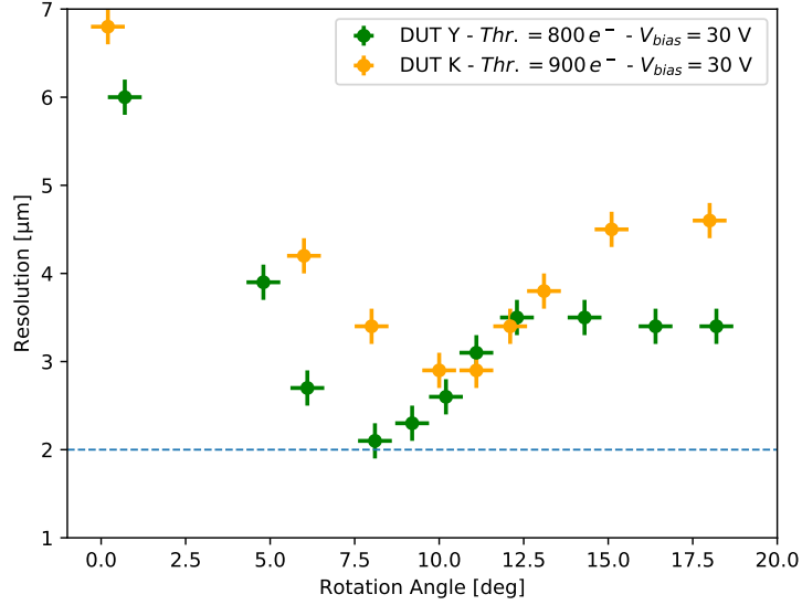
Figure 5.60: DUTs K and Y resolution versus the rotation angle around the y axis (along the 25 \mu\text{m} pitch) with V_{\text{bias}} = 30\text{ V} for both modules. The horizontal line marks 2 \mu\text{m} resolution.
