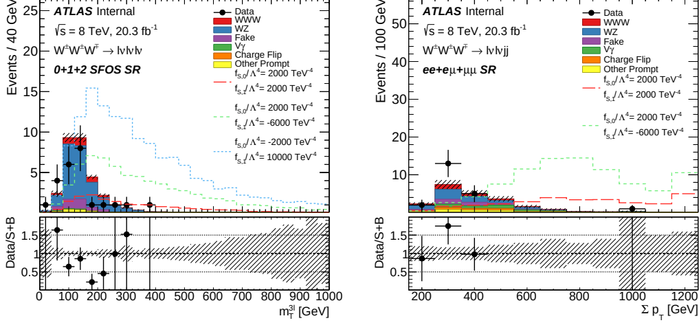
Figure 4.2: The m_T^{3\ell} distribution in the \ell\nu\ell\nu\ell\nu channel (left) and the \Sigma p_T distribution in the \ell\nu\ell\nu jj channel (right). All events from the three signal regions are summed in each channel. The error bars on the data points represent the statistical uncertainty on the data. The hashed area represents the total systematic uncertainties on the signal plus background model. The last bin includes the overflow. The non-unitarized ( \Lambda_F = \infty ) aQGC predictions with nonzero values of some of the anomalous coupling parameters are also represented by the dashed lines.
