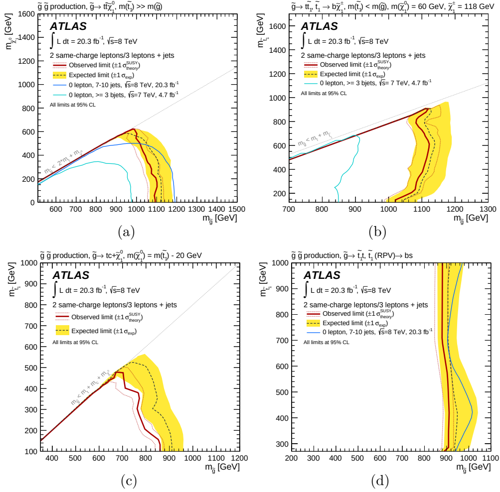
Figure 5.19: Exclusion limits on gluino-mediated top squark production for four different models: (a) gluino-top squark ( t\tilde{\chi}_1^0 ) off-shell, (b) gluino-top squark ( b\tilde{\chi}_1^\pm ) on-shell, (c) gluino-top squark ( c\tilde{\chi}_1^0 ) on-shell and (d) gluino-top squark ( bs ) RPV. A comparison with the previous ATLAS searches available at the time of publication is shown [260, 261].
