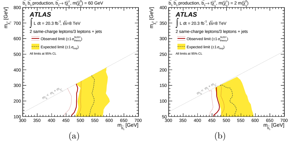
Figure 5.21: Exclusion limits on direct bottom squark production for \tilde{b}_1 \rightarrow t\tilde{\chi}_1^\pm for two different models: (a) m_{\tilde{\chi}_1^0} = 60 \text{ GeV} and (b) m_{\tilde{\chi}_1^\pm} = 2m_{\tilde{\chi}_1^0} .
