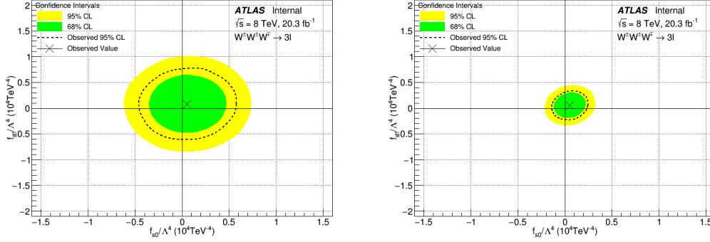
Figure 3.33: Expected 68% and 95% CL contour limits on (f_{S,1}/\Lambda^4, f_{S,0}/\Lambda^4) compared to the observed 95% CL contour limit and observed best fit value for cases when \Lambda_F = 1 \text{ TeV} (left) and \Lambda_F = \infty (right).
