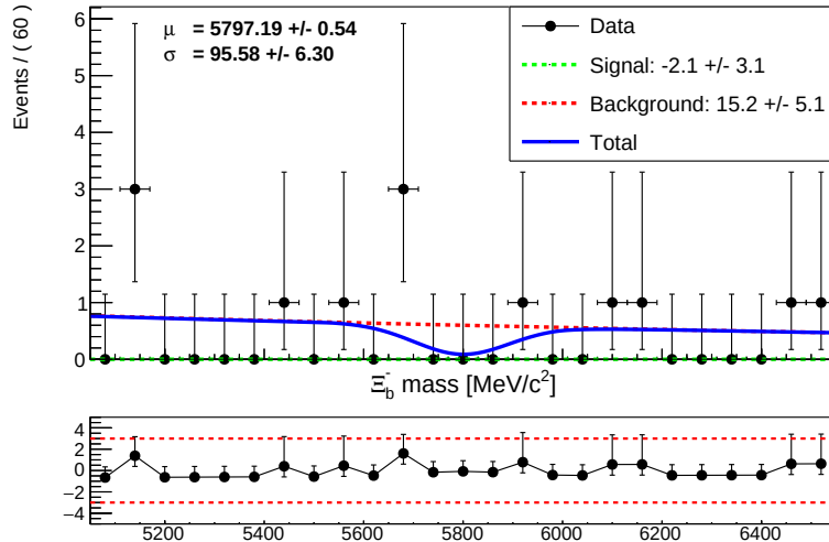
Figure 6.9: Projection to the \Xi_b^- \rightarrow \Xi^- \gamma mass of the simultaneous fit to the \Xi_b^- invariant mass distributions of \Xi_b^- \rightarrow \Xi^- \gamma and \Xi_b^- \rightarrow \Xi^- J/\psi selected candidates with track topology LLL from the 2018 data sample.
