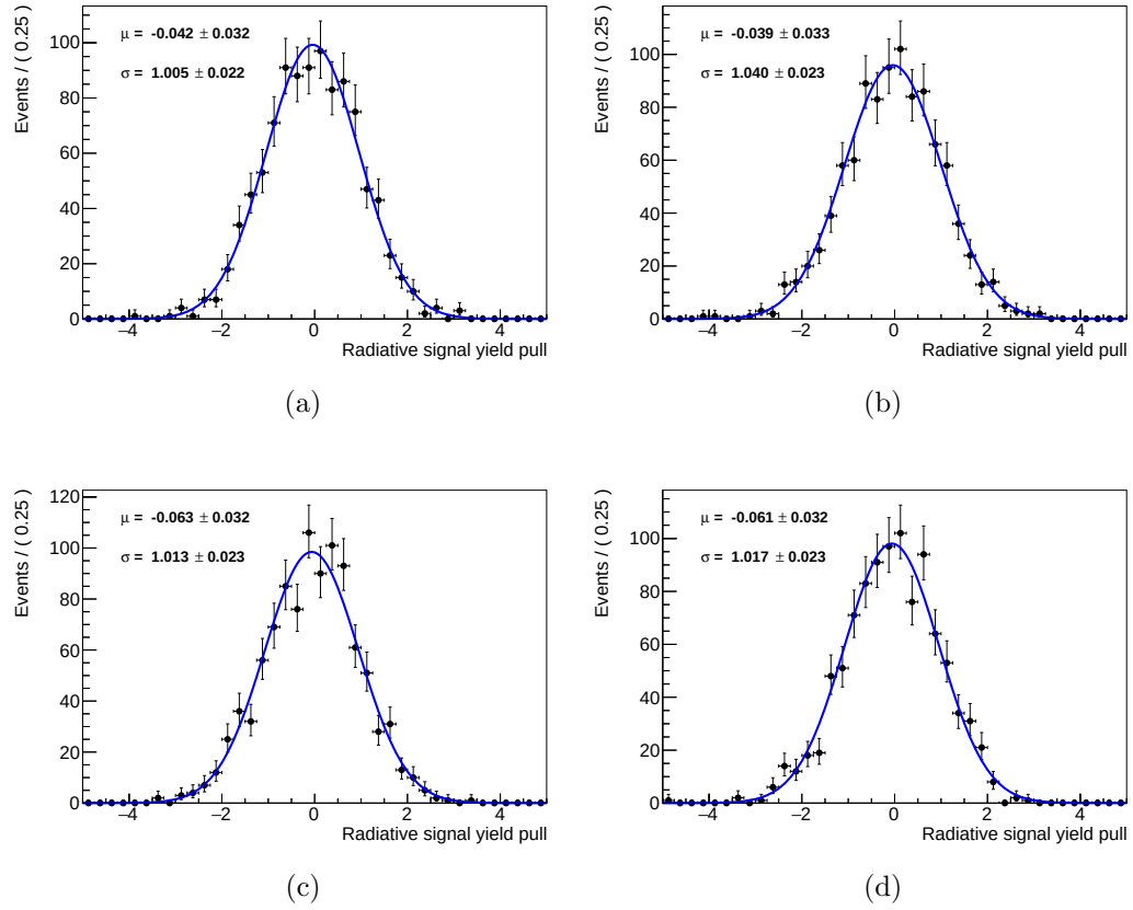
Figure 6.4: Pull distributions for the \Xi_b^- \rightarrow \Xi^- \gamma signal yields generated with the \mathcal{B}(\Xi_b^- \rightarrow \Xi^- \gamma) = (a) 1 \times 10^{-3} , (b) 5 \times 10^{-4} , (c) 1 \times 10^{-4} , (d) 1.1 \times 10^{-5} hypotheses.
