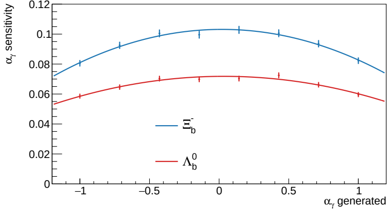
Figure 5.2: Sensitivity to the photon polarization as a function of its value for the \Lambda_b^0 \rightarrow \Lambda \gamma (red) and \Xi_b^- \rightarrow \Xi^- \gamma (blue) decays. A fit to a second order polynomial distribution is overlaid for better visualization.
