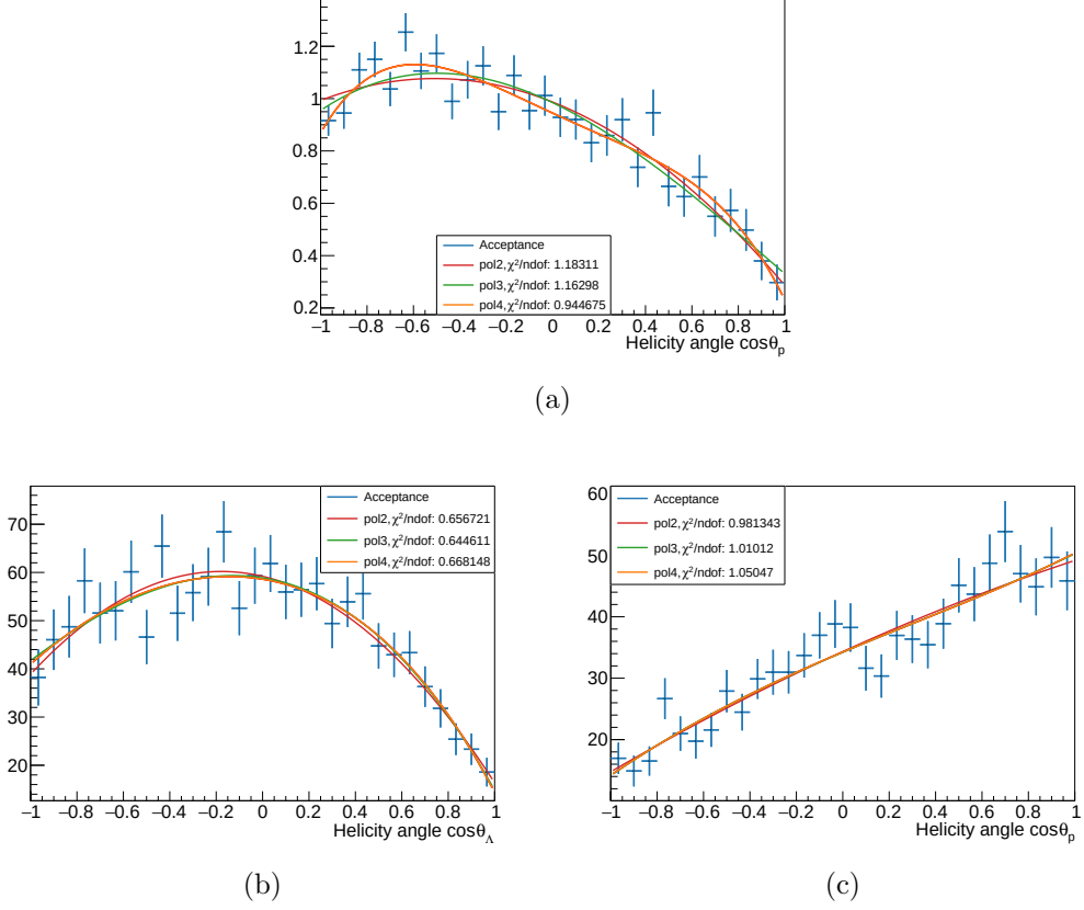
Figure 5.8: Acceptance for the (a) proton helicity angle of \Lambda_b^0 \rightarrow \Lambda\gamma decay, and for the (b) \Lambda and (c) proton helicity angles of the \Xi_b^- \rightarrow \Xi^-\gamma decay after the full selection. Polynomial of different orders are overlaid, along with the \chi^2 of the associated fit.
