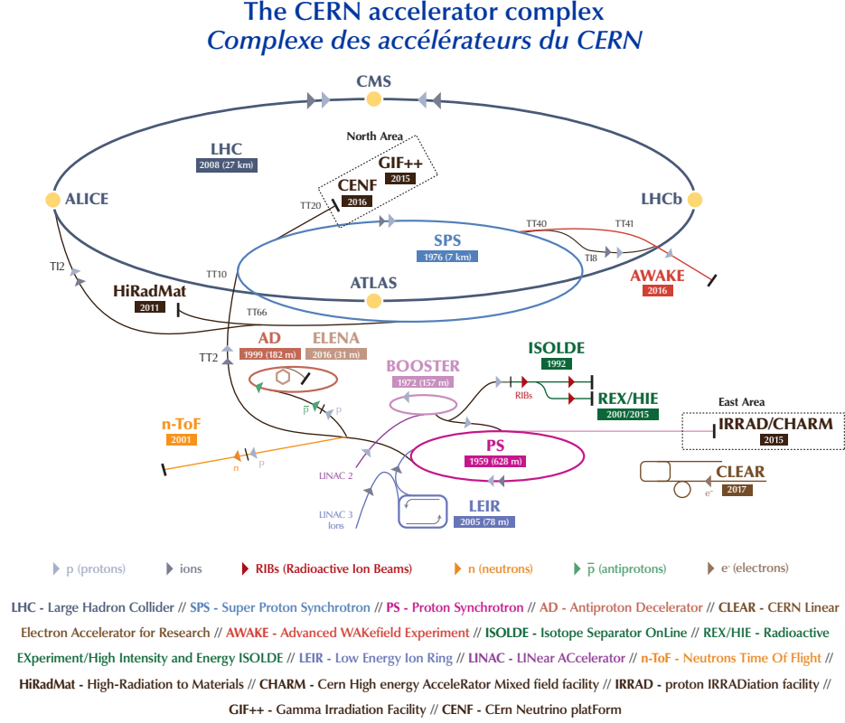
Figure 2.1: Scheme of the CERN accelerator complex [48].
