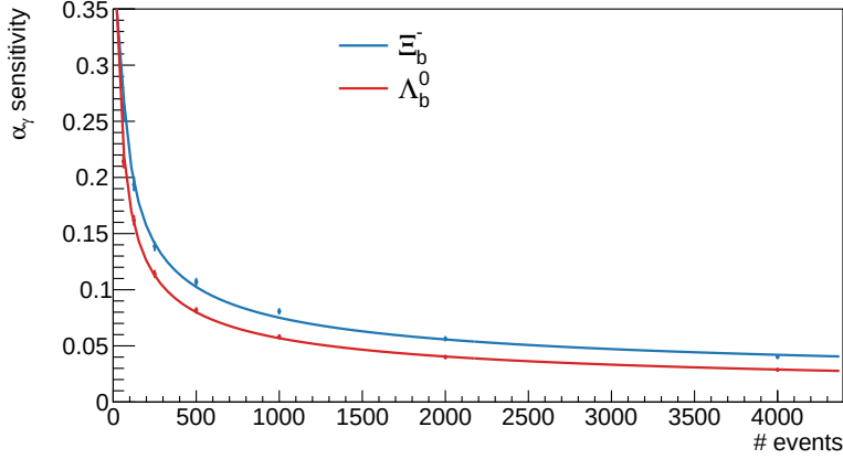
Figure 5.1: Statistical sensitivity to the photon polarization as a function of the number of reconstructed signal events for the \Lambda_b^0 \rightarrow \Lambda \gamma (red) and \Xi_b^- \rightarrow \Xi^- \gamma (blue) decays. The distribution is fitted to a 1/\sqrt{N} function for better visualization.
