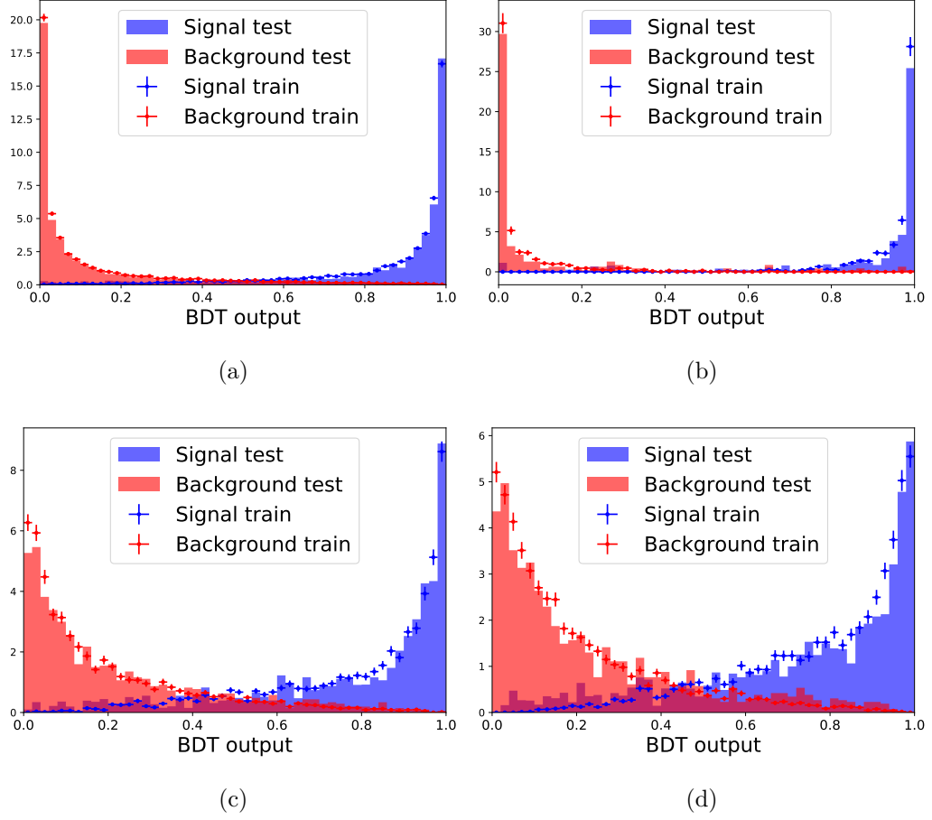
Figure 4.17: Response of the BDT used in the (a) \Lambda_b^0 \rightarrow \Lambda \gamma decay channel and \Xi_b^- \rightarrow \Xi^- \gamma for topologies (b) LLL, (c) DDL and (d) DDD for the signal (blue) and background (red) samples used for training (points) and testing (filled histogram).
