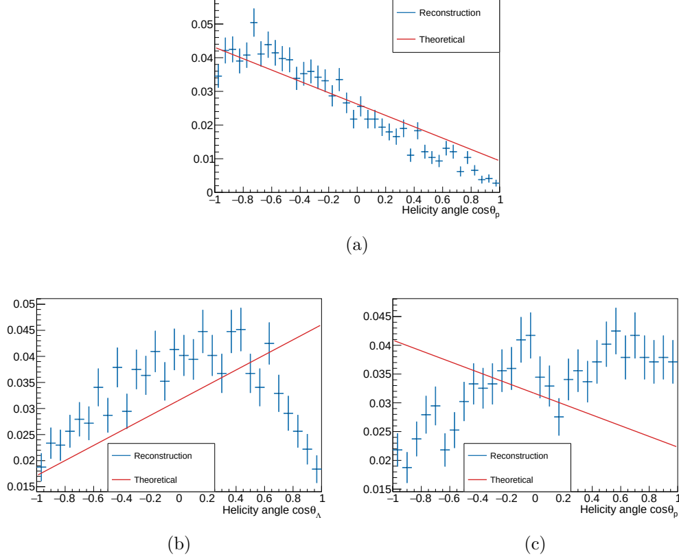
Figure 5.5: Distributions of the (a) proton helicity angle for \Lambda_b^0 \rightarrow \Lambda \gamma , and the (b) \Lambda and (c) proton helicity angles for \Xi_b^- \rightarrow \Xi^- \gamma , for simulated events after selection. The theoretical angular distribution is superimposed for comparison. Only Long tracks are considered here.
