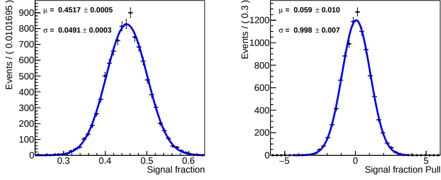
Figure 6.20: Dispersion (left) and pull distribution (right) for signal fraction fitted values from the MC study performed for \Lambda_b^0 \rightarrow \Lambda \gamma , including acceptance and background effects. A Gaussian fit is superimposed.
