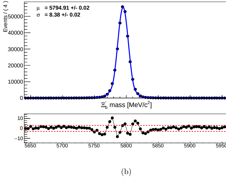
Figure 6.2: Projections of the simultaneous fit to the \Xi_b^- invariant mass distributions of (a) \Xi_b^- \rightarrow \Xi^- \gamma and (b) \Xi_b^- \rightarrow \Xi^- J/\psi in the full mass range for signal MC selected candidates. A DSCB function is used for the mass modeling. All track topologies (LLL, DDL and DDD) are combined.
