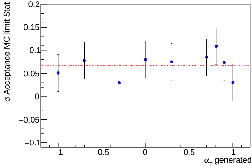
Figure 6.21: Systematic uncertainty as a function of the generated \alpha_\gamma value in the \Lambda_b^0 \rightarrow \Lambda \gamma MC study performed to account for the limited statistics on the acceptance parametrization.
