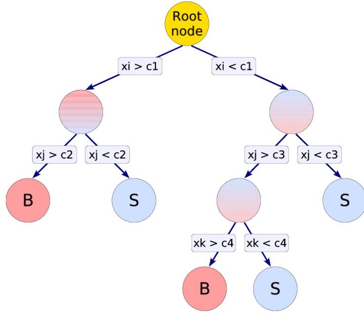
Figure 4.16: Structure of a general Decision Tree [107].
