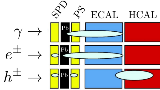
Figure 2.13: Sketch of the calorimeter system of the LHCb. The light blue zones represent the typical response of the system to different species of particles.
