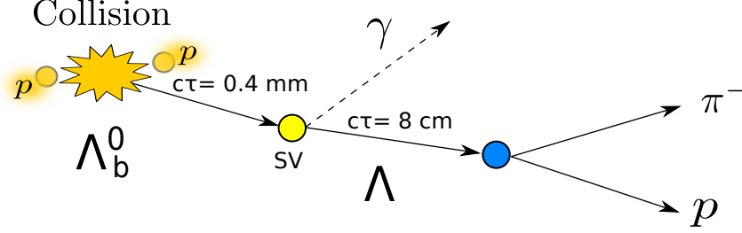
Figure 4.1: Topology of the \Lambda_b^0 \rightarrow \Lambda \gamma decay.
