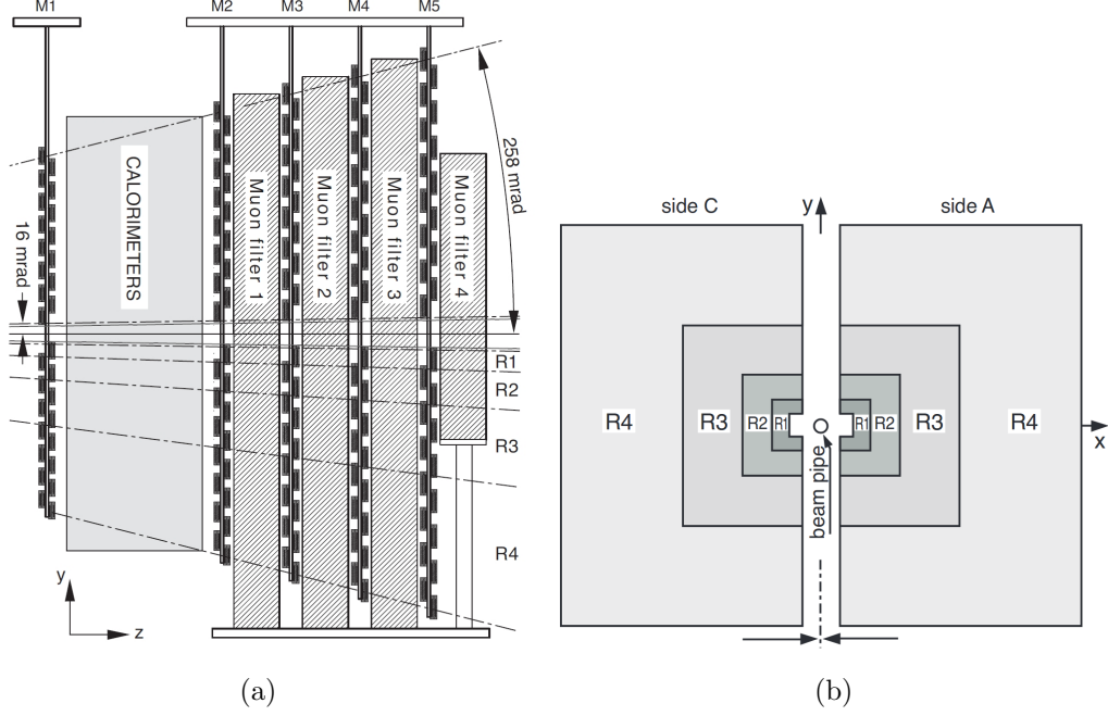
Figure 2.14: (a) Cross section view of the muon chambers and the relative location of the muon station with respect to the calorimeter system. The muon filters can also be seen. (b) Frontal view of one of the muon stations where the four regions with different granularity are shown [64].
