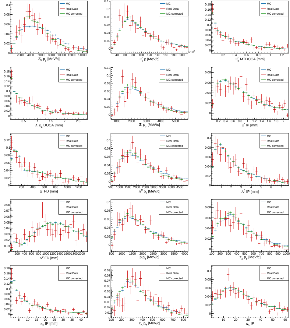
Figure A.7: Distributions from \Xi_b^- \rightarrow \Xi^- J/\psi s-weighted data (red), MC (blue) and corrected MC (green).
