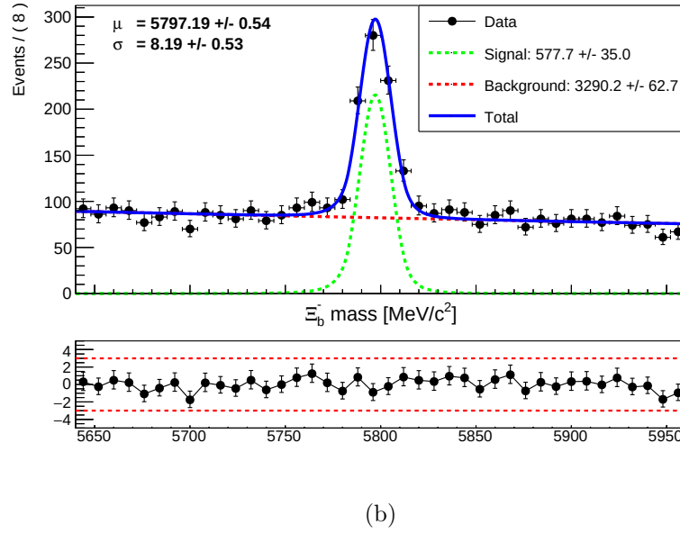
Figure 6.6: Projections of the simultaneous fit to the \Xi_b^- invariant mass distributions of (a) blinded \Xi_b^- \rightarrow \Xi^- \gamma and (b) \Xi_b^- \rightarrow \Xi^- J/\psi selected candidates from the 2018 data sample.
