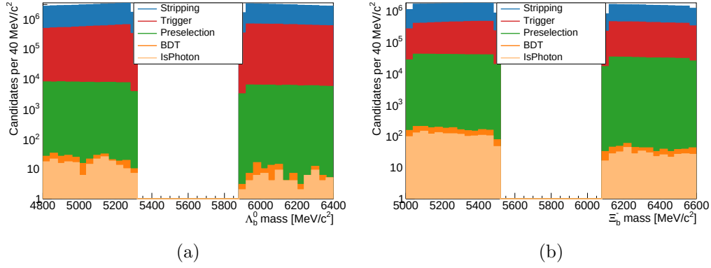
Figure 4.20: Effect of each selection stage in the side-bands of the b -baryon invariant mass distribution for the (a) \Lambda_b^0 \rightarrow \Lambda \gamma and (b) \Xi_b^- \rightarrow \Xi^- \gamma decay channels.
