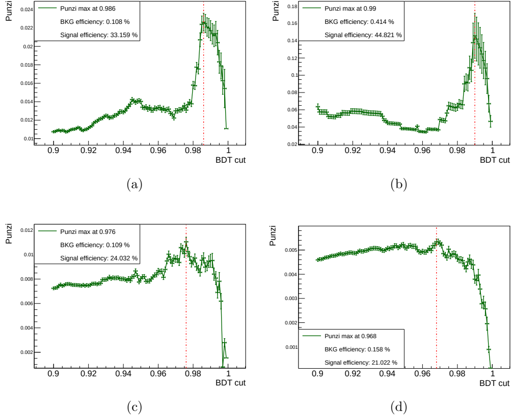
Figure 4.19: Punzi Figure of Merit as a function of the requirement (cut value) on the BDT response for (a) \Lambda_b^0 \rightarrow \Lambda \gamma and \Xi_b^- \rightarrow \Xi^- \gamma for topologies (b) LLL, (c) DDL and (d) DDD. The optimal cut along with the background rejection and signal efficiency are also shown.
