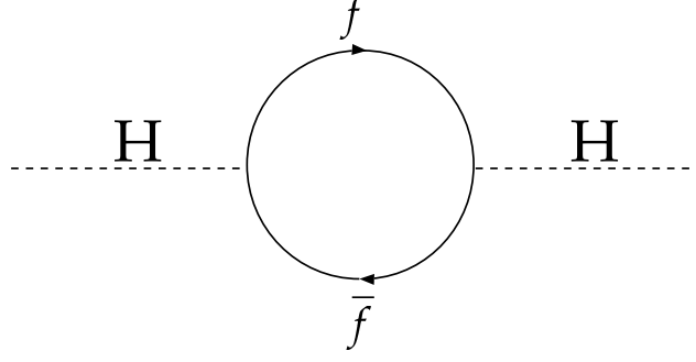
Figure 1.2: 1-loop diagrams contributing to m_H correction
