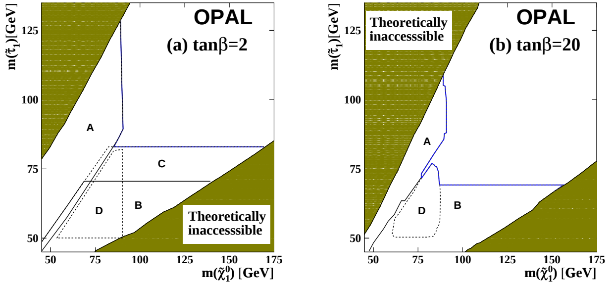
Figure 6.3: Excluded regions at the 95 % C.L. in the m_{\tilde{\ell}} versus m_{\tilde{\chi}_1^0} plane for (a) \tan\beta = 2 (slepton co-NLSP case) and (b) \tan\beta = 20 (stau NLSP case). Also shown are the regions exclusively excluded by (A) \tilde{\chi}_1^0\tilde{\chi}_1^0 \rightarrow \gamma\tilde{G}\gamma\tilde{G} , (B) \tilde{\tau}^+\tilde{\tau}^- \rightarrow \tau^+\tilde{G}\tau^-\tilde{G} , (C) \tilde{\mu}^+\tilde{\mu}^- \rightarrow \mu^+\tilde{G}\mu^-\tilde{G} and (D) \tilde{\chi}_1^0\tilde{\chi}_1^0 \rightarrow 4\text{-lepton final states} . The other search channels do not contribute significantly to the exclusion regions in the MGM model. The shaded regions are theoretically inaccessible.
