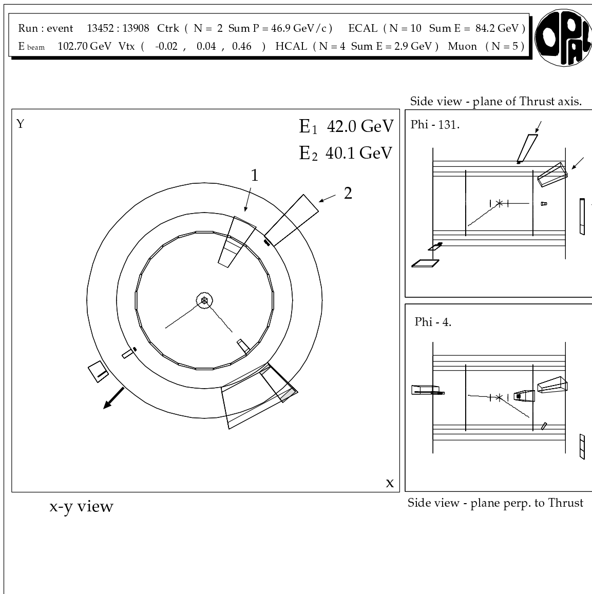
Figure 5.17: The candidate (#run=13452 , #evt=13908) selected by Analysis A.
