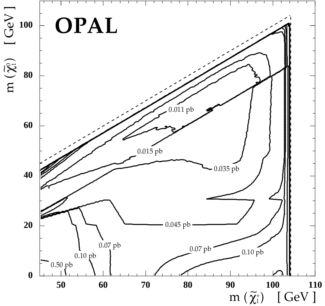
Figure 5.23: Limits at the 95 % C.L. for the production cross-section of e^+e^- \rightarrow \tilde{\chi}_1^+ \tilde{\chi}_1^- at \sqrt{s} = 208.0 GeV are shown, assuming the decays \tilde{\chi}_2^0 \rightarrow \tilde{\chi}_1^0 W^{\pm(*)} followed by the prompt decays \tilde{\chi}_1^0 \rightarrow \gamma \tilde{G} . The dashed line indicates the kinematic limit.
