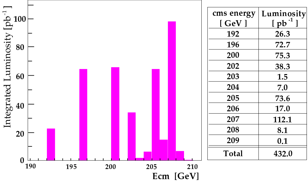
Figure 5.1: Luminosities at each cms energy during 1999 and 2000 data taking. The total luminosity is 432 pb -1 .
