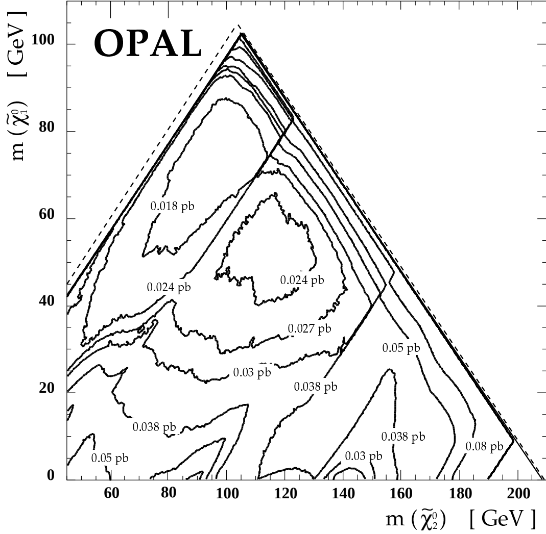
Figure 5.24: Limits at the 95 % C.L. for the production cross-section of e^+e^- \rightarrow \tilde{\chi}_1^0 \tilde{\chi}_2^0 at \sqrt{s} = 208.0 GeV are shown, assuming the decays \tilde{\chi}_2^0 \rightarrow \tilde{\chi}_1^0 Z^{0(*)} followed by the prompt decays \tilde{\chi}_1^0 \rightarrow \gamma \tilde{G} . The dashed line indicates the kinematic limit.
