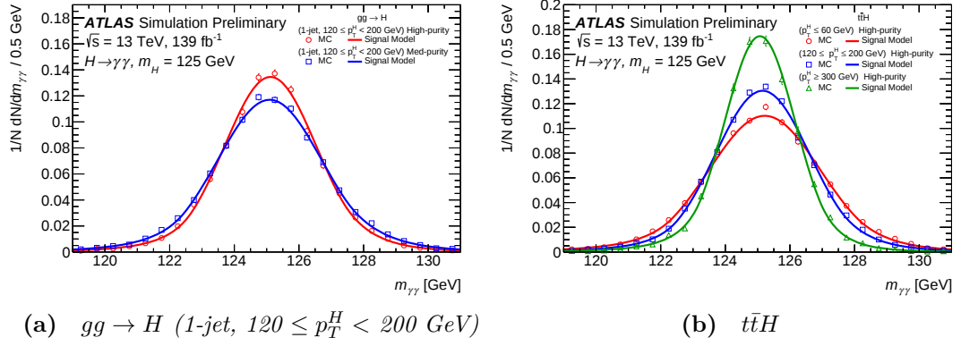
Figure 6.2 Signal shapes in the diphoton invariant mass spectra for two purity categories for gg \rightarrow H (1-jet, 120 \leq p_T^H < 200 \text{ GeV} ) and three t\bar{t}H analysis categories, fitted as double-sided Crystal Ball functions to signal Monte Carlo samples [53].
