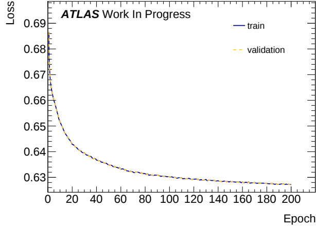
Figure 9.3 Loss values as a function of epoch when training the CARL neural network on the training and validation samples.
