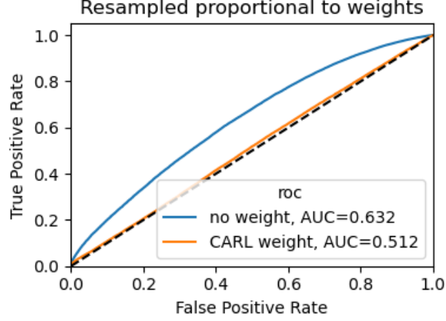
Figure 9.5 Validation sample ROC curves for the neural network classifier trained to distinguish 4-flavour and 5-flavour generated tHqb events. The blue curve is the performance of the classifier in distinguishing unweighted 4-flavour events, while the orange shows that of the performance on CARL weighted events.
