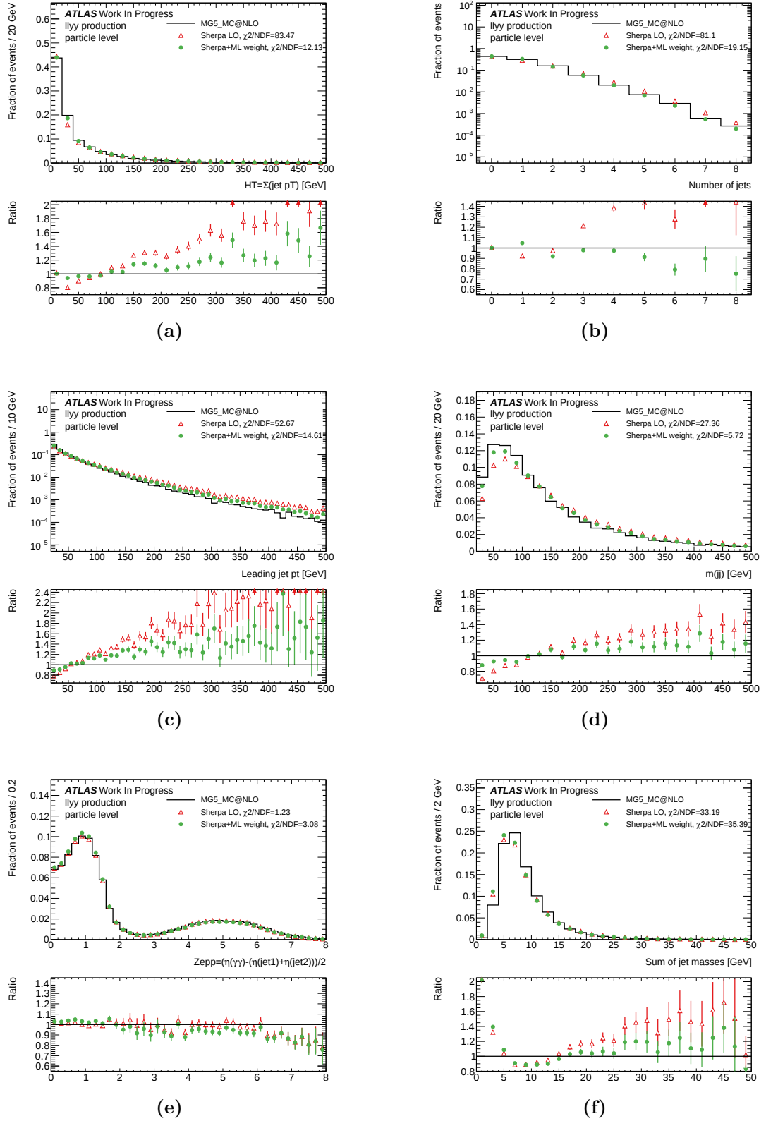
Figure 10.6 Comparing the distributions of the CARL weighted and unweighted SHERPA@LO \ell\ell\gamma\gamma events to MADGRAPH_AMC@NLO for the variables with the four greatest ((a)–(d)) and two least ((e)–(f)) \Delta\chi^2/NDF improvement scores.
