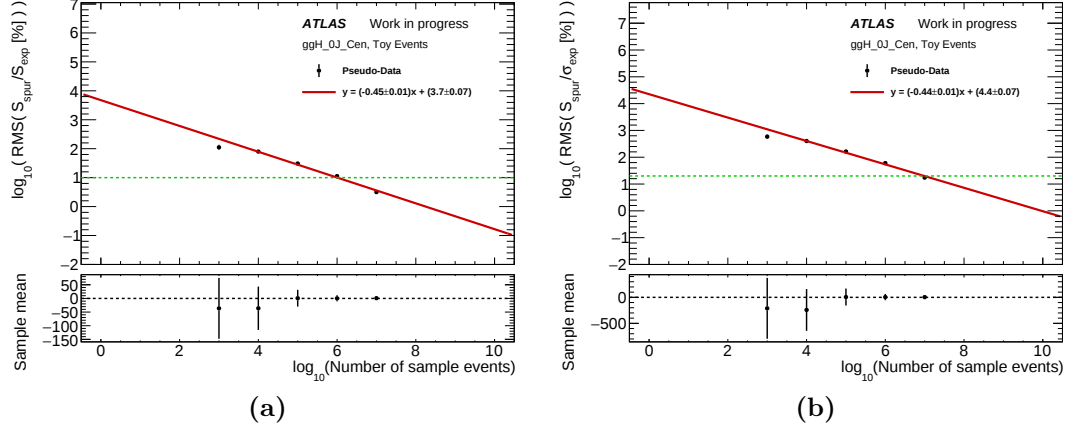
Figure 7.2 The dependence of spurious signal test quantities on the size of the background template it was performed on for the legacy ggH\_0J\_Cen H \rightarrow \gamma\gamma analysis category. The green dotted lines represent the spurious signal passing criteria thresholds, valued at 10 % for (a) and 20 % for (b).
