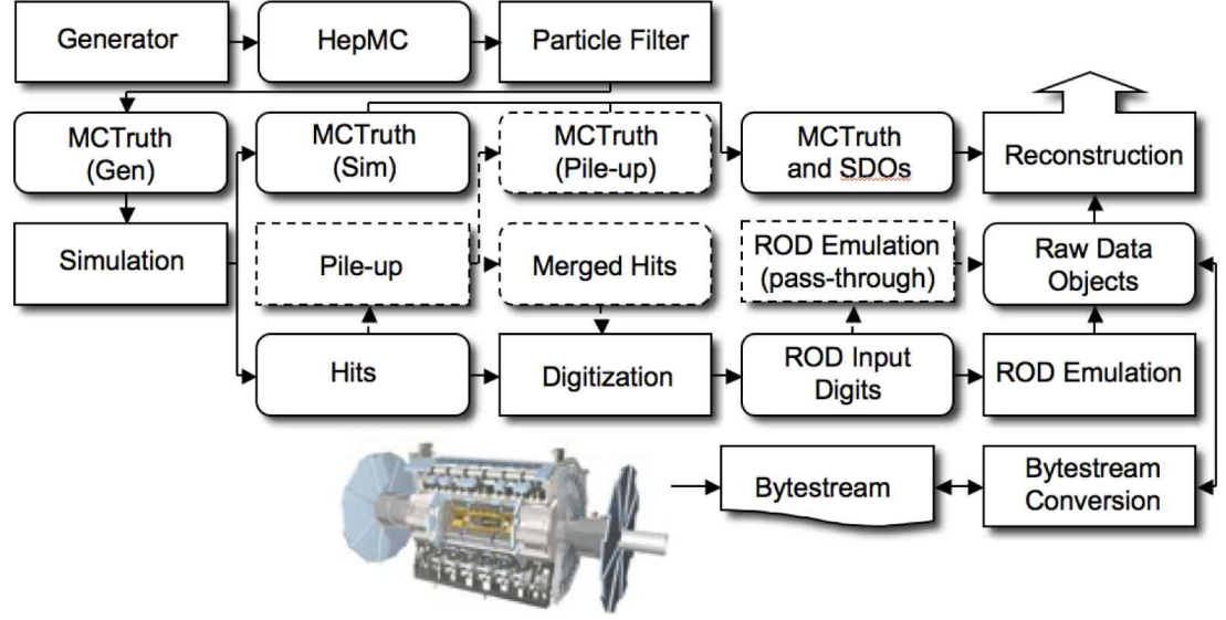
Figure 4.1 Overview of the flow of ATLAS simulation software. The flow-chart starts with event generators in the top left corner through to reconstruction in the top right and also includes the real data path from detector to reconstruction [37].
