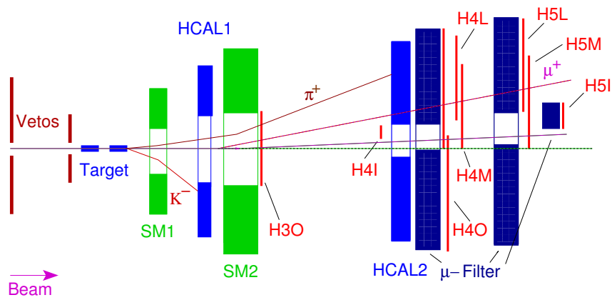
Figure 4.11: Location of the components relevant for the trigger (schematically).
