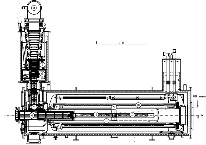
Figure 4.6: Side view of the 2002–2004 COMPASS polarised target: (1) upstream target cell and (2) downstream target cell inside mixing chamber, (3) microwave cavity, (4) target holder, (5) still ^3\text{He} evaporator, (6) ^4\text{He} evaporator, (7) ^4\text{He} liquid/gas phase separator, (8) ^3\text{He} pumping port, (9) solenoid coil, (10) correction coils, (11) end compensation coil, (12) dipole coil. The muon beam enters from the left. The two halves of the microwave cavity are separated by a thin microwave stopper.
