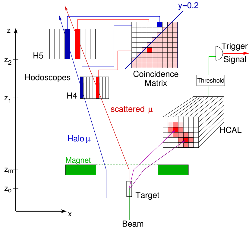
Figure 4.10: Concept of the trigger for quasi-real photoproduction with high energy loss. The scattered muon leads to a coincidence in the activated area of the coincidence matrix while the halo muon fails to do so. In addition, a minimum hadron energy can be required in the calorimeter.
