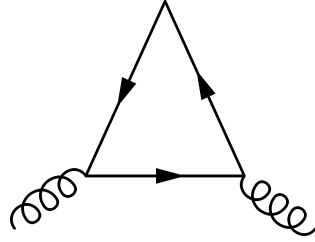
Figure 3.4: Triangle diagram which gives rise to the axial anomaly.
