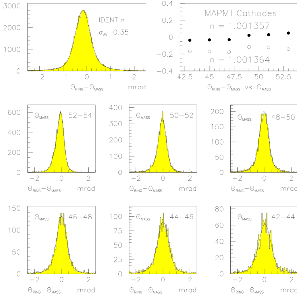
Figure 5.7: \theta_{ring} - \theta_{mass} distribution (top left plot) and the same distribution in bins of \theta_{mass} (centre and bottom plots). The distribution of the mean values of \theta_{ring} - \theta_{mass} as a function of \theta_{mass} is plotted on the top right side. \theta_{mass} is the Cherenkov angle for a particle assuming the pion mass hypothesis.
