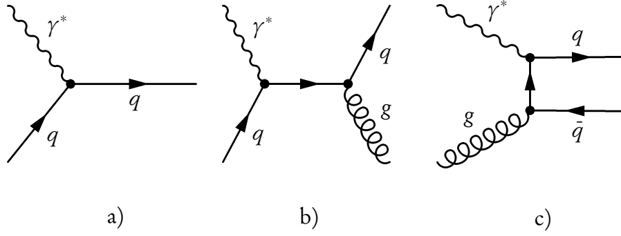
Figure 8.1: The contributing processes: a) DIS LO, b) QCD Compton and c) Photon-Gluon Fusion.
