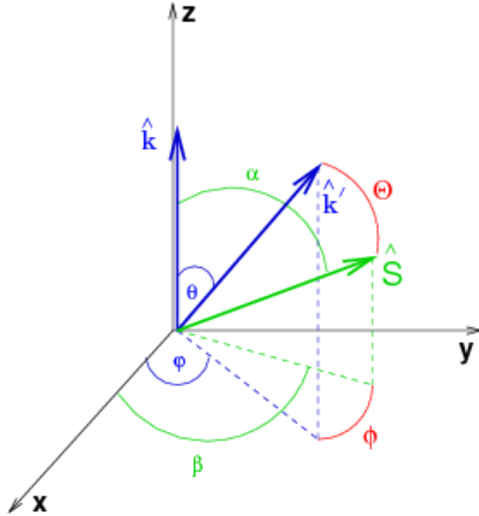
Figure 2.2: Reference system used to represent spin polarisations and their associated angles.
