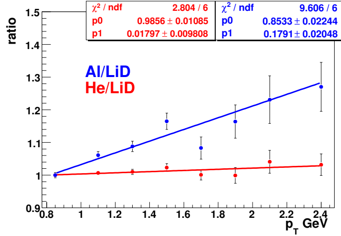
Figure 11.1: Ratios of the observed number of events for different nuclei as functions of the hadron p_T .
