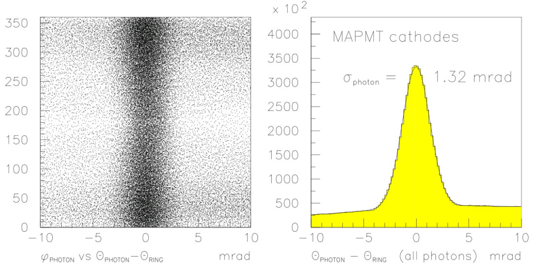
Figure 5.6: \phi_{\text{photon}} against \theta_{\text{photon}} - \theta_{\text{ring}} (left side) and the integrated distribution of \theta_{\text{photon}} - \theta_{\text{ring}} , where \theta_{\text{photon}} and \phi_{\text{photon}} are the photon polar angles around the particle trajectory from pseudo-pads for the MAPMT cathodes.
