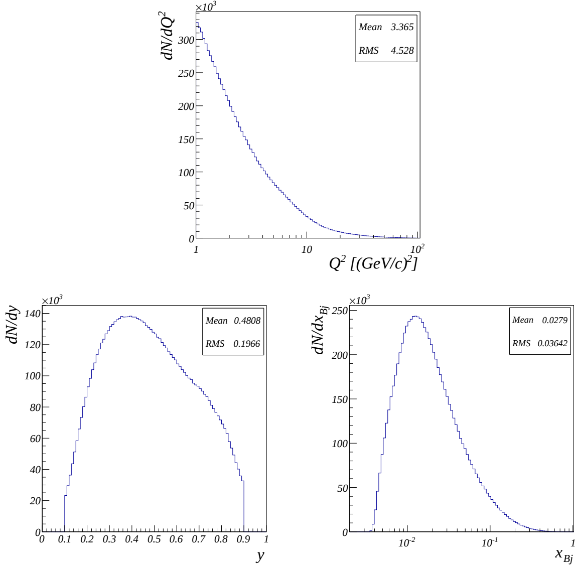
Figure 9.9: Q^2 , y and x distributions after all cuts applied.
