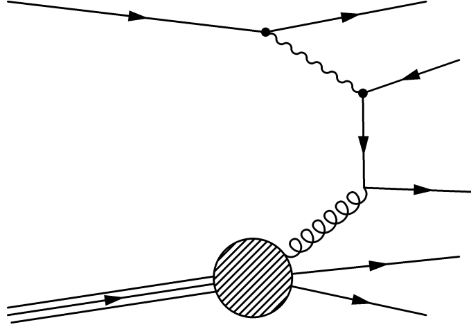
Figure 3.6: Photon-gluon fusion (PGF) process.
