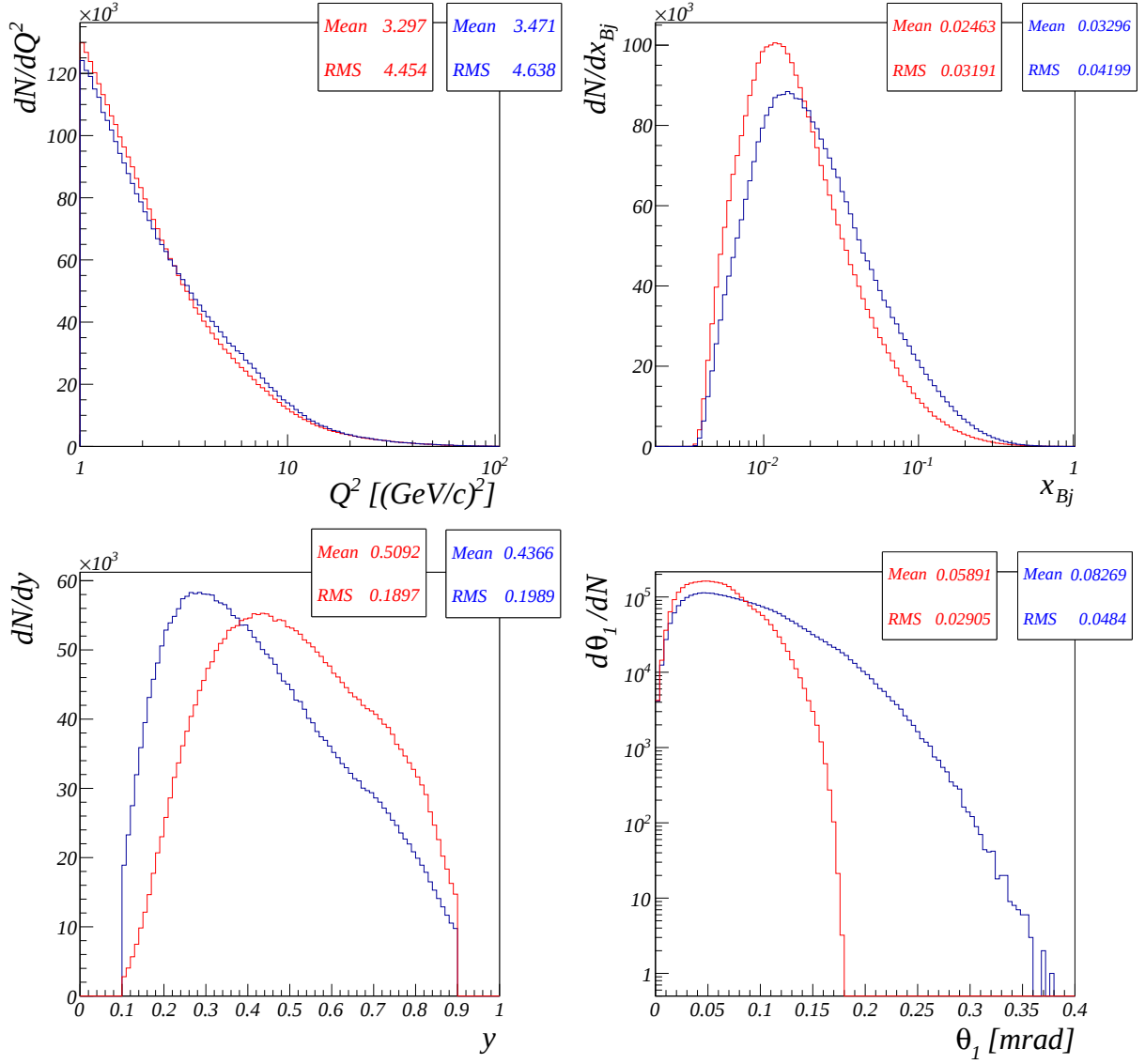
Figure 9.15: Q^2 (top left plot), x_{Bj} (top right plot), y (bottom left plot) and \theta for the leading high p_T (bottom right plot) distributions for 2002-2004 (in red) and 2006 (in blue) data.
