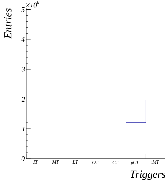
Figure 9.12: Trigger distribution.
