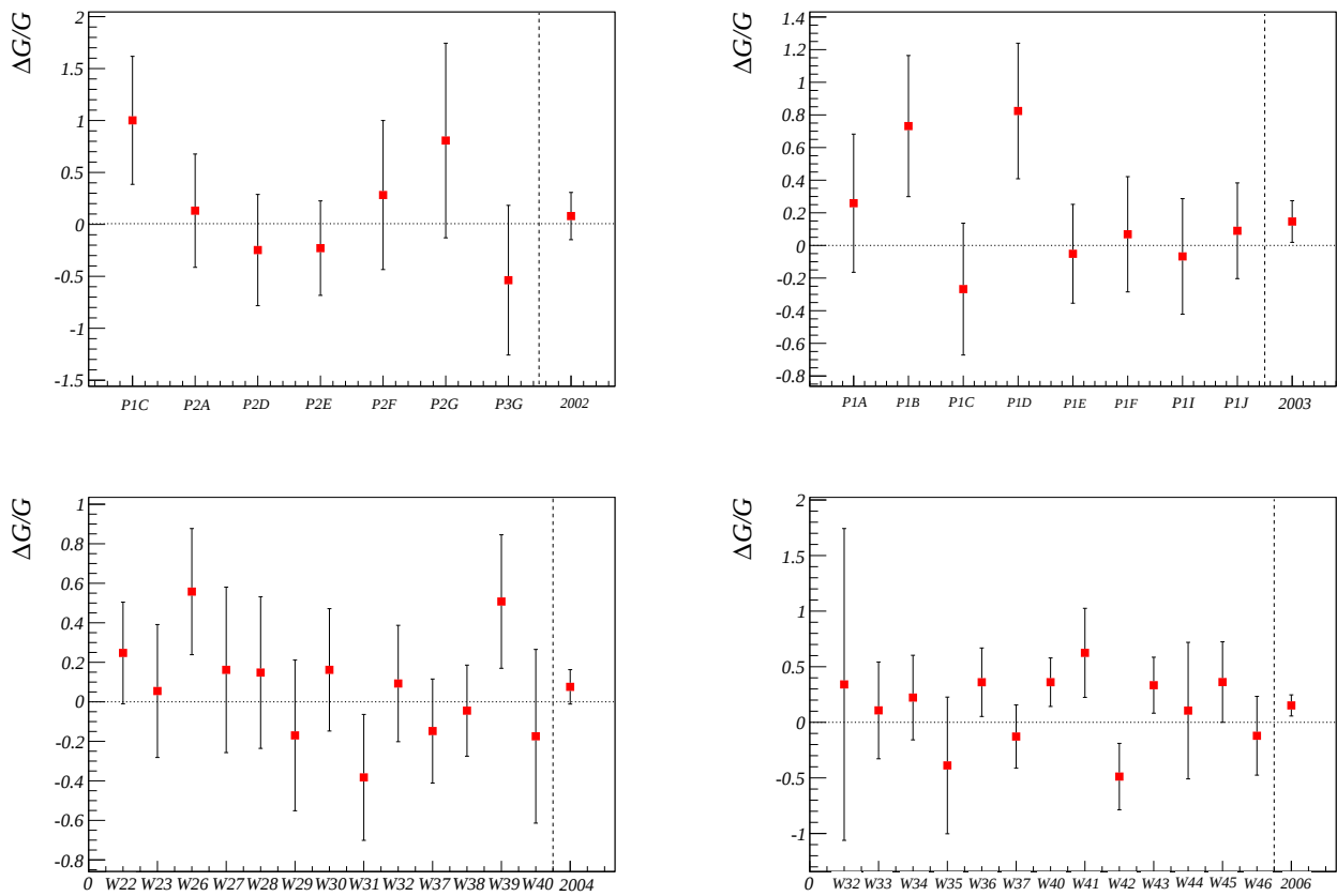
Figure 12.4: The gluon polarisation results are presented per period and distributed in four plots related to the data taking year: 2002 (top left), 2003 (top right), 2004 (bottom left) and 2006 (bottom right). NB. the y-axis of the plot are not at the same scale.
