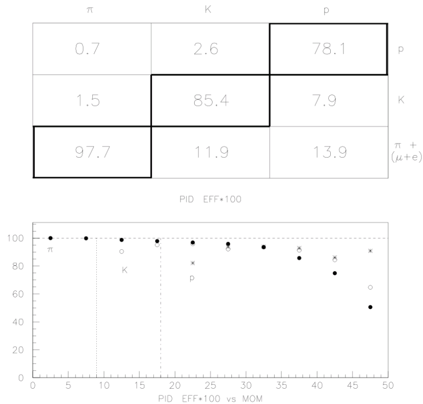
Figure 5.8: On the top part, the table shows the efficiency of identifying the particles, which are divided into pions, kaons and protons, in columns, according to the MC truth information. The values of the efficiencies for the protons, kaons and pions (together with muons and electrons) are given in rows. On the bottom part of the figure, the distribution of the MC PID efficiency for pions (stars), kaons (open dots) and protons (full dots) as a function of the particle momentum.
