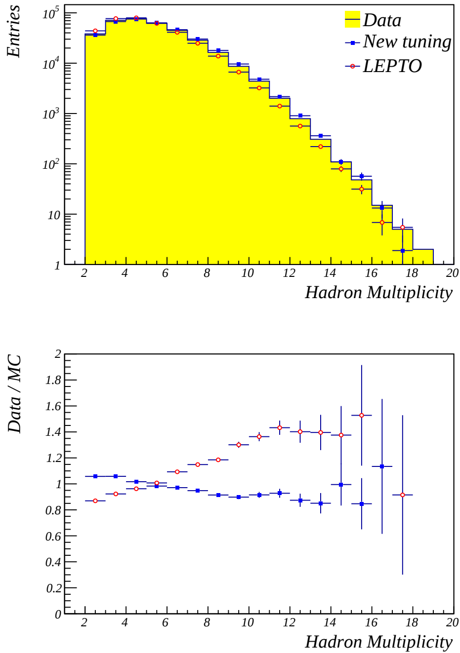
Figure 10.9: Comparison between data and MC simulation: distributions (top) and also Data/MC ratios (bottom) of the hadron multiplicities for the leading and sub-leading hadrons.
