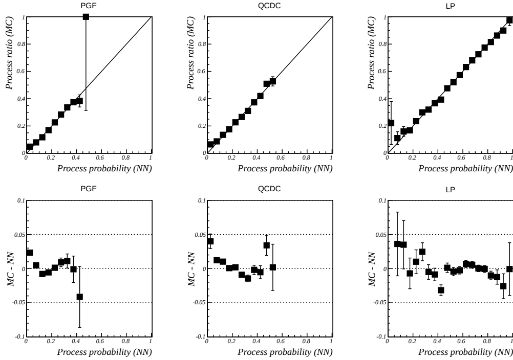
Figure 11.4: Neural network and MC comparison for R_{PGF} , R_{QCDC} and R_{LP} as function of the neural network output.
