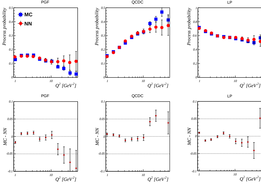
Figure 11.5: Neural network and MC comparison for R_{PGF} , R_{QDC} and R_{LP} as functions of Q^2 . The average of the probability given by the MC (blue squares) and the neural network (red circles) in bins of Q^2 for the three processes is shown in the top row. The differences between the MC and the neural network probabilities are shown in the bottom row.
