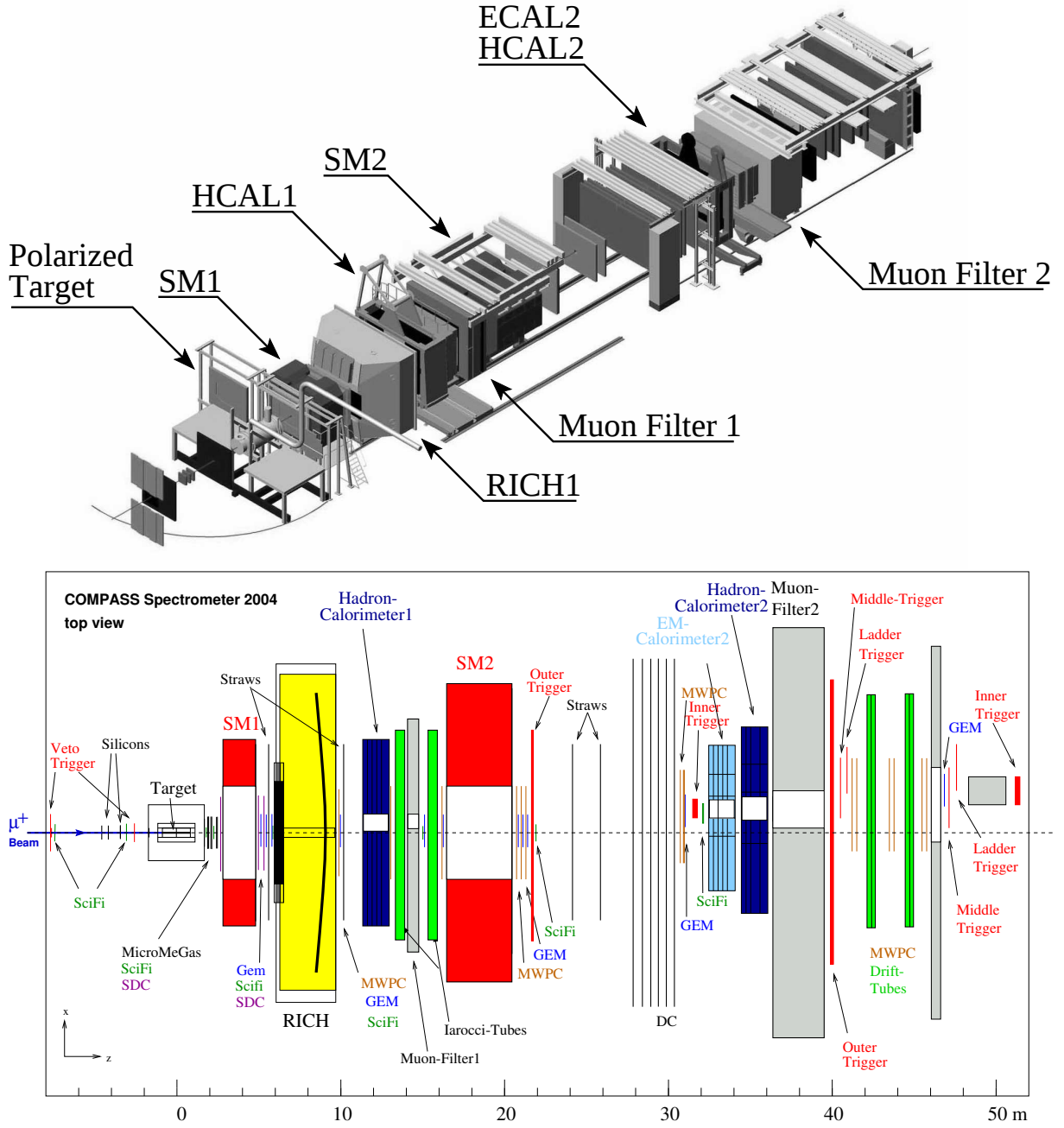
Figure 4.1: Compass 2004 muon setup (top) artistic view, (bottom) top view (for detector names, see text).
