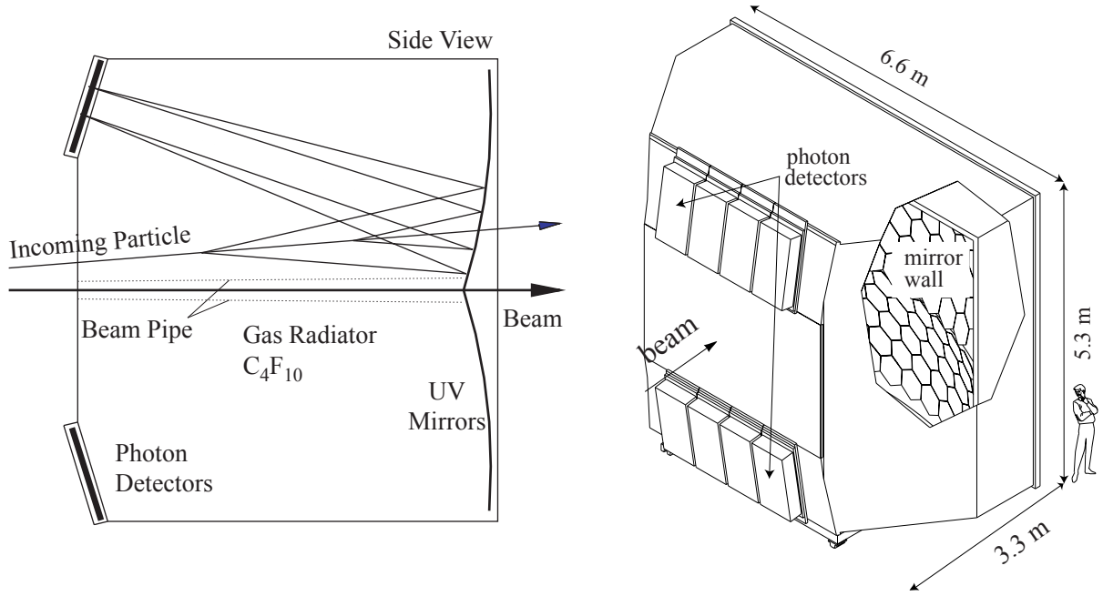
Figure 5.1: COMPASS RICH-1: principle and artistic view.
