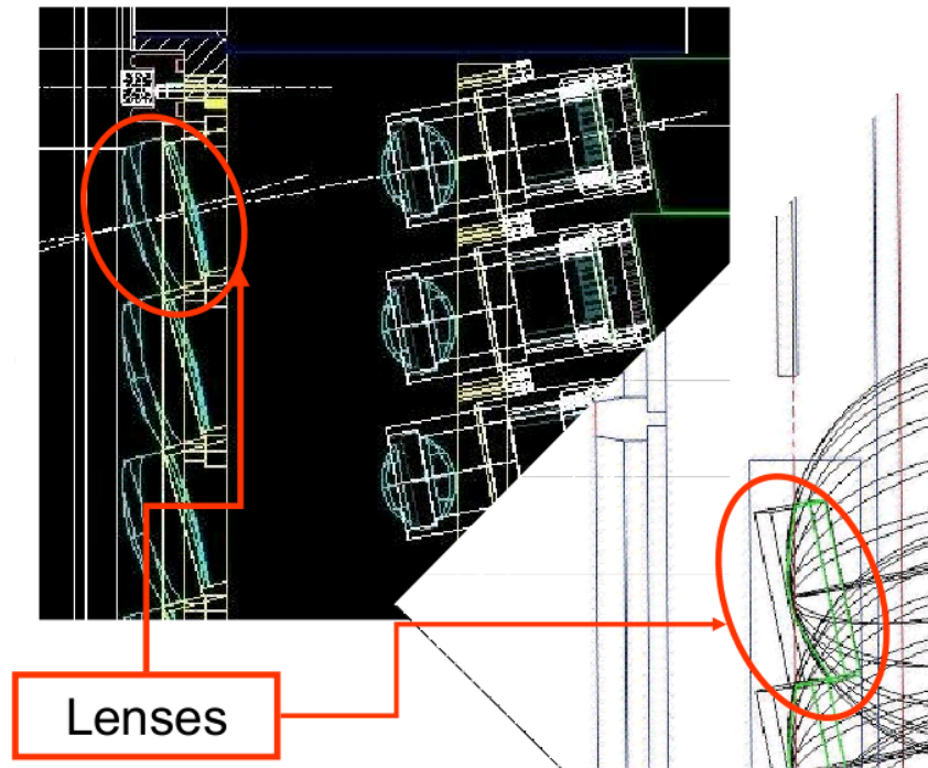
Figure 5.4: The field lens. The field lens and the telescope system (top left) and the field lens implemented in the MC detector simulation (bottom right).
