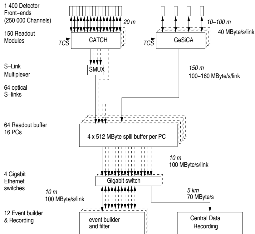
Figure 4.13: General architecture of the DAQ system. Digitised data from the detector front-ends are combined on the readout modules named CATCH and GeSiCA close to the detectors. The storage of the data during the spill and the event building is performed locally. The data are stored at the CERN computer centre.
