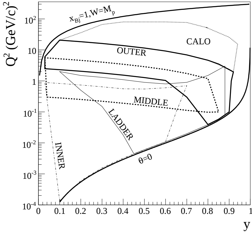
Figure 4.12: The kinematic coverage in y and Q^2 for the four hodoscope trigger subsystems and the standalone calorimetric trigger. The two lines, x_{Bj} = 1, W = M_p and \theta = 0 show the kinematic limits of elastic scattering and forward scattering, respectively.
