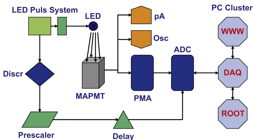
Figure 5.9: Scheme of the test setup showing analog-to-digital converter (ADC), dark current measurement (pA), oscilloscope analysis (osc), data acquisition (DAQ), online monitoring and analysis system based on ROOT [66] (ROOT), data storage and web hosting (WWW).
