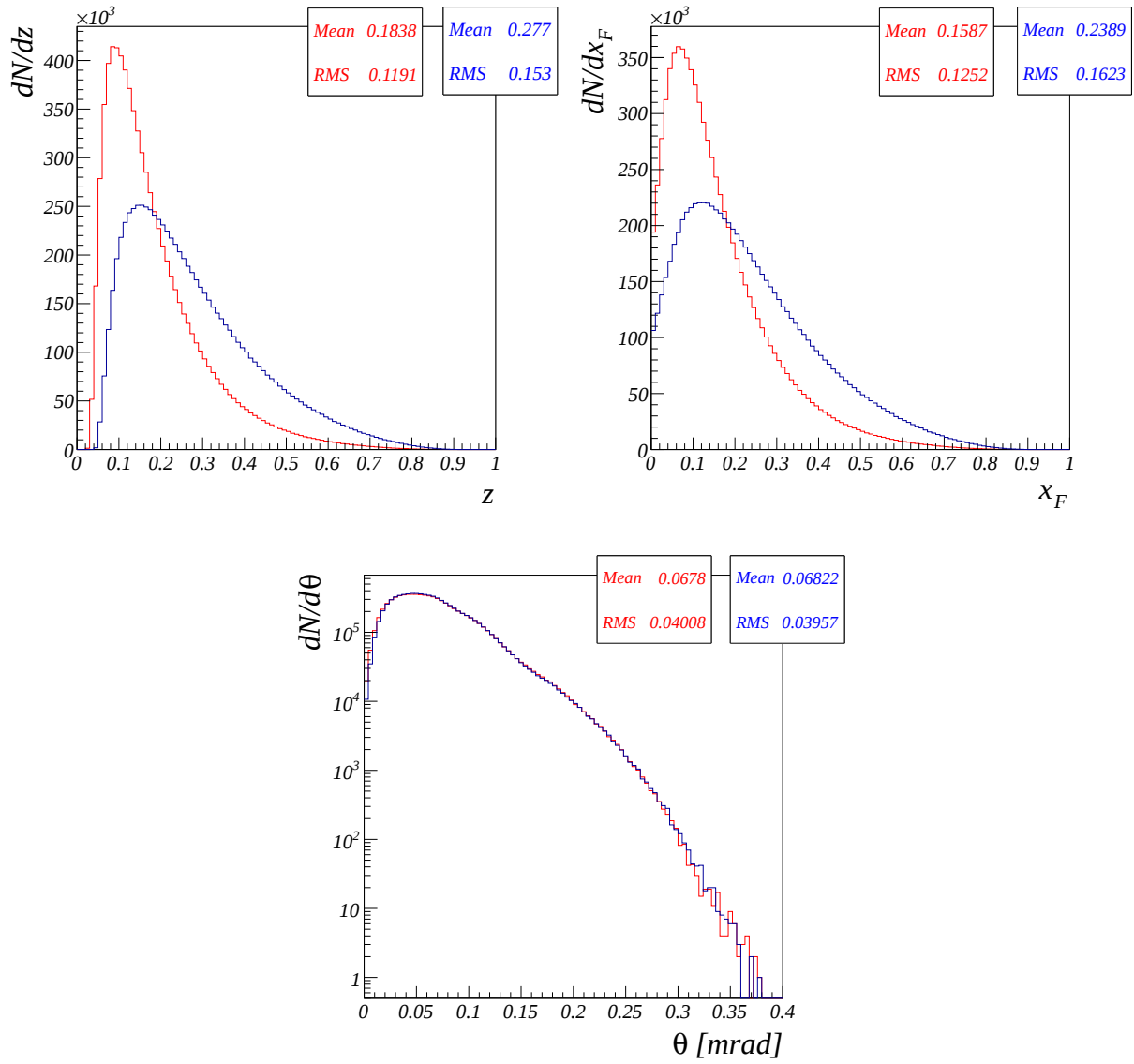
Figure 9.14: z , x_F and \theta distributions for the leading (in blue) and sub-leading (in red) hadrons.
