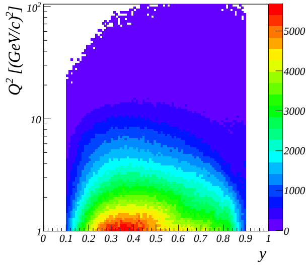
Figure 9.10: Q^2 vs y distribution.
