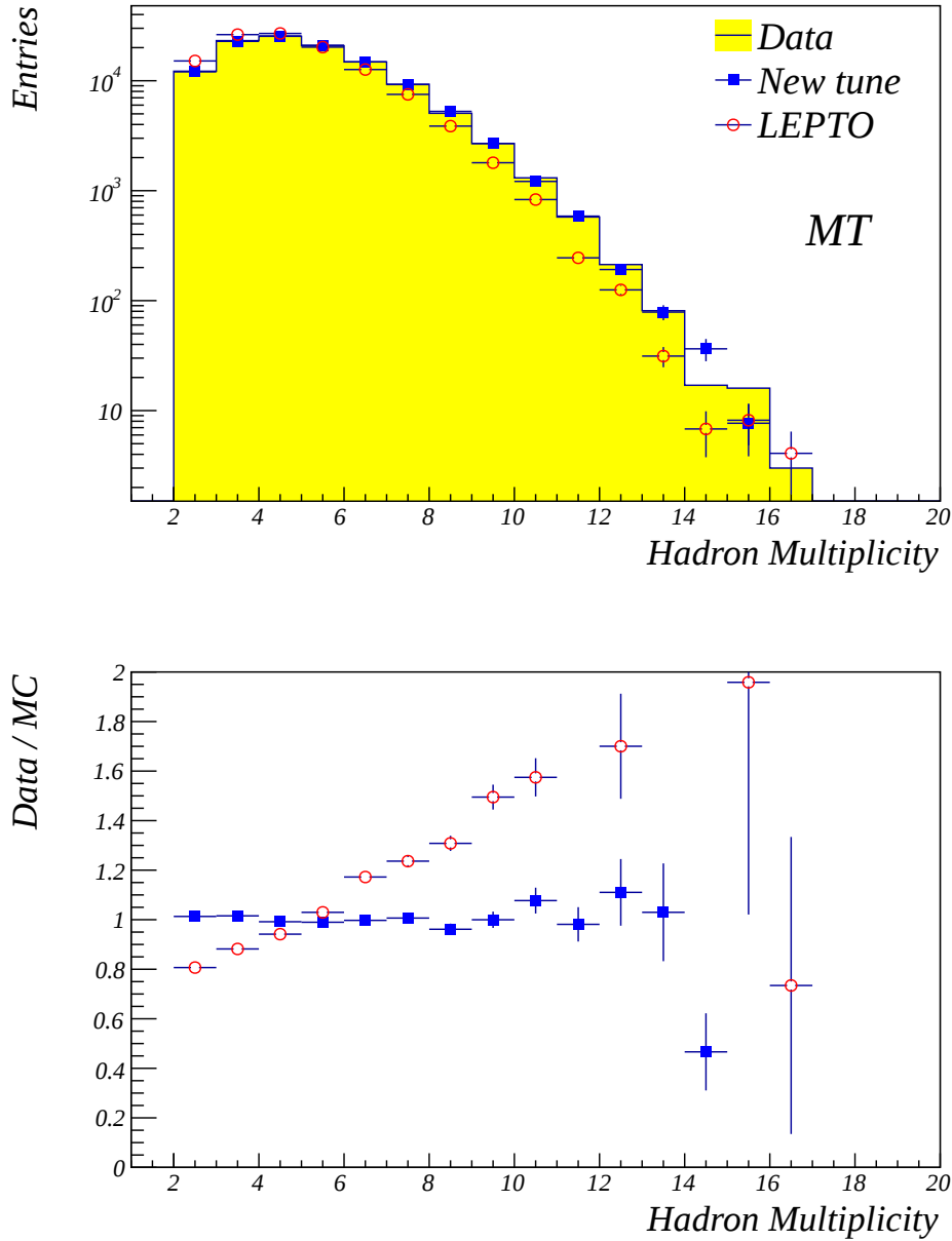
Figure 10.30: Comparison between data and MC simulation for Middle triggers events: distributions (top) and also Data/MC ratios (bottom) of the hadron multiplicities for the leading and sub-leading hadrons.
