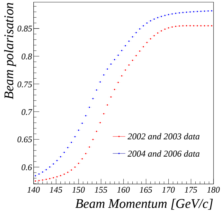
Figure 9.3: Polarisation as a function of the muon momentum.
