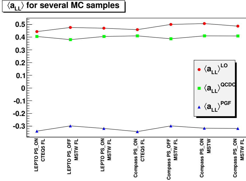
Figure 11.3: Analysing power per process , a_{LL} , for several high p_T MC samples.
