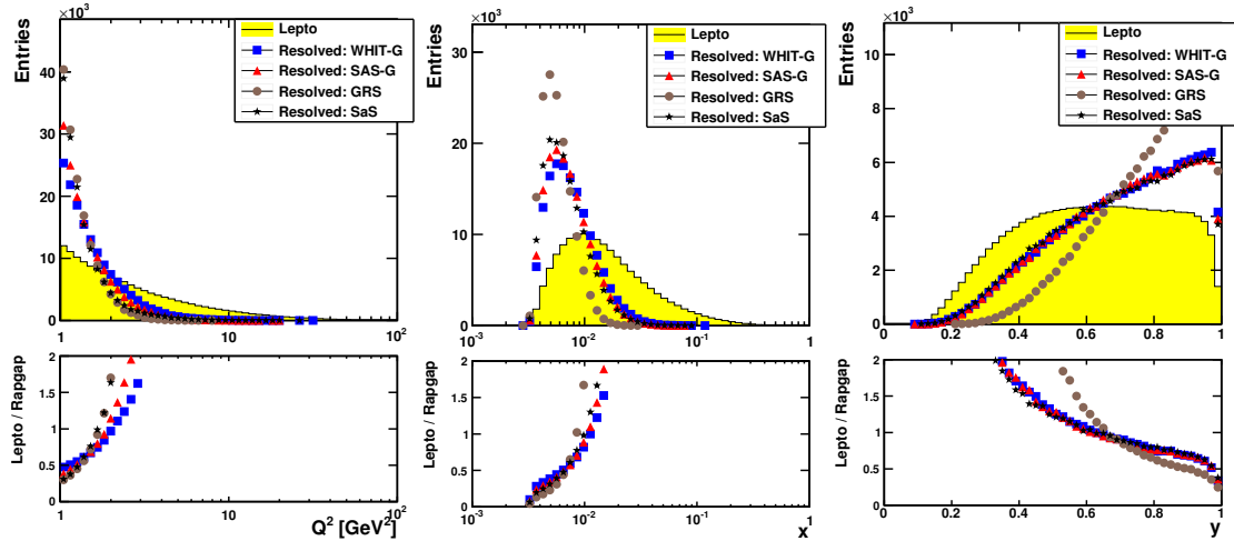
Figure 11.8: Comparison of kinematic distributions of events generated by LEPTO with distributions originating from resolved photon processes obtained from RAPGAP. Different photon PDFs are shown.
