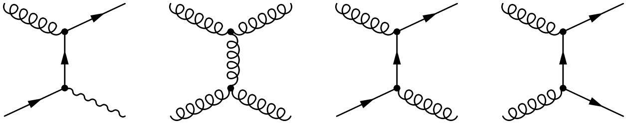
Figure 3.8: Processes involved in the gluon polarisation measurement in p - p collisions.
