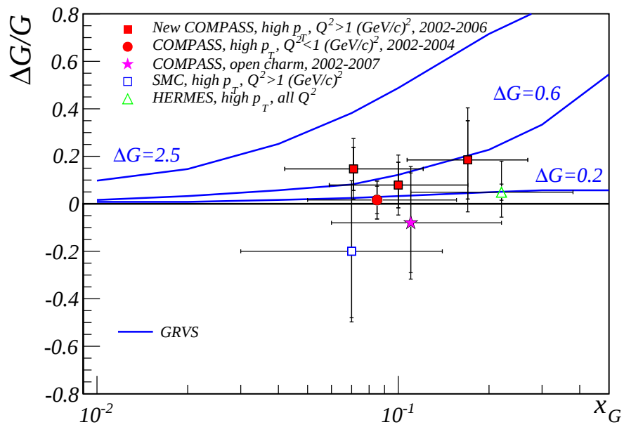
Figure 12.3: \Delta G/G Results from COMPASS [99], SMC [102] and HERMES [101]. Also shown are the QCD fits curves from the GRVS [103] group assuming three different values for \Delta G .
