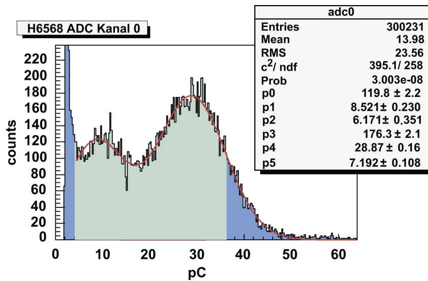
Figure 5.11: Typical single photoelectron response measured at 970 V using 360 nm photons. The shaded area shows the \pm 1\sigma region of each of the two contributing peaks.
