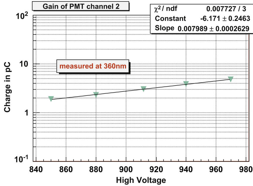
Figure 5.12: Gain values measured at 360 nm wavelength for a channel of a MAPMT. The curve is the exponentially fitted function.
