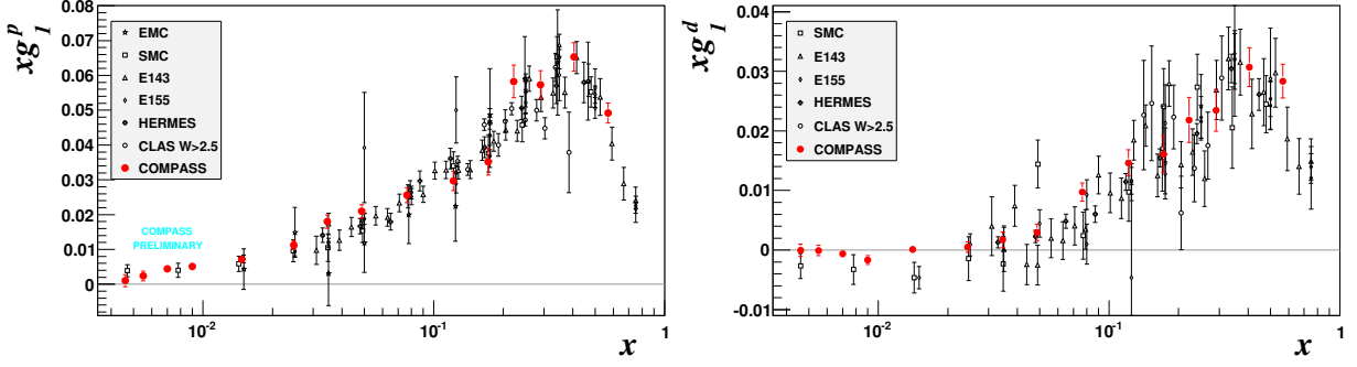
Figure 2.3: Spin dependent structure function g_1 for proton (left) and deuteron (right) data.
