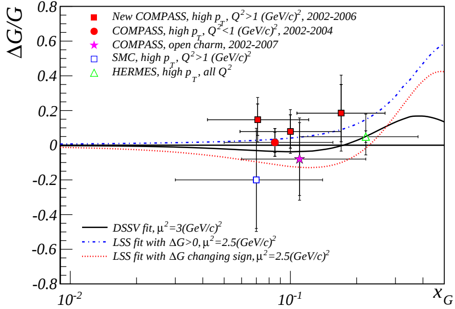
Figure 12.2: \Delta G/G Results from COMPASS [99], SMC [102] and HERMES [101] experiments. Also shown are the QCD fits curves from the LSS [76] and the DSSV [27,77] groups.
