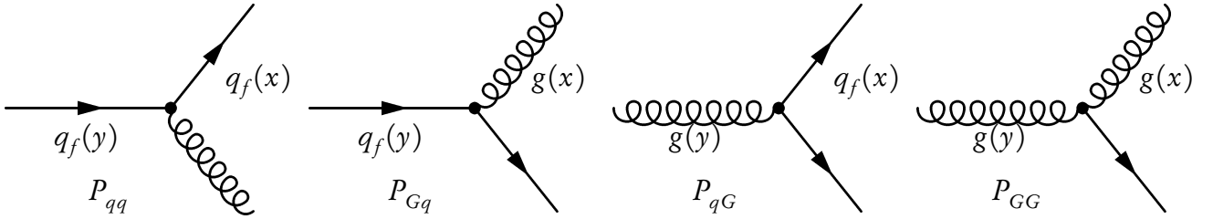
Figure 3.3: The Feynman diagrams for splitting functions.
