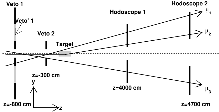
Figure 4.9: Schematic layout of the veto system. The tracks \mu_1 and \mu_3 are vetoed, whereas the track \mu_2 fulfils the inclusive trigger condition.
