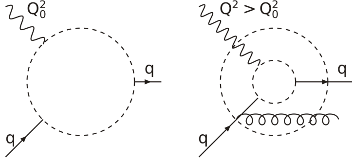
Figure 3.2: In a lepton-nucleon scattering, increasing Q^2 reveals the gluon radiation which explains the small violation in the Bjorken Scaling.
