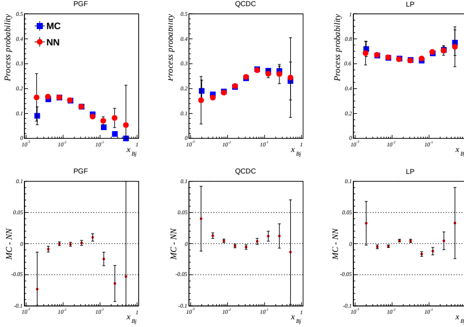
Figure 11.6: Neural network and MC comparison for R_{PGF} , R_{QCDC} and R_{LP} as functions of x_{Bj} . The average of the probability given by the MC (blue squares) and the neural network (red circles) in bins of x_{Bj} for the three processes is shown in the top row. The differences between the MC and the neural network probabilities are shown in the bottom row.
