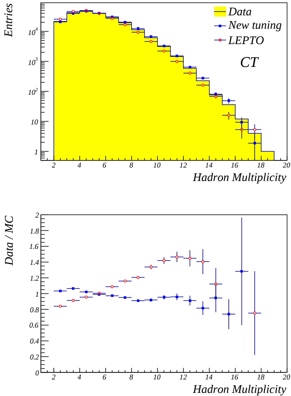
Figure 10.16: Comparison between data and MC simulation for Calorimetric triggers events: distributions (top) and also Data/MC ratios (bottom) of the hadron multiplicities for the leading and sub-leading hadrons.
