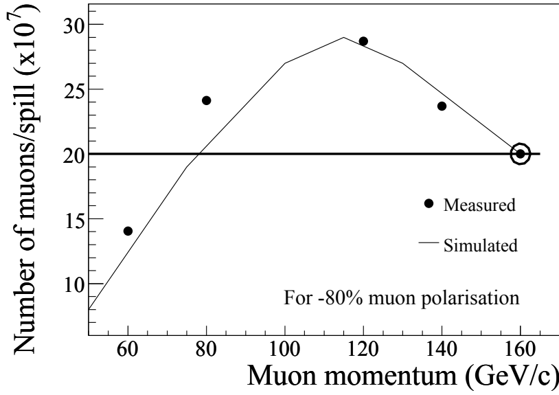
Figure 7.1: Polarisation and flux of the muon beam as a function of the muon momentum.
