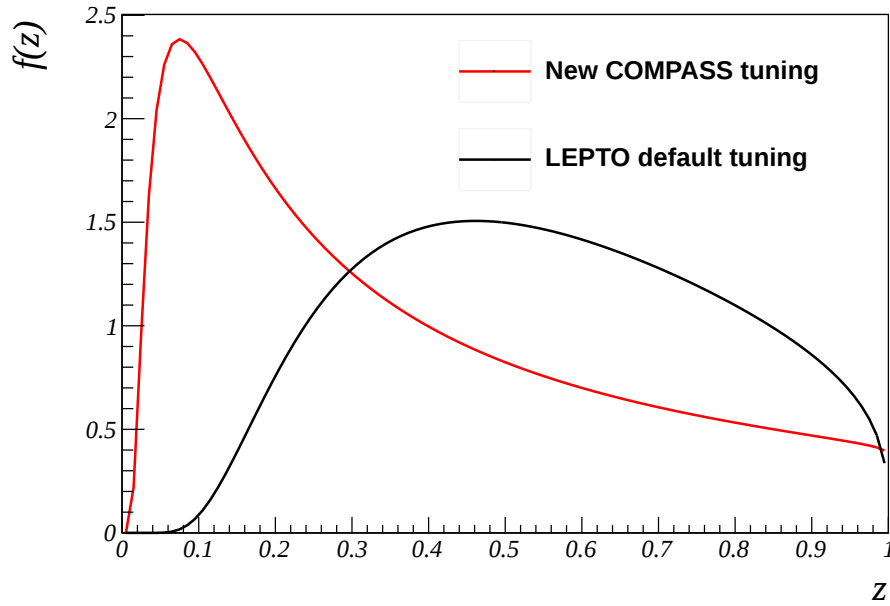
Figure 10.1: The Lund symmetric string fragmentation function is depicted for two different sets of a (PARJ(41)) and b (PARJ(42)), namely the LEPTO default set ( a = 0.3 and b = 0.58(\text{GeV})^{-2} ) and the new COMPASS tuning ( a = 0.025 and b = 0.075(\text{GeV})^{-2} ).
