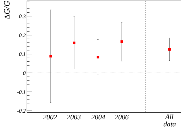
Figure 12.1: Gluon polarisation results per year and combined.
