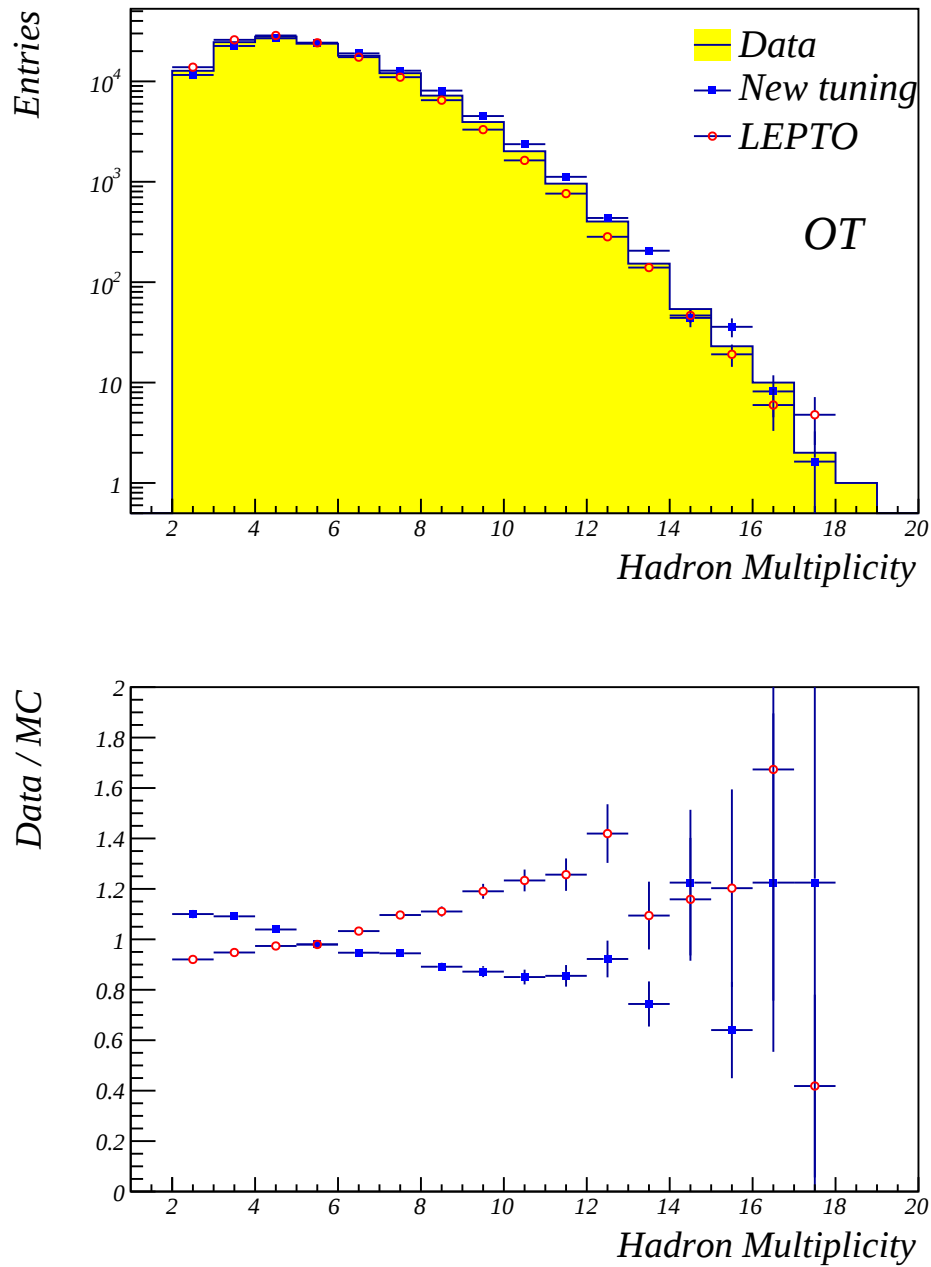
Figure 10.23: Comparison between data and MC simulation for Outer triggers events: distributions (top) and also Data/MC ratios (bottom) of the hadron multiplicities for the leading and sub-leading hadrons.
