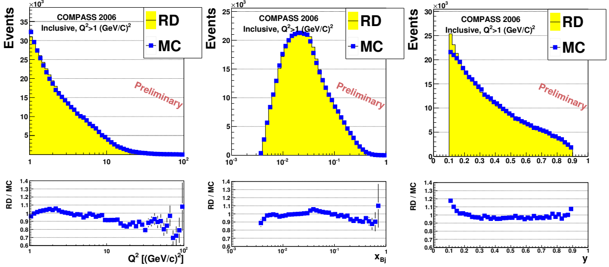
Figure 10.33: Comparison between data and MC simulation: On plots distributions (top) and ratios Data/MC (bottom) for the inclusive sample: Q^2 , x_{Bj} and y are shown.
