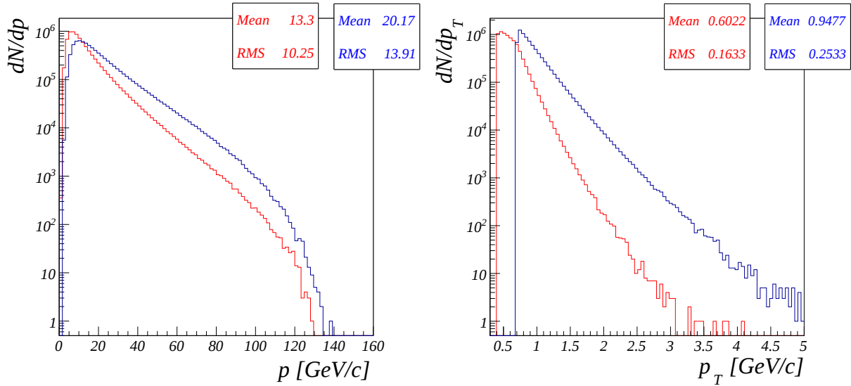
Figure 9.13: p and p_T distributions for leading (in blue) and sub-leading (in red) hadrons.
