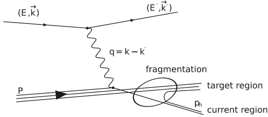
Figure 2.4: Schematic representation of the fragmentation process. The hadrons production in DIS.
