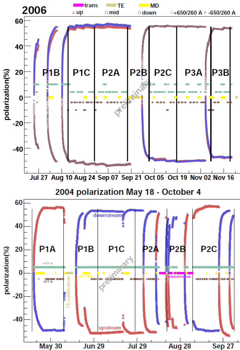
Figure 9.5: Target polarisation for 2006 (top) and for 2004 (bottom). These distributions are plotted against the data taking time period.
