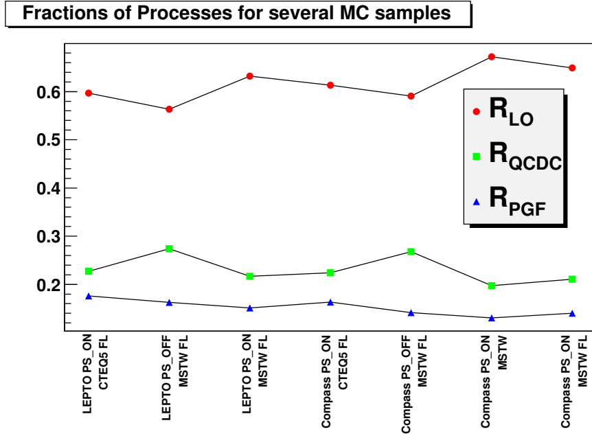
Figure 11.2: Fractions of processes, R , for several high p_T MC samples.
