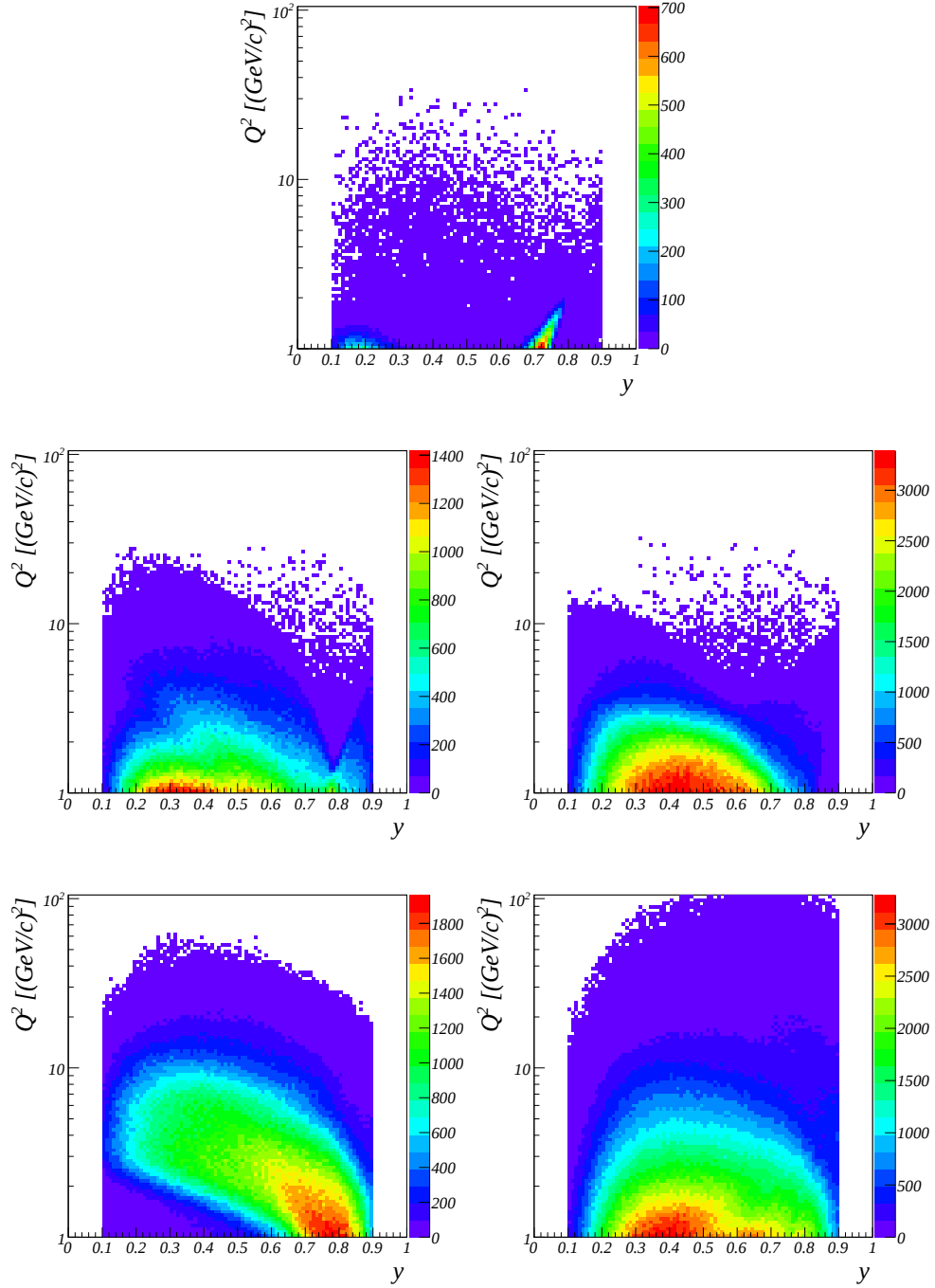
Figure 9.11: Q^2 vs y per trigger. Inner (top plot), Ladder (centre left plot), Middle (centre right plot), Outer (bottom left plot) and Calorimetric (bottom right plot) triggers.
