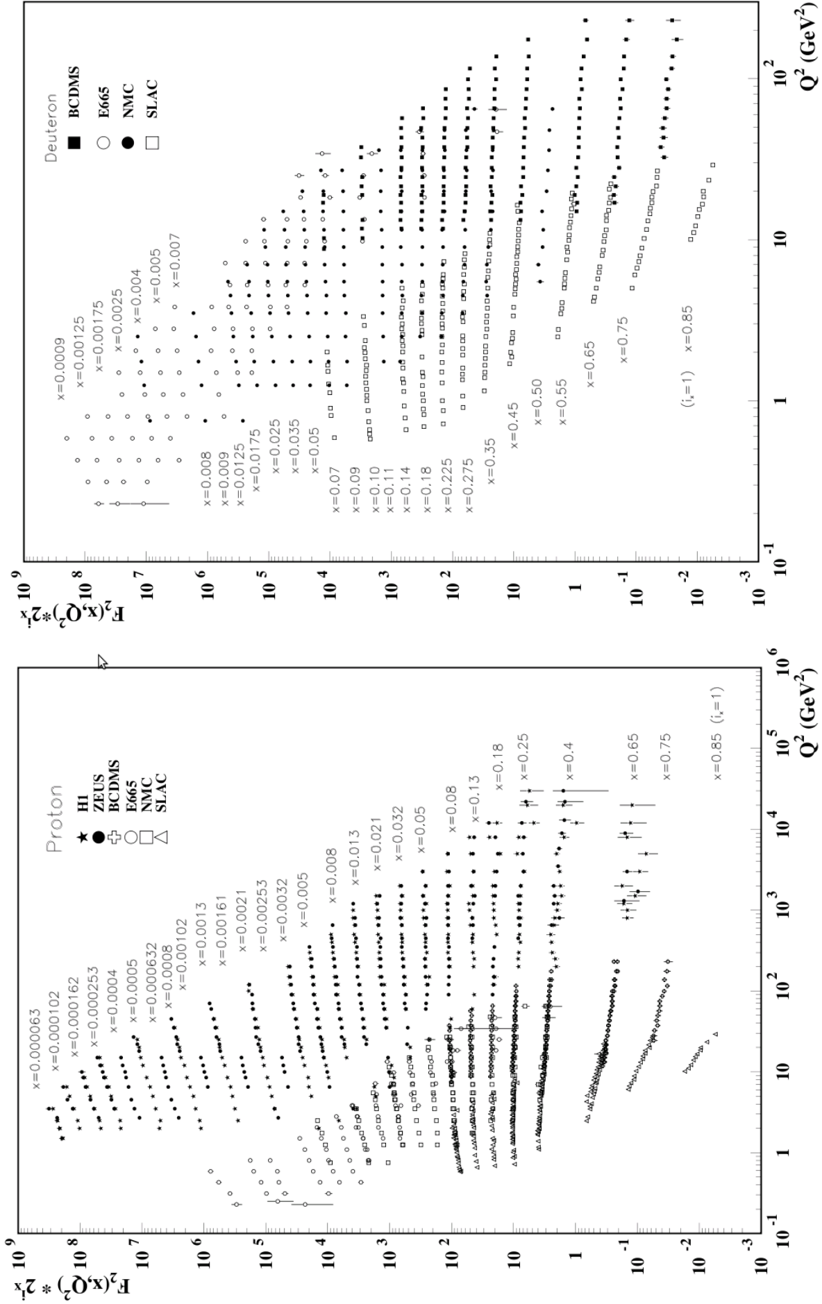
Figure 3.1: Spin in dependent structure function F_2 , for proton (left) and deuteron (right) data.
