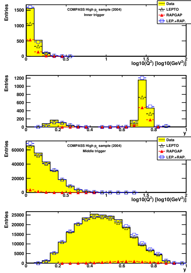
Figure 11.9: Q^2 and \gamma distributions for LEPTO LO and RAPGAP resolved photon simulations compared to the experimental data. The RAPGAP simulations are performed with the photon PDFs of Ref. [98] and with the scale \mu^2 = m^2 + p_T^2 . The MC distributions are normalised to the fraction obtained from a 2D fit to the data (see text for details). The results are presented for two samples: a) Inner Trigger and b) Middle Trigger. The green circles represent the sum of LEPTO and RAPGAP distributions.
