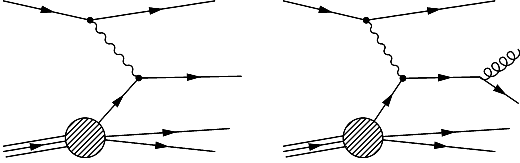
Figure 3.7: Virtual photo-absorption (left) and gluon radiation – QCD Compton (right) processes.
