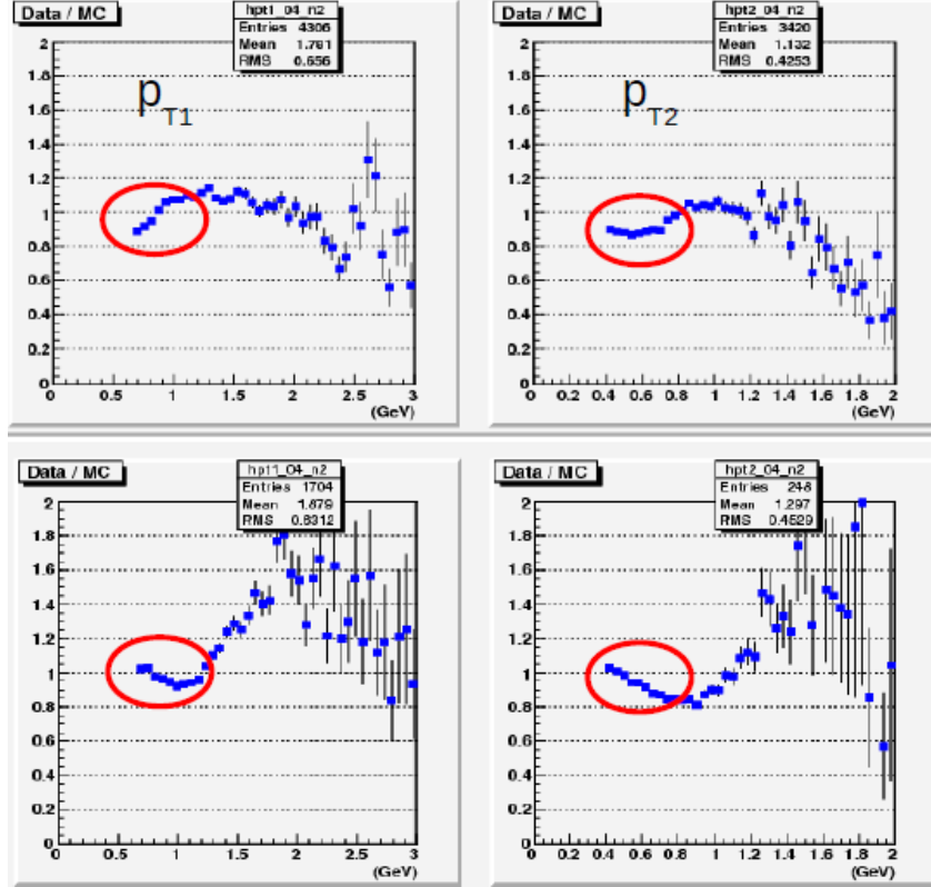
Figure 10.2: Transverse momentum distributions for the leading and sub-leading hadrons. The top plots show the distributions for the case PARJ(21) = 0.30 \text{ GeV}/c . The bottom plots show the same distributions for the case PARJ(21) = 0.42 \text{ GeV}/c . The region of interest is enclosed by the red ellipse. See text for details.
