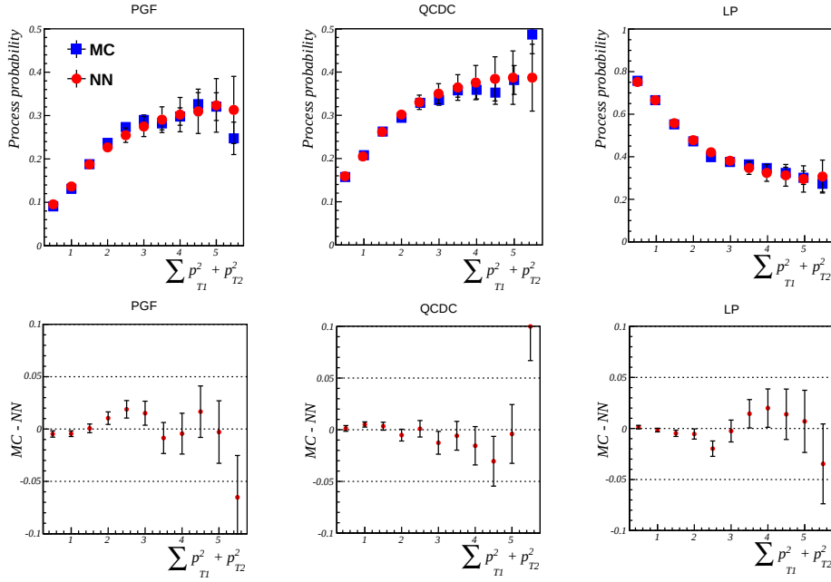
Figure 11.7: Neural network and MC comparison for R_{PGF} , R_{QCDC} and R_{LP} as functions of \sum p_T^2 . The average of the probability given by the MC (blue squares) and the neural network (red circles) in bins of \sum p_T^2 for the three processes is shown in the top row. The differences between the MC and the neural network probabilities are shown in the bottom row.
