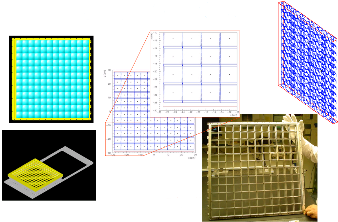
Figure 5.3: Technical drawing of the grid panel which supports the 144 lenses with (left top figure) and without the lenses (left bottom figure). Implementation in the detector MC simulation of the grid panel (centre and top right figure). Picture of a machined grid panel (right bottom figure).
