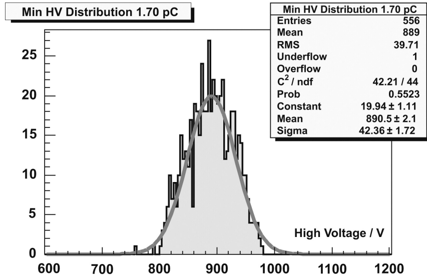
Figure 5.13: Distribution of the high voltage value needed to get a minimum output charge of 1.7 pC for a sample of 556 MAPMTs.
