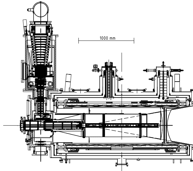
Figure 4.7: Side view of the 2006 COMPASS polarised target.
