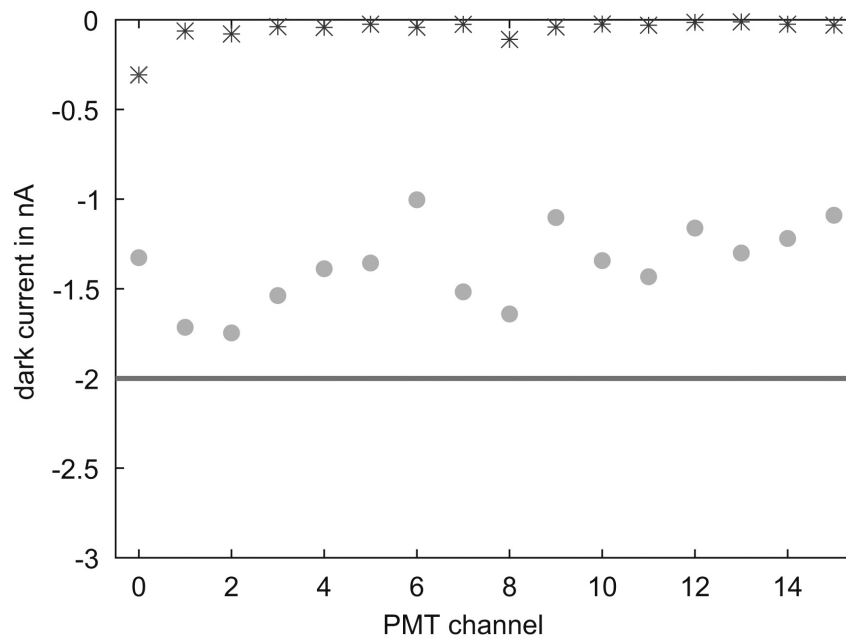
Figure 5.10: Dark current values for the 16 channels of a MAPMT before (circles) and after (stars) the measurement procedure. The line marks the specification limit.
