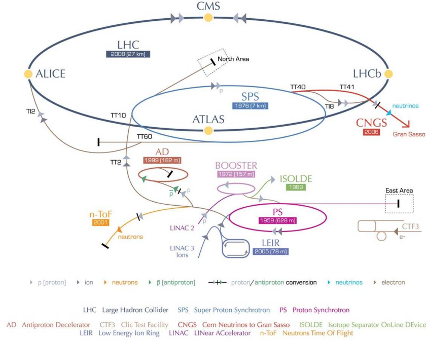
Figure 4.2: Schematic drawing of the CERN accelerator complex.
