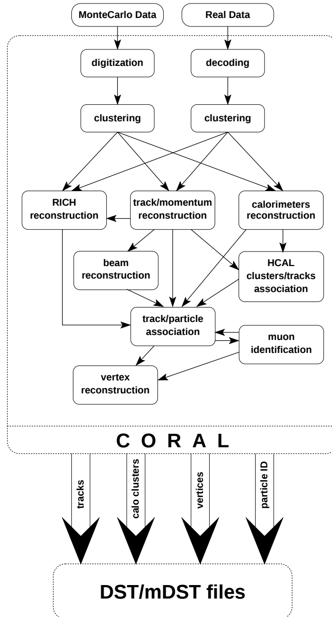
Figure 9.6: Schematic representation of the COMPASS reconstruction software.
