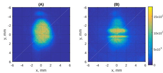
Fig 2. Schlieren images obtained with the ionizing laser beam (A) and without out it (B)
