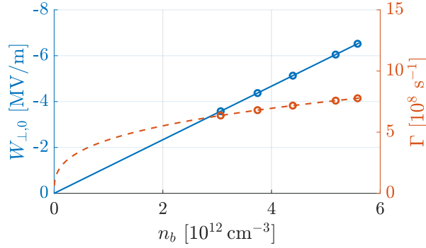
Figure 1.8: Transverse seed wakefield amplitude W_{\perp,0} at r = \sigma_r (Equation 1.11, blue solid line) and growth rate \Gamma at z = 0 and \xi - \xi_{Seed} = \lambda_{pe} (Equation 1.9, red dashed line) as a function of initial bunch density at the seed position. Values for the initial bunch densities used in the experiment later are marked with circles. Here, n_{pe} = 0.92 \cdot 10^{14} \text{ cm}^{-3} .
