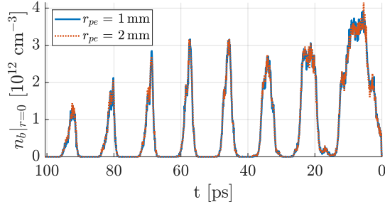
Figure A.31: Longitudinal on-axis charge density profile of the self-modulated proton bunch profile at the position of the OTR screen with plasma radius r_{pe} = 1 \text{ mm} (blue solid line) and r_{pe} = 2 \text{ mm} (red dotted line) from simulations with parameters of Table 4.4.
