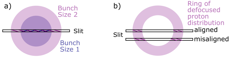
Figure 3.1: Schematic of the light collection through the streak camera slit for a) two different bunch sizes; b) a misaligned bunch
