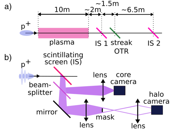
Figure 2.10: Schematic setup of the fluorescent screens for acquisition of the time-integrated transverse proton bunch distribution; a) shows the location of the screens after the plasma, b) the division of the light onto a core camera and a halo camera, where the light of the core is blocked by a mask; from [14].
