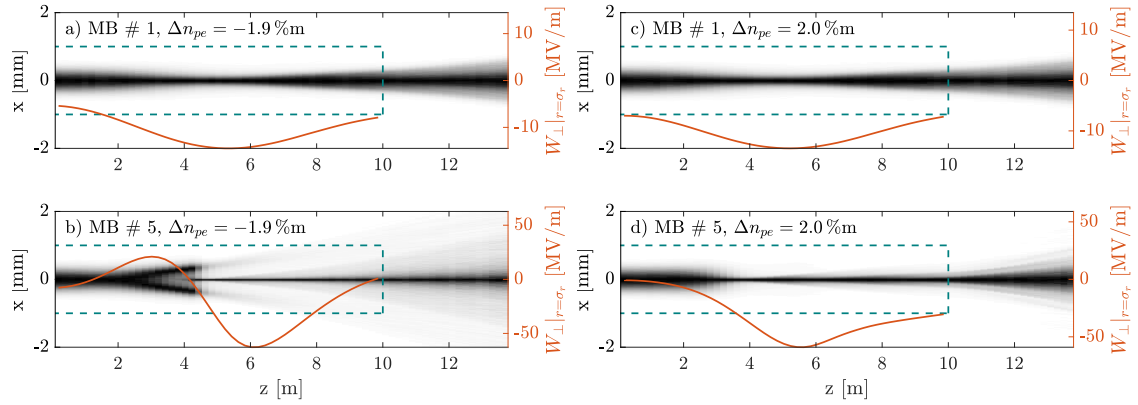
Figure 5.18: Micro-bunch evolution for a plasma density gradient of \Delta n_{pe} = -1.9\%/m (a, b) and \Delta n_{pe} = 2.0\%/m (c, d), for the first (a, c) and fifth (b, d) micro-bunch (location \xi determined in Section A.4). The 2D plots show the transverse profile of the charge density, normalized to 1 for each position z . The red curves show the transverse wakefield at r = \sigma_{r,0} = 200 \mu m along z . The plasma edge is marked with the blue dashed lines.
