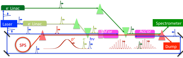
Figure 5: AWAKE setup planned for future measurements.
