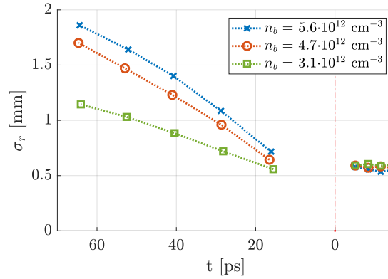
Figure 6.4: The rms width of defocused proton distributions along the bunch in experiment with initial bunch density n_b = 5.6 \cdot 10^{12} \text{ cm}^{-3} (blue crosses), n_b = 4.7 \cdot 10^{12} \text{ cm}^{-3} (red circles) and n_b = 3.1 \cdot 10^{12} \text{ cm}^{-3} (green squares). RIF at t = 0 ; points at t < 0 correspond to rms bunch size from the unmodulated bunch head. Here, n_{pe} = 0.92 \cdot 10^{14} \text{ cm}^{-3} and \Delta n_{pe} = 0 .
