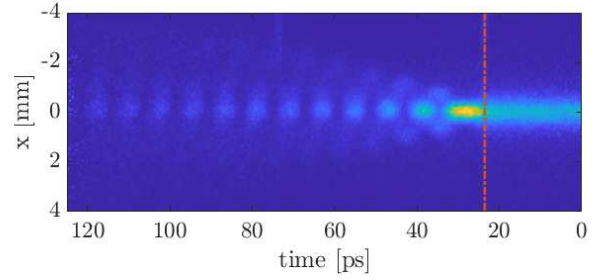
Figure 5. Stacked streak camera image of the proton bunch with plasma. The red line shows the location of the ionizing laser pulse ( t = 24 ps). The head of the bunch ( t < 24 ps) propagated through vapor. The tail ( t > 24 ps) propagated through plasma and is self-modulated.
