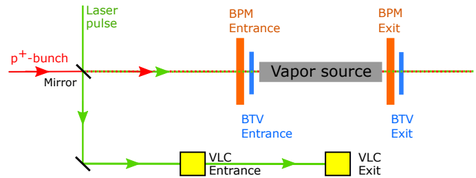
Figure 2.5: Experimental setup with devices used for the alignment of the laser pulse (green line) onto the proton bunch trajectory (red line).
