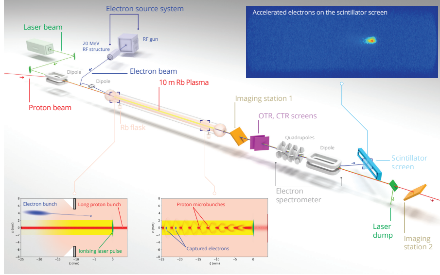
Figure 2.3: Schematic layout of the AWAKE experiment (not to scale): The Rb vapor is ionized by a laser pulse (green line), the proton bunch (red line) self-modulates in the plasma (right inset) and the train of micro-bunches resonantly drive the wakefield. The SM is seeded with the co-moving RIF (left inset). An externally injected electron bunch (blue line) is accelerated in the wakefield. Diagnostics for the self-modulated proton bunch (OTR, CTR screens, imaging stations 1, 2) and for the electron bunch (electron spectrometer) are located after the plasma.
