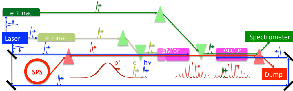
Figure 2.20: Schematic of the AWAKE Run 2 experimental setup from [43]: Plasma is divided into self-modulator (“SM’or”) and accelerator (“Acc’or”); In the self-modulator the SM is seeded with a preceding electron bunch in pre-formed plasma.
