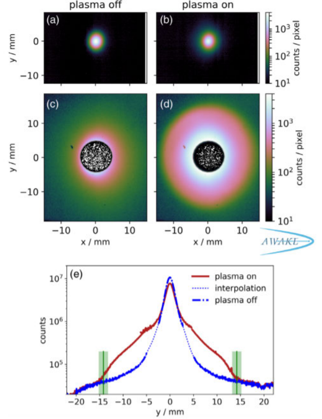
Figure 4: Time integrated transverse proton bunch density distribution acquired with fluorescent screens for the measurement of defocused protons and transverse wakefields' amplitude determination (from [4]). Images a), b) show core images, c), d) halo images for the same events with a), c) plasma OFF and b), d), plasma ON. Image e) shows the reconstructions of the bunch profile from the two cameras, as well as the value determined for the halo radius (green lines) and its uncertainty (green shaded regions). These images were obtained at imaging station 2 ( \approx 10 \text{ m} from the plasma exit). Similar images were obtained at imaging station 1.
