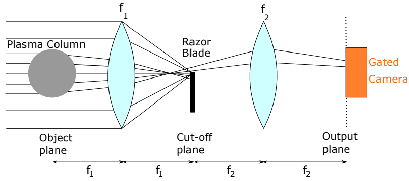
Figure A.3: Schematic of the setup for plasma radius determination with Schlieren imaging: A collimated beam propagates through the plasma column (coming out of the page), is focused and re-collimated by the lenses f_1 and f_2 and sent to a gated camera that images the plasma column. The razor blade in the focus of lens f_1 blocks rays that were not propagating through the plasma to increase the contrast of the image.
