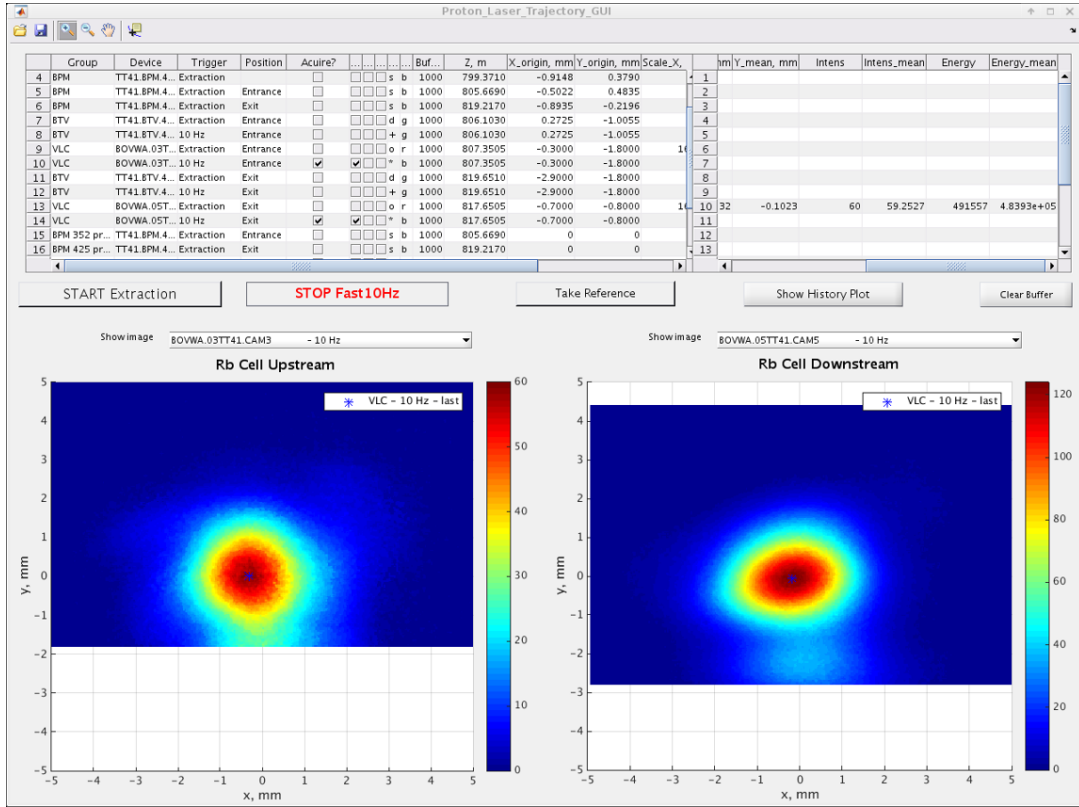
Figure A.1: MATLAB Laser Alignment GUI. Choice of diagnostics (BPMs, BTVs, VLCs) for acquisition and plotting (upper left section), diagnostic value of the previous acquisition from buffer (upper right section), trigger selection for acquisition (central left, 10 Hz trigger from the laser or extraction trigger from SPS). Bottom images show the acquisition for selected devices before (left image) or after (right image) the plasma. Acquisition of selected devices, determination of their mean value, and shifting them to the origin of the plots on the bottom with the function “Take Reference” (center).
