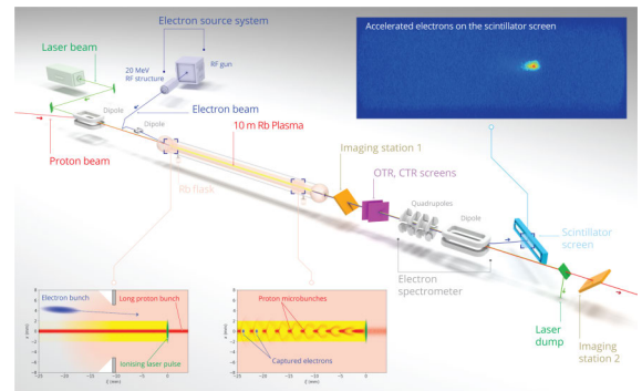
Figure 1: Layout of the AWAKE experiment [6].
