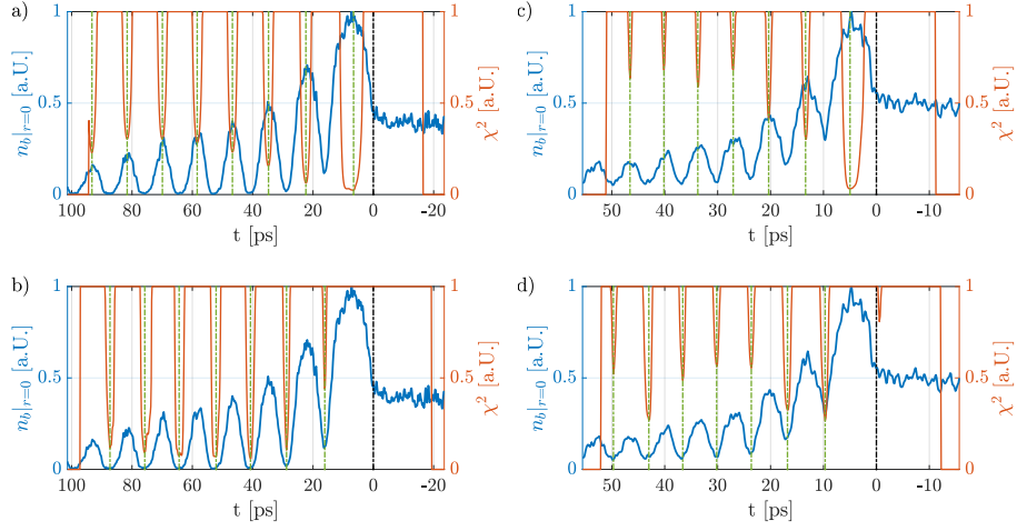
Figure A.14: Central bunch density n_b|_{r=0} modulation (projection of |x| \leq 0.1 mm from time-resolved images, blue lines), weighted distance squared function \chi^2 (cut for high values, red lines) using a parabola as polynomial fit to the data and its minima (green dashed-dotted lines), location of micro-bunches (a, c) and defocused proton regions (b, d) with plasma density n_{pe} = 0.92 \cdot 10^{14} \text{ cm}^{-3} (a, b) and n_{pe} = 2.9 \cdot 10^{14} \text{ cm}^{-3} (c, d) from experiment. Here, n_b = 5.6 \cdot 10^{12} \text{ cm}^{-3} and \Delta n_{pe} = 0 .
