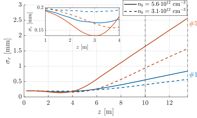
Figure 6.8: The rms width of defocused proton distributions \sigma_r as a function of propagation distance z (plasma z = 1 - 10 m, vacuum z = 10 - 13.5 m) with seed position n_b = 5.6 \cdot 10^{12} \text{ cm}^{-3} (solid lines) and n_b = 3.1 \cdot 10^{12} \text{ cm}^{-3} (dashed lines) at a fixed \xi of the first (blue lines) and fifth (red lines) period. Inset zooms in at z = 1 - 4 m. Here, n_{pe} = 0.92 \cdot 10^{14} \text{ cm}^{-3} and \Delta n_{pe} = 0 .
