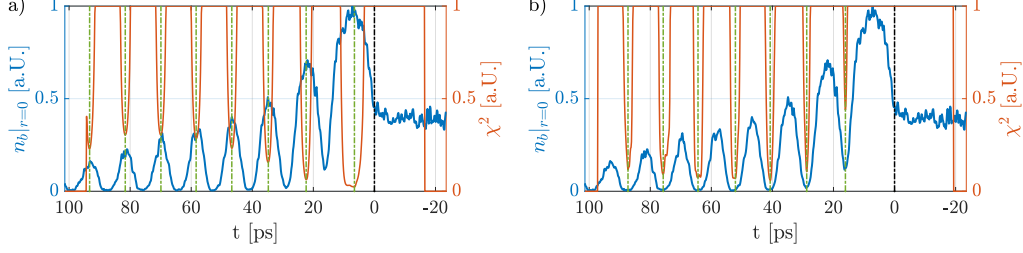
Figure 3.14: Central bunch density modulation ( n_b|_{r=0} , projection of |x| \leq 0.11 mm, blue lines), weighted distance squared function \chi^2 (cut for high values, red lines) using a parabola as polynomial fit to the data and its minima (green dashed-dotted lines), location of micro-bunches (a) and defocused proton regions (b).
