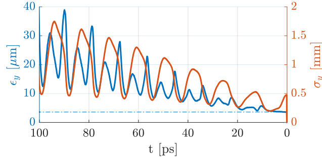
Figure A.30: The rms width \sigma_y (red solid line) and normalized slice emittance \epsilon_y (blue solid line) along the bunch axis t from the simulation (parameters Table 4.4, except n_{pe} = 1.0 \cdot 10^{14} \text{ cm}^{-3} ) after 10 m of plasma with an incoming normalized bunch emittance 3.6 \mu\text{m} (blue dash-dotted line).
