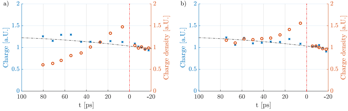
Figure 5.20: Integrated charge density ( \sum n_{b,i} , red circles), integrated charge ( \sum n_{b,i} x_i , blue crosses) and longitudinal incoming bunch charge (density) profile (Gaussian, black dash-dotted line) with plasma density gradient \Delta n_{pe} = -1.9\%/m (a) and \Delta n_{pe} = 2.0\%/m (b). Here, n_{pe,Entr.} = 1.8 \cdot 10^{14} \text{ cm}^{-3} , n_b = 5.6 \cdot 10^{12} \text{ cm}^{-3} , \sigma_\xi = 6.6 \text{ cm} , i.e. \sigma_t = 230 \text{ ps} and \xi_{Seed} = 0.6 \sigma_\xi .
