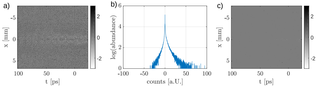
Figure 3.11: a) Difference between original and median filtered image; b) Abundance of the value in count difference from image a); c) Difference between original and filtered image, applying a median filter to selected pixels with abundance \leq 3 in b).
