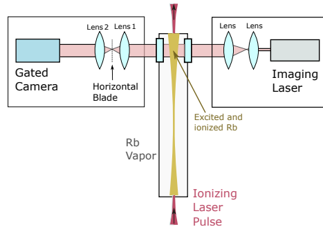
Fig 1. Setup for Schlieren Imaging of a column of excited and ionized rubidium vapor
