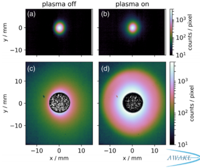
Figure 2.11: Time-integrated transverse proton bunch distribution at imaging station 2, acquired with the core camera (a, b) and with the halo camera (c, d), without plasma (a, c) and with plasma (b, d), from [14].
