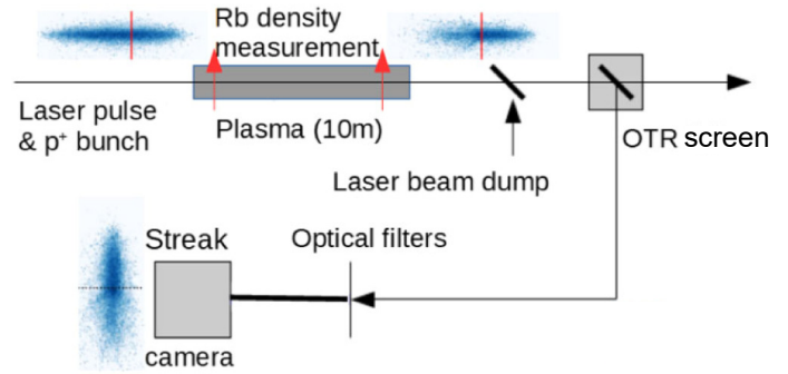
Figure 2.13: Schematic setup of acquisition of time-resolved transverse proton bunch distribution, imaging the OTR screen onto a streak camera, from [13].
