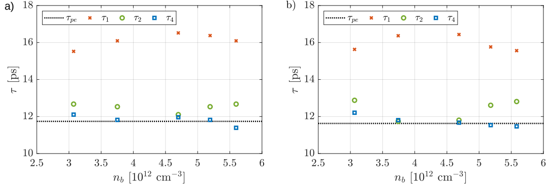
Figure 5.3: Length \tau of the first (red crosses), second (green circles) and fourth (blue squares) modulation period as a function of initial bunch density, obtained from experiment (a) and simulations (b, parameters in Table 4.4). The black dotted line shows the plasma period ( \tau_{pe} = 11.6 \text{ ps} , as n_{pe} = 0.92 \cdot 10^{14} \text{ cm}^{-3} ).
