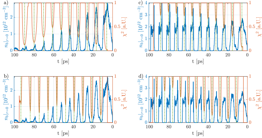
Figure A.17: Central bunch density n_b|_{r=0} modulation (projection of |x| \leq 0.1 mm from time-resolved images, blue lines), weighted distance squared function \chi^2 (cut for high values, red lines) using a parabola as polynomial fit to the data and its minima (green dashed-dotted lines), location of micro-bunches (a, c) and defocused proton regions (b, d) with plasma density gradient \Delta n = -1.9\%/m (a, b) and \Delta n = 2.0\%/m (c, d) from simulations. Here, n_{pe,Entr.} = 1.8 \cdot 10^{14} \text{ cm}^{-3} and n_b = 5.4 \cdot 10^{12} \text{ cm}^{-3} .
