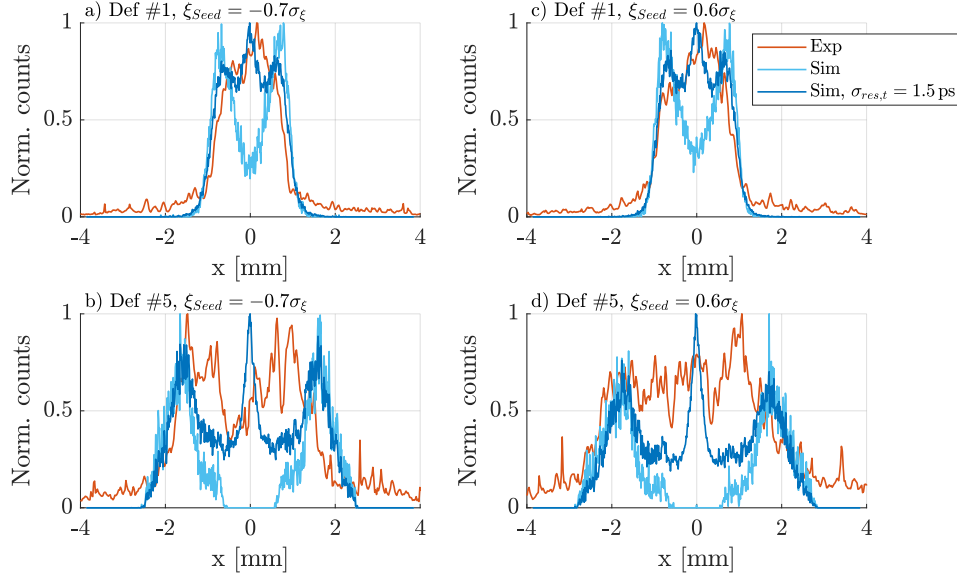
Figure A.34: Transverse profiles of defocused proton distributions from experiment (red lines) and simulations without (bright blue lines) and with (dark blue lines) \sigma_{res,t} = 1.5 ps Gaussian temporal resolution convolution; (a, b) with seed position \xi_{Seed} = -0.7\sigma_\xi , n_b = 3.9 \cdot 10^{12} \text{ cm}^{-3} and (c, d) with \xi_{Seed} = 0.6\sigma_\xi , n_b = 4.1 \cdot 10^{12} \text{ cm}^{-3} (a, c) of the first period, (b, d) of the fifth period. Here, n_{pe} = 2.0 \cdot 10^{14} \text{ cm}^{-3} and \Delta n_{pe} = 0 .
