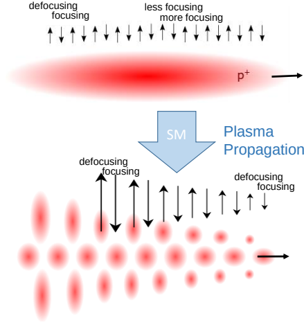
Figure 1.2: Schematic of the self-modulation instability: The transverse wakefield of focusing and defocusing (or less focusing) phase, driven by the initially long charged particle bunch in plasma acts back on the driver, transforming the long bunch into a train of micro-bunches.
