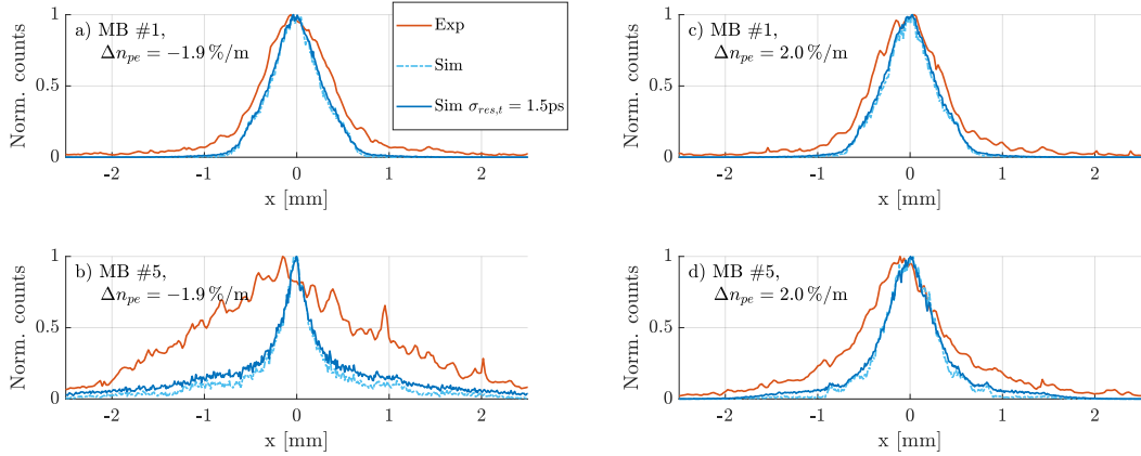
Figure 5.19: Normalized transverse charge density profiles for a plasma density gradient \Delta n_{pe} = -1.9\%/m (a, b) and \Delta n_{pe} = 2.0\%/m (c, d) for the first (a, c) and fifth (b, d) micro-bunch. Profiles from the simulation (bright blue dashed lines), their convolution with temporal resolution \sigma_{res,t} = 1.5 ps (dark blue solid lines) and the experimental profiles (red solid lines). Here, n_{pe,Entr.} = 1.8 \cdot 10^{14} \text{ cm}^{-3} and n_b = 5.6 \cdot 10^{12} \text{ cm}^{-3} .
