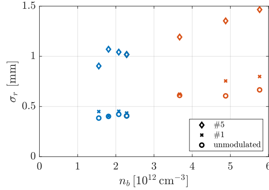
Figure A.29: The rms width \sigma_r of defocused proton distributions of the first (crosses) and fifth (diamonds) period and the unmodulated bunch head (circles) as a function of initial bunch density. Measurements with a bunch population of N_{p^+} = (0.9 \pm 0.1) \cdot 10^{11} , \sigma_\xi = 250 \text{ ps} and \xi_{Seed} = [-0.1, 0.4, 0.7, 0.9] \sigma_\xi (blue symbols) and with a bunch population of N_{p^+} = (2.8 \pm 0.2) \cdot 10^{11} , \sigma_\xi = 300 \text{ ps} and \xi_{Seed} = [0.1, 0.6, 1.0] \sigma_\xi (red symbols). Here, n_{pe} = 2.0 \cdot 10^{14} \text{ cm}^{-3} and \Delta n_{pe} = 0 .
