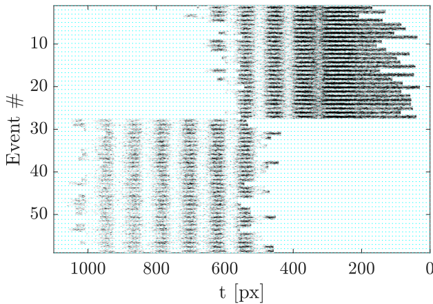
Figure 3.9: Central bunch modulation ( 320 \text{ px} < x < 400 \text{ px} ) of 59 proton bunch images. Events #1 – 27 cover the RIF (at t \approx 200 \text{ px} ), events #28 – 59 are acquired with a 50 ps delay of camera trigger and reference laser pulse.
