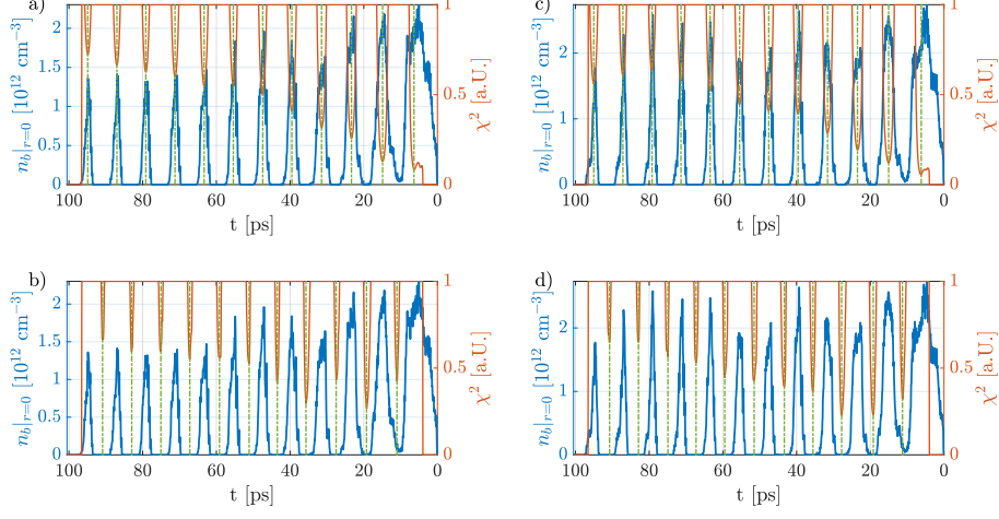
Figure A.20: Central bunch density n_b|_{r=0} modulation (projection of |x| \leq 0.1 mm from time-resolved images, blue lines), weighted distance squared function \chi^2 (cut for high values, red lines) using a parabola as polynomial fit to the data and its minima (green dashed-dotted lines), location of micro-bunches (a, c) and defocused proton regions (b, d) with seed position \xi_{Seed} = -0.7 \sigma_\xi ( n_b = 3.9 \cdot 10^{12} \text{ cm}^{-3} , Figures a, b) and \xi_{Seed} = 0.6 \sigma_\xi ( n_b = 4.1 \cdot 10^{12} \text{ cm}^{-3} , Figures c, d) from simulations. Here, n_{pe} = 2.0 \cdot 10^{14} \text{ cm}^{-3} and \Delta n_{pe} = 0 .
