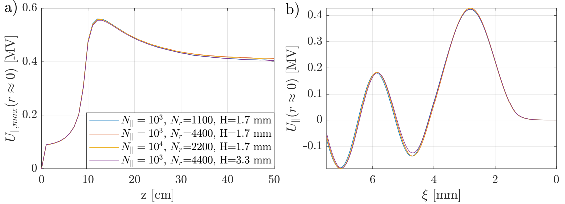
Figure 7.10: Validity tests of OSIRIS simulations increasing the resolution (transverse by a factor of 4, red lines, longitudinal by a factor of 10, yellow lines) or transverse box size (by a factor of 2, violet lines) of the baseline simulation (blue lines); a) maximum longitudinal wakefield potential along the first z = 50 \text{ cm} of plasma; b) longitudinal wakefield potential along the bunch after z = 30 \text{ cm} of plasma.
