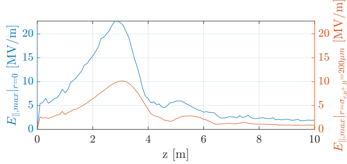
Figure 7.12: Maximum longitudinal wakefield along the bunch E_{\parallel,max} versus distance in plasma z , at radial position r \approx 0 (blue curve) and r = \sigma_{r,0,p^+} = 200 \mu\text{m} (red curve).
