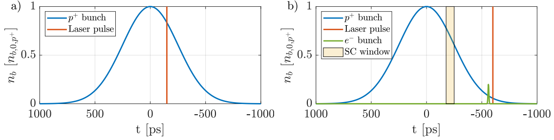
Figure 7.1: Schematic of seeding SM with a) a RIF (red line) close to bunch center or b) a relativistic electron bunch (green curve) ahead of the proton bunch (blue curve) in a pre-performed plasma.
