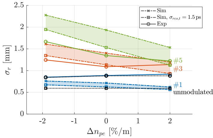
Figure 6.18: The rms width of defocused proton distributions from experiment (circles) and simulations without (crosses) and with (squares) \sigma_{res,t} = 1.5 ps resolution convolution as a function of plasma density gradient \Delta n_{pe} of the first (blue symbols), third (red symbols) and fifth (green symbols) period and rms width of unmodulated bunch (black lines). Here, n_{pe,Entr.} = 1.8 \cdot 10^{14} \text{ cm}^{-3} and n_b = 5.6 \cdot 10^{12} \text{ cm}^{-3} .
