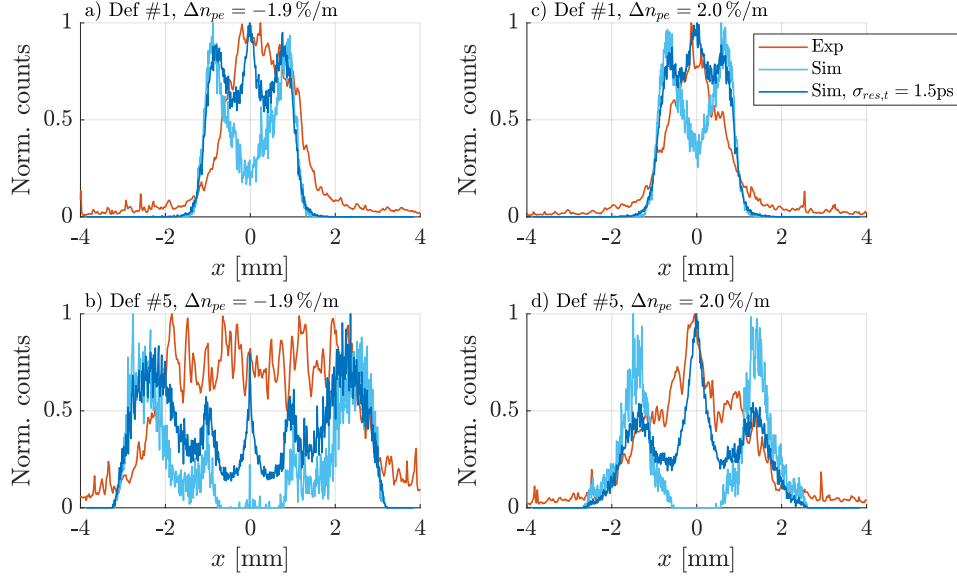
Figure 6.17: Transverse profiles of defocused proton distributions from experiment (red lines) and simulations without (bright blue lines) and with (dark blue lines) \sigma_{res,t} = 1.5 ps Gaussian temporal resolution convolution; with plasma density gradient \Delta n_{pe} = -1.9\%/m (a, b) and \Delta n_{pe} = 2.0\%/m (c, d), of the first period (a, c) and fifth period (b, d). Here, n_{pe,Entr.} = 1.8 \cdot 10^{14} \text{ cm}^{-3} and n_b = 5.6 \cdot 10^{12} \text{ cm}^{-3} .
