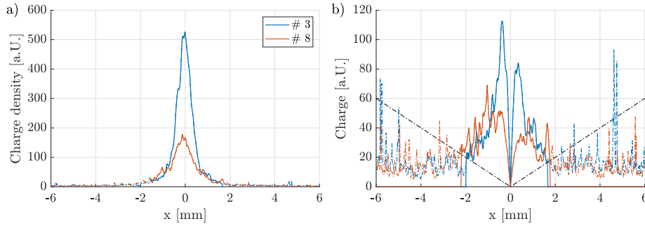
Figure 3.18: Transverse profiles of the charge density (a) and charge (b) of micro-bunch #3 (blue lines) and #8 (red lines) above (solid lines) and below (dashed lines) the noise threshold. Noise threshold for charge density 10 [a.u.], i.e. for charge 10 [a.u.] \cdot |x[\text{mm}]| (black dashed line in b).
