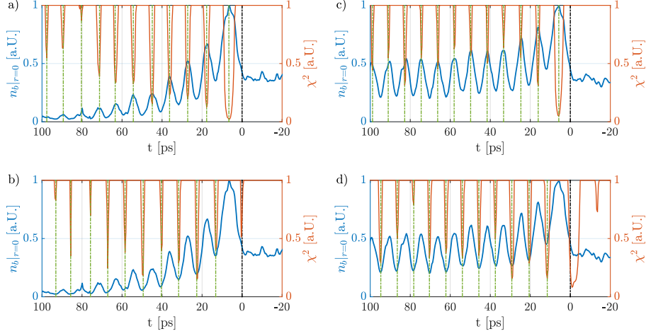
Figure A.16: Central bunch density n_b|_{r=0} modulation (projection of |x| \leq 0.1 mm from time-resolved images, blue lines), weighted distance squared function \chi^2 (cut for high values, red lines) using a parabola as polynomial fit to the data and its minima (green dashed-dotted lines), location of micro-bunches (a, c) and defocused proton regions (b, d) with plasma density gradient \Delta n = -1.9\%/m (a, b) and \Delta n = 2.0\%/m (c, d) from experiment. Here, n_{pe,Entr.} = 1.8 \cdot 10^{14} \text{ cm}^{-3} and n_b = 5.8 \cdot 10^{12} \text{ cm}^{-3} .
