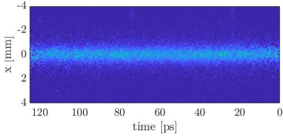
Figure 4. Stacked streak camera image of the proton bunch after propagation without plasma (bunch front at t = 0 ). The marker laser pulses used for stitching are at the top edge of the image. The bunch density is almost uniform along the bunch.
