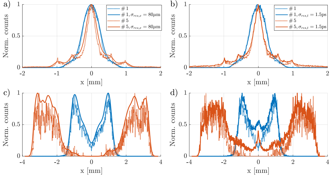
Figure 4.3: Transverse profiles of focused (a, b) and defocused (c, d) proton distributions of the first (blue lines) and fifth (red lines) period of time-resolved images after the plasma in simulations with parameters of Table 4.4. Figures a, c) show the results without (dotted lines) and with (solid lines) spatial \sigma_{res,x} = 80\mu\text{m} Gaussian convolution; Figures b, d) without (dotted lines) and with (solid lines) longitudinal \sigma_{res,t} = 1.5\text{ps} Gaussian convolution. All curves normalized to 1.
