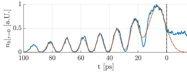
Figure 3.15: Central bunch density modulation n_b|_{r=0} (projection of |x| \leq 0.11 mm, blue solid line) with its peaks (micro-bunches) fitted with Gaussian functions (sum of the functions, red dash-dotted line) to determine their length.
