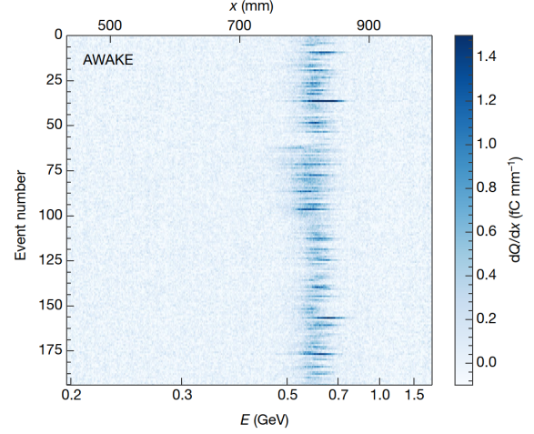
Figure 2.18: Waterfall plot of the electron energy distribution of more than 185 consecutive events, from [42].
