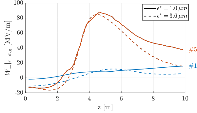
Figure A.27: Transverse wakefield at r = \sigma_{r,0} of defocused proton regions of the first (blue lines) and fifth (red lines) period as a function of distance in plasma z with normalized incoming bunch emittance \epsilon^* = 1.0 \mu\text{m} (solid lines) and \epsilon^* = 3.6 \mu\text{m} (dashed lines). Here, n_b = 5.6 \cdot 10^{12} \text{ cm}^{-3} , n_{pe} = 0.9 \cdot 10^{14} \text{ cm}^{-3} and \Delta n_{pe} = 0 .
