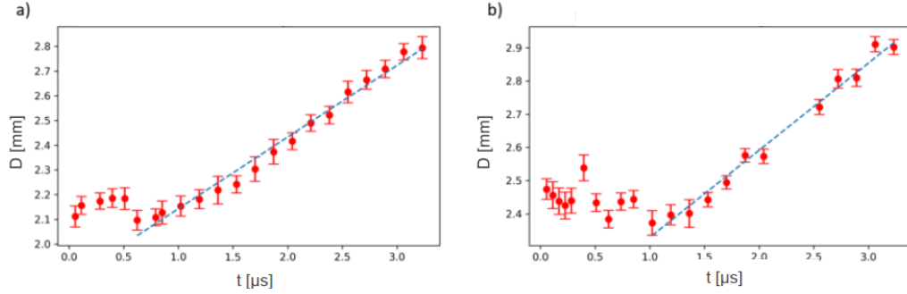
Figure 2.9: Time evolution of the plasma diameter D (error bars give the std divided by the square root of number of measurements) with imaging laser detuning frequencies of a) \Delta f = -16 GHz and b) \Delta f = 8 GHz), from [37].
