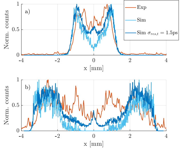
Figure 4.6: Transverse profile of defocused proton distributions of the first (a) and fifth (b) modulation period of the simulation without (bright blue curves), with (dark blue curves) \sigma_{res,t} = 1.5 ps Gaussian temporal resolution convolution and from the experiment (red curves). Projection with \Delta t = 1.5 ps centered at the location of defocused proton regions determined in Section A.4
