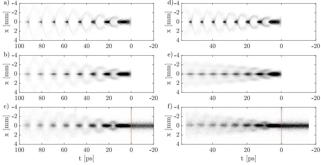
Figure 4.10: Time-resolved images of the bunch after the plasma with plasma density n_{pe} = 0.92 \cdot 10^{14} \text{ cm}^{-3} (a-c) and n_{pe} = 2.9 \cdot 10^{14} \text{ cm}^{-3} (d-f). Images (a, d) are simulation results without, (b, e) with \sigma_{res,t} = 1.5 \text{ ps} temporal resolution convolution and (c, f) the corresponding experimental images. Color scale saturated to 50 % of the maximum value. Here, n_b = 5.6 \cdot 10^{12} \text{ cm}^{-3} and \Delta n_{pe} = 0 .
