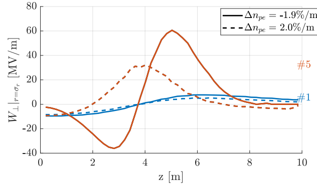
Figure 6.21: Transverse wakefield W_{\perp} evaluated at the rms width of the proton distributions of the first (blue lines) and fifth (red lines) period as a function of distance in plasma z with plasma density gradient \Delta n_{pe} = -1.9\%/m (solid lines) and \Delta n_{pe} = 2.0\%/m (dashed lines). Here, n_{pe,Entr.} = 1.8 \cdot 10^{14} \text{ cm}^{-3} and n_b = 5.6 \cdot 10^{12} \text{ cm}^{-3} .
