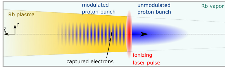
Figure 1.3: Seeding of the proton bunch self-modulation in AWAKE: The ionizing laser pulse co-propagates with the bunch, close to the bunch center, creating the relativistic ionization front at a high incoming bunch density.
