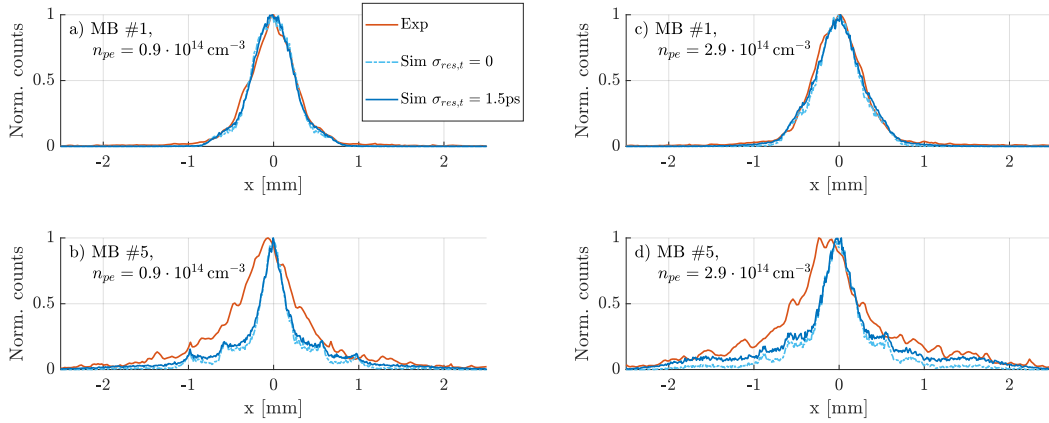
Figure 5.17: Normalized transverse charge density profiles with plasma density n_{pe} = 0.92 \cdot 10^{14} \text{ cm}^{-3} (a, b) and n_{pe} = 2.9 \cdot 10^{14} \text{ cm}^{-3} (c, d) for the first (a, c) and fifth (b, d) micro-bunch. Profiles from the simulation (bright blue dashed lines), their convolution with temporal resolution \sigma_{res,t} = 1.5 \text{ ps} (dark blue solid lines) and the experimental profiles (red solid lines). Here, n_b = 5.6 \cdot 10^{12} \text{ cm}^{-3} and \Delta n_{pe} = 0 .
