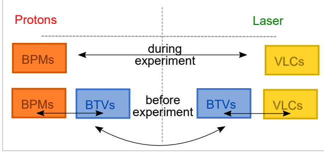
Figure 2.6: Diagnostics for proton bunch trajectory (BPMs and BTVs) and laser pulse trajectory (BTVs and VLCs); Correlation between the trajectories with BTVs.
