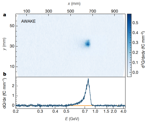
Figure 2.17: Spectrometer image (top figure) of an electron bunch accelerated to \sim 0.7 GeV and the energy projection with background subtraction (bottom figure), from [42].
