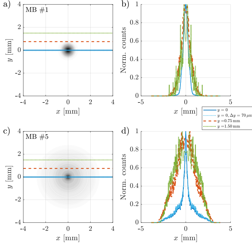
Figure A.23: Transverse charge density distributions of micro-bunches (a, c) and line outs (b, d) from images (a, c) along x at y = 0 (dark blue solid line), y = 0.75 \text{ mm} (red dashed line), y = 1.5 \text{ mm} (green dotted line) and average over the slit width of \Delta y = 70 \mu\text{m} at y = 0 (bright blue dotted line). Images correspond to the first (a, b) and fifth (c, d) period. Charge density distributions from the simulation with parameters of Table 4.7 with plasma density gradient \Delta n_{pe} = -1.9 \text{ \%}/\text{m} at the position of the OTR screen after \sigma_{res,t} = 1.5 \text{ ps} Gaussian temporal resolution convolution.
