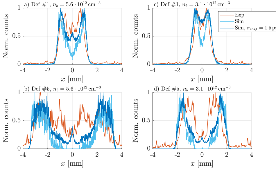
Figure 6.5: Transverse profiles of defocused proton distributions from experiment (red lines) and simulations without (bright blue lines) and with (dark blue lines) \sigma_{res,t} = 1.5 ps Gaussian temporal resolution convolution, with initial bunch density n_b = 5.6 \cdot 10^{12} \text{ cm}^{-3} (a, b) and n_b = 3.1 \cdot 10^{12} \text{ cm}^{-3} (c, d), of the first period (a, c) and fifth period (b, d). Here, n_{pe} = 0.92 \cdot 10^{14} \text{ cm}^{-3} and \Delta n_{pe} = 0 .
