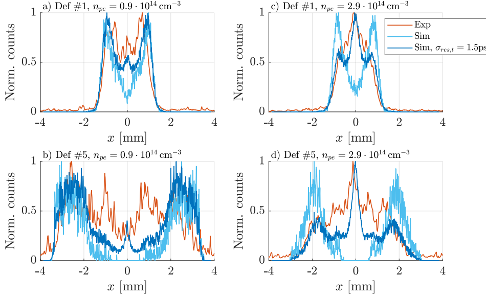
Figure 6.11: Transverse profiles of defocused proton distributions from experiment (red lines) and simulations without (bright blue lines) and with (dark blue lines) \sigma_{res,t} = 1.5 ps Gaussian temporal resolution convolution; with plasma density n_{pe} = 0.9 \cdot 10^{14} \text{ cm}^{-3} (a, b) and n_{pe} = 2.9 \cdot 10^{14} \text{ cm}^{-3} (c, d), of the first period (a, c) and fifth period (b, d). Here, n_b = 5.6 \cdot 10^{12} \text{ cm}^{-3} and \Delta n_{pe} = 0 .
