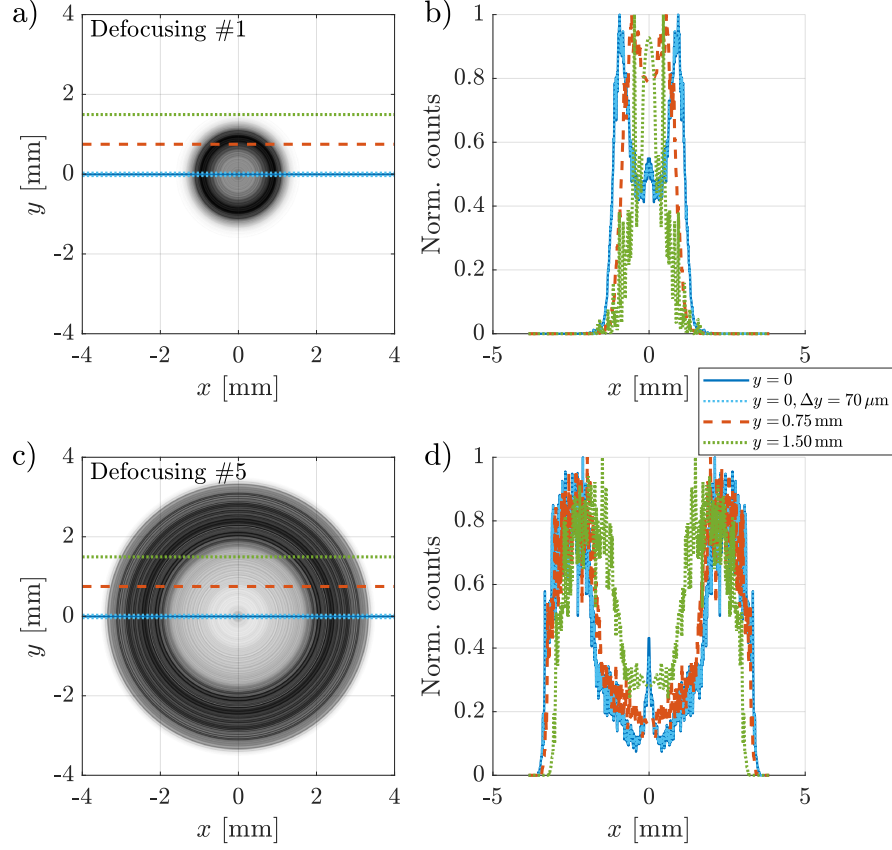
Figure A.22: Transverse charge density distributions of defocused proton regions (a, c) and line outs (b, d) from images (a, c) along x at y = 0 (dark blue solid line), y = 0.75\text{mm} (red dashed line), y = 1.5\text{mm} (green dotted line) and average over the slit width of \Delta y = 70\text{ }\mu\text{m} at y = 0 (bright blue dotted line). Images correspond to the first (a, b) and fifth (c, d) period. Charge density distributions from the simulation with parameters of Table 4.4 at the position of the OTR screen after \sigma_{res,t} = 1.5\text{ ps} Gaussian temporal resolution convolution.
