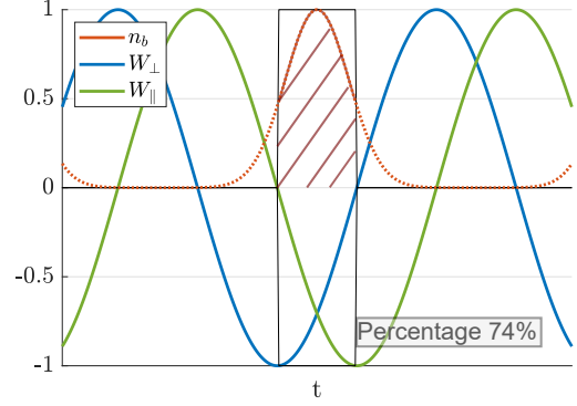
Figure 5.9: Schematic of a train of Gaussian micro-bunches ( n_b red line) in a linear wakefield approximated with cosine functions ( W_\perp blue line, negative for focusing, W_\parallel green line, negative for decelerating) with wakefield period \tau_{cos} . A micro-bunch length of \sigma_t = 0.1 \tau_{cos} results in 74 % of the charge in one quarter of the wakefield period \tau_{cos} .
