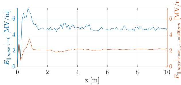
Figure 7.17: Maximum longitudinal wakefield along the bunch E_{||,max} versus distance in plasma z , at radial position r \approx 0 (blue curve) and r = 200 \mu\text{m} (red curve), driven by the 165 MeV electron bunch.
