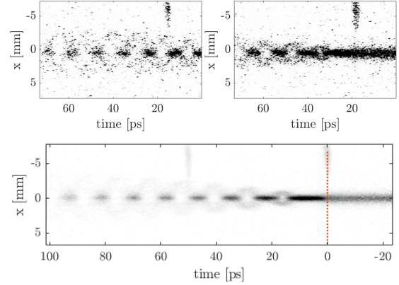
Figure 2: Single streak camera image of the start of the SM (top right), single streak camera image with a 50 ps time delay to the start of the SM (top left) and sets of the two time delays of 20 streak camera images each, stitched together using the timing reference signal (bottom).
