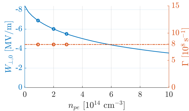
Figure 1.9: Transverse seed wakefield amplitudes W_{\perp,0} at r = \sigma_r (Equation 1.11, blue solid line) and growth rate \Gamma at z = 0 and \xi - \xi_{Seed} = \lambda_{pe} (Equation 1.9, red dashed line) as a function of plasma density. Values for the plasma densities used in the experiment later are marked with circles. Here, n_b = 5.6 \cdot 10^{12} \text{ cm}^{-3} .
