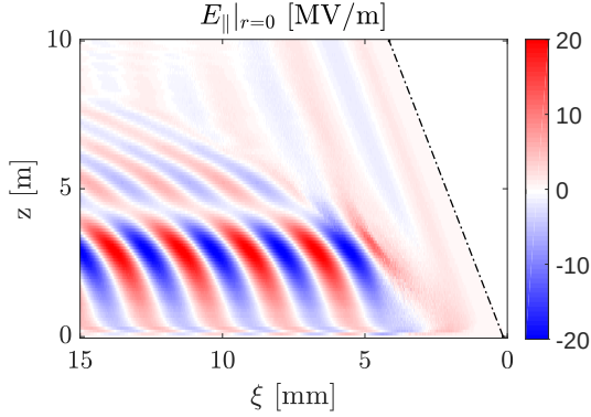
Figure 7.13: Longitudinal wakefield amplitude along the bunch \xi -axis and along the plasma z at r \approx 0 driven by 18 MeV electron bunch. Bunch dephases ( \gamma_0 = 35 , black dash-dotted line) with respect to the speed of light (velocity of the simulation window).
