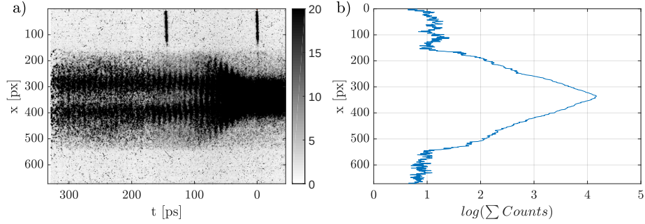
Figure 3.13: a) Stitched proton bunch image and b) its projection on logarithmic scale.
