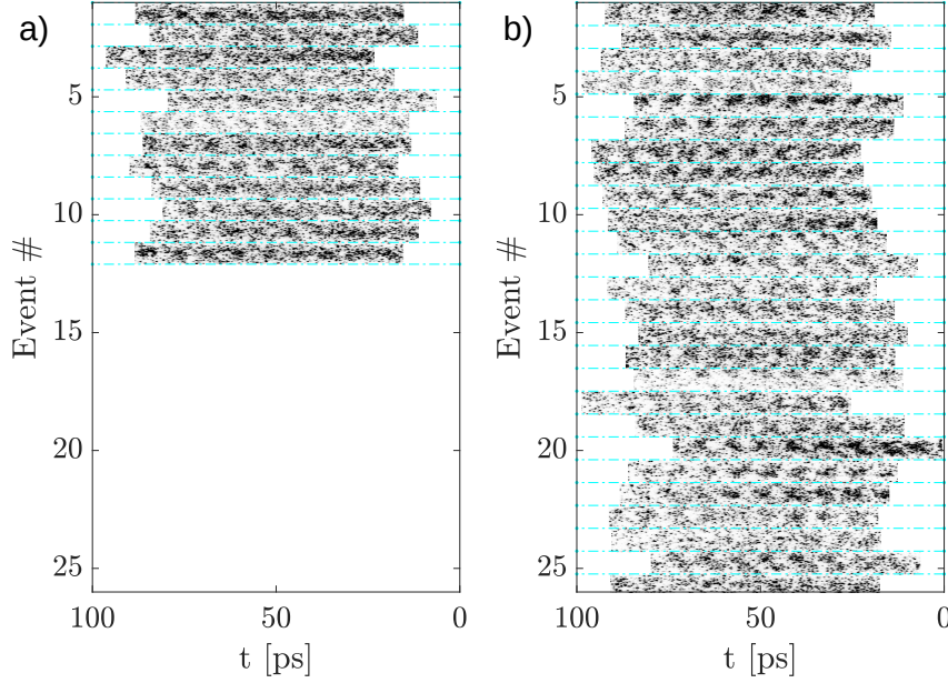
Figure 7.6: Waterfall plots of the central bunch density modulation using the region -0.8 \text{ mm} < x < 1.9 \text{ mm} from time-resolved images; a) without and b) with preceding electron bunch.
