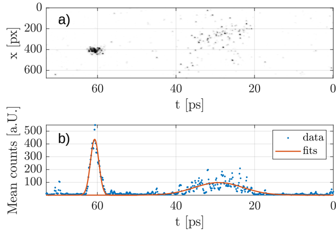
Figure 7.2: a) Streak camera image with electron bunch (at t \approx 30 ps) and low energy laser pulse (at t \approx 60 ps); b) Image projection (blue points), fitting a Gaussian function to each signal (red line).
