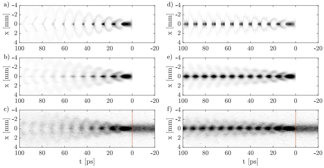
Figure 4.11: Time-resolved images of the bunch after the plasma with plasma density gradient \Delta n_{pe} = -1.9\%/m (a-c) and \Delta n_{pe} = 2.0\%/m (d-f). Images (a, d) are simulation results without, (b, e) with \sigma_{res,t} = 1.5 ps temporal resolution convolution and (c, f) the corresponding experimental images. Color scale saturated to 50 % of the maximum value. Here, the plasma entrance density is fixed to n_{pe,Entr.} = 1.8 \cdot 10^{14} \text{ cm}^{-3} and n_b = 5.6 \cdot 10^{12} \text{ cm}^{-3} .
