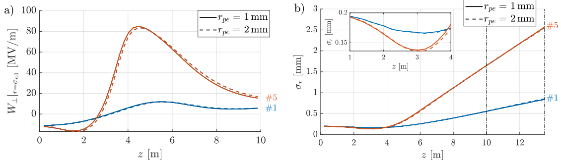
Figure A.32: a) Transverse wakefields at r = \sigma_{r,0} and b) rms width; both of defocused proton regions at a fixed \xi of the first (blue lines) and fifth (red lines) period as a function of propagation distance z (plasma z = 1 - 10 \text{ m} , vacuum z = 10 - 13.5 \text{ m} ) with plasma radius r_{pe} = 1 \text{ mm} (solid lines) and r_{pe} = 2 \text{ mm} (dashed lines) from simulations with parameters of Table 4.4. Inset in b) zooms in at z = 1 - 4 \text{ m} .
