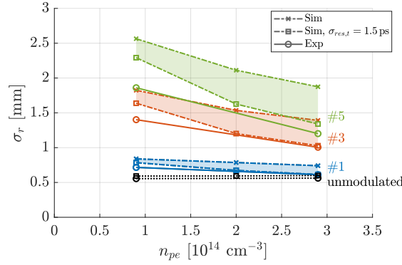
Figure 6.12: The rms width of defocused proton distributions from experiment (circles) and simulations without (crosses) and with (squares) \sigma_{res,t} = 1.5 ps resolution convolution as a function of plasma density n_{pe} of the first (blue symbols), third (red symbols) and fifth (green symbols) period and rms width of unmodulated bunch (black symbols). Here, n_b = 5.6 \cdot 10^{12} \text{ cm}^{-3} and \Delta n_{pe} = 0 .
