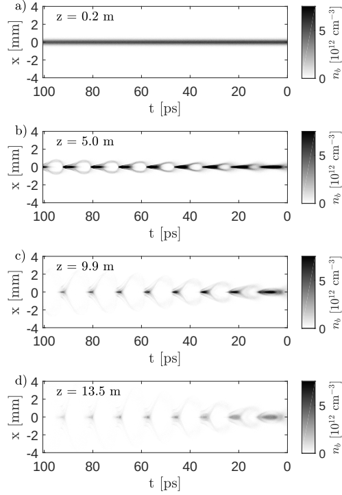
Figure 4.7: Time-resolved images of the proton bunch after 0.2 m, 5.0 m, 9.9 m of plasma (a-c) and subsequent 3.5 m of vacuum propagation after the 10 m of plasma (d) from simulation with parameters in Table 4.4.
