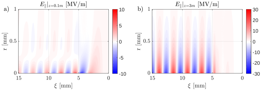
Figure 7.14: Radial extent of the longitudinal wakefield along the bunch \xi after a) 0.1 m and b) 3 m of plasma.
