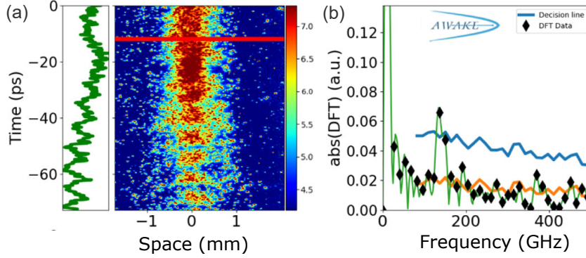
Figure 2.14: a) Streak camera image of the self-modulated proton bunch, propagating from bottom to top, ionizing laser position (red line) and projection of the central density modulation (green curve); b) DFT of the projection and its peaks (black diamonds); dominating frequency that exceeds the noise threshold (blue line) at 137 GHz (here n_{pe} \approx 2.5 \cdot 10^{14} \text{ cm}^{-3} , i.e. f_{pe} = 142 \text{ GHz} ), from [13].
