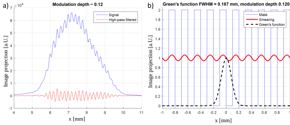
Figure 3.3: a) Projection of the light intensity of a streak camera image with a grid in the object plane without (blue line) and with (red line) high-pass filter to measure the modulation depth of the signal caused by the grid. b) Square shaped grid signal (blue line) convoluted with a Green's function (black dashed line), resulting in a signal with similar modulation depth (red line) as measured for the grid. Both from [46].
