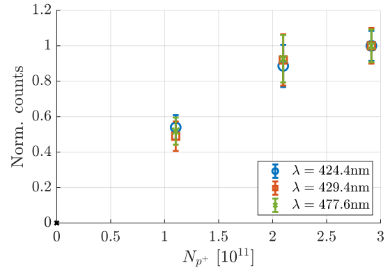
Figure A.10: Peak intensity of the Rb ion transition lines at 424.4 nm (blue circles), 429.4 nm (red squares) and 477.6 nm (green crosses) as a function of proton bunch population, background subtracted and normalized to the maximum mean value. The error bars give the std of the measurements.
