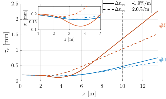
Figure 6.20: The rms width of defocused proton distributions \sigma_r as a function of propagation distance z (plasma z = 1 - 10 m, vacuum z = 10 - 13.5 m) with plasma density gradient \Delta n_{pe} = -1.9\%/m (solid lines) and \Delta n_{pe} = 2.0\%/m (dashed lines) at a fixed \xi of the first (blue lines) and fifth (red lines) period. Inset zooms in at z = 1 - 5 m. Here, n_{pe,Entr.} = 1.8 \cdot 10^{14} \text{ cm}^{-3} and n_b = 5.6 \cdot 10^{12} \text{ cm}^{-3} .
