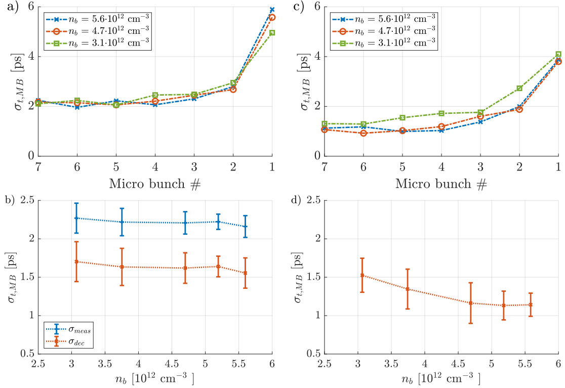
Figure 5.11: Length \sigma_{t,MB} of the fits of the individual micro-bunches for the data with various initial bunch densities n_b = [5.6, 4.7, 3.1] \cdot 10^{12} \text{ cm}^{-3} (blue crosses, red circles, green squares) from experiment (a) and simulations (c). Averaged length over micro-bunch #3 – 7 as a function of initial bunch density from experiment (b) and simulations (d). The error bars give the std variations between micro-bunch #3 and #7. The experimental data (b) contains the directly measured length (blue symbols) and the length deconvolved with \sigma_{res,t} = 1.5 \text{ ps} (red symbols). Here, n_{pe} = 0.9 \cdot 10^{14} \text{ cm}^{-3} and \Delta n_{pe} = 0 .
