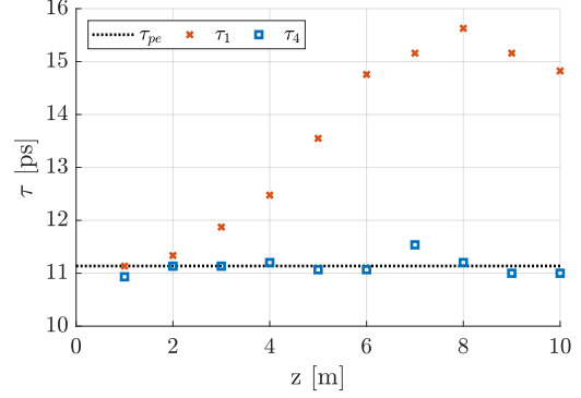
Figure 5.2: Length \tau of the first (red crosses) and fourth (blue squares) modulation period as a function of distance in the plasma z , as obtained from simulations (Table 4.4 except n_{pe} = 1 \cdot 10^{14} \text{ cm}^{-3} ), compared to the plasma period ( \tau_{pe} = 11.1 \text{ ps} , black dotted line).
