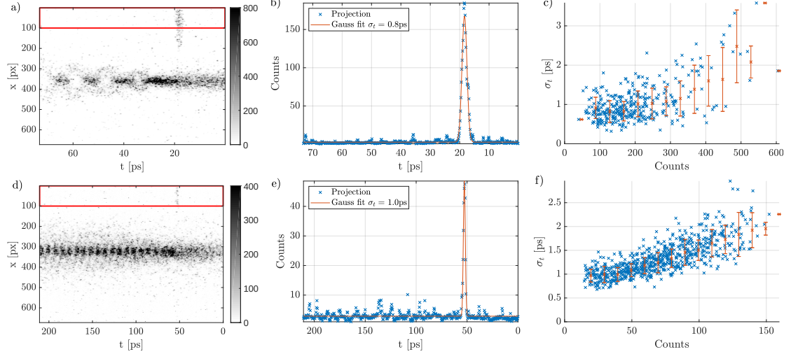
Figure 3.2: Images (a, d) streak camera images with reference laser pulse ( x \leq 100 px, red box). Images (b, e) projection of x \leq 100 px of the streak camera images (blue crosses) and Gaussian fit (red line). Images (c, f) width of the fits as a function of fit amplitude (blue crosses) and data binned in amplitude (red crosses with std as error bars). Here, images (a-c) are obtained with the 73 ps and images (d-f) with the 211 ps streak camera time window.
