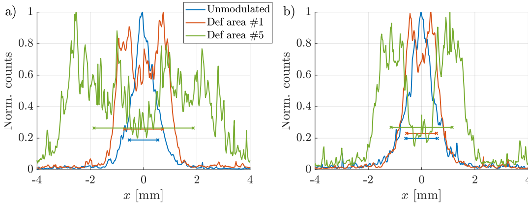
Figure 6.3: Normalized transverse defocused proton distributions from experiment with initial bunch density n_b = 5.6 \cdot 10^{12} \text{ cm}^{-3} (a) and n_b = 3.1 \cdot 10^{12} \text{ cm}^{-3} (b). Transverse profiles of the unmodulated head (blue lines), the first (red lines) and the fifth (green lines) period. The horizontal lines show the rms width of the given distribution with the respective colors. Here, n_{pe} = 0.92 \cdot 10^{14} \text{ cm}^{-3} and \Delta n_{pe} = 0 .
