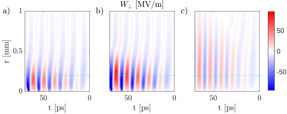
Figure A.24: Transverse wakefield along the bunch t and along the radius component r for the simulation with parameters of Table 4.4 after a) 3 m, b) 5 m and c) 10 m of plasma. Proton bunch incoming radius \sigma_{r,0} = 200 \mu\text{m} (cyan dash-dotted line).
