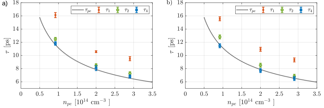
Figure 5.4: Length \tau of the first (red crosses), second (green circles) and fourth (blue squares) modulation period as a function of plasma density, obtained from experiment (a) and simulations (b, parameters in Table 4.4). The black dotted line shows the plasma period ( \tau_{pe} = [11.6, 7.9, 6.5] ps for n_{pe} = [0.92, 2.0, 2.9] \cdot 10^{14} \text{ cm}^{-3} ). The error bars show the rms variation from different initial bunch density measurements in Figure 5.3.
