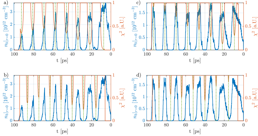
Figure A.13: Central bunch density n_b|_{r=0} modulation (projection of |x| \leq 0.1 mm from time-resolved images, blue lines), weighted distance squared function \chi^2 (cut for high values, red lines) using a parabola as polynomial fit to the data and its minima (green dashed-dotted lines), location of micro-bunches (a, c) and defocused proton regions (b, d) with initial bunch density n_b = 5.6 \cdot 10^{12} \text{ cm}^{-3} (a, b) and n_b = 3.1 \cdot 10^{12} \text{ cm}^{-3} (c, d) from simulations. Here, n_{pe} = 0.92 \cdot 10^{14} \text{ cm}^{-3} and \Delta n_{pe} = 0 .
