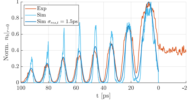
Figure 4.5: Normalized on-axis bunch charge density (projection of |r| \leq 0.1 mm) of the simulation before (bright blue curve) and after \sigma_{res,t} = 1.5 ps Gaussian resolution convolution (dark blue curve) and of the experiment (red curve).
