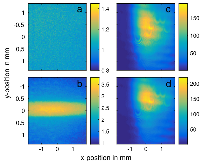
Fig. 6. CCD camera images in the four blocking configurations at high density ( T = 150^\circ\text{C} ) and a laser detuning frequency \Delta\nu_L = -8.7\text{ GHz} : (a) Schlieren and pump beam blocked, (b) only Schlieren beam blocked, (c) only pump beam blocked, (d) neither Schlieren nor pump beam blocked.
