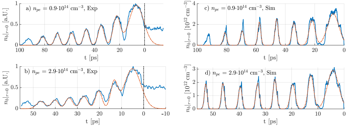
Figure 5.12: On-axis charge density (blue curves) with Gaussian fits to each micro-bunch (red curves) for plasma density n_{pe} = 0.92 \cdot 10^{14} \text{ cm}^{-3} (a, c) and n_{pe} = 2.9 \cdot 10^{14} \text{ cm}^{-3} (b, d), experimentally (a, b) and from simulations (c, d). Here, n_b = 5.6 \cdot 10^{12} \text{ cm}^{-3} and \Delta n_{pe} = 0 .
