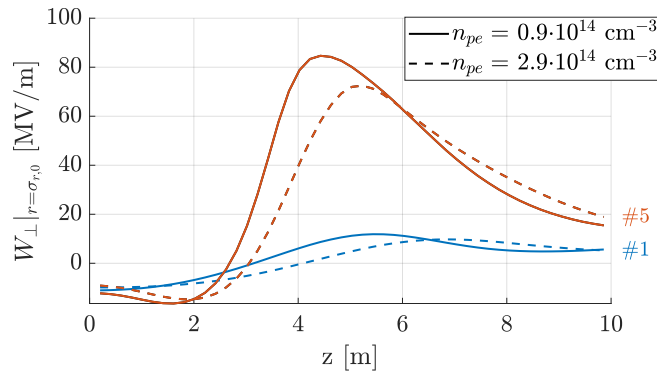
Figure 6.13: Transverse wakefield W_{\perp} at r = \sigma_{r,0} of defocused proton distributions of the first (blue lines) and fifth (red lines) period as a function of distance in plasma z with plasma density n_{pe} = 0.9 \cdot 10^{14} \text{ cm}^{-3} (solid lines) and n_{pe} = 2.9 \cdot 10^{14} \text{ cm}^{-3} (dashed lines). Here, n_b = 5.6 \cdot 10^{12} \text{ cm}^{-3} and \Delta n_{pe} = 0 .
