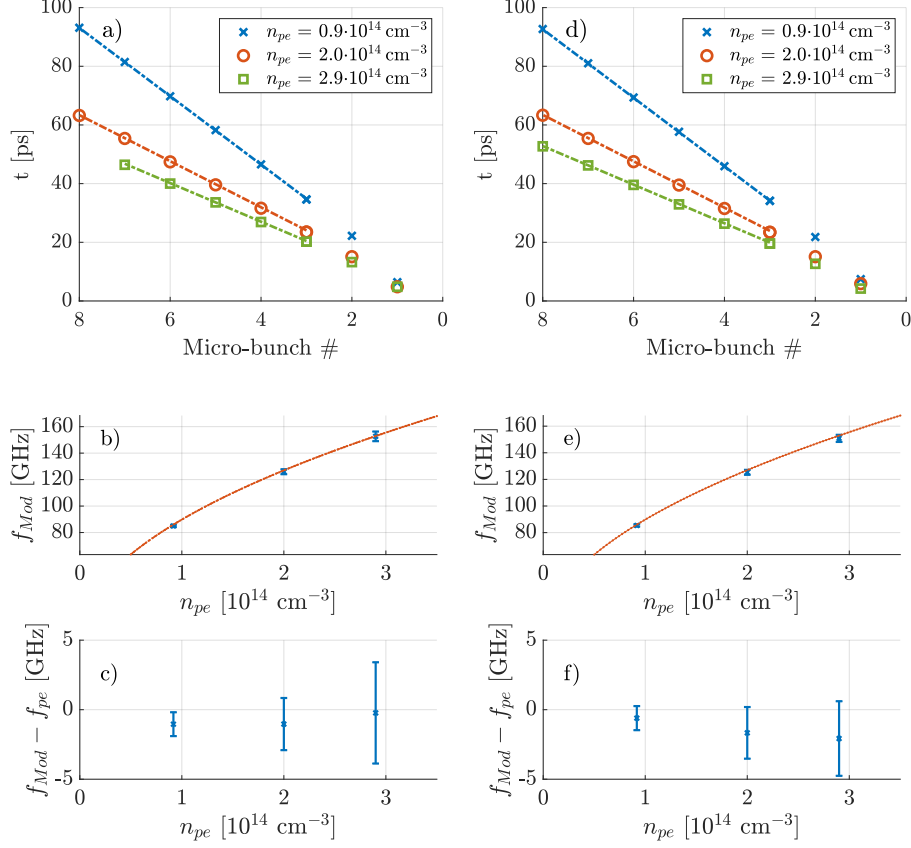
Figure 5.6: Modulation frequency determination from experiment (a-c) and simulations (d-f). Images (a, d) micro-bunch locations (see appendix, Section A.4) for plasma densities n_{pe} = [0.9, 2.0, 2.9] \cdot 10^{14} \text{ cm}^{-3} (blue crosses, red circles, green squares) and their linear fit (dashed lines). Images (b, e) modulation frequency f_{Mod} from the slope of the fit (blue crosses, error bar for a micro-bunch location std uncertainty of 0.5 ps) versus plasma density and the corresponding plasma frequency (red line). Image (c, f) difference between modulation and plasma frequency for the various plasma density measurements.
