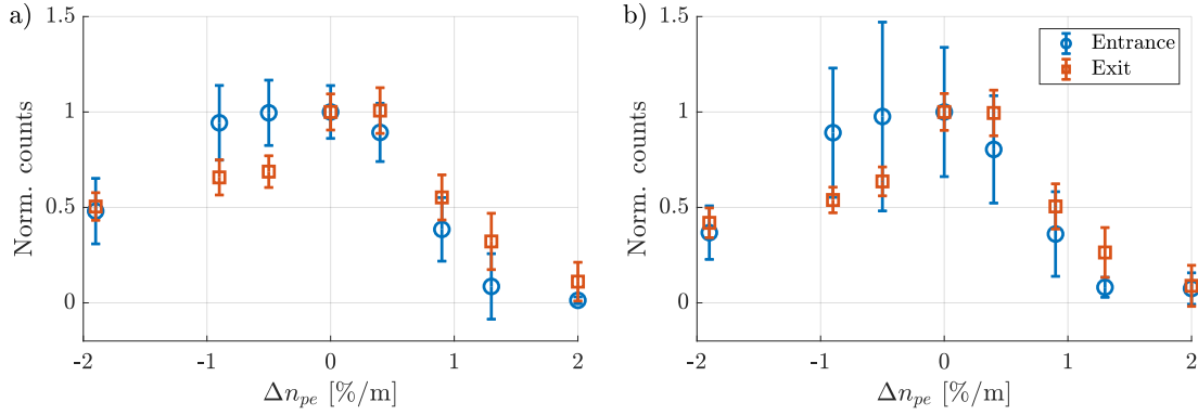
Figure A.7: Peak intensity of the a) \lambda = 424.4 nm and b) \lambda = 477.6 nm Rb ion transition lines with varying plasma density gradient \Delta n_{pe} , measured at the plasma entrance (blue circles) and exit (red squares), both background subtracted and normalized to the value with \Delta n_{pe} = 0 . The error bars give the standard deviation of the variation of the 28 spectra.
