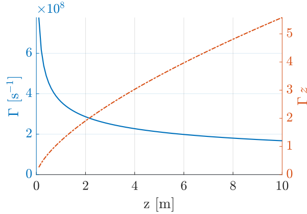
Figure 1.7: Growth rate \Gamma (blue line) and growth \Gamma z (red dashed line) as a function of distance in plasma z at \xi - \xi_{Seed} = \lambda_{pe} . Here, n_b = 5.6 \cdot 10^{12} \text{ cm}^{-3} and n_{pe} = 0.92 \cdot 10^{14} \text{ cm}^{-3} .
