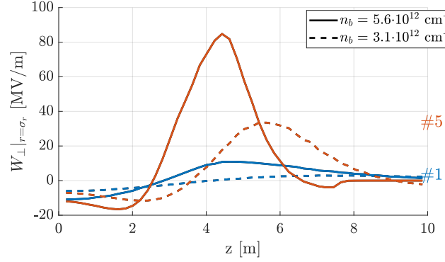
Figure 6.9: Transverse wakefield W_{\perp} evaluated at the rms width of the proton distributions of the first (blue lines) and fifth (red lines) period as a function of distance in plasma z with n_b = 5.6 \cdot 10^{12} \text{ cm}^{-3} (solid lines) and n_b = 3.1 \cdot 10^{12} \text{ cm}^{-3} (dashed lines). Here, n_{pe} = 0.92 \cdot 10^{14} \text{ cm}^{-3} and \Delta n_{pe} = 0 .
