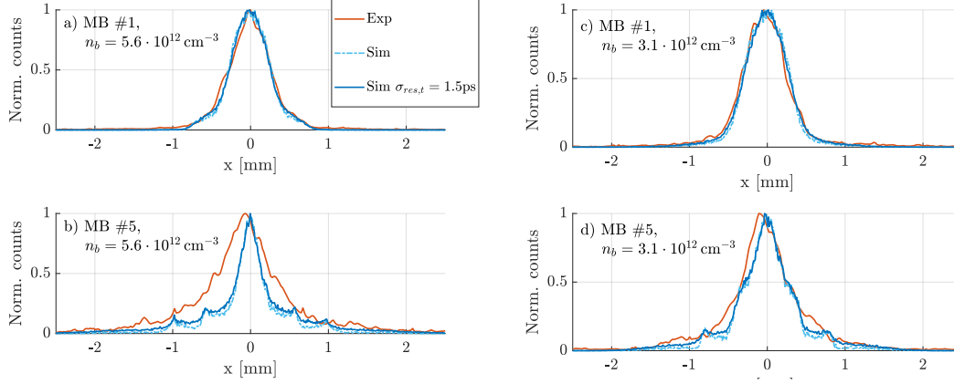
Figure 5.16: Normalized transverse charge density profiles with initial bunch density n_b = 5.6 \cdot 10^{12} \text{ cm}^{-3} (a, b) and n_b = 3.1 \cdot 10^{12} \text{ cm}^{-3} (c, d) for the first (a, c) and fifth (b, d) micro-bunch. Profiles from simulations (bright blue dashed lines), their convolution with temporal resolution \sigma_{res,t} = 1.5 \text{ ps} (dark blue solid lines) and the experimental profiles (red solid lines). Here, n_{pe} = 0.92 \cdot 10^{14} \text{ cm}^{-3} and \Delta n_{pe} = 0 .
