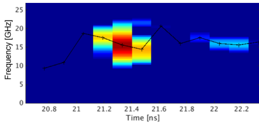
Figure 2.15: Oscilloscope measurement of intermediate beat frequency between CTR signal of the modulated proton bunch and reference signal as a function of time, signal intensity from blue to red, from [39].
