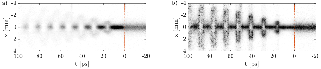
Figure 6.1: Time-resolved images of the modulated bunch; a) original image b) transverse profiles normalized to 1 for each pixel along t . Here, n_{pe} = 0.92 \cdot 10^{14} \text{ cm}^{-3} , \Delta n_{pe} = 0 and n_b = 5.6 \cdot 10^{12} \text{ cm}^{-3} .
