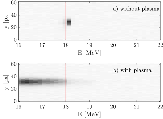
Figure 7.4: Comparison of the energy spectrum of the electron bunch on electron spectrometer a) without, b) with plasma.
