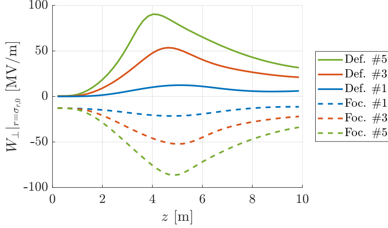
Figure 4.8: Transverse wakefield W_{\perp} at the incoming proton bunch radius r = \sigma_{r,0} as a function of distance in plasma z . Maximum defocusing fields (solid lines) and maximum focusing fields (dashed lines) over the first (blue lines), third (red lines) and fifth (green lines) modulation period.
