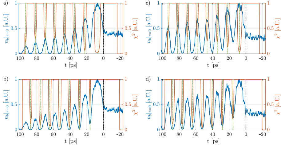
Figure A.12: Central bunch density n_b|_{r=0} modulation (projection of |x| \leq 0.1 mm from time-resolved images, blue lines), weighted distance squared function \chi^2 (cut for high values, red lines) using a parabola as polynomial fit to the data and its minima (green dashed-dotted lines), location of micro-bunches (a, c) and defocused proton regions (b, d) with initial bunch density n_b = 5.6 \cdot 10^{12} \text{ cm}^{-3} (a, b) and n_b = 3.1 \cdot 10^{12} \text{ cm}^{-3} (c, d) from experiment. Here, n_{pe} = 0.92 \cdot 10^{14} \text{ cm}^{-3} and \Delta n_{pe} = 0 .
