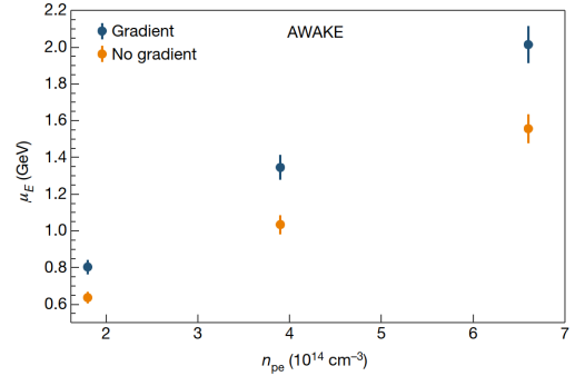
Figure 2.19: Highest peak energy \mu_E as a function of plasma density n_{pe} with constant plasma density (orange points) and with optimum linear plasma density gradient (blue points) over the 10 m, from [42].
