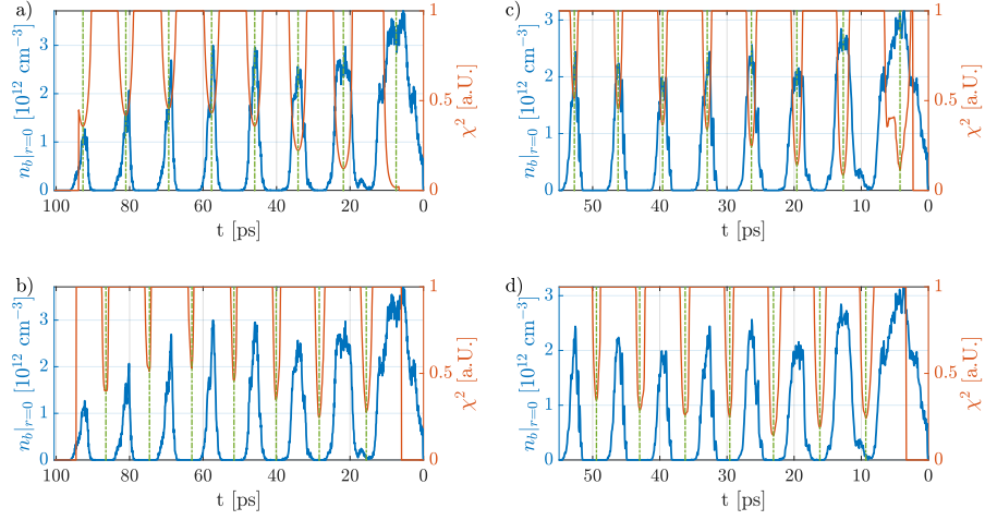
Figure A.15: Central bunch density n_b|_{r=0} modulation (projection of |x| \leq 0.1 mm from time-resolved images, blue lines), weighted distance squared function \chi^2 (cut for high values, red lines) using a parabola as polynomial fit to the data and its minima (green dashed-dotted lines), location of micro-bunches (a, c) and defocused proton regions (b, d) with plasma density n_{pe} = 0.92 \cdot 10^{14} \text{ cm}^{-3} (a, b) and n_{pe} = 2.9 \cdot 10^{14} \text{ cm}^{-3} (c, d) from simulations. Here, n_b = 5.6 \cdot 10^{12} \text{ cm}^{-3} and \Delta n_{pe} = 0 .
