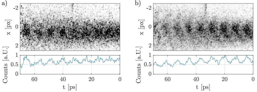
Figure 7.7: Top: average of normalized time-resolved images of a) 12 images without and b) 26 images with preceding electron bunch; bottom: projection over -0.5 \text{ mm} < x < 1 \text{ mm} , normalized to 1.
