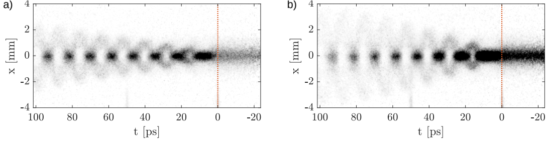
Figure 4.1: Two stitched streak camera images of the modulated proton bunch after plasma. The bunch is propagating from left to right, where the unmodulated head of the bunch propagated through vapor ( t < 0 ), the modulated back of the bunch through plasma ( t > 0 ). Relativistic ionization front at t = 0 (red dotted line). Images are saturated for better visibility of lower charge density defocused proton distributions between micro-bunches. Image a) shows the modulated bunch starting the interaction with plasma at lower ( n_b = 3.1 \cdot 10^{12} \text{ cm}^{-3} ), image b) with higher ( n_b = 5.6 \cdot 10^{12} \text{ cm}^{-3} ) initial bunch density. The higher initial bunch density leads to wider defocused proton distributions.
