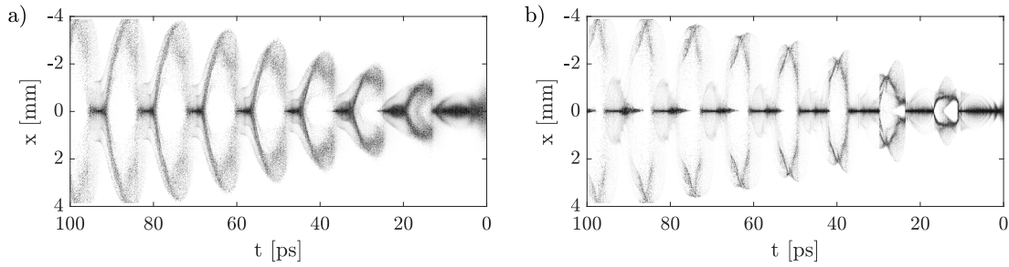
Figure A.26: Normalized time-resolved images from simulations with a normalized bunch emittance of a) \epsilon^* = 3.6 \mu\text{m} and b) \epsilon^* = 1.0 \mu\text{m} . Here, n_b = 5.6 \cdot 10^{12} \text{ cm}^{-3} , n_{pe} = 0.9 \cdot 10^{14} \text{ cm}^{-3} and \Delta n_{pe} = 0 .
