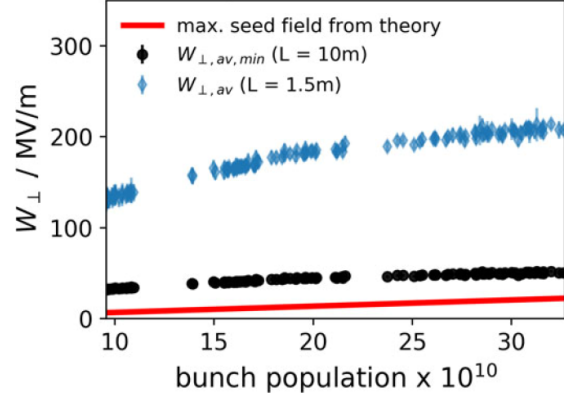
Figure 2.12: Transverse wakefield amplitude as a function of proton bunch population with n_{pe} = 2.1 \cdot 10^{14} \text{ cm}^{-3} . Seed wakefield amplitude (red line), average of the transverse wakefield assuming protons exit the wakefield after L = 10 \text{ m} of plasma ( W_{\perp,av,min} , black circles) or assuming protons exit the wakefield at 4m after L = 1.5 \text{ m} distance of interaction with the wakefield ( W_{\perp,av} , blue diamonds), from [14].
