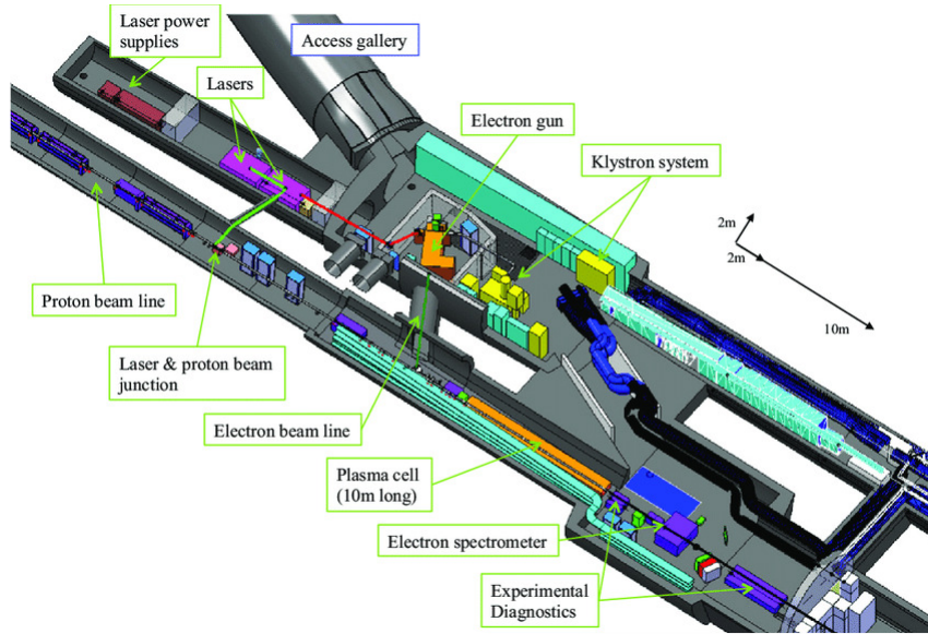
Figure 2.2: Overview of the AWAKE facility [32].
