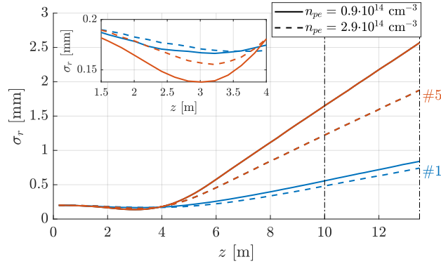
Figure 6.14: The rms width of defocused proton distributions \sigma_r as a function of propagation distance z (plasma z = 1 - 10 m, vacuum z = 10 - 13.5 m) with plasma density n_{pe} = 0.9 \cdot 10^{14} \text{ cm}^{-3} (solid lines) and n_{pe} = 2.9 \cdot 10^{14} \text{ cm}^{-3} (dashed lines) at a fixed \xi of the first (blue lines) and fifth (red lines) period. Inset zooms in at z = 1.5 - 4 m. Here, n_b = 5.6 \cdot 10^{12} \text{ cm}^{-3} and \Delta n_{pe} = 0 .
