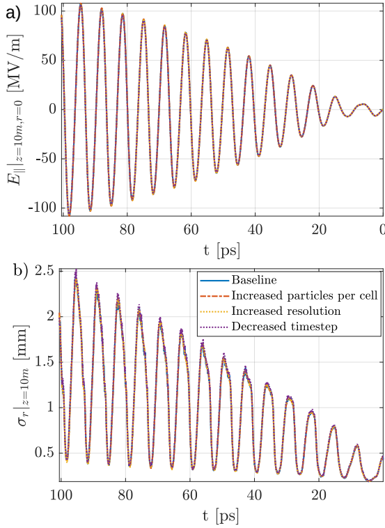
Figure 4.2: a) On-axis ( r = 0 ) longitudinal electric field E_{\parallel} ; b) rms bunch width distribution, both as a function of time t along the bunch (bunch cut at t = 0 ) and at the plasma exit ( z = 10 m). Baseline simulation (blue lines) with particles per cell 4 (plasma electrons) and 32 (on-axis, proton bunch), grid size \delta x, \delta y = 10 \mu\text{m} , \delta z = 20 \mu\text{m} and time step dt = 20 cm. Simulation results for particles per cell 16 (plasma electrons) and 128 (on-axis, proton bunch) (red dash-dotted lines), for grid size \delta x, \delta y = 5 \mu\text{m} , \delta z = 10 \mu\text{m} (yellow dotted line) and for time step dt = 10 cm (violet dotted line). Here, n_{pe} = 2.9 \cdot 10^{14} \text{ cm}^{-3} and bunch parameters from Table 4.4.
