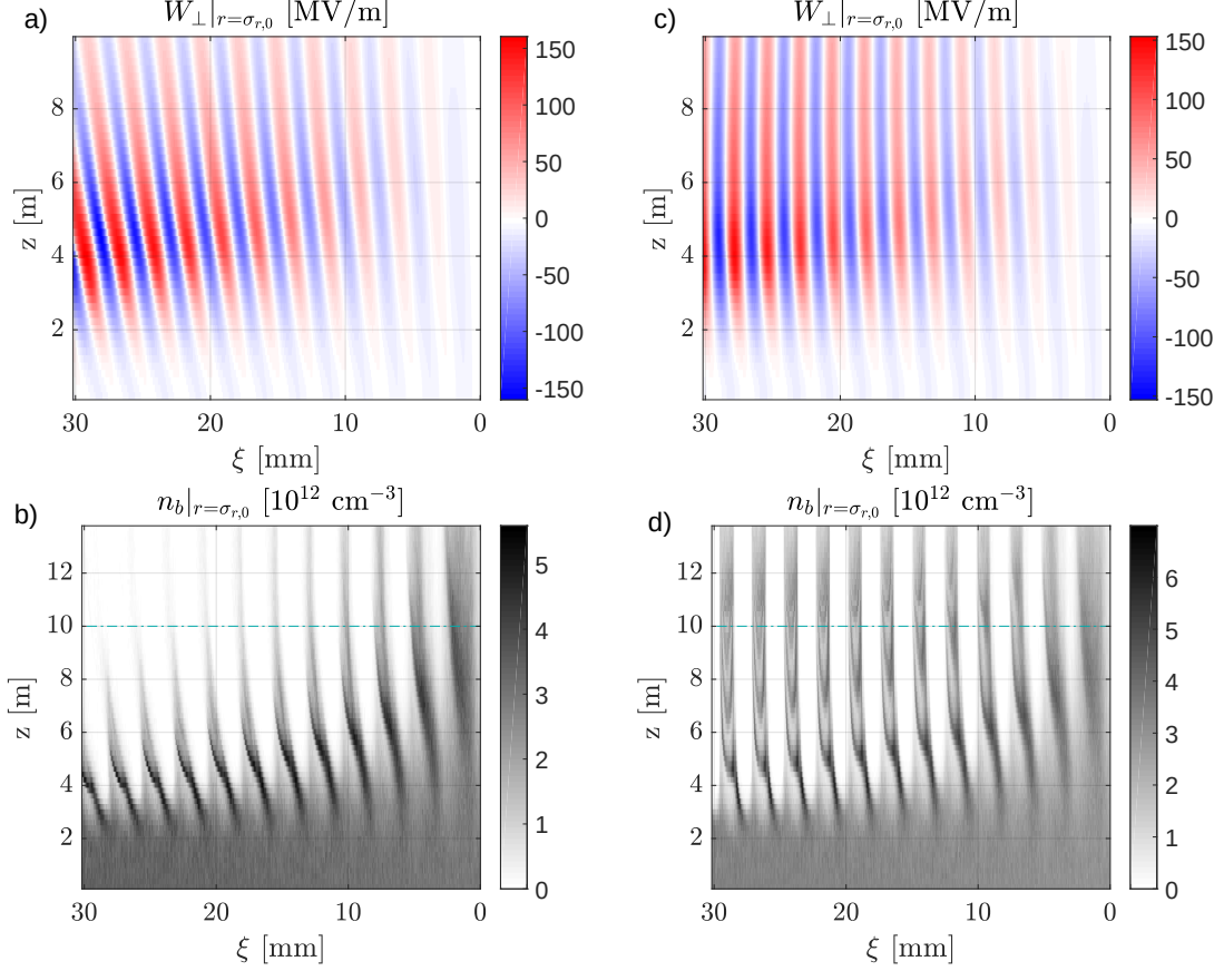
Figure 5.21: Transverse wakefield (a, c) and bunch density (b, d) at r = \sigma_{r,0} = 200 \mu\text{m} along the bunch \xi and along the plasma z with plasma density gradient \Delta n_{pe} = -1.9 \text{ \%/m} (a, b) and \Delta n_{pe} = 2.0 \text{ \%/m} (c, d). Images are saturated to also show small wakefield amplitudes and densities. Plasma ends at z = 10 m (cyan dash-dotted line in b, d). Here, n_b = 5.6 \cdot 10^{12} \text{ cm}^{-3} and n_{pe,Entr.} = 1.8 \cdot 10^{14} \text{ cm}^{-3} .
