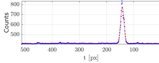
Figure 3.8: Gaussian fit (red line) to the projection of the timing reference laser pulse ( 15 \text{ px} \leq x \leq 110 \text{ px} of the streak camera image of Figure 3.4) (blue points). The center of the fitted peak is used for temporal alignment of multiple events.
