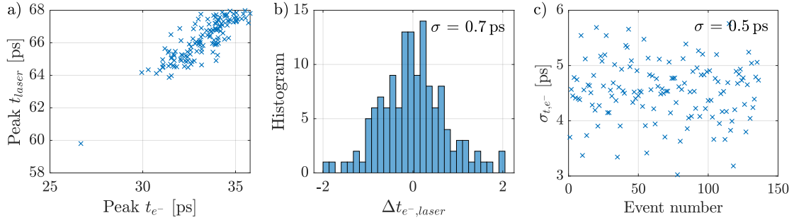
Figure 7.3: Determination of temporal jitter between laser pulse and electron bunch from 136 events. a) Gaussian fit peak position of the laser pulse versus fit peak position of the electron bunch; b) histogram of difference between laser pulse and electron bunch timing, mean value \overline{\Delta t} = 32.9 ps subtracted; c) Gaussian fit width of electron bunch.
