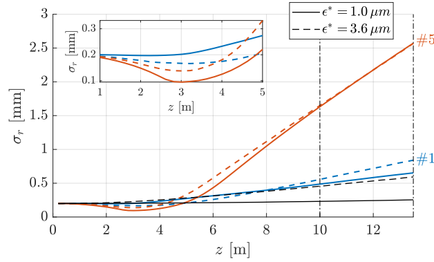
Figure A.28: The rms width of defocused proton distributions \sigma_r as a function of propagation distance z (plasma z = 1 - 10 m, vacuum z = 10 - 13.5 m) with normalized incoming bunch emittance \epsilon^* = 1.0 \mu\text{m} (solid lines) and \epsilon^* = 3.6 \mu\text{m} (dashed lines) at a fixed \xi of the first (blue lines) and fifth (red lines) period and without plasma (black lines). Inset zooms in at z = 1 - 5 m. Here, n_b = 5.6 \cdot 10^{12} \text{ cm}^{-3} , n_{pe} = 0.9 \cdot 10^{14} \text{ cm}^{-3} and \Delta n_{pe} = 0 .
