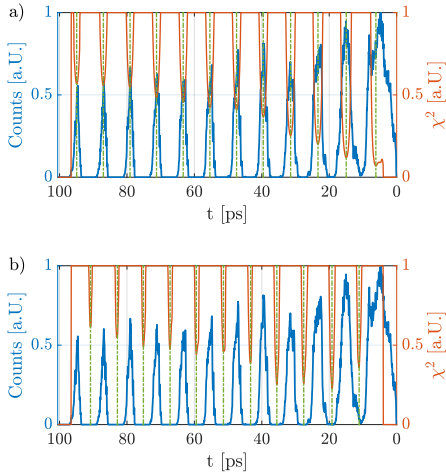
Figure A.21: Central bunch density n_b|_{r=0} modulation (projection of |x| \leq 0.1 mm from time-resolved images, blue lines), weighted distance squared function \chi^2 (cut for high values, red lines) using a parabola as polynomial fit to the data and its minima (green dashed-dotted lines), location of micro-bunches (a) and defocused proton regions (b) with seed position \xi_{Seed} = -0.6 \sigma_\xi ( n_b = 4.1 \cdot 10^{12} \text{ cm}^{-3} ) from simulations. Here, n_{pe} = 2.0 \cdot 10^{14} \text{ cm}^{-3} and \Delta n_{pe} = 0 .
