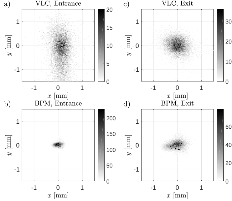
Figure 2.7: Laser alignment results of more than 6000 events. Position of the laser pulse on the VLCs (a, c), position of the proton bunch from BPMs (b, d), before (a, b) and after (c, d) the plasma; counts give number of events. The origin x = y = 0 of the figures corresponds to the proton bunch reference trajectory.
