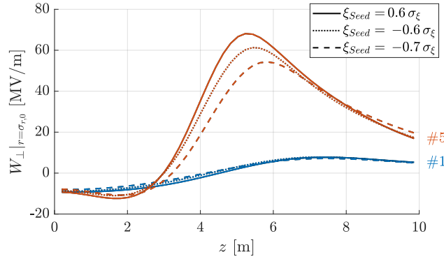
Figure A.36: Transverse wakefield at r = \sigma_{r,0} of defocused protons of the first (blue lines) and fifth (red lines) period as a function of distance in plasma z with seed position \xi_{Seed} = 0.6\sigma_\xi (solid lines), \xi_{Seed} = -0.6\sigma_\xi (dotted lines), \xi_{Seed} = -0.7\sigma_\xi (dashed lines). Here, n_{pe} = 2.0 \cdot 10^{14} \text{ cm}^{-3} and \Delta n_{pe} = 0 .
