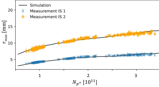
Figure A.11: Maximum radius of time-integrated proton bunch distribution r_{max} as a function of proton bunch population N_{p+} , measured 2 m (blue crosses) and 10 m (yellow circles) after the plasma, from [69].
