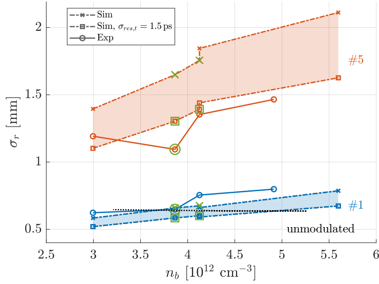
Figure A.35: The rms width of defocused proton distributions from experiment (circles) and simulations without (crosses) and with (squares) \sigma_{res,t} = 1.5 ps resolution convolution) as a function of initial bunch density n_b for the first (blue lines) and fifth (red lines) period and rms width of unmodulated bunch (black lines). Seed positions behind the bunch center ( \xi_{Seed} = -0.7 \sigma_\xi , i.e. n_b = 3.9 \cdot 10^{14} \text{ cm}^{-3} in experiment and simulation and \xi_{Seed} = -0.6 \sigma_\xi , i.e. n_b = 4.1 \cdot 10^{14} \text{ cm}^{-3} in simulation) marked in green. Here, n_{pe} = 2.0 \cdot 10^{14} \text{ cm}^{-3} and \Delta n_{pe} = 0 .
