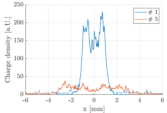
Figure 3.20: Transverse defocused proton distribution of the first (blue line) and fifth (red line) period with the signal above (solid lines) and below (dashed lines) the noise threshold, here 5 [a.u.].
