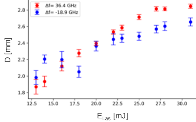
Figure 2.8: Plasma column diameter D versus ionizing laser energy E_{Las} (error bars give the std divided by the square root of number of measurements) with the imaging laser frequency below ( \Delta f = -18.9 GHz, blue symbols) and above ( \Delta f = 36.4 GHz, red symbols) the Rb D2 transition line, from [37].
