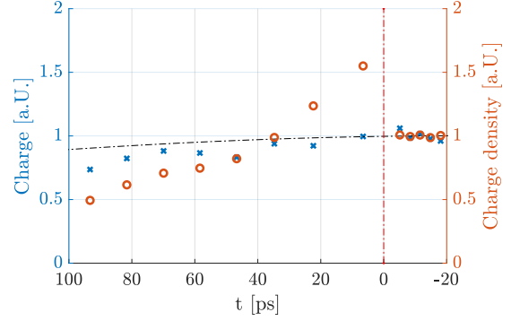
Figure 3.19: Integrated charge density (red circles), integrated charge (blue crosses) and longitudinal incoming bunch charge (density) profile (Gaussian, black dash-dotted line). Here, \xi_{Seed} = -0.1 \sigma_\xi and \sigma_\xi = 7.92 \text{ cm} \hat{=} \sigma_t = 264 \text{ ps} .
