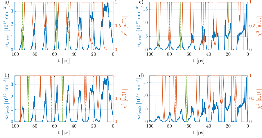
Figure A.18: Central bunch density n_b|_{r=0} modulation (projection of |x| \leq 0.1 mm from time-resolved images, blue lines), weighted distance squared function \chi^2 (cut for high values, red lines) using a parabola as polynomial fit to the data and its minima (green dashed-dotted lines), location of micro-bunches (a, c) and defocused proton regions (b, d) with normalized incoming bunch emittance \epsilon^* = 3.6 \mu\text{m} (a, b) and \epsilon^* = 1.0 \mu\text{m} (c, d) from simulations. Here, n_{pe} = 0.92 \cdot 10^{14} \text{ cm}^{-3} , n_b = 5.6 \cdot 10^{12} \text{ cm}^{-3} and \Delta n_{pe} = 0 .
