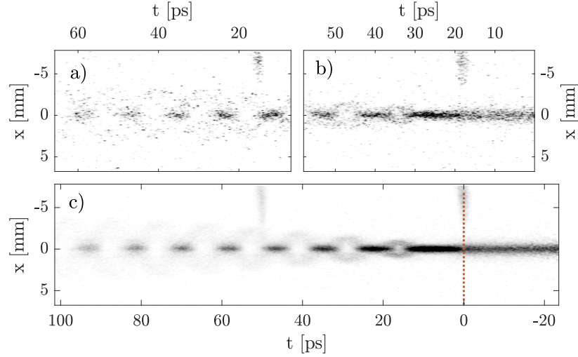
Figure 3.10: a) Single streak camera image with a 50 ps time delay to the start of the SM, b) single streak camera image at the start of the SM and c) sets of the two time delays of 20 streak camera images each stitched together using the timing reference signal [43].
