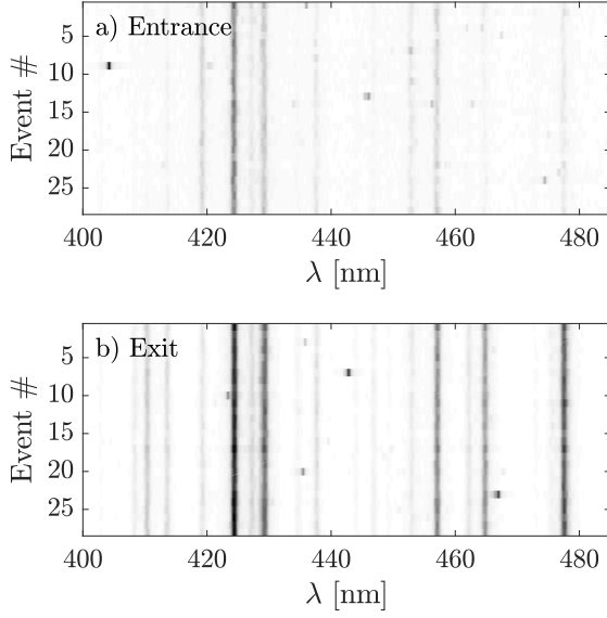
Figure A.5: Plasma light spectrum around \lambda = 424.4 nm for 28 subsequent events without plasma density gradient ( \Delta n_{pe} = 0 ) at the plasma entrance (a) and exit (b).
