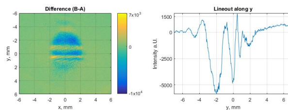
Fig 3. Difference of the two images in Fig. 2 (B)-(A) (left), profile of the image averaged between -1 \text{ mm} \leq x \leq 1 \text{ mm} (right)
