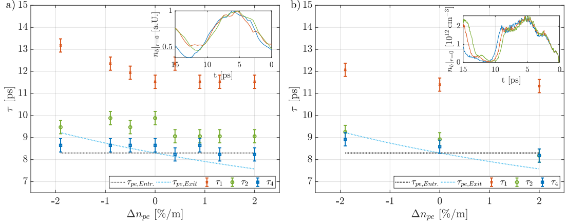
Figure 5.5: Length \tau of the first (red crosses), second (green circles) and fourth (blue squares) modulation period as a function of plasma density gradient \Delta n_{pe} , obtained from experiment (a) and simulations (b, parameters in Table 4.4). The black dotted line shows the plasma period at the entrance ( \tau_{pe,Entr.} = 8.3 ps for n_{pe,Entr.} = 1.8 \cdot 10^{14} \text{ cm}^{-3} ), the blue dotted line at the exit ( \tau_{pe,Exit} = (9.2 - 7.6) ps for n_{pe,Exit} = (1.46 - 2.16) \cdot 10^{14} \text{ cm}^{-3} ). The error bars show the rms variation from different initial bunch density measurements. Insets: Normalized on-axis charge density of the first modulation period for \Delta n_{pe} = -1.9 %/m (blue lines), \Delta n_{pe} = 0 (red lines) and \Delta n_{pe} = 2.0 %/m (green lines).
