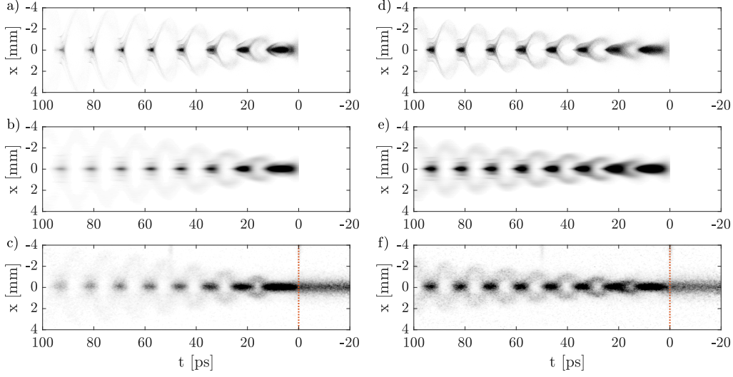
Figure 4.9: Time-resolved images of the bunch after the plasma with initial bunch density n_b = 5.6 \cdot 10^{12} \text{ cm}^{-3} (a-c) and n_b = 3.1 \cdot 10^{12} \text{ cm}^{-3} (d-f). Images (a, d) are simulation results without, (b, e) with \sigma_{res,t} = 1.5 \text{ ps} temporal resolution convolution and (c, f) the corresponding experimental images. Color scale saturated to 50 % of the maximum value. Here, n_{pe} = 0.92 \cdot 10^{14} \text{ cm}^{-3} and \Delta n_{pe} = 0 .
