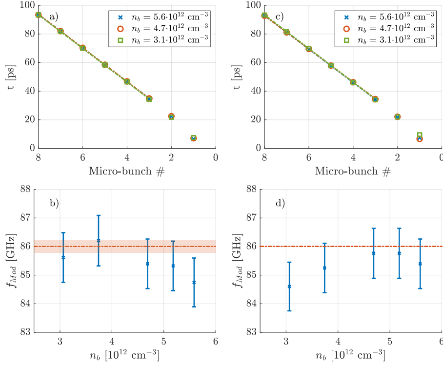
Figure 5.7: Modulation frequency determination from experiment (a, b) and simulations (c, d). Images (a, c) micro-bunch locations (see appendix, Section A.4) for initial bunch densities n_b = [5.6, 4.7, 3.1] \cdot 10^{12} \text{ cm}^{-3} (blue crosses, red circles, green squares) and their linear fits (dashed lines). Images (b, d) modulation frequency f_{Mod} from the slopes of the fits (blue crosses, error bar for a micro-bunch location std uncertainty of 0.5 ps) versus initial bunch density and plasma frequency f_{pe} = 86.0 \text{ GHz} for n_{pe} = 0.9175 \cdot 10^{14} \text{ cm}^{-3} (red line). The error of the plasma frequency in experiment (b) results from the Rb density measurement precision of < 0.5 \% .
