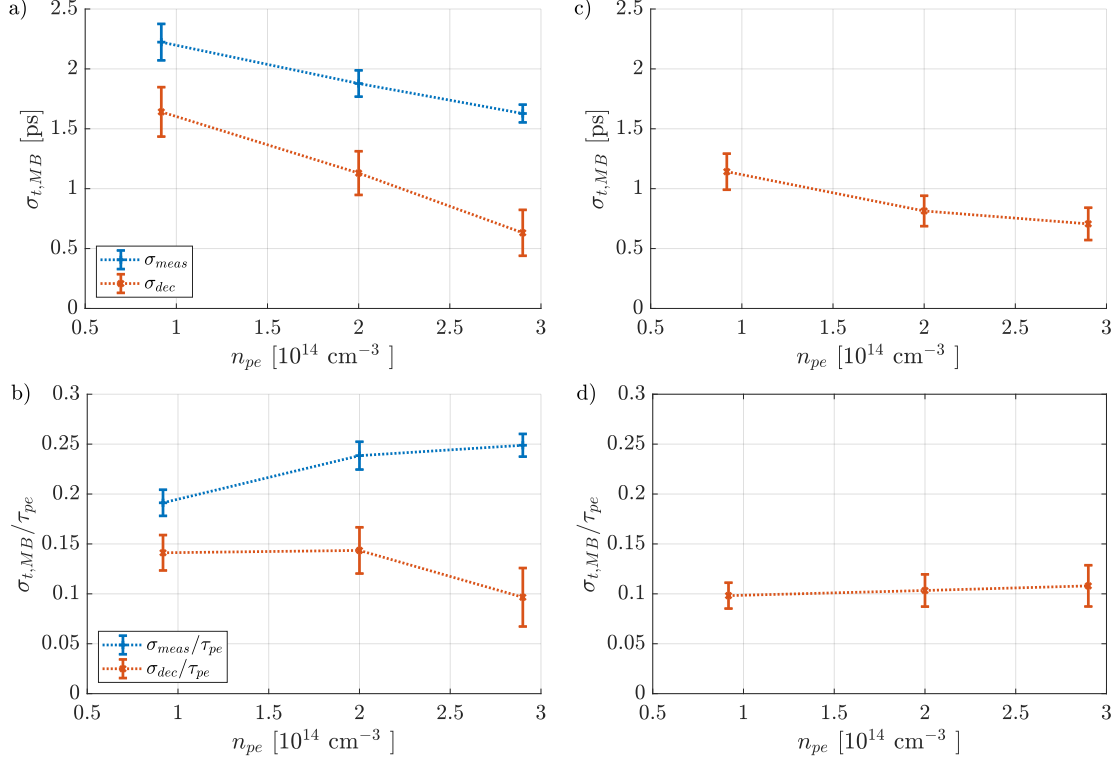
Figure 5.13: Micro-bunch length determined from Gaussian fits as a function of plasma density in experiment (a, b) and simulations (c, d). Images (a, c) show the absolute micro-bunch length, images (b, d) the length normalized to the corresponding plasma period. The error bars give the rms variations from different initial bunch density measurements and from micro-bunch #3 – 7. The experimental data contains the directly measured length (blue symbols) and the length deconvolved with \sigma_{res,t} = 1.5 \text{ ps} (red symbols). Here, n_b = 5.6 \cdot 10^{12} \text{ cm}^{-3} and \Delta n_{pe} = 0 .
