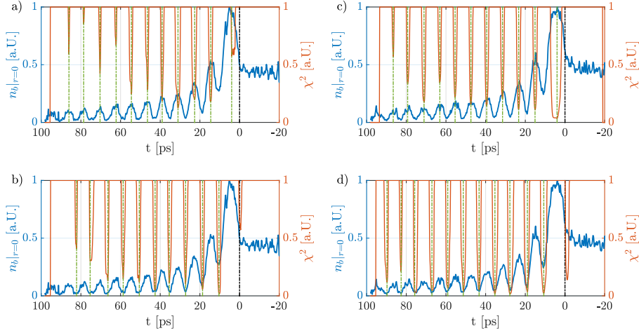
Figure A.19: Central bunch density n_b|_{r=0} modulation (projection of |x| \leq 0.1 mm from time-resolved images, blue lines), weighted distance squared function \chi^2 (cut for high values, red lines) using a parabola as polynomial fit to the data and its minima (green dashed-dotted lines), location of micro-bunches (a, c) and defocused proton regions (b, d) with seed position \xi_{Seed} = -0.7 \sigma_\xi ( n_b = 3.9 \cdot 10^{12} \text{ cm}^{-3} , Figures a, b) and \xi_{Seed} = 0.6 \sigma_\xi ( n_b = 4.1 \cdot 10^{12} \text{ cm}^{-3} , Figures c, d) from experiment. Here, n_{pe} = 2.0 \cdot 10^{14} \text{ cm}^{-3} and \Delta n_{pe} = 0 .
