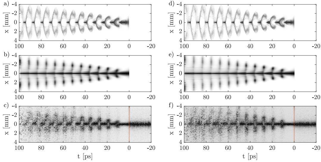
Figure A.33: Normalized time-resolved images of the modulated bunch with seed position \xi_{Seed} = -0.7\sigma_\xi ( n_b = 3.9 \cdot 10^{12} \text{ cm}^{-3} , a-c) and \xi_{Seed} = 0.6\sigma_\xi ( n_b = 4.1 \cdot 10^{12} \text{ cm}^{-3} , d-f). Images (a, b) show the simulation results without, (b, e) with \sigma_{res,t} = 1.5 \text{ ps} Gaussian temporal resolution convolution and (c, f) the streak camera images. Here, n_{pe} = 2.0 \cdot 10^{14} \text{ cm}^{-3} and \Delta n_{pe} = 0 .
