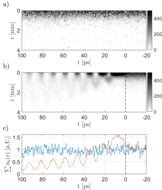
Figure 3.16: Streak camera image (i.e. charge density) of the a) unmodulated and b) modulated bunch; c) charge density integrated over r \leq 4\text{mm} of the unmodulated (blue line) and modulated (red line) bunch, both normalized to the mean value of the sum of the incoming bunch charge density over -15\text{ps} \leq t \leq -4\text{ps} . Here, \xi_{Seed} = -0.1\sigma_\xi .
