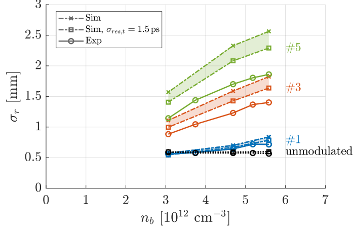
Figure 6.6: The rms width of defocused proton distributions from experiment (circles) and simulations without (crosses) and with (squares) \sigma_{res,t} = 1.5 ps resolution convolution as a function of initial bunch density n_b of the first (blue symbols), third (red symbols) and fifth (green lines) period and rms width of unmodulated bunch (black symbols). Here, n_{pe} = 0.92 \cdot 10^{14} \text{ cm}^{-3} and \Delta n_{pe} = 0 .
