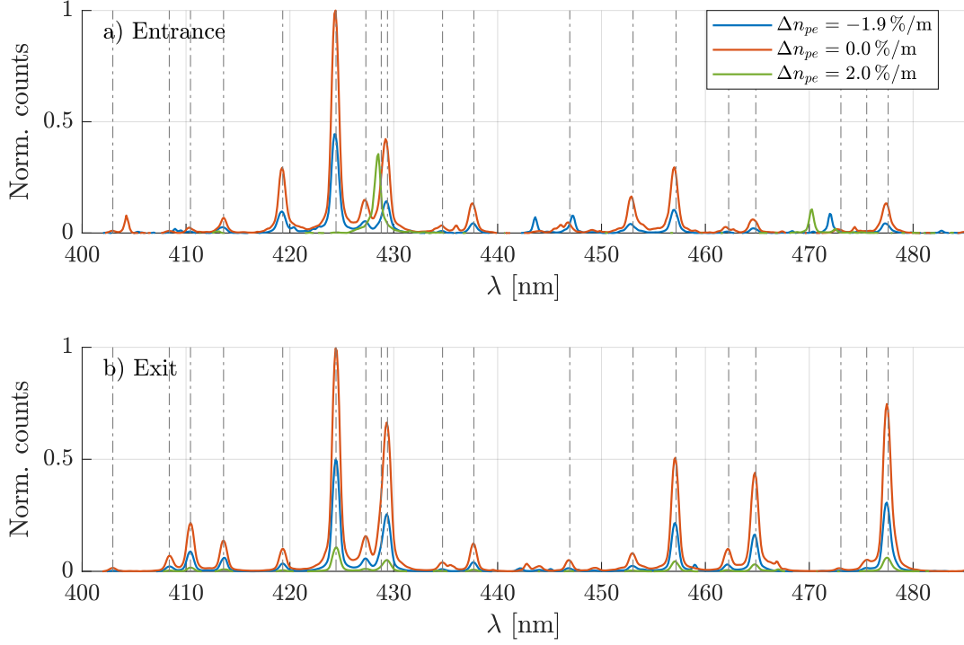
Figure A.6: Average of the plasma light spectra at \lambda = 400 - 480 nm with most negative ( \Delta n_{pe} = -1.9 \text{ \%/m} , blue line), without ( \Delta n_{pe} = 0 , red line) and most positive ( \Delta n_{pe} = 2.0 \text{ \%/m} , green line) density gradient at the plasma entrance (a) and exit (b).
