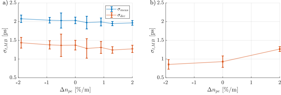
Figure 5.15: Micro-bunch length determined from Gaussian fits as a function of plasma density gradient in experiment (a) and simulations (b). The error bars give the rms variations from micro-bunch #3 – 7. The experimental data contains the directly measured length (blue symbols) and the length deconvolved with \sigma_{res,t} = 1.5 ps (red symbols). Here, n_{pe,Entr.} = 1.8 \cdot 10^{14} \text{ cm}^{-3} and n_b = 5.6 \cdot 10^{12} \text{ cm}^{-3} .
