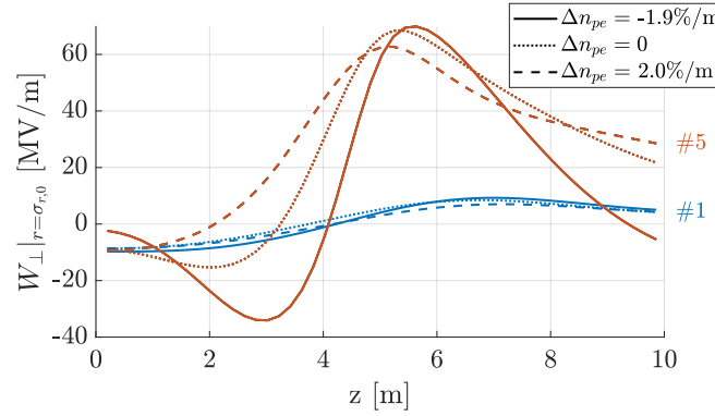
Figure 6.19: Transverse wakefield W_{\perp} at r = \sigma_{r,0} of defocused proton distributions of the first (blue lines) and fifth (red lines) period as a function of distance in plasma z with plasma density gradient \Delta n_{pe} = -1.9\%/m (solid lines) \Delta n_{pe} = 0 (dotted lines) and \Delta n_{pe} = 2.0\%/m (dashed lines). Here, n_{pe,Entr.} = 1.8 \cdot 10^{14} \text{ cm}^{-3} and n_b = 5.6 \cdot 10^{12} \text{ cm}^{-3} .
