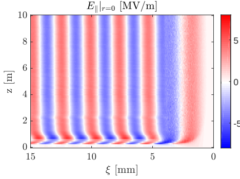
Figure 7.16: Longitudinal wakefield amplitudes along the bunch axis \xi and along the plasma z at r \approx 0 driven by 165 MeV electron bunch.
