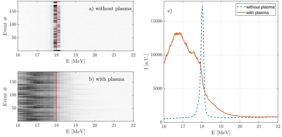
Figure 7.5: Waterfall plot of the integrated electron bunch energy distribution spectrum a) without and b) with plasma; c) mean of the integrated energy distribution spectrum without (blue dashed line) and with (red solid line) plasma.
