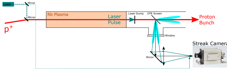
Figure 2. Transport of OTR light of a modulated proton bunch to streak camera at AWAKE (not to scale)
