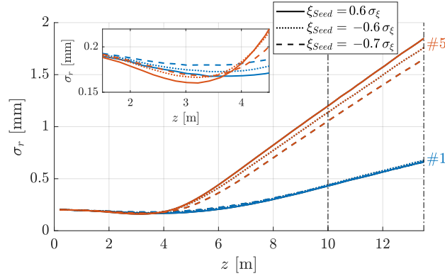
Figure A.37: The rms width of defocused proton distributions \sigma_r as a function of distance in plasma z with seed position \xi = 0.6 \sigma_\xi (solid lines), \xi = -0.6 \sigma_\xi (dotted lines) and \xi = -0.7 \sigma_\xi (dashed lines) at a fixed \xi of the first (blue lines) and fifth (red lines) period and without plasma (black lines). Inset zooms in at z = 1 - 5 m. Here, n_{pe} = 2.0 \cdot 10^{14} \text{ cm}^{-3} and \Delta n_{pe} = 0 .
