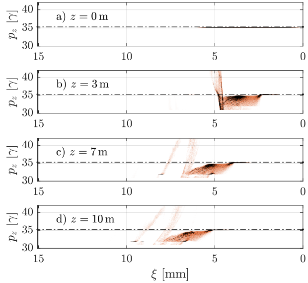
Figure 7.15: Longitudinal momentum p_z of electrons versus bunch position \xi after z = 0, 3, 7, 10 m (from a to d) of plasma.
