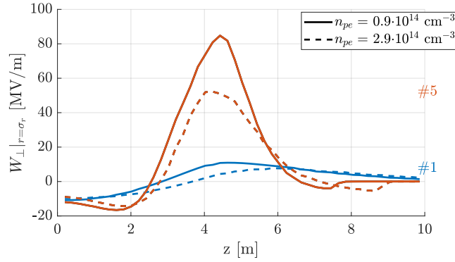
Figure 6.15: Transverse wakefield W_{\perp} evaluated at the rms width of the proton distributions of the first (blue lines) and fifth (red lines) period as a function of distance in plasma z with plasma density n_{pe} = 0.9 \cdot 10^{14} \text{ cm}^{-3} (solid lines) and n_{pe} = 2.9 \cdot 10^{14} \text{ cm}^{-3} (dashed lines). Here, n_b = 5.6 \cdot 10^{12} \text{ cm}^{-3} and \Delta n_{pe} = 0 .
