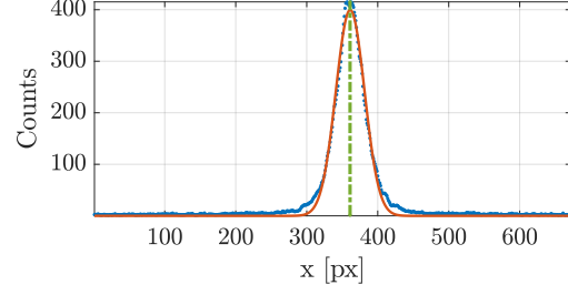
Figure 3.12: Projection of -22 \text{ ps} < t < -9 \text{ ps} of the stitched image (Figure 3.10) (blue dots) fitted with a Gaussian function (red line). The transverse bunch center is determined by the center of the fit peak (green dash-dotted line).
