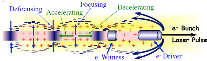
Figure 1.1: Schematic of the principle of plasma wakefield acceleration: A short particle bunch or laser pulse (propagating from left to right) drives a wakefield inside plasma, consisting of focusing/defocusing (blue arrows) and accelerating/decelerating (green arrows) phases. A to be accelerated witness particle (here electron e^- ) bunch is injected in the focusing and accelerating phase of the wakefield [2]
