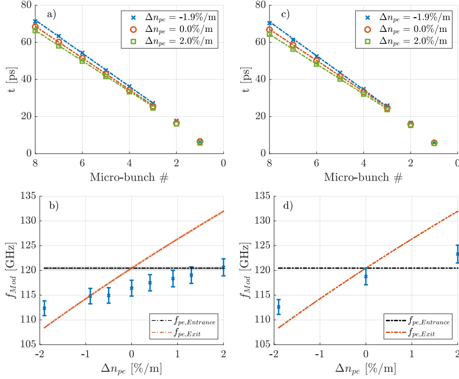
Figure 5.8: Modulation frequency determination from experiment (a, b) and simulations (c, d). Images (a, c) micro-bunch locations (see appendix, Section A.4) for plasma density gradients [-1.9, 0, 2.0]\%/m (blue crosses, red circles, green squares) and their linear fit (dashed lines). Images (b, d) modulation frequency f_{Mod} from the slope of the fit (blue crosses, error bar for a micro-bunch location std uncertainty of 0.5 ps) versus density gradient [-1.9, (-0.9), (-0.5), 0, (0.4), (0.9), (1.3), 2.0]\%/m (values in brackets only in experiment) and plasma frequency at the entrance f_{pe,Entr.} = 120.5 GHz for n_{pe} = 1.8 \cdot 10^{14} \text{ cm}^{-3} (black line) and exit f_{pe,Exit} = 108.4 - 132.0 GHz for n_{pe} = 1.46 - 2.16 \cdot 10^{14} \text{ cm}^{-3} (red line).
