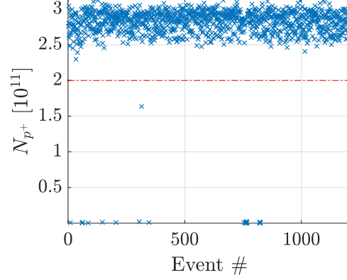
Figure 3.7: Proton bunch population N_{p+} (blue crosses) of more than 1200 consecutive events, measured by the beam current transformers. Events with a population of < 2 \cdot 10^{11} (red line) are considered failed extractions.
