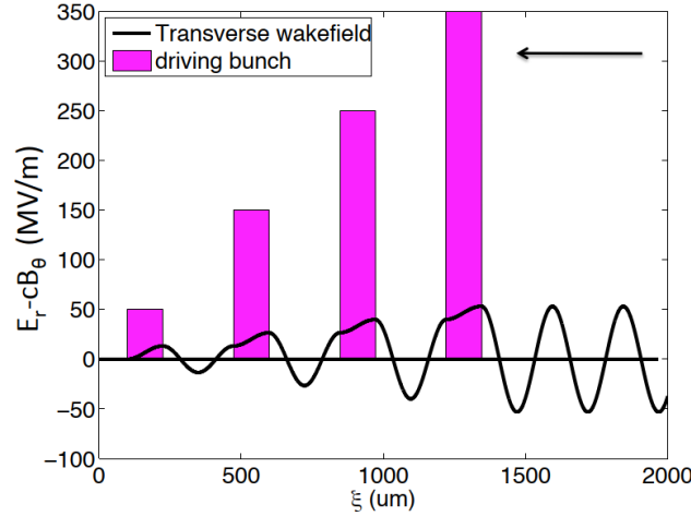
Figure 1.6: Transverse wakefield W_{\perp} = E_r - c B_{\theta} (black line, from radial electric field E_r and azimuthal magnetic field B_{\theta} ), along the train of four square micro-bunches with increasing charge Q_m = [1, 3, 5, 7] \cdot Q_{m,0} (violet bars), from [18].
