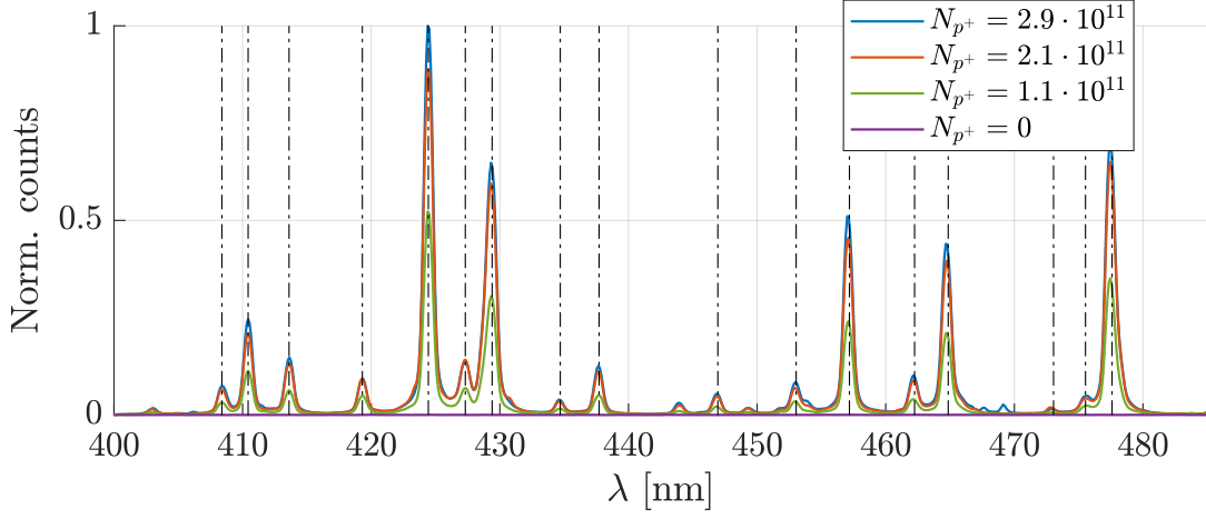
Figure A.9: Average of \sim 30 plasma light spectra with various Rb ion transition lines (black dash-dotted lines) for different proton bunch populations N_{p+} = [0, 1.1, 2.1, 2.9] \cdot 10^{11} (violet, green, red, blue curve).
