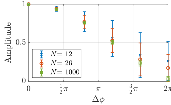
Figure 7.8: Amplitude (difference between maximum and minimum value) of the sum of 12 (blue crosses), 26 (red circles) or 1000 (green squares) cosine functions with amplitude 1 as a function of the range of their phase variations. The error bars correspond to the standard deviation of the amplitude when repeating the calculation with random phase, within their phase range, 1000 times.
