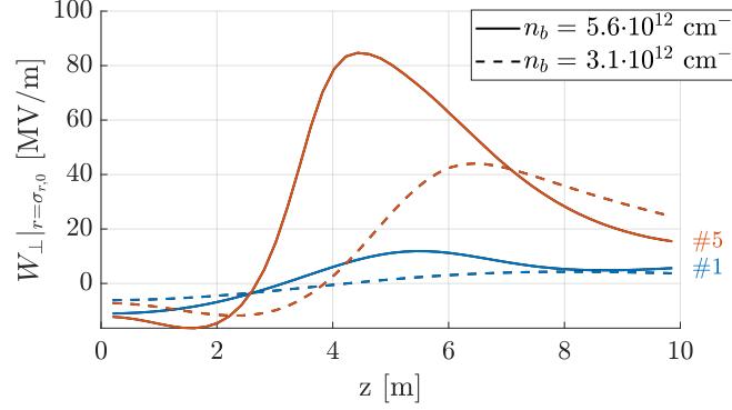
Figure 6.7: Transverse wakefield W_{\perp} at r = \sigma_{r,0} of defocused proton distributions of the first (blue lines) and fifth (red lines) period as a function of distance in plasma z with n_b = 5.6 \cdot 10^{12} \text{ cm}^{-3} (solid lines) and n_b = 3.1 \cdot 10^{12} \text{ cm}^{-3} (dashed lines). Here, n_{pe} = 0.92 \cdot 10^{14} \text{ cm}^{-3} and \Delta n_{pe} = 0 .
