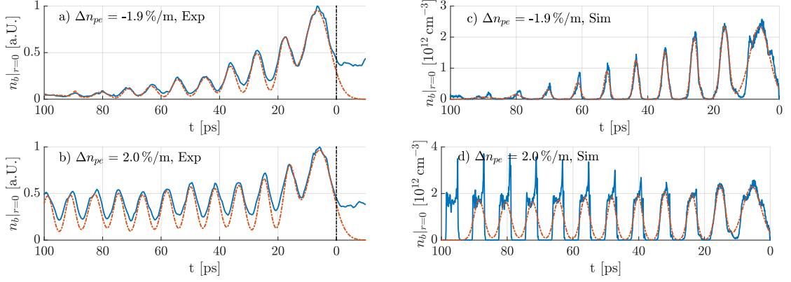
Figure 5.14: On-axis charge density (blue curves) with Gaussian fits to each micro-bunch (red curves) for plasma density gradient \Delta n_{pe} = -1.9\%/m (a, c) and \Delta n_{pe} = 2.0\%/m (b, d), experimentally (a, b) and from simulations (c, d). Here, n_{pe,Entr.} = 1.8 \cdot 10^{14} \text{ cm}^{-3} and n_b = 5.6 \cdot 10^{12} \text{ cm}^{-3} .
