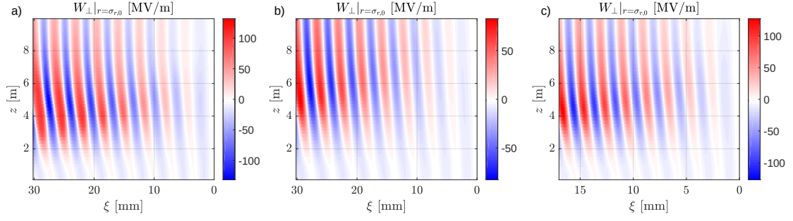
Figure A.25: Transverse wakefield at r = \sigma_{r,0} = 200 \mu\text{m} along the bunch \xi and along the plasma z for a) n_{pe} = 0.92 \cdot 10^{14} \text{ cm}^{-3} , n_b = 5.6 \cdot 10^{12} \text{ cm}^{-3} , b) n_{pe} = 0.92 \cdot 10^{14} \text{ cm}^{-3} , n_b = 3.1 \cdot 10^{12} \text{ cm}^{-3} , c) n_{pe} = 2.9 \cdot 10^{14} \text{ cm}^{-3} , n_b = 5.6 \cdot 10^{12} \text{ cm}^{-3} . Here, \Delta n_{pe} = 0 in all cases.
