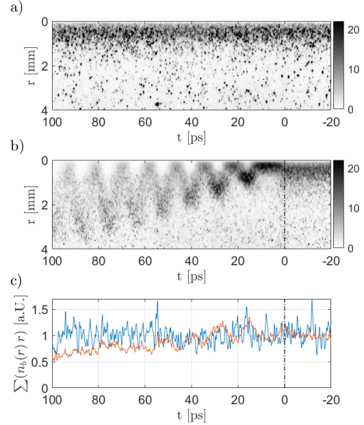
Figure 3.17: Streak camera image multiplied with transverse position (i.e. charge) of the a) unmodulated and b) modulated bunch; c) charge integrated over r \leq 4 mm of the unmodulated (blue line) and modulated (red line) bunch, both normalized to the mean value of the sum of the incoming bunch charge over -15 \text{ ps} \leq t \leq -4 \text{ ps} . Here, \xi_{Seed} = -0.1 \sigma_\xi and \sigma_\xi = 7.92 \text{ cm} \hat{=} \sigma_t = 264 \text{ ps} .
