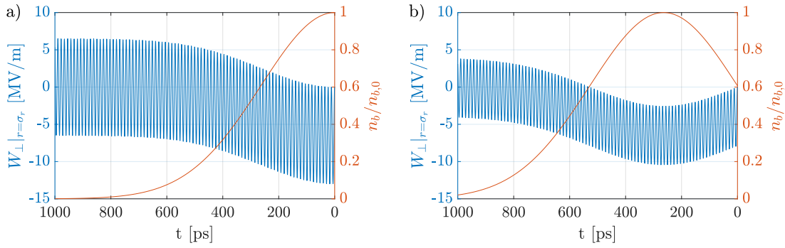
Figure 1.5: Transverse seed wakefield W_\perp|_{r=\sigma_r} (blue line) driven by the proton bunch with Gaussian bunch density profile n_b (normalized to peak density n_{b,0} , red line), propagating from left to right, with seeding (bunch cut) a) in the bunch center and b) 1\sigma_\xi ahead (right figure). Here N_{p+} = 2.8 \cdot 10^{11} , \sigma_r = 200 \mu\text{m} , \sigma_\xi = 7.92 \text{ cm} ( \hat{=} \sigma_t = 264 \text{ ps} ), i.e. n_{b,0} = 5.6 \cdot 10^{12} \text{ cm}^{-3} , and n_{pe} = 0.92 \cdot 10^{14} \text{ cm}^{-3} .
