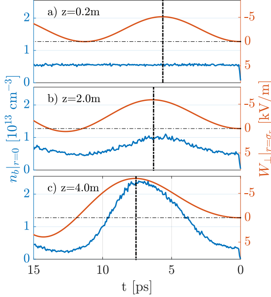
Figure 5.1: On-axis bunch density n_b|_{r=0} (blue lines) and transverse wakefield W_\perp|_{r=\sigma_r} (red lines) over the first modulation/wakefield period after a distance of 0.2 m (a), 2.0 m (b) and 4.0 m (c) in plasma, obtained from the simulation with parameters of Table 4.4, i.e. \tau_{pe} = 11.6 ps.
