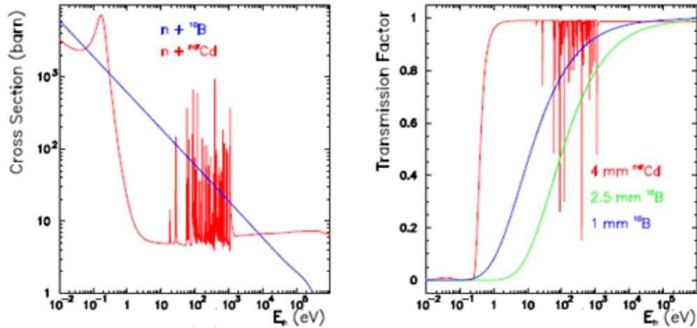
Figure 3.1: The total neutron induced cross section on ^{nat}\text{Cd} and on ^{10}\text{B} , taken from ENDF/B-VI [105] (left), together with the calculated transmission of the overlap filters [35] (right).
