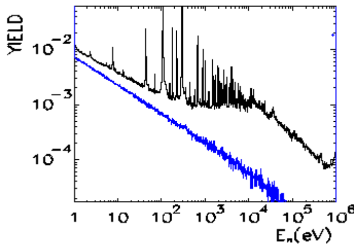
Figure 5.12 Capture yield of the sample used for the ^{93}\text{Zr}(n,\gamma) measurement (black) and background due to the activity of the sample
