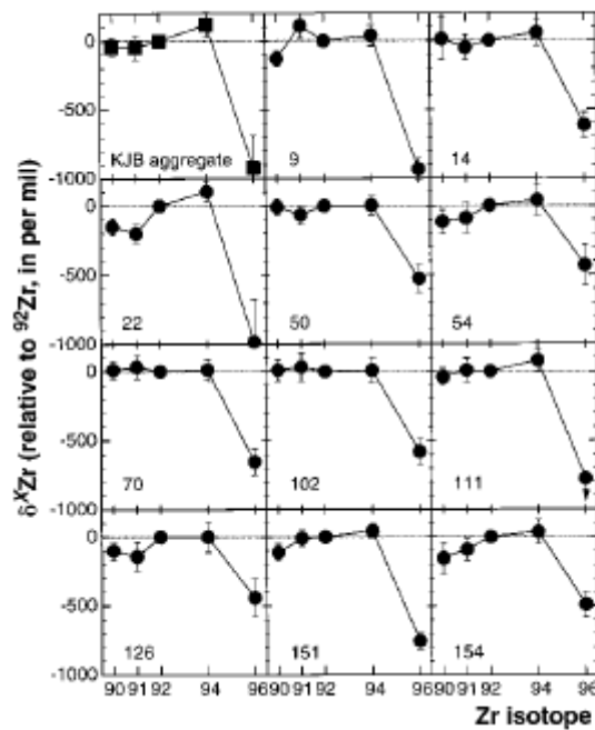
Figure 2.4 Zirconium isotopes patterns as function of mass for single SiC grains (circles) and an aggregate SiC grain (squares) from the Murchison meteorite. The graphs are in the \delta notation (see § 6.3.2 for more details). The number in the bottom left of each plot indicate the number of SiC grains (200 single SiC where isolated from the meteorite). For grain 111, a 2\sigma upper limit for \delta^{96}\text{Zr} is indicated by an arrow. (Picture from [129])
