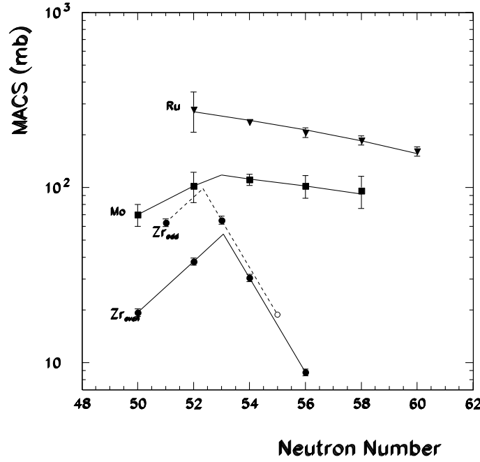
Figure 6.8. Experimental and calculated Maxwellian-averaged capture cross sections in the mass region 90 < A < 102 versus neutron number. Open symbol denote the calculated cross section for the ^{95}\text{Zr} . Even isotopes are connected with solid line, odd isotopes with dashed line.
