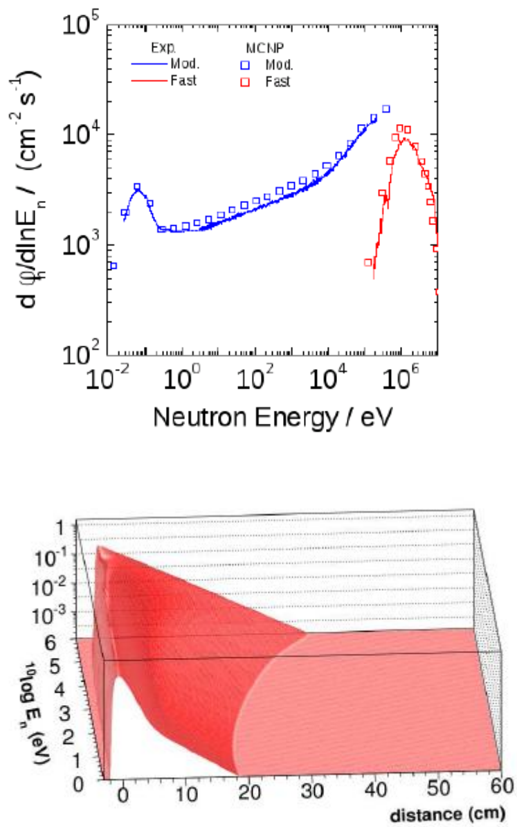
Figura 3.8 The Gelina neutron flux obtained by means of simulations and measurements, top part, and the energy resolution at flight path FP15-30 m, lower part, [47, 48]
