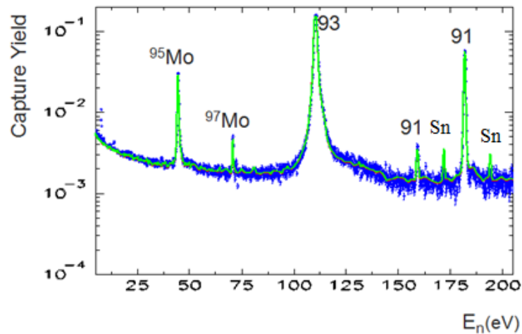
Figura 5.13 Capture yield of the sample of Zr in the neutron energy range 0,25 eV – 200 eV. Besides the contamination of the other Zr isotopes also the contribution due to other impurities, (Mo e Sn in the Fig) is clear. Although, the sample contains less than 1% of these elements, at low energy their contributions cannot be neglected.
