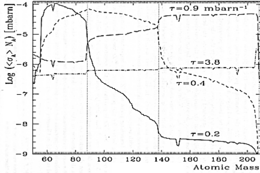
Figure 1.9 The \langle\sigma_A\rangle N_A distribution produced by the s-process after different neutron exposures as function of the atomic mass A . Neutron-capture cross section values are chosen for a temperature of 8 keV, corresponding to \approx 9 \times 10^7 K. Difference distributions are obtained for different values of the neutron exposure \tau , as indicated. Dotted lines are drawn in correspondence to the magic neutron nuclei ^{88}\text{Sr} , ^{138}\text{Ba} , and ^{208}\text{Pb} . Local equilibrium \langle\sigma_A\rangle N_A \approx \text{constant} is roughly verified far from nuclei with magic neutron numbers. Higher neutron exposures produce heavier nuclei as the bottlenecks at magic neutron numbers are more easily bypassed. (Picture from [14])
