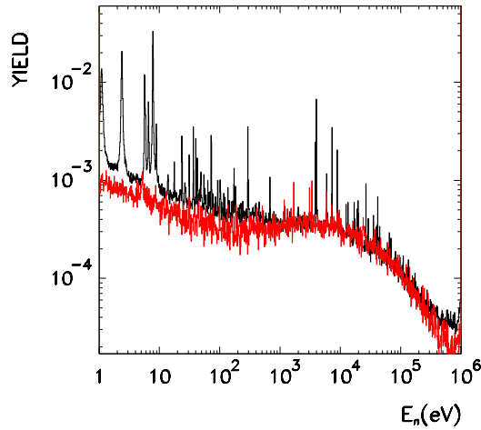
Figure 5.1: The ^{90}\text{Zr}(n,\gamma)^{91}\text{Zr} normalized yield (black) and the overall background (red)
