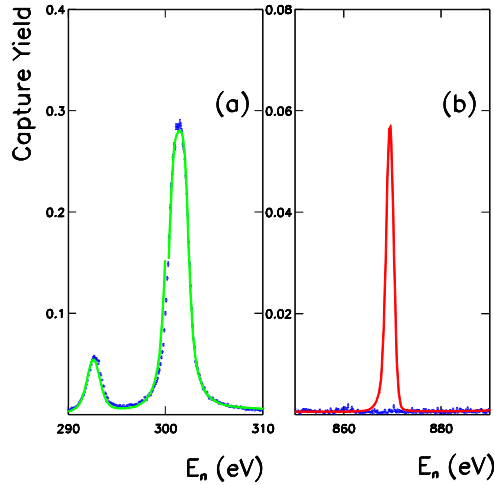
Figure 5.17: ^{96}\text{Zr} capture yield as a function of the energy of incident neutrons ( E_n ). Examples for fits with the R-matrix code SAMMY; in the panel (b) a previously reported resonance [79] that was not observed in this work is drawn (red) using the parameters listed in the JENDL3.3 compilation [88].
