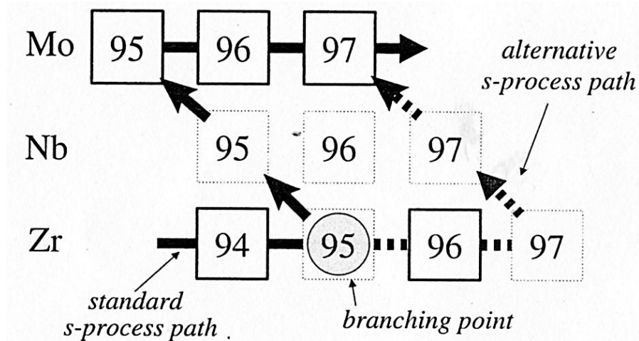
Figure 1.10 Section of the nuclide chart showing the branching path that is open in ^{95}\text{Zr} in conditions of high neutron density. When the branching is open, part of the flux goes through ^{96}\text{Zr} , skipping ^{95}\text{Mo} and ^{96}\text{Mo} . (Picture from [14])
