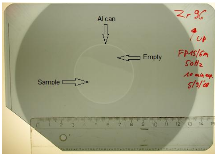
Figure 5.20 X-ray scan of the ^{96}\text{Zr} sample used in the GELINA.
