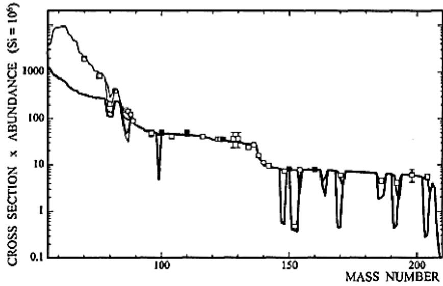
Fig 2.1 The product N_0\langle\sigma\rangle_A (in units of millibarn per 10^6 Si atoms ) of solar system s-process abundance and Maxwellian-averaged cross section (at thermal energy of kT = 30 keV) versus mass number A . The symbols correspond to s-only nuclides. The solid curves are obtained fitting the data to an expression similar to Eq. (2.1) but which includes the effect of significant s-process branching. The thick solid line is calculated by using a single exponential distribution neutron exposure (main s-process component). For A \leq 90 , the main component falls below the data points and a second distribution (weak s-process component) must be included in the fit (thin solid line). The sharp structures result from s-process branching. (Picture from [7])
