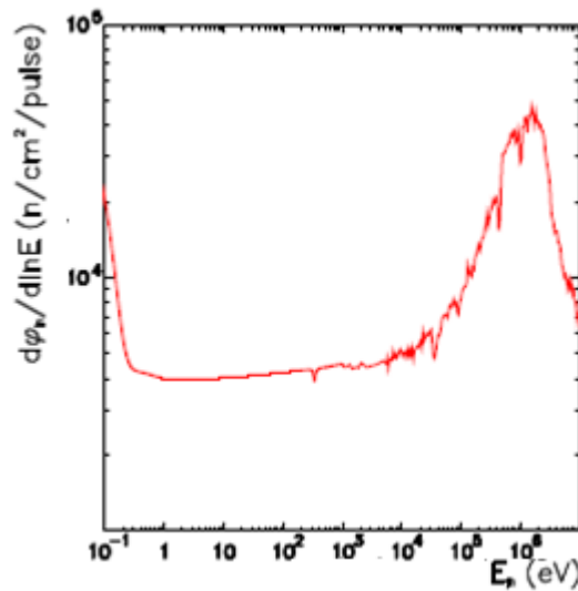
Figure 3.3 The n_TOF neutron flux per bunch at the sample position in the experimental area at 185 m from the spallation target for a standard pulse of 7 \times 10^{12} protons.
