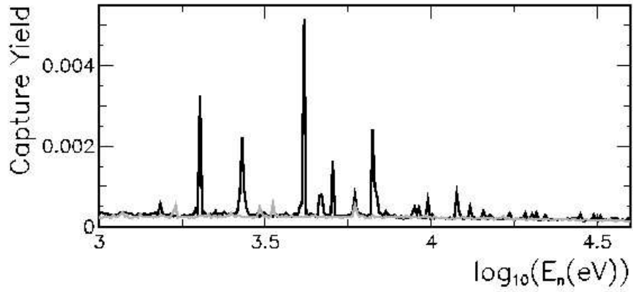
Figure 5.9: ^{92}\text{Zr} capture yield (black) and overall background (gray) in the investigated energy range ( 1 \text{ keV} < E_n < 40 \text{ keV} ).
