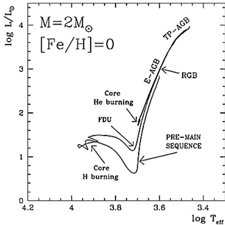
Figura 1.3 Hertzsprung-Russell diagram, in which the stellar luminosity (on a \text{Log}_{10} scale) is plotted as a function of the effective (i.e. surface) temperature also in ( \text{Log}_{10} scale) and decreasing to the right, showing the theoretical evolution of a star of initial M = 2M_{\odot} and solar metallicity. The label FDU is for first dredge up, RGB is for red giant branch, E-AGB if for early Asymptotic Giant Branch, TP-AGB is for thermally pulsing Asymptotic Giant Branch[13]. The meaning of dredge up will be explained further in this paragraph.
