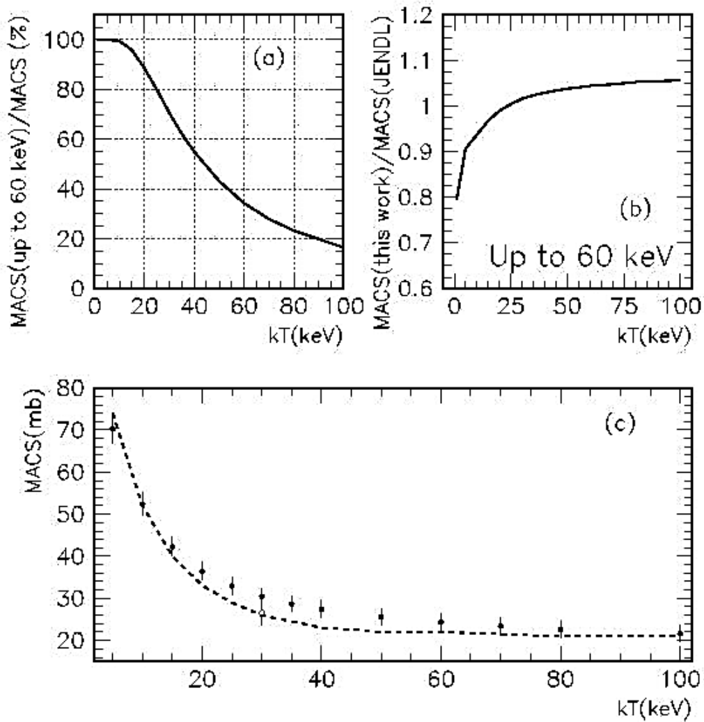
Figure 6.6 ^{94}\text{Zr} (a) Relative contribution to MACS as a function of the upper integration limit; (b) Ratio between MACS extracted from the present work and those evaluated in the JENDL library [88], limiting the calculation to the energy range [0, 60] keV, as a function of thermal energy; (c) MACS extracted in present work, complemented above 60 keV by means of JENDL evaluations (full points), as a function of thermal energy. The values at 30 keV extracted in Ref. [85] (open point) and those given by the compilation of Ref. [6] (dashed line) are also reported.
