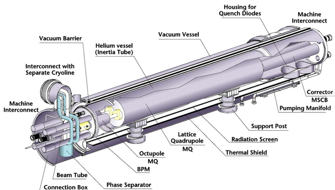
Fig. 2.5 Short Straight Section 3-D cross-section. Source: CERN.
