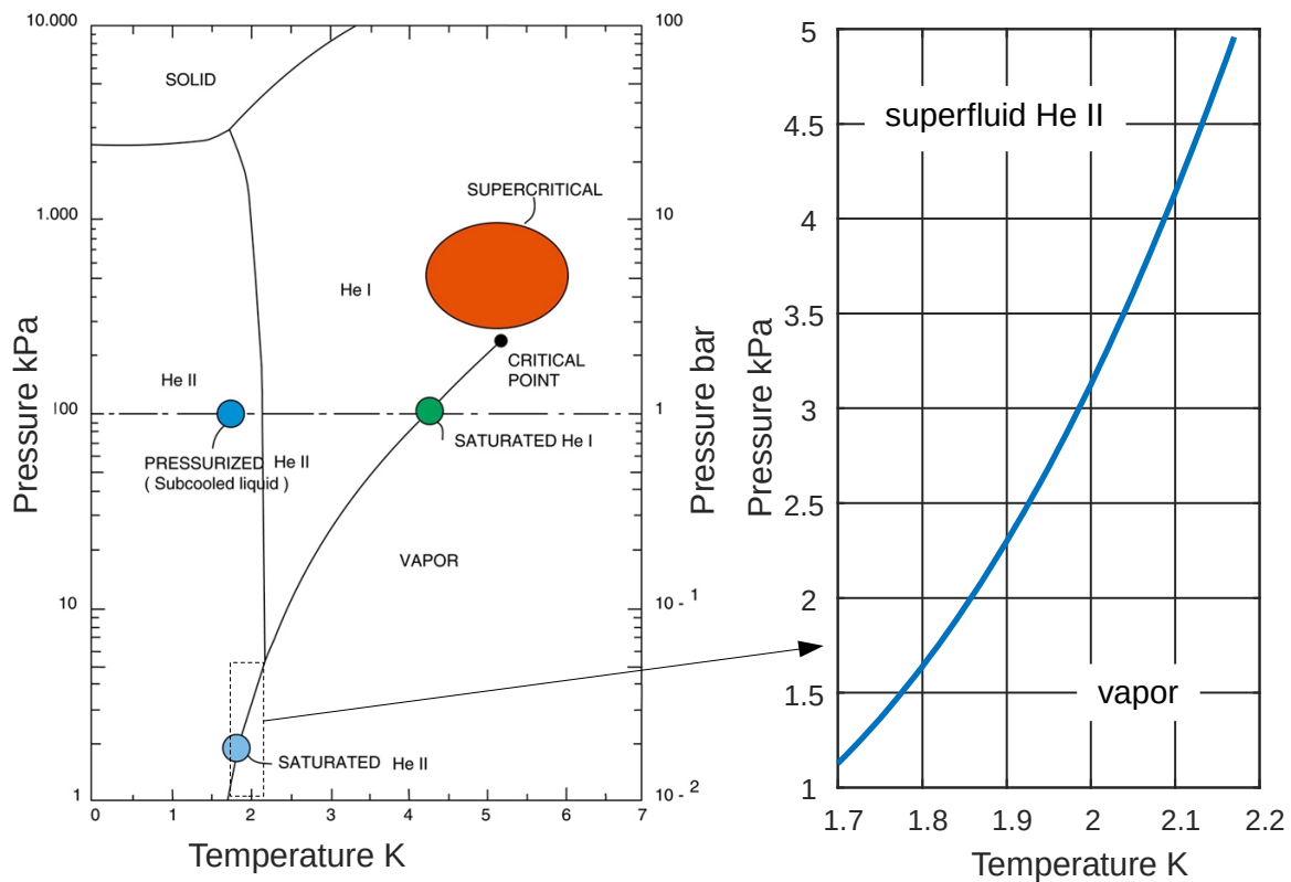
Fig. 2.3 Phase diagram of helium. Source: CERN.
