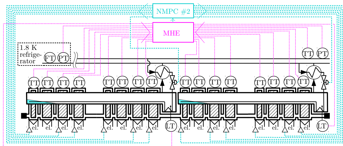
Fig. 7.3 NMPC formulations
