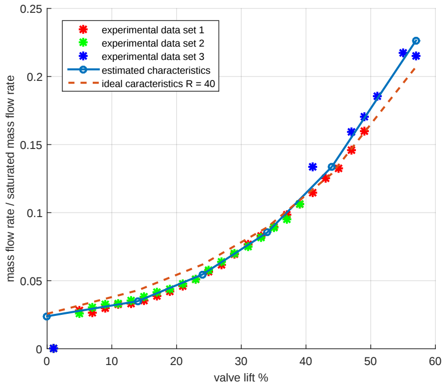
Fig. 5.15 Estimated and ideal valve characteristics
