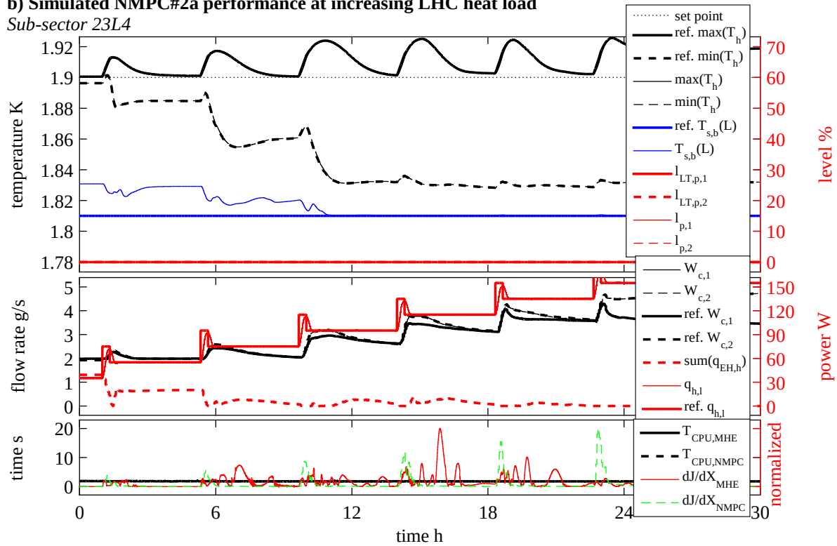
Fig. 8.2 Simulated NMPC #2a performance.
