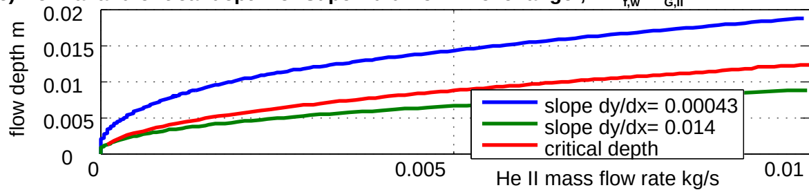
Fig. 5.12 Superfluid flow parameters in bayonet heat exchanger.
