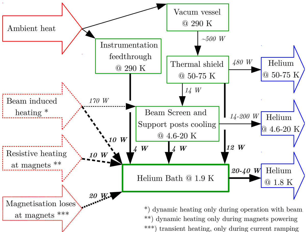
Fig. 5.5 Heat loads in a Standard Cell. Most values from Heat Load Working Group (2001) .
