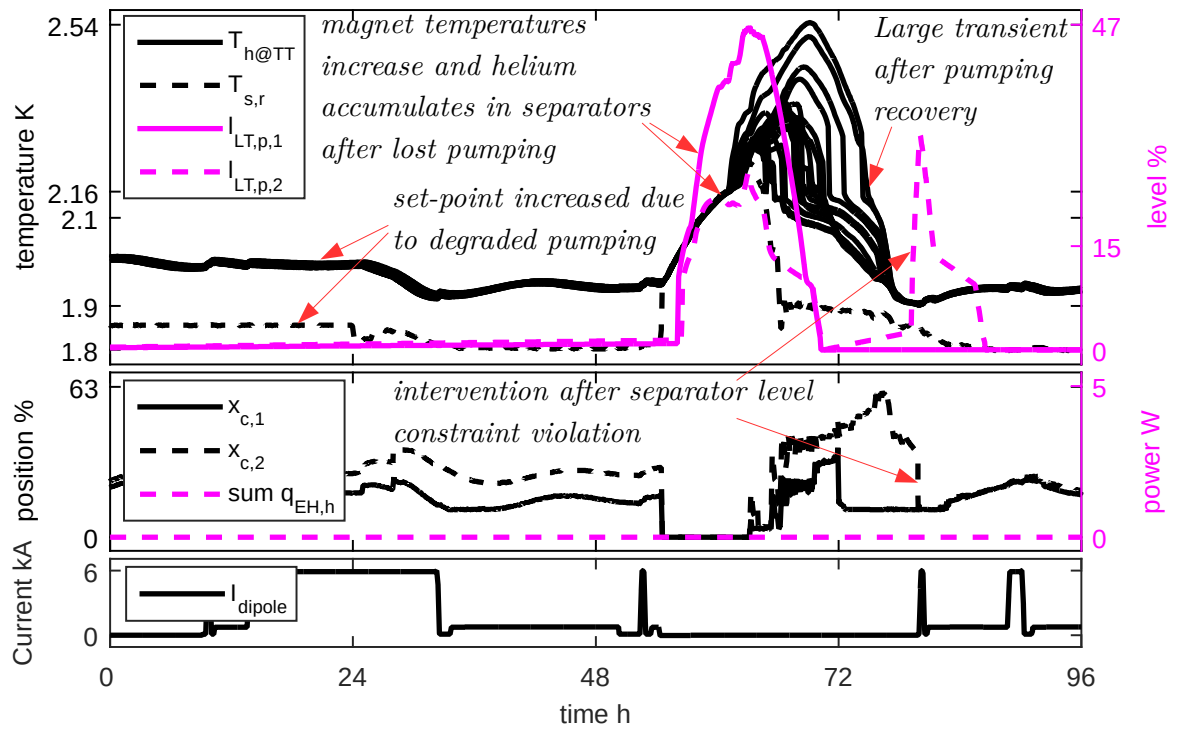
Fig. 2.14 LHC operation
