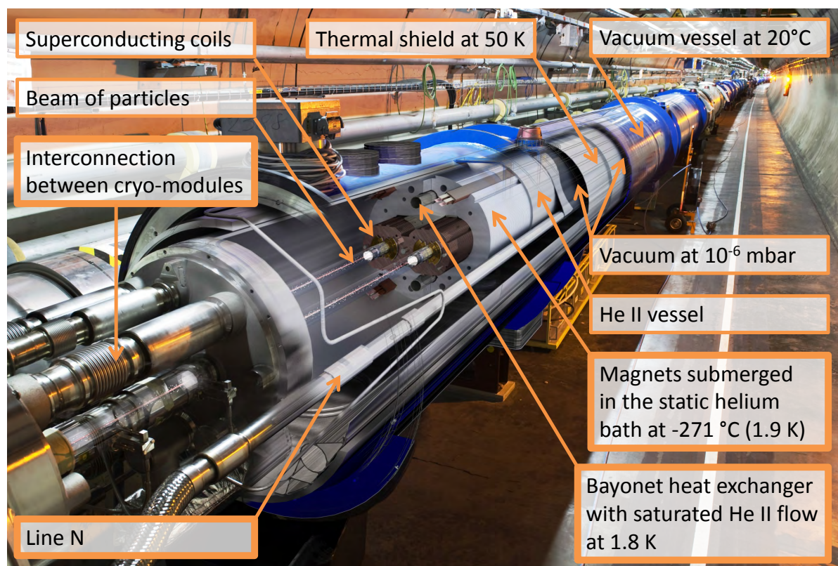
Fig. 2.1 The LHC in its tunnel and section through a cryo-dipole. Source of image: CERN
