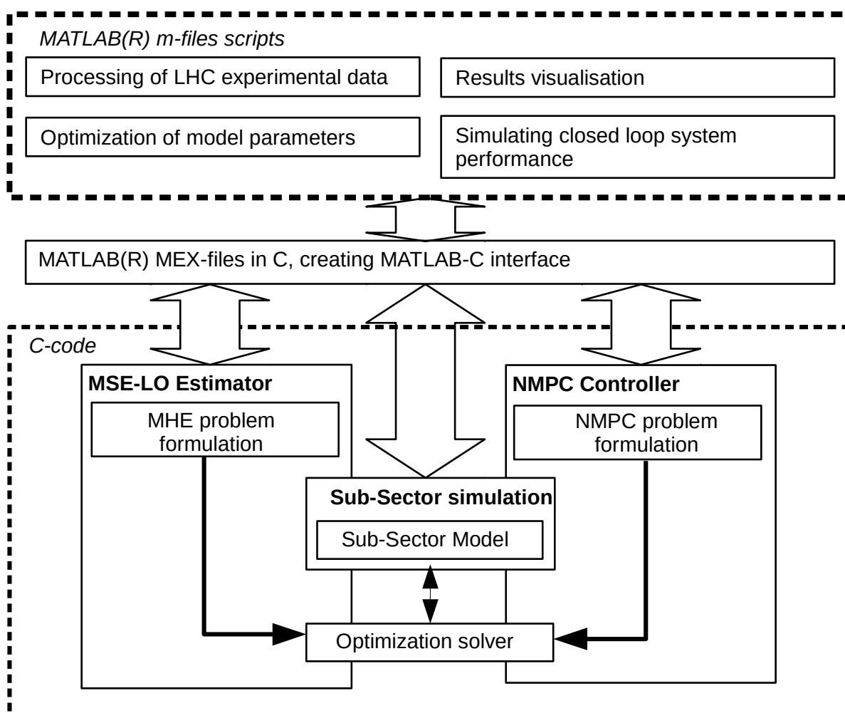
Fig. 6.3 Model implementation and integration in simulation environment.
