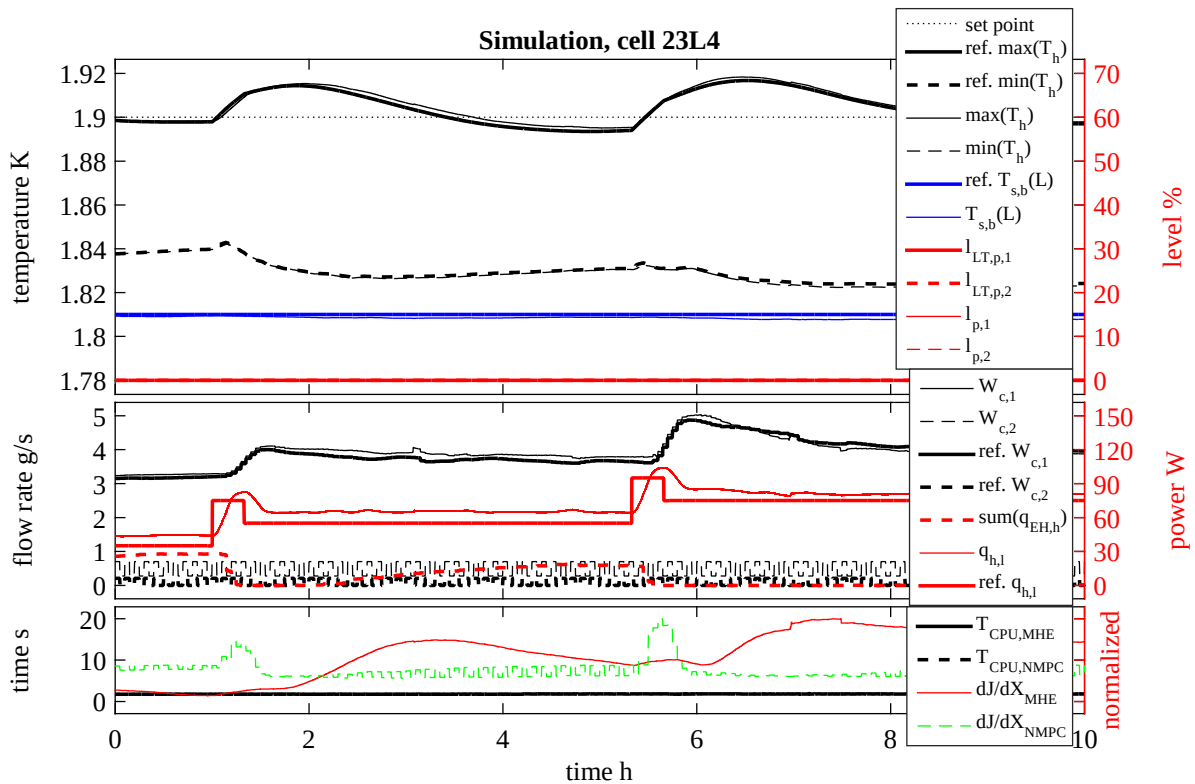
Fig. 8.6 Simulated NMPC #2a CV2 failure performance.
