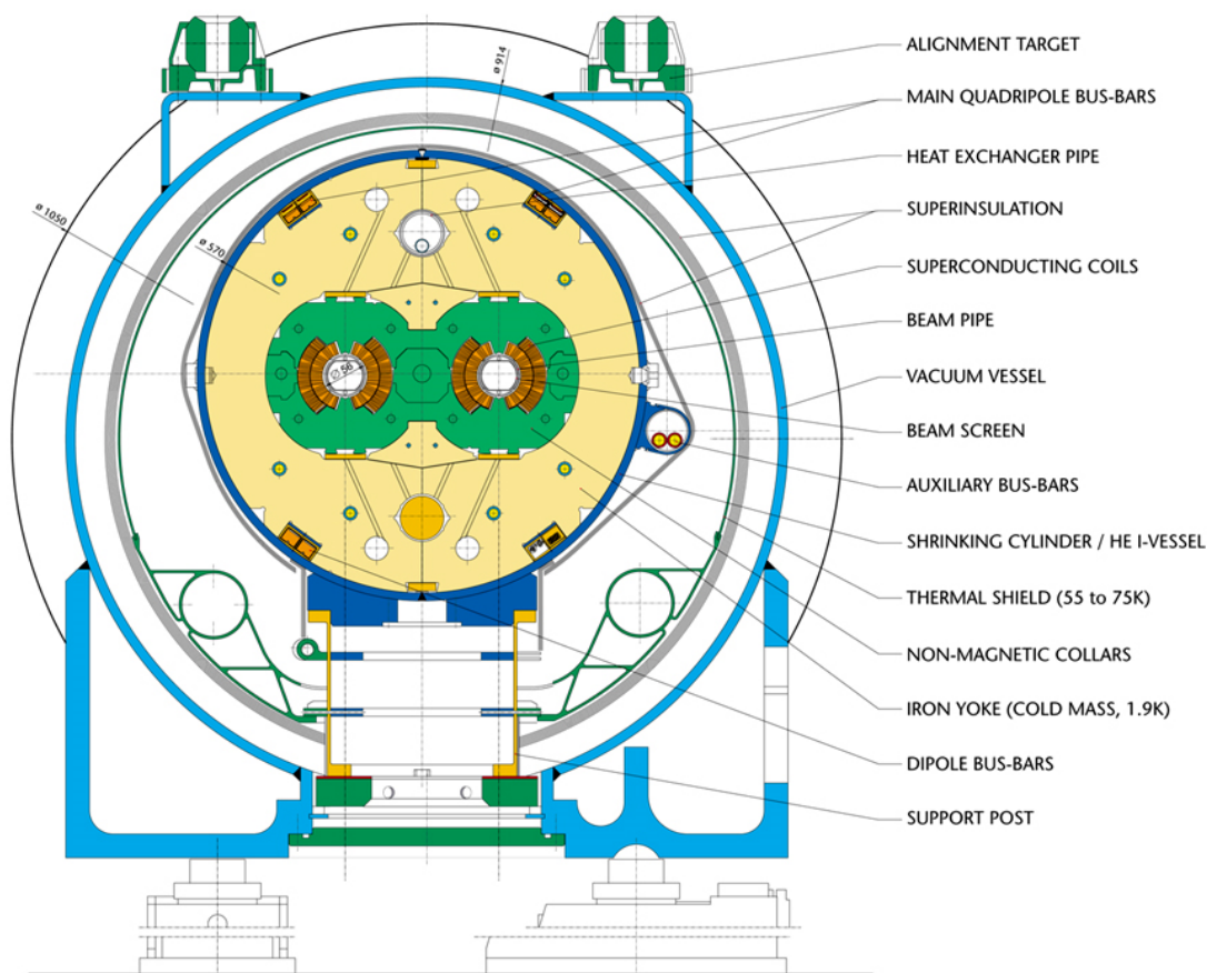
Fig. 2.4 Cryodipole cross-section. Image source: CERN.
