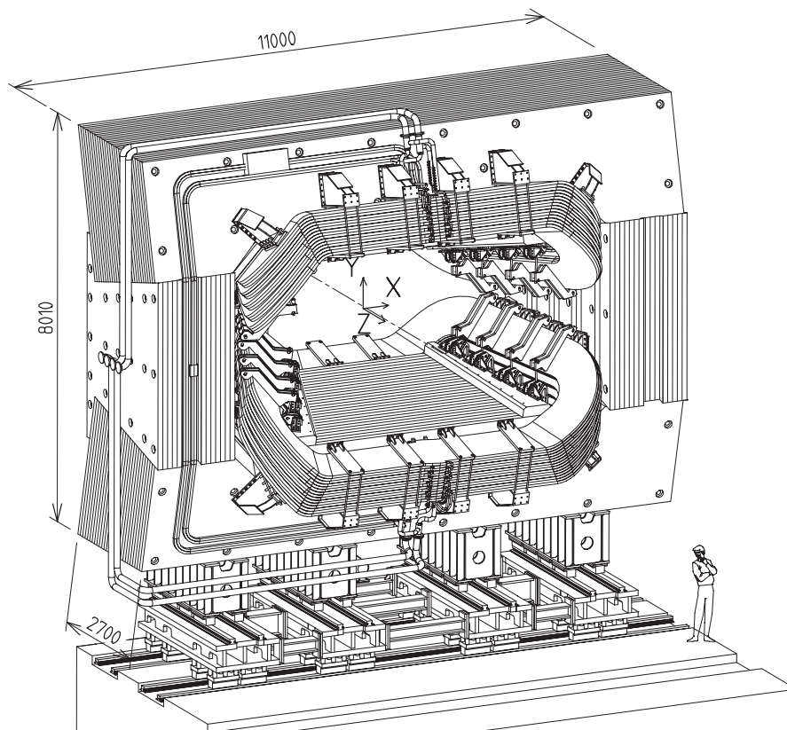
Figure 2.12: Perspective view of the LHCb dipole magnet.
