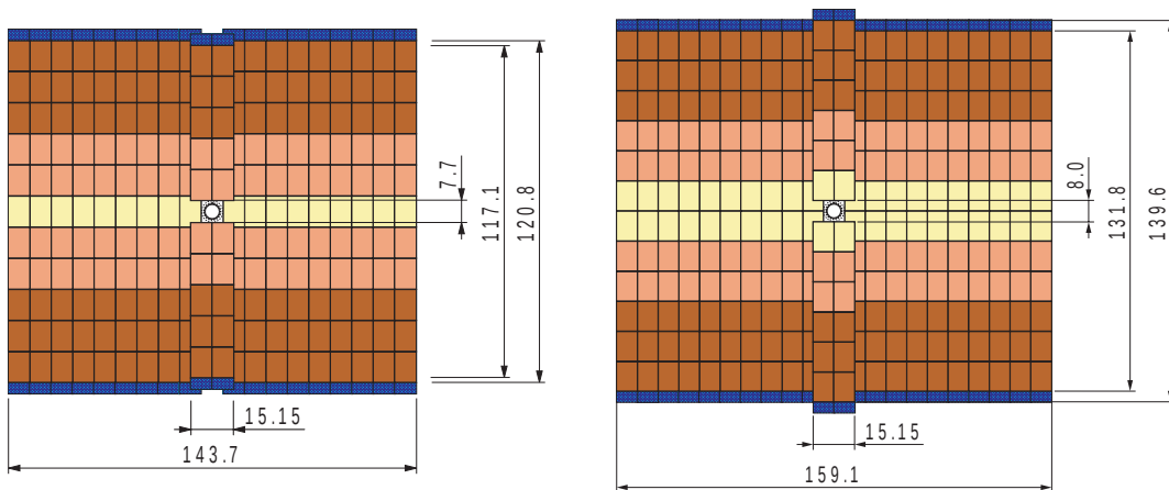
Figure 2.7: Layout of the x -layers of the TTa (left) and TTb (right) stations. Dimensions are reported in centimeters.
