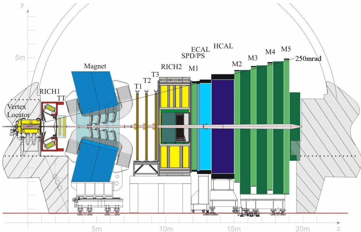
Figure 2.4: Side view of the LHCb detector in the (y, z) plane. The various sub-detectors are also shown and labelled.
