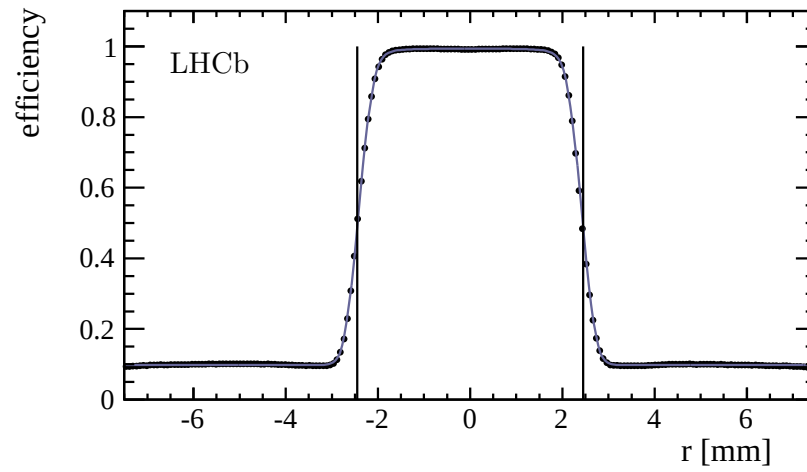
Figure 2.11: Hit efficiency in the OT modules as a function of the track distance from the center of the straw.
