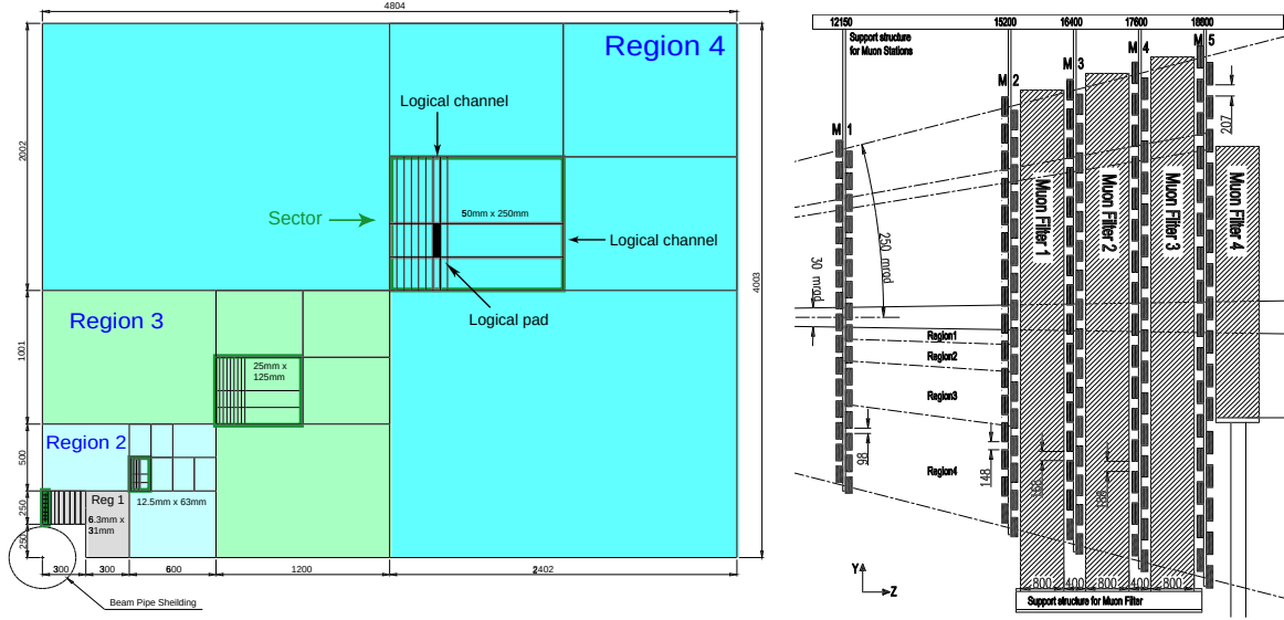
Figure 2.22: Left: front view of one stations of the muon system, where the segmentation in four regions can be seen. Right: side view of the muon system in the (y, z) plane.
