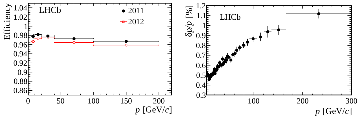
Figure 2.14: Tracking efficiency (left) and momentum resolution (right) as a function of particle momentum.
