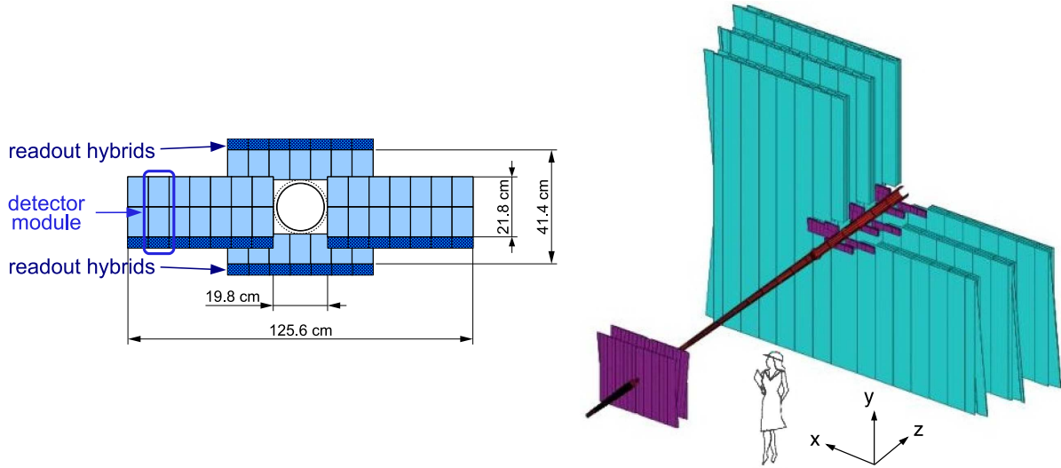
Figure 2.9: Left: view of one layer of the IT detector, with the four detector modules in a cross shape around the beam pipe. Right: arrangement of the OT modules and layers in cyan, with the IT stations in purple.
