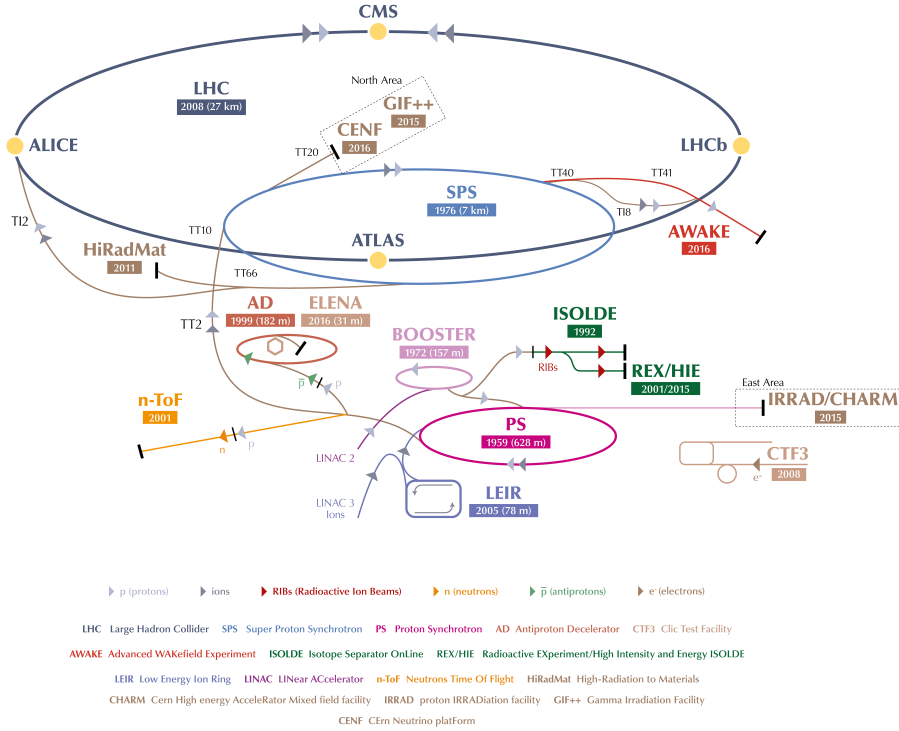
Figure 2.1: The CERN accelerator complex [88].
