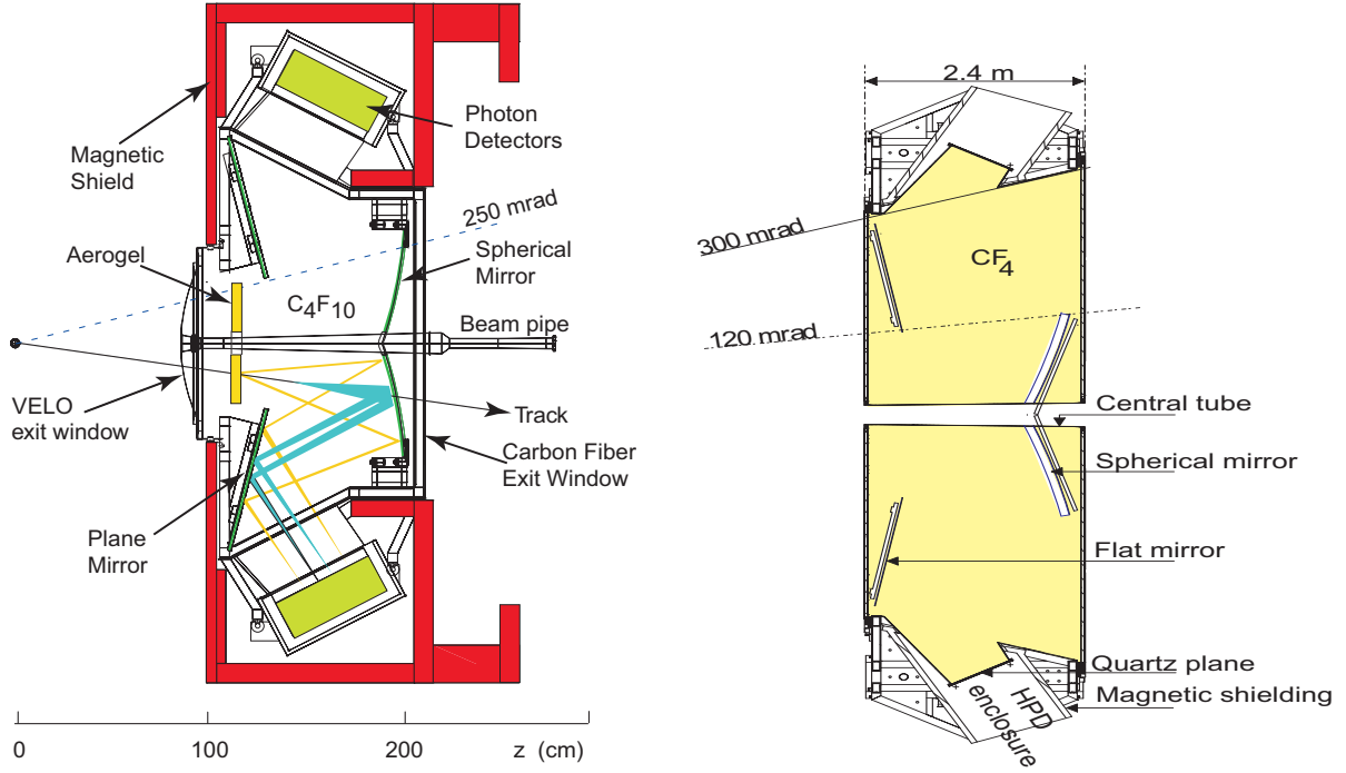
Figure 2.15: Side view of the (left) RICH1 detector and (right) RICH2 detector.
