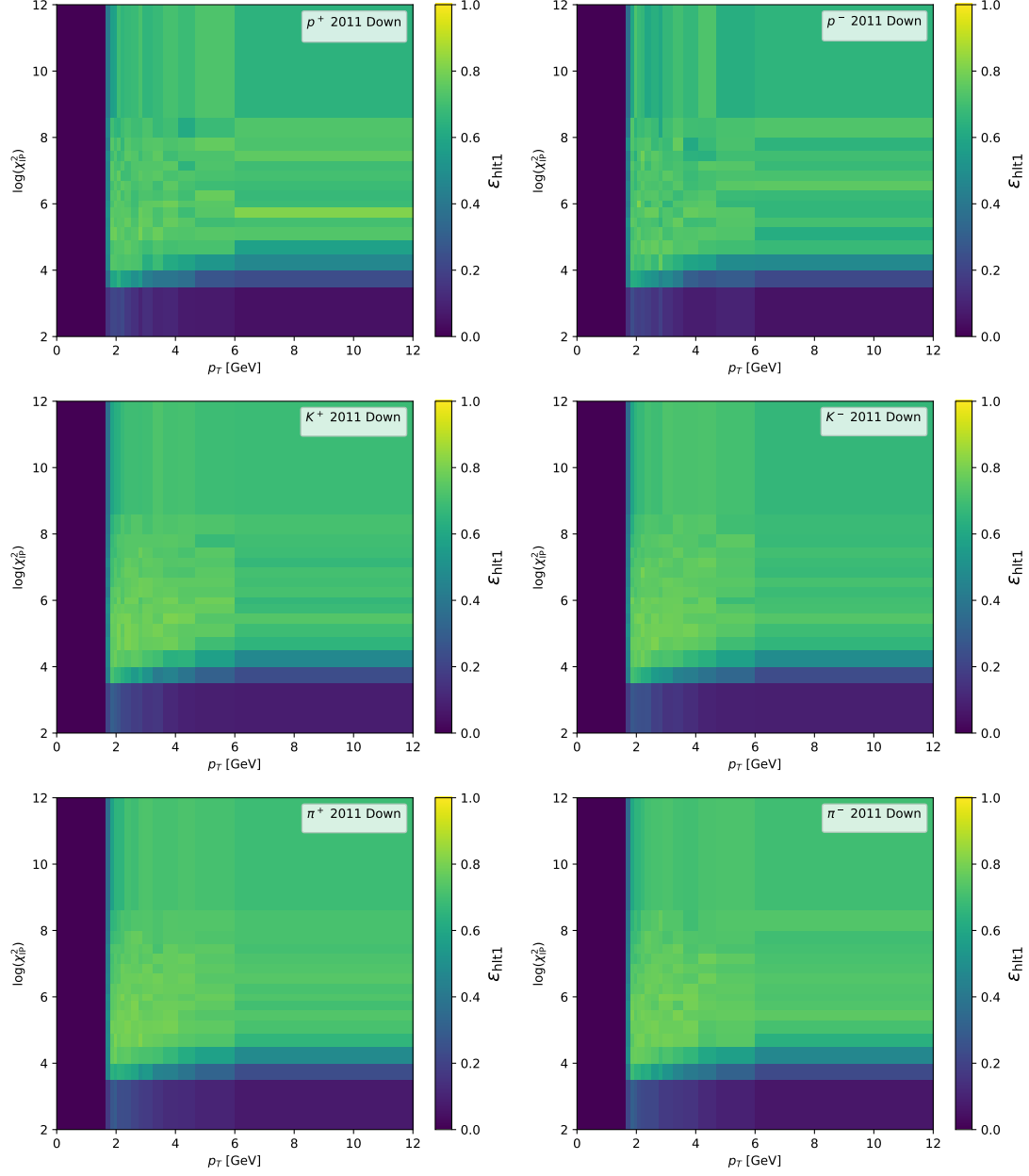
Figure C.2: Hlt1_TrackMVA efficiency as a function of p_T and \log(\chi_{\text{IP}}^2) for (top row) protons, (middle row) kaons, and (bottom row) pions of (left) positive and (right) negative charge. These are the plots for the 2011 magnet Down sample.
