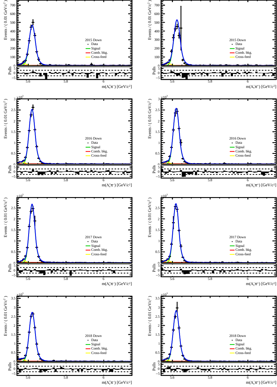
Figure D.2: Fits to the invariant-mass distributions of (left) \Lambda_b^0 \rightarrow \Lambda_c^+ \pi^- and (right) \Lambda_b^0 \rightarrow \Lambda_c^- \pi^+ decays for the years from 2015 to 2018 magnet Down from top to bottom; the plots are in linear scale.
