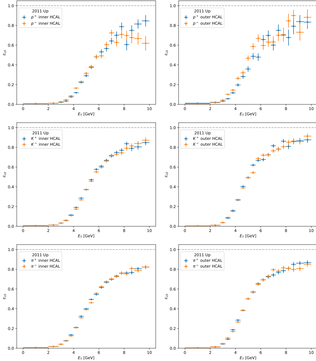
Figure B.1: L0_Hadron efficiency as a function of E_T for (top row) protons, (middle row) kaons, and (bottom row) pions hitting the (left) inner and (right) outer region of HCAL. These are the plots for the 2011 magnet Up sample.
