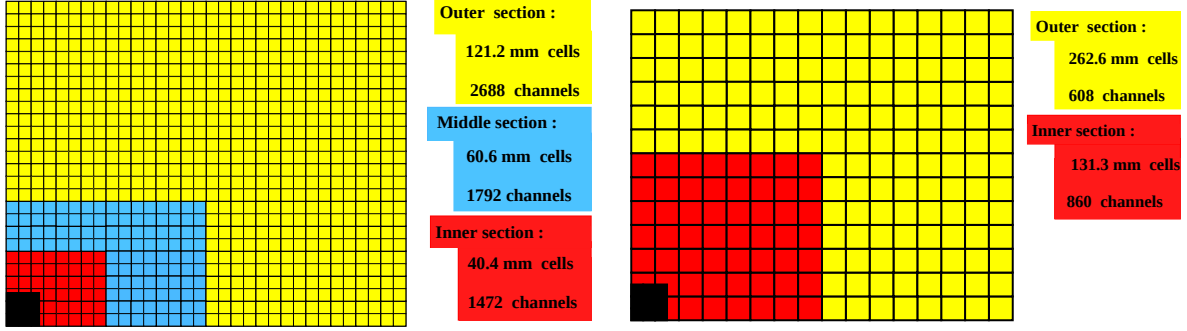
Figure 2.18: Lateral segmentation of one quarter of the (left) SPD, PS, and ECAL and (right) HCAL. The cell dimension must be reduced by about 1.5% for SPD and PS.
