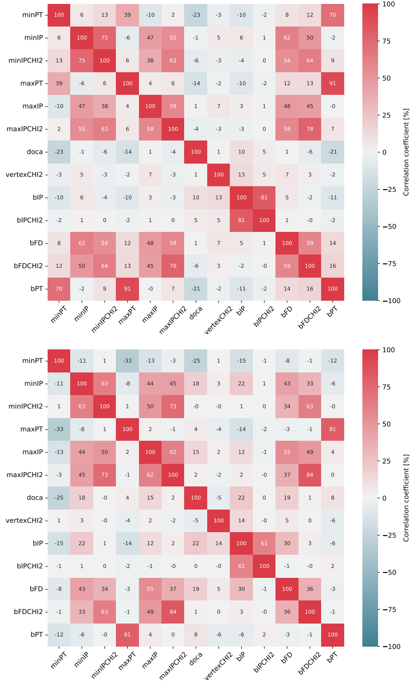
Figure 3.13: Correlation matrices of the variables used to train the BDT for (top) signal and (bottom) background samples. The dataset corresponds to a particular set of cuts for Selection A.
