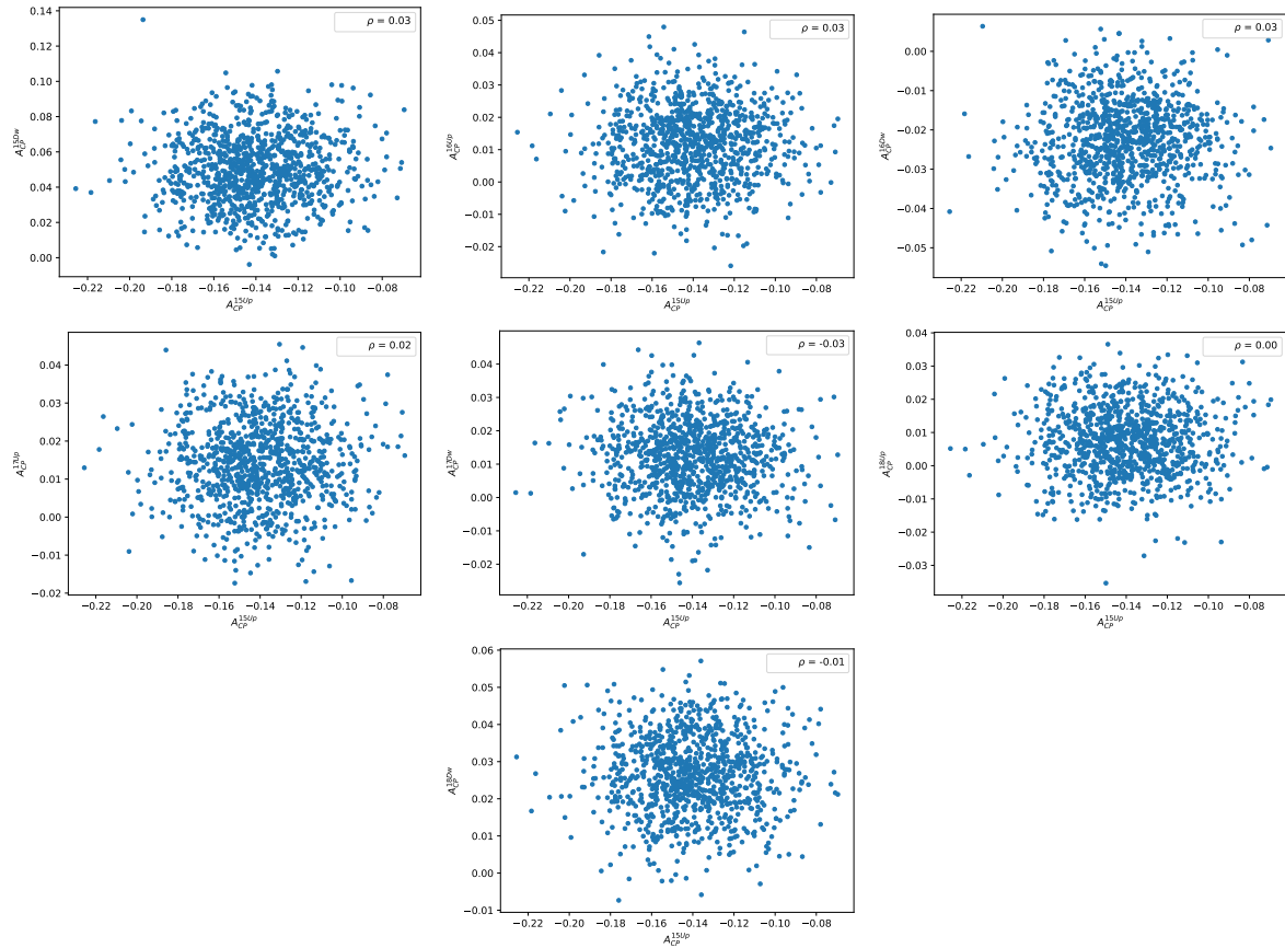
Figure E.5: Scatter plots of the 1000 values of A_{CP}(pK^-) obtained from the pseudoexperiments in the 2015 magnet Up sample and the other subsamples. The correlation coefficient is shown in the upper right corner of each plot.
