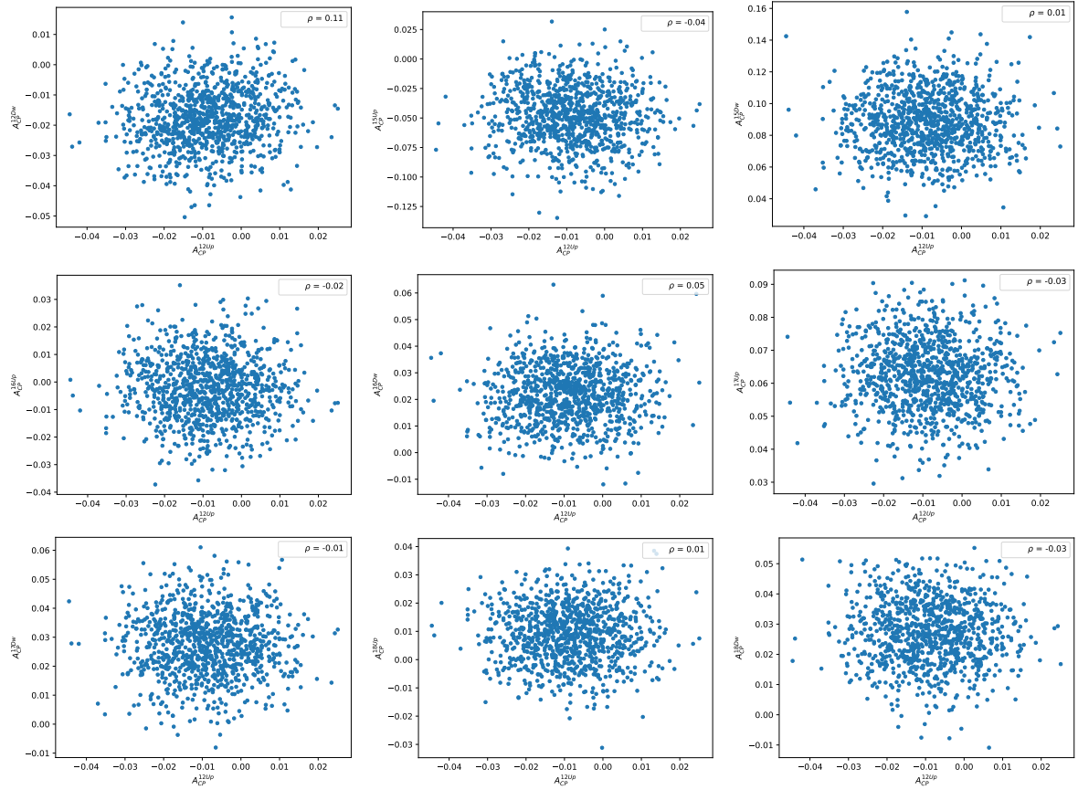
Figure E.13: Scatter plots of the 1000 values of A_{CP}(p\pi^-) obtained from the pseudoexperiments in the 2012 magnet Up sample and the other subsamples. The correlation coefficient is shown in the upper right corner of each plot.
