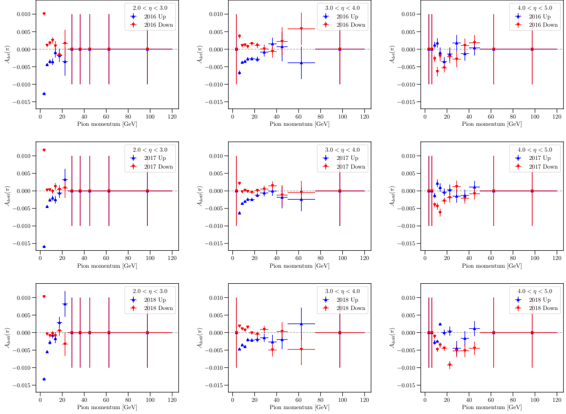
Figure 3.29: Values of the pion interaction asymmetry in (top) 2016, (middle) 2017, and (bottom) 2018, for increasing pseudorapidity from left to right, separated by magnet polarity.
