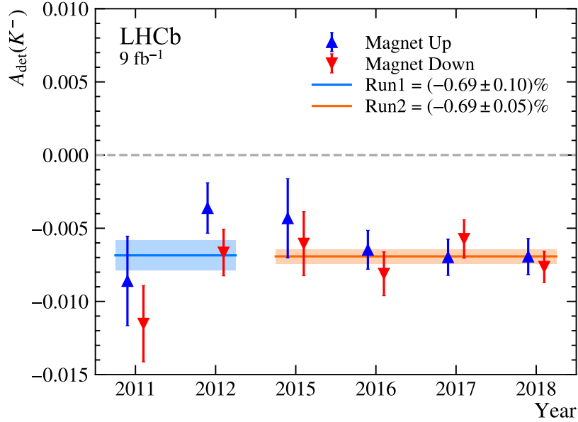
Figure 3.33: Values of A_D(K^-) reweighted over the signal \Lambda_b^0 \rightarrow pK^- sample's kinematics, separated by year and magnet polarity.
