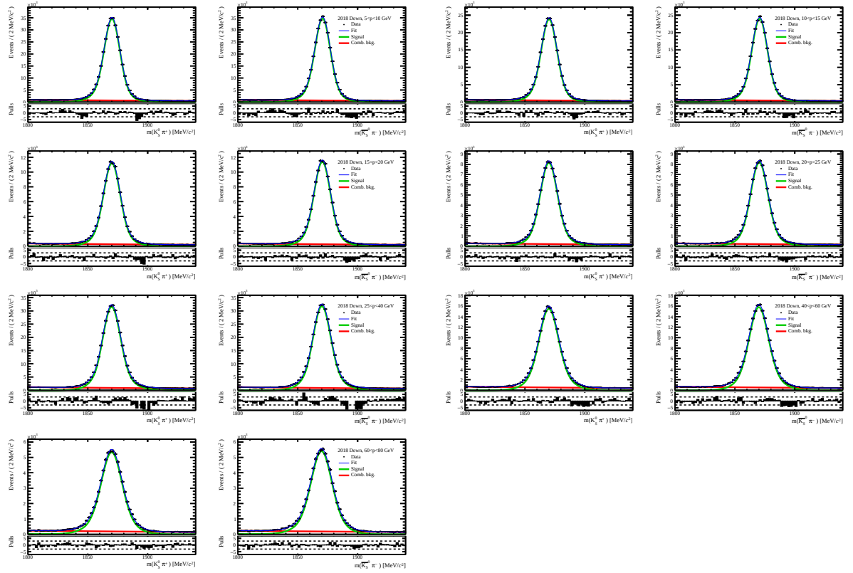
Figure 74: Fits to the invariant-mass distributions of (left of the pair) K_S^0 \pi^+ and (right of the pair) K_S^0 \pi^- decays in the year 2018 and magnet polarity down sample. The samples are divided in bins of kaon momentum, from lowest to highest from the top to the bottom and from left to right.
