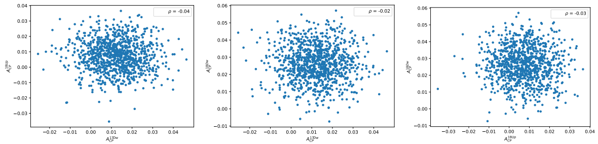
Figure E.10: Scatter plots of the 1000 values of A_{CP}(pK^-) obtained from the pseudoexperiments in the 2017 magnet Down sample and 2018 magnet Up and the other subsamples. The correlation coefficient is shown in the upper right corner of each plot.
