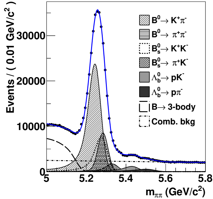
Figure 3.10: Invariant-mass distribution of H_b \rightarrow h^+ h'^- candidates reconstructed under the \pi^+ \pi^- invariant-mass hypothesis. The results of the best fit are superimposed. No PID requirements are imposed on the events, whereas a cut on the BDT classifier is requested. No H_b \rightarrow h^+ h'^- events are present above 5.6 \text{ GeV}/c^2 .
