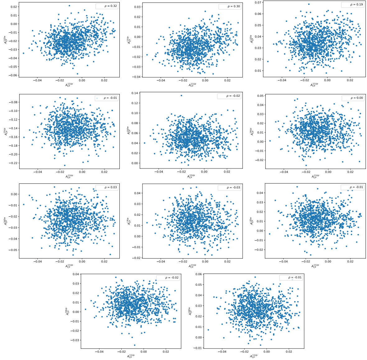
Figure E.1: Scatter plots of the 1000 values of A_{CP}(pK^-) obtained from the pseudoexperiments in the 2011 magnet Up sample and the other subsamples. The correlation coefficient is shown in the upper right corner of each plot.
