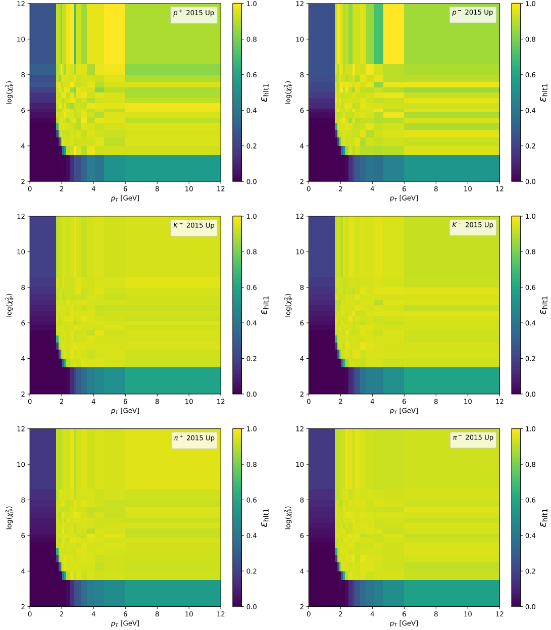
Figure C.5: HLT1_TrackMVA efficiency as a function of p_T and \log(\chi_{\text{IP}}^2) for (top row) protons, (middle row) kaons, and (bottom row) pions of (left) positive and (right) negative charge. These are the plots for the 2015 magnet Up sample.
