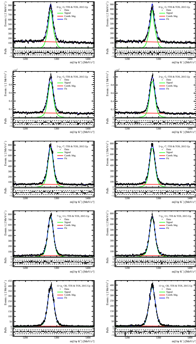
Figure A.17: Fits to the invariant-mass distributions of (left) J/\psi K^+ and (right) J/\psi K^- decays in the trigger category !TIS & TOS , year 2015, and magnet polarity up. The samples are divided in bins of B^+ transverse momentum, from lowest to highest from the top to the bottom.
