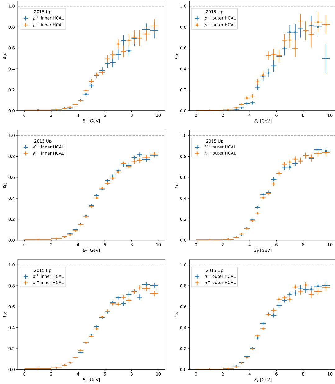
Figure B.5: L0_Hadron efficiency as a function of E_T for (top row) protons, (middle row) kaons, and (bottom row) pions hitting the (left) inner and (right) outer region of HCAL. These are the plots for the 2015 magnet Up sample.
