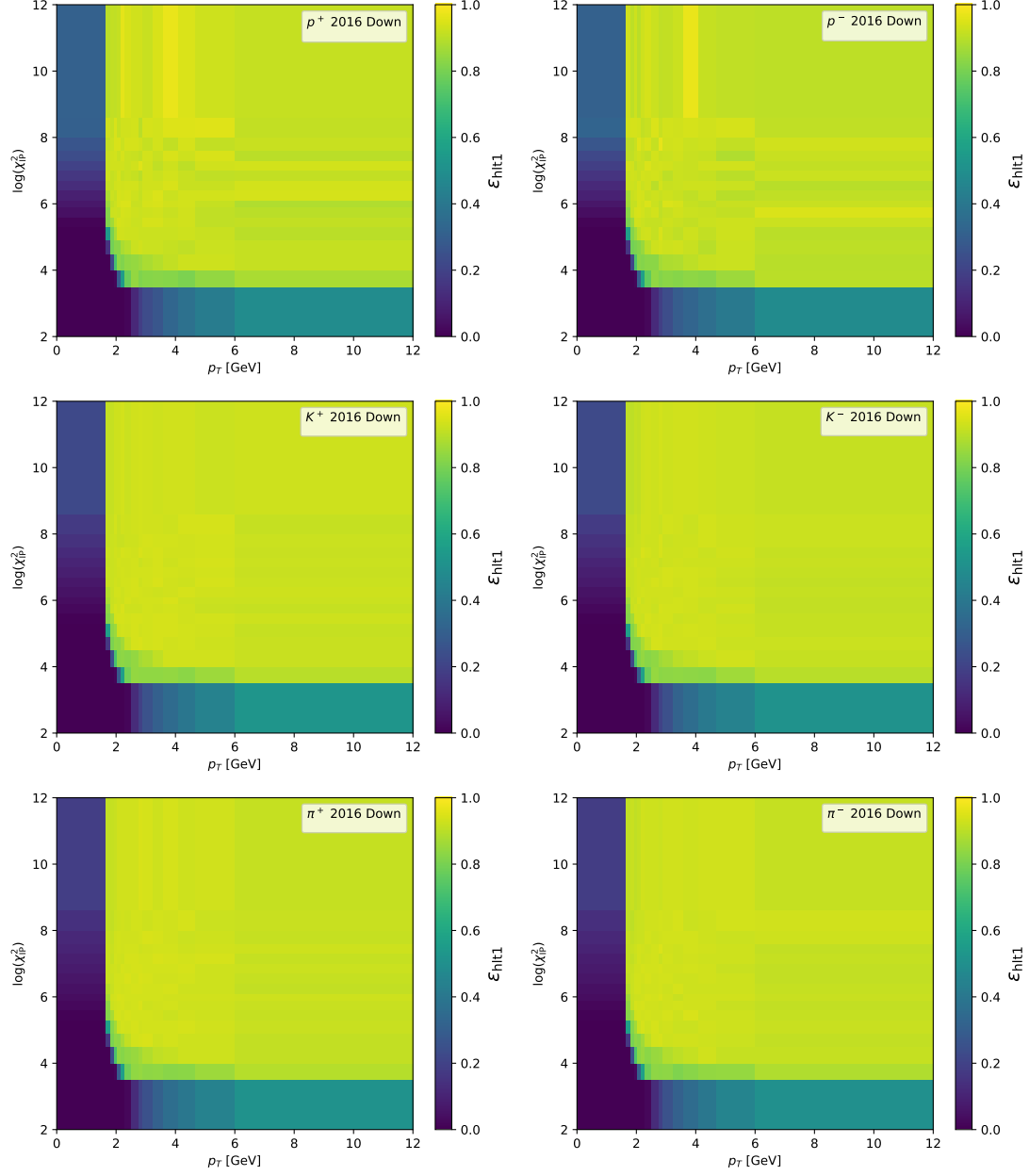
Figure C.8: Hlt1_TrackMVA efficiency as a function of p_T and \log(\chi_{IP}^2) for (top row) protons, (middle row) kaons, and (bottom row) pions of (left) positive and (right) negative charge. These are the plots for the 2016 magnet Down sample.
