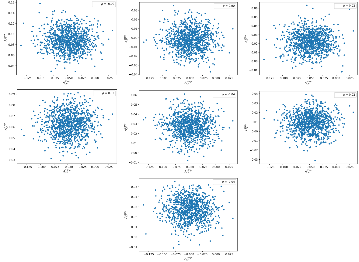
Figure E.15: Scatter plots of the 1000 values of A_{CP}(p\pi^-) obtained from the pseudoexperiments in the 2015 magnet Up sample and the other subsamples. The correlation coefficient is shown in the upper right corner of each plot.
