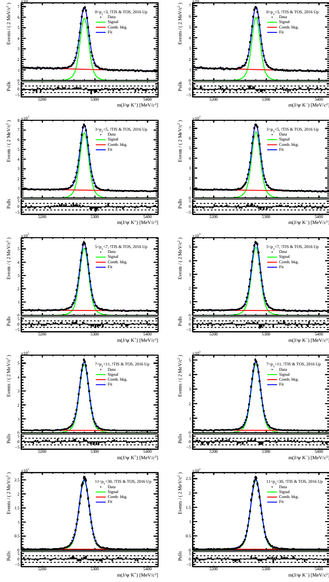
Figure A.19: Fits to the invariant-mass distributions of (left) J/\psi K^+ and (right) J/\psi K^- decays in the trigger category !TIS & TOS , year 2016, and magnet polarity up. The samples are divided in bins of B^+ transverse momentum, from lowest to highest from the top to the bottom.
