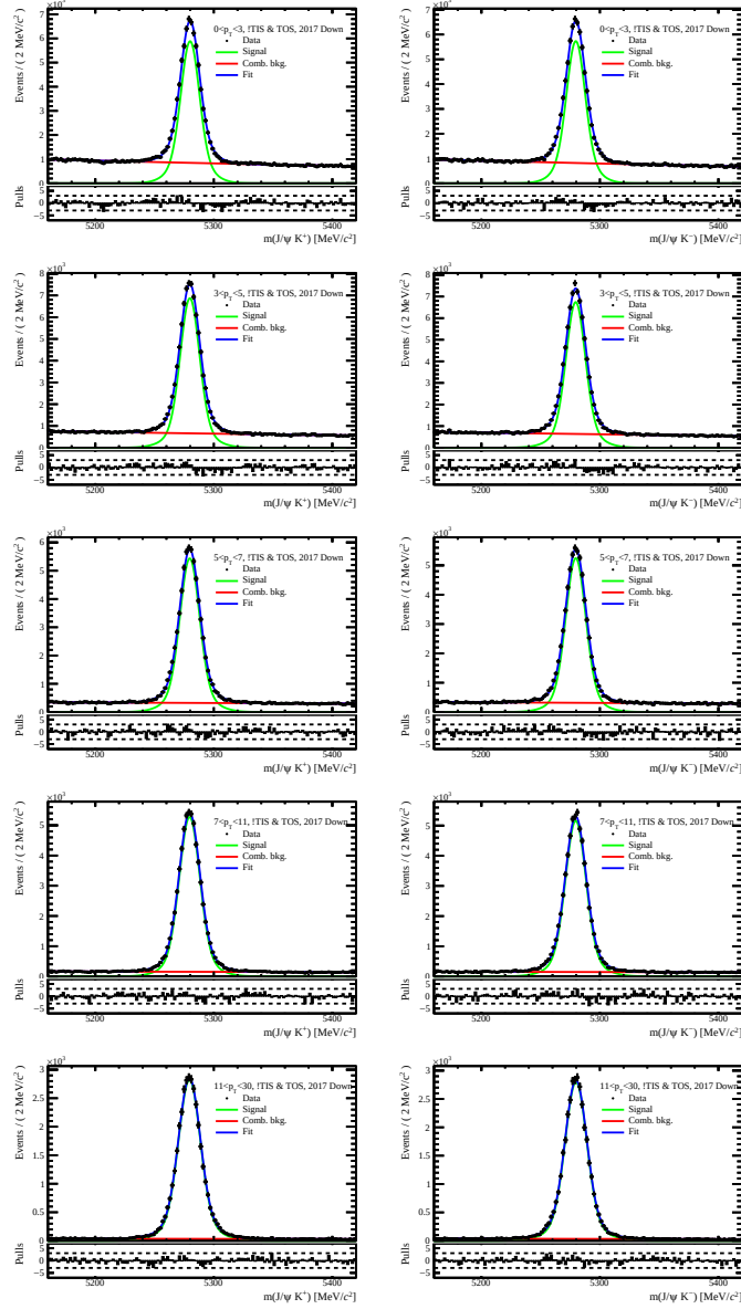
Figure A.22: Fits to the invariant-mass distributions of (left) J/\psi K^+ and (right) J/\psi K^- decays in the trigger category !TIS & TOS, year 2017, and magnet polarity down. The samples are divided in bins of B^+ transverse momentum, from lowest to highest from the top to the bottom.
