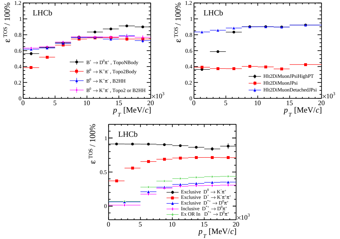
Figure 2.26: Efficiencies of selected HLT2 lines as a function of p_T : beauty lines (top left), J/\psi lines (top right), and charm lines (bottom).
