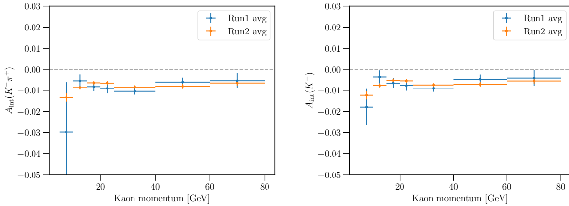
Figure 3.32: Values of the (left) K^-\pi^+ and (right) K^- interaction asymmetries obtained from the Run 1 and Run 2 samples.
