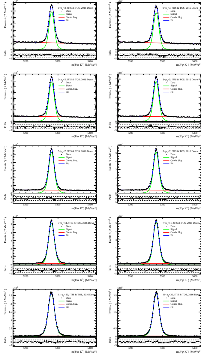
Figure A.20: Fits to the invariant-mass distributions of (left) J/\psi K^+ and (right) J/\psi K^- decays in the trigger category !TIS & TOS, year 2016, and magnet polarity down. The samples are divided in bins of B^+ transverse momentum, from lowest to highest from the top to the bottom.
