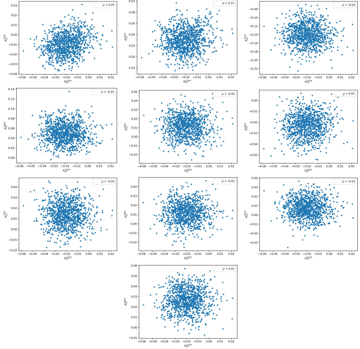
Figure E.2: Scatter plots of the 1000 values of A_{CP}(pK^-) obtained from the pseudoexperiments in the 2011 magnet Down sample and the other subsamples. The correlation coefficient is shown in the upper right corner of each plot.
