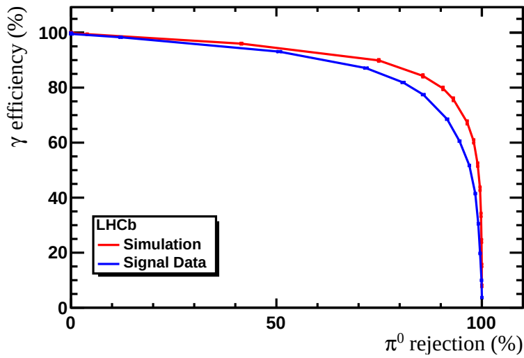
Figure 2.20: Photon identification efficiency as a function of \pi^0 rejection efficiency measured from simulation (red) and data (blue).
