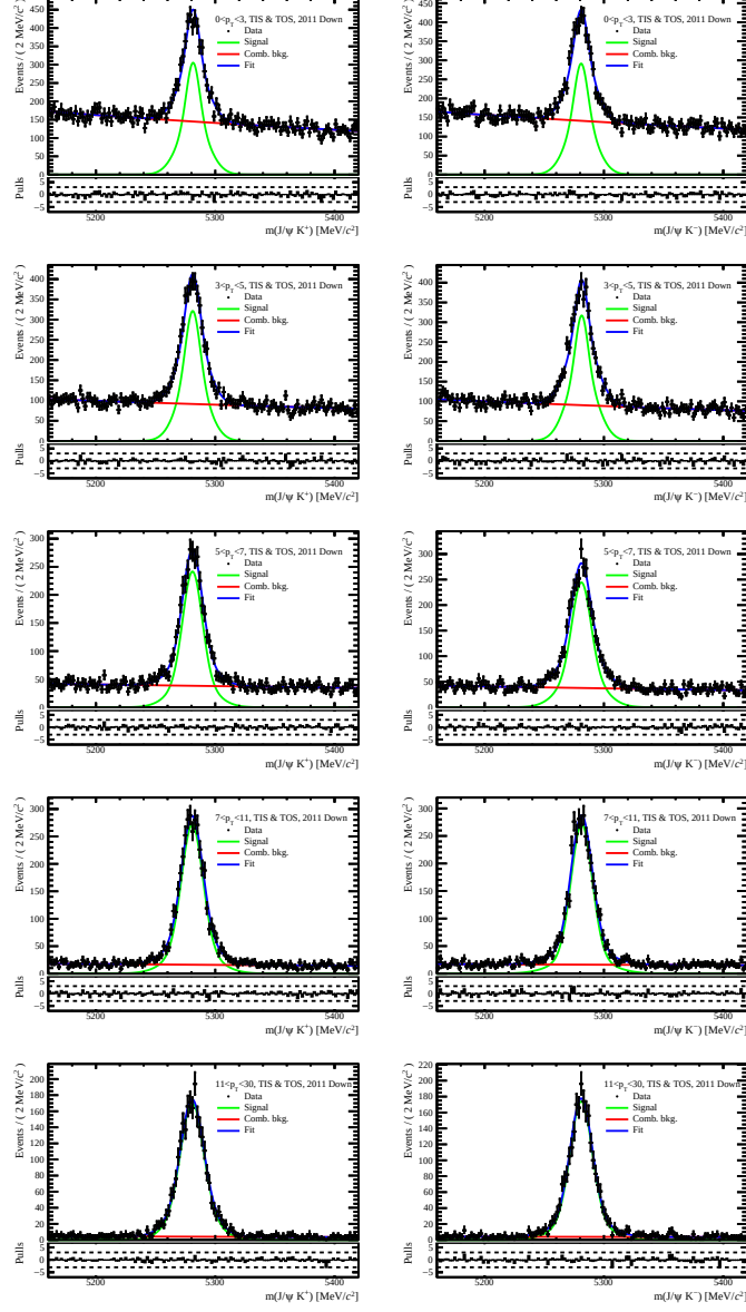
Figure A.2: Fits to the invariant-mass distributions of (left) J/\psi K^+ and (right) J/\psi K^- decays in the trigger category TIS & TOS, year 2011, and magnet polarity down. The samples are divided in bins of B^+ transverse momentum, from lowest to highest from the top to the bottom.
