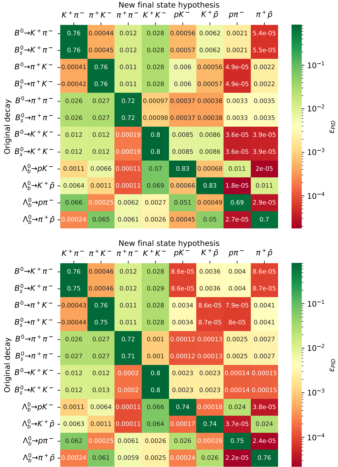
Figure 3.17: PID efficiencies of (mis)identifying a two-body decay (y-axis) as a particular final state (x-axis), computed with the method described in Section 3.3. The top and bottom tables correspond to the optimal values for Selection A and B, respectively, which are reported in Table 3.6.
