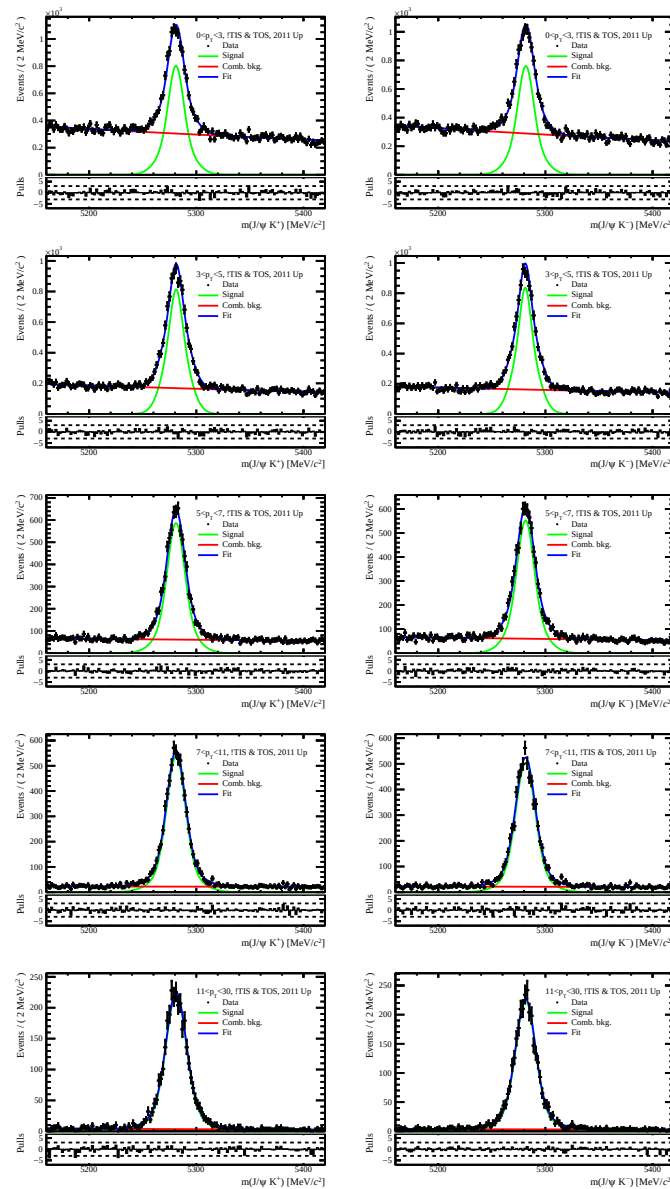
Figure A.13: Fits to the invariant-mass distributions of (left) J/\psi K^+ and (right) J/\psi K^- decays in the trigger category !TIS & TOS, year 2011, and magnet polarity up. The samples are divided in bins of B^+ transverse momentum, from lowest to highest from the top to the bottom.
