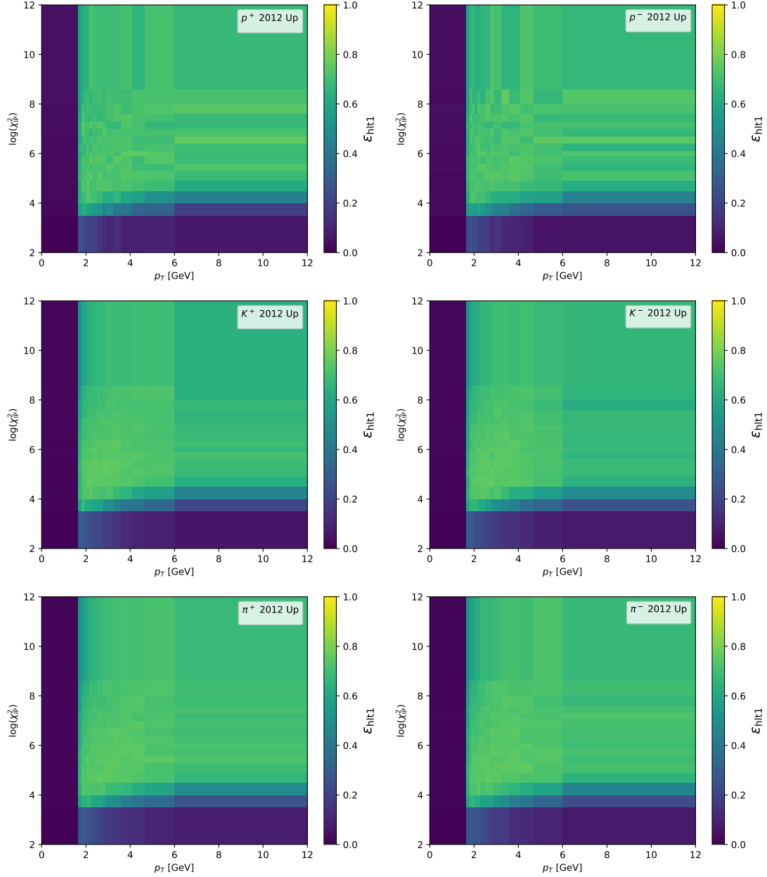
Figure C.3: HLT1_TrackMVA efficiency as a function of p_T and \log(\chi_{\text{IP}}^2) for (top row) protons, (middle row) kaons, and (bottom row) pions of (left) positive and (right) negative charge. These are the plots for the 2012 magnet Up sample.
