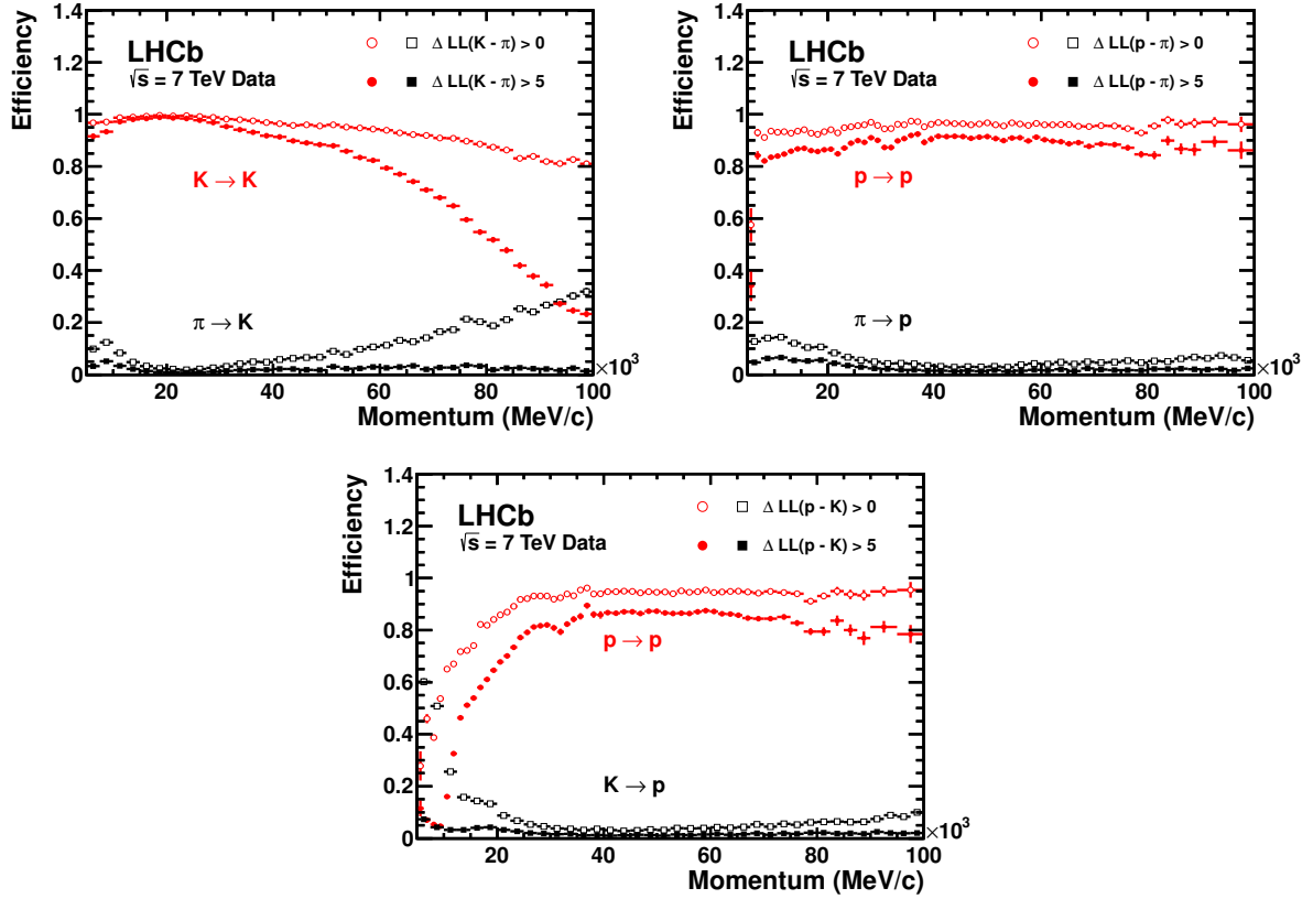
Figure 2.17: Efficiencies of correctly and incorrectly identifying hadrons from the RICH detectors while requiring different values of the DLL variables (described in the text). Top left: K identification and \pi - K misidentification. Top right: p identification and \pi - p misidentification. Bottom: p identification and K - p misidentification.
