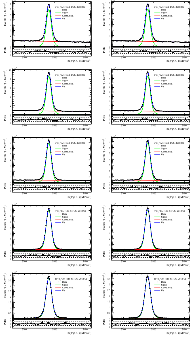
Figure A.23: Fits to the invariant-mass distributions of (left) J/\psi K^+ and (right) J/\psi K^- decays in the trigger category !TIS & TOS , year 2018, and magnet polarity up. The samples are divided in bins of B^+ transverse momentum, from lowest to highest from the top to the bottom.
