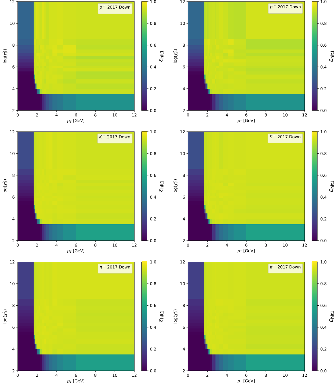
Figure C.10: Hlt1_TrackMVA efficiency as a function of p_T and \log(\chi_{IP}^2) for (top row) protons, (middle row) kaons, and (bottom row) pions of (left) positive and (right) negative charge. These are the plots for the 2017 magnet Down sample.
