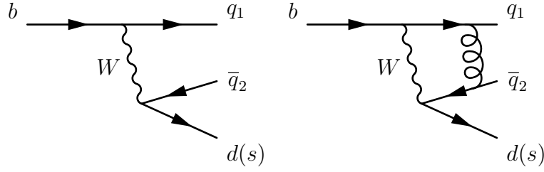
Figure 1.4: Example of Feynman diagrams for a b \rightarrow q_1 \bar{q}_2 d(s) transition at tree-level (left) and with a first-order QCD correction (right).
