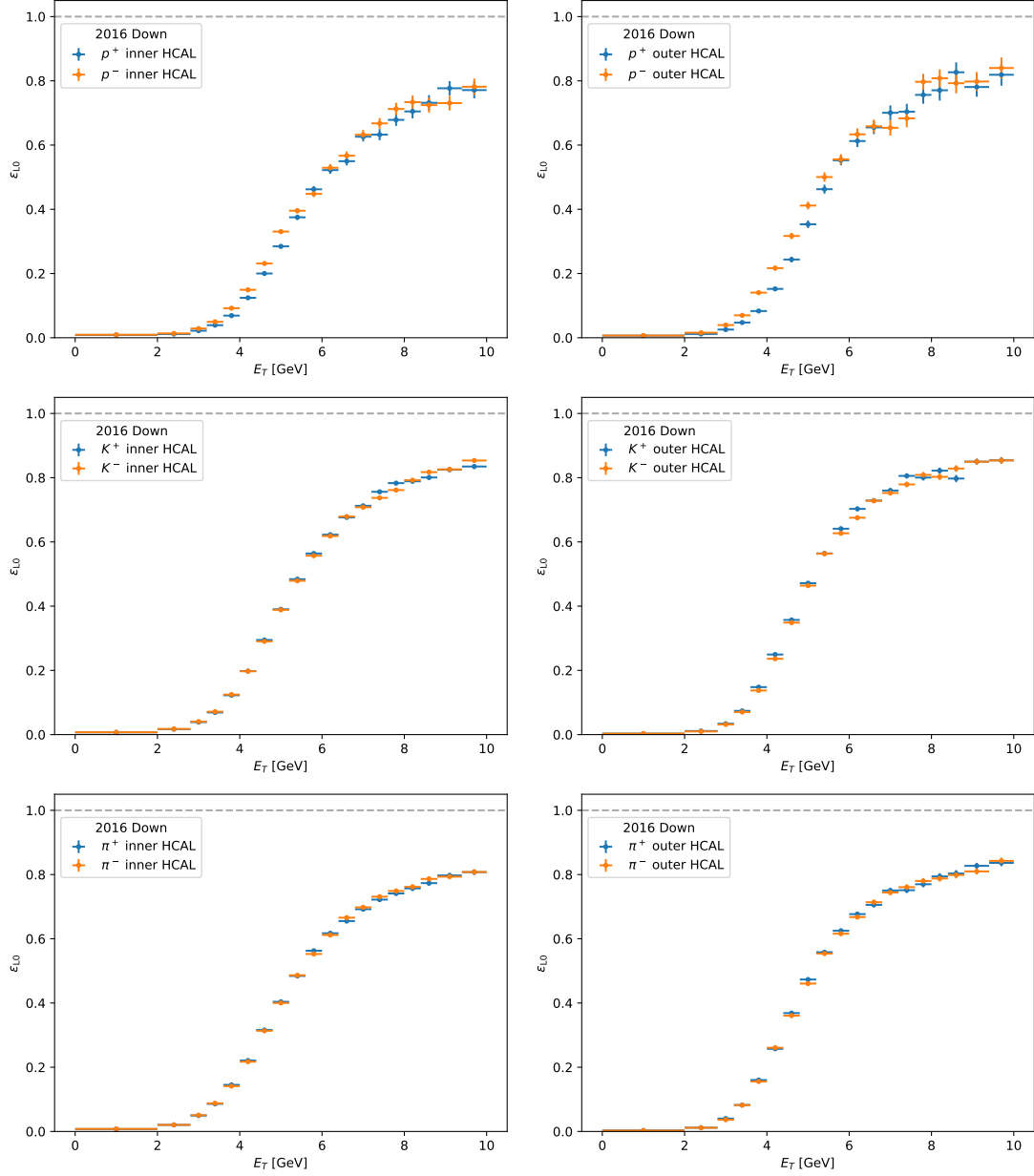
Figure B.8: L0_Hadron efficiency as a function of E_T for (top row) protons, (middle row) kaons, and (bottom row) pions hitting the (left) inner and (right) outer region of HCAL. These are the plots for the 2016 magnet Down sample.
