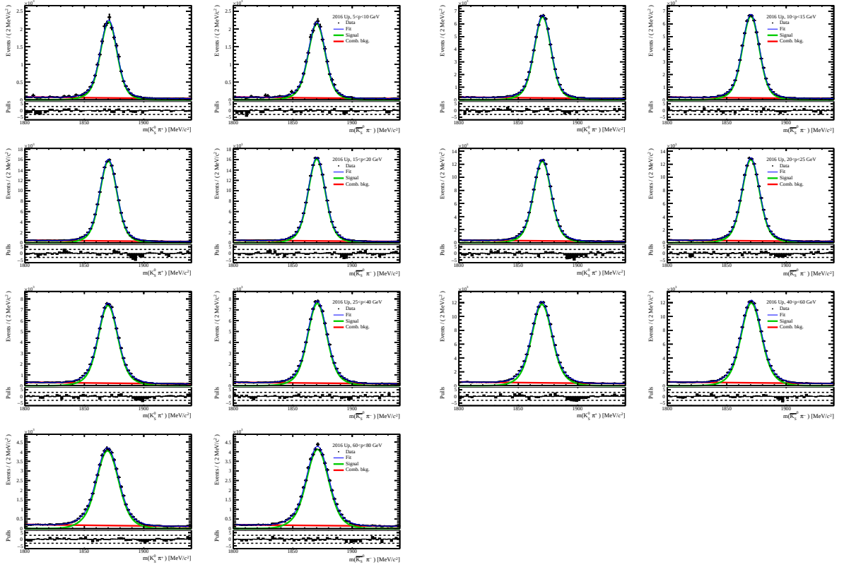
Figure 69: Fits to the invariant-mass distributions of (left of the pair) K_S^0\pi^+ and (right of the pair) \bar{K}_S^0\pi^- decays in the year 2016 and magnet polarity up sample. The samples are divided in bins of kaon momentum, from lowest to highest from the top to the bottom and from left to right.
