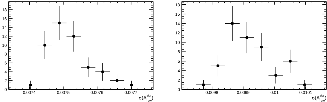
Figure 3.18: Histograms of the 50 asymmetry errors obtained from the toys for (left) Selection A and (right) Selection B with the optimal cuts.
