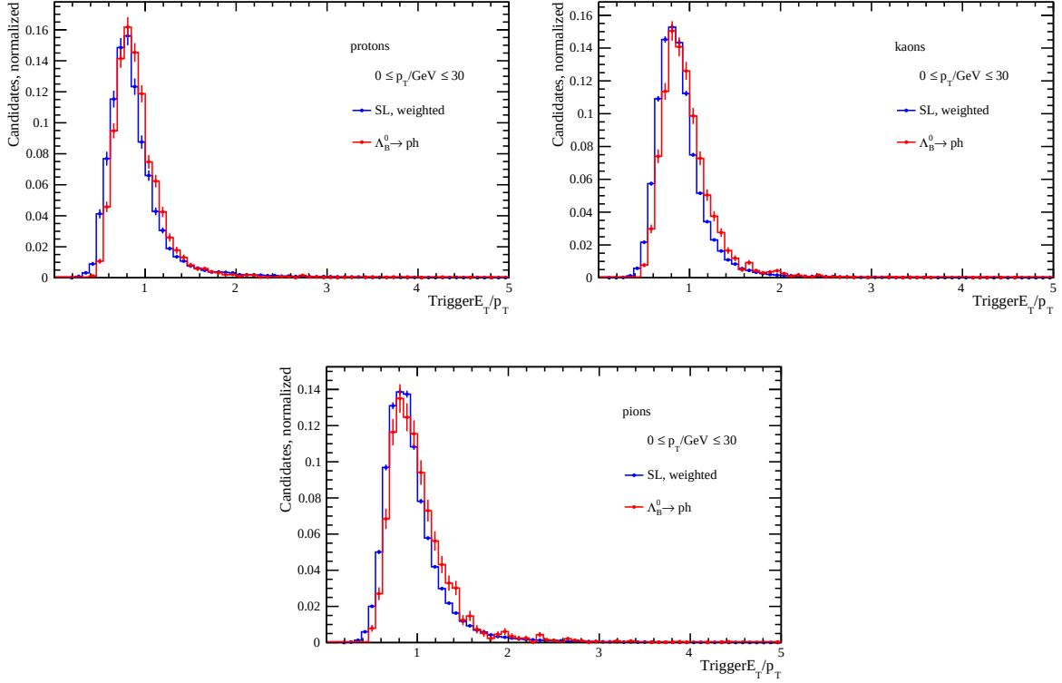
Figure 3.39: Plot of E_T/p_T for (top left) protons, (top right) kaons, and (bottom) pions in the inner HCAL region and for 0 < p_T < 30 GeV/c. The blue line corresponds to the reweighted semileptonic samples, while the red line to background-subtracted \Lambda_b^0 \rightarrow ph^- decays.
