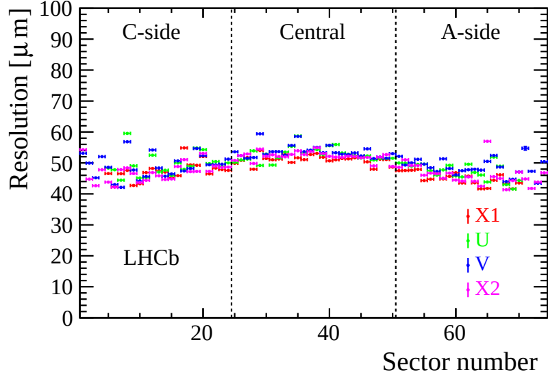
Figure 2.8: Hit resolution of the TT measured with 2012 data. The resolution of the four layers x-u-v-x is shown separately. The “Sector number” label on the horizontal axis approximately corresponds to the x direction.
