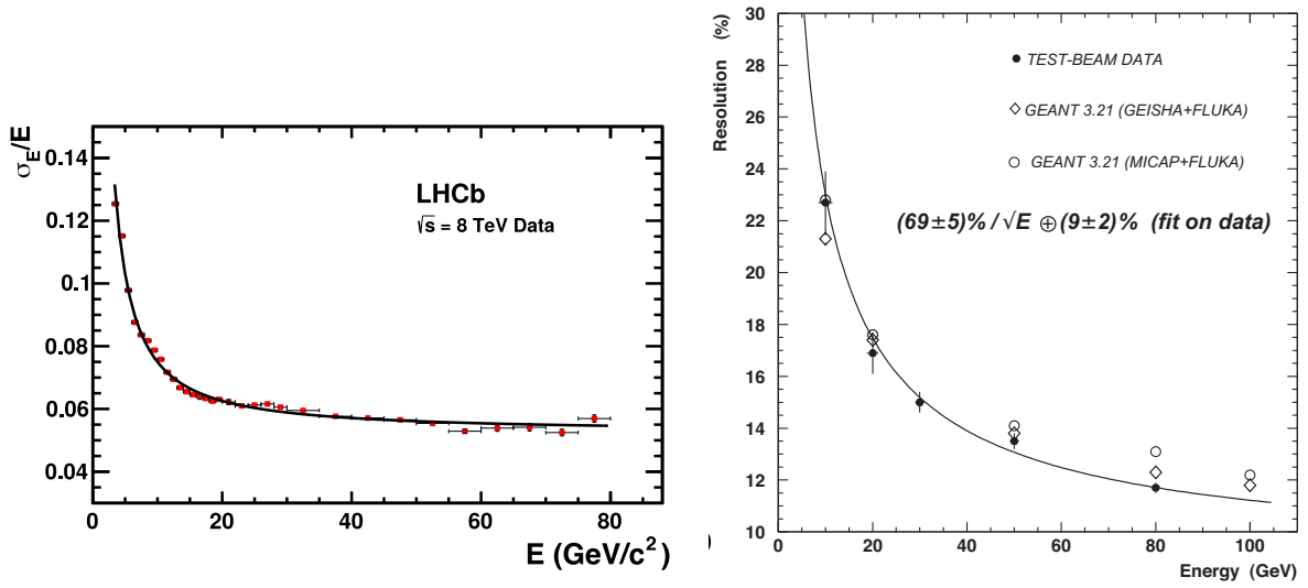
Figure 2.19: Energy resolution of (left) ECAL and (right) HCAL.
