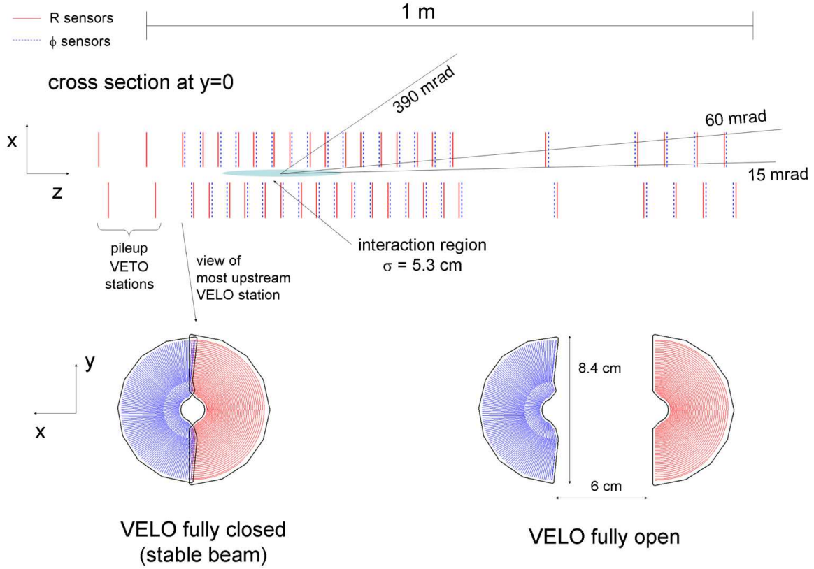
Figure 2.6: Cross-section in the (x, z) plane of the VELO silicon sensors, at y = 0 , with the detector in the fully closed position. The front face of the first modules is illustrated in both the closed and open positions. The two pile-up veto stations are located upstream of the VELO sensors.
