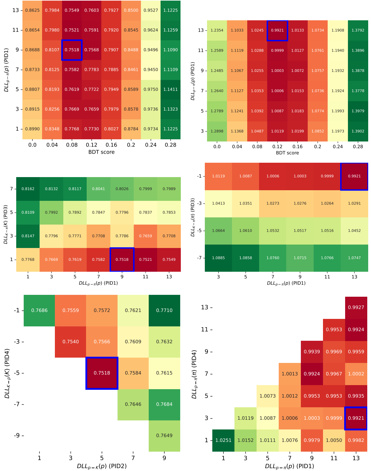
Figure 3.19: Plots showing the predicted uncertainty on (left) A_{\text{raw}}(pK^-) and (right) A_{\text{raw}}(p\pi^-) as a function of different combinations of BDT and PID requirements. The highlighted square indicates the optimal value found in the optimization.
