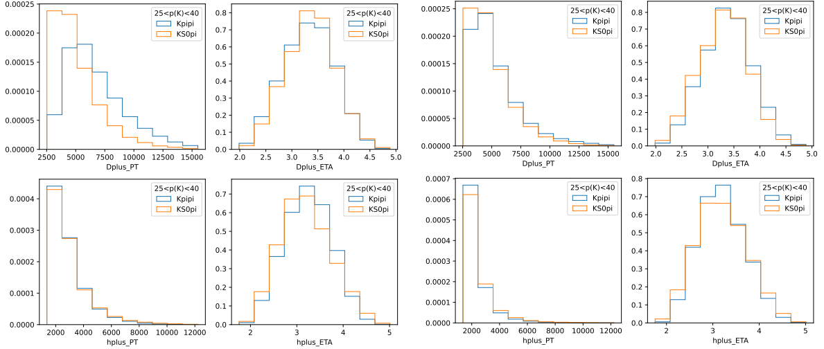
Figure 3.31: Kinematic distributions of the D^+ \rightarrow K^-\pi^+\pi^+ and D^+ \rightarrow K_S^0\pi^+ samples before (left) and after (right) the kinematic reweighting. The plots correspond to the fifth momentum bin ( 25 < p < 40 GeV/ c^2 ) of the 2018, magnet down sample.
