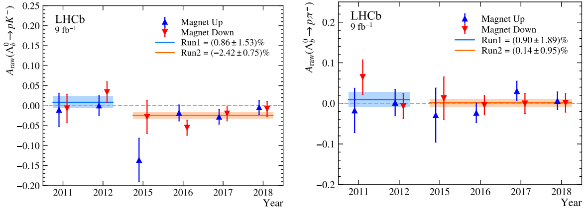
Figure 3.24: Values of the raw asymmetries of (left) \Lambda_b^0 \rightarrow pK^- and (right) \Lambda_b^0 \rightarrow p\pi^- decays, divided by year and magnet polarity.
