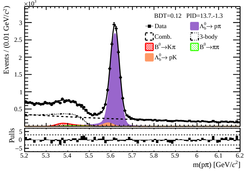
Figure 3.16: p\pi invariant-mass spectrum fitted with the model defined in Section 3.4 and selected requiring DLL_{p\pi}(p) > 13 , DLL_{pK}(p) > 7 , DLL_{K\pi}(\pi) < -1 , DLL_{p\pi}(\pi) < 3 and BDT > 0.12 . The results of the binned maximum-likelihood fit are superimposed.
