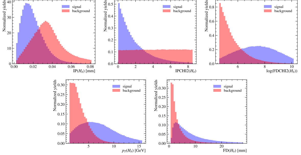
Figure 3.11: Distribution of part of the variables used in the BDT training for (blue) signal and (red) background events. The dataset corresponds to a particular set of PID cuts for Selection A.
