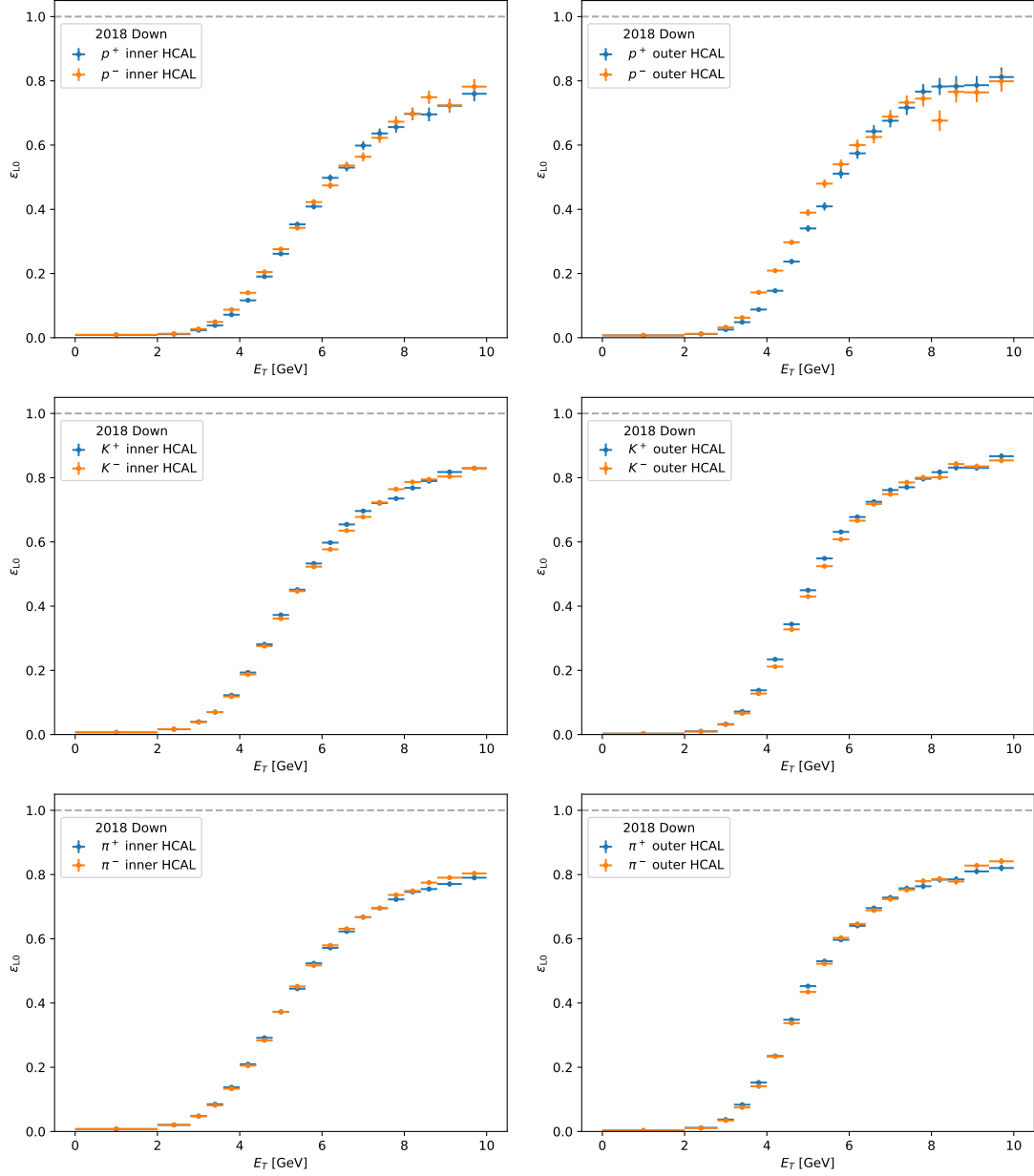
Figure B.12: L0_Hadron efficiency as a function of E_T for (top row) protons, (middle row) kaons, and (bottom row) pions hitting the (left) inner and (right) outer region of HCAL. These are the plots for the 2018 magnet Down sample.
