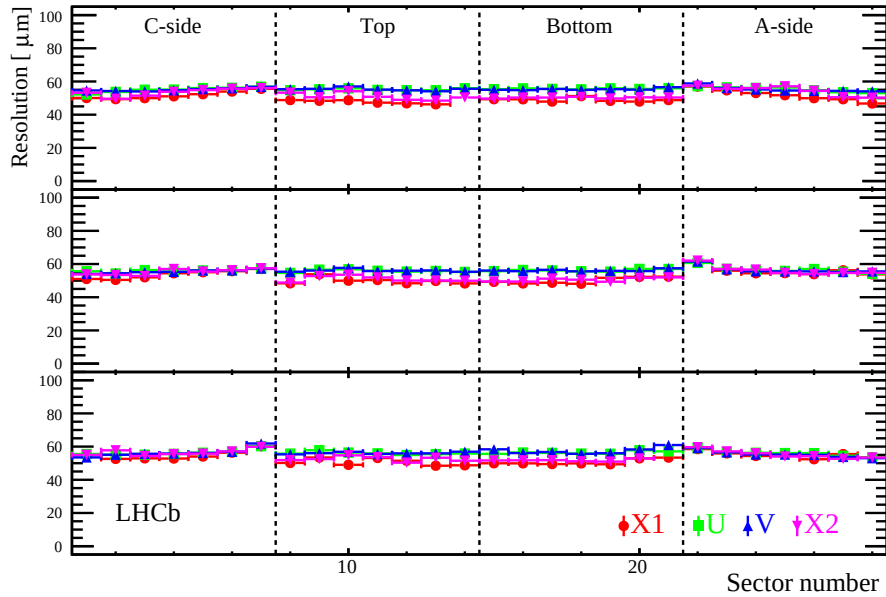
Figure 2.10: Hit resolution in the four modules of IT1 (bottom), IT2 (middle), and IT3 (top). The resolution is shown separately for each of the four x - u - v - x layers. The “Sector number” label approximately corresponds to the x direction.
