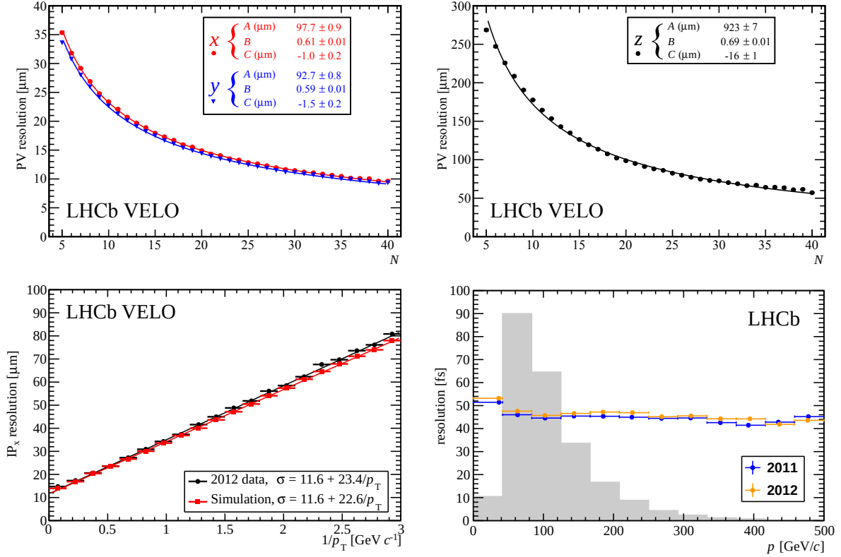
Figure 2.5: Summary of the performance of the VELO: x , y , and z PV position resolution versus track multiplicity (top), IP resolution versus 1/p_T (bottom left), decay time resolution versus momentum (bottom right).
