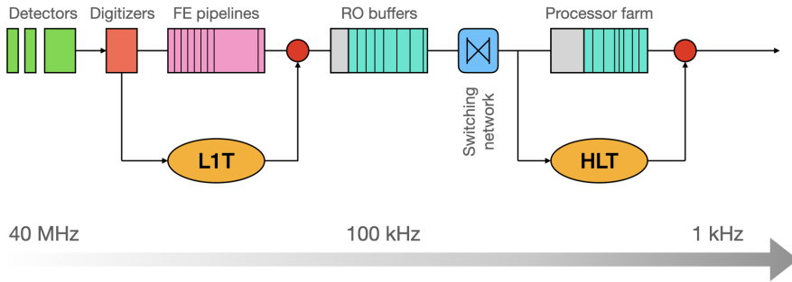
Figure 2: Schematic representation of the CMS Phase-1 trigger system.
