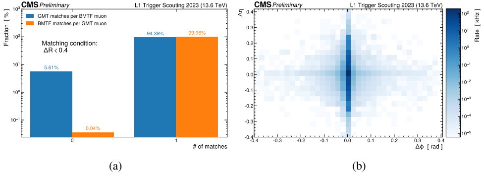
Figure 11: Left: matching fractions per BMTF candidate (blue) and GMT muon (orange). Right: Differences in \eta and \phi between matched objects.
