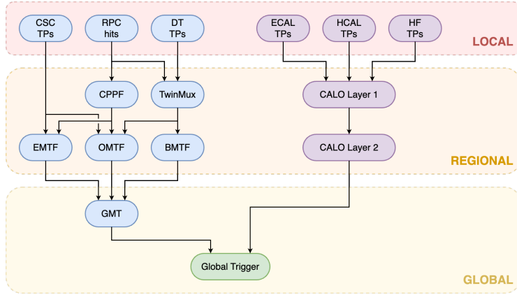
Figure 3: Schematic representation of the Phase-1 Level-1 trigger of CMS. CSC: Cathode Strip Chambers; RPC: Resistive Plate Chambers; DT: Drift Tubes; HF: Hadronic Calorimeter-Forward; ECAL: Electromagnetic Calorimeter; HCAL: Hadronic Calorimeter; TPs: Trigger Primitives; CPPF: Concentration, Pre-processing and Fan-out system; EMTF: Endcap Muon Track Finder; OMTF: Overlap Muon Track Finder; BMTF: Barrel Muon Track Finder; GMT: Global Muon Trigger.
