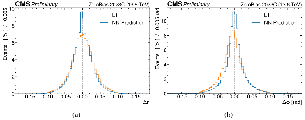
Figure 14: Left: \eta residuals, relative to offline reconstruction, of the neural network prediction (blue) and the BMTF assignment (orange). Right: \phi residuals, relative to offline reconstruction, of the neural network prediction (blue) and the BMTF assignment (orange).
