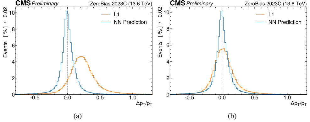
Figure 13: Transverse momentum resolution, relative to offline reconstruction, of the neural network prediction (blue) and the BMTF assignment (orange). The right figure shows the p_T resolution using a re-calibrated BMTF candidate transverse momentum.
