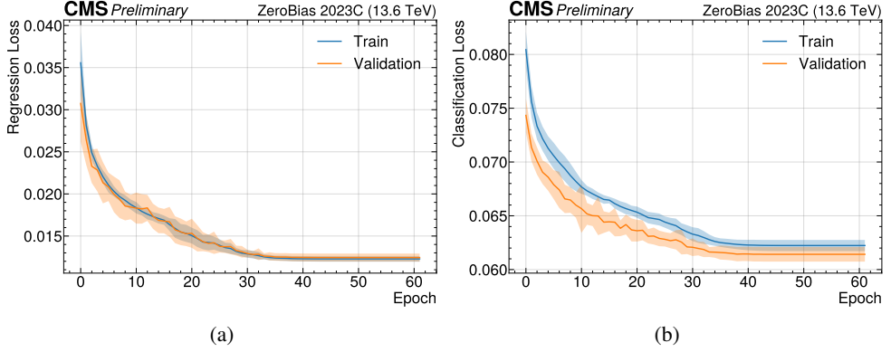
Figure 12: Left: regression loss function per epoch, averaged over 50 iterations, during training (blue) and validation (orange). Right: classification loss function per epoch, averaged over 50 iterations, during training (blue) and validation (orange).
