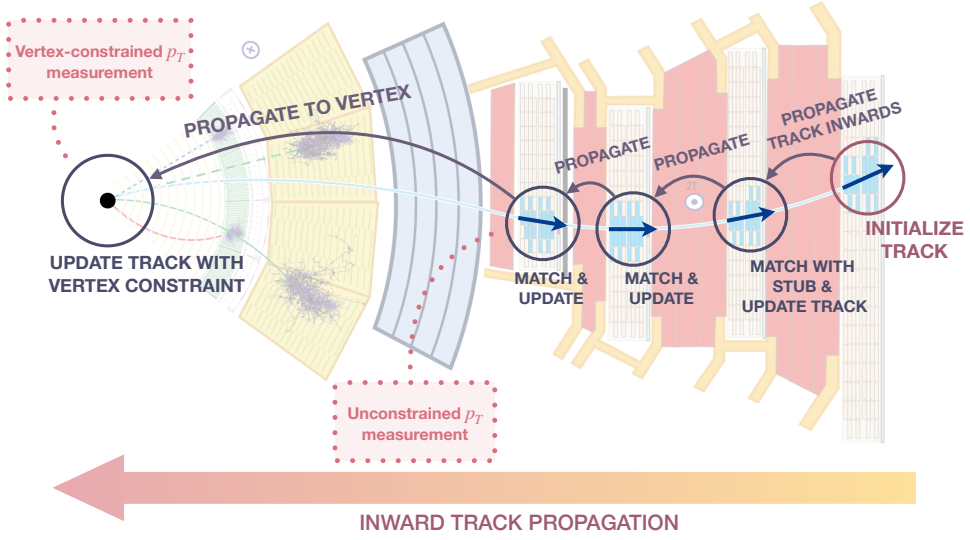
Figure 8: Visualization of the Kalman filter procedure applied to muon track reconstruction.
