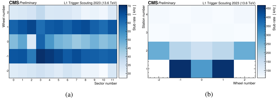
Figure 6: Stub collection rate for each wheel, sector and station, presented as heatmaps.
