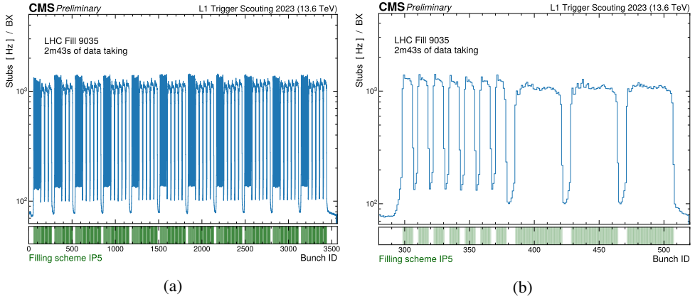
Figure 5: Stub collection rate per bunch crossing relative to the bunch crossing identifier, showing the LHC filling scheme structure. The bottom panel shows, in green, the nominal LHC filling scheme at interaction point five, identified by the string 25ns_2464b_2452_1842_1821_236bpi_12inj_hybrid.
