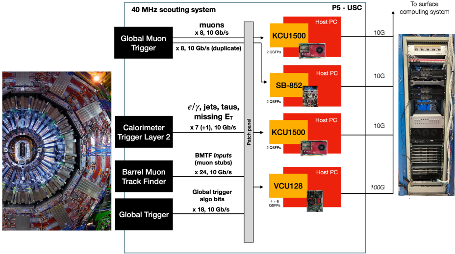
Figure 4: The L1 data scouting system demonstrator at the LHC Run-3 [31].
