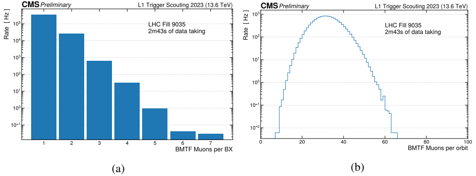
Figure 10: BMTF candidates multiplicity per bunch crossing (left) and orbit (right).
