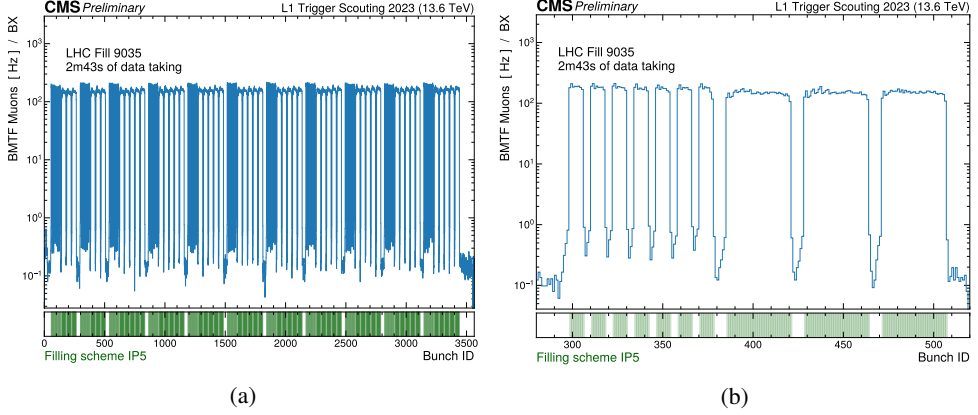
Figure 9: BMTF candidates rate per bunch crossing relative to the bunch crossing identifier, showing the LHC filling scheme structure.
