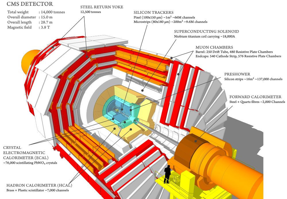
Figure 1: Illustrative depiction of the CMS detector showcasing its diverse subdetectors [26].
