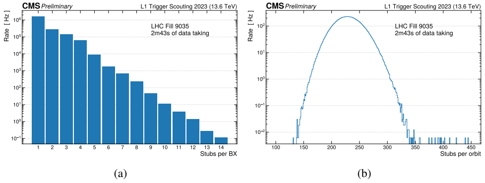
Figure 7: Stub multiplicity per bunch crossing (left) and orbit (right).
